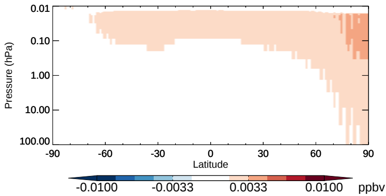
v11-02b-HP - v11-02a BrO - Strat zonal mean abs diff for Apr
