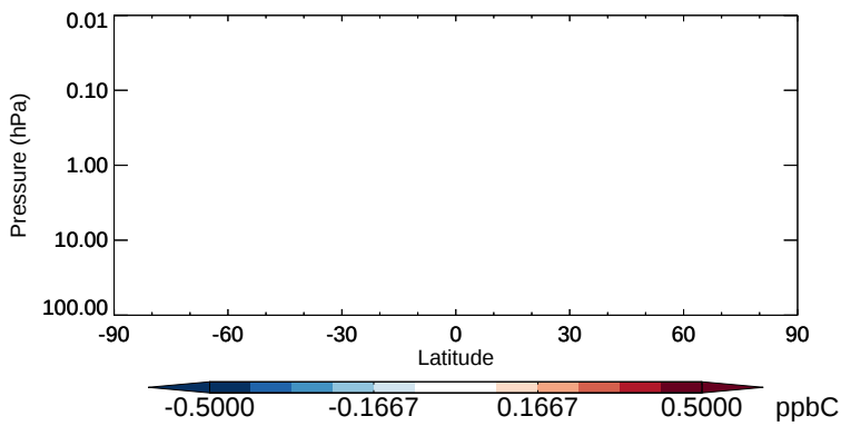
v11-02b-HP - v11-02a ALD2 - Strat zonal mean abs diff for Apr
