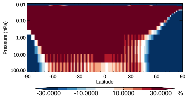
v11-02b-HP / v11-02a ALK4 - Strat zonal mean % diff for Apr
