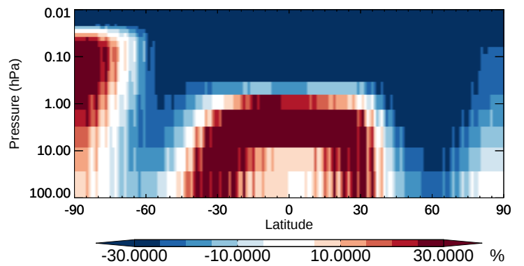
v11-02b-HP / v11-02a ISOG1 - Strat zonal mean % diff for Apr
