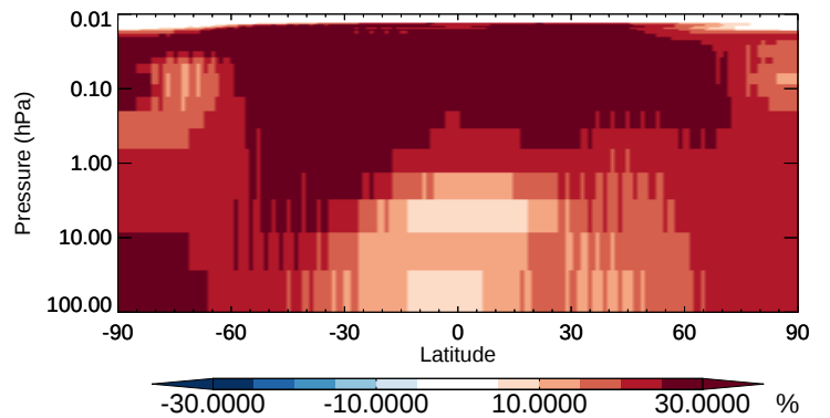
v11-02b-HP / v11-02a HBr - Strat zonal mean % diff for Apr
