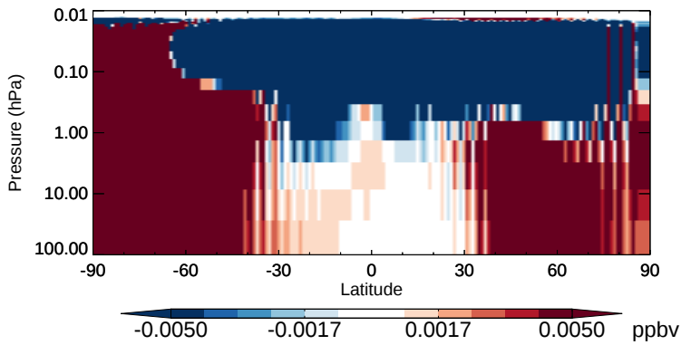
v11-02b-HP - v11-02a N2O5 - Strat zonal mean abs diff for Apr
