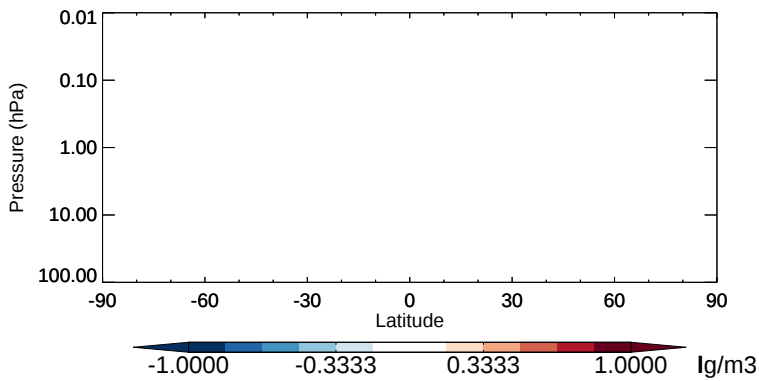
v11-02b-HP - v11-02a NITs - Strat zonal mean abs diff for Apr
