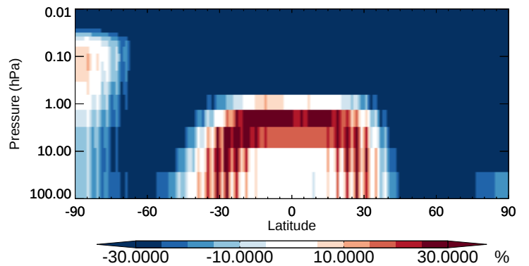
v11-02b-HP / v11-02a TSOG1 - Strat zonal mean % diff for Apr
