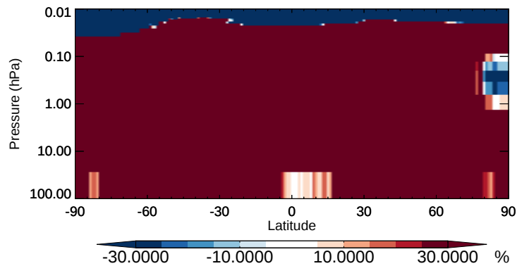
v11-02b-HP / v11-02a TOLU - Strat zonal mean % diff for Apr
