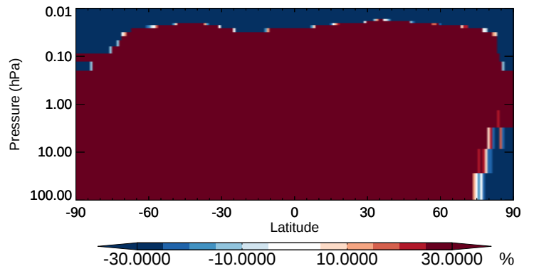
v11-02b-HP / v11-02a OCPO - Strat zonal mean % diff for Apr
