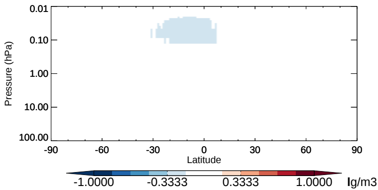
v11-02b-HP - v11-02a SO4 - Strat zonal mean abs diff for Apr
