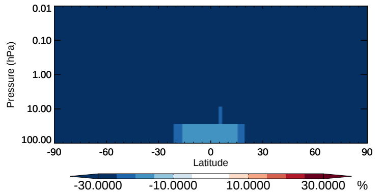
v11-02b-HP / v11-02a TSOA1 - Strat zonal mean % diff for Apr
