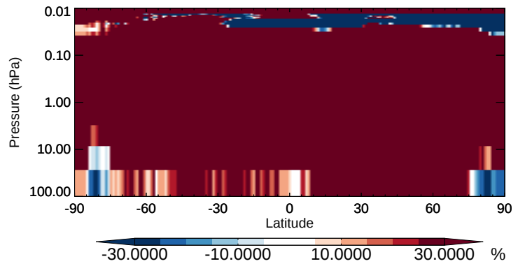
v11-02b-HP / v11-02a MVKN - Strat zonal mean % diff for Apr
