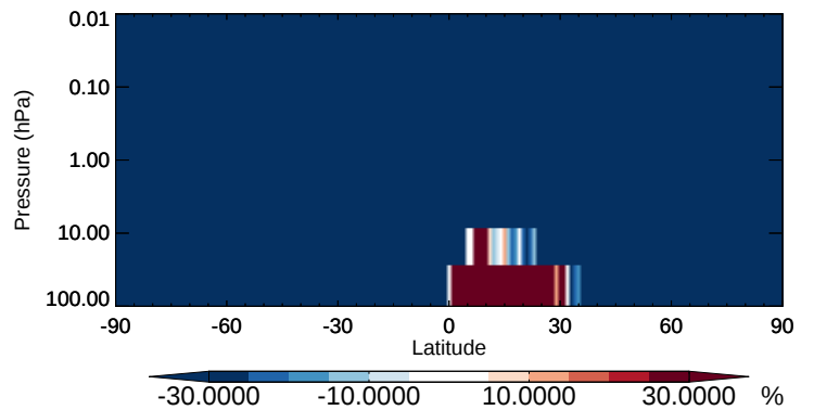
v11-02b-HP / v11-02a NH 3 - Strat zonal mean % diff for Apr
