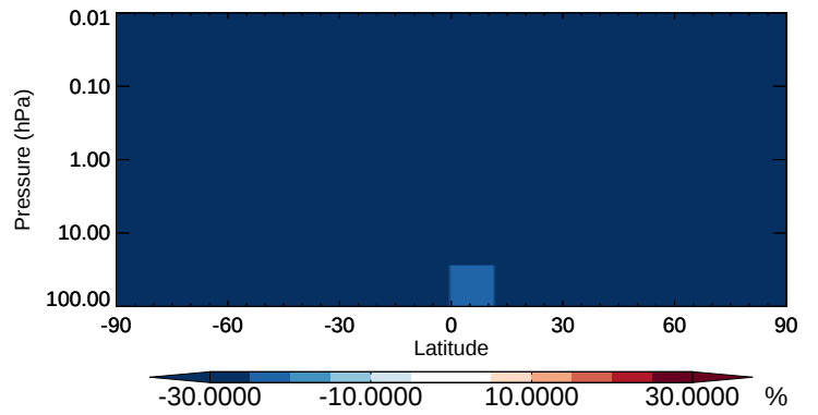
v11-02b-HP / v11-02a BCPI - Strat zonal mean % diff for Apr
