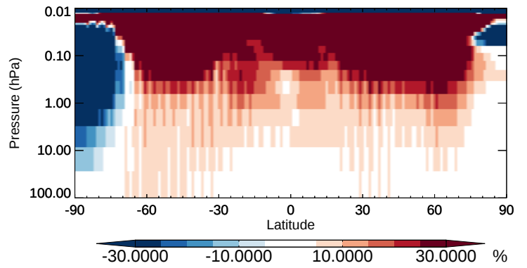
v11-02b-HP / v11-02a H2402 - Strat zonal mean % diff for Apr
