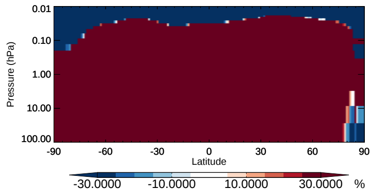
v11-02b-HP / v11-02a BCPO - Strat zonal mean % diff for Apr
