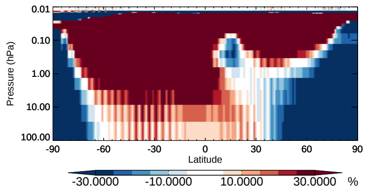
v11-02b-HP / v11-02a R4N2 - Strat zonal mean % diff for Apr
