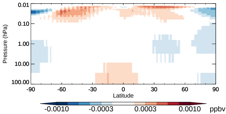
v11-02b-HP - v11-02a PPN - Strat zonal mean abs diff for Apr
