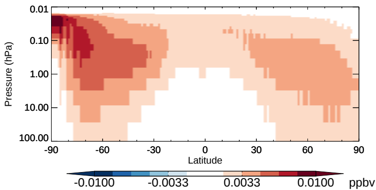
v11-02b-HP - v11-02a BrNO 3 - Strat zonal mean abs diff for Apr
