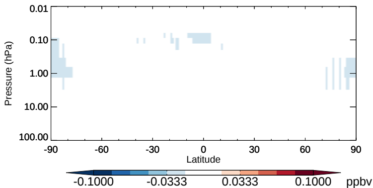
v11-02b-HP - v11-02a MPN - Strat zonal mean abs diff for Apr
