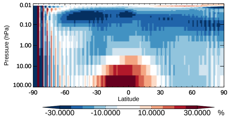
v11-02b-HP / v11-02a NO - Strat zonal mean % diff for Apr
