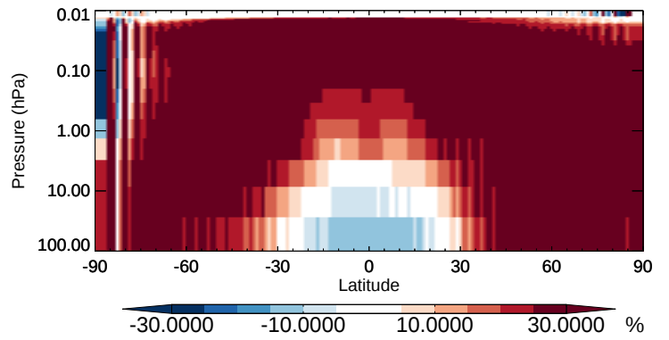
v11-02b-HP / v11-02a BrO - Strat zonal mean % diff for Apr
