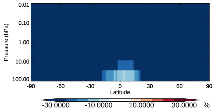
v11-02b-HP / v11-02a ASOA2 - Strat zonal mean % diff for Apr
