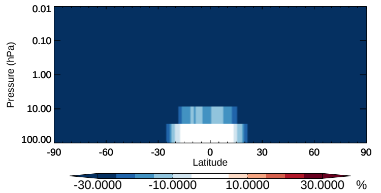
v11-02b-HP / v11-02a ISOA2 - Strat zonal mean % diff for Apr
