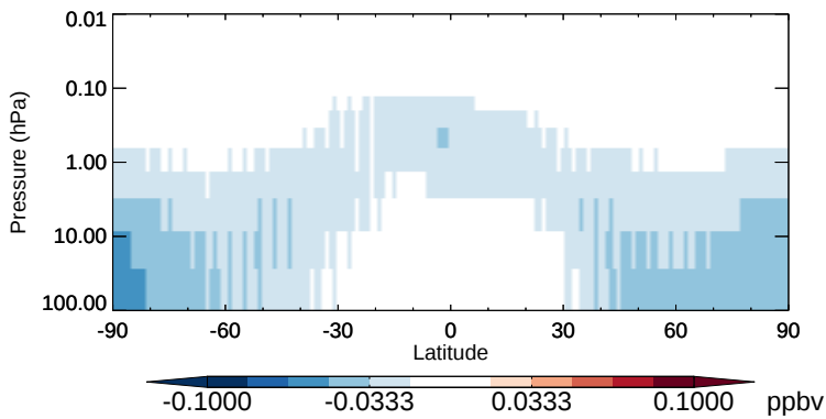
v11-02b-HP - v11-02a EOH - Strat zonal mean abs diff for Apr
