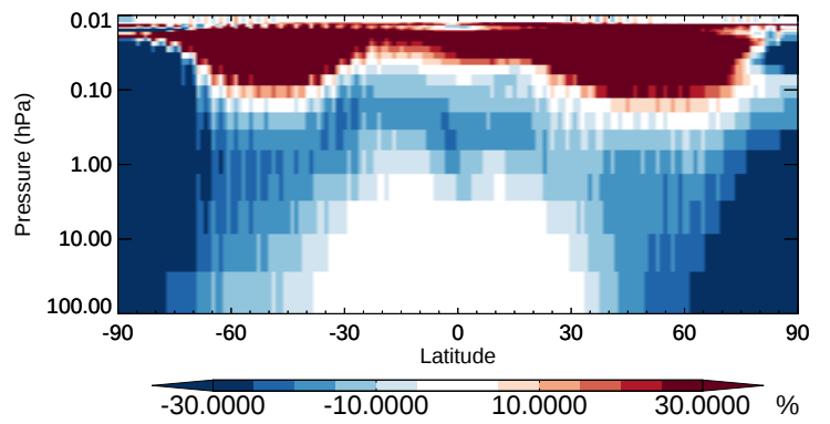
v11-02b-HP / v11-02a ALD2 - Strat zonal mean % diff for Apr
