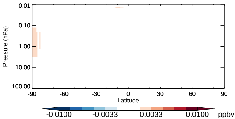
v11-02b-HP - v11-02a HOBr - Strat zonal mean abs diff for Apr
