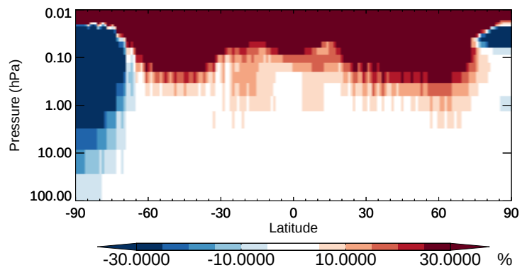
v11-02b-HP / v11-02a CH 3 Br - Strat zonal mean % diff for Apr
