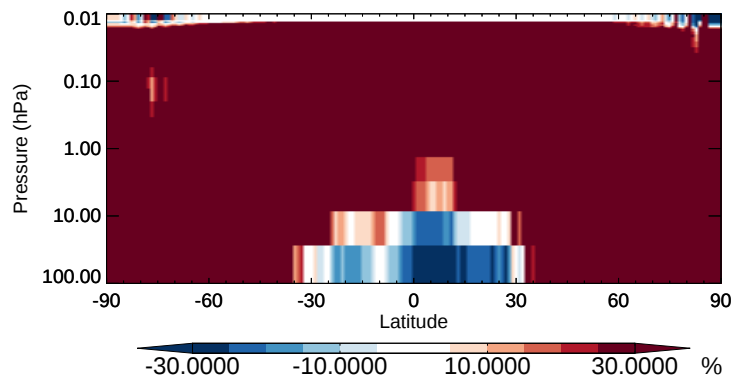
v11-02b-HP / v11-02a Br2 - Strat zonal mean % diff for Apr
