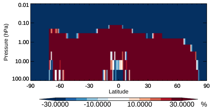
v11-02b-HP / v11-02a RIP - Strat zonal mean % diff for Apr
