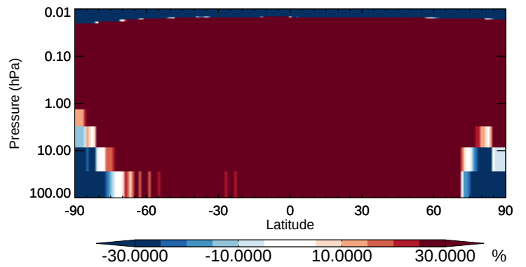
v11-02b-HP / v11-02a DST2 - Strat zonal mean % diff for Apr
