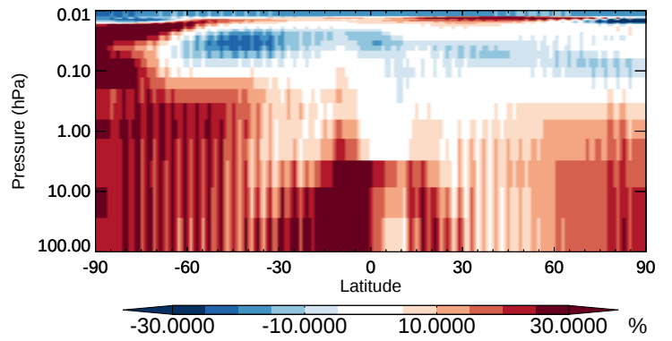
v11-02b-HP / v11-02a BrNO 2 - Strat zonal mean % diff for Apr
