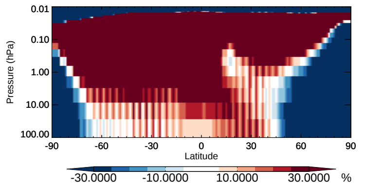
v11-02b-HP / v11-02a BENZ - Strat zonal mean % diff for Apr
