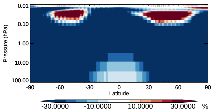
v11-02b-HP / v11-02a MGLY - Strat zonal mean % diff for Apr
