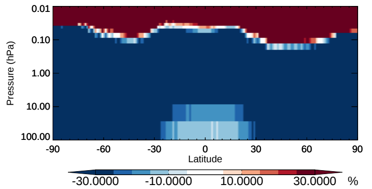
v11-02b-HP / v11-02a SALA - Strat zonal mean % diff for Apr
