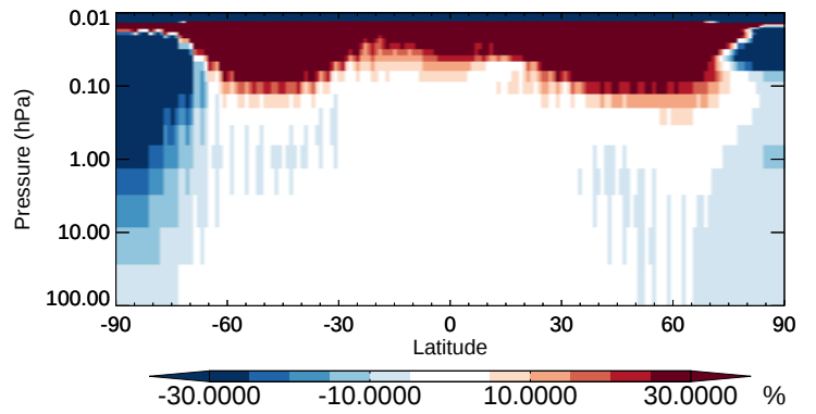
v11-02b-HP / v11-02a OCS - Strat zonal mean % diff for Apr
