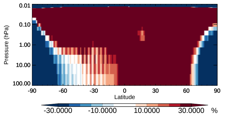
v11-02b-HP / v11-02a DST1 - Strat zonal mean % diff for Apr
