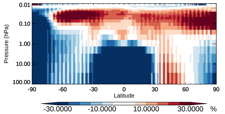
v11-02b-HP / v11-02a HOCl - Strat zonal mean % diff for Apr
