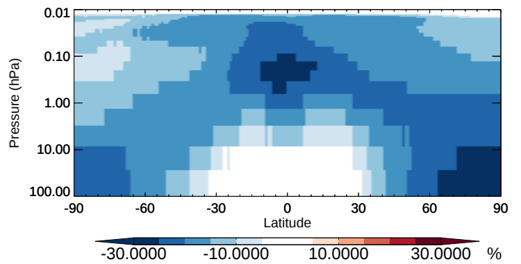
v11-02b-HP / v11-02a H 2 O - Strat zonal mean % diff for Apr
