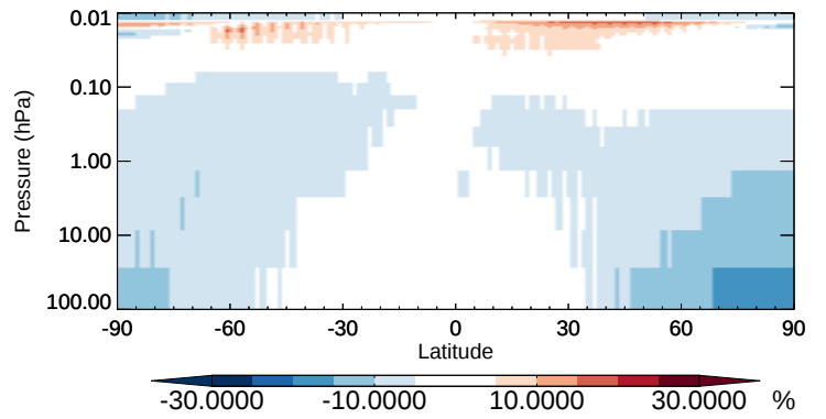
v11-02b-HP / v11-02a CO - Strat zonal mean % diff for Apr
