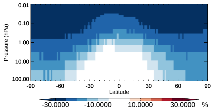
v11-02b-HP / v11-02a MSA - Strat zonal mean % diff for Apr
