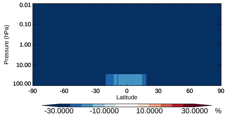
v11-02b-HP / v11-02a TSOA0 - Strat zonal mean % diff for Apr
