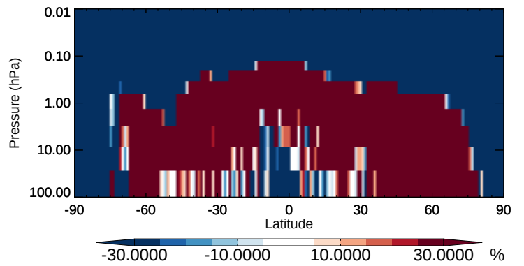
v11-02b-HP / v11-02a ISOP - Strat zonal mean % diff for Apr
