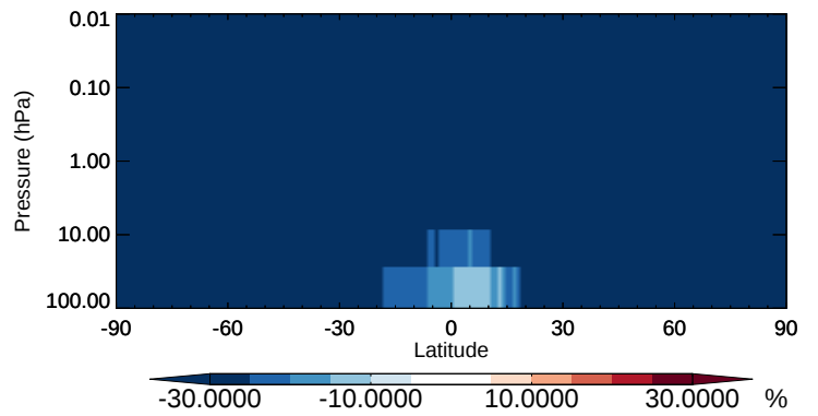
v11-02b-HP / v11-02a TSOA3 - Strat zonal mean % diff for Apr
