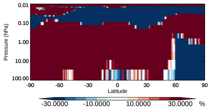
v11-02b-HP / v11-02a MACRN - Strat zonal mean % diff for Apr
