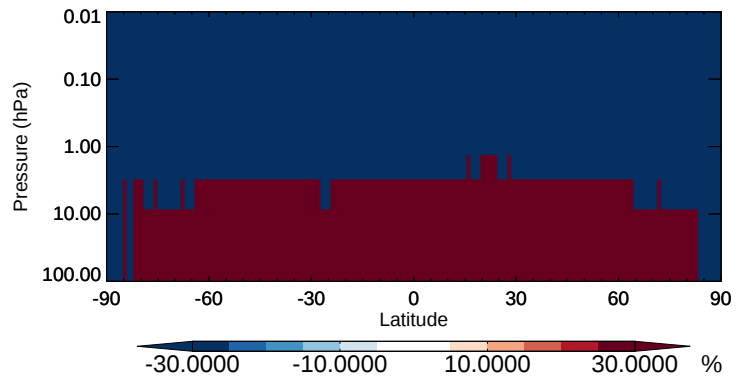
v11-02b-HP / v11-02a SO 4 s - Strat zonal mean % diff for Apr
