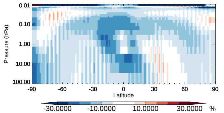
v11-02b-HP / v11-02a HNO4 - Strat zonal mean % diff for Apr
