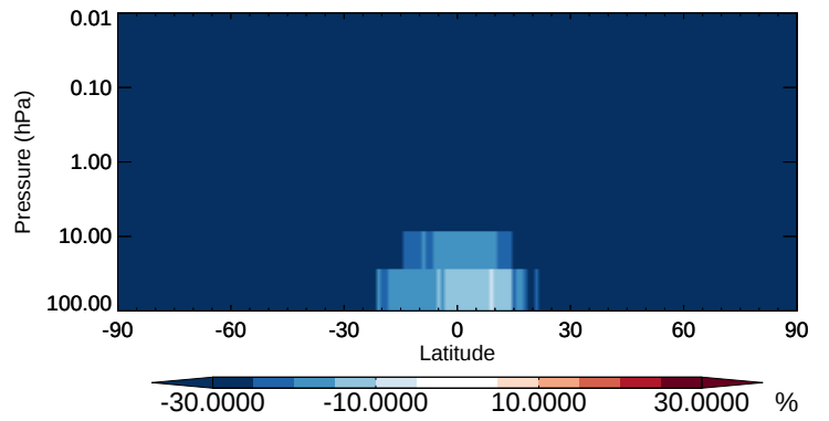
v11-02b-HP / v11-02a ISOA3 - Strat zonal mean % diff for Apr
