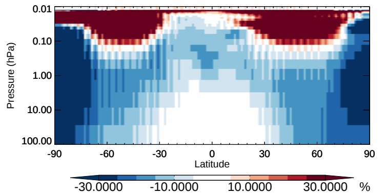
v11-02b-HP / v11-02a EOH - Strat zonal mean % diff for Apr
