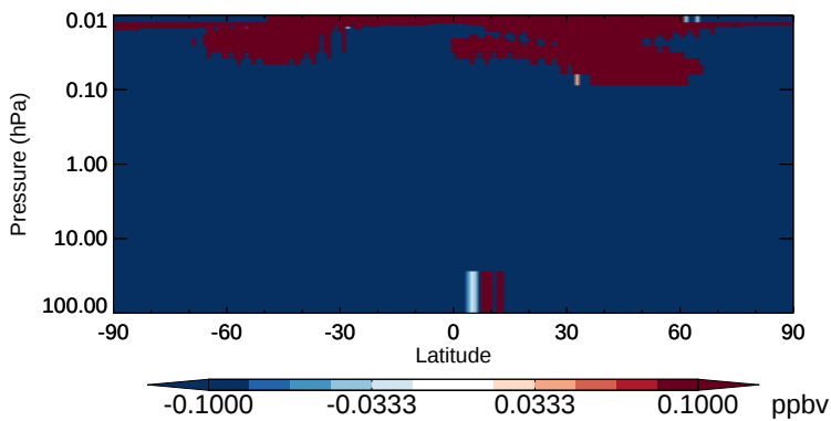
v11-02b-HP - v11-02a CH4 - Strat zonal mean abs diff for Apr
