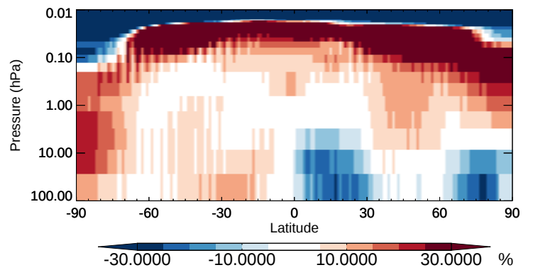
v11-02b-HP / v11-02a SO2 - Strat zonal mean % diff for Apr
