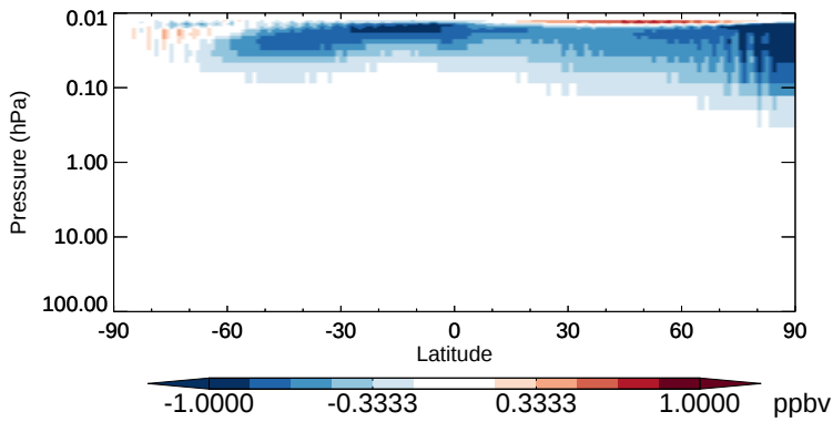
v11-02b-HP - v11-02a NO - Strat zonal mean abs diff for Apr
