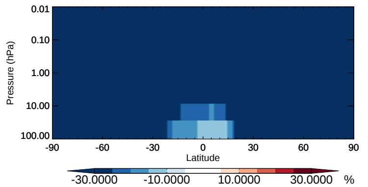
v11-02b-HP / v11-02a TSOA2 - Strat zonal mean % diff for Apr
