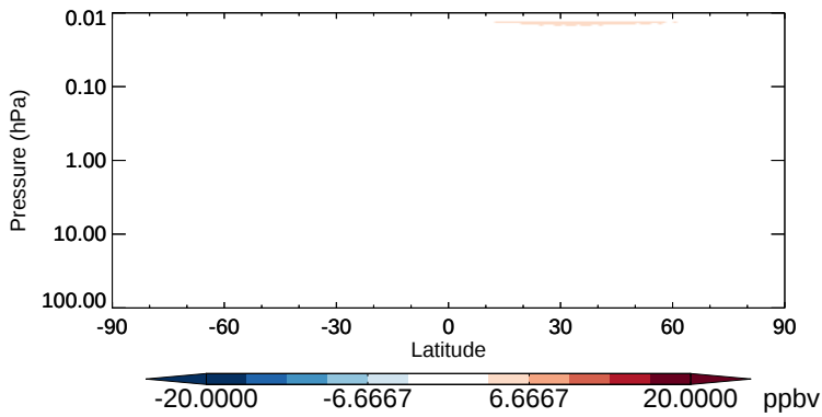
v11-02b-HP - v11-02a CO - Strat zonal mean abs diff for Apr
