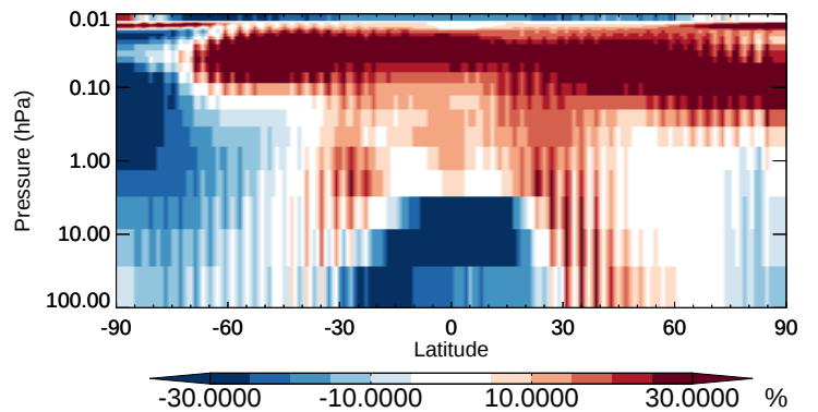
v11-02b-HP / v11-02a MP - Strat zonal mean % diff for Apr
