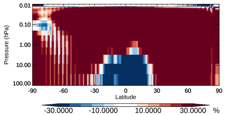
v11-02b-HP / v11-02a OCIO - Strat zonal mean % diff for Apr
