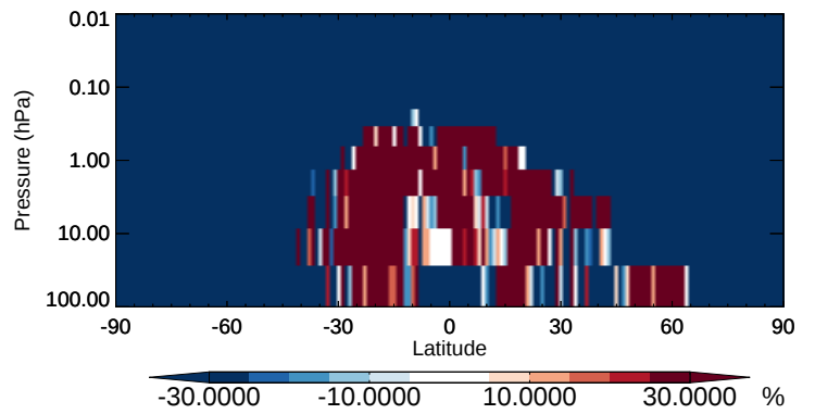
v11-02b-HP / v11-02a MTPA - Strat zonal mean % diff for Apr
