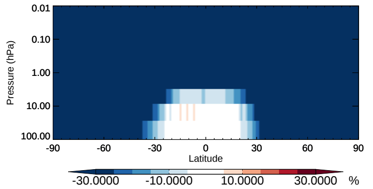
v11-02b-HP / v11-02a ISOG3 - Strat zonal mean % diff for Apr
