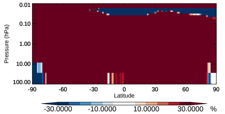
v11-02b-HP / v11-02a DMS - Strat zonal mean % diff for Apr
