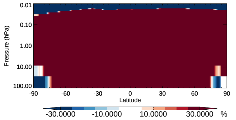
v11-02b-HP / v11-02a DST3 - Strat zonal mean % diff for Apr
