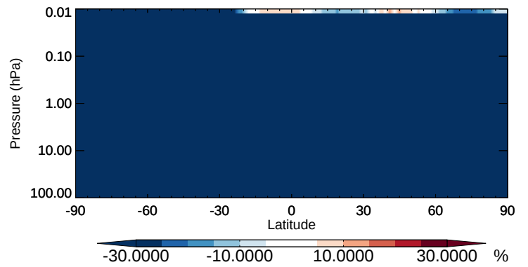
v11-02b-HP / v11-02a SO4 - Strat zonal mean % diff for Apr
