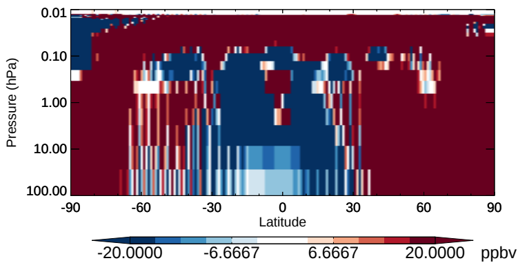
v11-02b-HP - v11-02a O3 - Strat zonal mean abs diff for Apr
