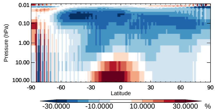
v11-02b-HP / v11-02a NO2 - Strat zonal mean % diff for Apr
