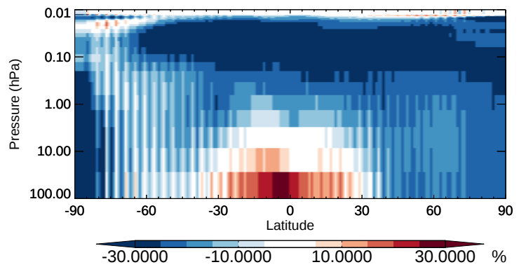
v11-02b-HP / v11-02a HNO 2 - Strat zonal mean % diff for Apr
