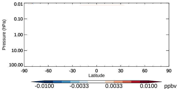
v11-02b-HP - v11-02a Br - Strat zonal mean abs diff for Apr
