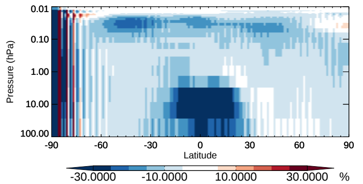
v11-02b-HP / v11-02a Cl - Strat zonal mean % diff for Apr
