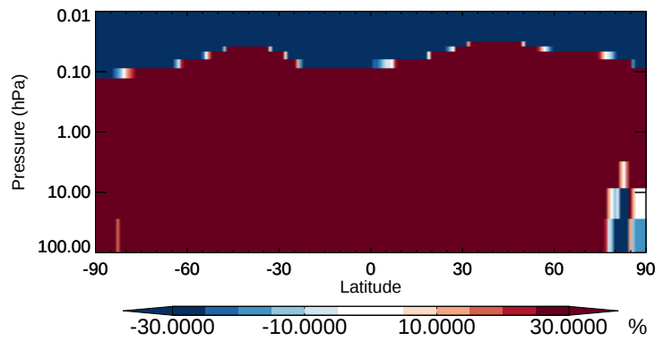
v11-02b-HP / v11-02a NITs - Strat zonal mean % diff for Apr
