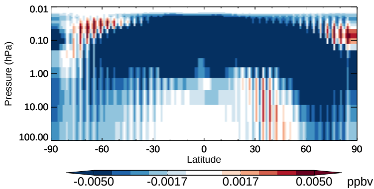
v11-02b-HP - v11-02a HNO4 - Strat zonal mean abs diff for Apr
