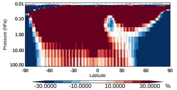
v11-02b-HP / v11-02a MEK - Strat zonal mean % diff for Apr
