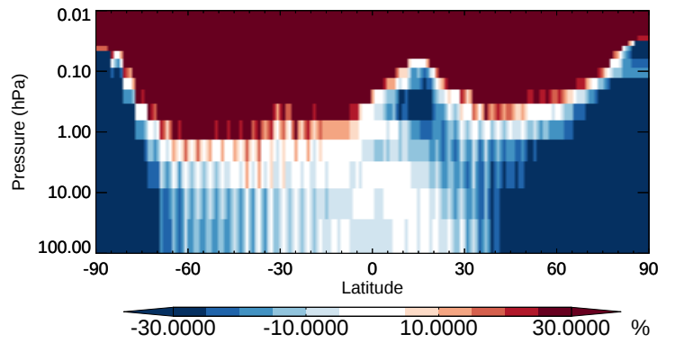
v11-02b-HP / v11-02a C3H8 - Strat zonal mean % diff for Apr
