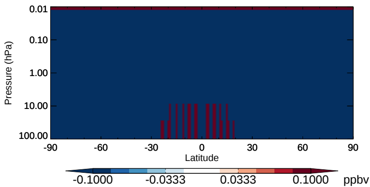
v11-02b-HP - v11-02a H 2 O - Strat zonal mean abs diff for Apr
