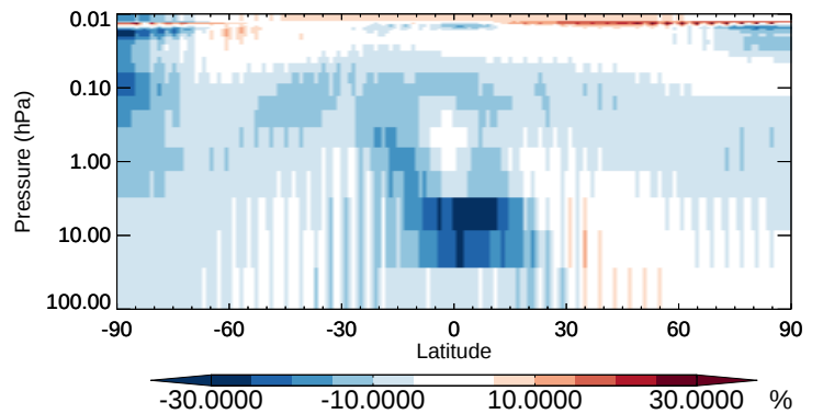
v11-02b-HP / v11-02a MPN - Strat zonal mean % diff for Apr
