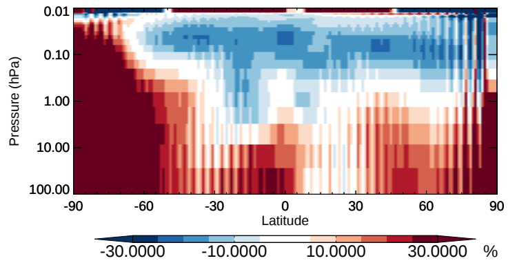
v11-02b-HP / v11-02a N2O5 - Strat zonal mean % diff for Apr
