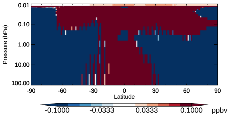
v11-02b-HP - v11-02a N 2 O - Strat zonal mean abs diff for Apr
