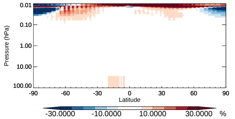
v11-02b-HP / v11-02a PPN - Strat zonal mean % diff for Apr
