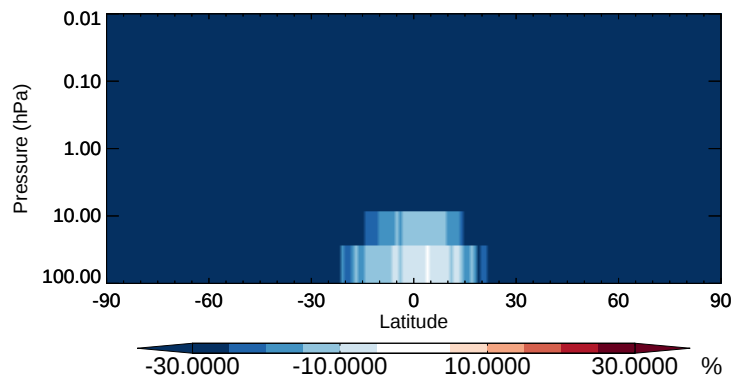
v11-02b-HP / v11-02a ASOA3 - Strat zonal mean % diff for Apr
