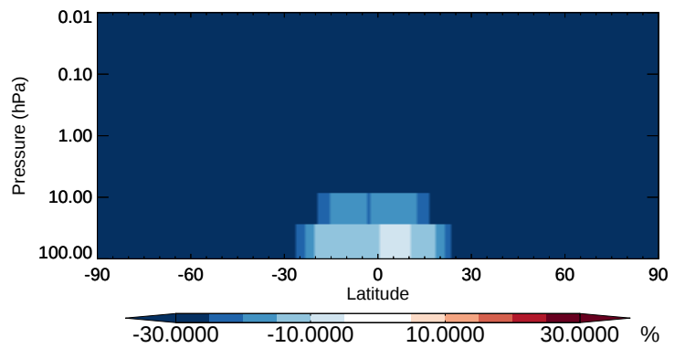
v11-02b-HP / v11-02a ISOA1 - Strat zonal mean % diff for Apr
