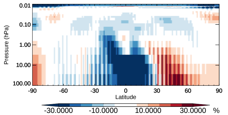
v11-02b-HP / v11-02a ClNO3 - Strat zonal mean % diff for Apr
