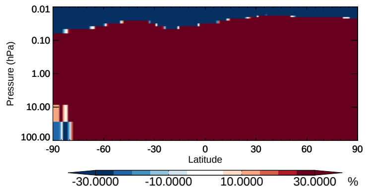
v11-02b-HP / v11-02a DST4 - Strat zonal mean % diff for Apr
