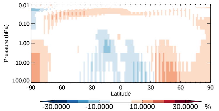
v11-02b-HP / v11-02a O3 - Strat zonal mean % diff for Apr
