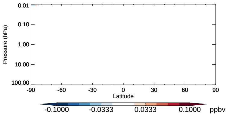
v11-02b-HP - v11-02a Cl - Strat zonal mean abs diff for Apr
