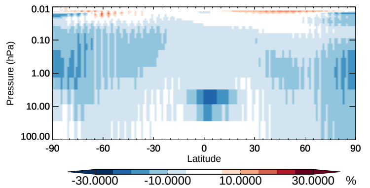
v11-02b-HP / v11-02a CH2O - Strat zonal mean % diff for Apr
