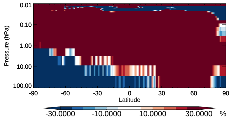
v11-02b-HP / v11-02a IEPOX - Strat zonal mean % diff for Apr
