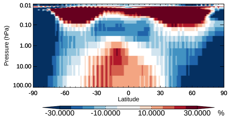
v11-02b-HP / v11-02a PAN - Strat zonal mean % diff for Apr
