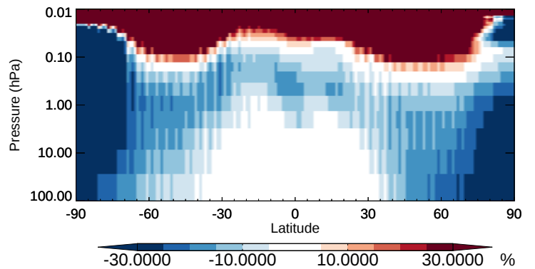
v11-02b-HP / v11-02a C2H6 - Strat zonal mean % diff for Apr
