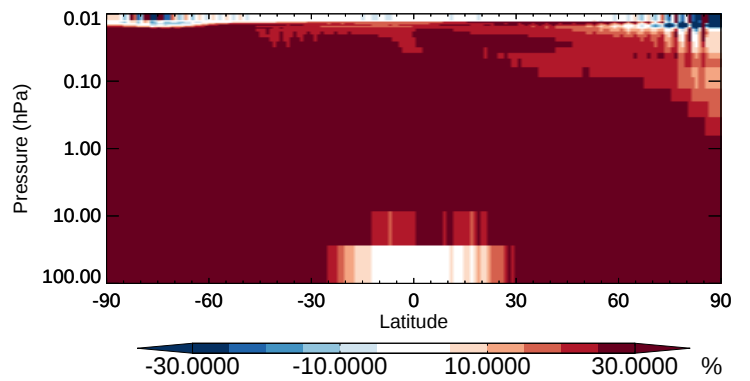
v11-02b-HP / v11-02a BrNO 3 - Strat zonal mean % diff for Apr
