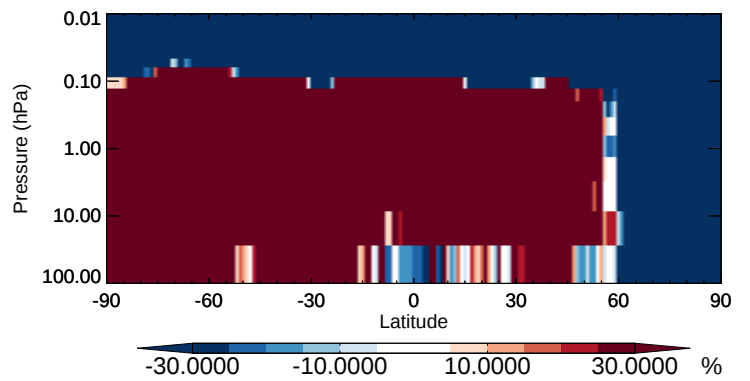
v11-02b-HP / v11-02a MACR - Strat zonal mean % diff for Apr
