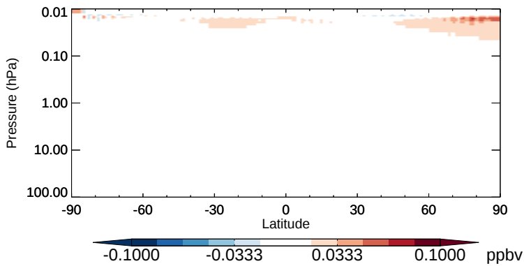
v11-02b-HP - v11-02a ClO - Strat zonal mean abs diff for Apr
