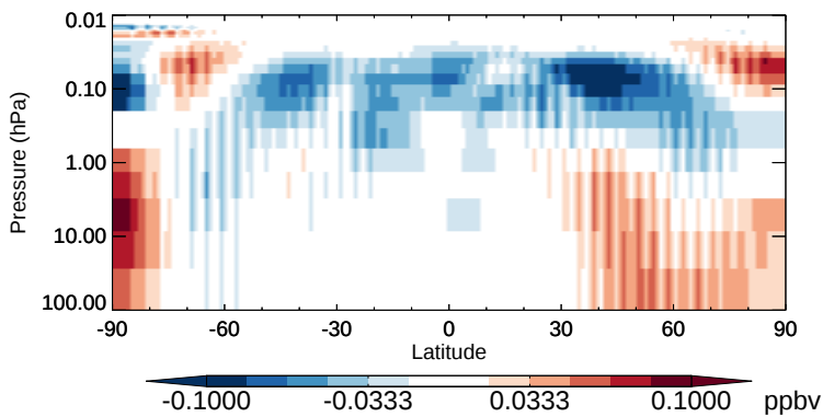
v11-02b-HP - v11-02a ClNO3 - Strat zonal mean abs diff for Apr
