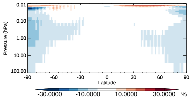
v11-02b-HP / v11-02a CH4 - Strat zonal mean % diff for Apr
