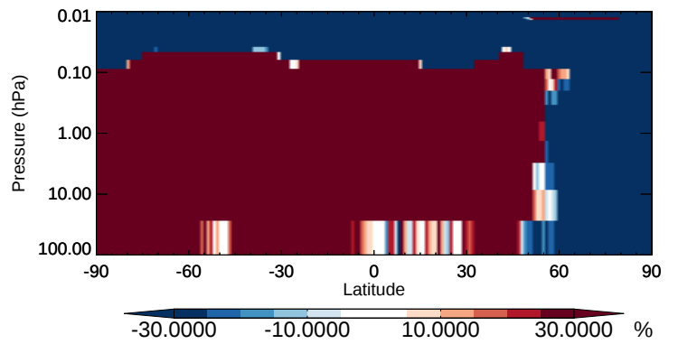
v11-02b-HP / v11-02a PRPE - Strat zonal mean % diff for Apr
