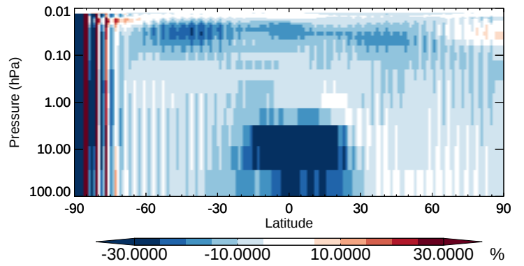
v11-02b-HP / v11-02a ClOO - Strat zonal mean % diff for Apr
