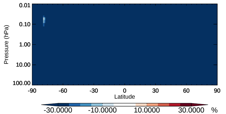
v11-02b-HP / v11-02a ClNO2 - Strat zonal mean % diff for Apr
