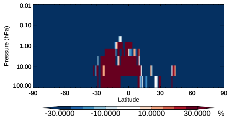
v11-02b-HP / v11-02a MTPO - Strat zonal mean % diff for Apr
