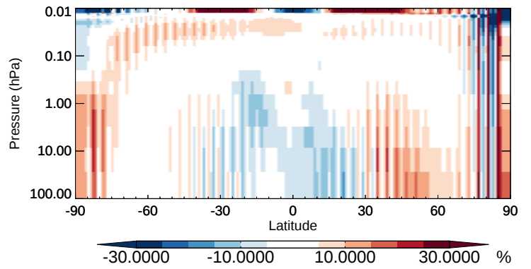
v11-02b-HP / v11-02a NO 3 - Strat zonal mean % diff for Apr
