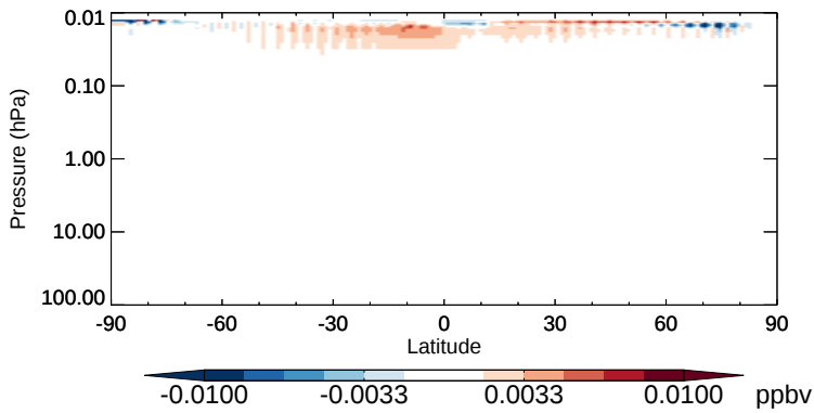
v11-02b-HP - v11-02a NO 3 - Strat zonal mean abs diff for Apr
