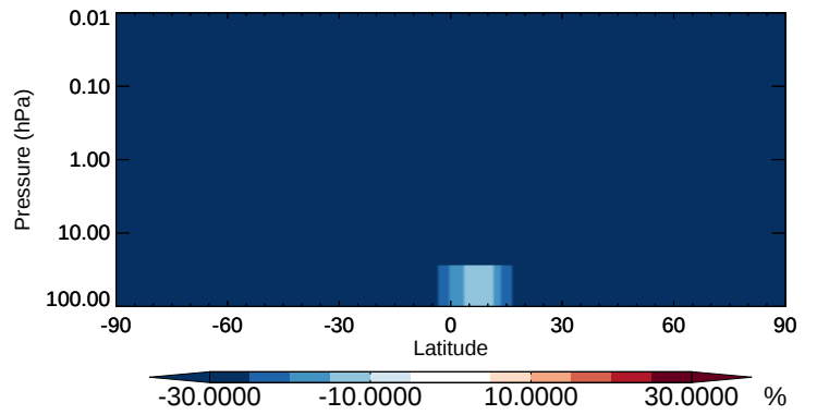
v11-02b-HP / v11-02a NH4 - Strat zonal mean % diff for Apr
