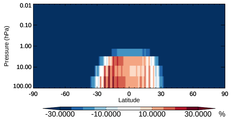
v11-02b-HP / v11-02a ISOG2 - Strat zonal mean % diff for Apr
