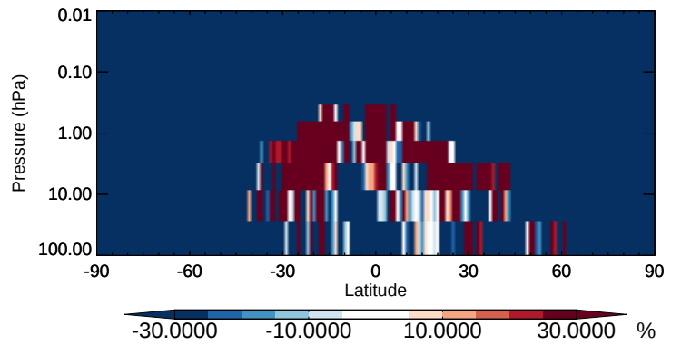
v11-02b-HP / v11-02a LIMO - Strat zonal mean % diff for Apr
