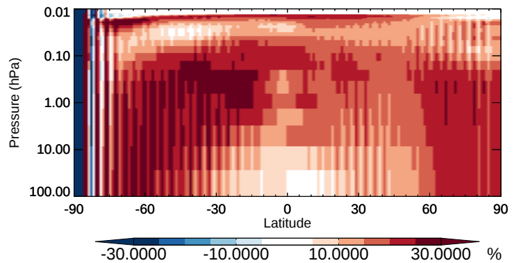
v11-02b-HP / v11-02a Br - Strat zonal mean % diff for Apr
