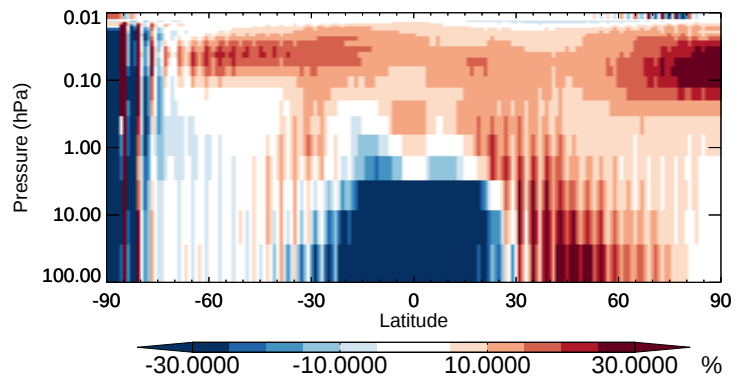
v11-02b-HP / v11-02a ClO - Strat zonal mean % diff for Apr
