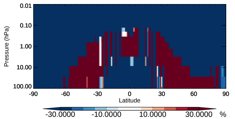
v11-02b-HP / v11-02a NIT - Strat zonal mean % diff for Apr
