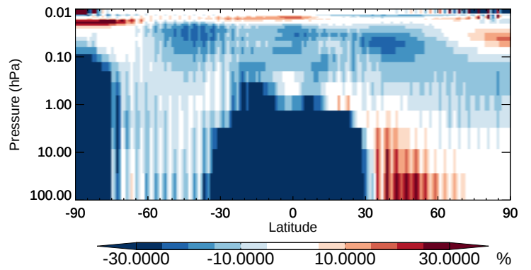
v11-02b-HP / v11-02a Cl2 - Strat zonal mean % diff for Apr
