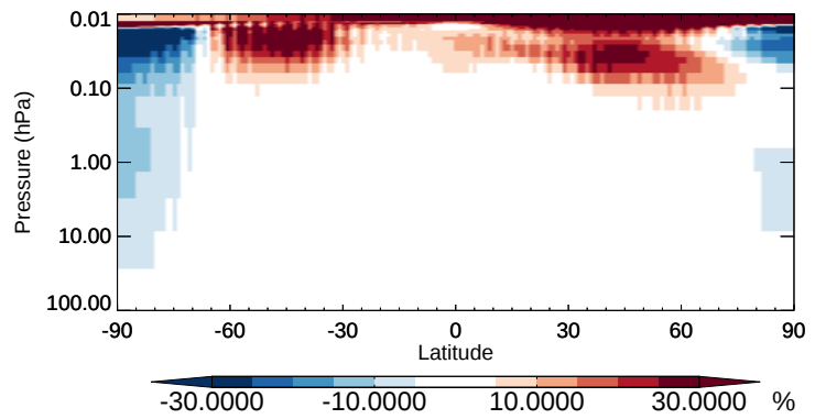
v11-02b-HP / v11-02a N 2 O - Strat zonal mean % diff for Apr
