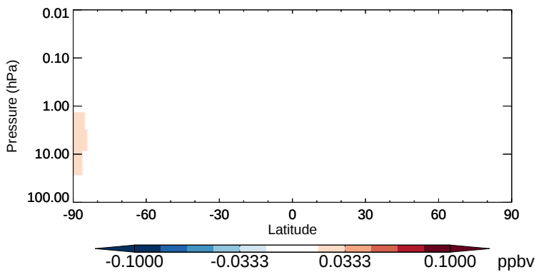
v11-02b-HP - v11-02a OCIO - Strat zonal mean abs diff for Apr
