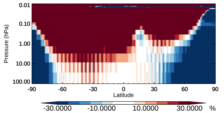
v11-02b-HP / v11-02a CHBr 3 - Strat zonal mean % diff for Apr
