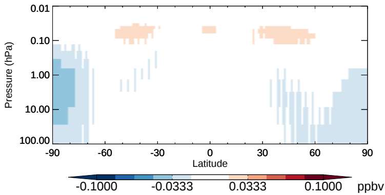
v11-02b-HP - v11-02a OCS - Strat zonal mean abs diff for Apr
