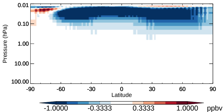
v11-02b-HP - v11-02a NO2 - Strat zonal mean abs diff for Apr
