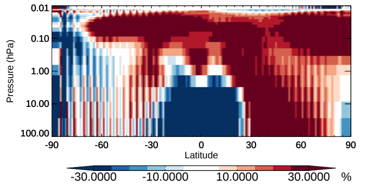
v11-02b-HP / v11-02a Cl 2 O 2 - Strat zonal mean % diff for Apr
