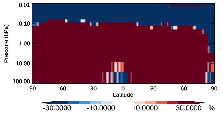
v11-02b-HP / v11-02a MVK - Strat zonal mean % diff for Apr
