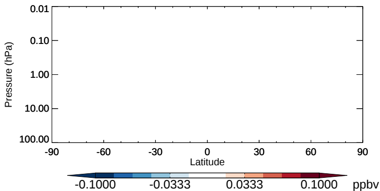
v11-02b-HP - v11-02a ClNO2 - Strat zonal mean abs diff for Apr
