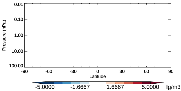
v11-02b-HP - v11-02a DST4 - Strat zonal mean abs diff for Apr
