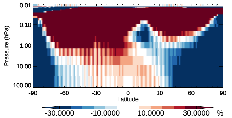
v11-02b-HP / v11-02a RCHO - Strat zonal mean % diff for Apr
