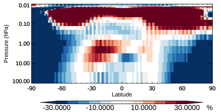
v11-02b-HP / v11-02a MAP - Strat zonal mean % diff for Apr
