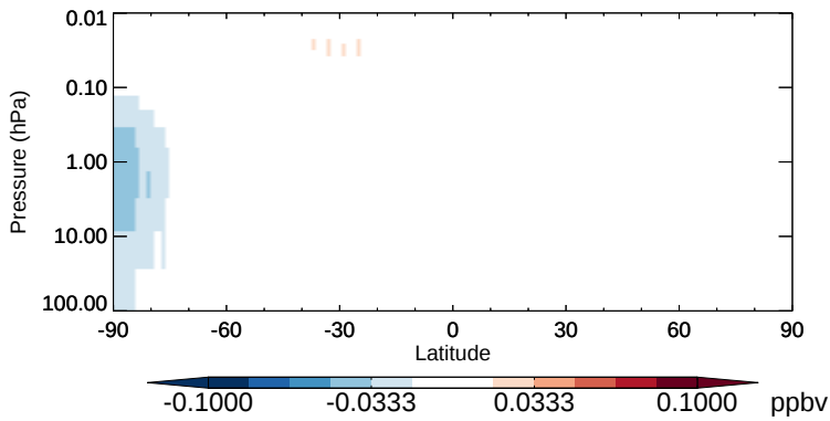
v11-02b-HP - v11-02a HOCl - Strat zonal mean abs diff for Apr
