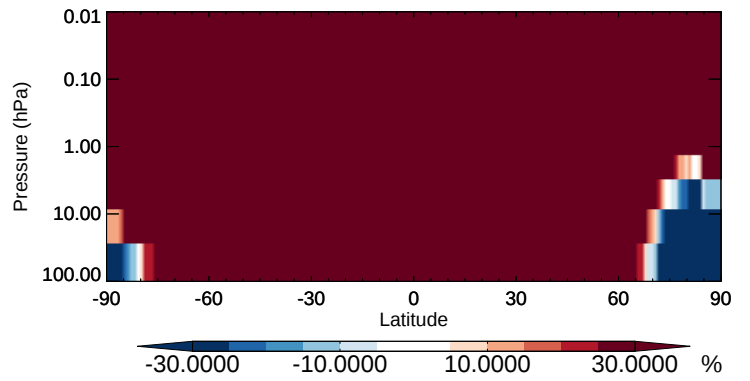
v11-02b-HP / v11-02a SALC - Strat zonal mean % diff for Apr
