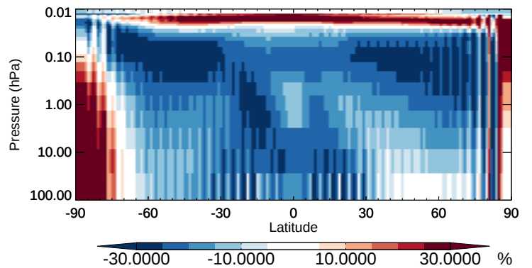
v11-02b-HP / v11-02a BrCl - Strat zonal mean % diff for Apr
