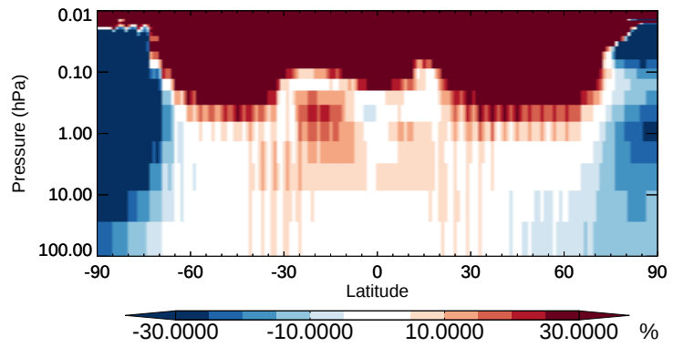
v11-02b-HP / v11-02a CH 2 Br 2 - Strat zonal mean % diff for Apr
