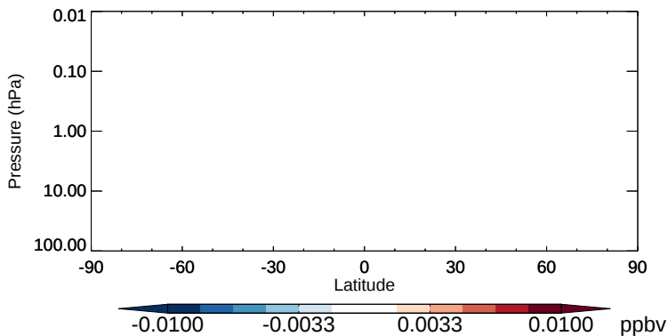
v11-02b-HP - v11-02a HBr - Strat zonal mean abs diff for Apr
