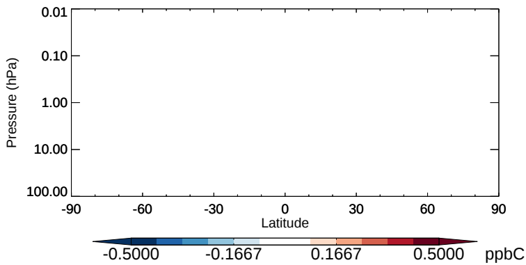
v11-02b-HP - v11-02a ISOP - Strat zonal mean abs diff for Apr
