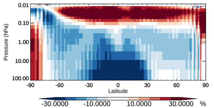
v11-02b-HP / v11-02a HOBr - Strat zonal mean % diff for Apr
