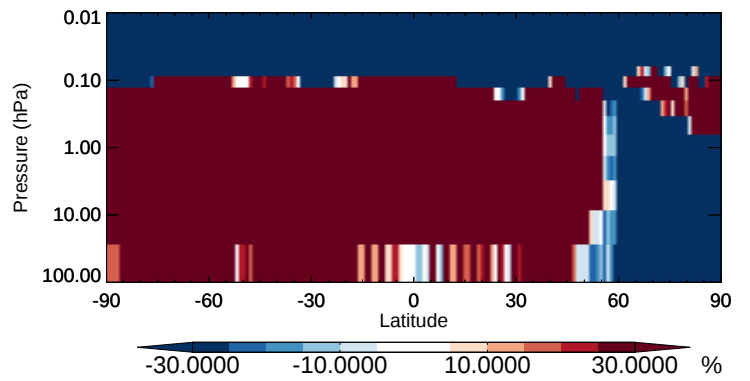
v11-02b-HP / v11-02a PMN - Strat zonal mean % diff for Apr
