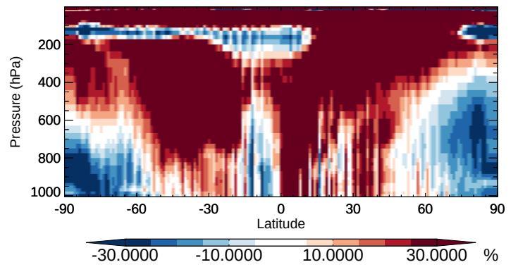
v11-02b-HP / v11-02a MVKN - Zonal mean % diff for Apr
