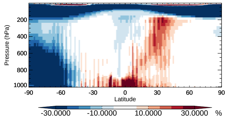
v11-02b-HP / v11-02a MGLY - Zonal mean % diff for Apr
