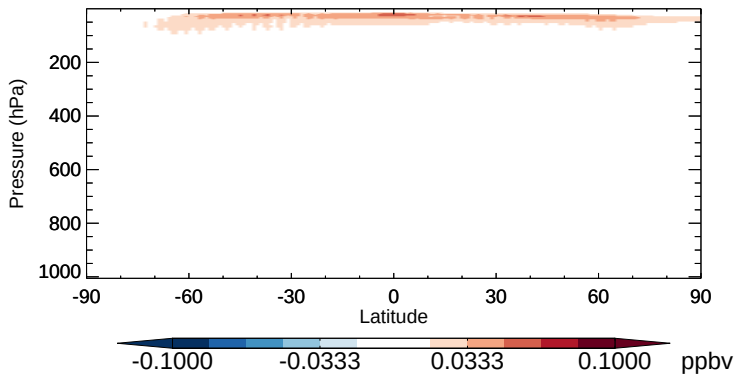
v11-02b-HP - v11-02a CFC12 - Zonal mean abs diff for Apr
