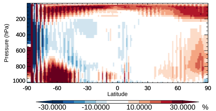
v11-02b-HP / v11-02a Br - Zonal mean % diff for Apr
