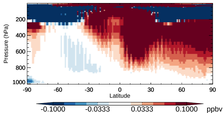
v11-02b-HP - v11-02a N 2 O - Zonal mean abs diff for Apr
