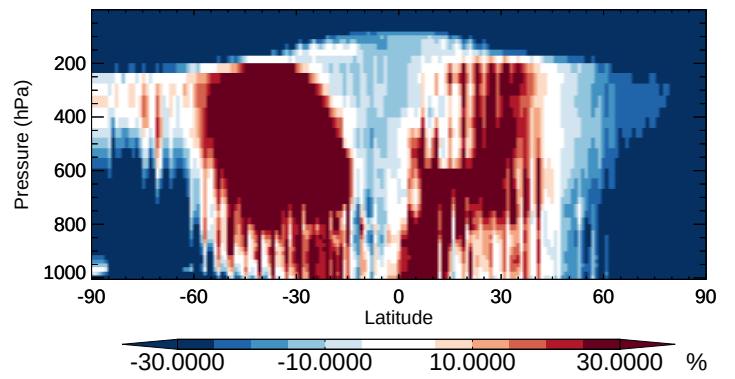
v11-02b-HP / v11-02a ISOA3 - Zonal mean % diff for Apr
