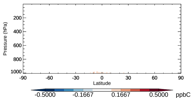
v11-02b-HP - v11-02a ALD2 - Zonal mean abs diff for Apr
