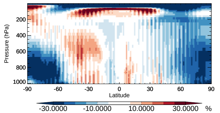
v11-02b-HP / v11-02a ISOG1 - Zonal mean % diff for Apr
