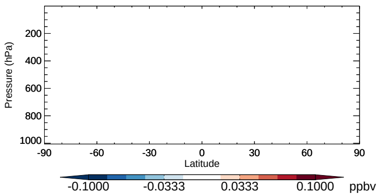
v11-02b-HP - v11-02a ISOPNB - Zonal mean abs diff for Apr
