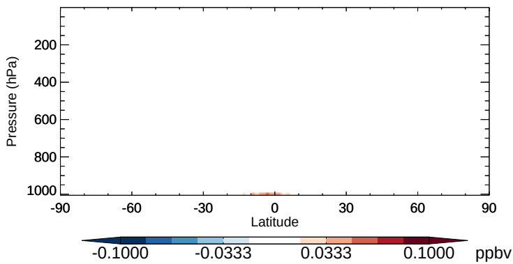
v11-02b-HP - v11-02a MTPA - Zonal mean abs diff for Apr
