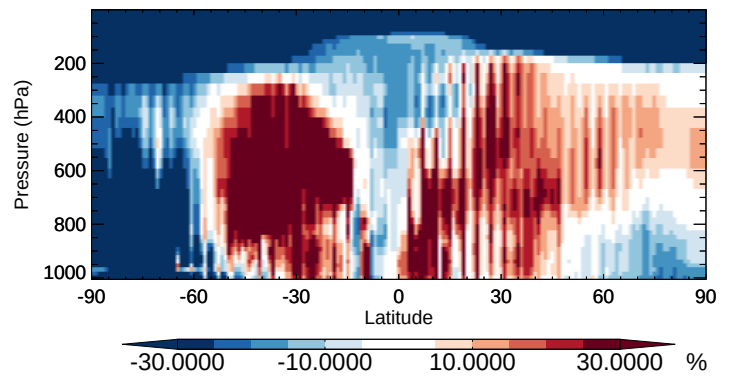
v11-02b-HP / v11-02a ASOA2 - Zonal mean % diff for Apr
