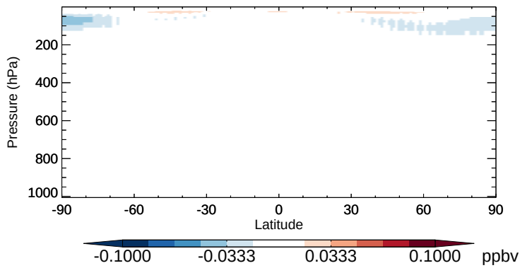
v11-02b-HP - v11-02a OCS - Zonal mean abs diff for Apr
