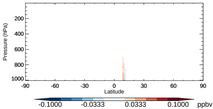
v11-02b-HP - v11-02a GLYC - Zonal mean abs diff for Apr
