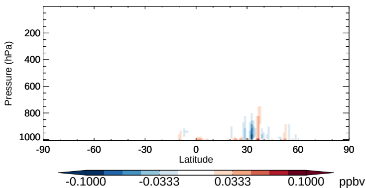
v11-02b-HP - v11-02a TOLU - Zonal mean abs diff for Apr
