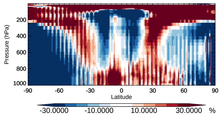
v11-02b-HP / v11-02a OC1O - Zonal mean % diff for Apr
