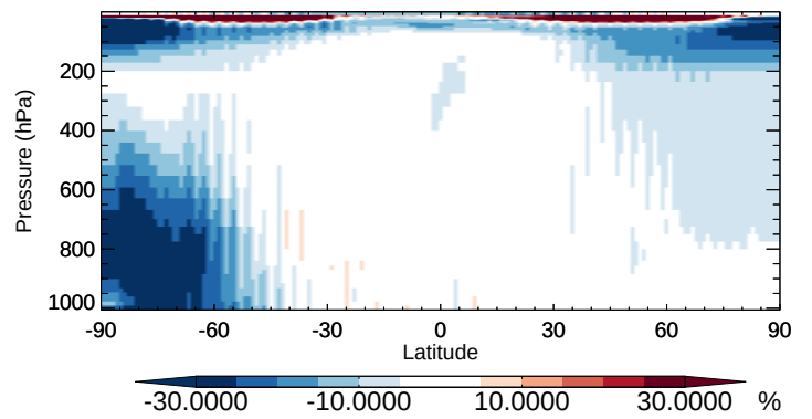
v11-02b-HP / v11-02a EOH - Zonal mean % diff for Apr
