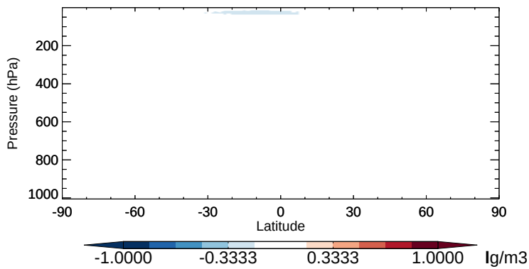
v11-02b-HP - v11-02a SO 4 - Zonal mean abs diff for Apr
