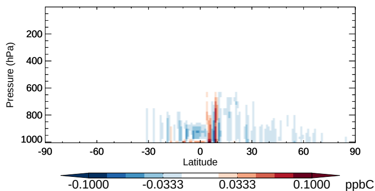
v11-02b-HP - v11-02a MEK - Zonal mean abs diff for Apr
