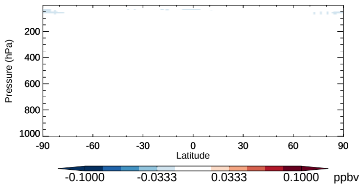
v11-02b-HP - v11-02a MPN - Zonal mean abs diff for Apr
