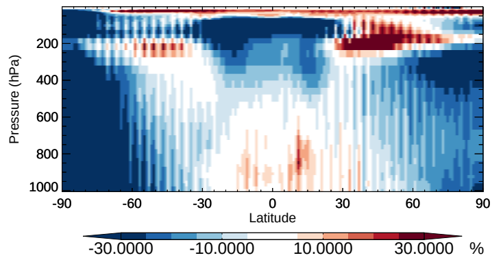
v11-02b-HP / v11-02a HOCl - Zonal mean % diff for Apr
