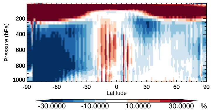
v11-02b-HP / v11-02a BrNO 3 - Zonal mean % diff for Apr
