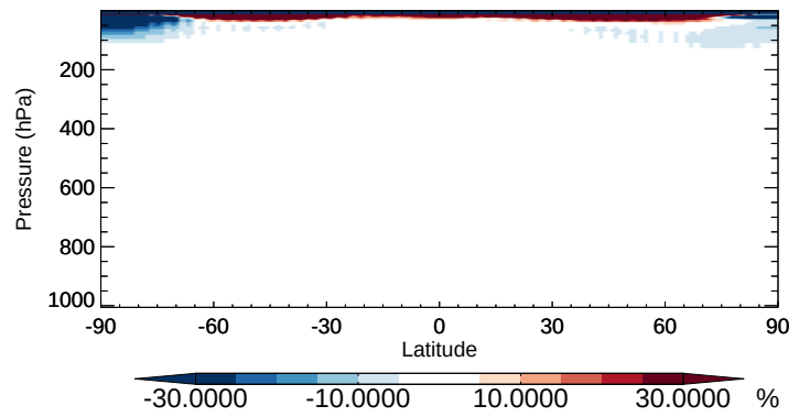
v11-02b-HP / v11-02a OCS - Zonal mean % diff for Apr
