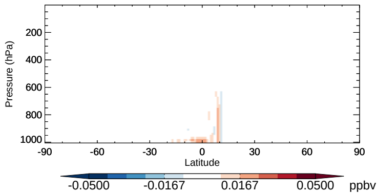
v11-02b-HP - v11-02a MVK - Zonal mean abs diff for Apr
