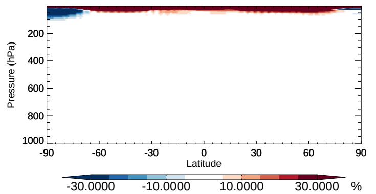
v11-02b-HP / v11-02a CH 3 Br - Zonal mean % diff for Apr
