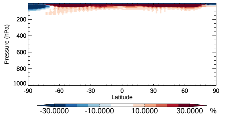
v11-02b-HP / v11-02a H2402 - Zonal mean % diff for Apr
