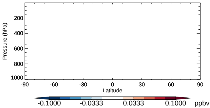
v11-02b-HP - v11-02a ISOA3 - Zonal mean abs diff for Apr
