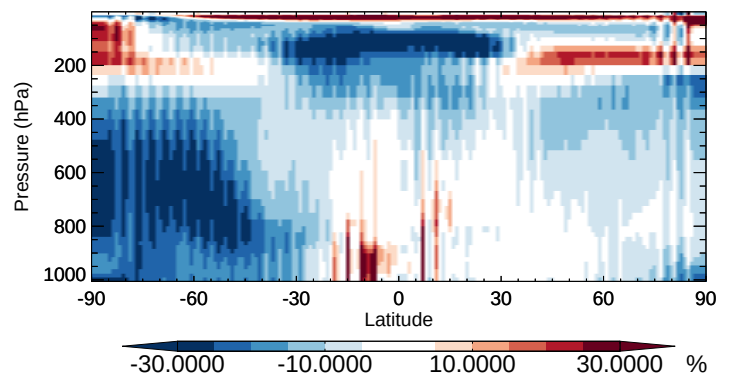
v11-02b-HP / v11-02a HOBr - Zonal mean % diff for Apr
