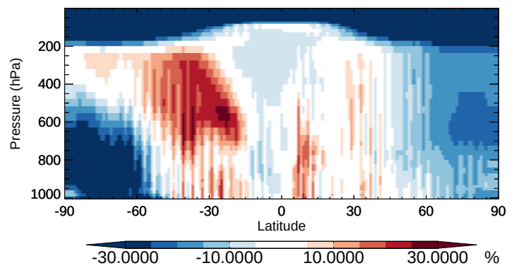
v11-02b-HP / v11-02a TSOG3 - Zonal mean % diff for Apr
