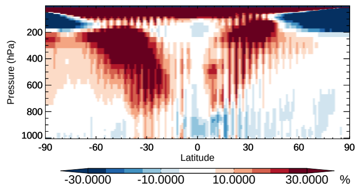
v11-02b-HP / v11-02a ALK4 - Zonal mean % diff for Apr
