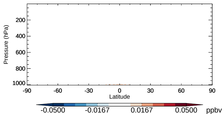
v11-02b-HP - v11-02a RCHO - Zonal mean abs diff for Apr
