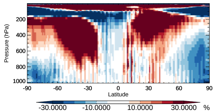
v11-02b-HP / v11-02a HAC - Zonal mean % diff for Apr
