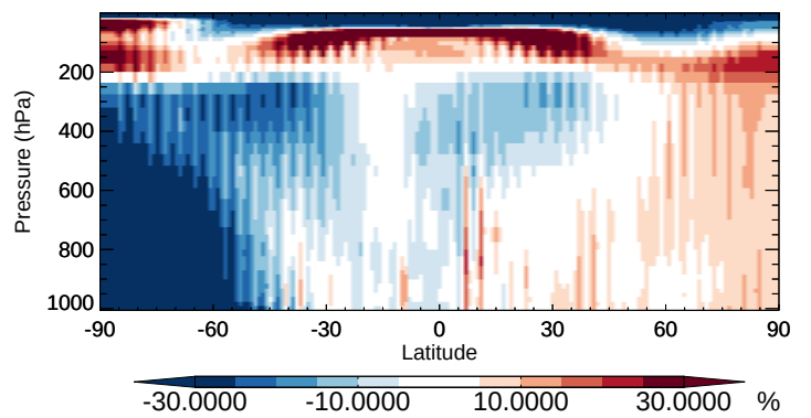
v11-02b-HP / v11-02a ASOG1 - Zonal mean % diff for Apr
