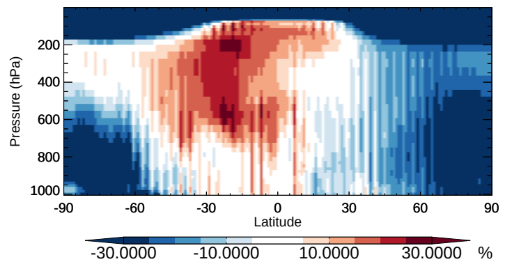
v11-02b-HP / v11-02a ISOG2 - Zonal mean % diff for Apr
