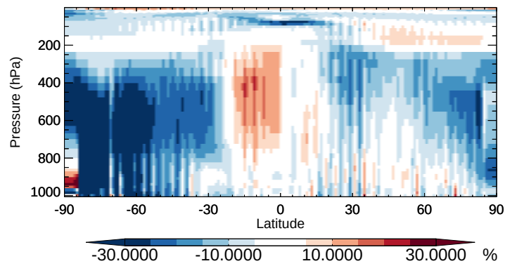
v11-02b-HP / v11-02a MPN - Zonal mean % diff for Apr
