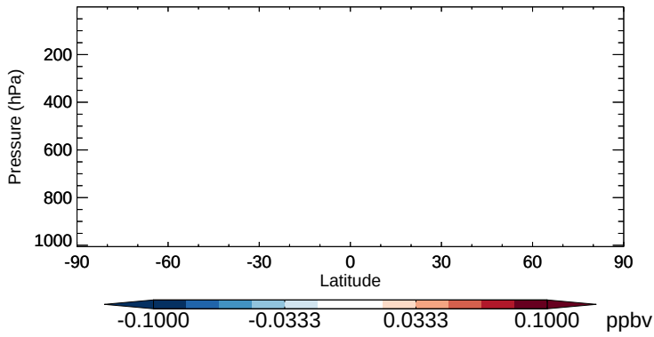
v11-02b-HP - v11-02a HCFC22 - Zonal mean abs diff for Apr
