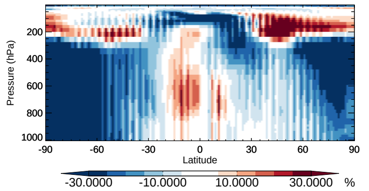
v11-02b-HP / v11-02a ClNO3 - Zonal mean % diff for Apr
