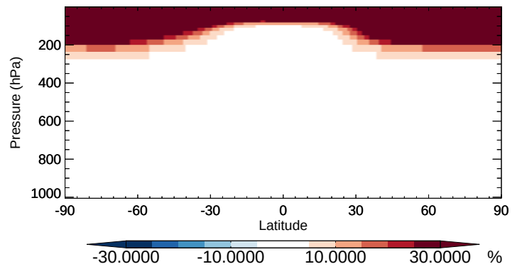
v11-02b-HP / v11-02a CFC115 - Zonal mean % diff for Apr
