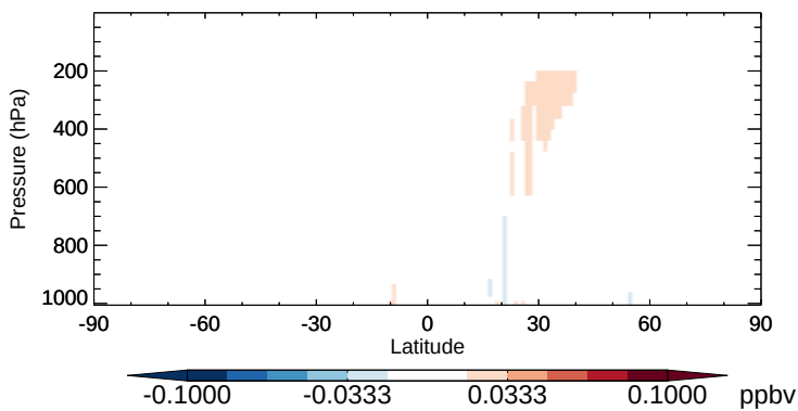
v11-02b-HP - v11-02a BENZ - Zonal mean abs diff for Apr
