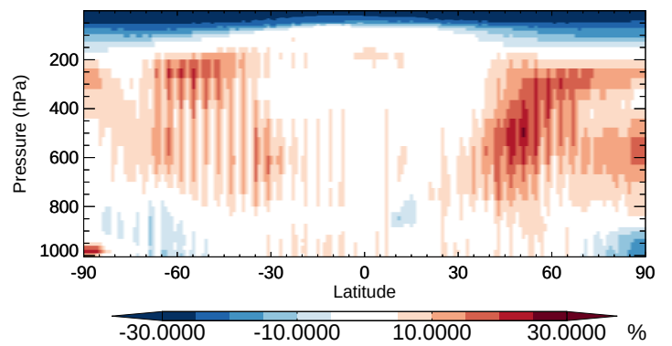
v11-02b-HP / v11-02a MSA - Zonal mean % diff for Apr
