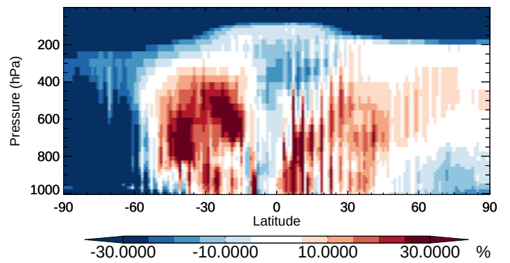
v11-02b-HP / v11-02a ASOA1 - Zonal mean % diff for Apr
