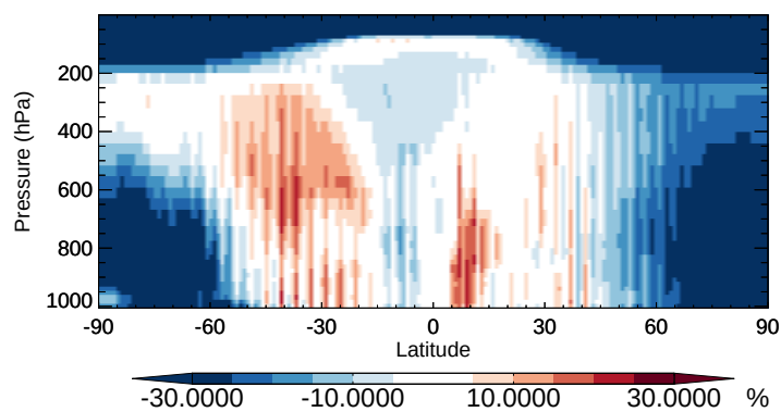
v11-02b-HP / v11-02a ISO3 - Zonal mean % diff for Apr
