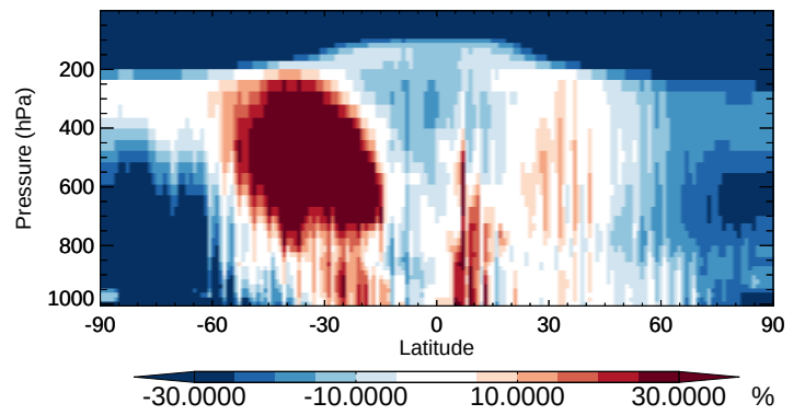
v11-02b-HP / v11-02a TSOA0 - Zonal mean % diff for Apr
