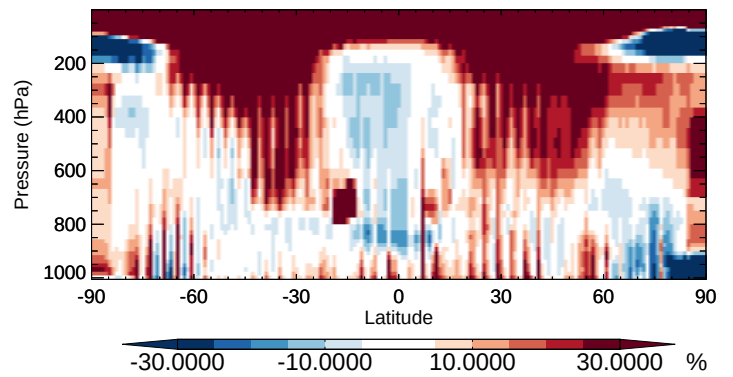
v11-02b-HP / v11-02a SALC - Zonal mean % diff for Apr
