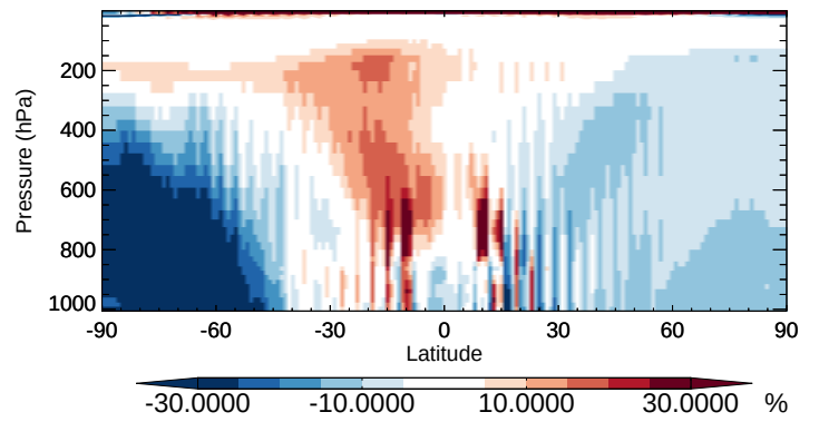
v11-02b-HP / v11-02a PPN - Zonal mean % diff for Apr
