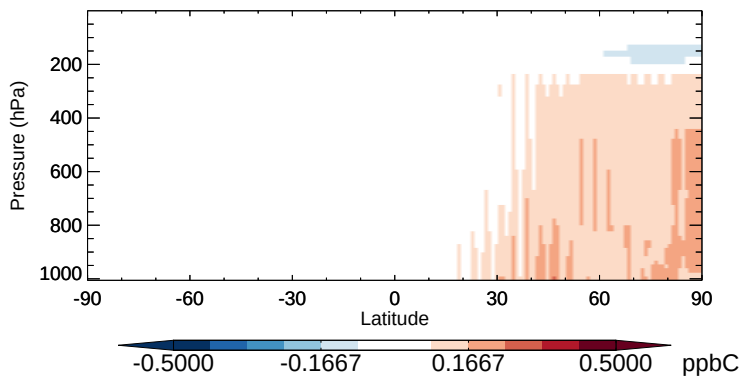
v11-02b-HP - v11-02a C2H6 - Zonal mean abs diff for Apr
