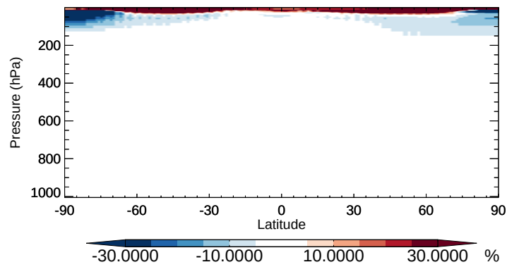
v11-02b-HP / v11-02a H1301 - Zonal mean % diff for Apr
