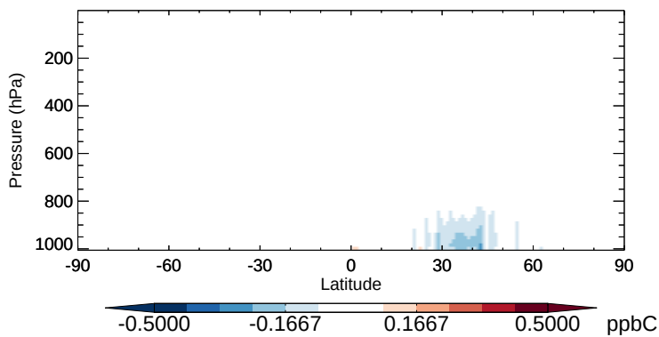
v11-02b-HP - v11-02a ALK4 - Zonal mean abs diff for Apr
