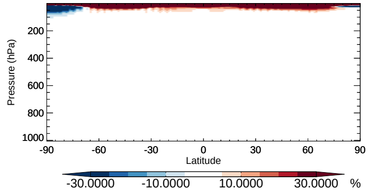
v11-02b-HP / v11-02a CFC11 - Zonal mean % diff for Apr
