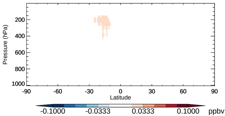
v11-02b-HP - v11-02a PAN - Zonal mean abs diff for Apr
