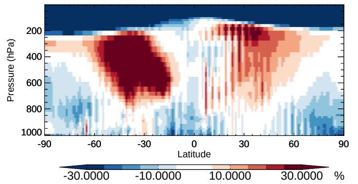
v11-02b-HP / v11-02a NH4 - Zonal mean % diff for Apr
