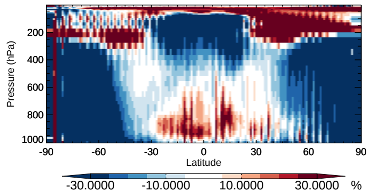
v11-02b-HP / v11-02a Cl 2 O 2 - Zonal mean % diff for Apr
