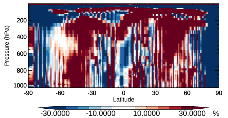
v11-02b-HP / v11-02a ISOPNB - Zonal mean % diff for Apr
