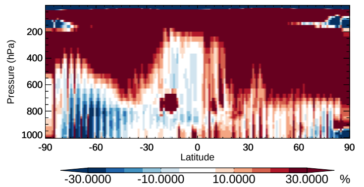
v11-02b-HP / v11-02a NITs - Zonal mean % diff for Apr
