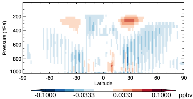
v11-02b-HP - v11-02a H 2 O 2 - Zonal mean abs diff for Apr
