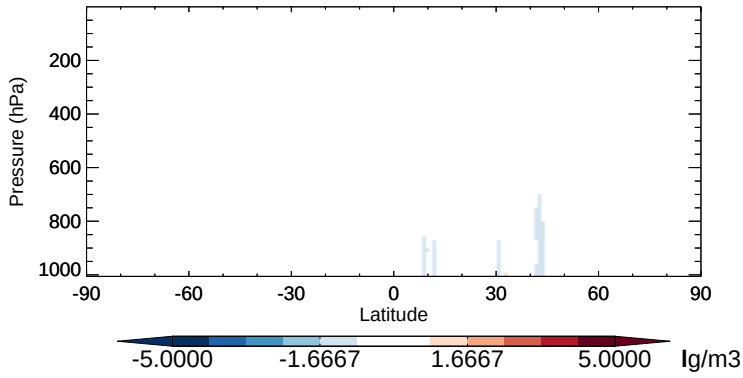
v11-02b-HP - v11-02a DST1 - Zonal mean abs diff for Apr
