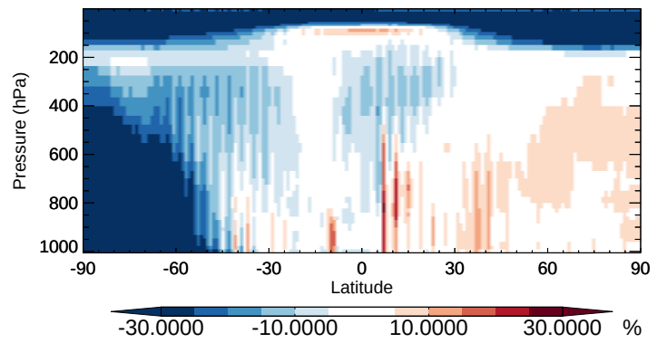
v11-02b-HP / v11-02a ASOG3 - Zonal mean % diff for Apr
