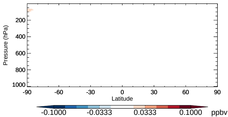
v11-02b-HP - v11-02a OC1O - Zonal mean abs diff for Apr
