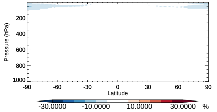
v11-02b-HP / v11-02a HCFC22 - Zonal mean % diff for Apr
