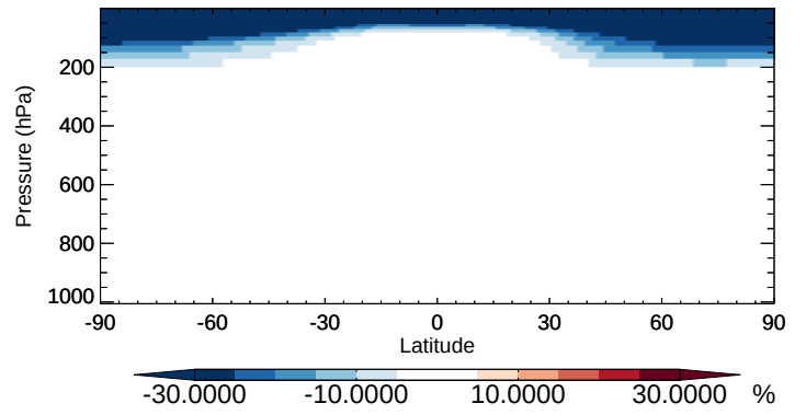
v11-02b-HP / v11-02a HCFC142b - Zonal mean % diff for Apr
