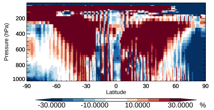
v11-02b-HP / v11-02a MACR - Zonal mean % diff for Apr
