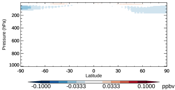
v11-02b-HP - v11-02a CH3Cl - Zonal mean abs diff for Apr
