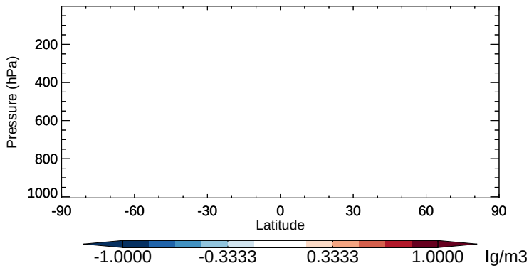
v11-02b-HP - v11-02a SALA - Zonal mean abs diff for Apr
