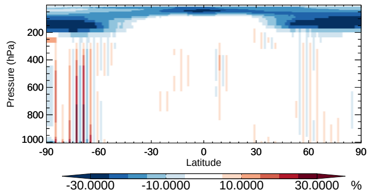
v11-02b-HP / v11-02a H 2 O - Zonal mean % diff for Apr
