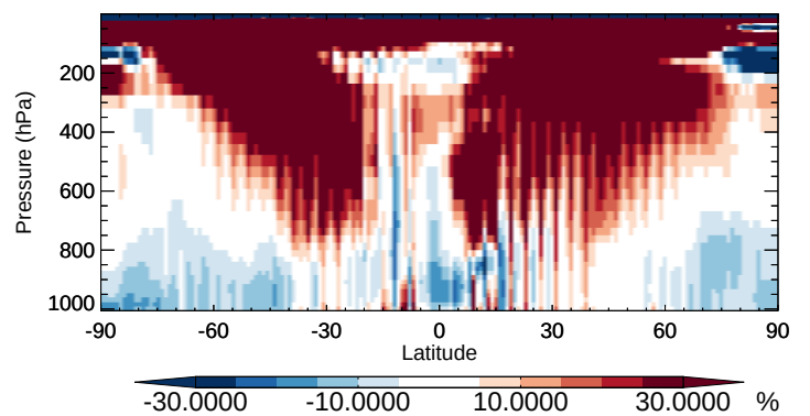
v11-02b-HP / v11-02a TOLU - Zonal mean % diff for Apr
