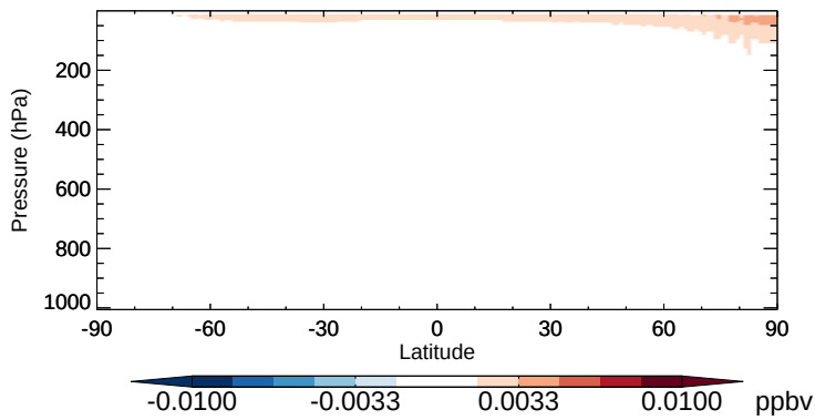
v11-02b-HP - v11-02a BrO - Zonal mean abs diff for Apr
