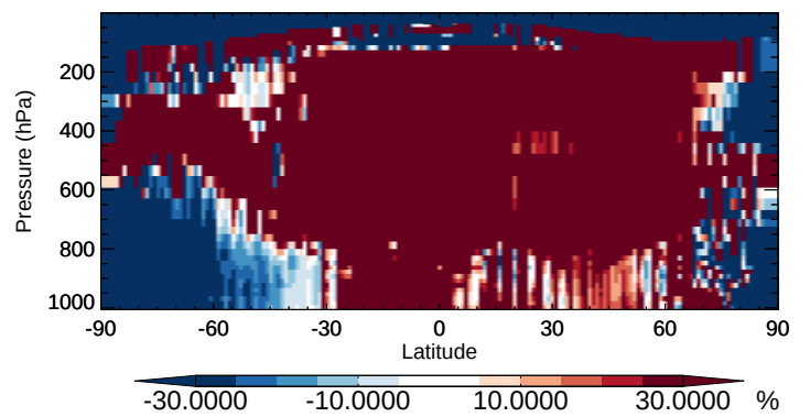
v11-02b-HP / v11-02a NIT - Zonal mean % diff for Apr
