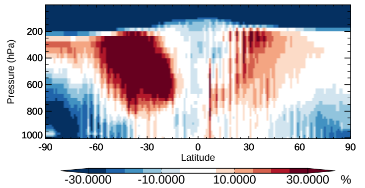
v11-02b-HP / v11-02a BCPI - Zonal mean % diff for Apr
