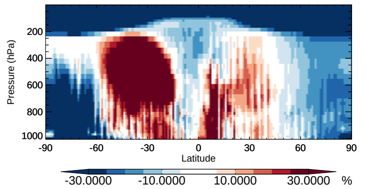
v11-02b-HP / v11-02a TSOA1 - Zonal mean % diff for Apr
