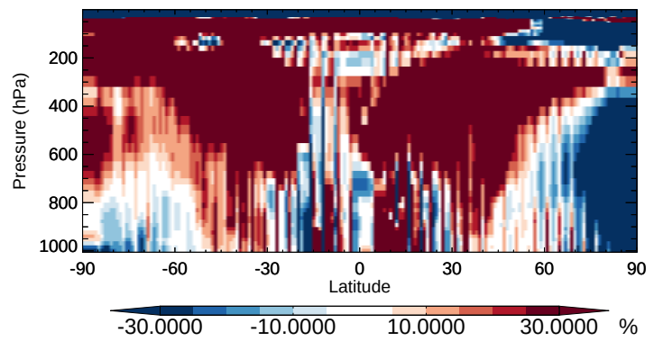
v11-02b-HP / v11-02a PMN - Zonal mean % diff for Apr
