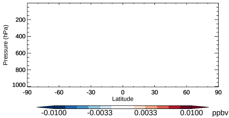
v11-02b-HP - v11-02a CH 2 Br 2 - Zonal mean abs diff for Apr
