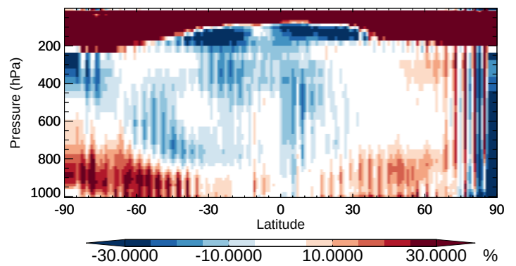
v11-02b-HP / v11-02a Br2 - Zonal mean % diff for Apr
