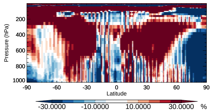
v11-02b-HP / v11-02a MACRN - Zonal mean % diff for Apr
