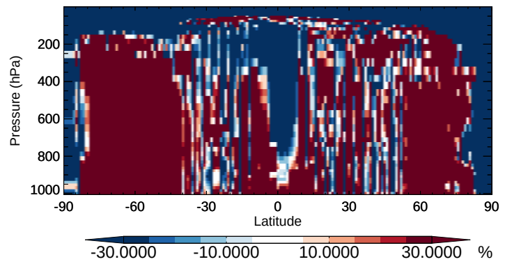
v11-02b-HP / v11-02a LIMO - Zonal mean % diff for Apr
