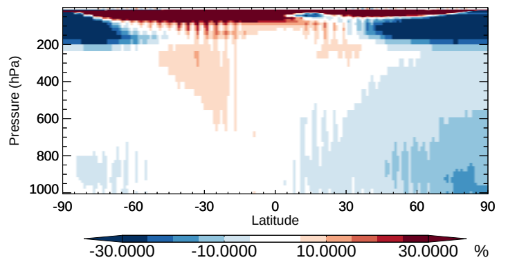
v11-02b-HP / v11-02a ACET - Zonal mean % diff for Apr
