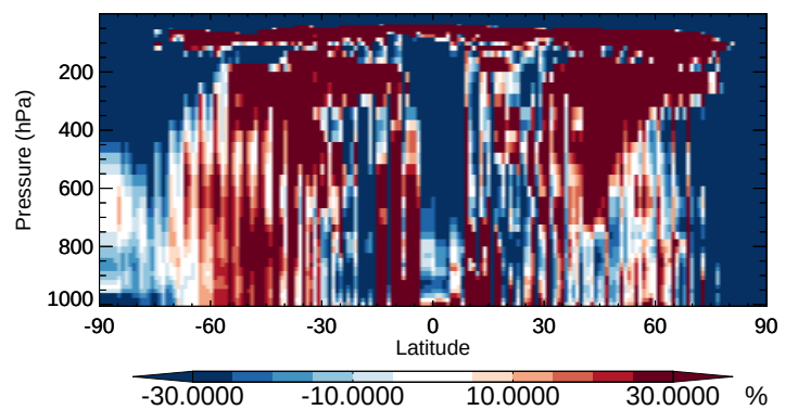
v11-02b-HP / v11-02a ISOP - Zonal mean % diff for Apr
