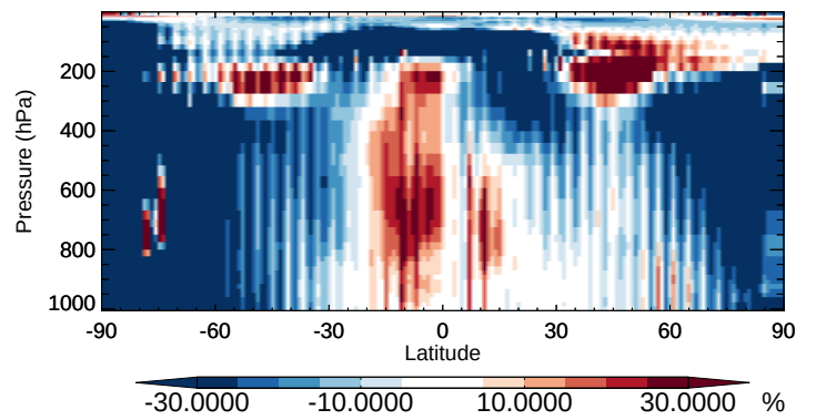
v11-02b-HP / v11-02a Cl2 - Zonal mean % diff for Apr
