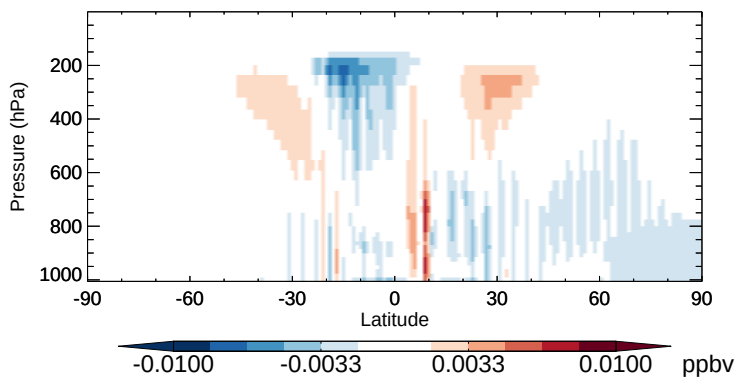
v11-02b-HP - v11-02a MAP - Zonal mean abs diff for Apr
