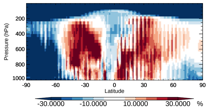
v11-02b-HP / v11-02a ASOA3 - Zonal mean % diff for Apr
