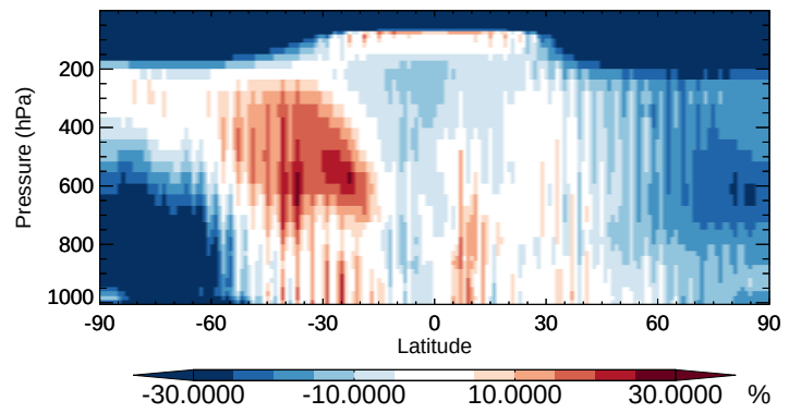
v11-02b-HP / v11-02a TSOG2 - Zonal mean % diff for Apr
