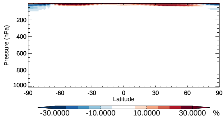
v11-02b-HP / v11-02a N 2 O - Zonal mean % diff for Apr
