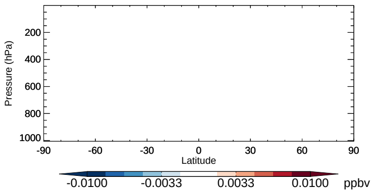
v11-02b-HP - v11-02a MOBA - Zonal mean abs diff for Apr
