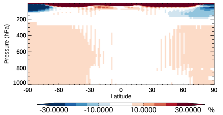
v11-02b-HP / v11-02a CH 2 Br 2 - Zonal mean % diff for Apr
