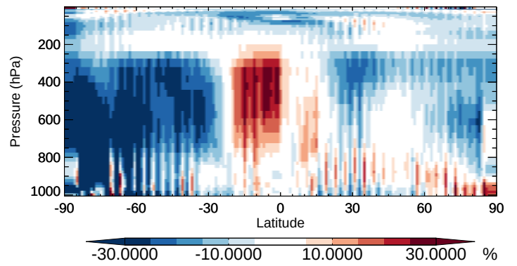
v11-02b-HP / v11-02a HNO 4 - Zonal mean % diff for Apr
