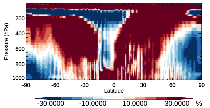
v11-02b-HP / v11-02a GLYC - Zonal mean % diff for Apr
