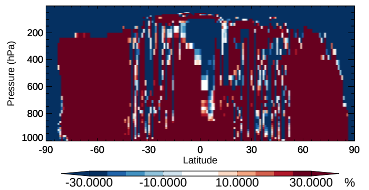
v11-02b-HP / v11-02a MTPO - Zonal mean % diff for Apr
