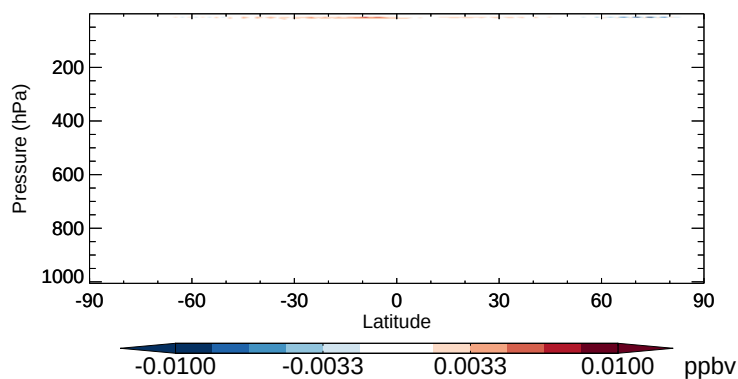
v11-02b-HP - v11-02a NO 3 - Zonal mean abs diff for Apr
