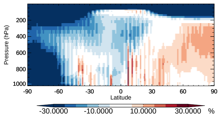
v11-02b-HP / v11-02a ASOG2 - Zonal mean % diff for Apr
