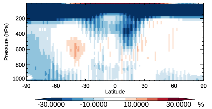
v11-02b-HP / v11-02a SO 4 - Zonal mean % diff for Apr
