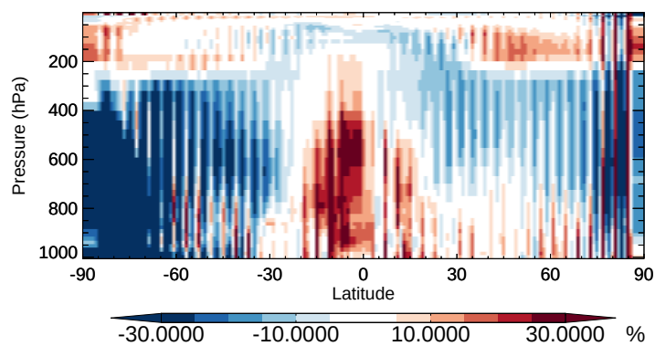
v11-02b-HP / v11-02a NO 3 - Zonal mean % diff for Apr
