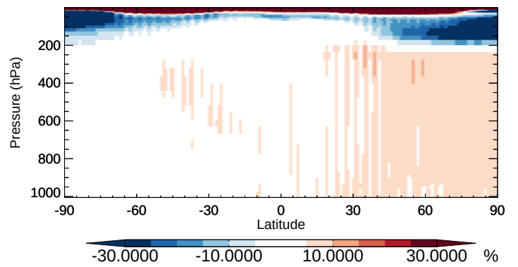
v11-02b-HP / v11-02a C2H6 - Zonal mean % diff for Apr
