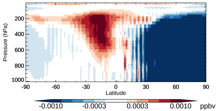
v11-02b-HP - v11-02a PPN - Zonal mean abs diff for Apr
