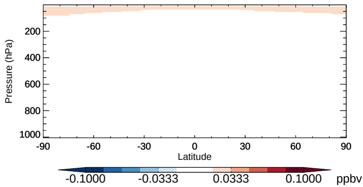
v11-02b-HP - v11-02a CFC115 - Zonal mean abs diff for Apr
