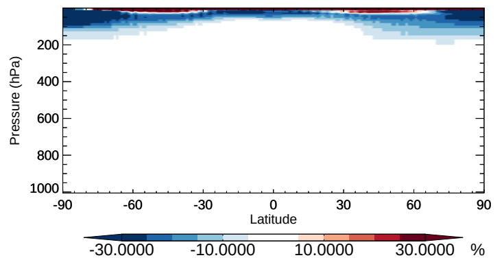
v11-02b-HP / v11-02a CFC113 - Zonal mean % diff for Apr
