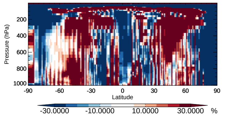
v11-02b-HP / v11-02a ISOPND - Zonal mean % diff for Apr
