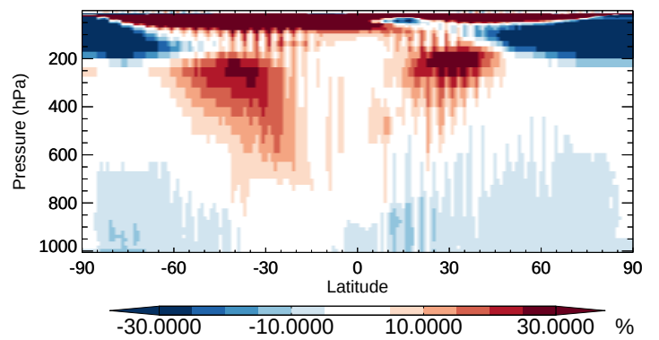
v11-02b-HP / v11-02a R4N2 - Zonal mean % diff for Apr
