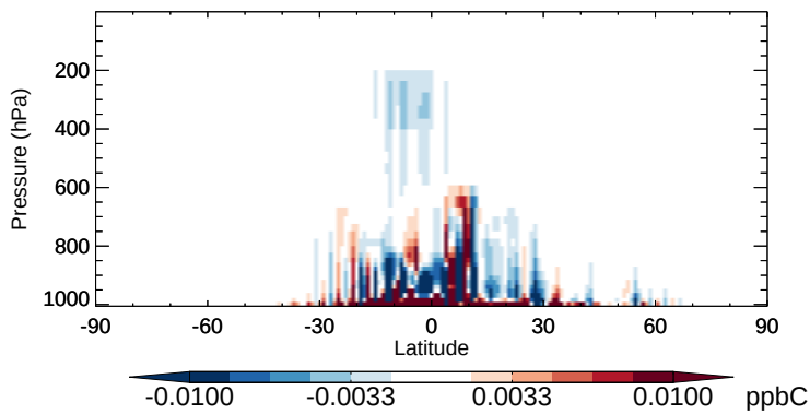
v11-02b-HP - v11-02a PRPE - Zonal mean abs diff for Apr
