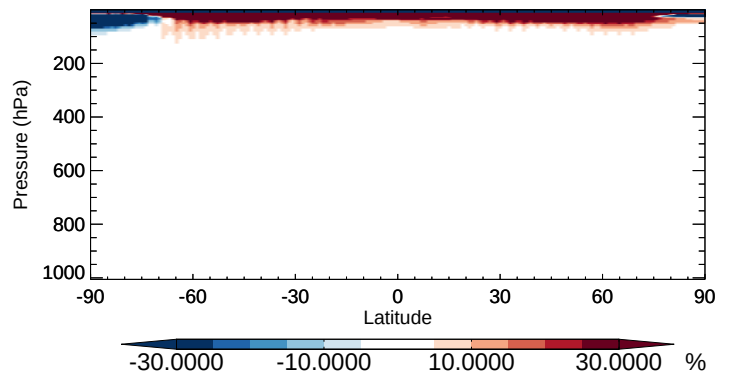
v11-02b-HP / v11-02a CCl4 - Zonal mean % diff for Apr
