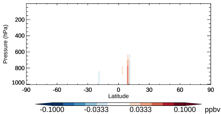
v11-02b-HP - v11-02a HAC - Zonal mean abs diff for Apr
