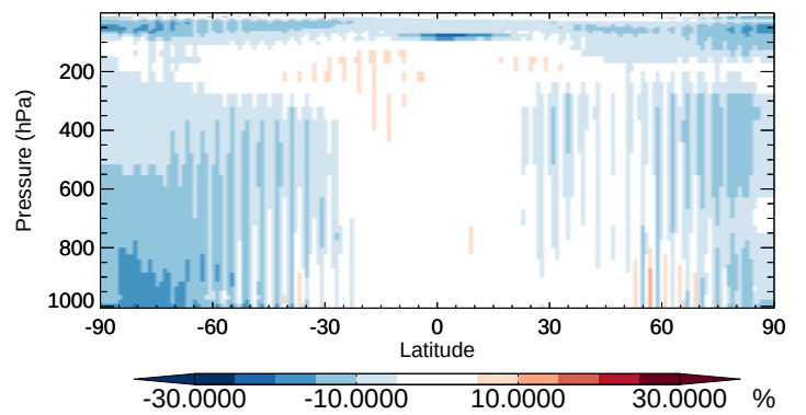
v11-02b-HP / v11-02a CH2O - Zonal mean % diff for Apr
