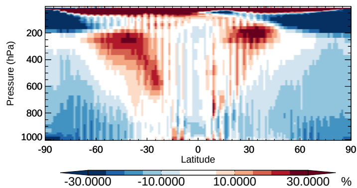
v11-02b-HP / v11-02a RCHO - Zonal mean % diff for Apr
