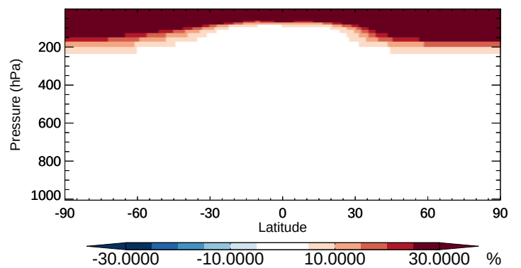
v11-02b-HP / v11-02a CFC114 - Zonal mean % diff for Apr
