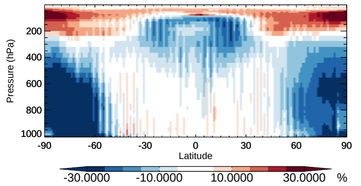
v11-02b-HP / v11-02a HCl - Zonal mean % diff for Apr
