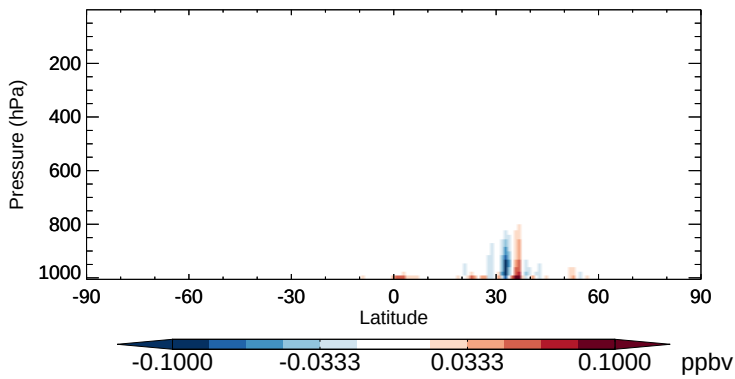
v11-02b-HP - v11-02a XYLE - Zonal mean abs diff for Apr
