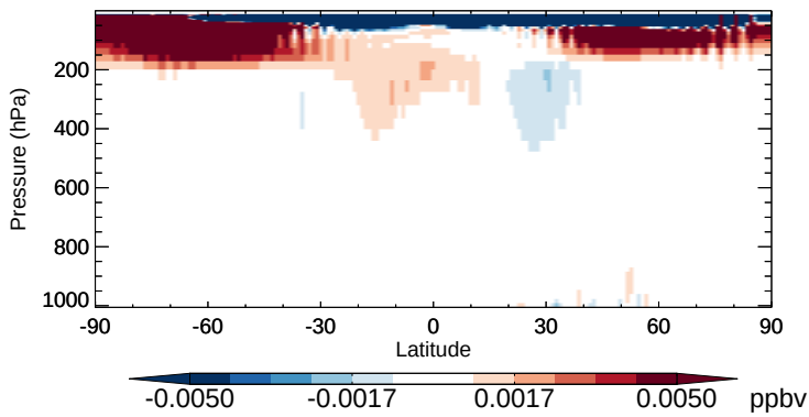
v11-02b-HP - v11-02a N 2 O 5 - Zonal mean abs diff for Apr
