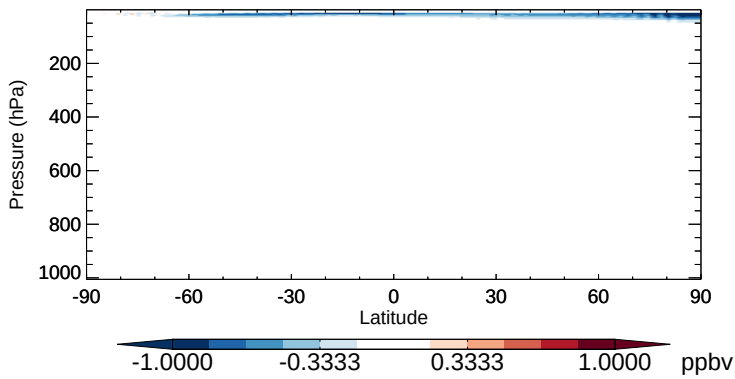
v11-02b-HP - v11-02a NO - Zonal mean abs diff for Apr
