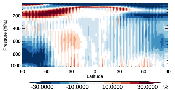
v11-02b-HP / v11-02a TSOG0 - Zonal mean % diff for Apr
