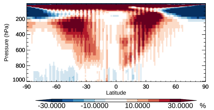
v11-02b-HP / v11-02a BENZ - Zonal mean % diff for Apr
