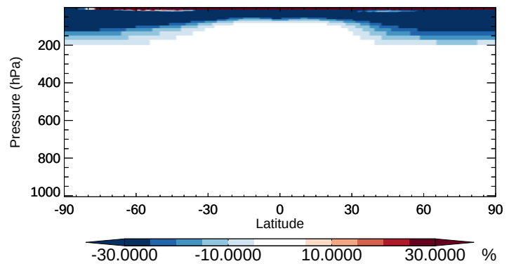
v11-02b-HP / v11-02a HCFC141b - Zonal mean % diff for Apr
