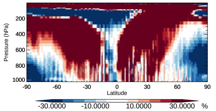
v11-02b-HP / v11-02a IEPOX - Zonal mean % diff for Apr
