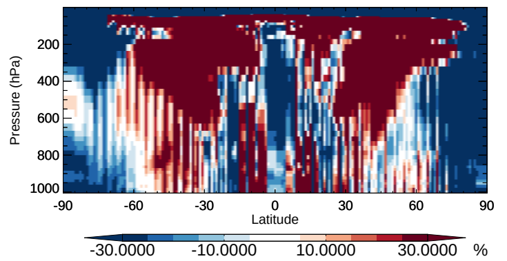
v11-02b-HP / v11-02a RIP - Zonal mean % diff for Apr
