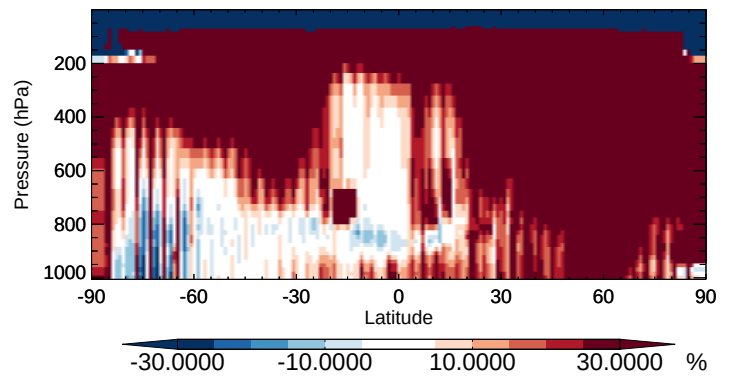
v11-02b-HP / v11-02a SO 4 s - Zonal mean % diff for Apr
