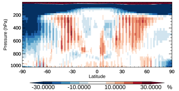
v11-02b-HP / v11-02a SALA - Zonal mean % diff for Apr
