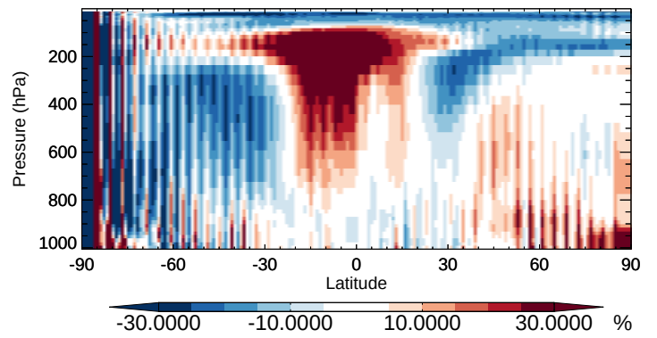
v11-02b-HP / v11-02a NO - Zonal mean % diff for Apr
