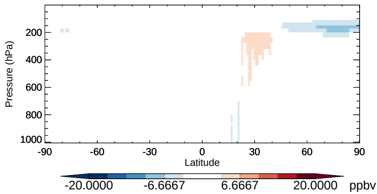
v11-02b-HP - v11-02a CO - Zonal mean abs diff for Apr
