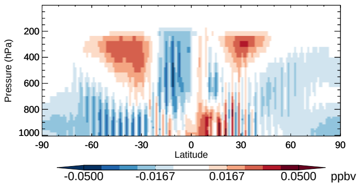
v11-02b-HP - v11-02a MP - Zonal mean abs diff for Apr
