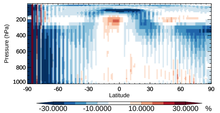
v11-02b-HP / v11-02a Cl - Zonal mean % diff for Apr
