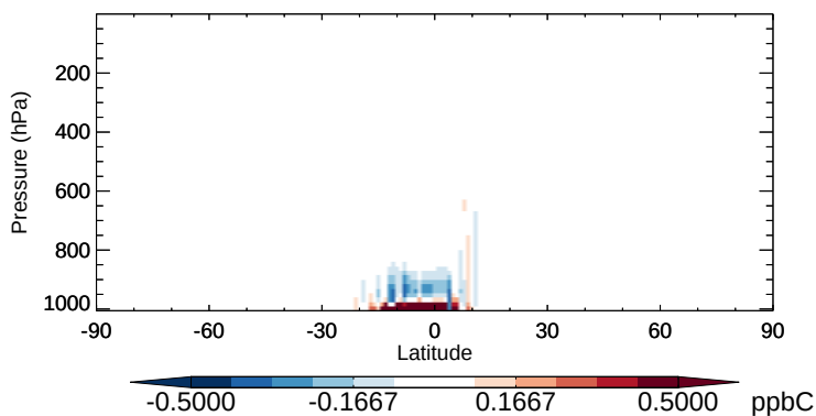
v11-02b-HP - v11-02a ISOP - Zonal mean abs diff for Apr
