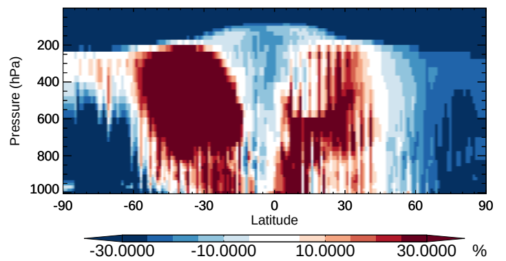
v11-02b-HP / v11-02a TSOA2 - Zonal mean % diff for Apr
