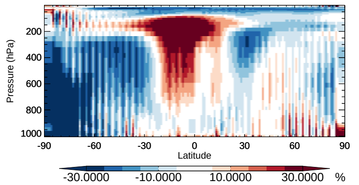
v11-02b-HP / v11-02a NO2 - Zonal mean % diff for Apr
