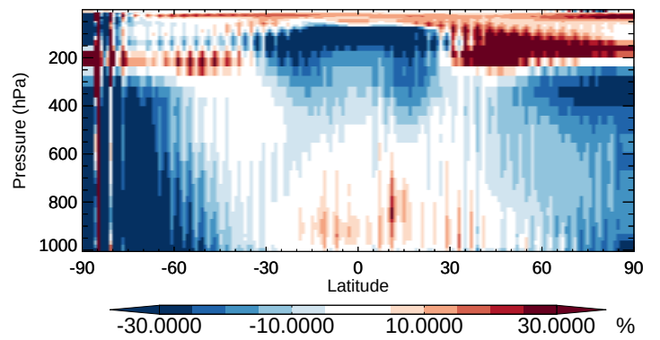
v11-02b-HP / v11-02a ClO - Zonal mean % diff for Apr
