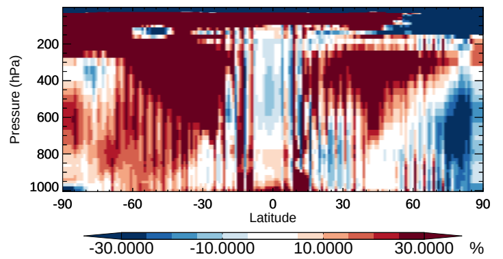
v11-02b-HP / v11-02a PRPE - Zonal mean % diff for Apr
