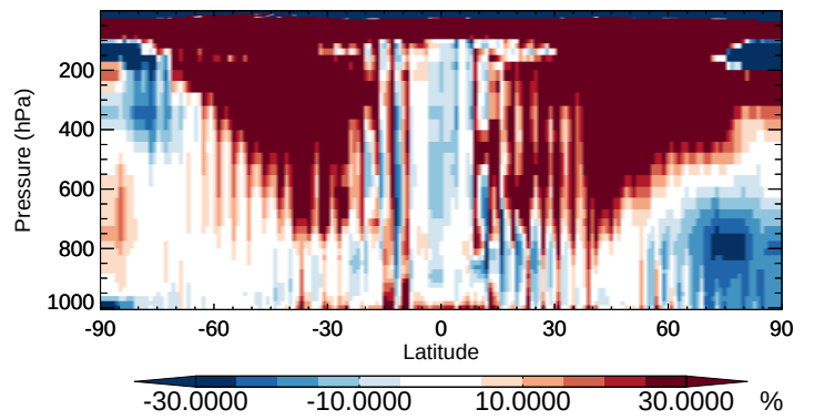
v11-02b-HP / v11-02a XYLE - Zonal mean % diff for Apr
