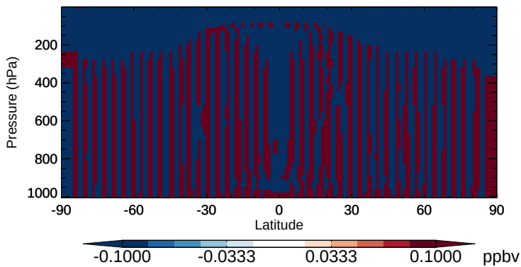
v11-02b-HP - v11-02a H 2 O - Zonal mean abs diff for Apr
