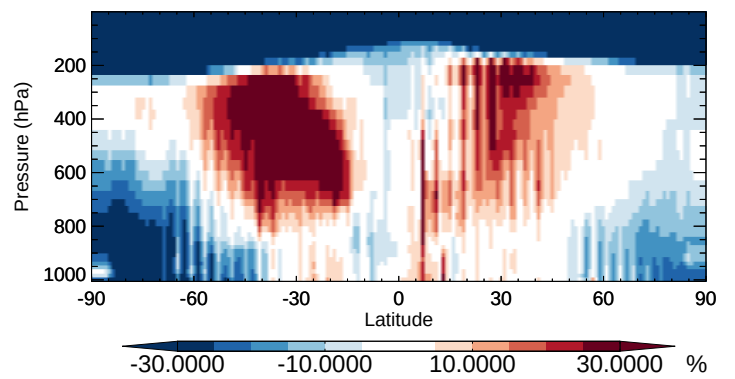
v11-02b-HP / v11-02a OCPI - Zonal mean % diff for Apr
