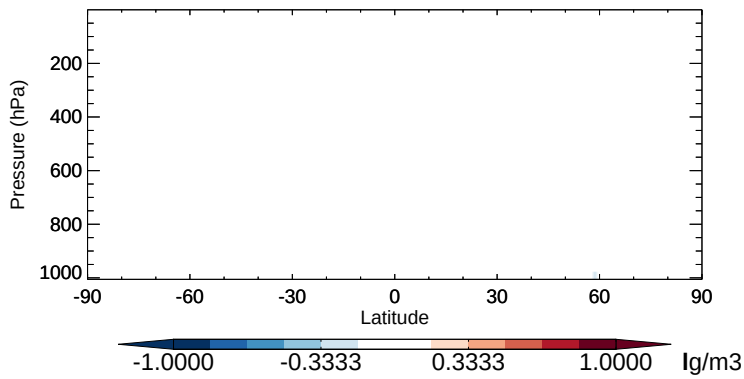
v11-02b-HP - v11-02a NH4 - Zonal mean abs diff for Apr
