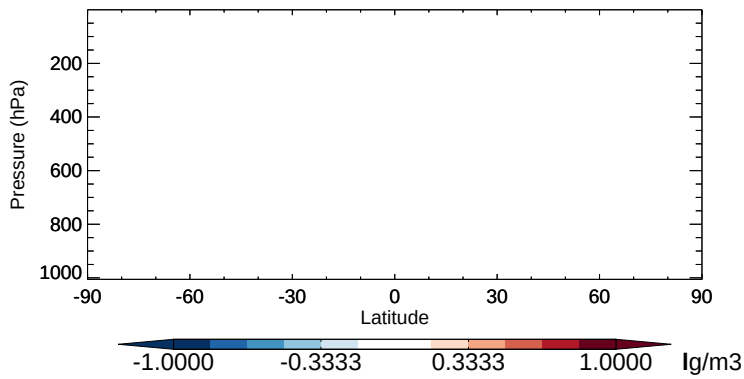
v11-02b-HP - v11-02a DMS - Zonal mean abs diff for Apr
