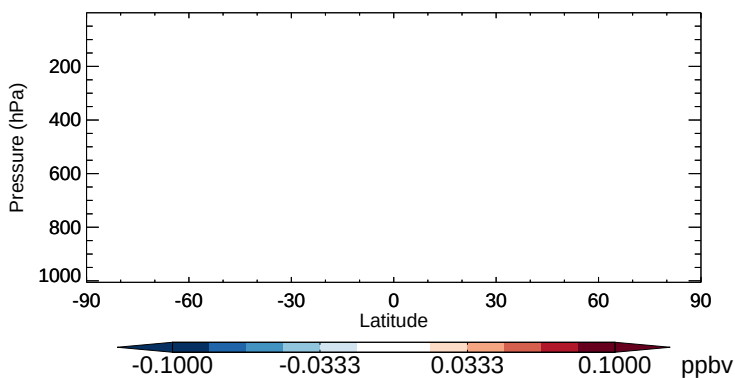
v11-02b-HP - v11-02a TSOG0 - Zonal mean abs diff for Apr
