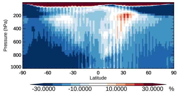
v11-02b-HP / v11-02a C3H8 - Zonal mean % diff for Apr
