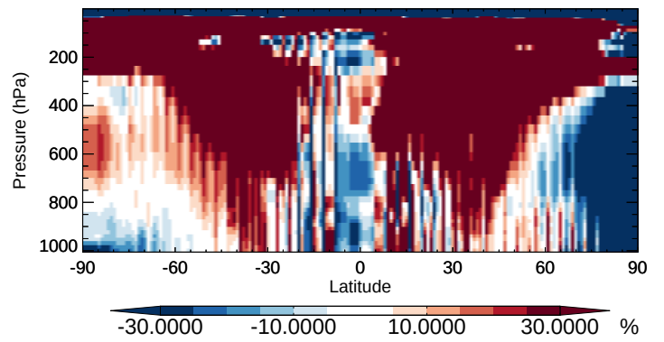
v11-02b-HP / v11-02a MVK - Zonal mean % diff for Apr
