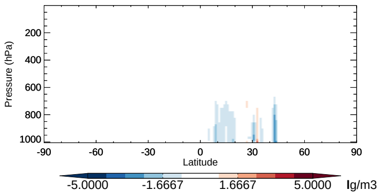
v11-02b-HP - v11-02a DST2 - Zonal mean abs diff for Apr
