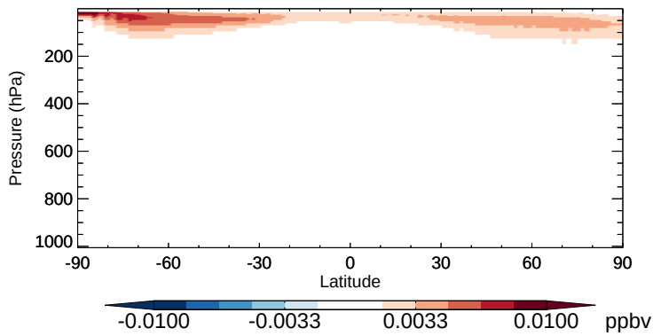
v11-02b-HP - v11-02a BrNO 3 - Zonal mean abs diff for Apr
