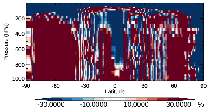
v11-02b-HP / v11-02a MTPA - Zonal mean % diff for Apr
