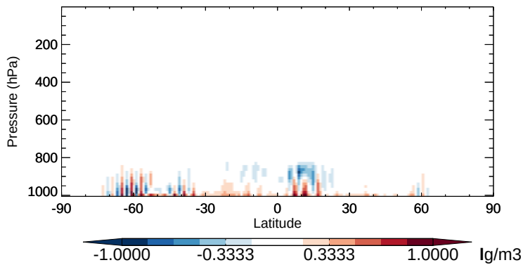
v11-02b-HP - v11-02a SALC - Zonal mean abs diff for Apr
