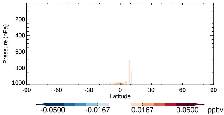
v11-02b-HP - v11-02a MACR - Zonal mean abs diff for Apr
