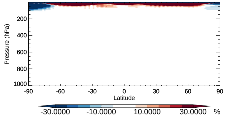
v11-02b-HP / v11-02a H1211 - Zonal mean % diff for Apr
