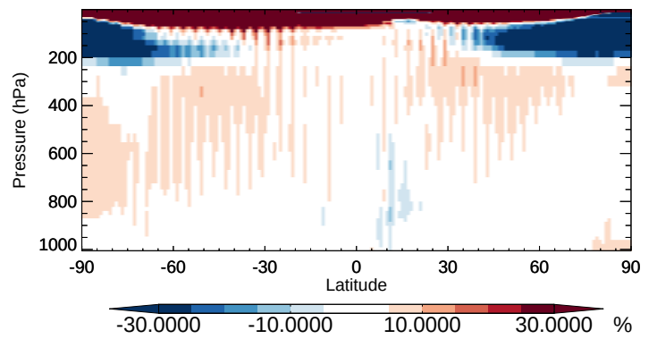
v11-02b-HP / v11-02a CHBr 3 - Zonal mean % diff for Apr
