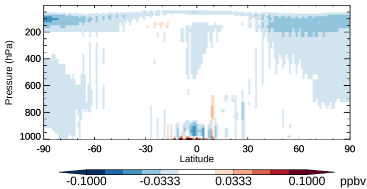
v11-02b-HP - v11-02a EOH - Zonal mean abs diff for Apr
