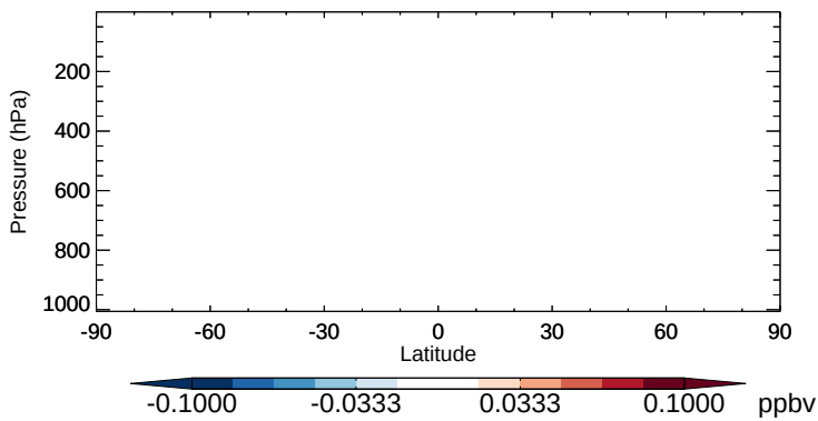
v11-02b-HP - v11-02a H1301 - Zonal mean abs diff for Apr
