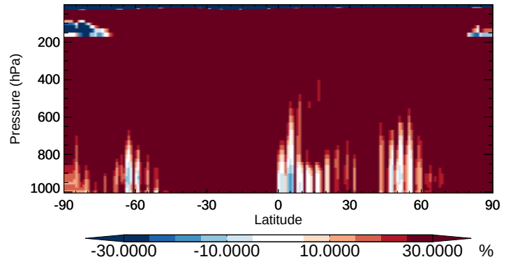
v11-02b-HP / v11-02a DST4 - Zonal mean % diff for Apr
