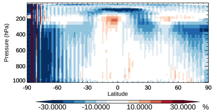
v11-02b-HP / v11-02a C10O - Zonal mean % diff for Apr
