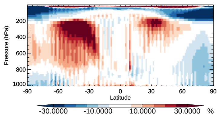
v11-02b-HP / v11-02a ALD2 - Zonal mean % diff for Apr
