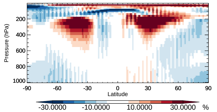
v11-02b-HP / v11-02a MP - Zonal mean % diff for Apr
