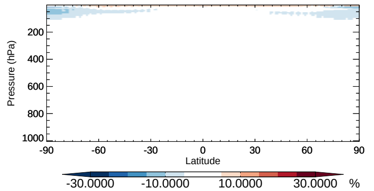
v11-02b-HP / v11-02a CH4 - Zonal mean % diff for Apr
