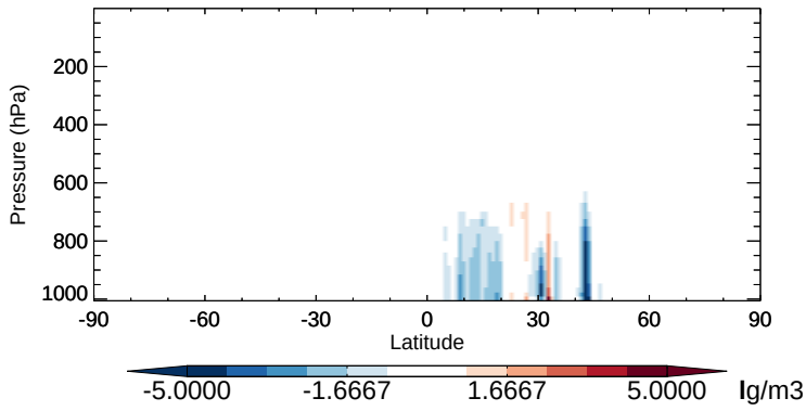
v11-02b-HP - v11-02a DST3 - Zonal mean abs diff for Apr
