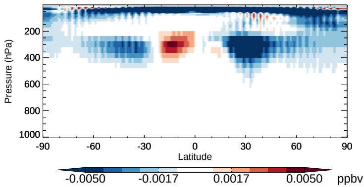
v11-02b-HP - v11-02a HNO 4 - Zonal mean abs diff for Apr
