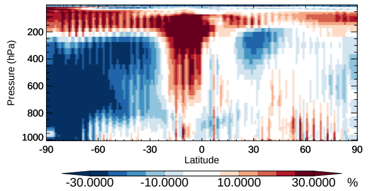
v11-02b-HP / v11-02a BrNO 2 - Zonal mean % diff for Apr
