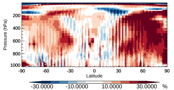
v11-02b-HP / v11-02a SO 2 - Zonal mean % diff for Apr
