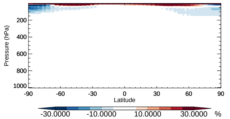
v11-02b-HP / v11-02a CH3Cl - Zonal mean % diff for Apr
