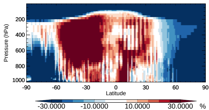
v11-02b-HP / v11-02a ISOA2 - Zonal mean % diff for Apr
