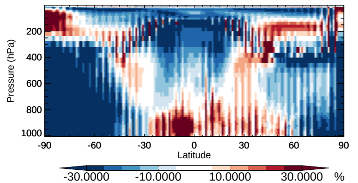
v11-02b-HP / v11-02a BrCl - Zonal mean % diff for Apr
