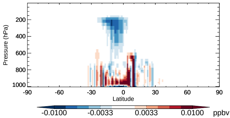
v11-02b-HP - v11-02a IEPOX - Zonal mean abs diff for Apr
