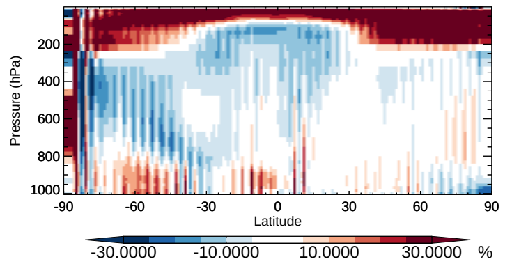
v11-02b-HP / v11-02a BrO - Zonal mean % diff for Apr
