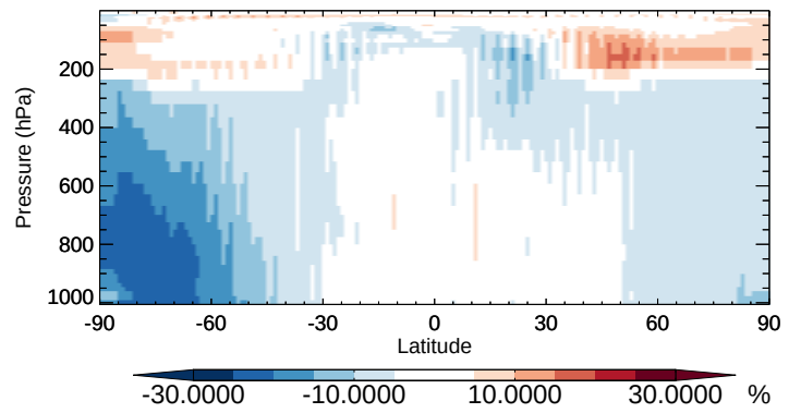
v11-02b-HP / v11-02a O3 - Zonal mean % diff for Apr
