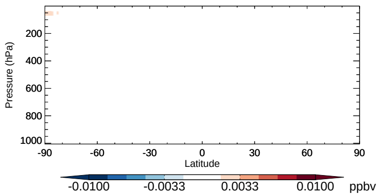
v11-02b-HP - v11-02a HOBr - Zonal mean abs diff for Apr
