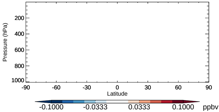
v11-02b-HP - v11-02a H1211 - Zonal mean abs diff for Apr
