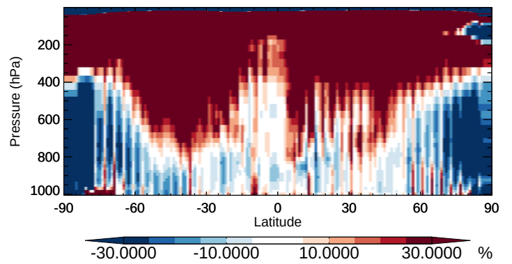
v11-02b-HP / v11-02a BCPO - Zonal mean % diff for Apr
