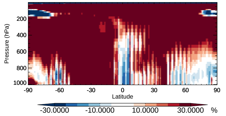
v11-02b-HP / v11-02a DST3 - Zonal mean % diff for Apr
