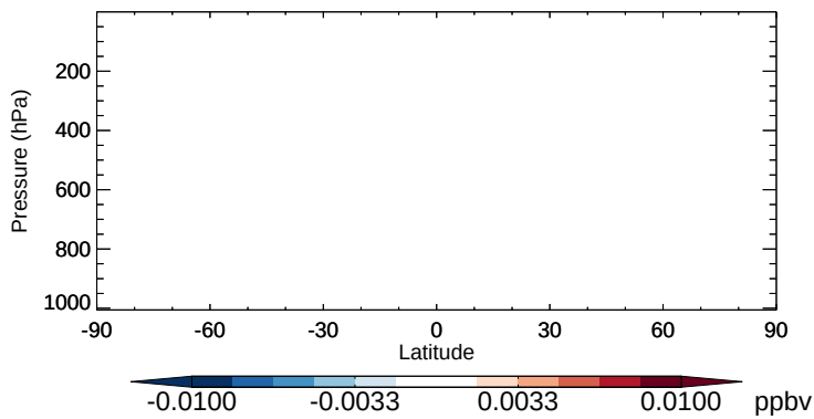
v11-02b-HP - v11-02a HBr - Zonal mean abs diff for Apr
