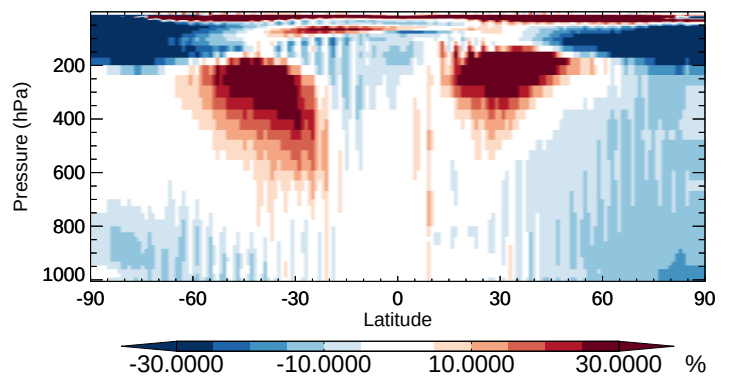
v11-02b-HP / v11-02a MAP - Zonal mean % diff for Apr
