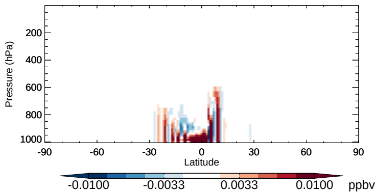
v11-02b-HP - v11-02a RIP - Zonal mean abs diff for Apr
