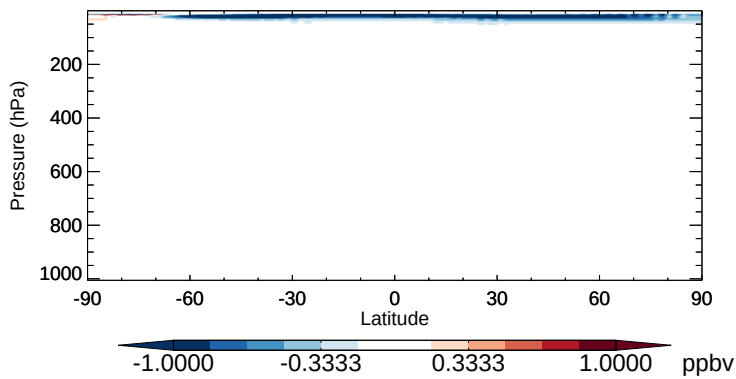
v11-02b-HP - v11-02a NO2 - Zonal mean abs diff for Apr
