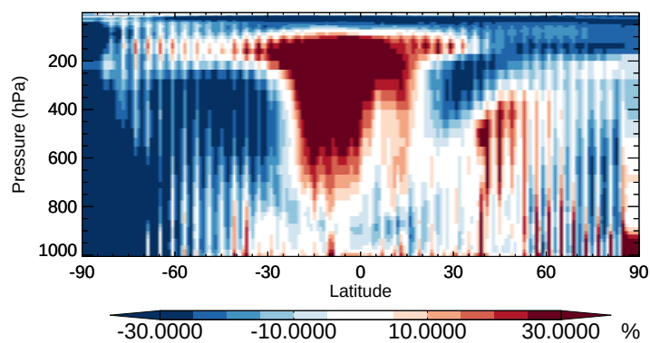
v11-02b-HP / v11-02a HNO 2 - Zonal mean % diff for Apr
