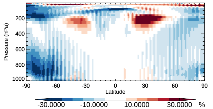
v11-02b-HP / v11-02a H 2 O 2 - Zonal mean % diff for Apr
