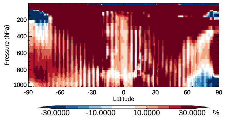
v11-02b-HP / v11-02a DMS - Zonal mean % diff for Apr
