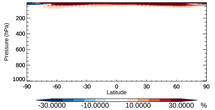
v11-02b-HP / v11-02a CFC12 - Zonal mean % diff for Apr
