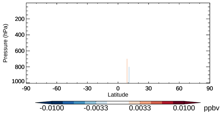
v11-02b-HP - v11-02a MVKN - Zonal mean abs diff for Apr
