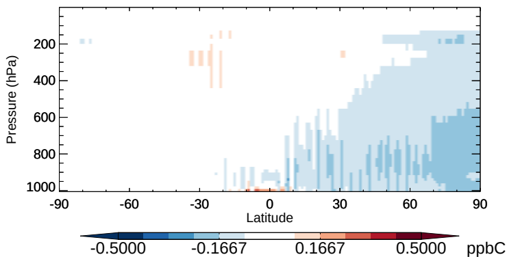
v11-02b-HP - v11-02a ACET - Zonal mean abs diff for Apr
