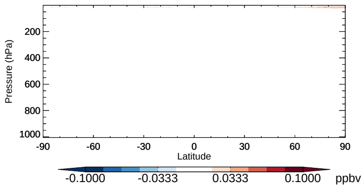
v11-02b-HP - v11-02a ClO - Zonal mean abs diff for Apr
