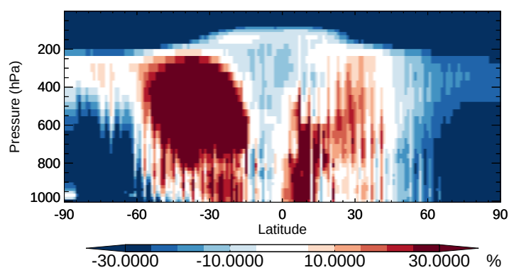
v11-02b-HP / v11-02a ISOA1 - Zonal mean % diff for Apr
