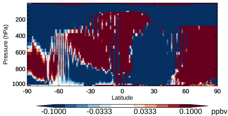
v11-02b-HP - v11-02a CH4 - Zonal mean abs diff for Apr
