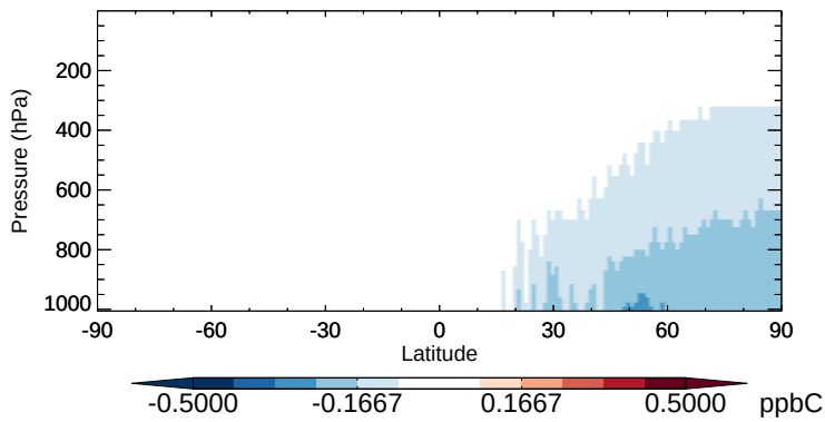
v11-02b-HP - v11-02a C3H8 - Zonal mean abs diff for Apr
