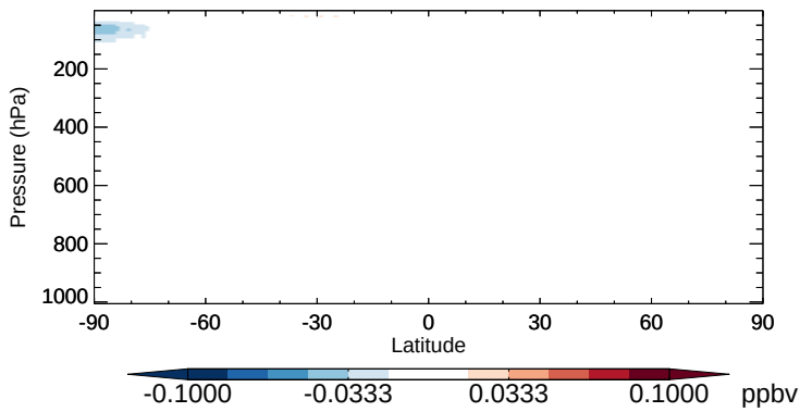
v11-02b-HP - v11-02a HOCl - Zonal mean abs diff for Apr
