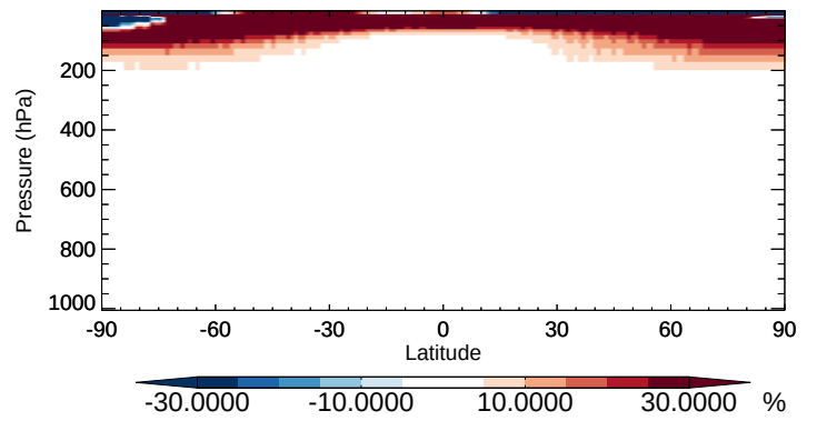
v11-02b-HP / v11-02a CH 3 CCl 3 - Zonal mean % diff for Apr
