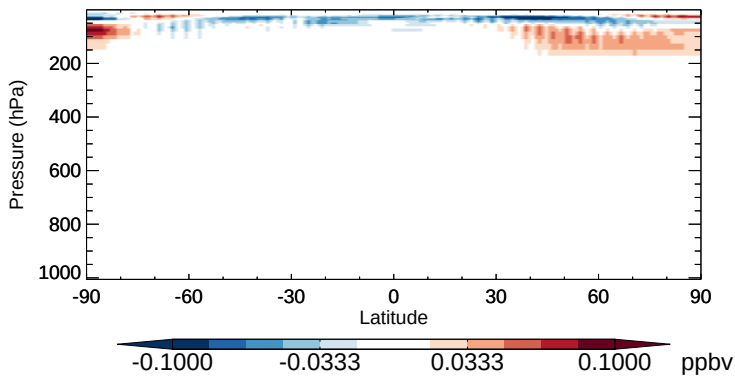
v11-02b-HP - v11-02a ClNO3 - Zonal mean abs diff for Apr
