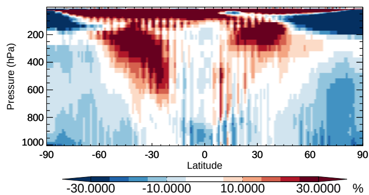
v11-02b-HP / v11-02a MEK - Zonal mean % diff for Apr
