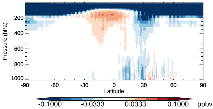
v11-02b-HP - v11-02a HNO 3 - Zonal mean abs diff for Apr
