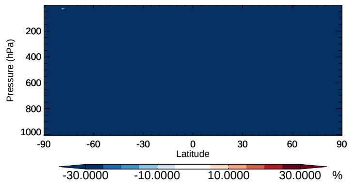
v11-02b-HP / v11-02a ClNO2 - Zonal mean % diff for Apr
