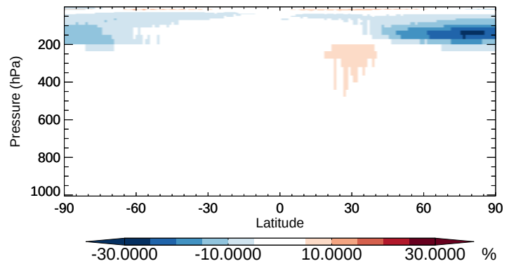
v11-02b-HP / v11-02a CO - Zonal mean % diff for Apr
