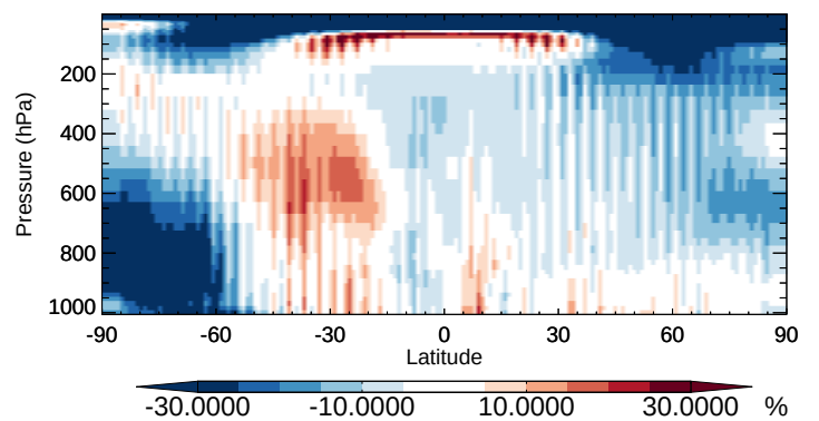
v11-02b-HP / v11-02a TSOG1 - Zonal mean % diff for Apr
