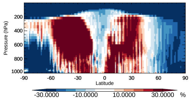
v11-02b-HP / v11-02a TSOA3 - Zonal mean % diff for Apr
