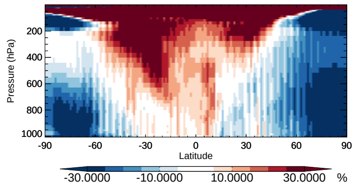
v11-02b-HP / v11-02a PROPNN - Zonal mean % diff for Apr
