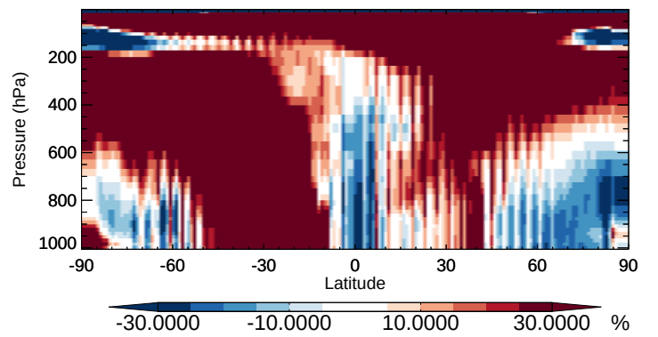
v11-02b-HP / v11-02a DST2 - Zonal mean % diff for Apr
