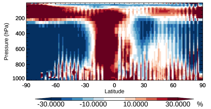
v11-02b-HP / v11-02a N 2 O 5 - Zonal mean % diff for Apr
