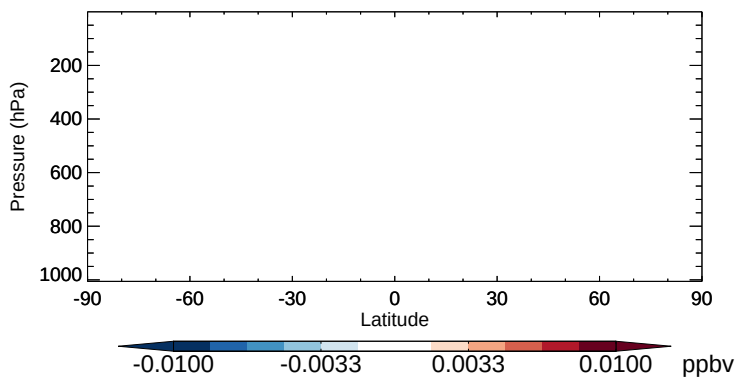
v11-02b-HP - v11-02a Br2 - Zonal mean abs diff for Apr
