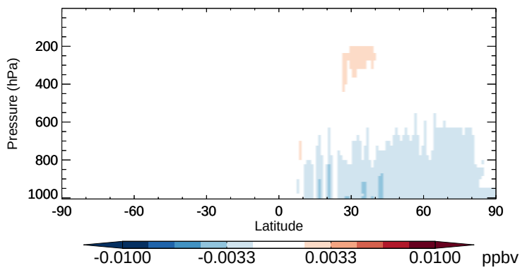
v11-02b-HP - v11-02a R4N2 - Zonal mean abs diff for Apr
