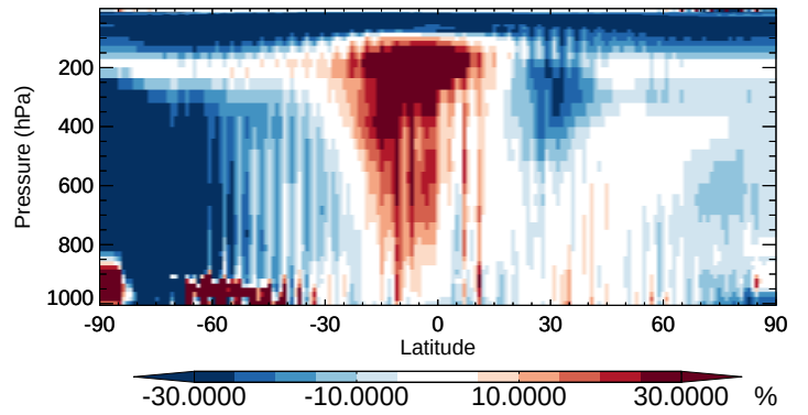
v11-02b-HP / v11-02a HNO 3 - Zonal mean % diff for Apr
