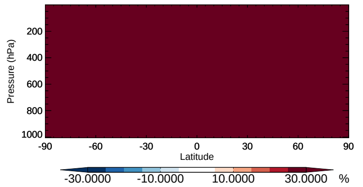
v11-02b-HP / v11-02a HCFC123 - Zonal mean % diff for Apr
