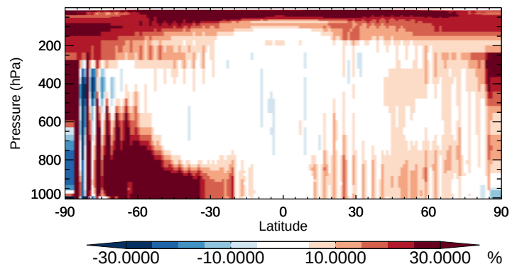
v11-02b-HP / v11-02a HBr - Zonal mean % diff for Apr
