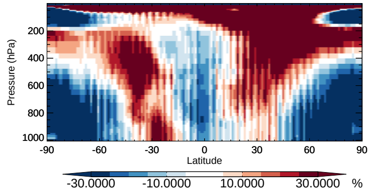
v11-02b-HP / v11-02a DST1 - Zonal mean % diff for Apr
