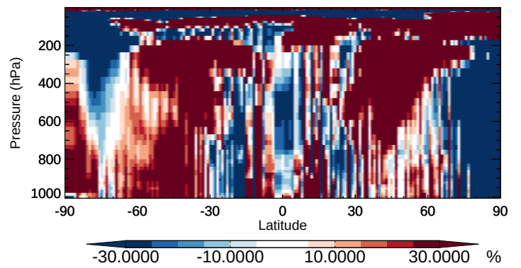
v11-02b-HP / v11-02a MOBA - Zonal mean % diff for Apr
