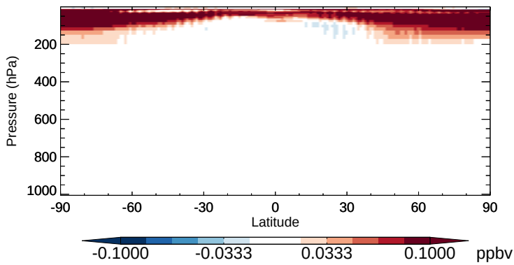
v11-02b-HP - v11-02a HCl - Zonal mean abs diff for Apr
