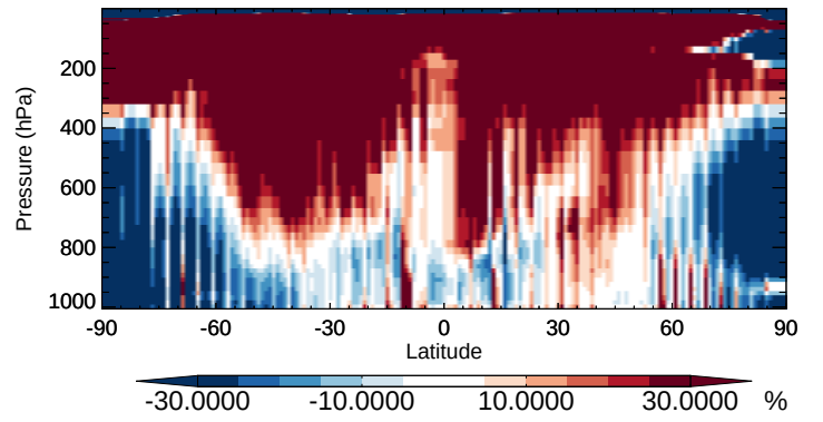
v11-02b-HP / v11-02a OCPO - Zonal mean % diff for Apr
