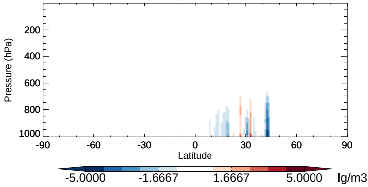
v11-02b-HP - v11-02a DST4 - Zonal mean abs diff for Apr
