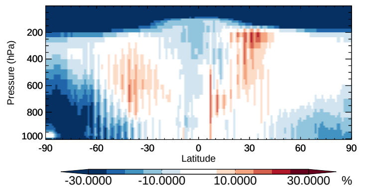
v11-02b-HP / v11-02a ASOAN - Zonal mean % diff for Apr
