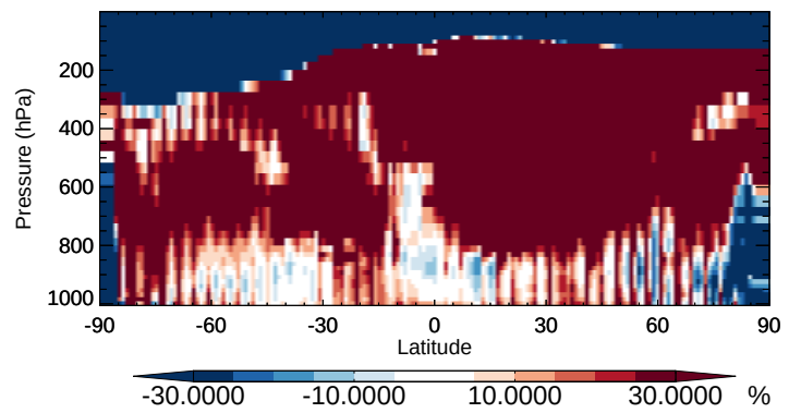
v11-02b-HP / v11-02a NH 3 - Zonal mean % diff for Apr
