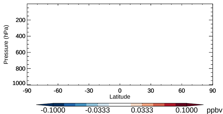
v11-02b-HP - v11-02a ISOA2 - Zonal mean abs diff for Apr
