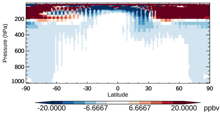
v11-02b-HP - v11-02a O3 - Zonal mean abs diff for Apr
