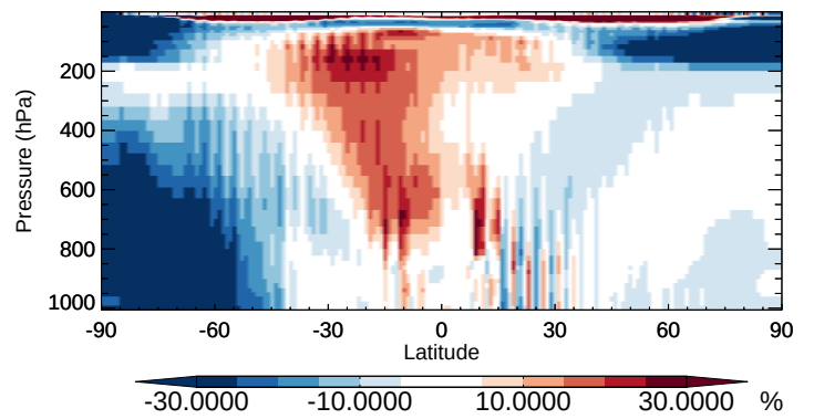
v11-02b-HP / v11-02a PAN - Zonal mean % diff for Apr
