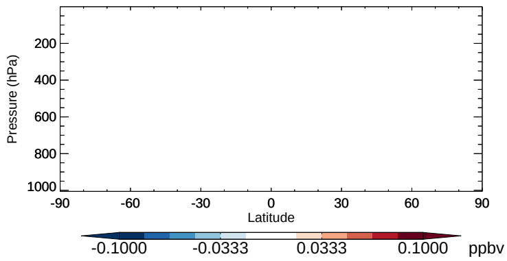
v11-02b-HP - v11-02a MGLY - Zonal mean abs diff for Apr
