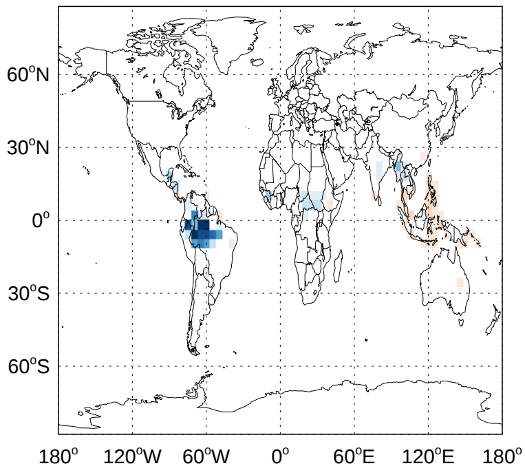
v11-02f-Run0 - v11-02e-Run0 ALD2 biogenic emissions for Apr
