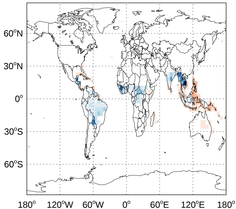
v11-02f-Run0 - v11-02e-Run1 ALD2 biogenic emissions for Apr
