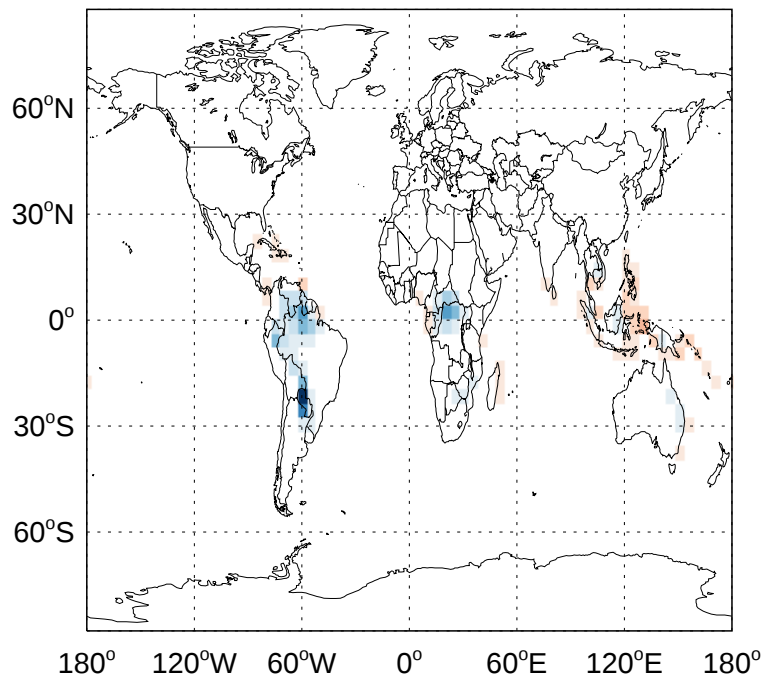
v11-02f-Run0 - v11-02e-Run1 ALD2 biogenic emissions for Jan
