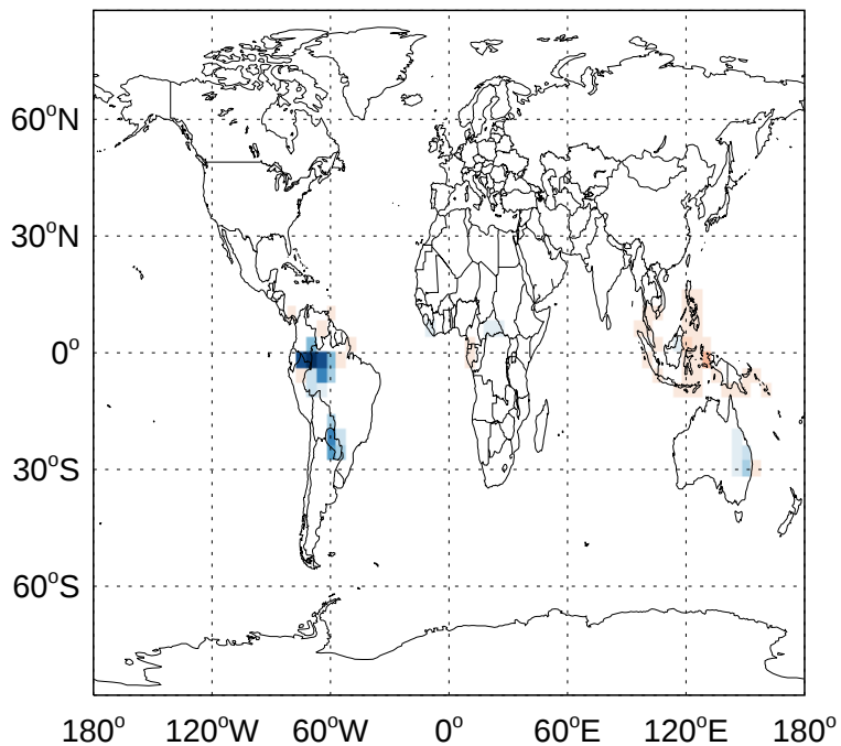
v11-02f-Run0 - v11-02e-Run0 ALD2 biogenic emissions for Jan
