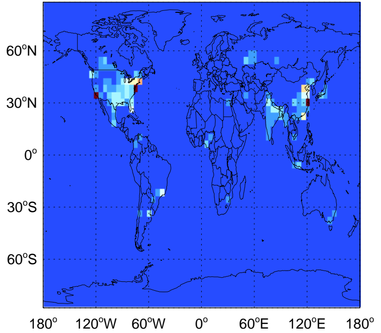
MEK column anth+biofl emissions for Jul
