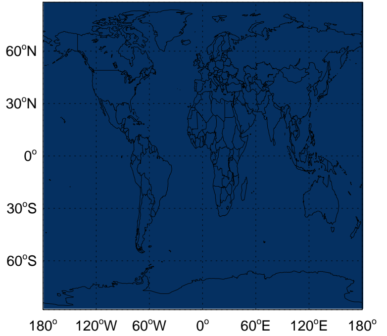
v11-02f-Run1 - v11-02e-Run1 CHBr3 biogenic emissions for Apr
