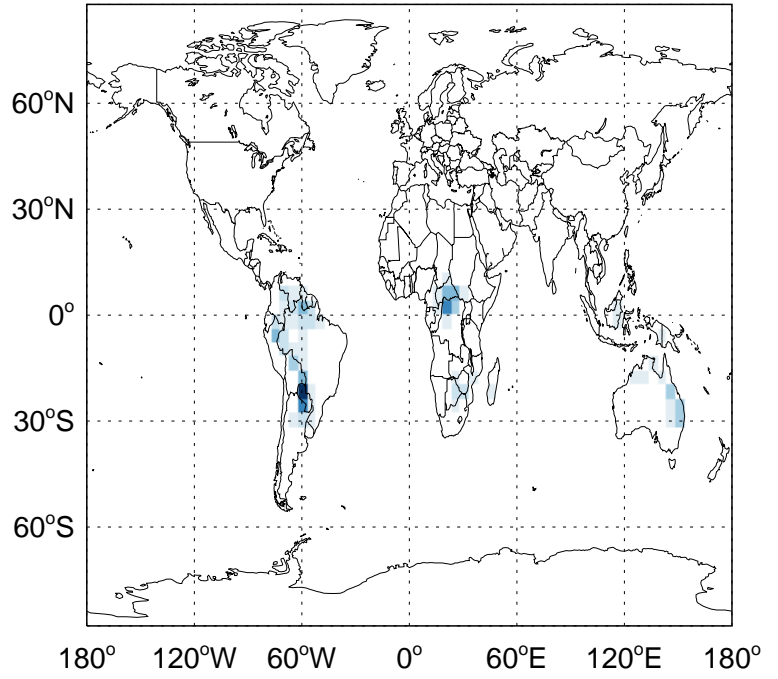
v11-02f-Run1 - v11-02e-Run1 ISOP biogenic emissions for Jan
