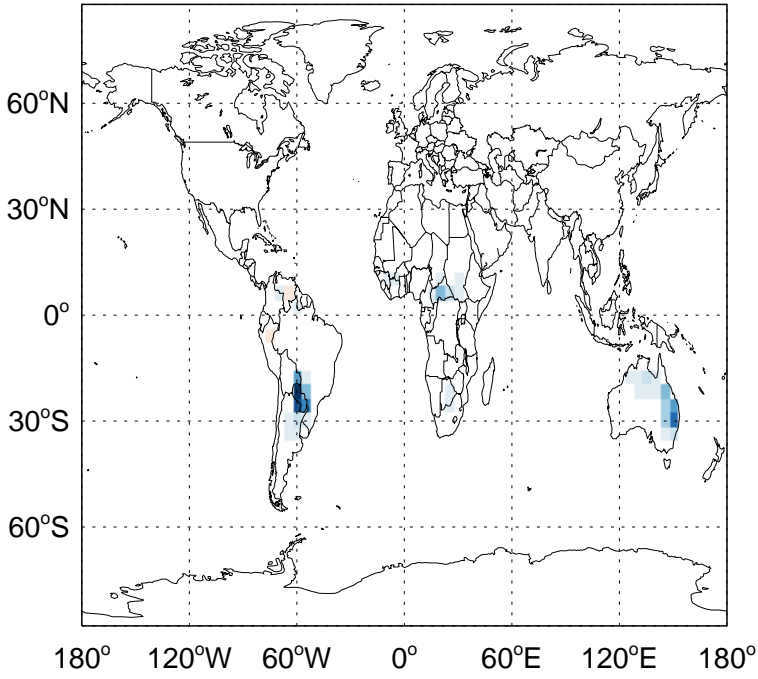
v11-02f-Run1 - v11-02e-Run0 ISOP biogenic emissions for Jan
