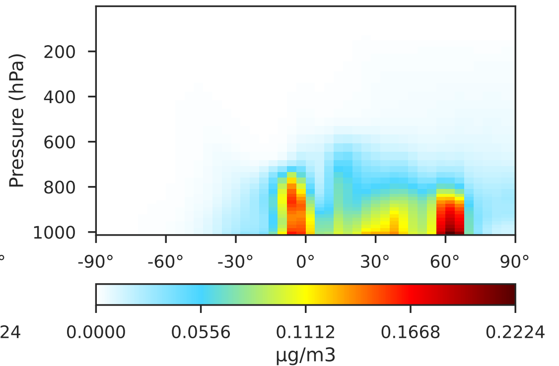
Cloud-J in 14.3.0 (Dev) 4.0x5.0
