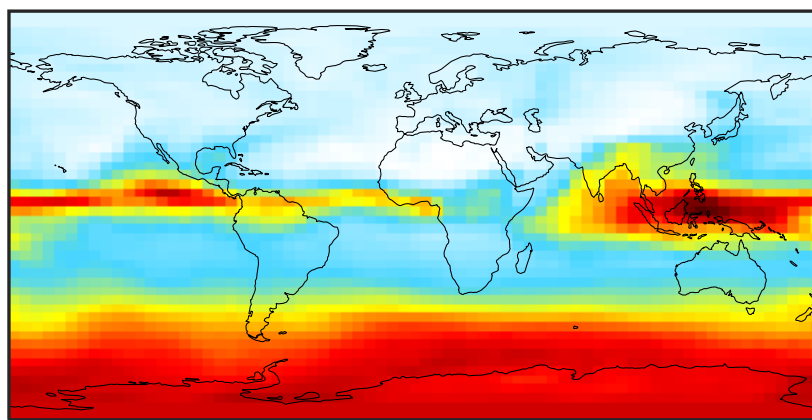
Cloud-J in 14.3.0 (Dev) 4.0x5.0
