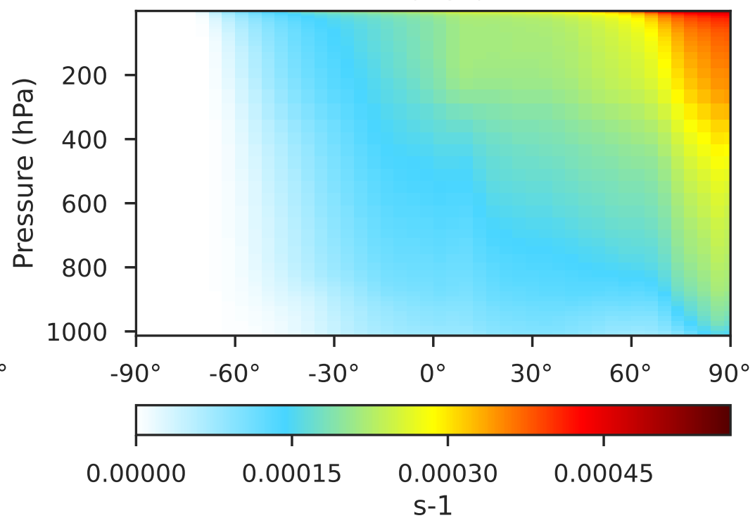
Cloud-J in 14.3.0 (Dev) 4.0x5.0
