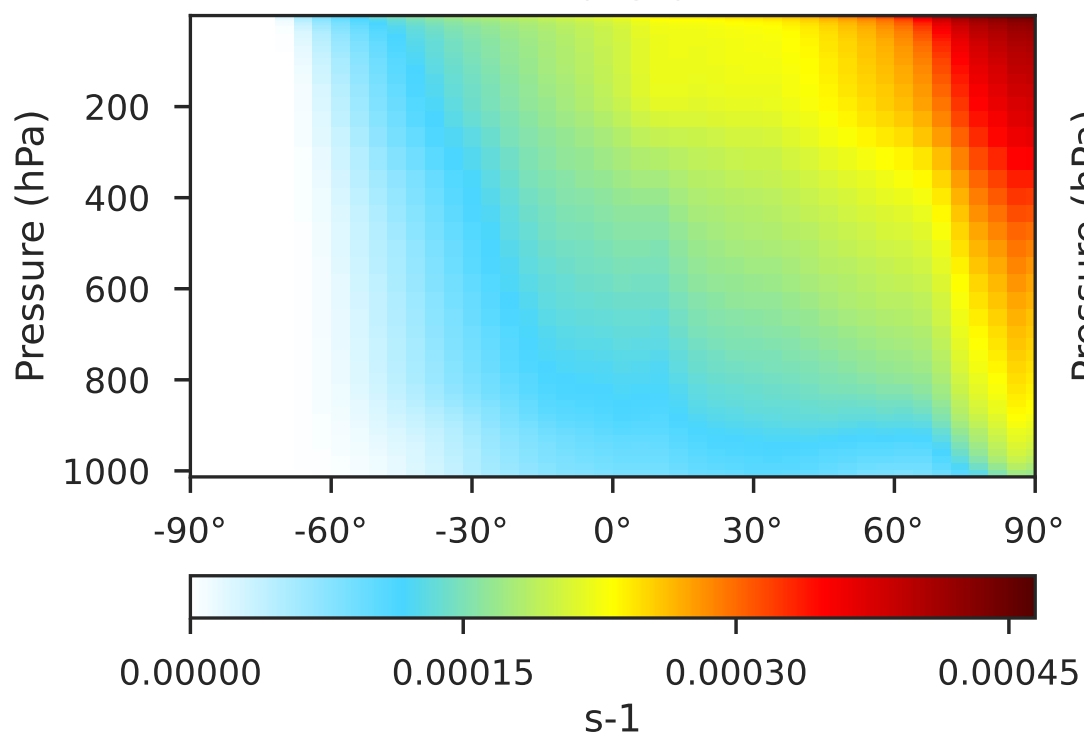
Fast-JX in 14.3.0 (Ref) 4.0x5.0
