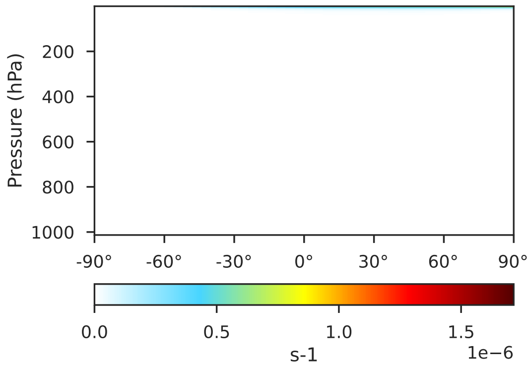
Fast-JX in 14.3.0 (Ref) 4.0x5.0
