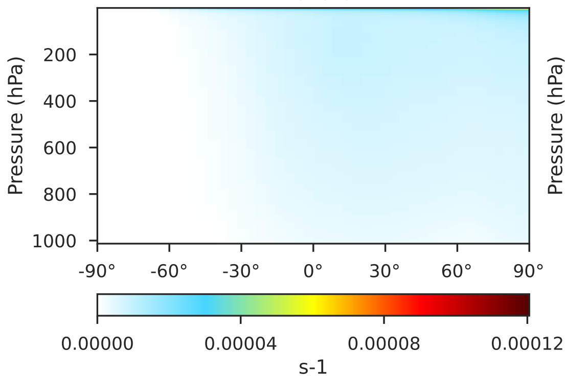
Fast-JX in 14.3.0 (Ref) 4.0x5.0
