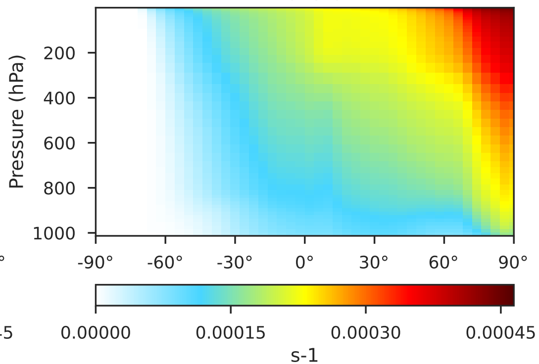
Cloud-J in 14.3.0 (Dev) 4.0x5.0
