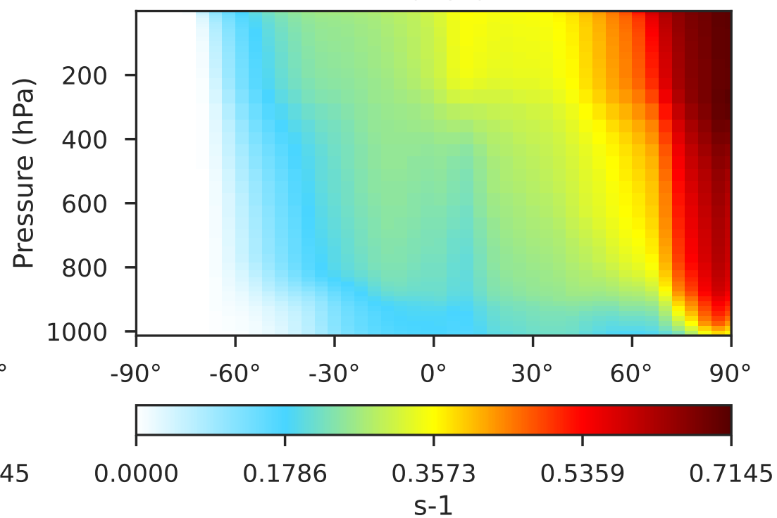
Cloud-J in 14.3.0 (Dev) 4.0x5.0
