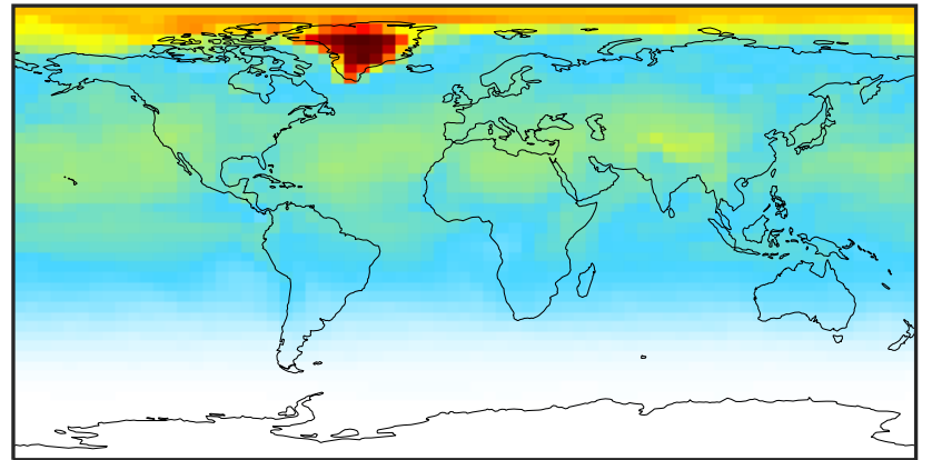
Cloud-J in 14.3.0 (Dev) 4.0x5.0
