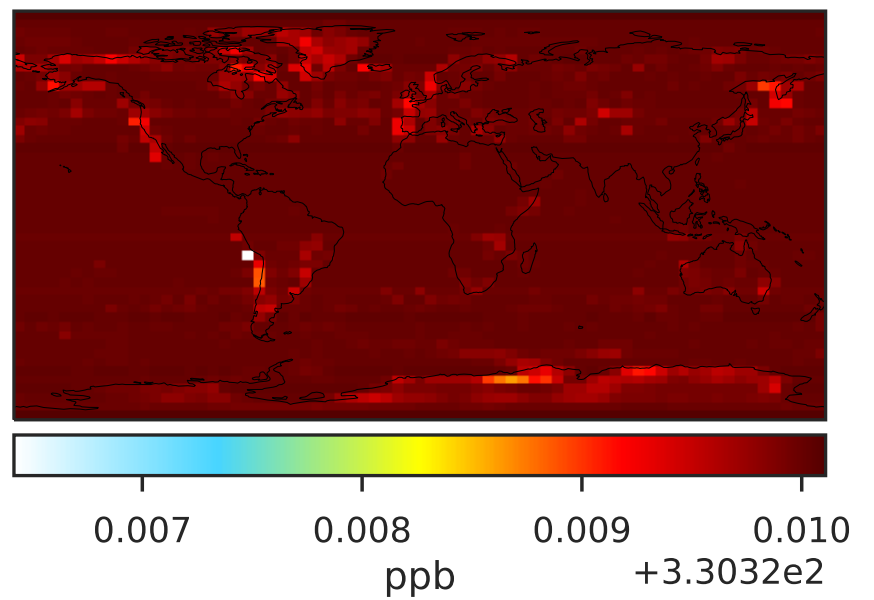
Cloud-J in 14.3.0 (Dev) 4.0x5.0
