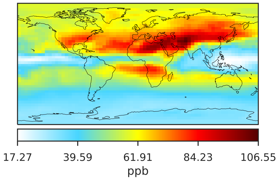
Fast-JX in 14.3.0 (Ref) 4.0x5.0
