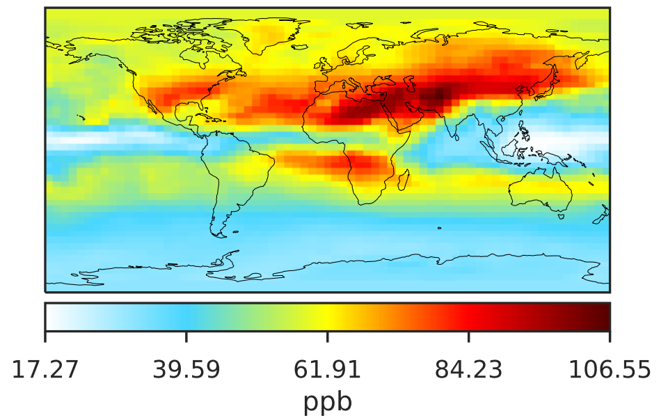
Cloud-J in 14.3.0 (Dev) 4.0x5.0
