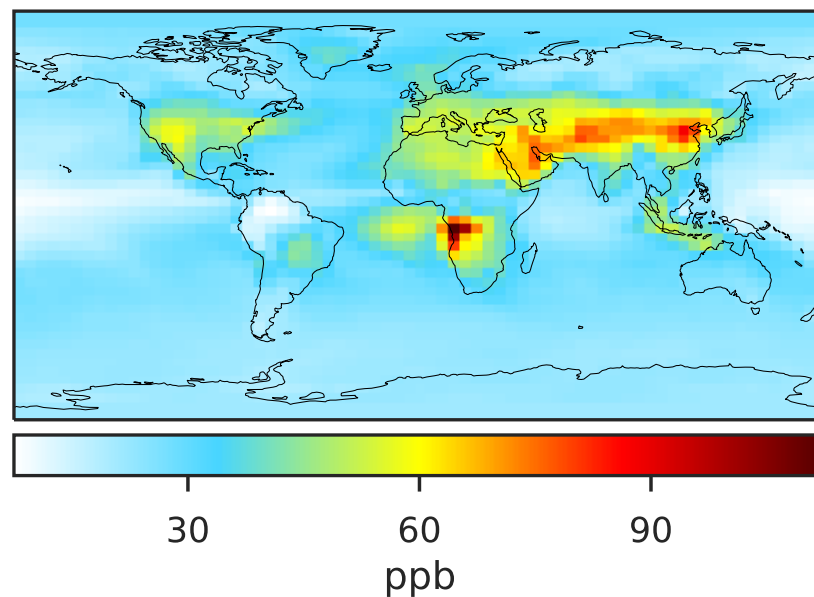
Cloud-J in 14.3.0 (Dev) 4.0x5.0
