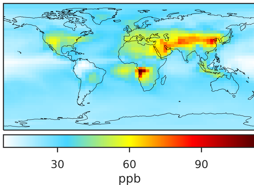
Fast-JX in 14.3.0 (Ref) 4.0x5.0
