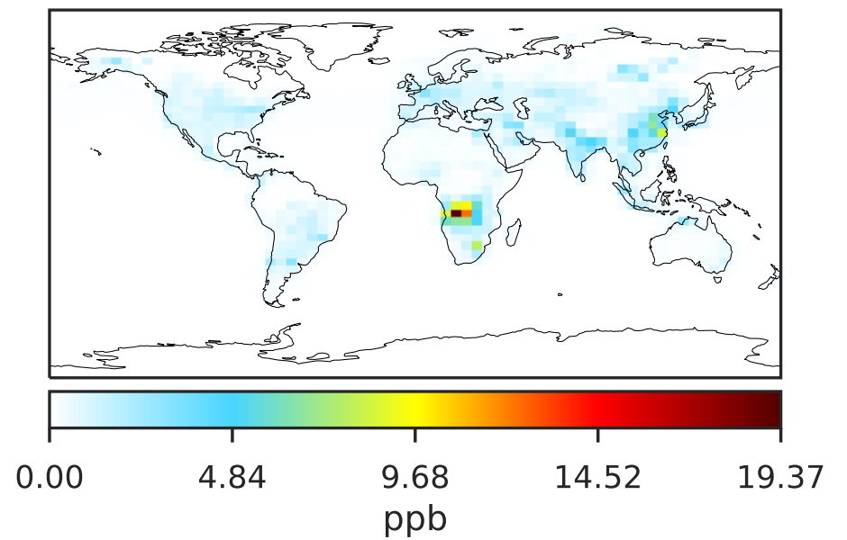
Cloud-J in 14.3.0 (Dev) 4.0x5.0
