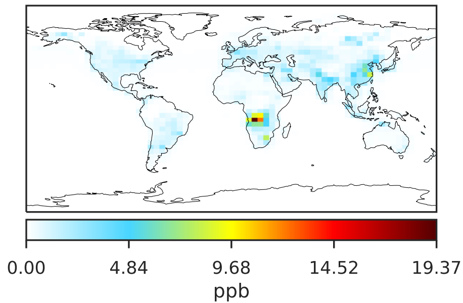
Fast-JX in 14.3.0 (Ref) 4.0x5.0
