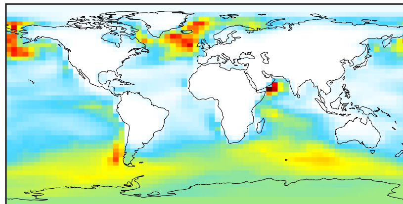
Cloud-J in 14.3.0 (Dev) 4.0x5.0
