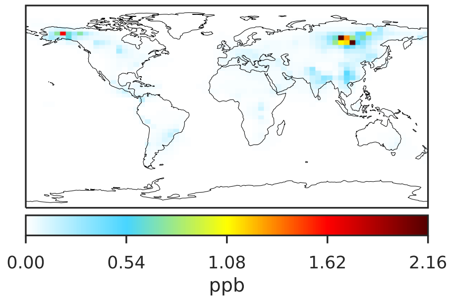
Fast-JX in 14.3.0 (Ref) 4.0x5.0
