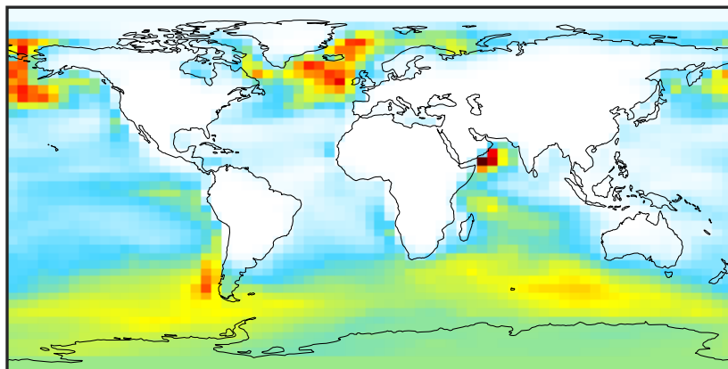
Fast-JX in 14.3.0 (Ref) 4.0x5.0
