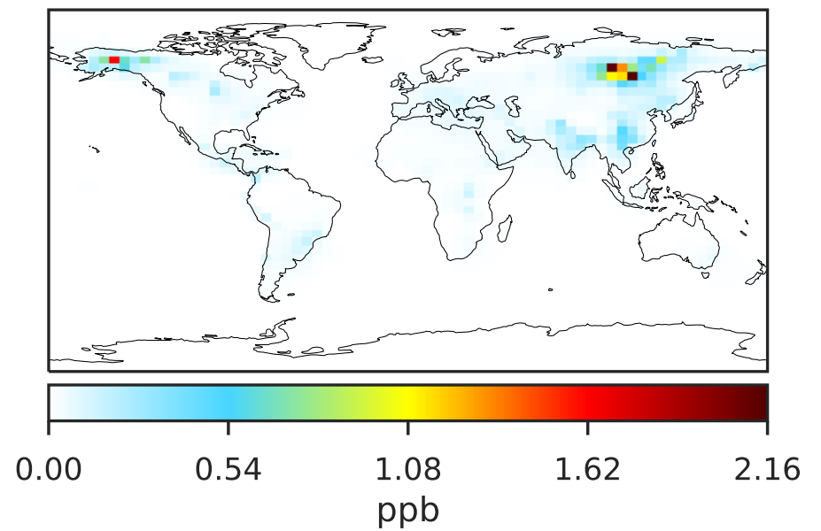
Cloud-J in 14.3.0 (Dev) 4.0x5.0
