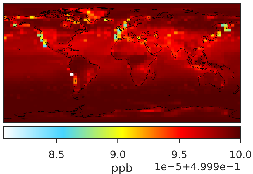
Fast-JX in 14.3.0 (Ref) 4.0x5.0
