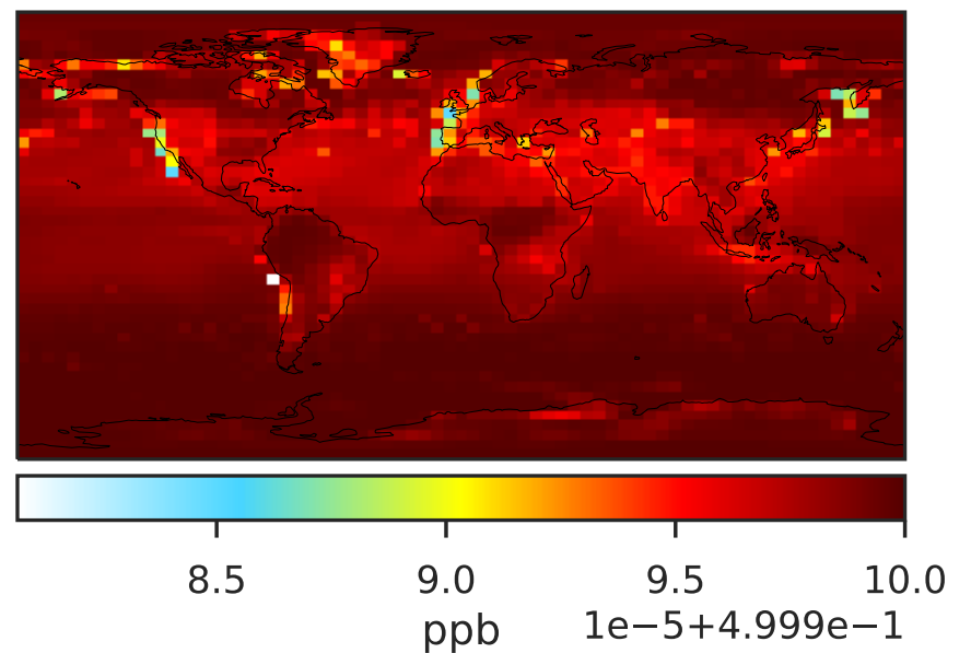
Cloud-J in 14.3.0 (Dev) 4.0x5.0
