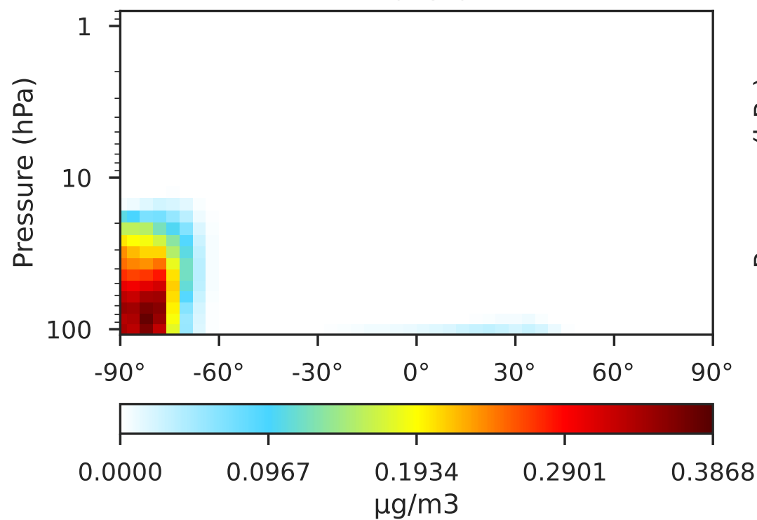
Cloud-J in 14.3.0 (Ref) 4.0x5.0
