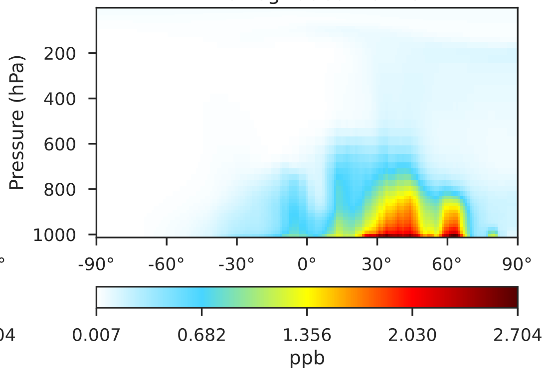
Cloud-J in 14.3.0 (Dev) 1x1.25 regrided from c24
