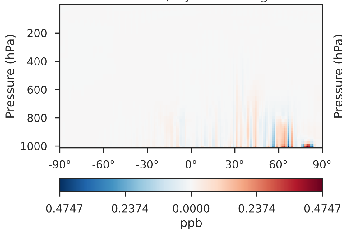
Difference (1x1.25) Dev - Ref, Dynamic Range
