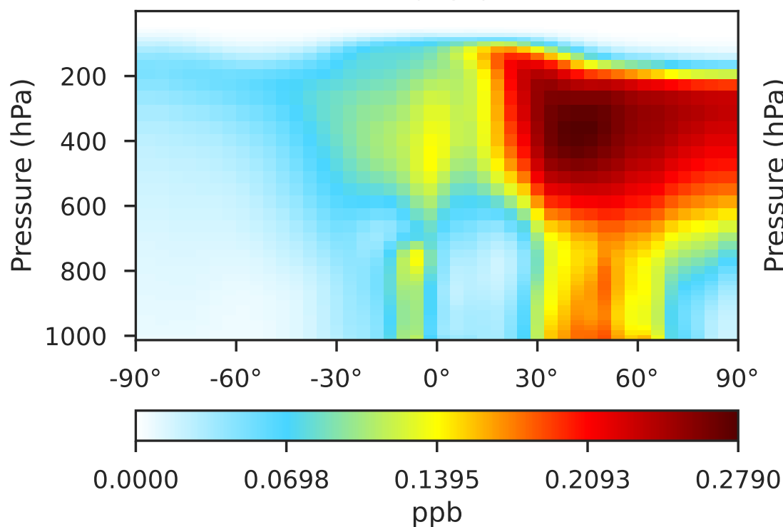
Cloud-J in 14.3.0 (Ref) 4.0x5.0
