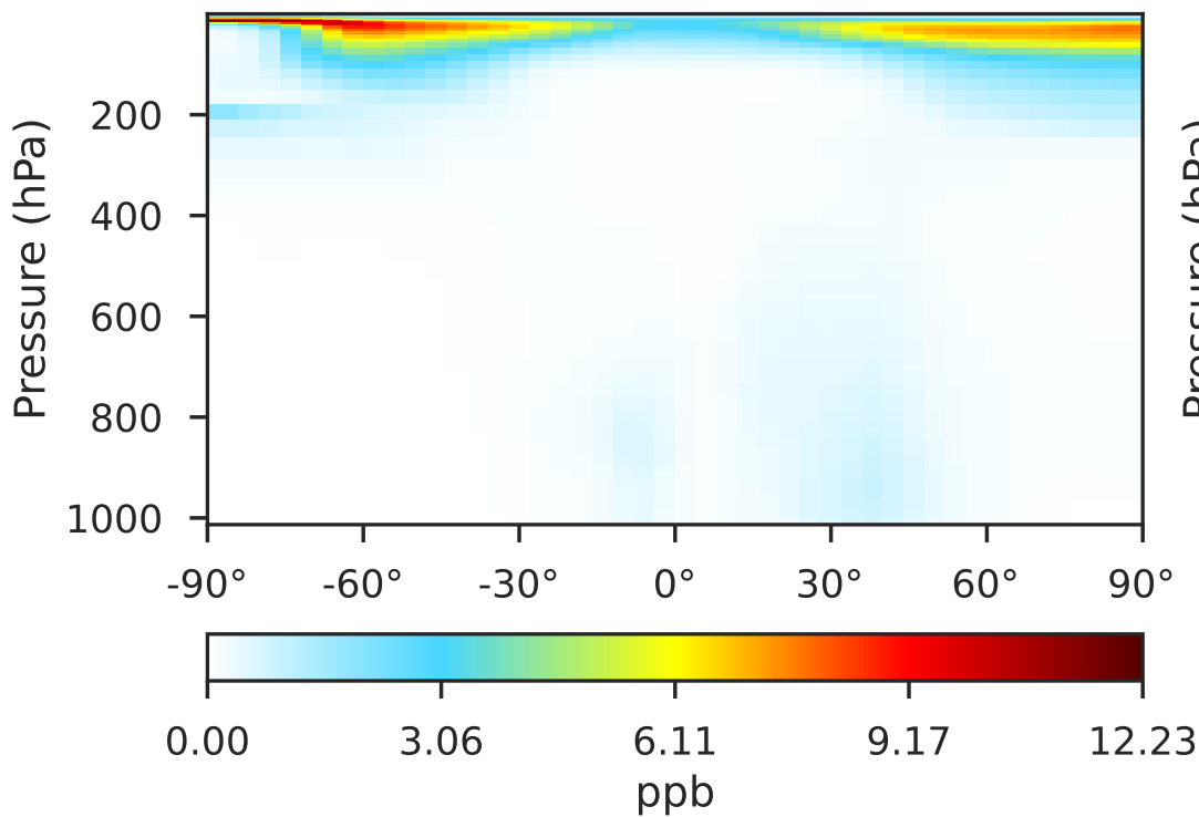
Cloud-J in 14.3.0 (Ref) 4.0x5.0
