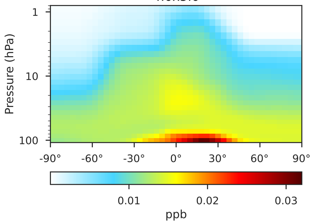
Cloud-J in 14.3.0 (Ref) 4.0x5.0
