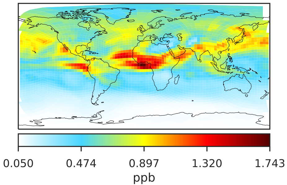
Fast-JX in 14.3.0 (Ref) c24
