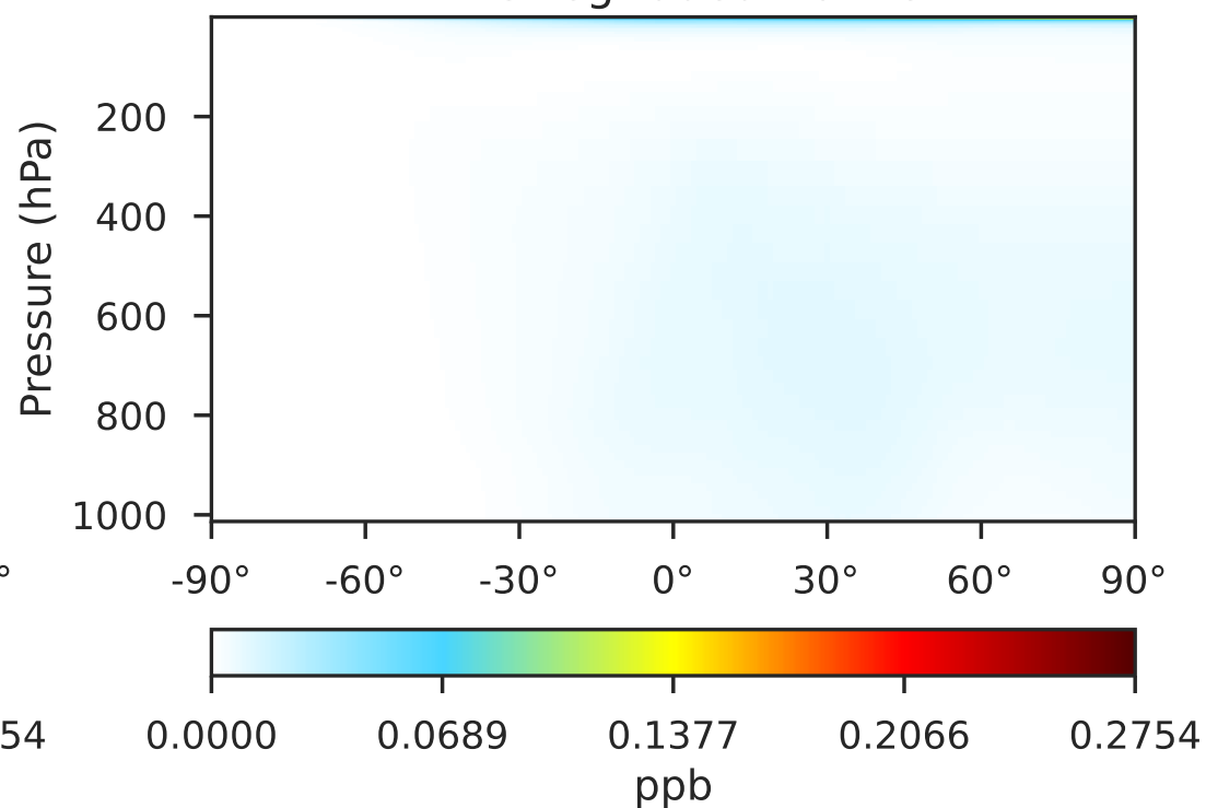
Cloud-J in 14.3.0 (Dev) 1x1.25 regridded from c24
