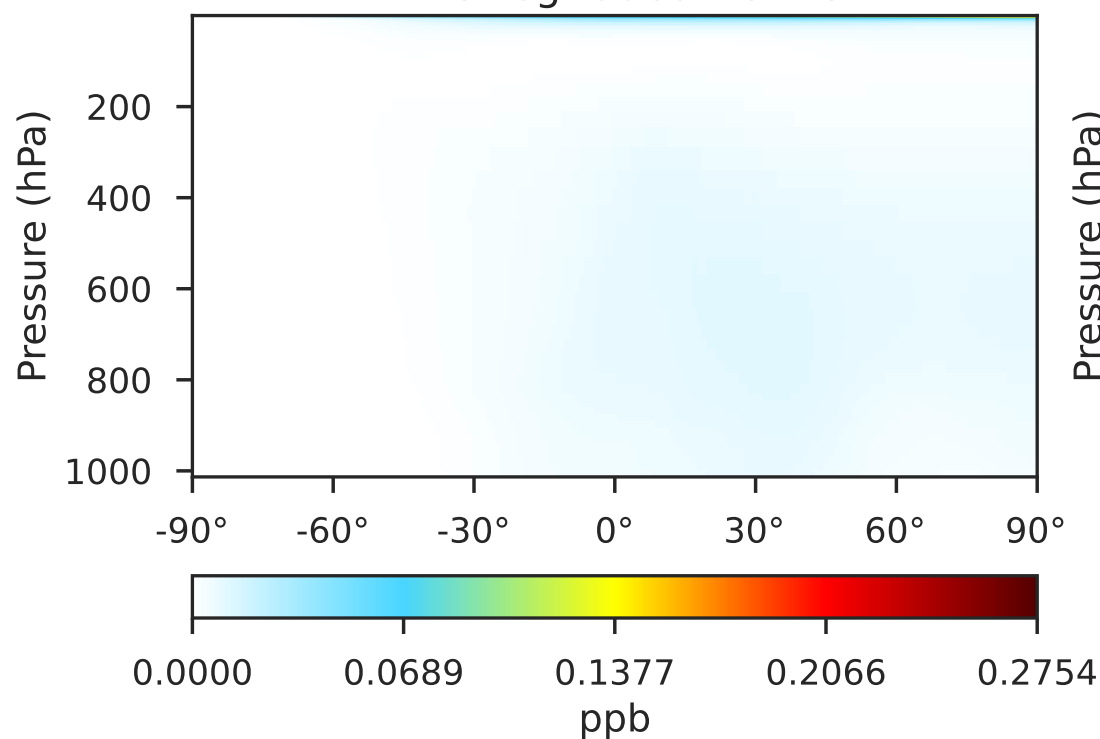
Fast-JX in 14.3.0 (Ref) 1x1.25 regridded from c24
