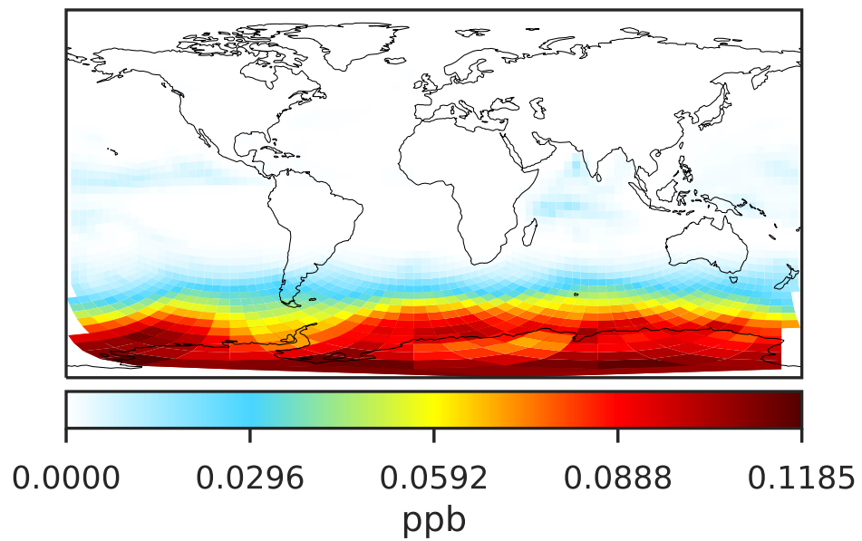
Fast-JX in 14.3.0 (Ref) c24
