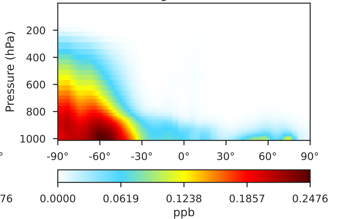
Cloud-J in 14.3.0 (Dev) 1x1.25 regridded from c24
