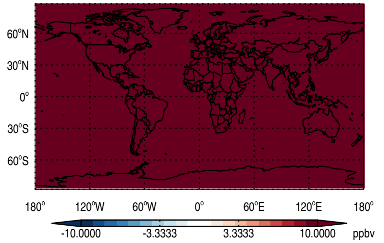
Abs Diff @ 500 hPa - SHEmis90dayTracer
