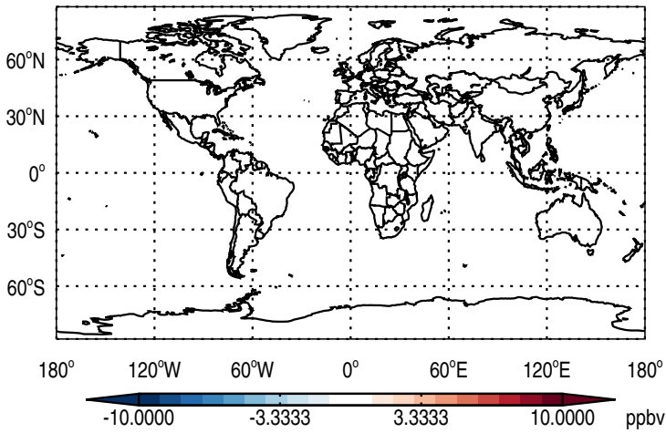
Abs Diff @ Surface - CH3ITracer
