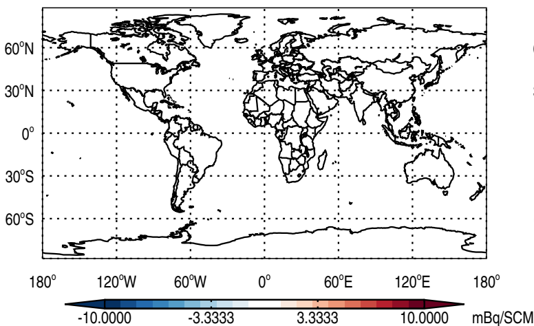
Abs Diff @ Surface - Pb210Strat
