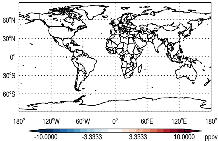
Abs Diff @ Surface - PassiveTracer
