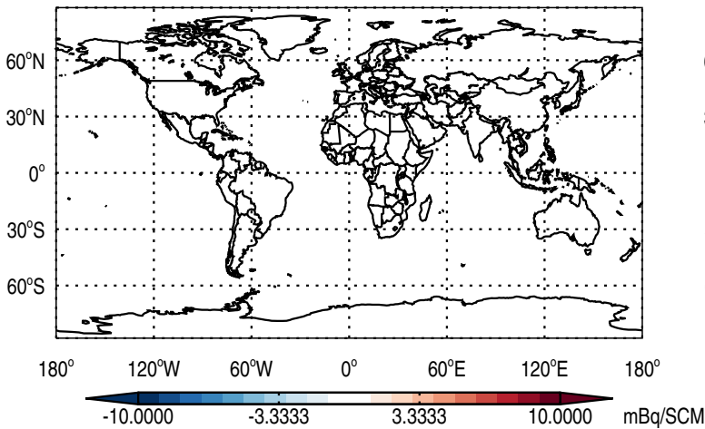
Abs Diff @ Surface - Pb210
