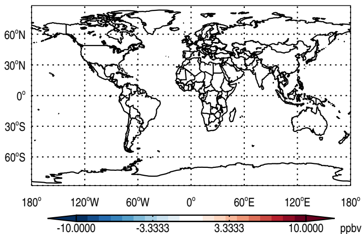
Abs Diff @ Surface - SF6Tracer
