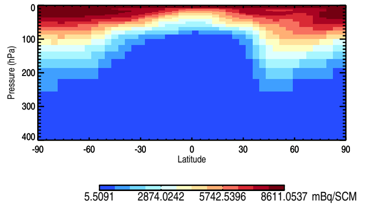
Tracer Curtain @ -180.000 - Be10
