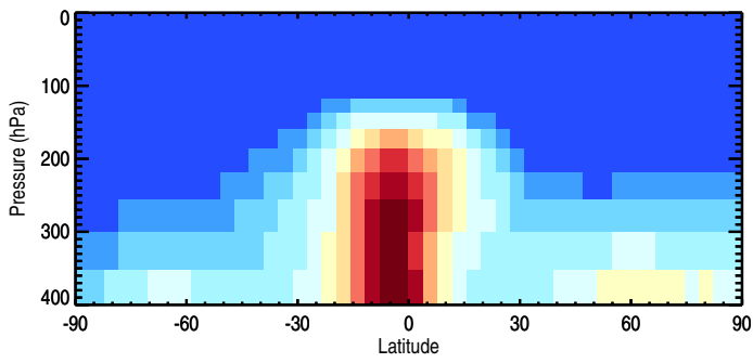
Tracer Curtain Zonal mean - CH3ITracer
