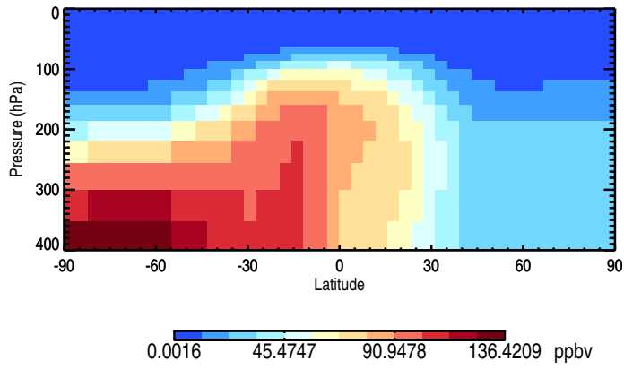
Tracer Curtain Zonal mean - SHEmis90dayTracer
