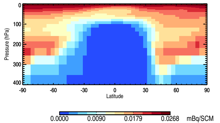
Tracer Curtain @ -180.000 - Pb210Strat
