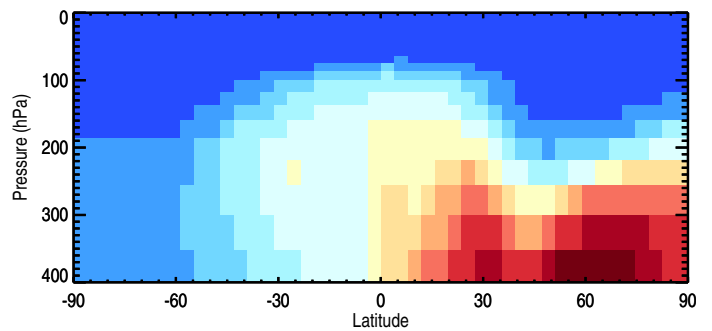
Tracer Curtain @ -180.000 - COAnthroEmis50dayTracer
