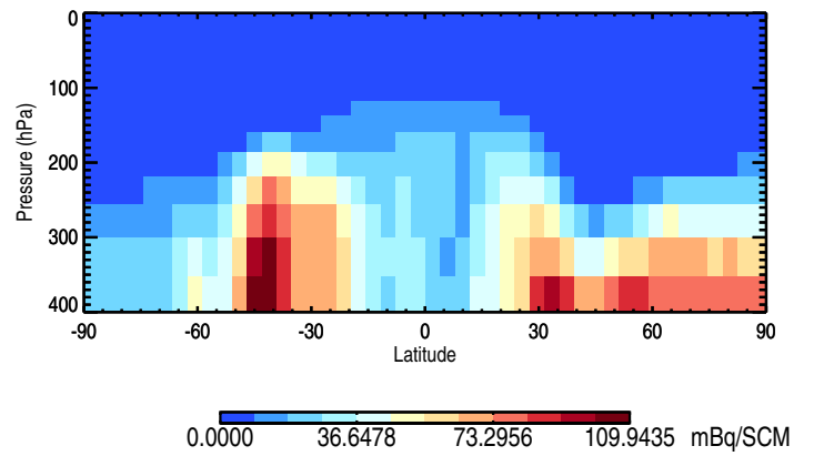
Tracer Curtain @ -180.000 - Rn222
