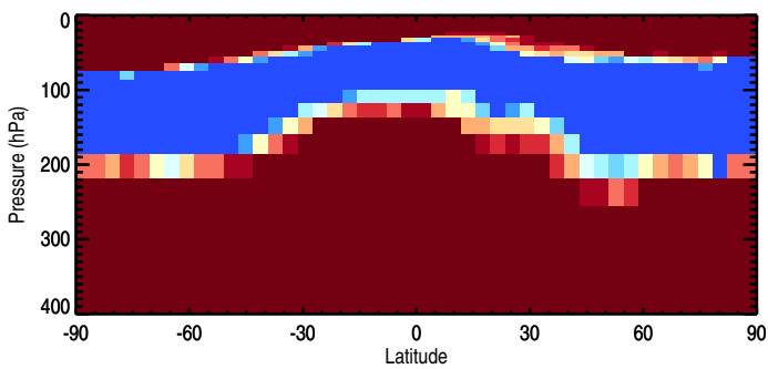
Tracer Curtain Zonal mean - PassiveTracer
