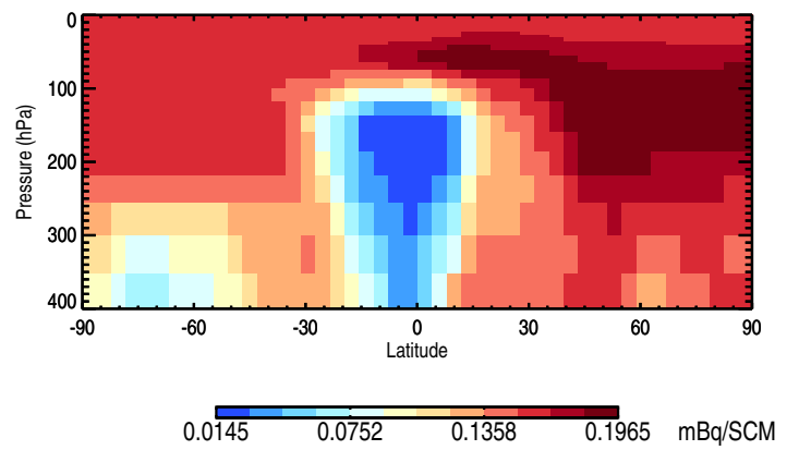
Tracer Curtain @ -180.000 - Pb210
