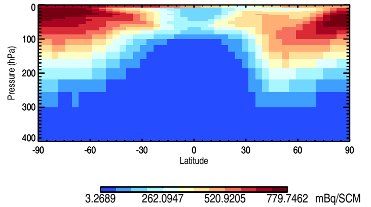
Tracer Curtain @ -180.000 - Be7
