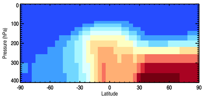
Tracer Curtain Zonal mean - COAnthroEmis25dayTracer
