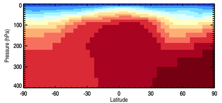
Tracer Curtain @ -180.000 - SF6Tracer
