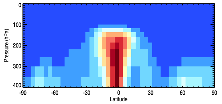
Tracer Curtain @ -180.000 - CH3ITracer
