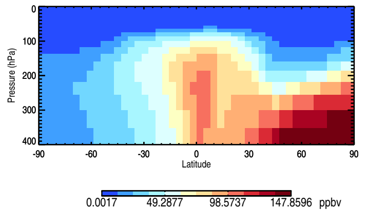
Tracer Curtain @ -180.000 - NHEmis90dayTracer
