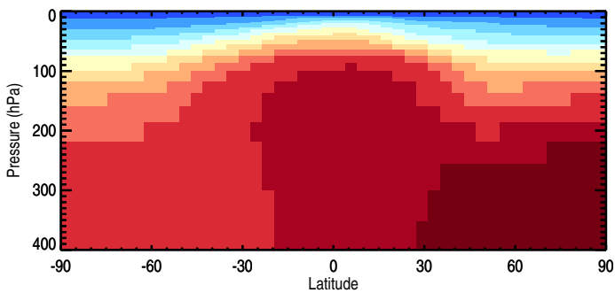
Tracer Curtain Zonal mean - SF6Tracer
