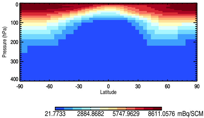
Tracer Curtain Zonal mean - Be10
