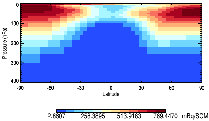
Tracer Curtain Zonal mean - Be7Strat
