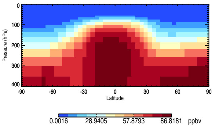
Tracer Curtain Zonal mean - GlobEmis90dayTracer
