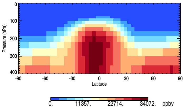
Tracer Curtain Zonal mean - COUniformEmis25dayTracer
