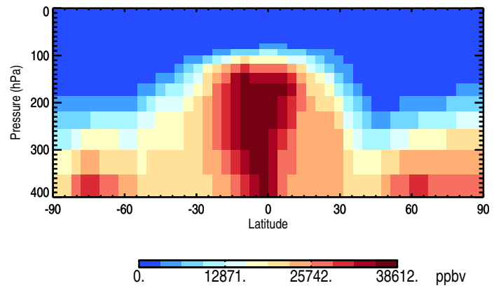
Tracer Curtain @ -180.000 - COUniformEmis25dayTracer
