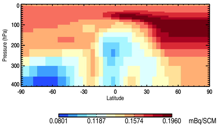
Tracer Curtain Zonal mean - Pb210
