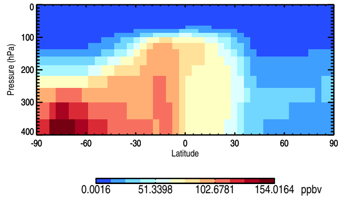
Tracer Curtain @ -180.000 - SHEmis90dayTracer
