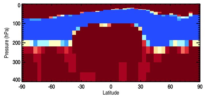
Tracer Curtain @ -180.000 - PassiveTracer
