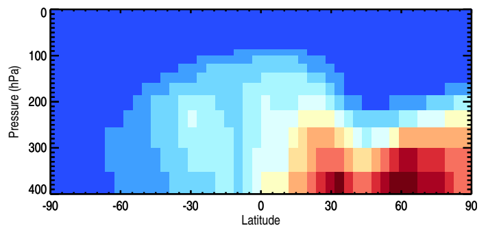
Tracer Curtain @ -180.000 - COAnthroEmis25dayTracer
