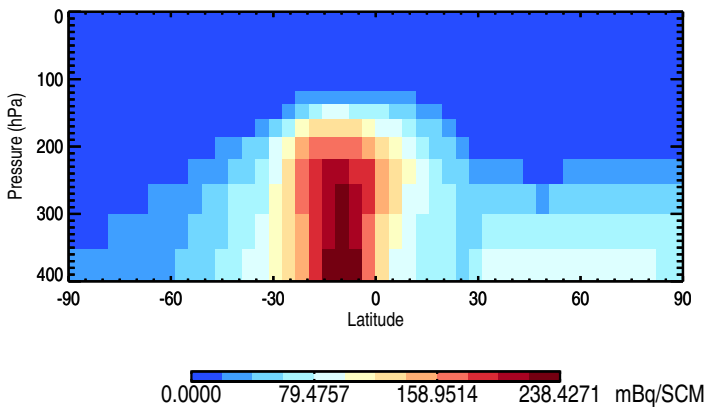
Tracer Curtain Zonal mean - Rn222
