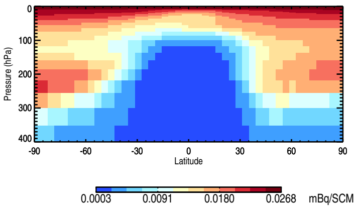
Tracer Curtain Zonal mean - Pb210Strat
