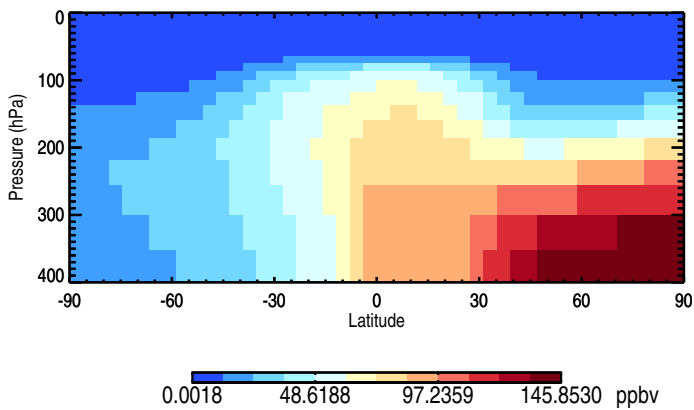
Tracer Curtain Zonal mean - NHEmis90dayTracer
