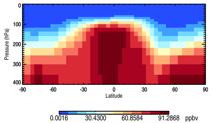
Tracer Curtain @ -180.000 - GlobEmis90dayTracer
