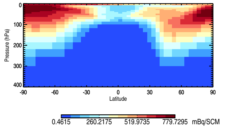
Tracer Curtain @ -180.000 - Be7Strat
