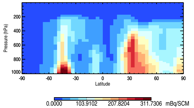
Tracer Curtain @ -180.000 - Rn222
