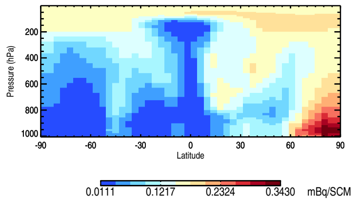
Tracer Curtain @ -180.000 - Pb210
