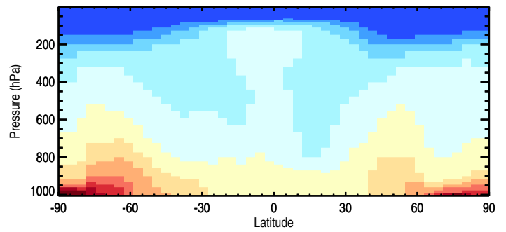
Tracer Curtain @ -180.000 - GlobEmis90dayTracer
