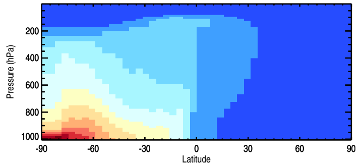
Tracer Curtain @ -180.000 - SHEmis90dayTracer
