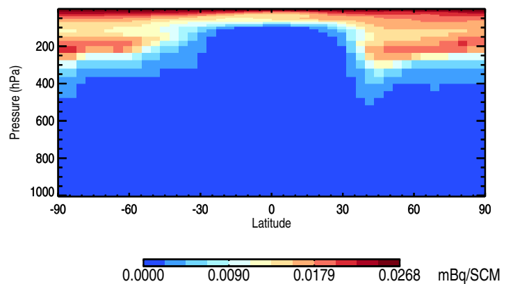
Tracer Curtain @ -180.000 - Pb210Strat
