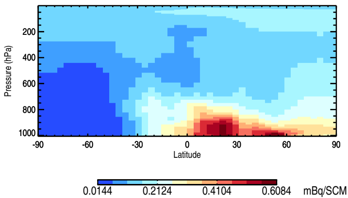
Tracer Curtain Zonal mean - Pb210
