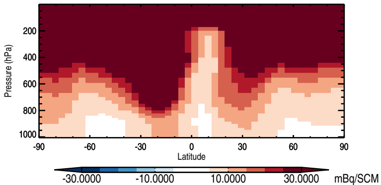
Zonal mean abs diff: Be10
