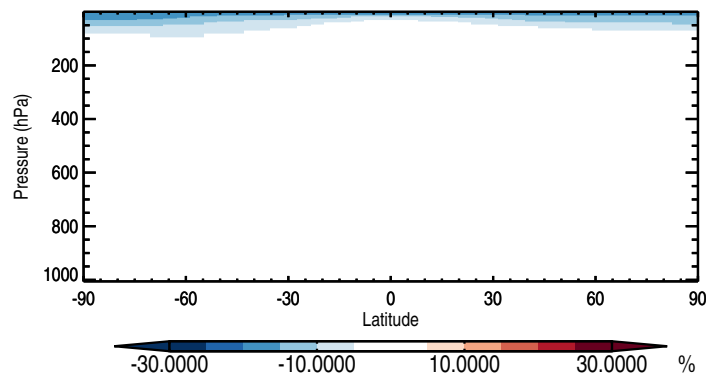
Zonal mean % diff: Pb210
