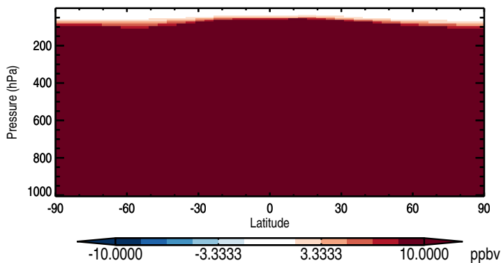
Zonal mean abs diff: GlobEmis90dayTracer
