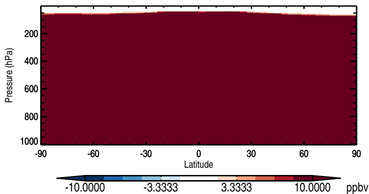
Zonal mean abs diff: COUniformEmis25dayTracer
