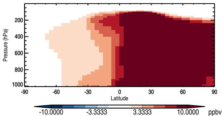
Zonal mean abs diff: COAnthroEmis25dayTracer
