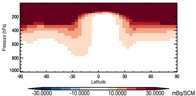
Zonal mean abs diff: Be7Strat
