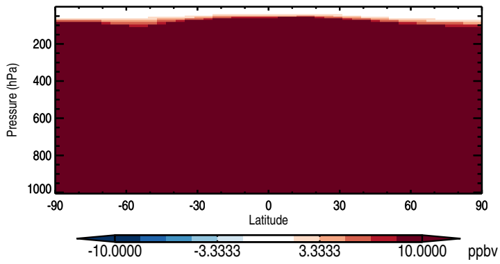
Zonal mean abs diff: SHEmis90dayTracer
