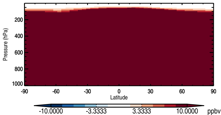
Zonal mean abs diff: NHEmis90dayTracer
