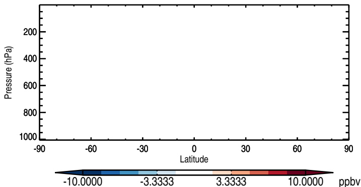
Zonal mean abs diff: PassiveTracer
