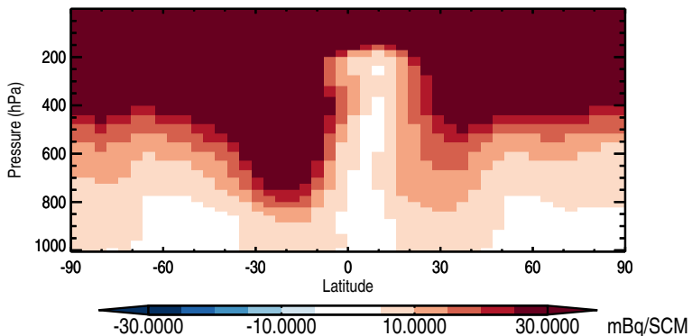
Zonal mean abs diff: Be10Strat
