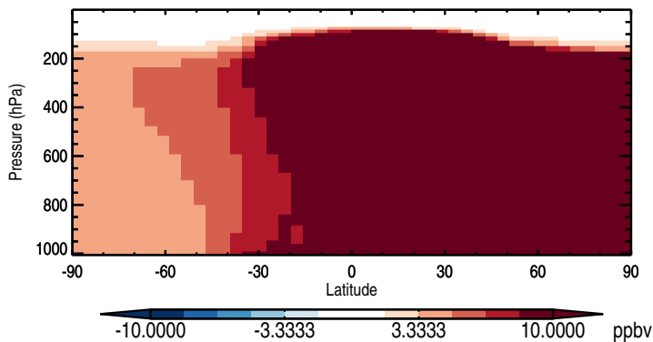
Zonal mean abs diff: COAnthroEmis50dayTracer
