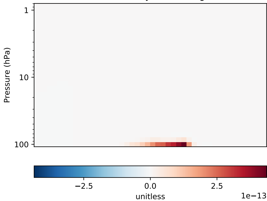
Fractional Difference (Dev-Ref)/Ref, Dynamic Range
