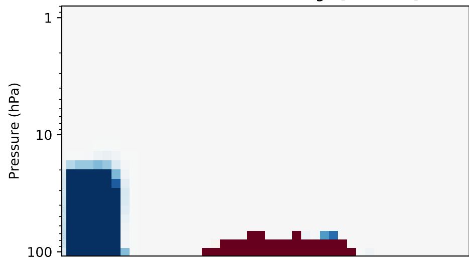
Difference Dev - Ref, Restricted Range [5%,95%]
