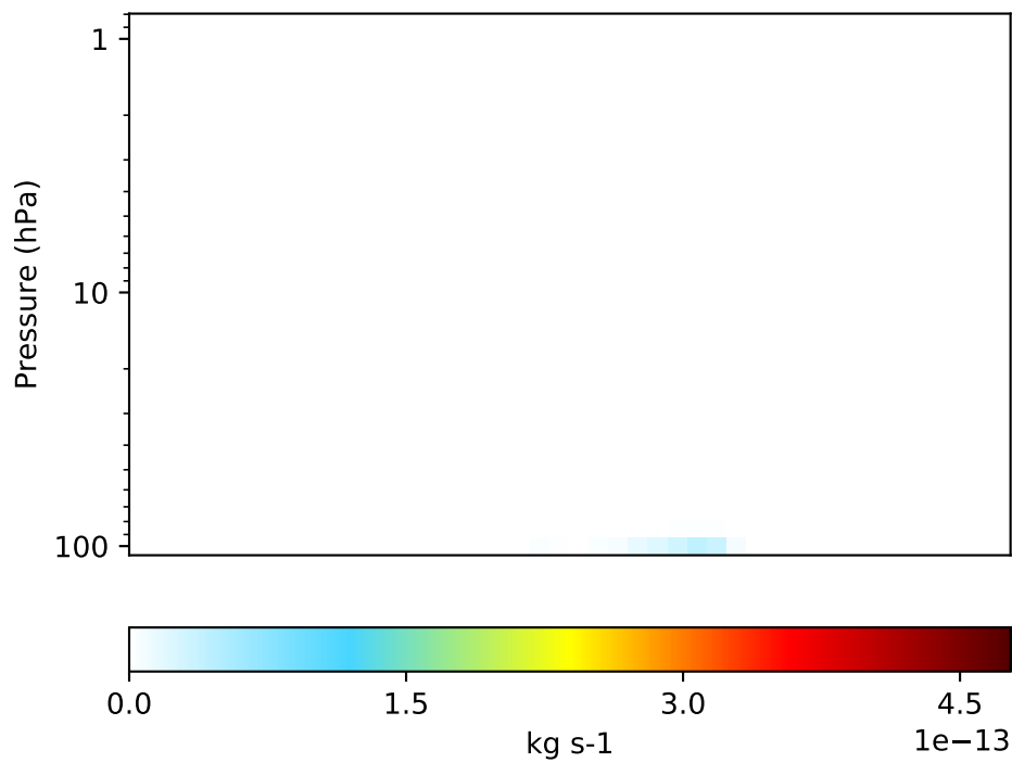
Difference Dev - Ref, Dynamic Range
