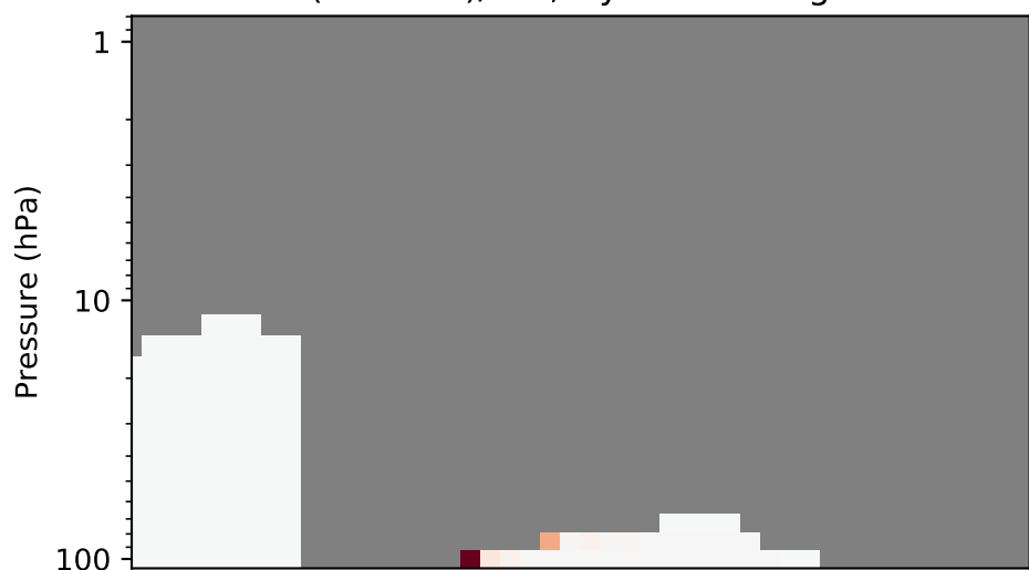
Fractional Difference (Dev-Ref)/Ref, Dynamic Range
