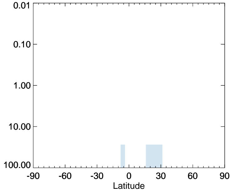
v11-01-public-Run0 / v11-01g-Run0 NH3 - Strat zonal mean % diff for Apr
