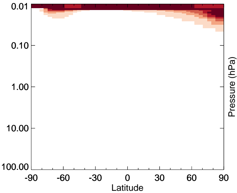
v11-01-public-Run0 - v11-01g-Run0 NO - Strat zonal mean abs diff for Apr
