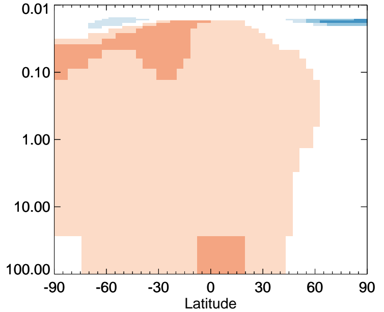
v11-01-public-Run0 / v11-01g-Run0 MEK - Strat zonal mean % diff for Apr
