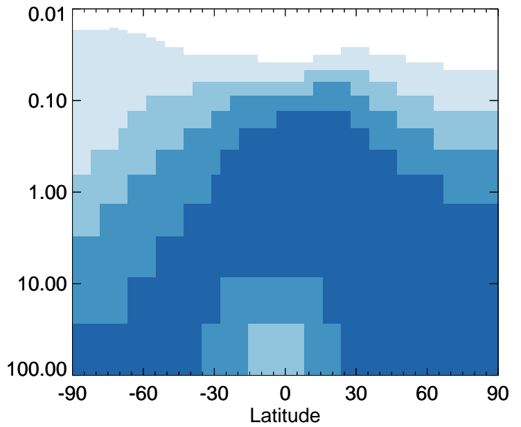
v11-01-public-Run0 / v11-01g-Run0 ALD2 - Strat zonal mean % diff for Apr
