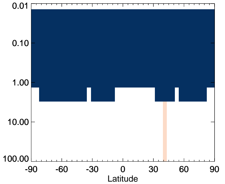
v11-01-public-Run0 / v11-01k-Run0 SO4s - Strat zonal mean % diff for Apr
