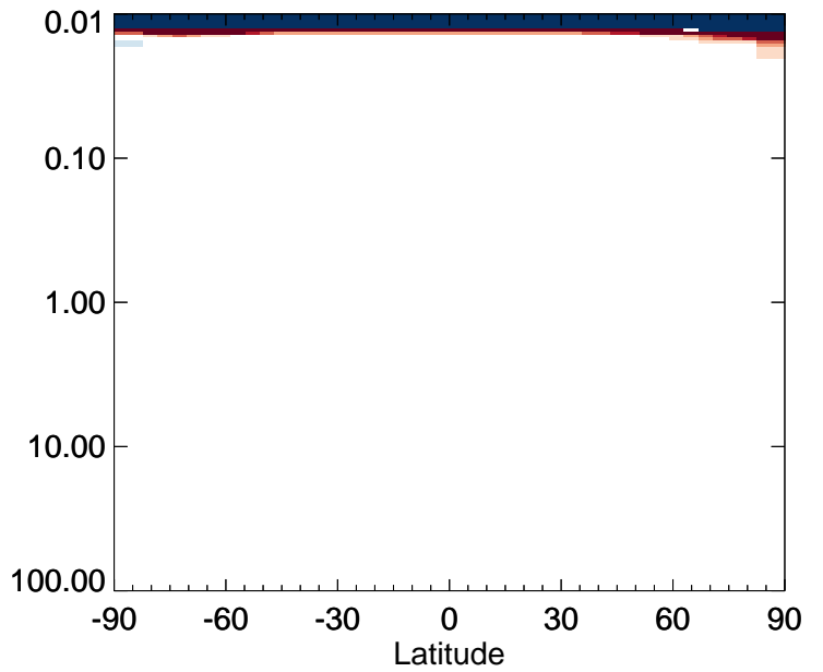
v11-01-public-Run0 / v11-01g-Run0 NO3 - Strat zonal mean % diff for Apr
