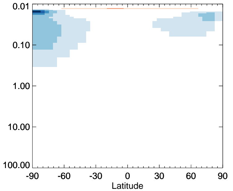
v11-01-public-Run0 / v11-01g-Run0 OCIO - Strat zonal mean % diff for Apr
