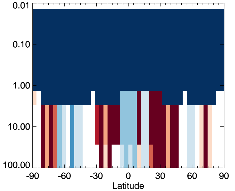
v11-01-public-Run0 / v11-01g-Run0 SO4s - Strat zonal mean % diff for Apr
