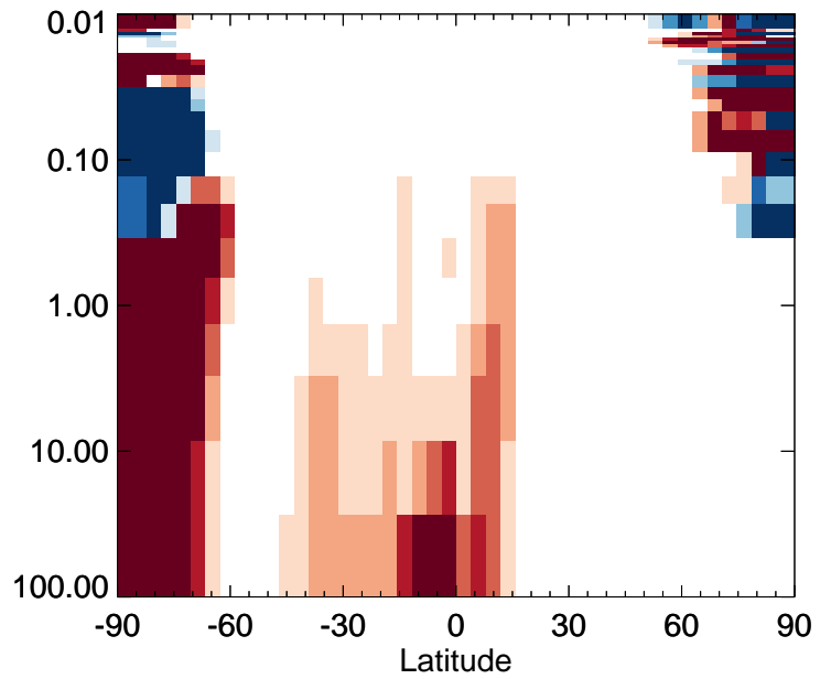
v11-01-public-Run0 / v11-01g-Run0 PMN - Strat zonal mean % diff for Apr
