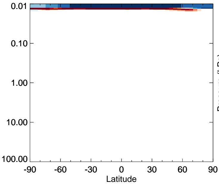
v11-01-public-Run0 - v11-01g-Run0 NO3 - Strat zonal mean abs diff for Apr
