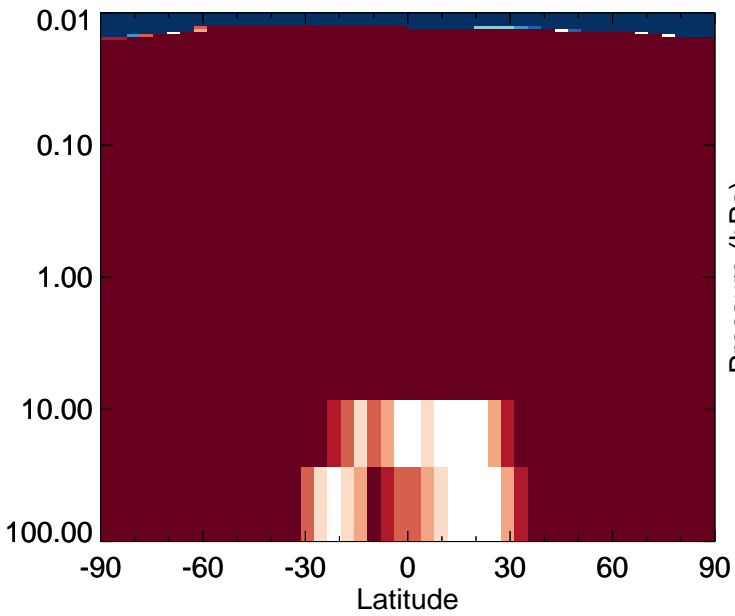
v11-01-public-Run0 - v11-01g-Run0 H2O - Strat zonal mean abs diff for Apr
