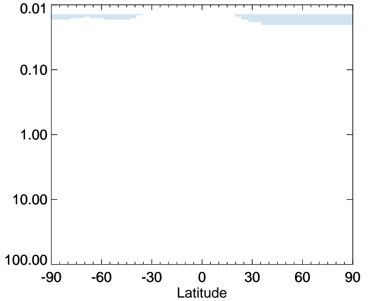
v11-01-public-Run0 / v11-01g-Run0 OCS - Strat zonal mean % diff for Apr
