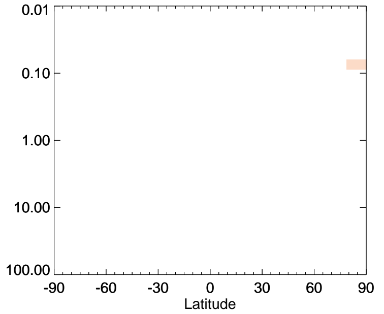
v11-01-public-Run0 / v11-01k-Run0 RIP - Strat zonal mean % diff for Apr
