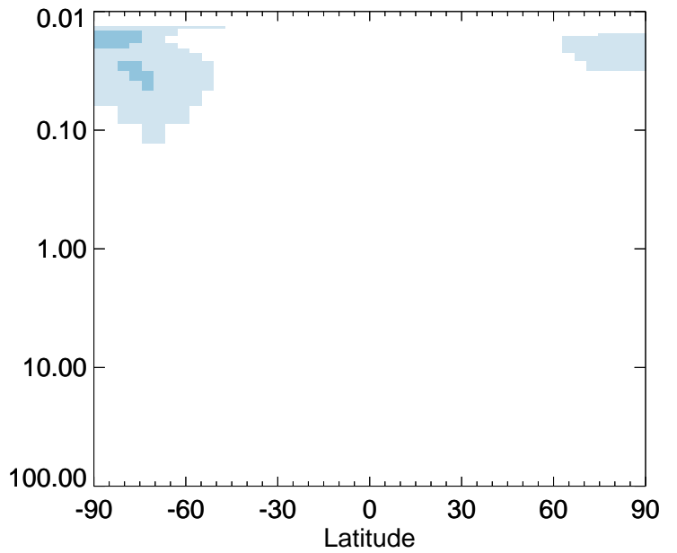
v11-01-public-Run0 / v11-01g-Run0 HOCl - Strat zonal mean % diff for Apr
