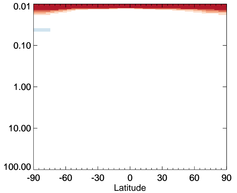
v11-01-public-Run0 / v11-01g-Run0 SO 2 - Strat zonal mean % diff for Apr
