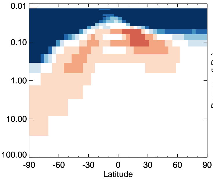
v11-01-public-Run0 - v11-01g-Run0 O3 - Strat zonal mean abs diff for Apr
