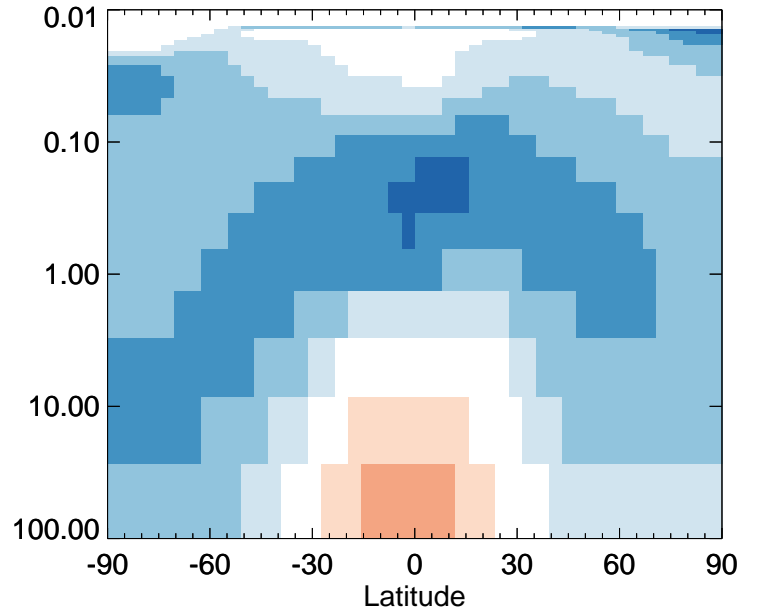
v11-01-public-Run0 / v11-01g-Run0 MAP - Strat zonal mean % diff for Apr
