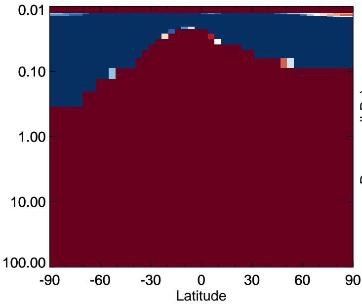
v11-01-public-Run0 - v11-01g-Run0 CH4 - Strat zonal mean abs diff for Apr
