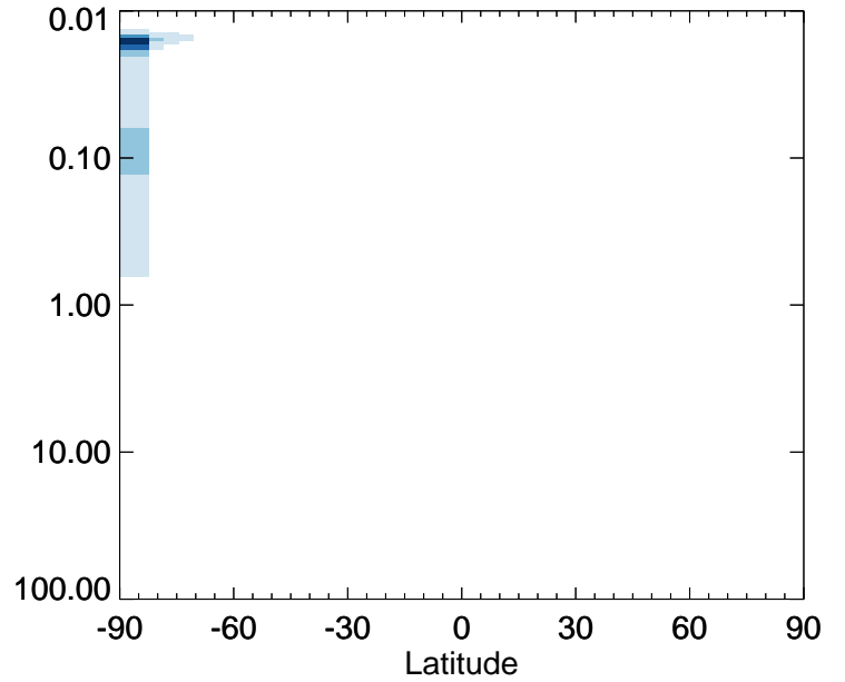
v11-01-public-Run0 / v11-01g-Run0 BrO - Strat zonal mean % diff for Apr
