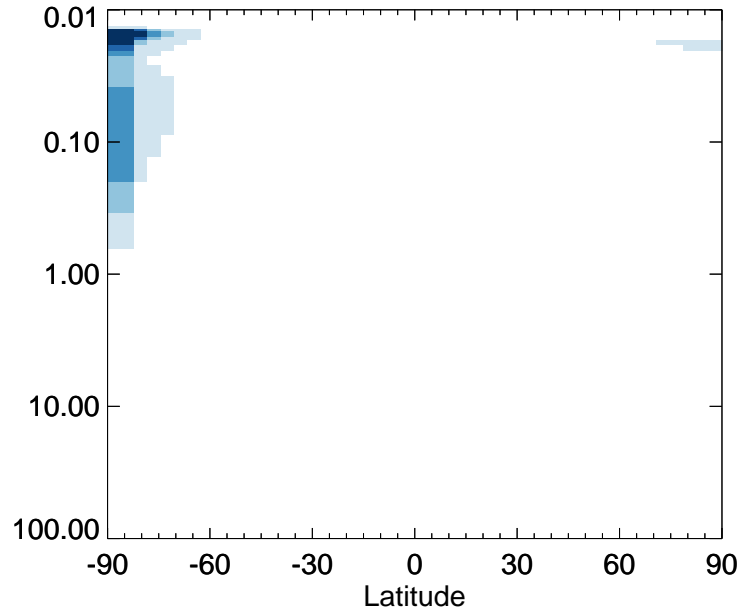
v11-01-public-Run0 / v11-01g-Run0 ClO - Strat zonal mean % diff for Apr
