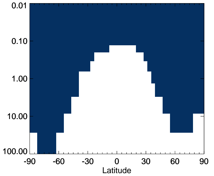
v11-01-public-Run0 / v11-01k-Run0 NIT - Strat zonal mean % diff for Apr
