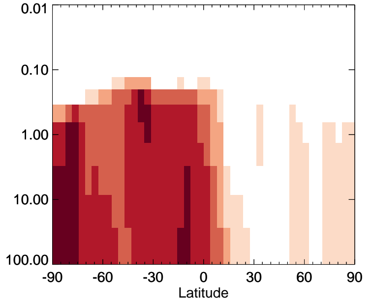
v11-01-public-Run0 / v11-01g-Run0 NITs - Strat zonal mean % diff for Apr
