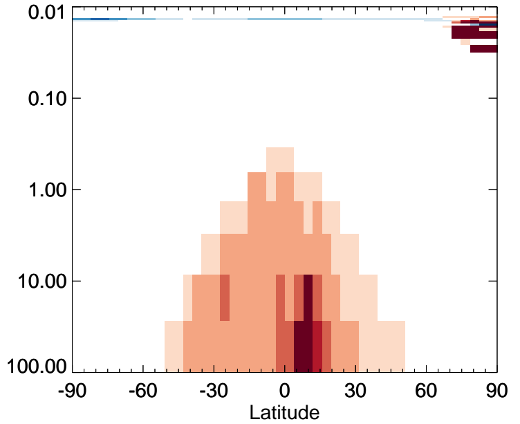
v11-01-public-Run0 / v11-01g-Run0 LIMO - Strat zonal mean % diff for Apr
