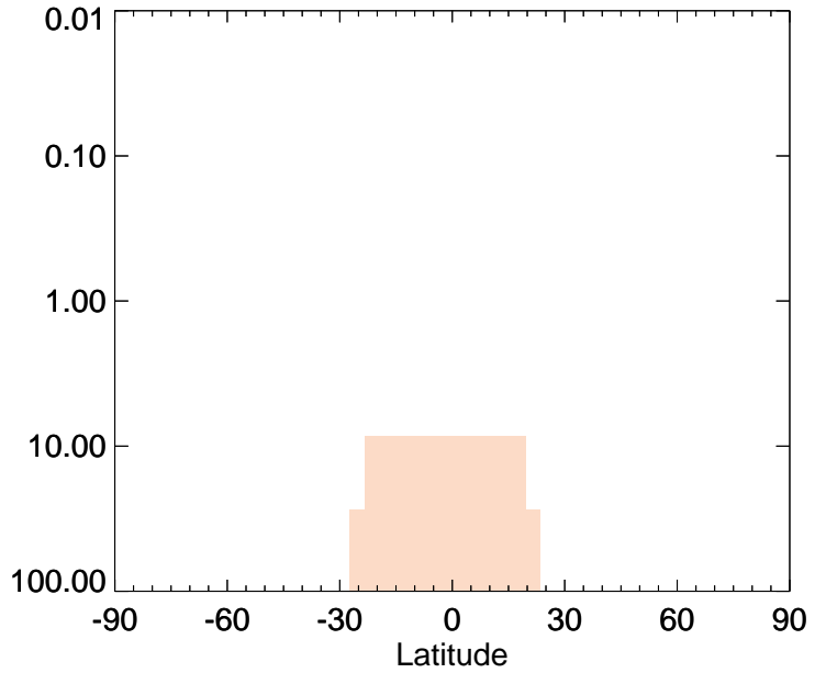
v11-01-public-Run0 / v11-01g-Run0 MSA - Strat zonal mean % diff for Apr
