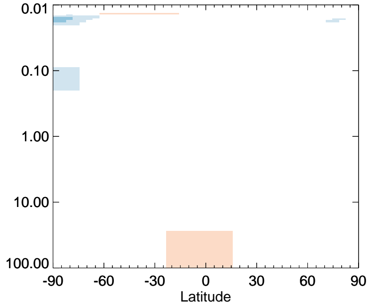
v11-01-public-Run0 / v11-01g-Run0 Br2 - Strat zonal mean % diff for Apr
