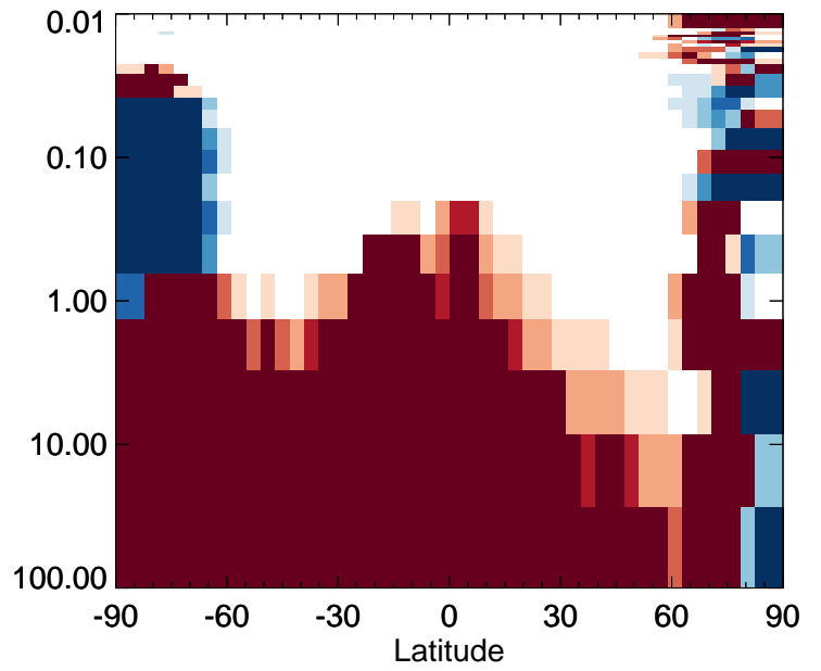
v11-01-public-Run0 / v11-01g-Run0 ISOP - Strat zonal mean % diff for Apr
