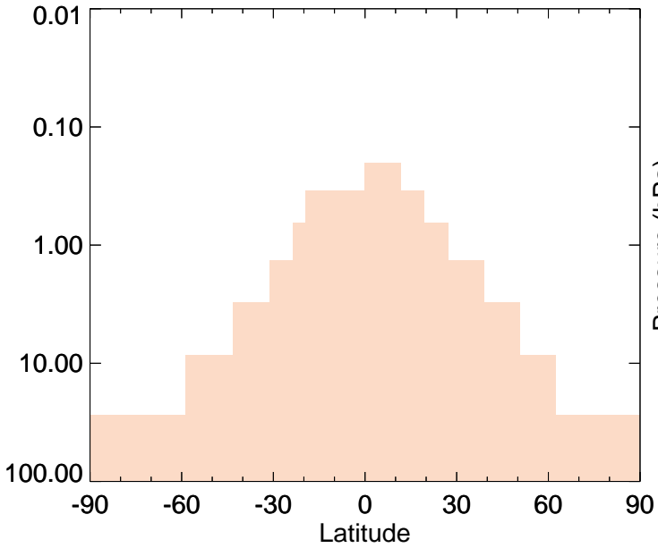
v11-01-public-Run0 - v11-01g-Run0 PPN - Strat zonal mean abs diff for Apr
