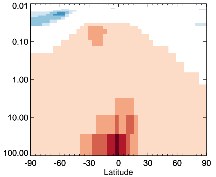
v11-01-public-Run0 / v11-01g-Run0 HAC - Strat zonal mean % diff for Apr
