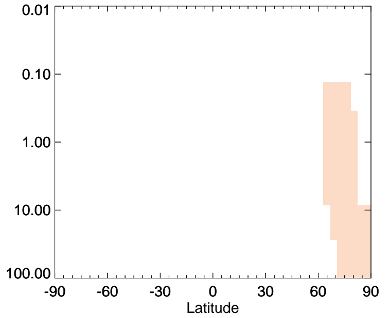
v11-01-public-Run0 / v11-01k-Run0 DMS - Strat zonal mean % diff for Apr
