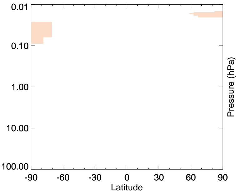
v11-01-public-Run0 - v11-01g-Run0 HCl - Strat zonal mean abs diff for Apr
