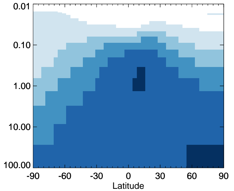
v11-01-public-Run0 / v11-01g-Run0 C2H6 - Strat zonal mean % diff for Apr
