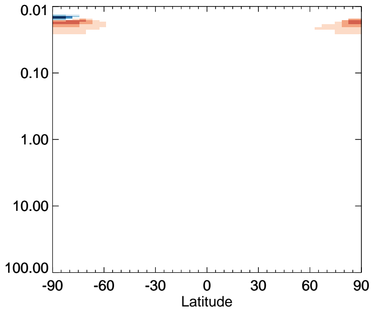
v11-01-public-Run0 / v11-01g-Run0 Cl2 - Strat zonal mean % diff for Apr
