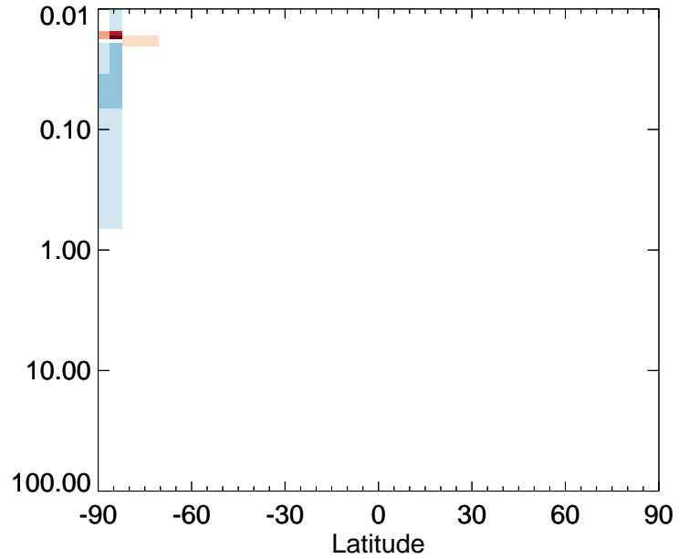
v11-01-public-Run0 / v11-01g-Run0 OH - Strat zonal mean % diff for Apr
