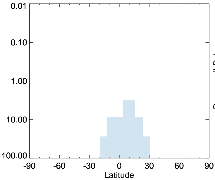
v11-01-public-Run0 - v11-01g-Run0 C2H6 - Strat zonal mean abs diff for Apr
