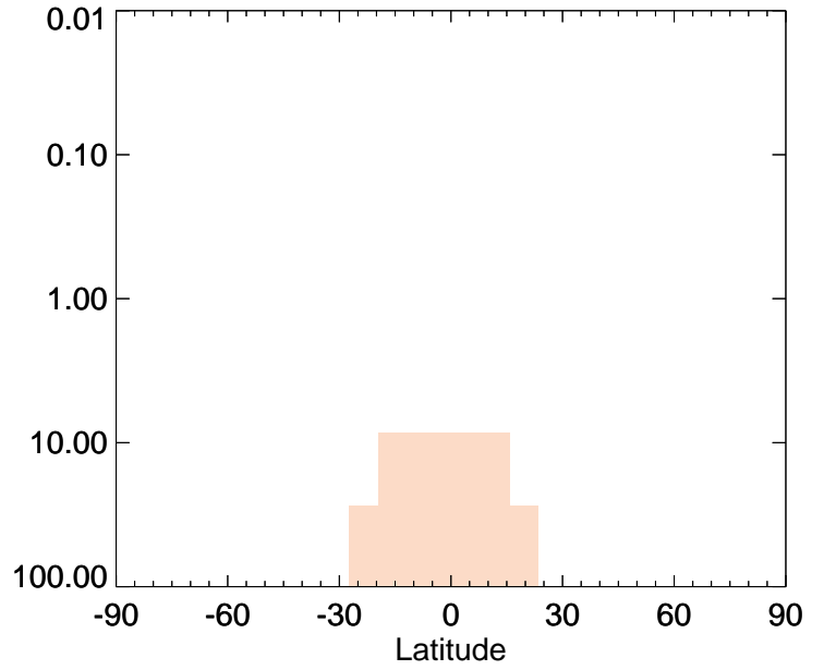
v11-01-public-Run0 / v11-01g-Run0 BCPI - Strat zonal mean % diff for Apr
