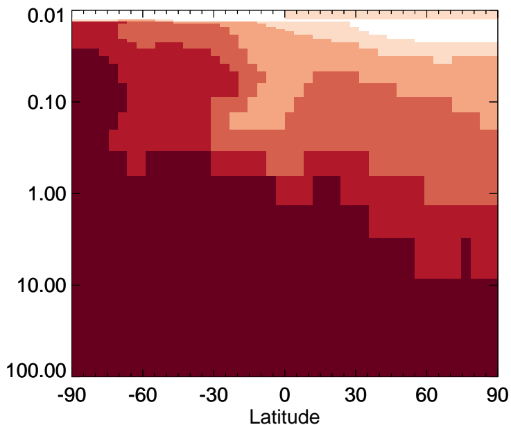
v11-01-public-Run0 / v11-01g-Run0 C3H8 - Strat zonal mean % diff for Apr
