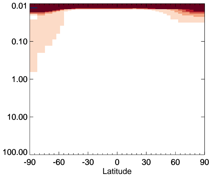
v11-01-public-Run0 / v11-01g-Run0 NO - Strat zonal mean % diff for Apr
