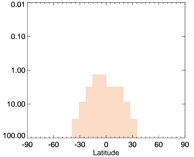
v11-01-public-Run0 / v11-01g-Run0 PPN - Strat zonal mean % diff for Apr
