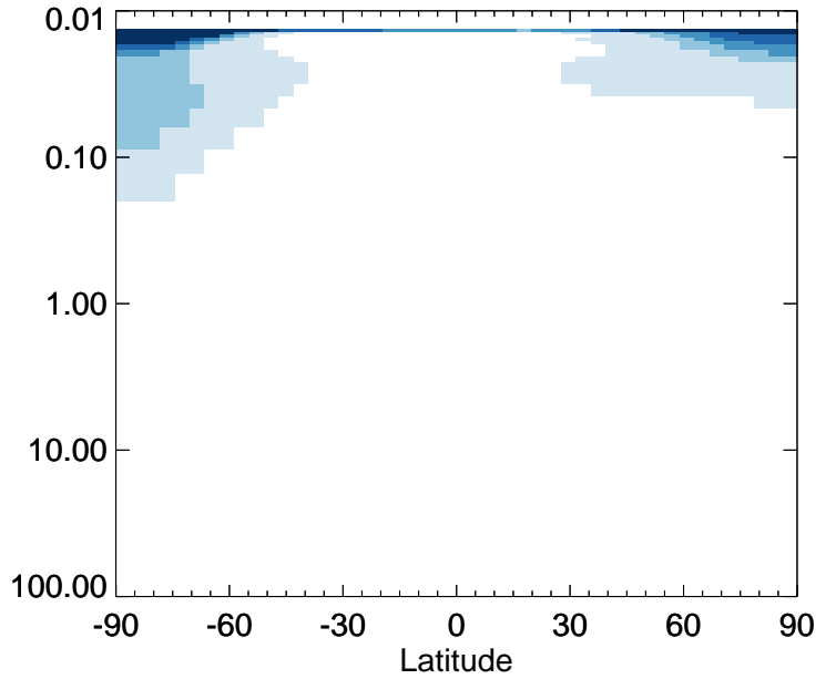
v11-01-public-Run0 / v11-01g-Run0 MP - Strat zonal mean % diff for Apr
