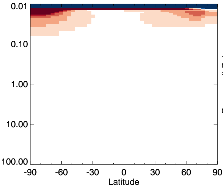
v11-01-public-Run0 - v11-01g-Run0 NO2 - Strat zonal mean abs diff for Apr
