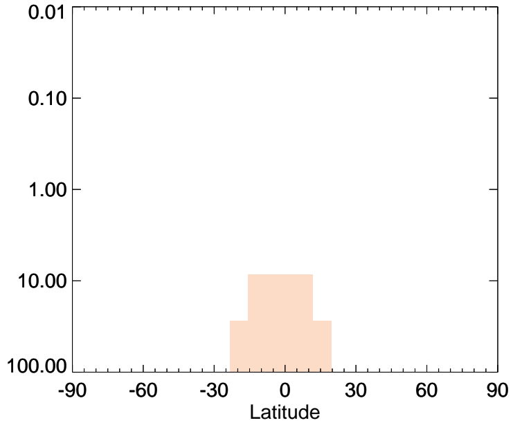
v11-01-public-Run0 / v11-01g-Run0 OCPI - Strat zonal mean % diff for Apr
