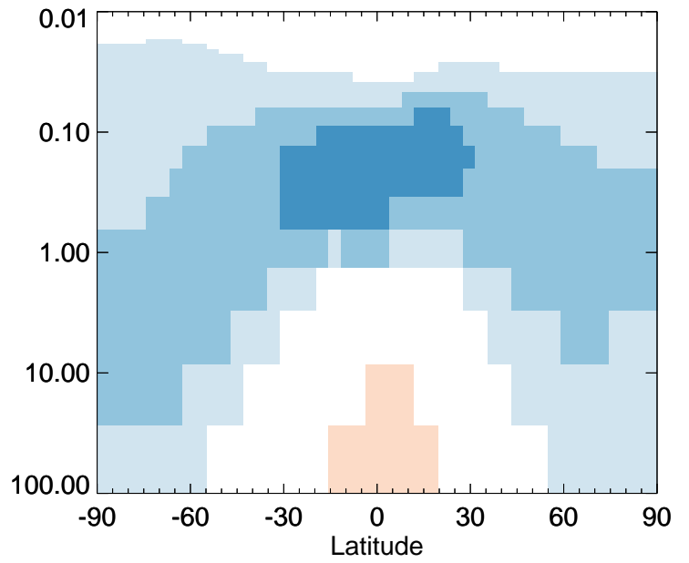
v11-01-public-Run0 / v11-01g-Run0 PAN - Strat zonal mean % diff for Apr
