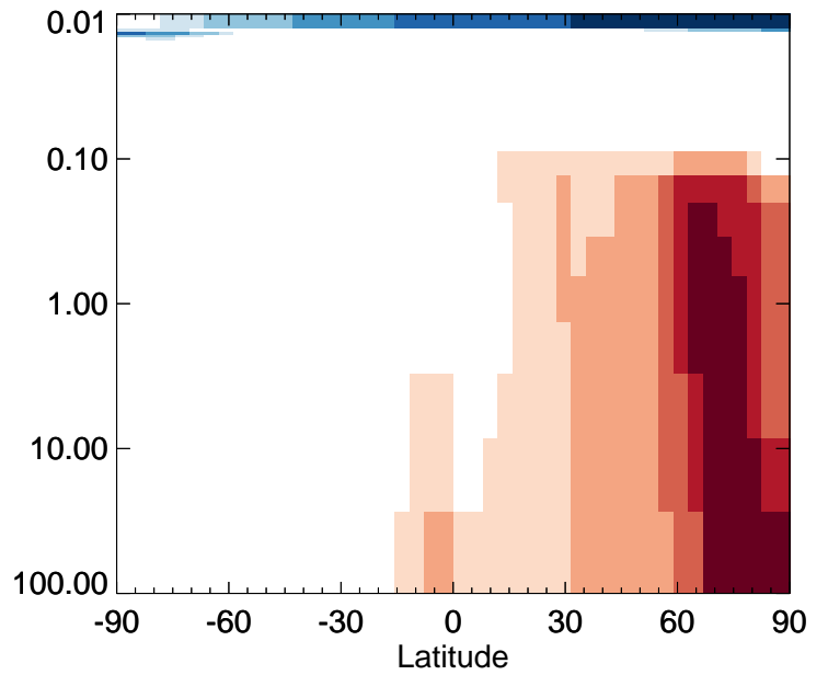
v11-01-public-Run0 / v11-01g-Run0 DMS - Strat zonal mean % diff for Apr
