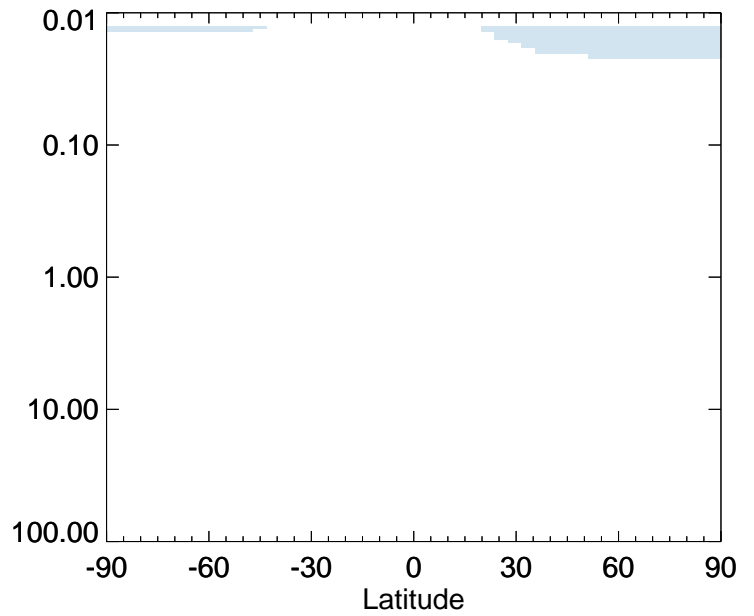
v11-01-public-Run0 / v11-01g-Run0 CCI4 - Strat zonal mean % diff for Apr
