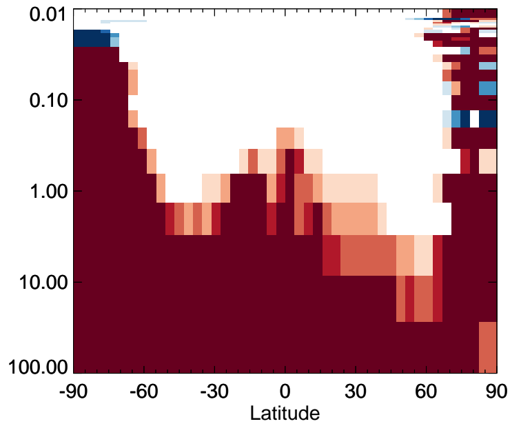
v11-01-public-Run0 / v11-01g-Run0 RIP - Strat zonal mean % diff for Apr
