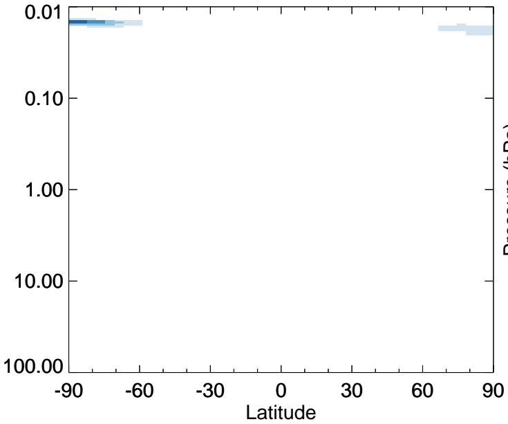
v11-01-public-Run0 - v11-01g-Run0 ClO - Strat zonal mean abs diff for Apr
