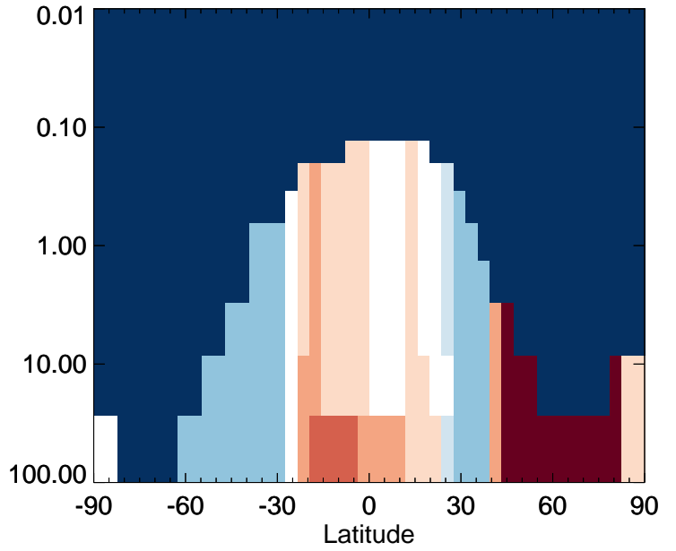
v11-01-public-Run0 / v11-01g-Run0 NIT - Strat zonal mean % diff for Apr
