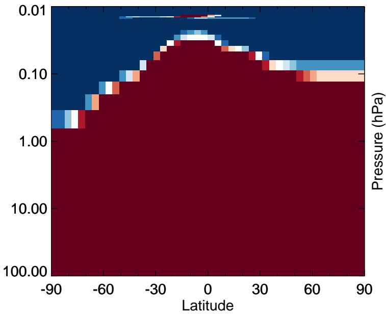
v11-01-public-Run0 - v11-01g-Run0 N2O - Strat zonal mean abs diff for Apr
