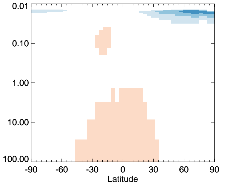
v11-01-public-Run0 / v11-01g-Run0 ALK4 - Strat zonal mean % diff for Apr
