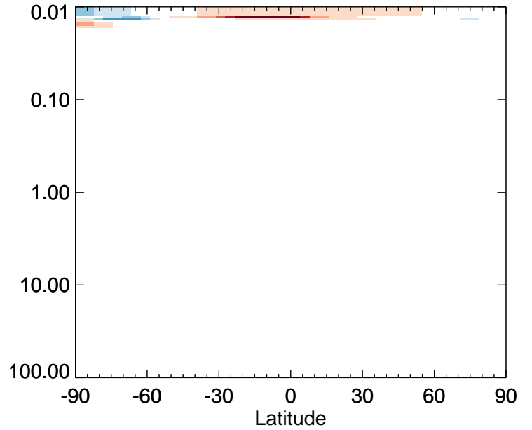
v11-01-public-Run0 / v11-01g-Run0 MPN - Strat zonal mean % diff for Apr
