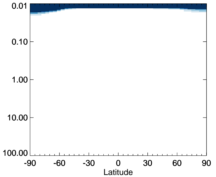
v11-01-public-Run0 / v11-01g-Run0 N2O - Strat zonal mean % diff for Apr
