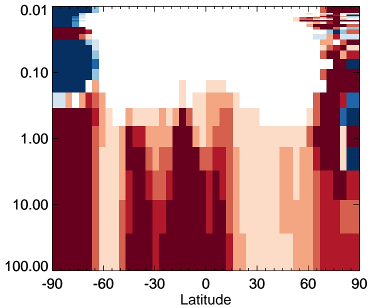
v11-01-public-Run0 / v11-01g-Run0 MVK - Strat zonal mean % diff for Apr
