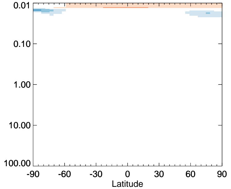
v11-01-public-Run0 / v11-01g-Run0 BrCl - Strat zonal mean % diff for Apr
