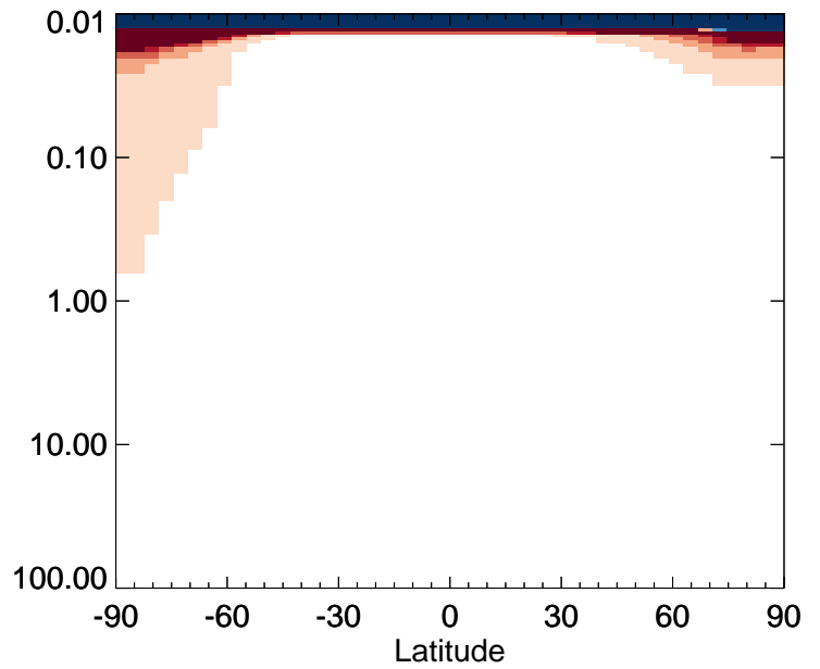
v11-01-public-Run0 / v11-01g-Run0 NO2 - Strat zonal mean % diff for Apr
