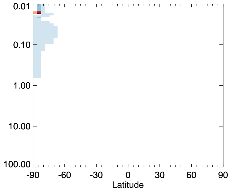
v11-01-public-Run0 / v11-01g-Run0 HO2 - Strat zonal mean % diff for Apr
