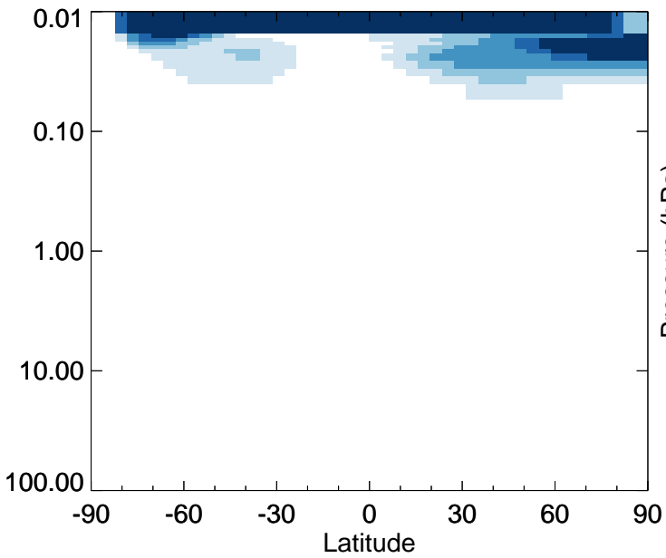
v11-01-public-Run0 - v11-01g-Run0 HO2 - Strat zonal mean abs diff for Apr
