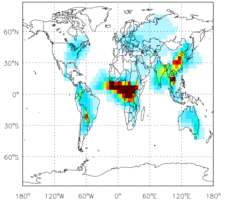
v11-01b-Run0 OC: Column AOD map for Jan
