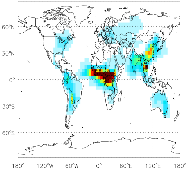
v10-01-public-Run0 OC: Column AOD map for Jan
