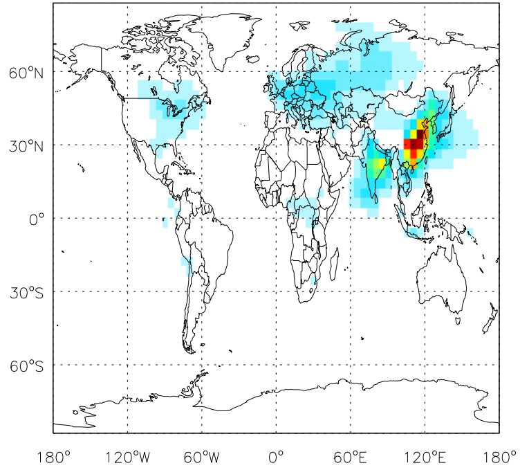
v11-01b-Run0 SO4: Column AOD map for Jan
