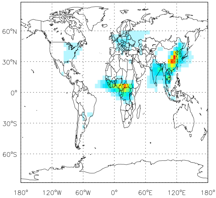
v10-01-public-Run0 BC: Column AOD map for Jan
