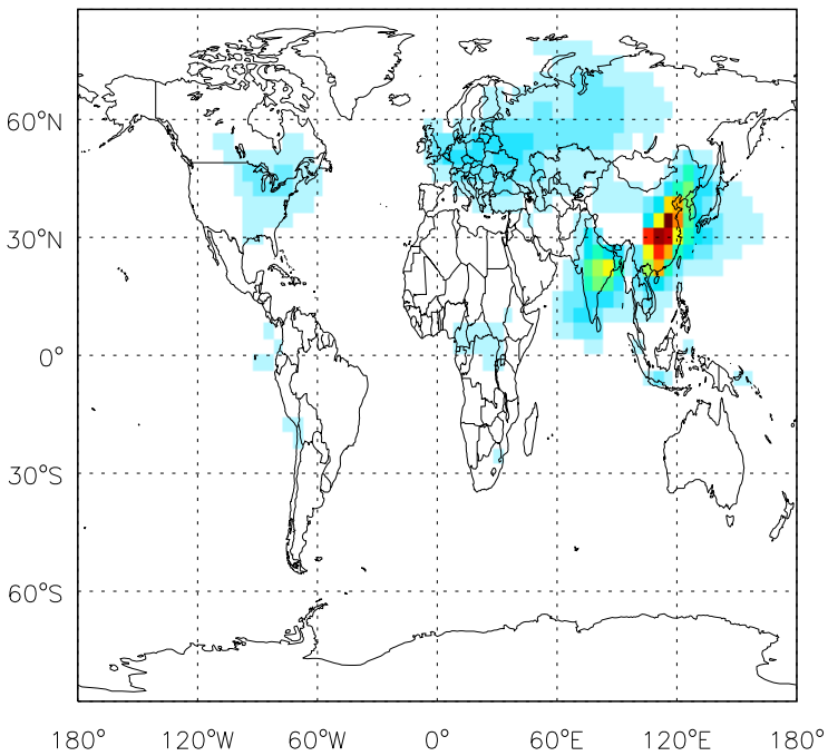
v11-01d-Run1 SO4: Column AOD map for Jan
