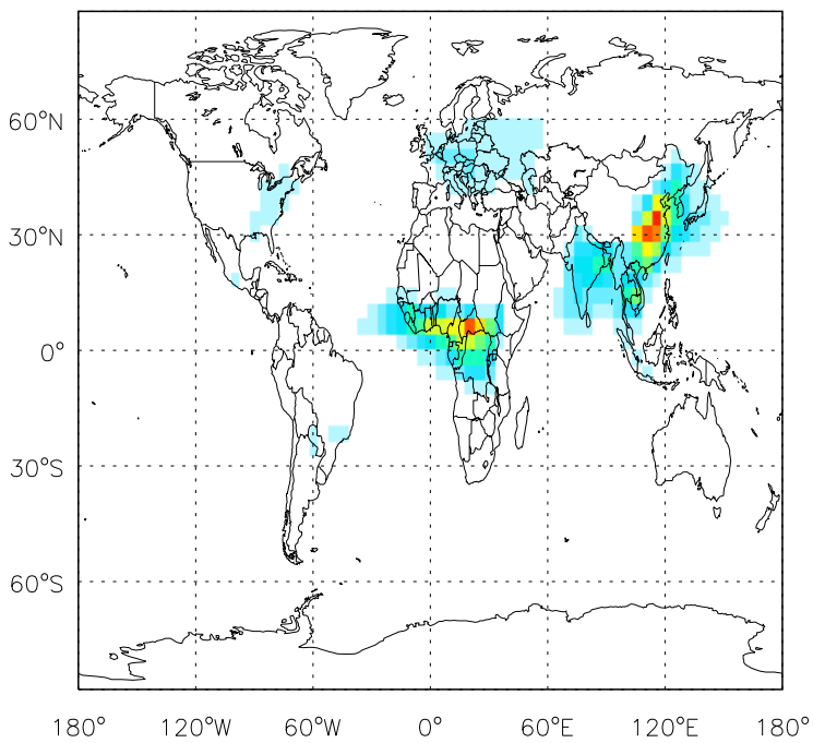
v11-01d-Run1 BC: Column AOD map for Jan
