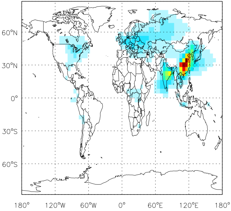
v10-01-public-Run0 SO4: Column AOD map for Jan
