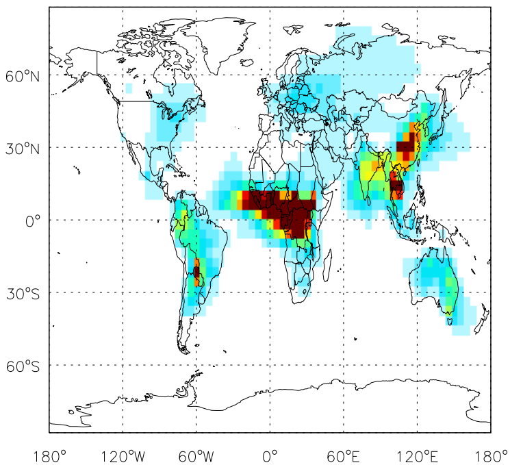
v11-01d-Run1 OC: Column AOD map for Jan
