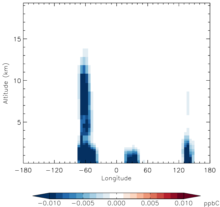
v11-01d-Run1 - v10-01-public-Run0 PRPE - Diff along 15S for Jan
