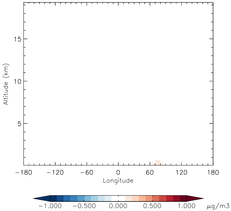
v11-01d-Run1 - v10-01-public-Run0 SO2 - Diff along 15S for Jan
