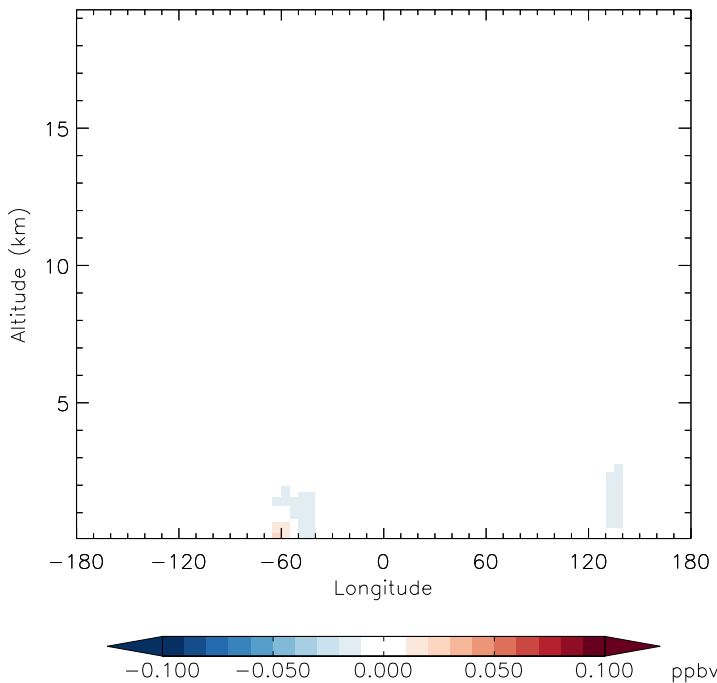
v11-01d-Run1 - v11-01b-Run0 GLYC - Diff along 15S for Jan
