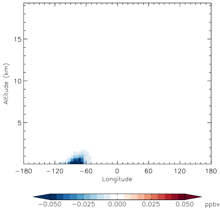
v11-01d-Run1 - v11-01b-Run0 RCHO - Diff along 42N for Jan
