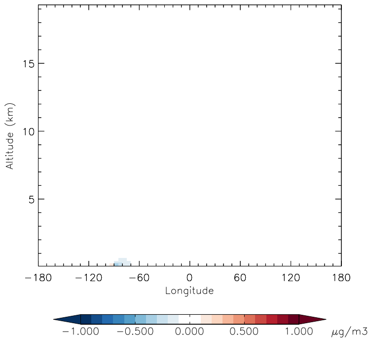
v11-01d-Run1 - v11-01b-Run0 NH3 - Diff along 42N for Jan
