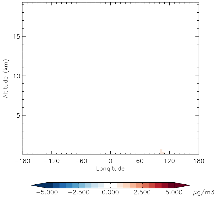
v11-01d-Run1 - v10-01-public-Run0 DST4 - Diff along 42N for Jan
