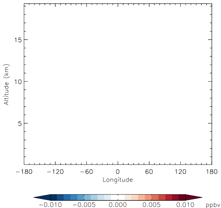
v11-01d-Run1 - v11-01b-Run0 BrNO3 - Diff along 42N for Jan
