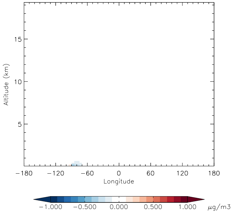
v11-01d-Run1 - v10-01-public-Run0 NH3 - Diff along 42N for Jan
