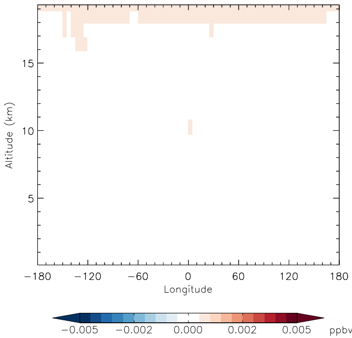
v11-01d-Run1 - v10-01-public-Run0 N2O5 - Diff along 15S for Jan
