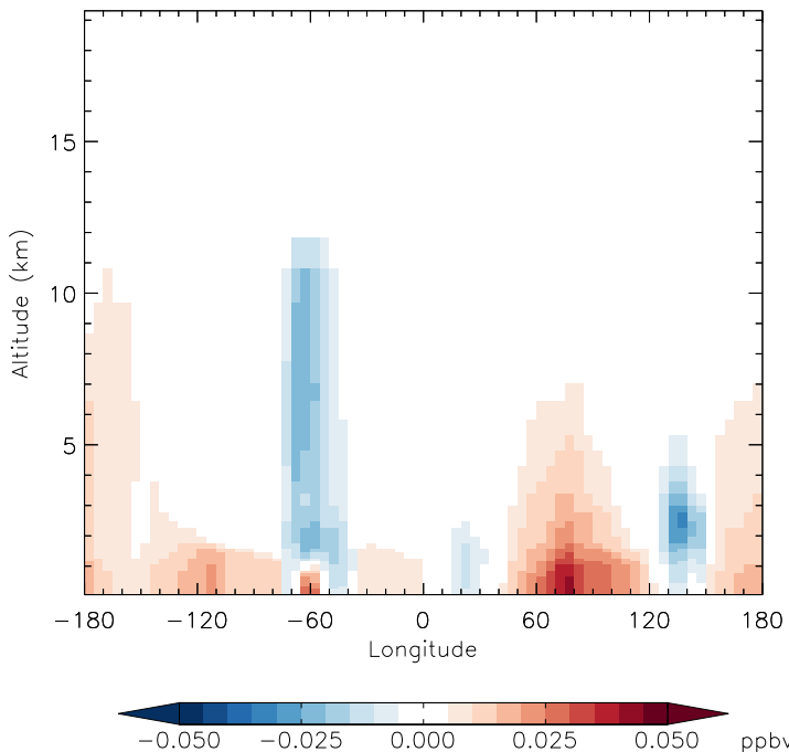
v11-01d-Run1 - v11-01b-Run0 MP - Diff along 15S for Jan
