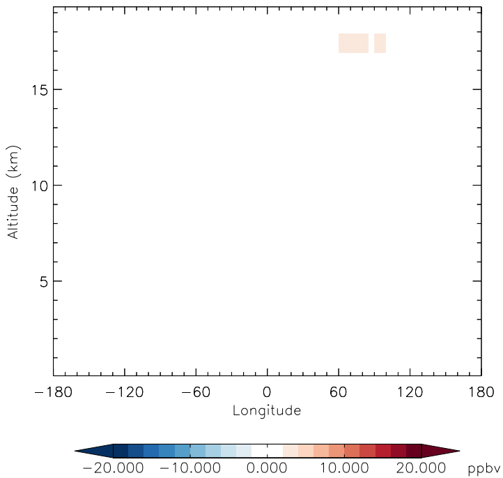
v11-01d-Run1 - v10-01-public-Run0 O3 - Diff along 15S for Jan
