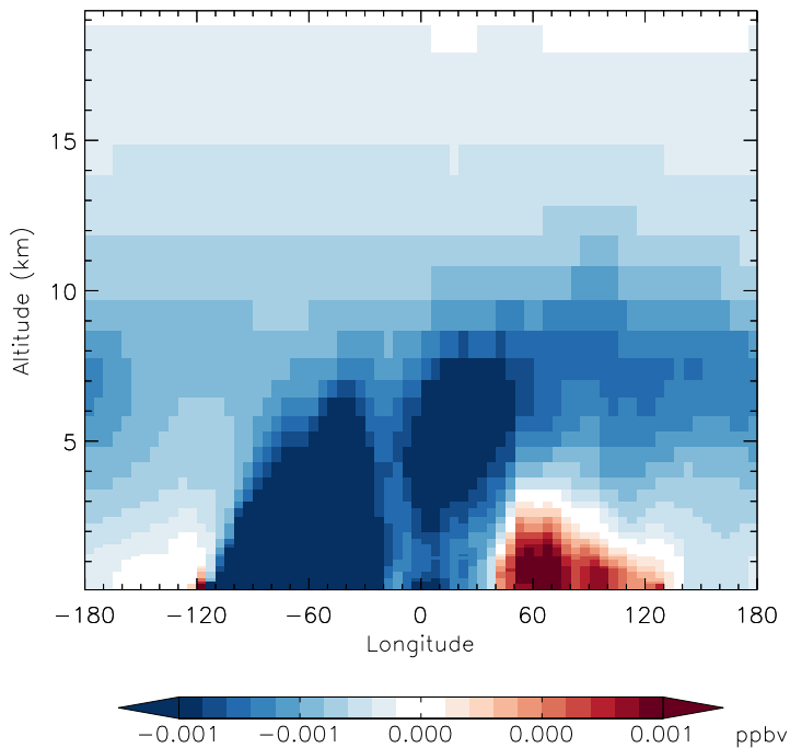
v11-01d-Run1 - v10-01-public-Run0 PPN - Diff along 42N for Jan
