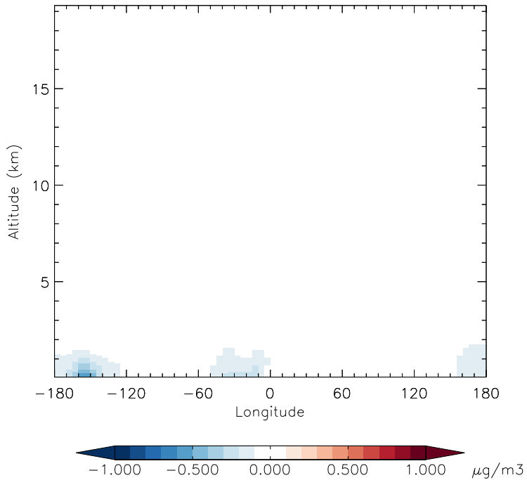
v11-01d-Run1 - v10-01-public-Run0 DMS - Diff along 42N for Jan
