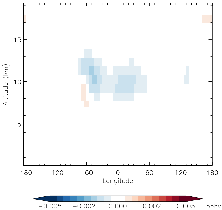
v11-01d-Run1 - v10-01-public-Run0 HNO 4 - Diff along 15S for Jan
