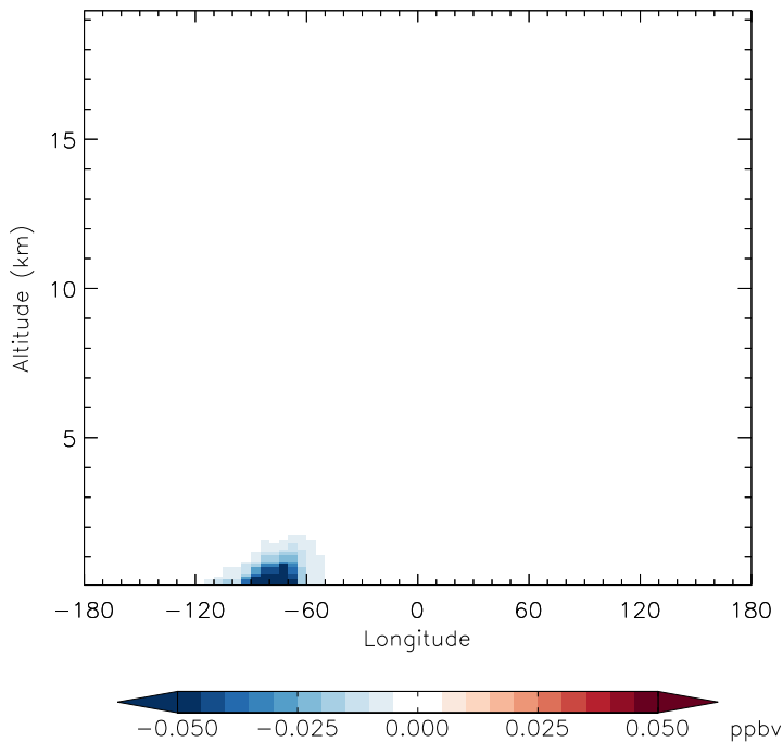
v11-01d-Run1 - v10-01-public-Run0 RCHO - Diff along 42N for Jan
