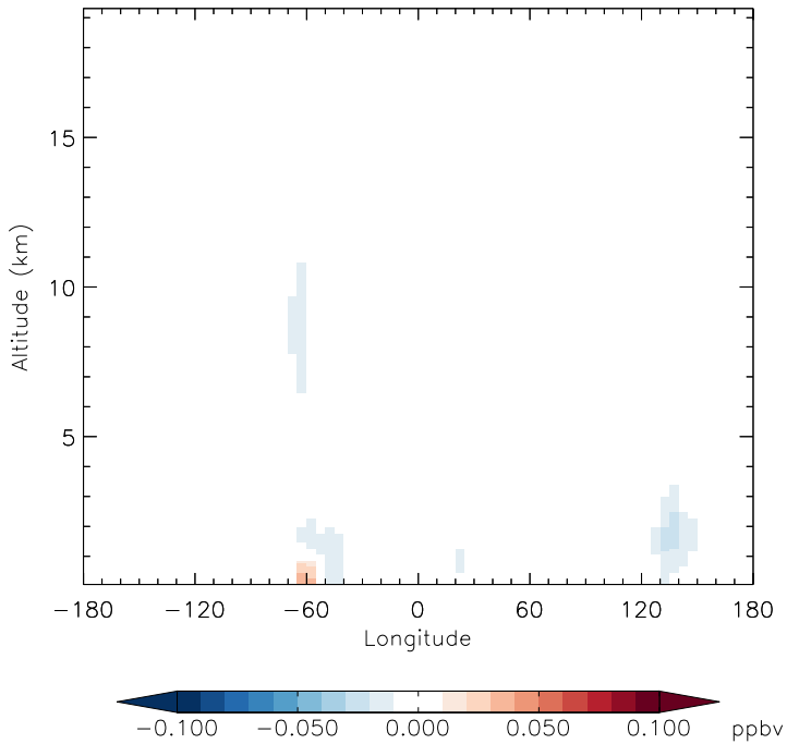
v11-01d-Run1 - v10-01-public-Run0 GLYC - Diff along 15S for Jan
