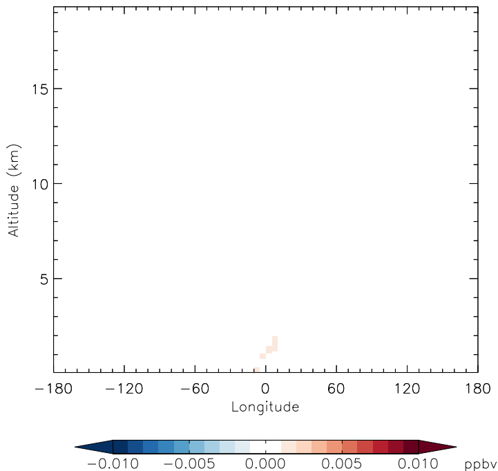
v11-01d-Run1 - v11-01b-Run0 NO3 - Diff along 42N for Jan
