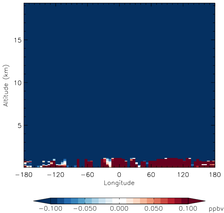
v11-01d-Run1 - v10-01-public-Run0 CH4 - Diff along 15S for Jan
