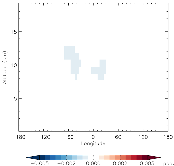
v11-01d-Run1 - v11-01b-Run0 HNO 4 - Diff along 15S for Jan
