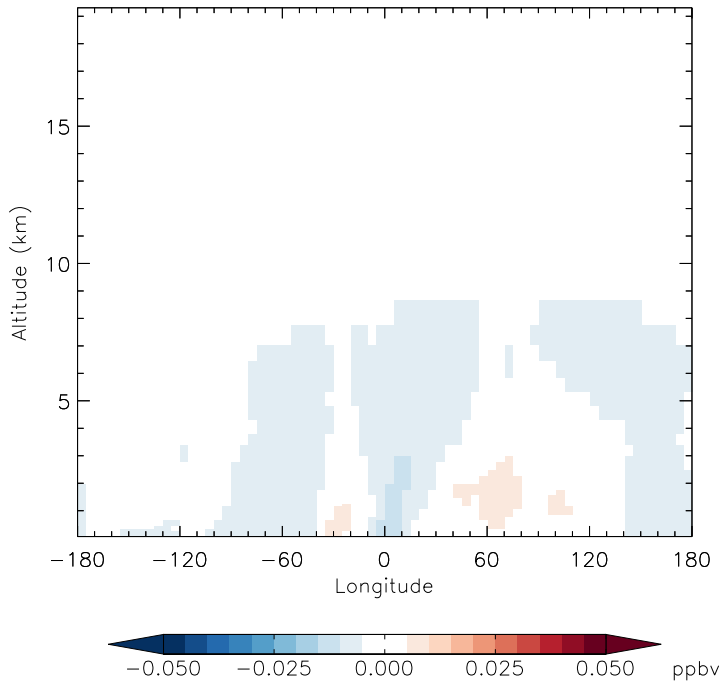
v11-01d-Run1 - v10-01-public-Run0 MP - Diff along 42N for Jan
