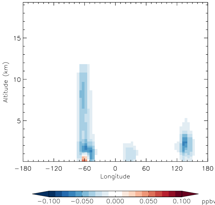
v11-01d-Run1 - v10-01-public-Run0 HAC - Diff along 15S for Jan
