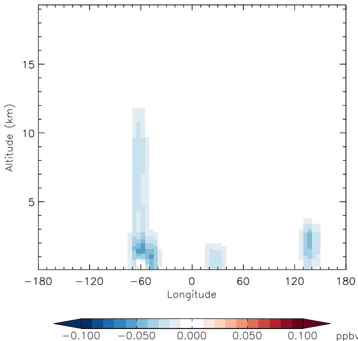
v11-01d-Run1 - v11-01b-Run0 HAC - Diff along 15S for Jan
