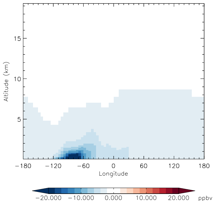
v11-01d-Run1 - v11-01b-Run0 CO - Diff along 42N for Jan
