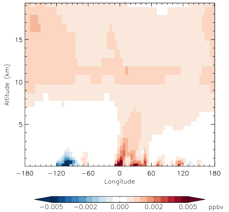
v11-01d-Run1 - v10-01-public-Run0 N2O5 - Diff along 42N for Jan
