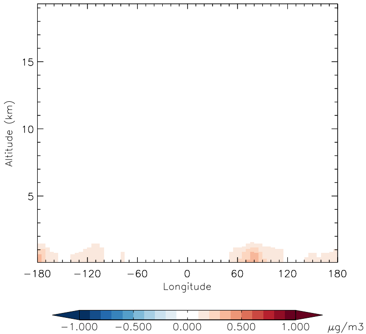
v11-01d-Run1 - v10-01-public-Run0 DMS - Diff along 15S for Jan
