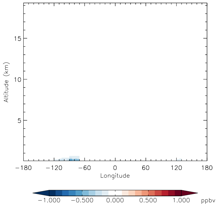
v11-01d-Run1 - v10-01-public-Run0 NO2 - Diff along 42N for Jan
