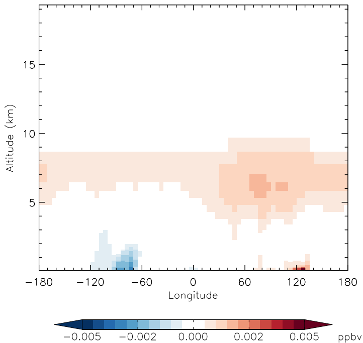
v11-01d-Run1 - v10-01-public-Run0 HNO 4 - Diff along 42N for Jan
