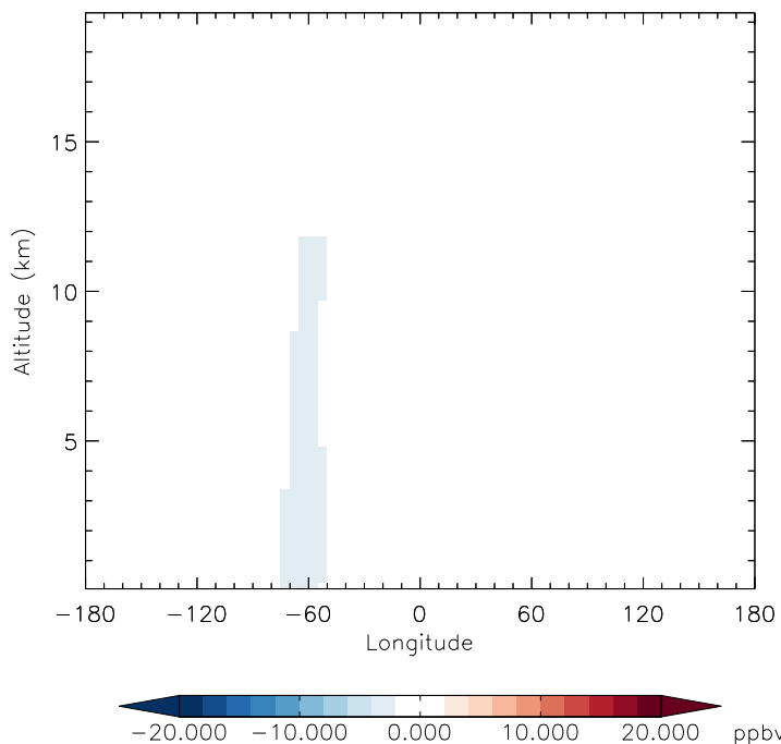
v11-01d-Run1 - v11-01b-Run0 CO - Diff along 15S for Jan
