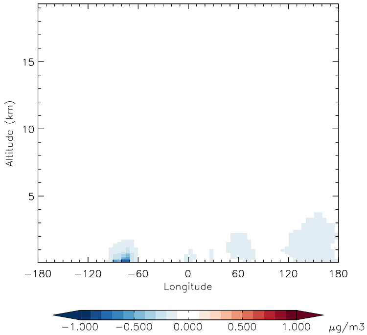
v11-01d-Run1 - v10-01-public-Run0 SO2 - Diff along 42N for Jan
