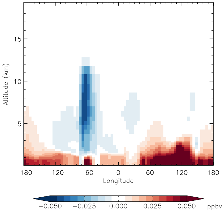
v11-01d-Run1 - v10-01-public-Run0 MP - Diff along 15S for Jan
