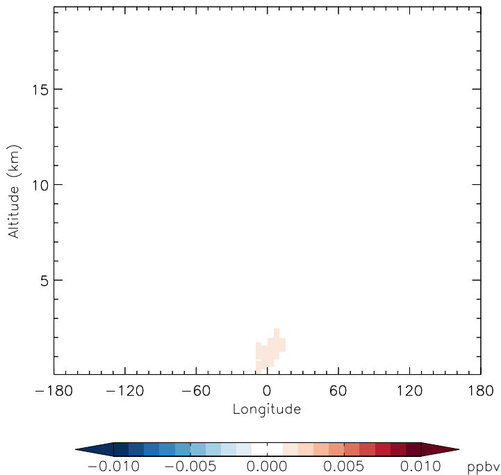
v11-01d-Run1 - v10-01-public-Run0 NO3 - Diff along 42N for Jan
