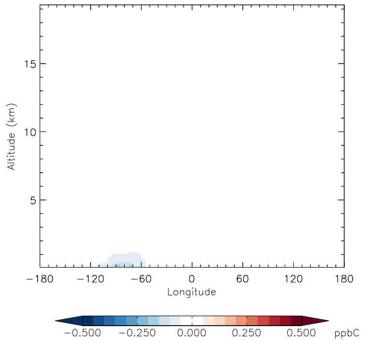
v11-01d-Run1 - v10-01-public-Run0 C3H8 - Diff along 42N for Jan
