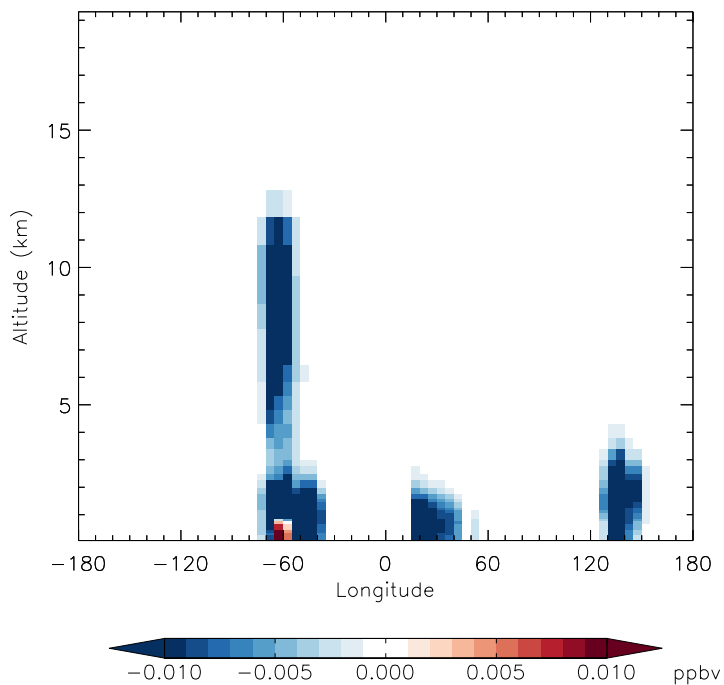
v11-01d-Run1 - v11-01b-Run0 IEPOX - Diff along 15S for Jan
