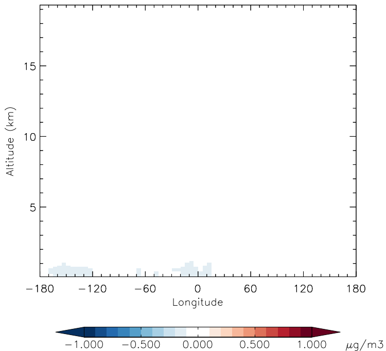
v11-01d-Run1 - v11-01b-Run0 S04 - Diff along 42N for Jan
