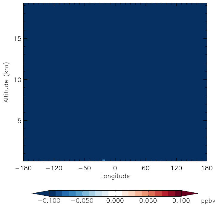
v11-01d-Run1 - v10-01-public-Run0 CH4 - Diff along 42N for Jan
