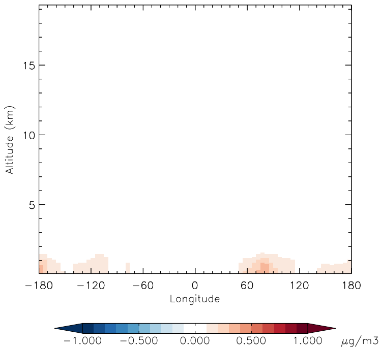
v11-01d-Run1 - v11-01b-Run0 DMS - Diff along 15S for Jan
