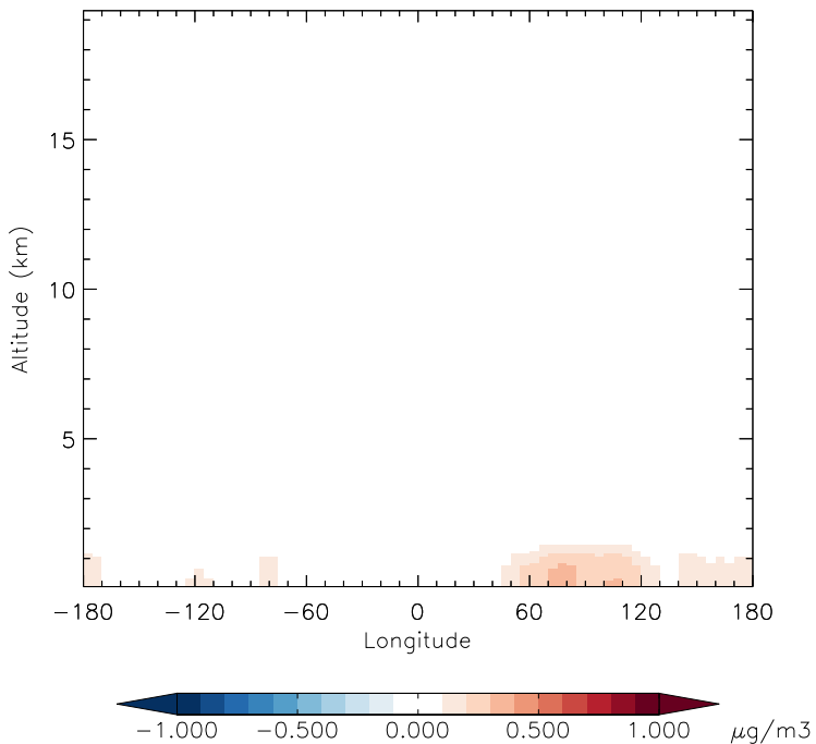
v11-01d-Run1 - v11-01b-Run0 S04 - Diff along 15S for Jan
