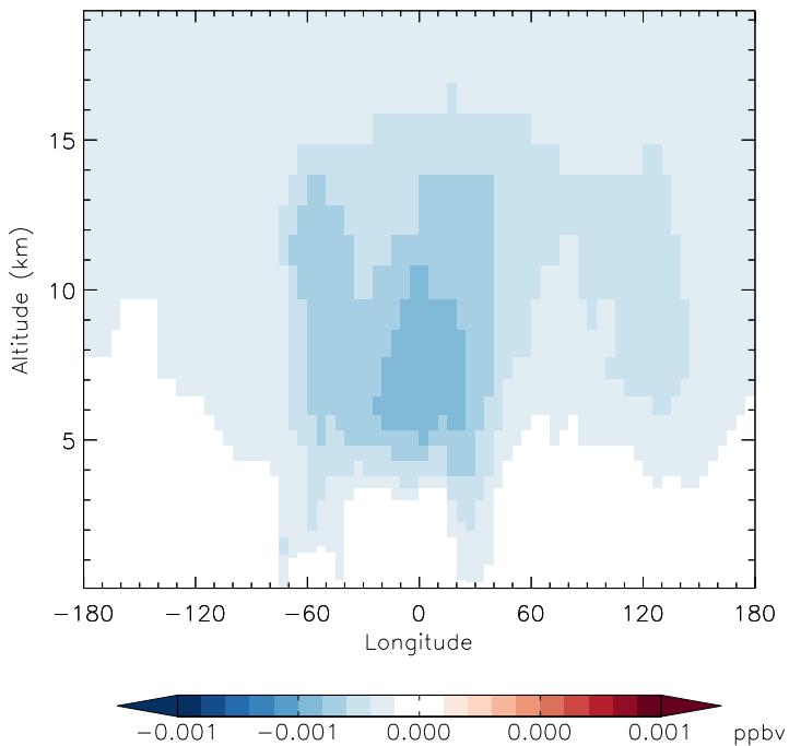
v11-01d-Run1 - v10-01-public-Run0 PPN - Diff along 15S for Jan
