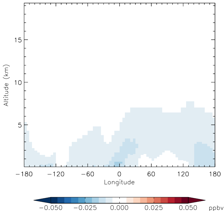
v11-01d-Run1 - v11-01b-Run0 MP - Diff along 42N for Jan
