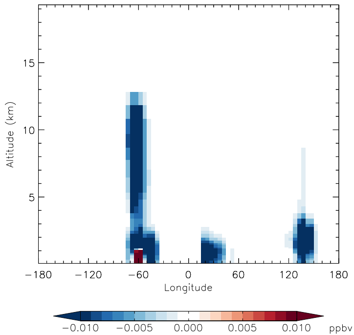
v11-01d-Run1 - v10-01-public-Run0 IEPOX - Diff along 15S for Jan
