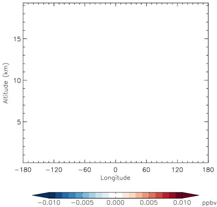
v11-01d-Run1 - v10-01-public-Run0 PMN - Diff along 15S for Jan
