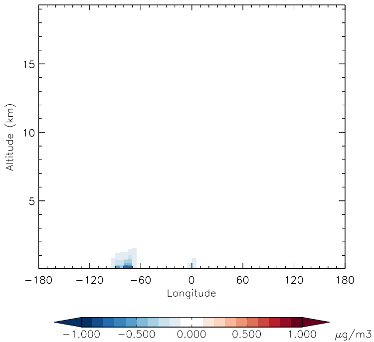
v11-01d-Run1 - v11-01b-Run0 SO2 - Diff along 42N for Jan
