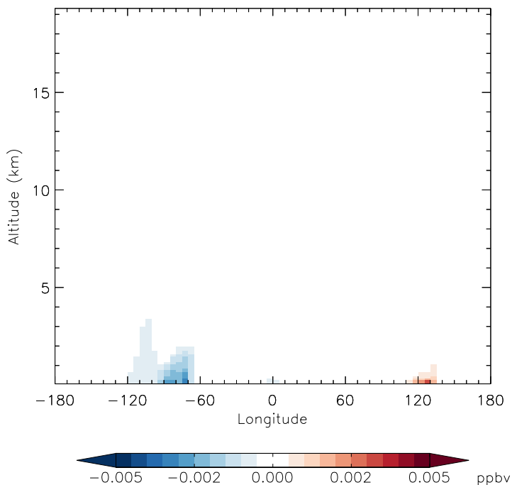
v11-01d-Run1 - v11-01b-Run0 HNO 4 - Diff along 42N for Jan
