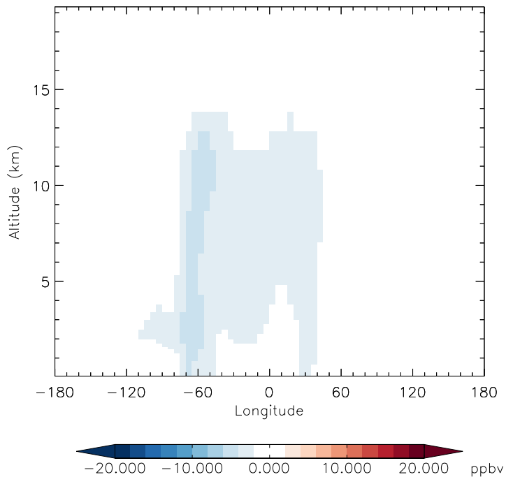
v11-01d-Run1 - v10-01-public-Run0 CO - Diff along 15S for Jan
