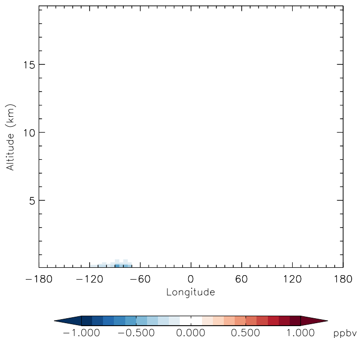
v11-01d-Run1 - v11-01b-Run0 NO2 - Diff along 42N for Jan
