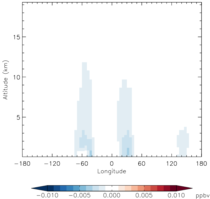
v11-01d-Run1 - v10-01-public-Run0 R4N2 - Diff along 15S for Jan
