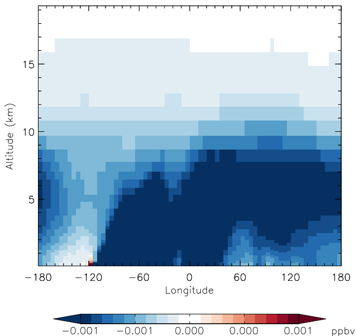
v11-01d-Run1 - v11-01b-Run0 PPN - Diff along 42N for Jan
