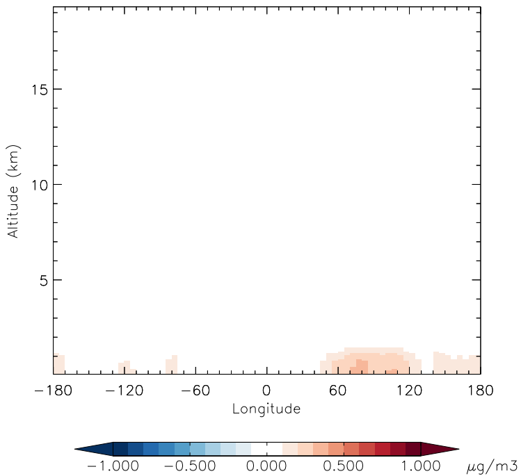
v11-01d-Run1 - v10-01-public-Run0 S04 - Diff along 15S for Jan
