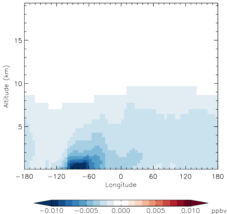
v11-01d-Run1 - v11-01b-Run0 R4N2 - Diff along 42N for Jan
