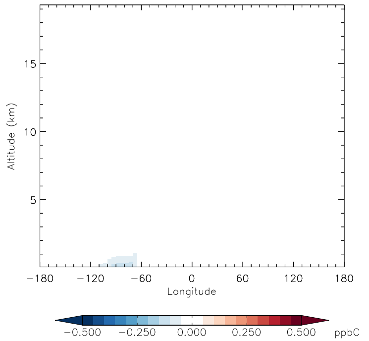
v11-01d-Run1 - v11-01b-Run0 C3H8 - Diff along 42N for Jan
