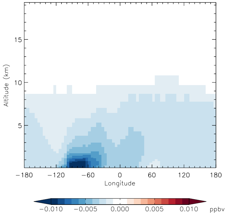
v11-01d-Run1 - v10-01-public-Run0 R4N2 - Diff along 42N for Jan
