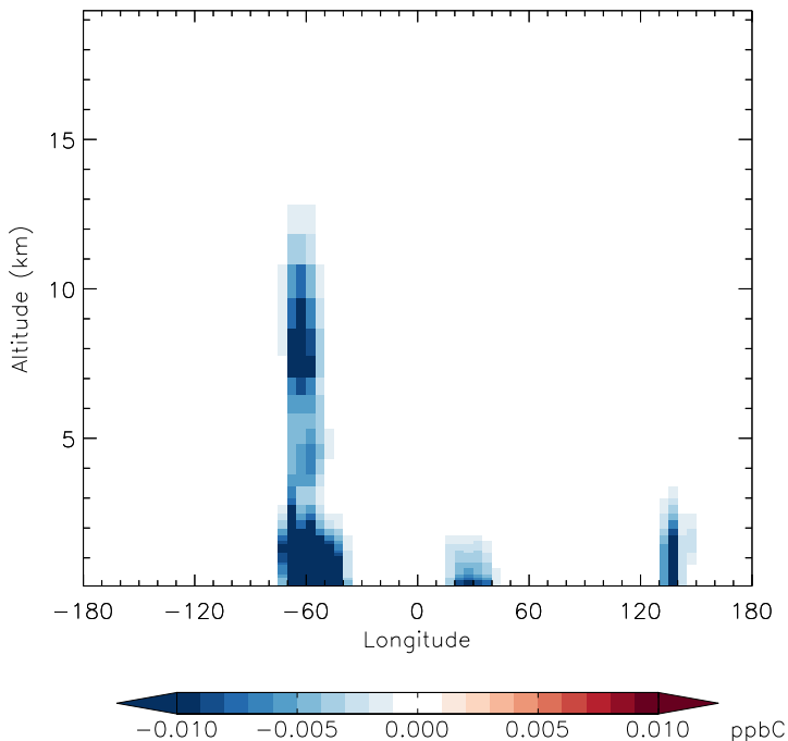
v11-01d-Run1 - v11-01b-Run0 PRPE - Diff along 15S for Jan
