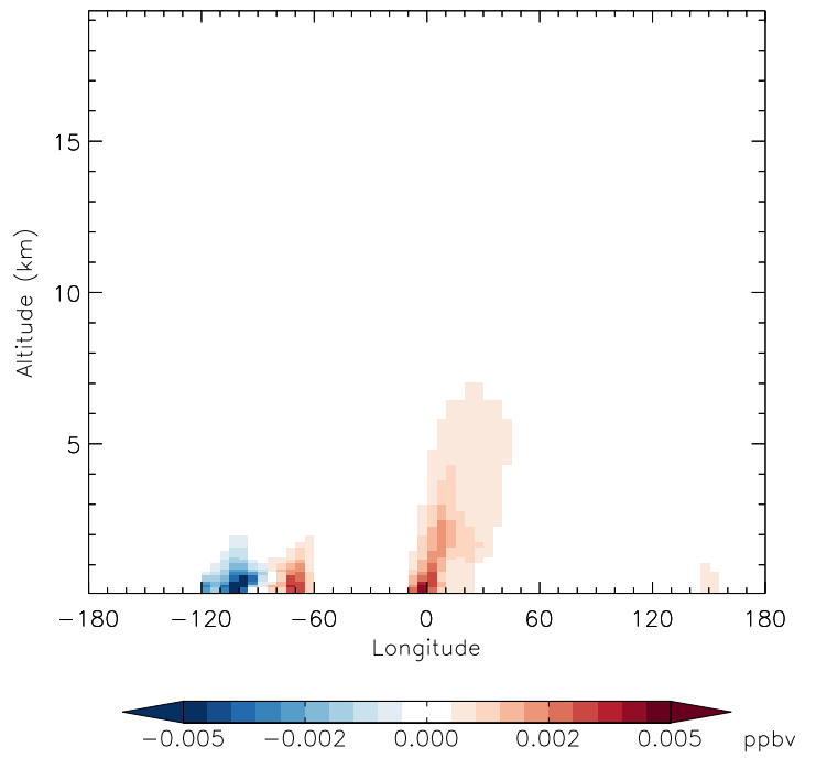
v11-01d-Run1 - v11-01b-Run0 N2O5 - Diff along 42N for Jan
