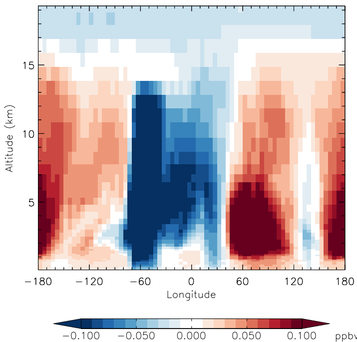
v11-01d-Run1 - v11-01b-Run0 CH4 - Diff along 15S for Jan
