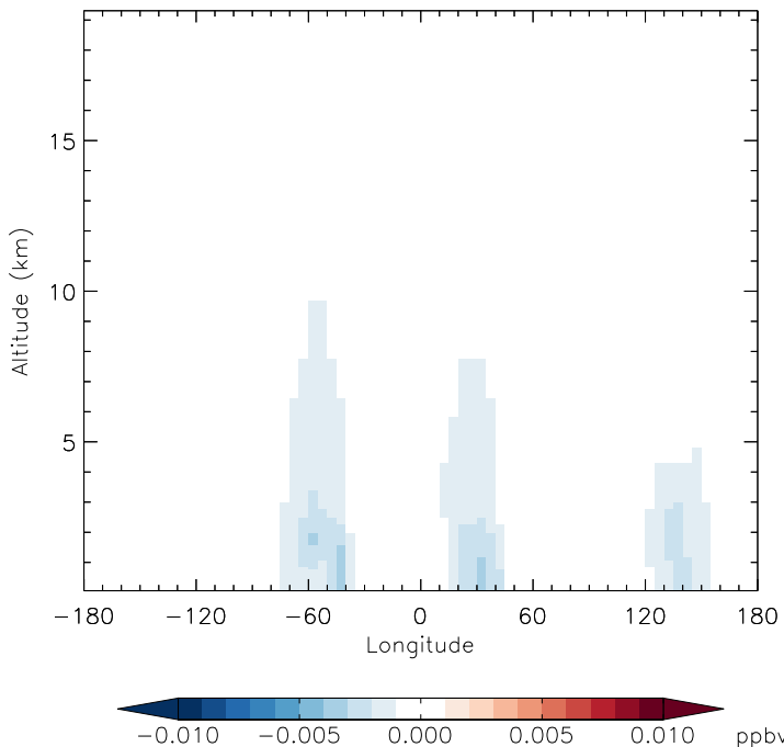
v11-01d-Run1 - v11-01b-Run0 R4N2 - Diff along 15S for Jan
