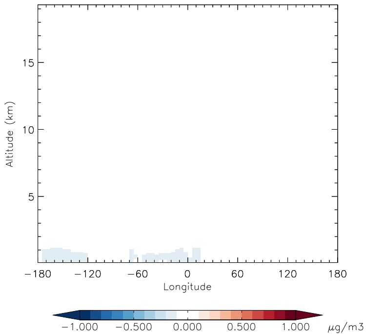
v11-01d-Run1 - v10-01-public-Run0 S04 - Diff along 42N for Jan
