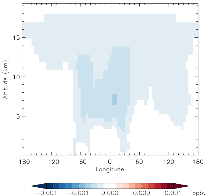
v11-01d-Run1 - v11-01b-Run0 PPN - Diff along 15S for Jan
