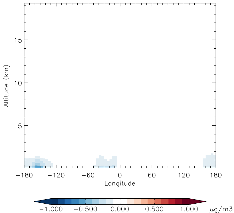
v11-01d-Run1 - v11-01b-Run0 DMS - Diff along 42N for Jan
