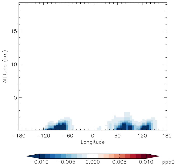
v11-01d-Run1 - v10-01-public-Run0 PRPE - Diff along 42N for Jan
