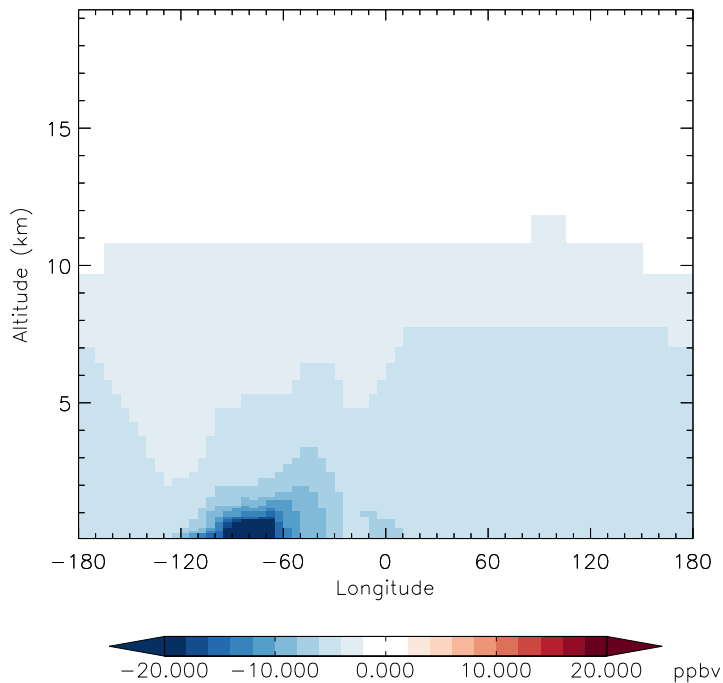
v11-01d-Run1 - v10-01-public-Run0 CO - Diff along 42N for Jan
