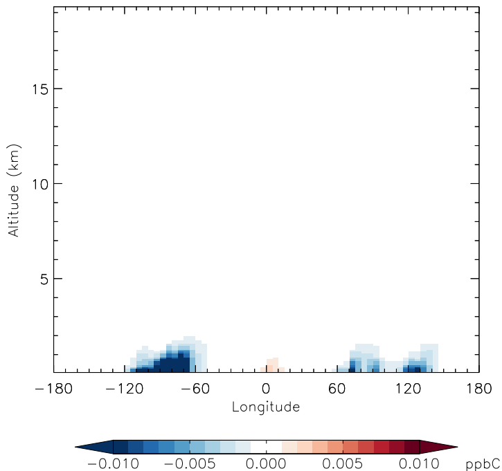
v11-01d-Run1 - v11-01b-Run0 PRPE - Diff along 42N for Jan
