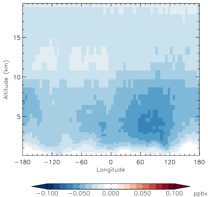
v11-01d-Run1 - v11-01b-Run0 CH4 - Diff along 42N for Jan
