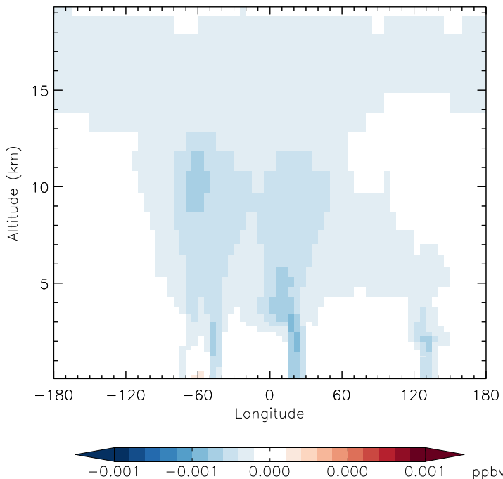
v11-01d-Run1 - v11-01b-Run0 PPN - Diff along 15S for Oct
