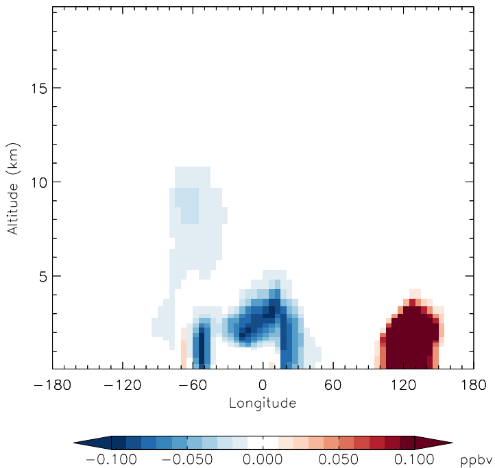
v11-01d-Run1 - v10-01-public-Run0 H2O2 - Diff along 15S for Oct
