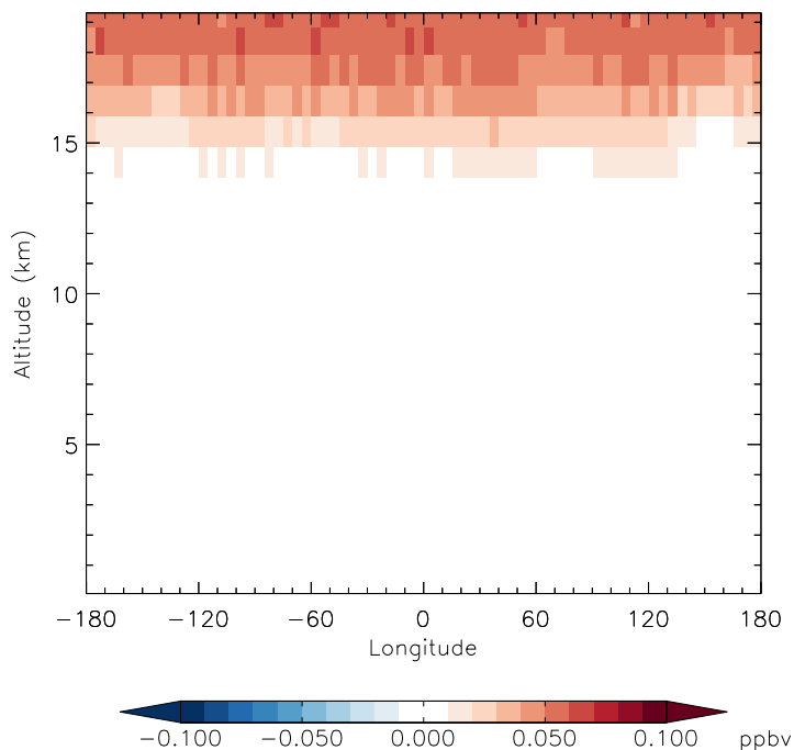
v11-01d-Run1 - v11-01b-Run0 H2O - Diff along 42N for Oct
