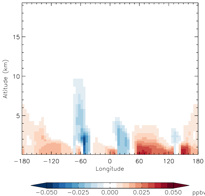
v11-01d-Run1 - v11-01b-Run0 MP - Diff along 15S for Oct
