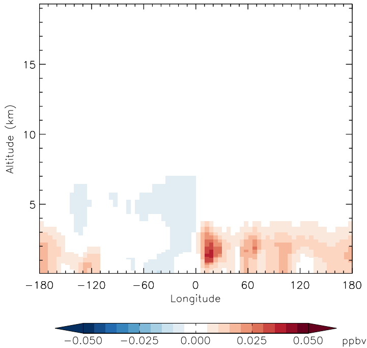
v11-01d-Run1 - v10-01-public-Run0 MP - Diff along 42N for Oct
