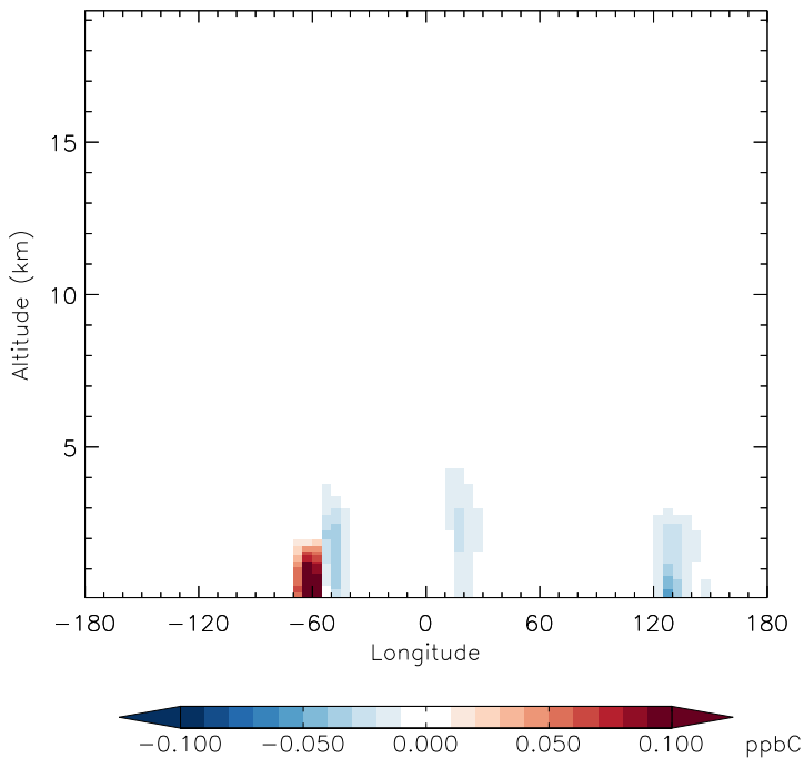
v11-01d-Run1 - v11-01b-Run0 MEK - Diff along 15S for Oct
