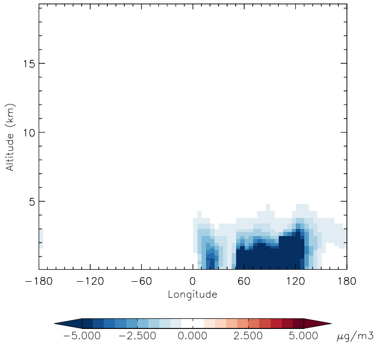
v11-01d-Run1 - v10-01-public-Run0 DST2 - Diff along 42N for Oct
