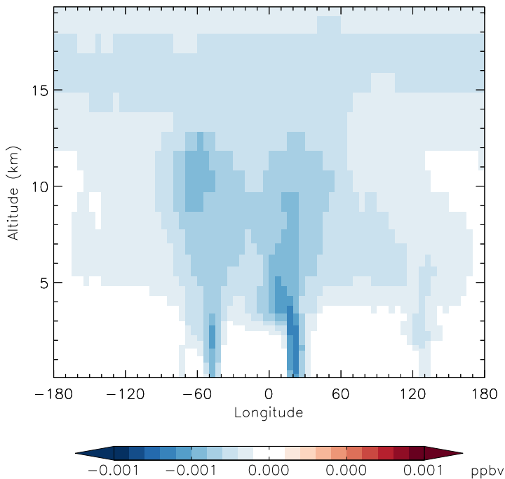
v11-01d-Run1 - v10-01-public-Run0 PPN - Diff along 15S for Oct
