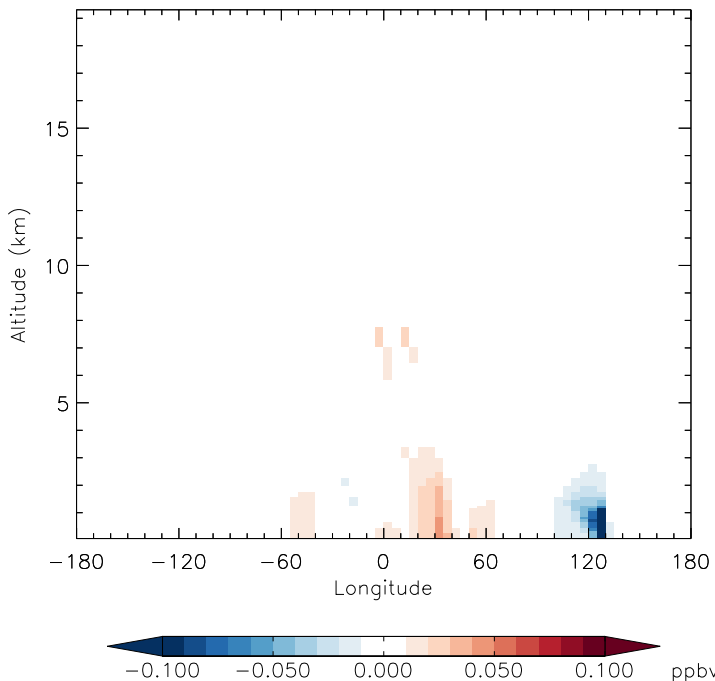
v11-01d-Run1 - v11-01b-Run0 HNO 3 - Diff along 15S for Oct
