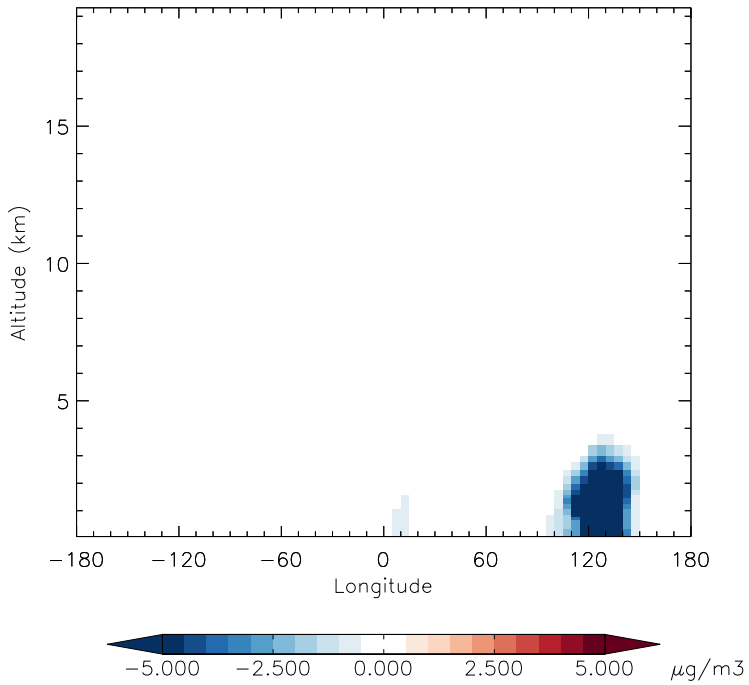
v11-01d-Run1 - v10-01-public-Run0 DST2 - Diff along 15S for Oct
