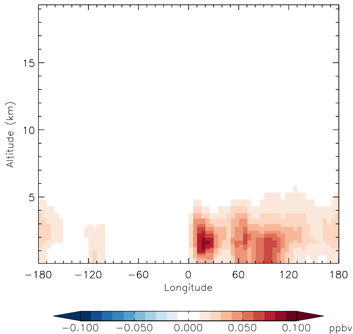
v11-01d-Run1 - v10-01-public-Run0 H2O2 - Diff along 42N for Oct
