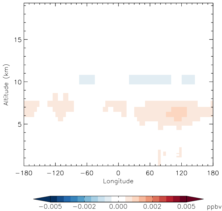
v11-01d-Run1 - v10-01-public-Run0 HNO4 - Diff along 42N for Oct
