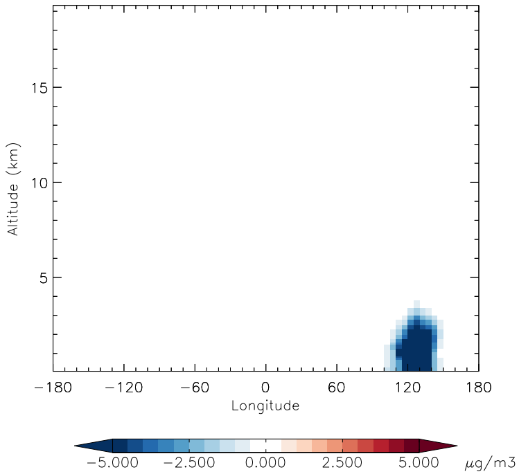
v11-01d-Run1 - v10-01-public-Run0 DST3 - Diff along 15S for Oct
