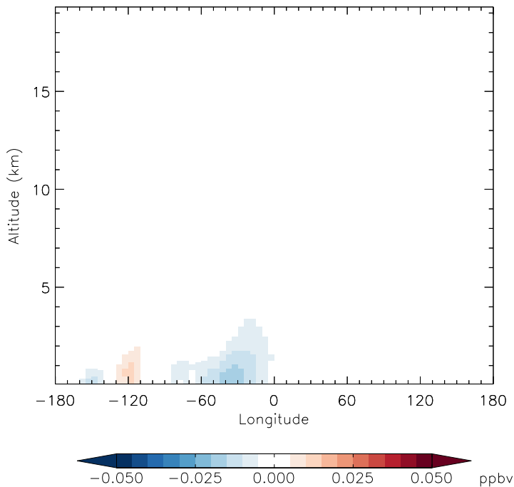
v11-01d-Run1 - v11-01b-Run0 MP - Diff along 42N for Oct
