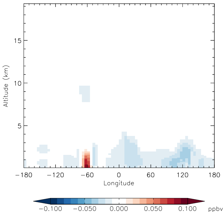
v11-01d-Run1 - v11-01b-Run0 H2O2 - Diff along 15S for Oct
