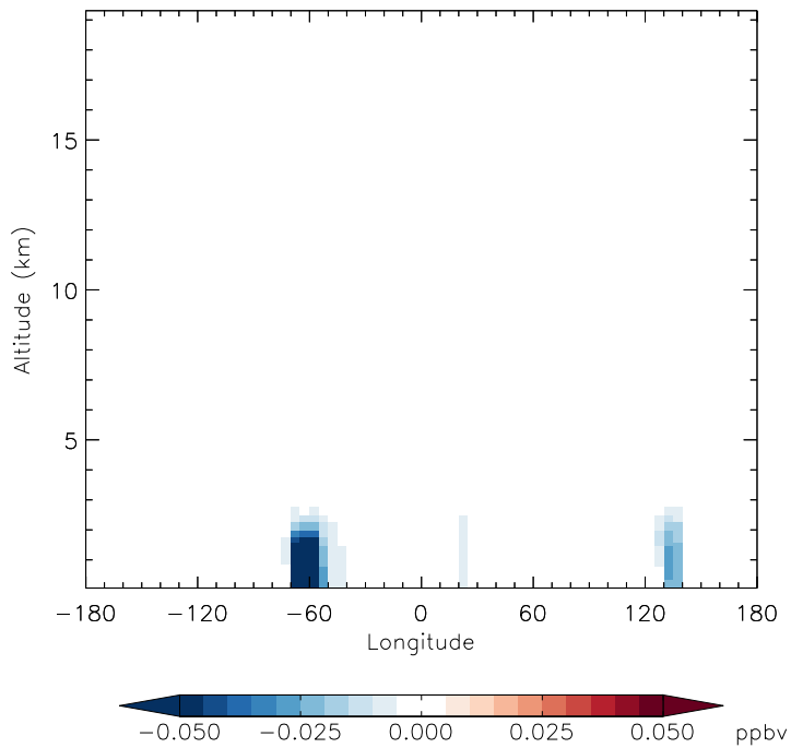
v11-01d-Run1 - v10-01-public-Run0 MACR - Diff along 15S for Oct
