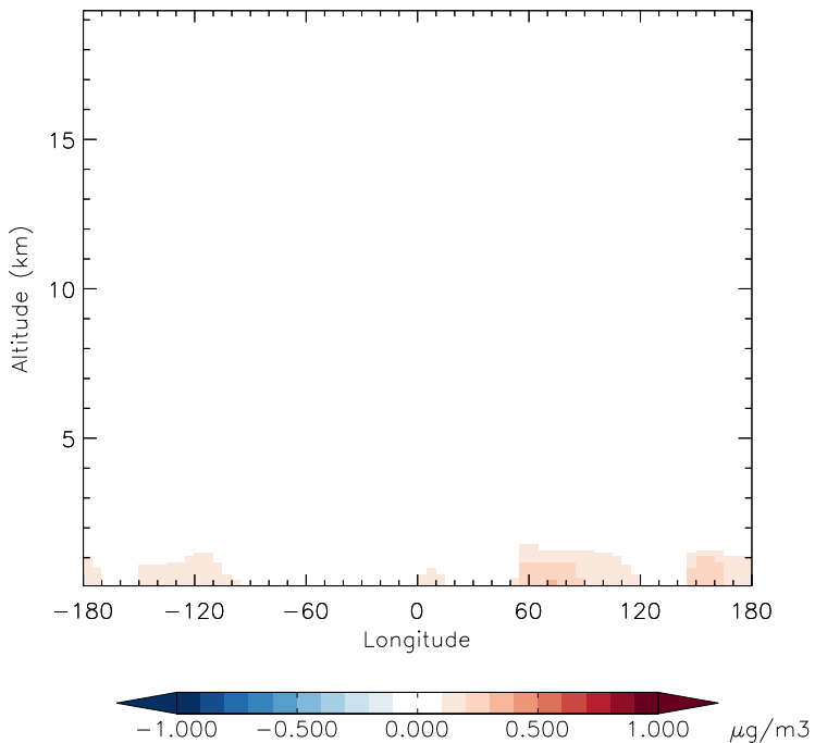
v11-01d-Run1 - v11-01b-Run0 DMS - Diff along 15S for Oct
