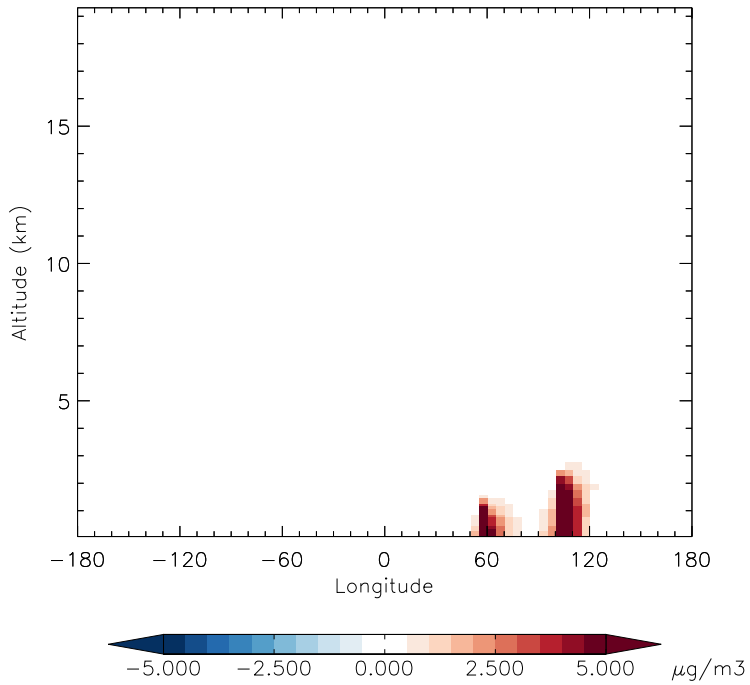
v11-01d-Run1 - v10-01-public-Run0 DST4 - Diff along 42N for Oct
