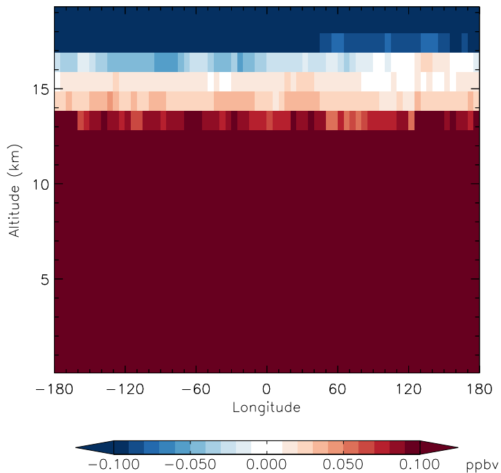
v11-01d-Run1 - v10-01-public-Run0 H2O - Diff along 15S for Oct
