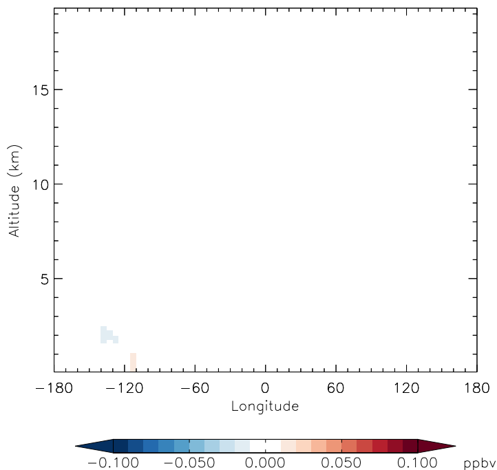
v11-01d-Run1 - v11-01b-Run0 H2O2 - Diff along 42N for Oct
