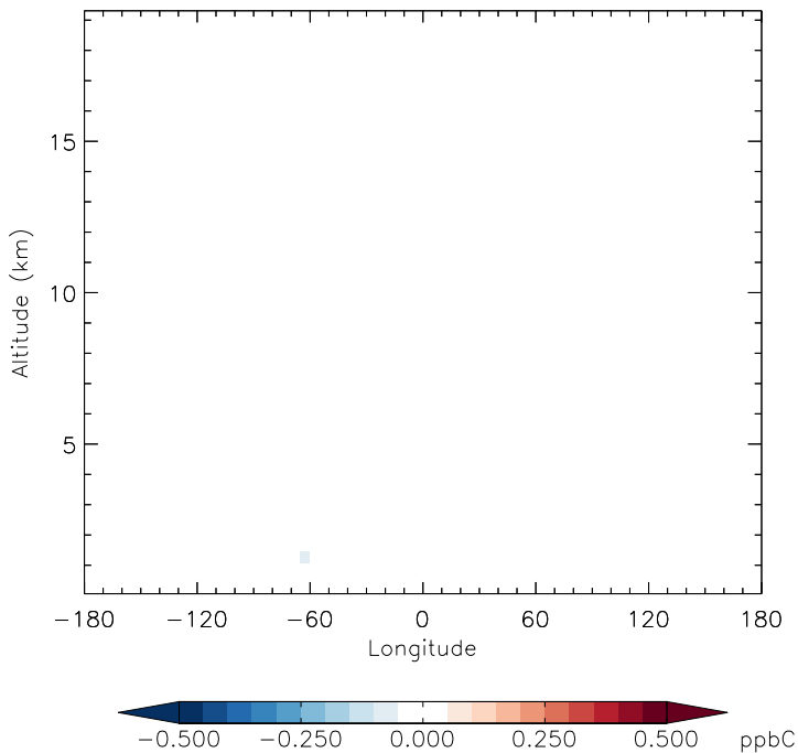
v11-01d-Run1 - v11-01b-Run0 ALD2 - Diff along 15S for Oct
