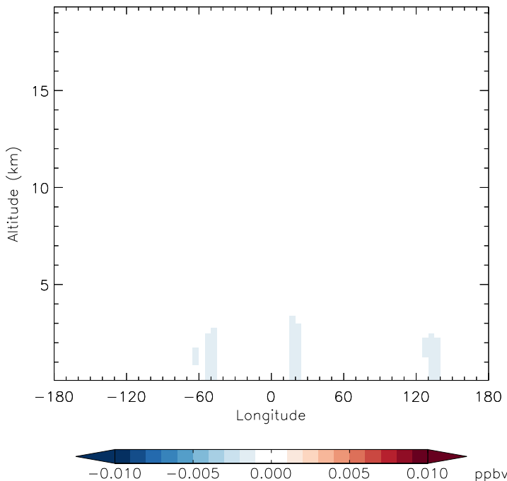
v11-01d-Run1 - v11-01b-Run0 MMN - Diff along 15S for Oct
