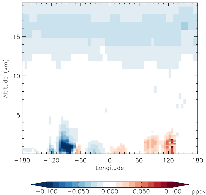
v11-01d-Run1 - v10-01-public-Run0 HNO 3 - Diff along 42N for Oct
