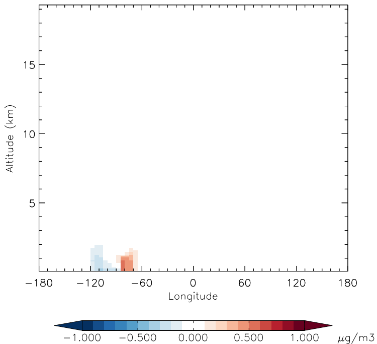
v11-01d-Run1 - v11-01b-Run0 NIT - Diff along 42N for Oct
