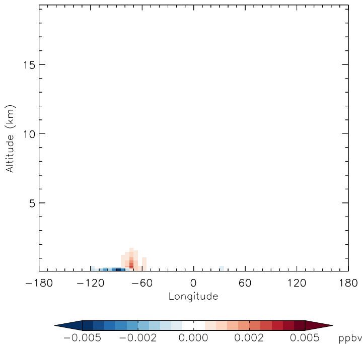
v11-01d-Run1 - v11-01b-Run0 N2O5 - Diff along 42N for Oct
