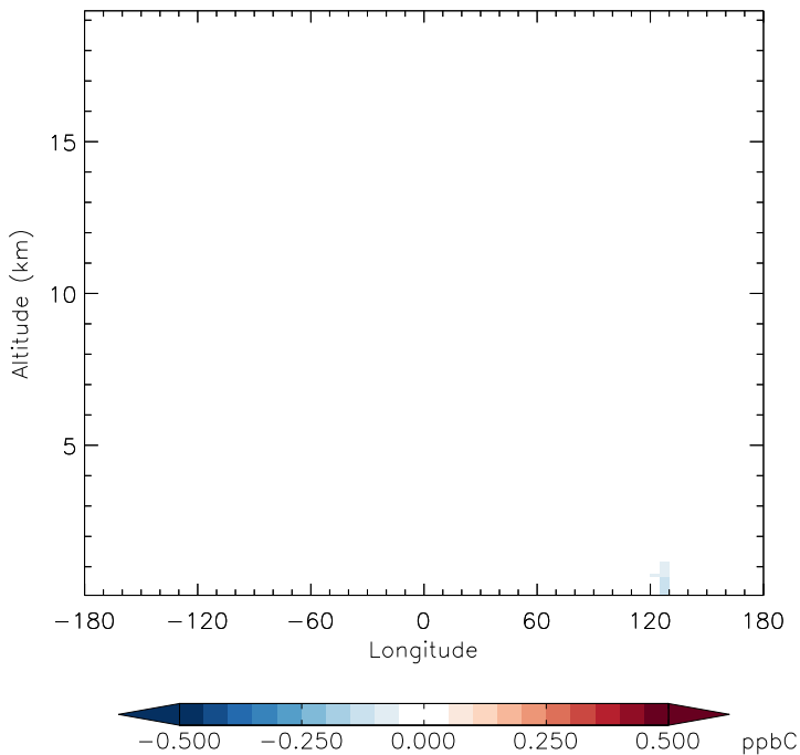
v11-01d-Run1 - v11-01b-Run0 ACET - Diff along 15S for Oct
