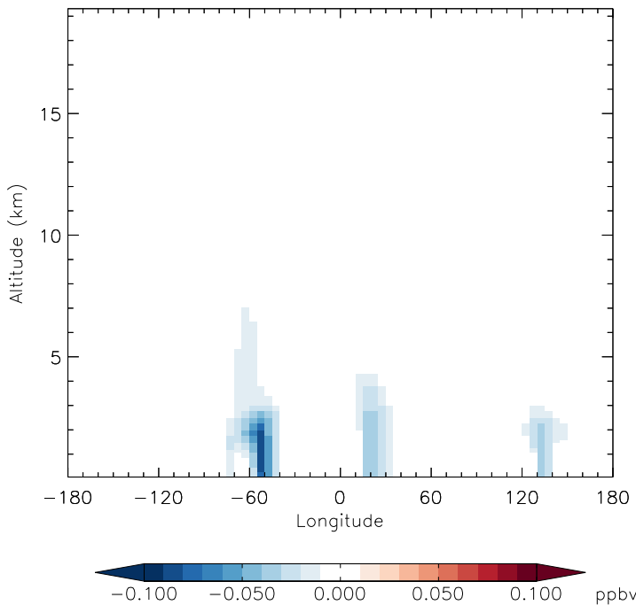
v11-01d-Run1 - v11-01b-Run0 HAC - Diff along 15S for Oct
