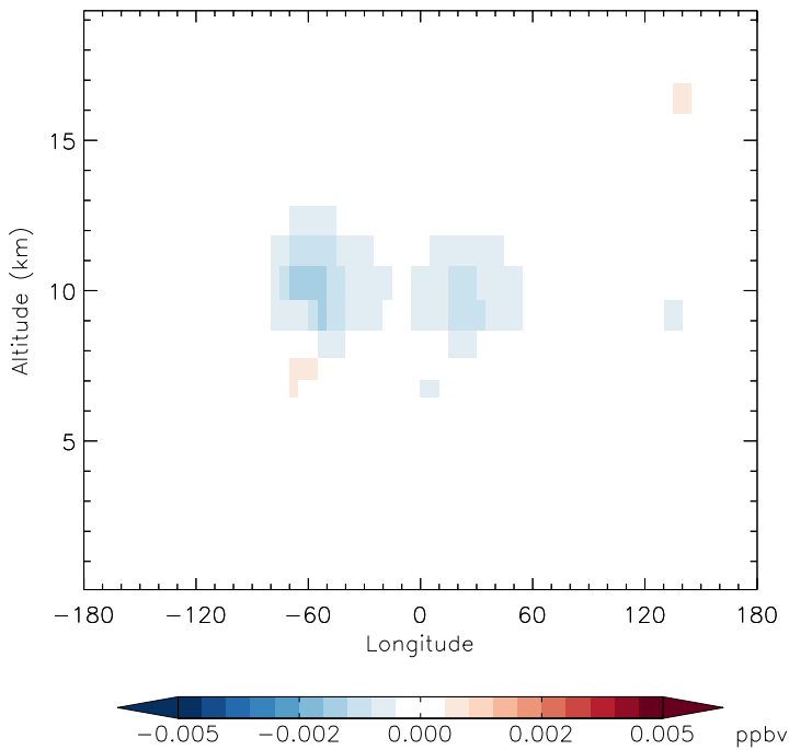
v11-01d-Run1 - v10-01-public-Run0 HNO4 - Diff along 15S for Oct
