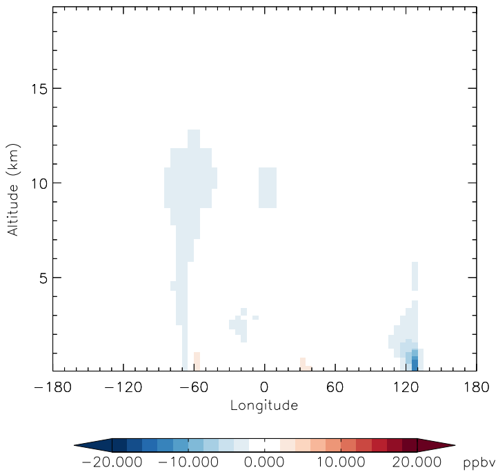
v11-01d-Run1 - v10-01-public-Run0 CO - Diff along 15S for Oct
