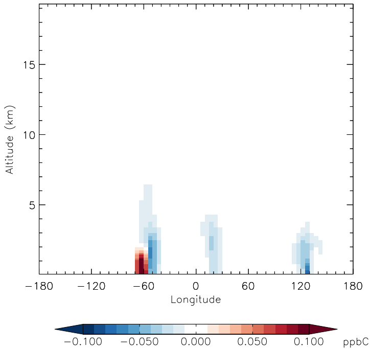
v11-01d-Run1 - v10-01-public-Run0 MEK - Diff along 15S for Oct
