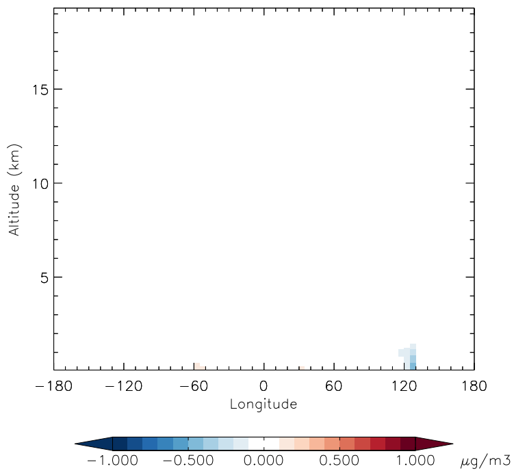
v11-01d-Run1 - v11-01b-Run0 OCPI - Diff along 15S for Oct
