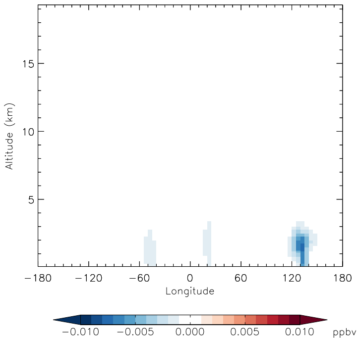
v11-01d-Run1 - v10-01-public-Run0 MMN - Diff along 15S for Oct
