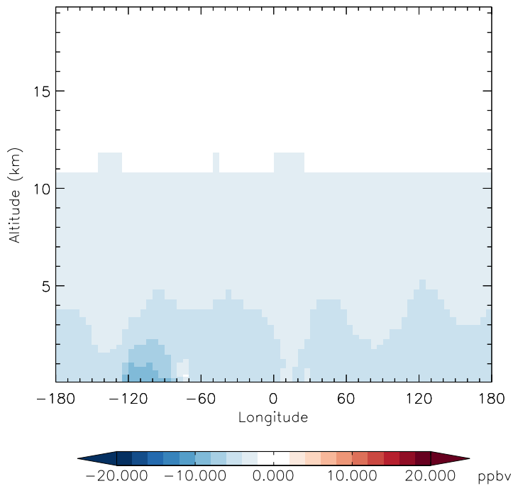
v11-01d-Run1 - v10-01-public-Run0 CO - Diff along 42N for Oct
