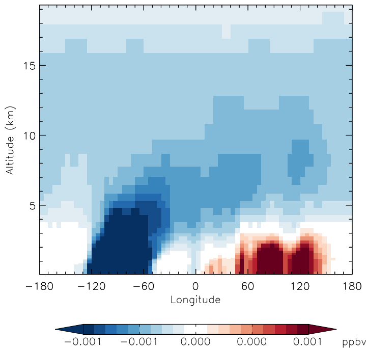
v11-01d-Run1 - v10-01-public-Run0 PPN - Diff along 42N for Oct
