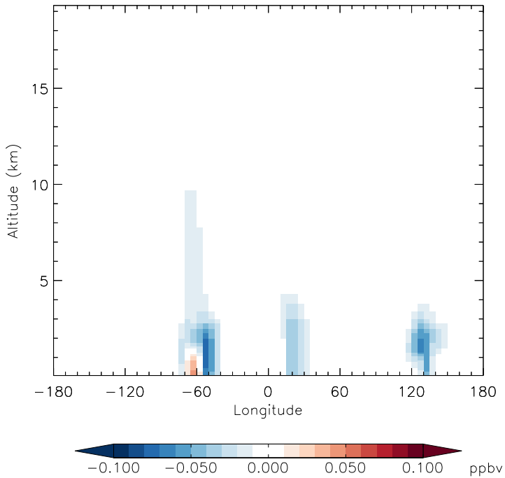
v11-01d-Run1 - v10-01-public-Run0 HAC - Diff along 15S for Oct
