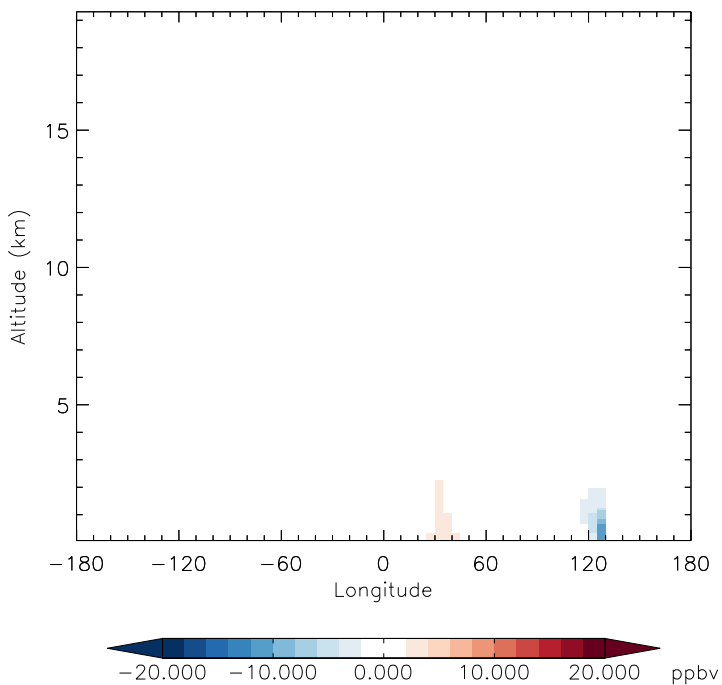
v11-01d-Run1 - v11-01b-Run0 CO - Diff along 15S for Oct
