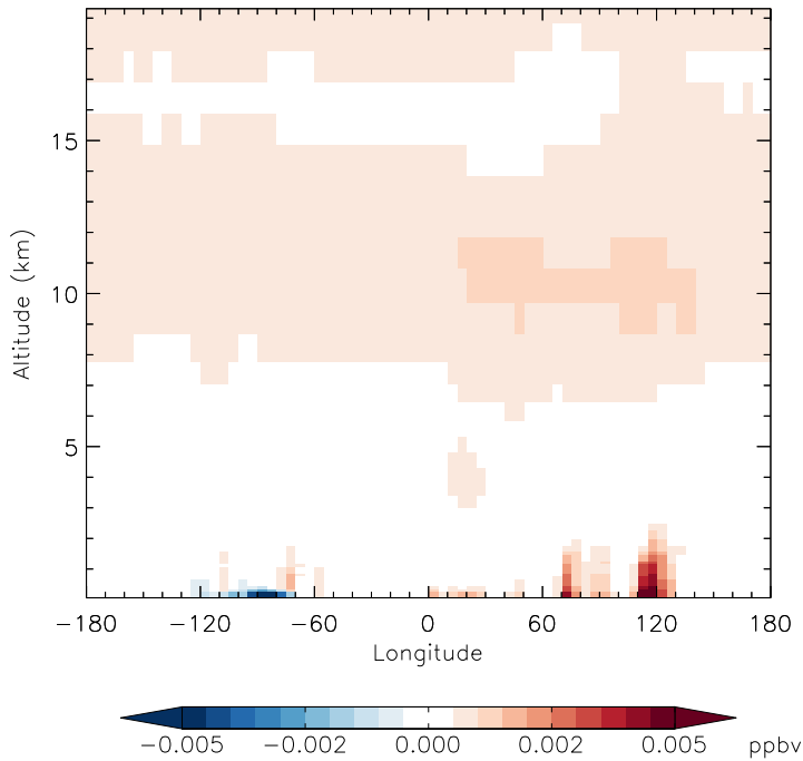
v11-01d-Run1 - v10-01-public-Run0 N2O5 - Diff along 42N for Oct
