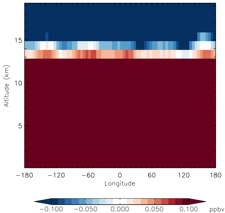
v11-01d-Run1 - v10-01-public-Run0 H2O - Diff along 42N for Oct
