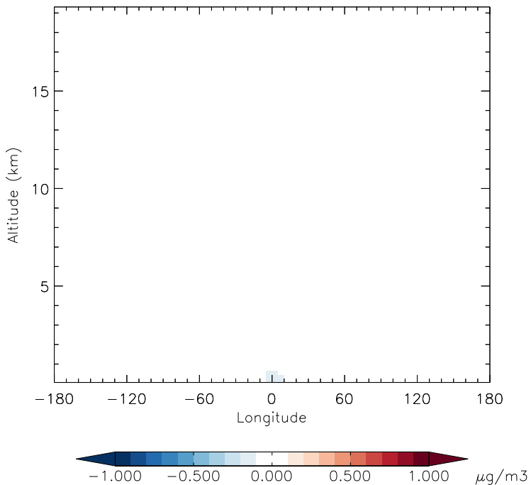
v11-01d-Run1 - v11-01b-Run0 NIT - Diff along 15S for Oct
