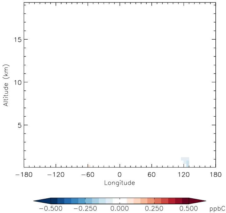
v11-01d-Run1 - v10-01-public-Run0 ACET - Diff along 15S for Oct
