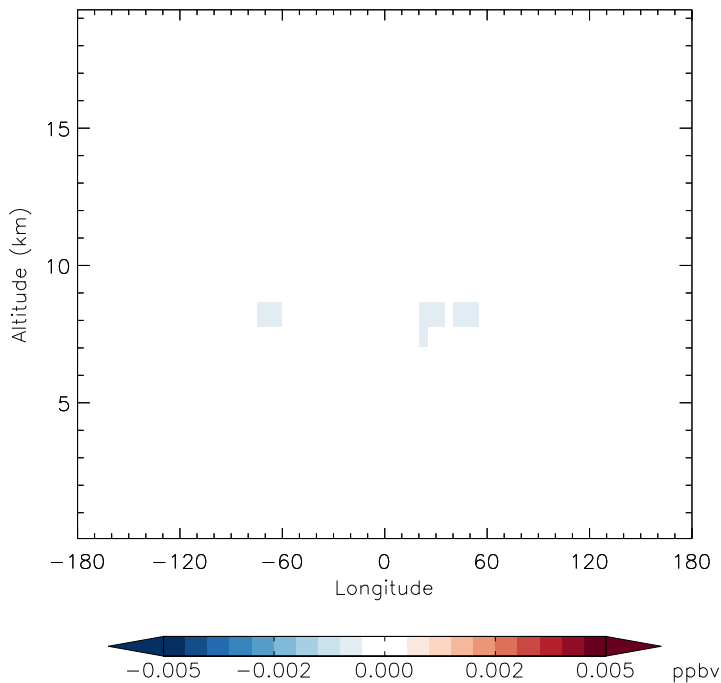
v11-01d-Run1 - v11-01b-Run0 HNO4 - Diff along 42N for Oct
