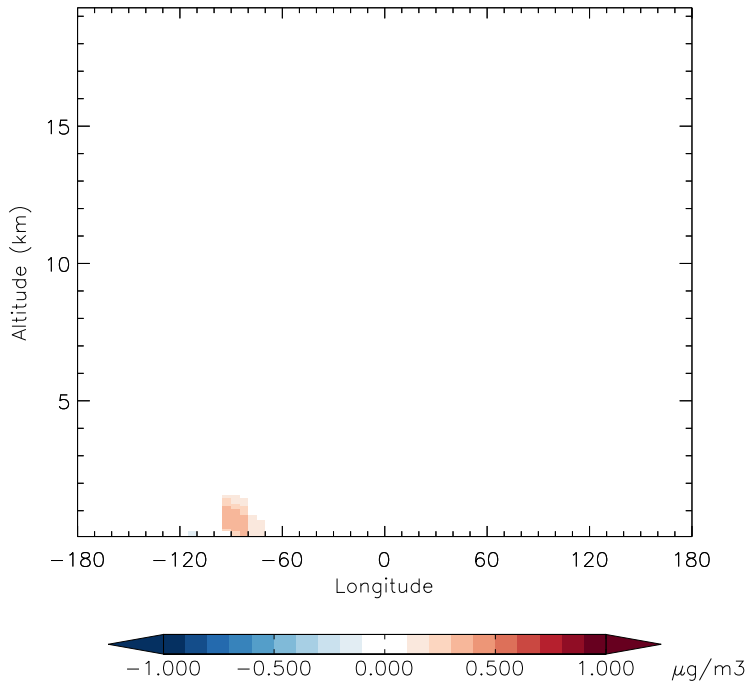
v11-01d-Run1 - v10-01-public-Run0 NH3 - Diff along 42N for Oct
