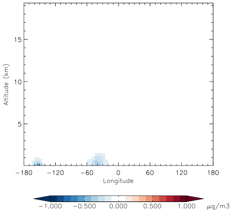
v11-01d-Run1 - v11-01b-Run0 DMS - Diff along 42N for Oct
