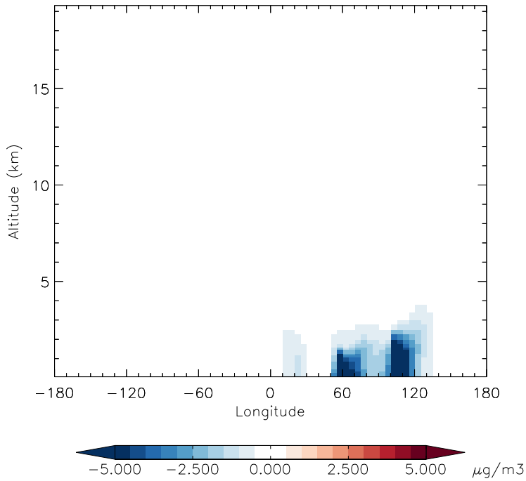
v11-01d-Run1 - v10-01-public-Run0 DST1 - Diff along 42N for Oct
