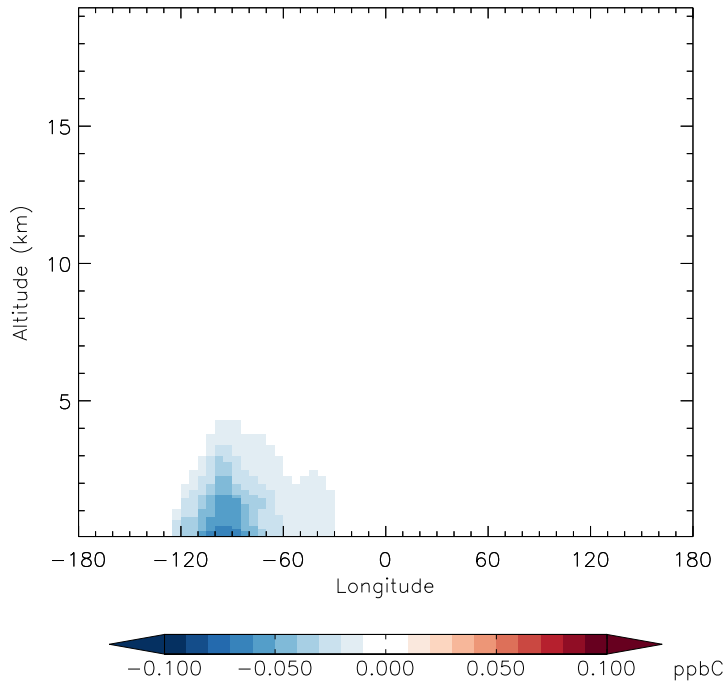
v11-01d-Run1 - v10-01-public-Run0 MEK - Diff along 42N for Oct
