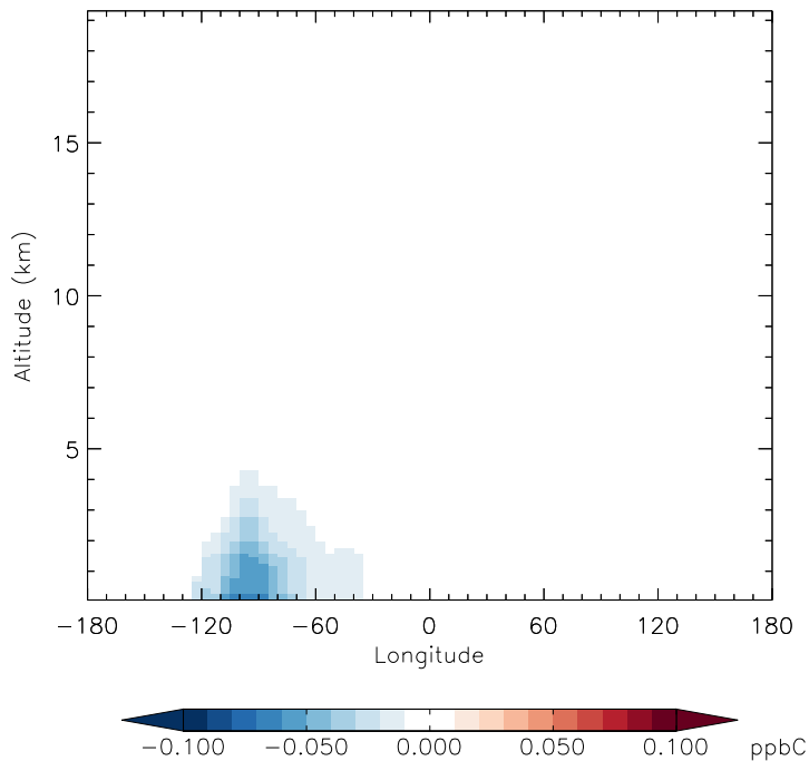
v11-01d-Run1 - v11-01b-Run0 MEK - Diff along 42N for Oct
