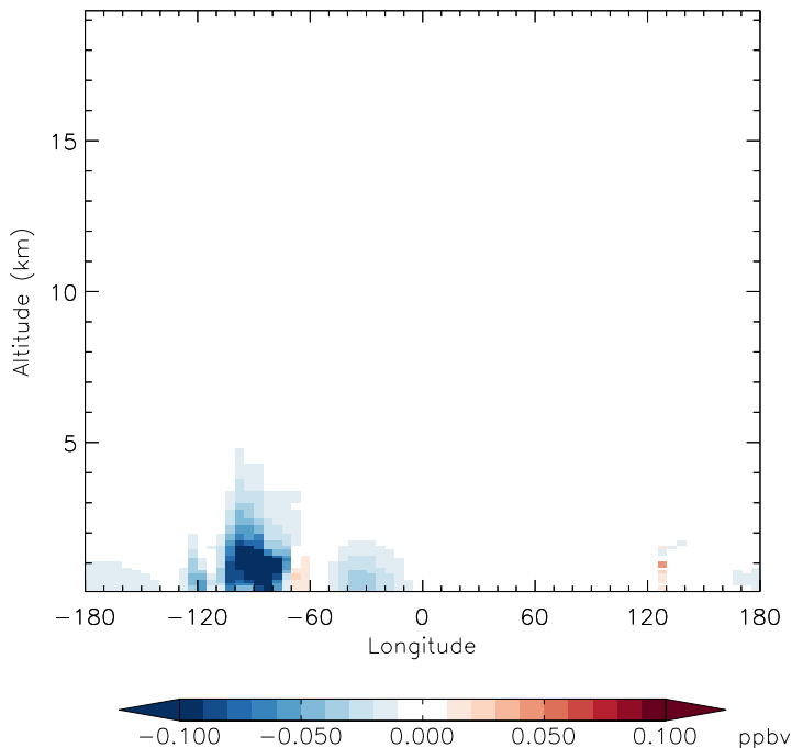
v11-01d-Run1 - v11-01b-Run0 HNO 3 - Diff along 42N for Oct
