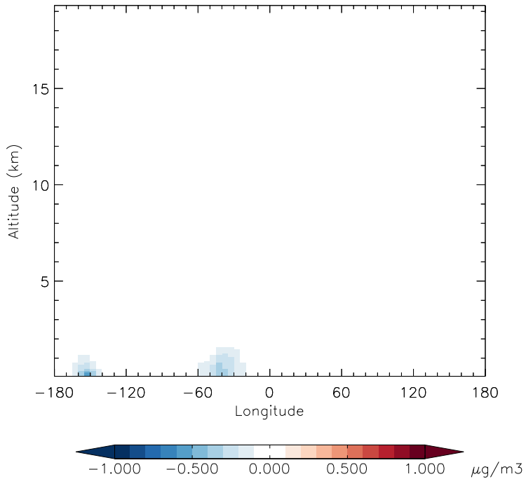
v11-01d-Run1 - v10-01-public-Run0 DMS - Diff along 42N for Oct
