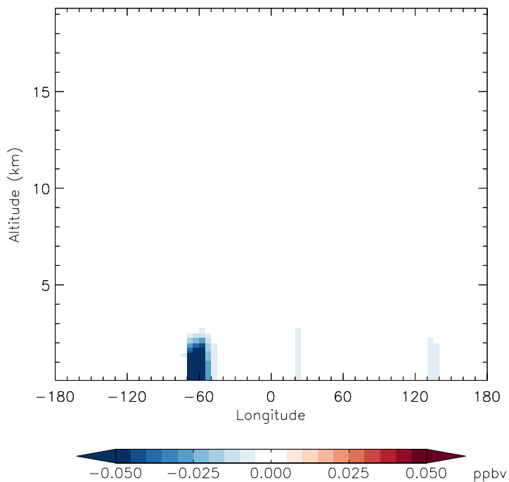
v11-01d-Run1 - v11-01b-Run0 MACR - Diff along 15S for Oct
