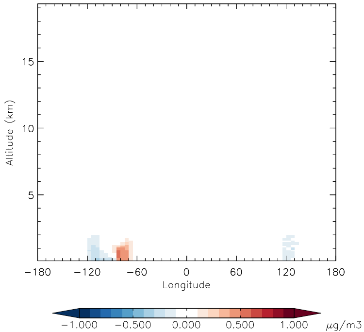
v11-01d-Run1 - v10-01-public-Run0 NIT - Diff along 42N for Oct
