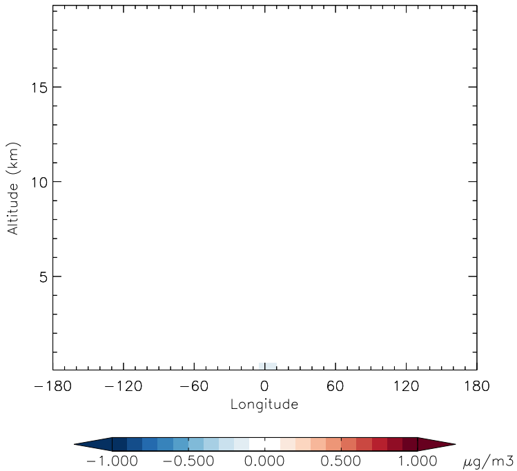
v11-01d-Run1 - v10-01-public-Run0 NIT - Diff along 15S for Oct
