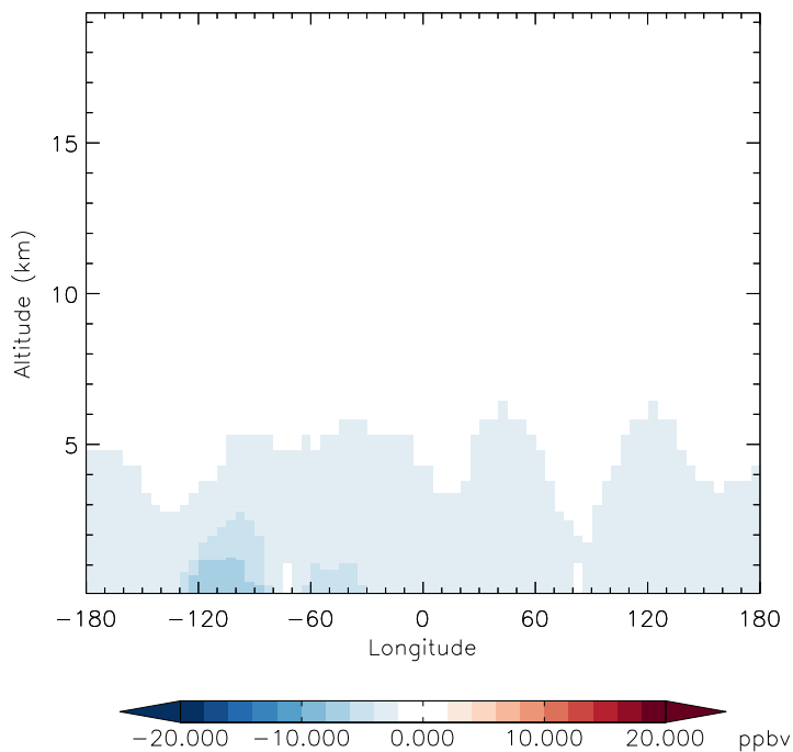
v11-01d-Run1 - v11-01b-Run0 CO - Diff along 42N for Oct
