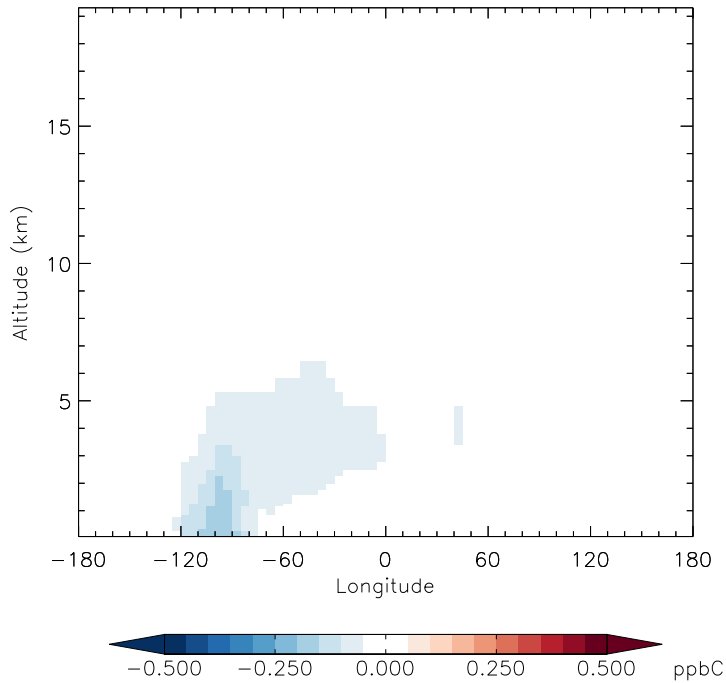
v11-01d-Run1 - v10-01-public-Run0 ACET - Diff along 42N for Oct
