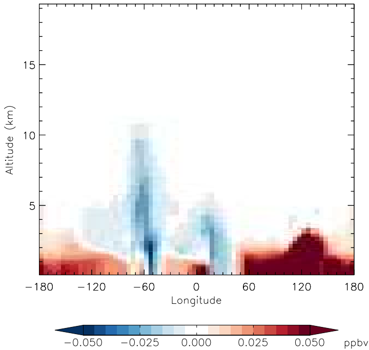
v11-01d-Run1 - v10-01-public-Run0 MP - Diff along 15S for Oct
