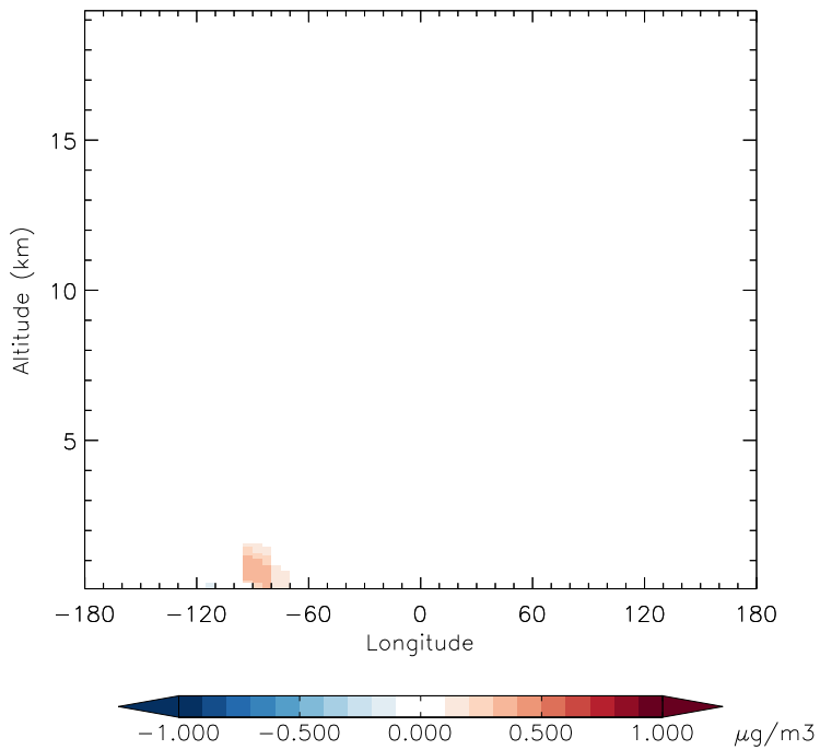
v11-01d-Run1 - v11-01b-Run0 NH3 - Diff along 42N for Oct
