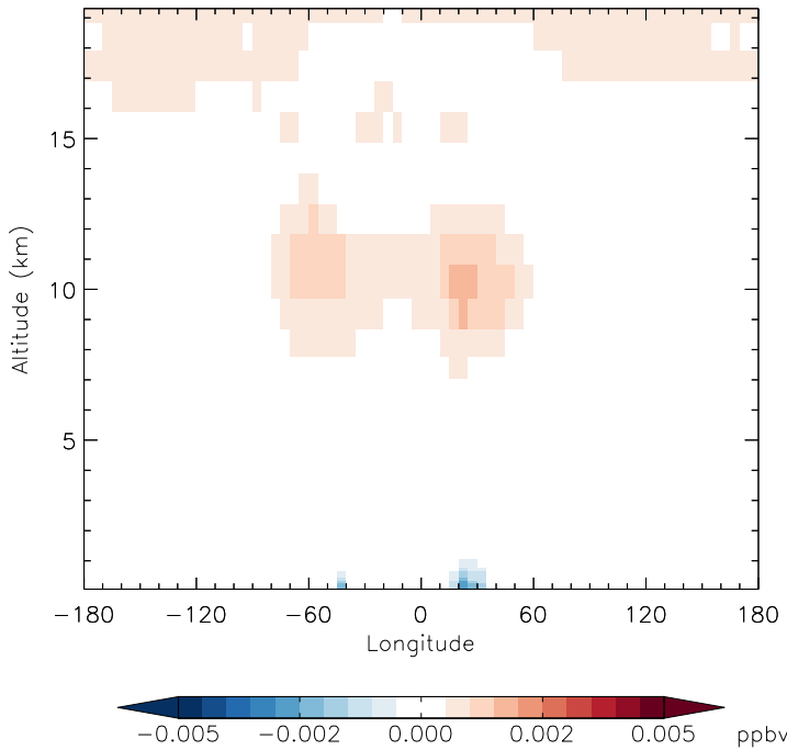
v11-01d-Run1 - v10-01-public-Run0 N2O5 - Diff along 15S for Oct
