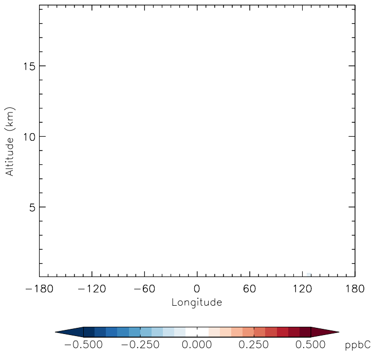
v11-01d-Run1 - v10-01-public-Run0 ALD2 - Diff along 15S for Oct
