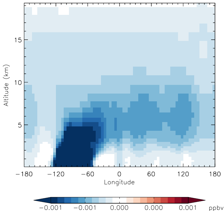
v11-01d-Run1 - v11-01b-Run0 PPN - Diff along 42N for Oct
