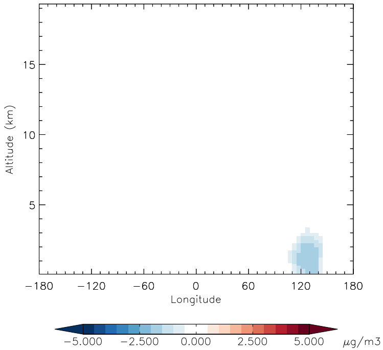
v11-01d-Run1 - v10-01-public-Run0 DST1 - Diff along 15S for Oct
