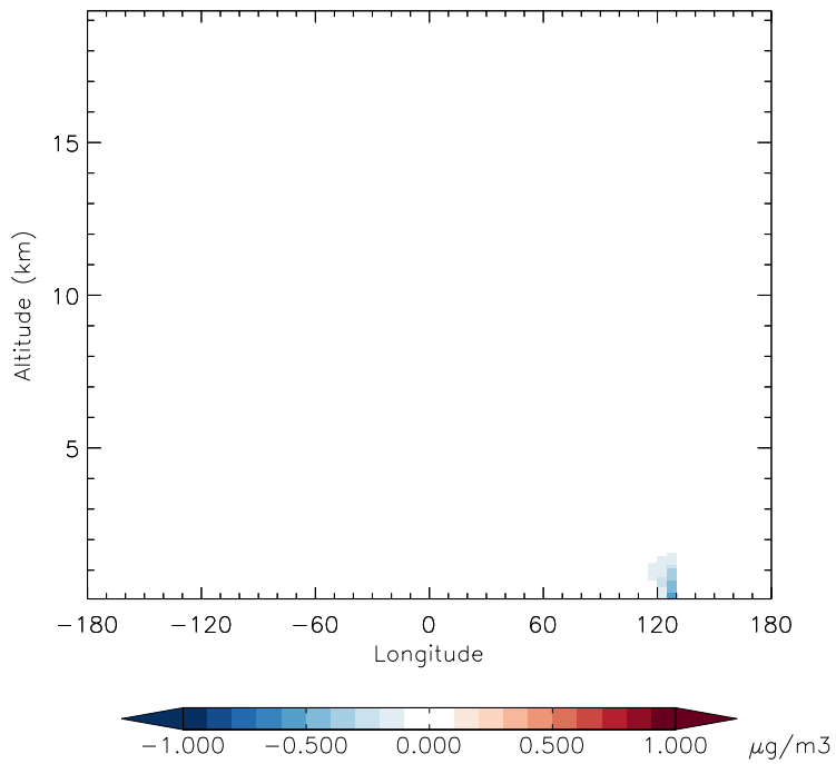
v11-01d-Run1 - v10-01-public-Run0 OCPI - Diff along 15S for Oct
