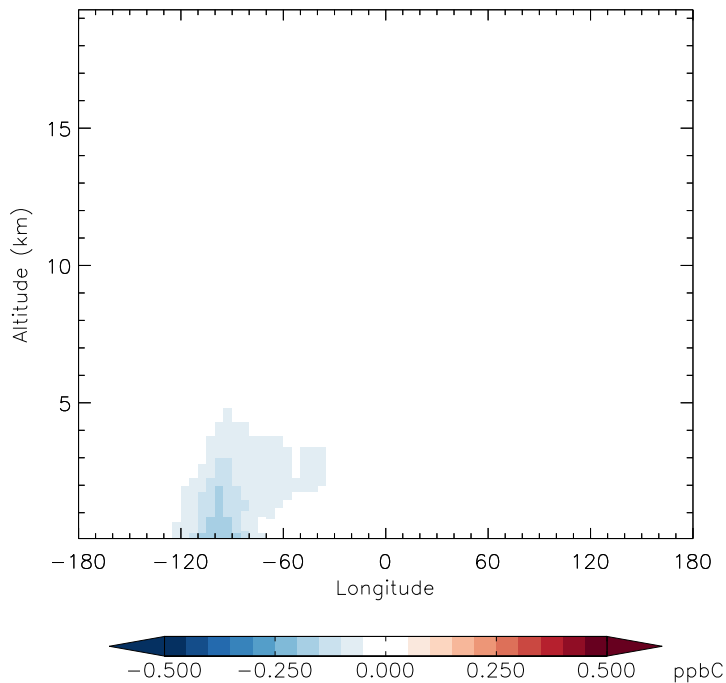
v11-01d-Run1 - v11-01b-Run0 ACET - Diff along 42N for Oct
