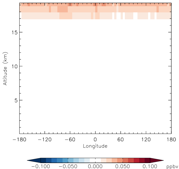
v11-01d-Run1 - v11-01b-Run0 H2O - Diff along 15S for Oct
