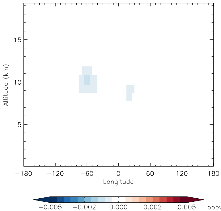
v11-01d-Run1 - v11-01b-Run0 HNO4 - Diff along 15S for Oct
