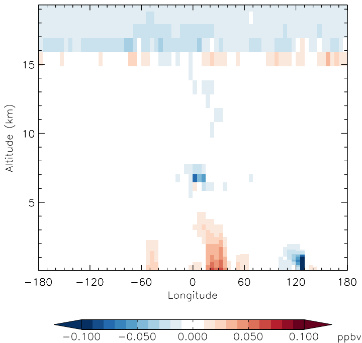
v11-01d-Run1 - v10-01-public-Run0 HNO 3 - Diff along 15S for Oct
