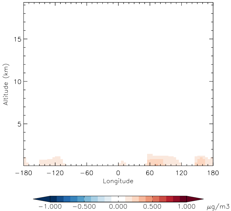
v11-01d-Run1 - v10-01-public-Run0 DMS - Diff along 15S for Oct
