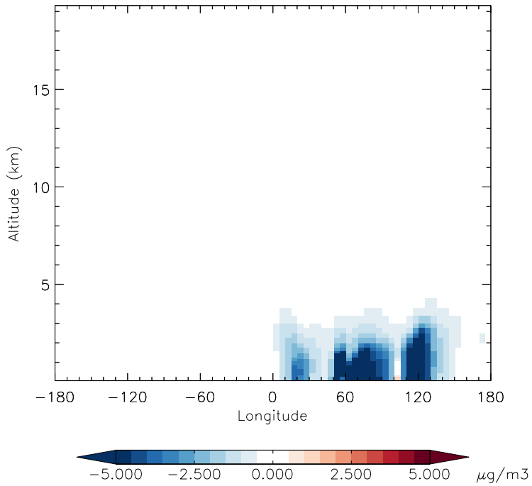
v11-01d-Run1 - v10-01-public-Run0 DST3 - Diff along 42N for Oct
