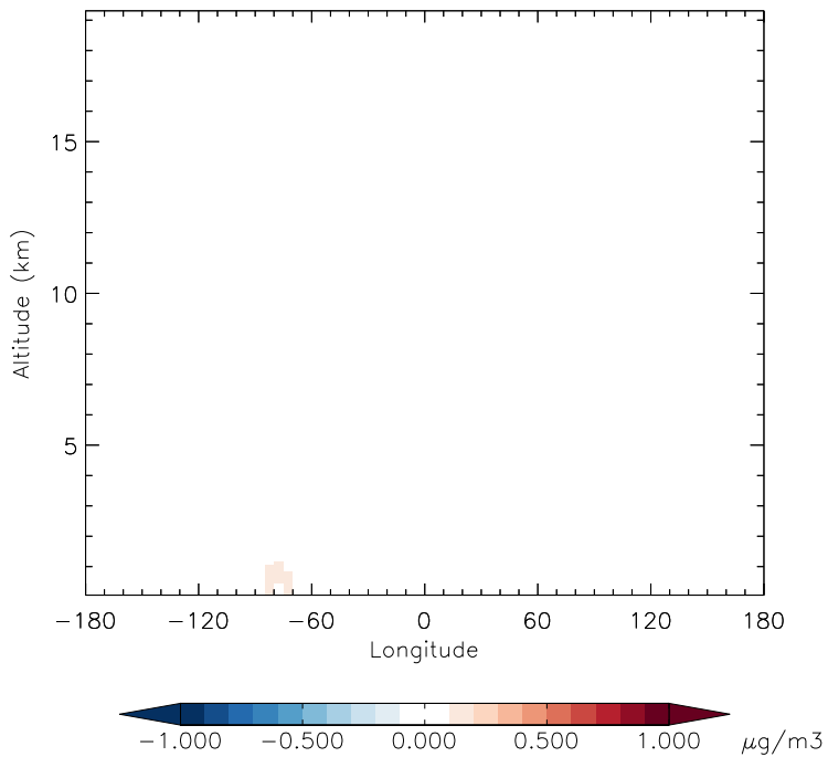
v11-01d-Run1 - v10-01-public-Run0 NH4 - Diff along 42N for Oct
