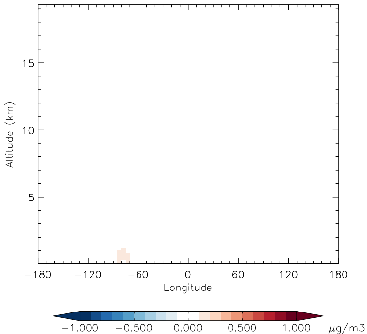
v11-01d-Run1 - v11-01b-Run0 NH4 - Diff along 42N for Oct
