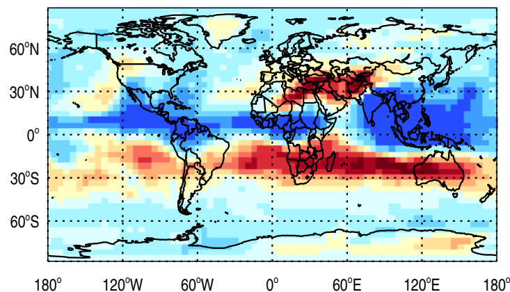
Tracer Map @ 500 hPa - Be7
