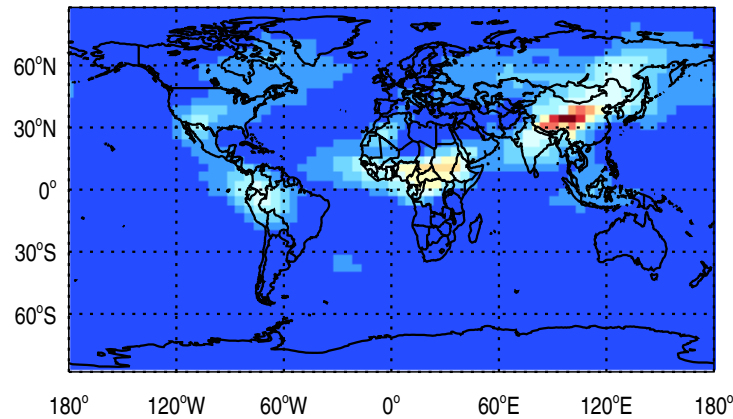
Tracer Map @ 500 hPa - Rn
