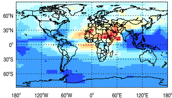
Tracer Map @ 500 hPa - Pb
