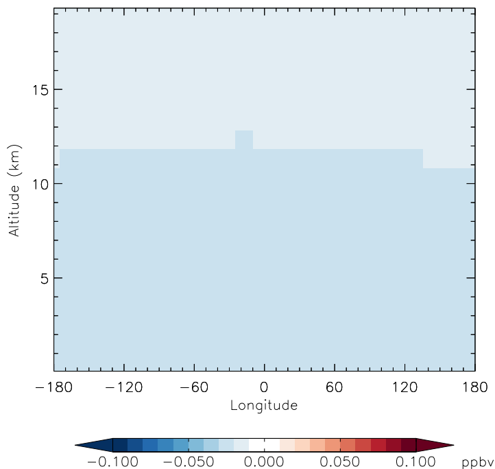
v11-01g-Run0 - v11-01f-geosfp-Run0 HCFC123 - Diff along 42N for Jan
