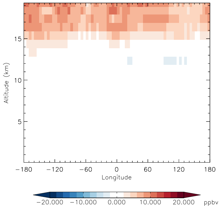
v11-01g-Run0 - v11-01d-Run1 O3 - Diff along 42N for Jan
