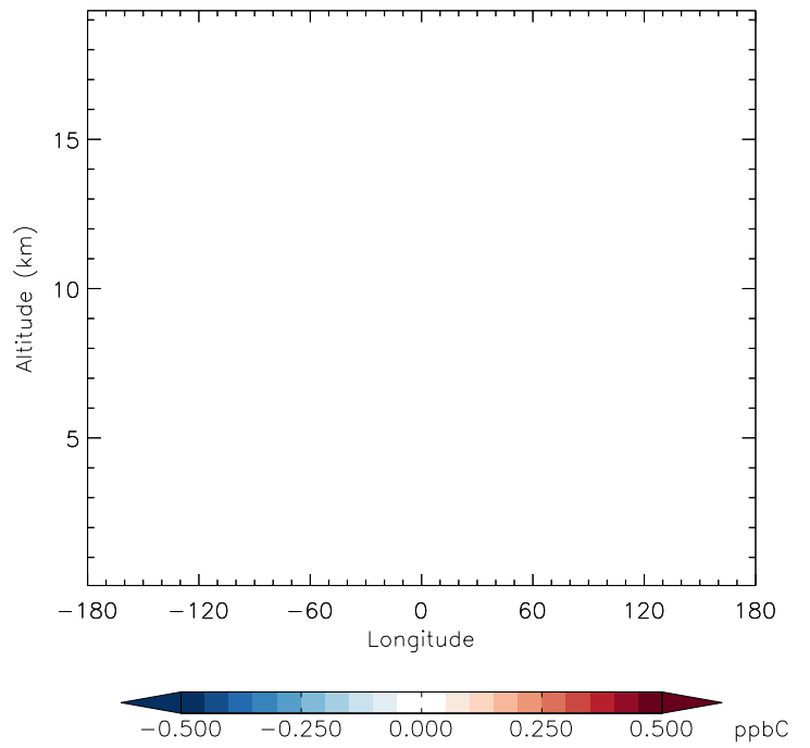
v11-01g-Run0 - v11-01f-geosfp-Run0 C3H8 - Diff along 42N for Jan
