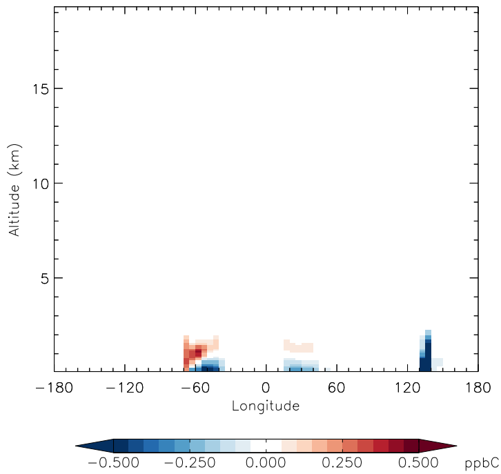
v11-01g-Run0 - v11-01d-Run1 ISOP - Diff along 15S for Jan
