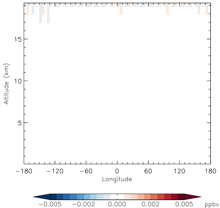
v11-01g-Run0 - v11-01d-Run1 N2O5 - Diff along 15S for Jan
