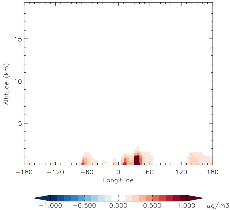
v11-01g-Run0 - v11-01d-Run1 S04 - Diff along 42N for Jan
