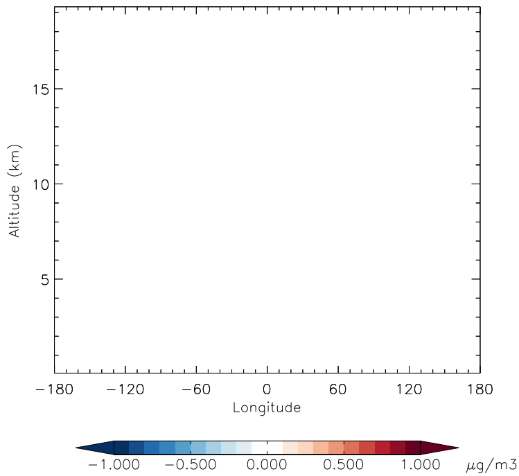
v11-01g-Run0 - v11-01d-Run1 SO4s - Diff along 42N for Jan
