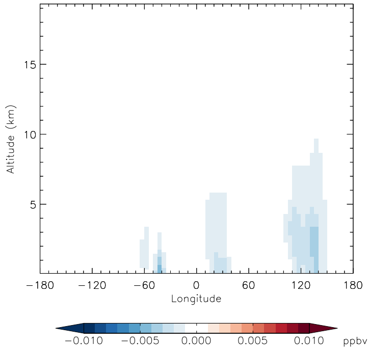
v11-01g-Run0 - v11-01d-Run1 R4N2 - Diff along 15S for Jan
