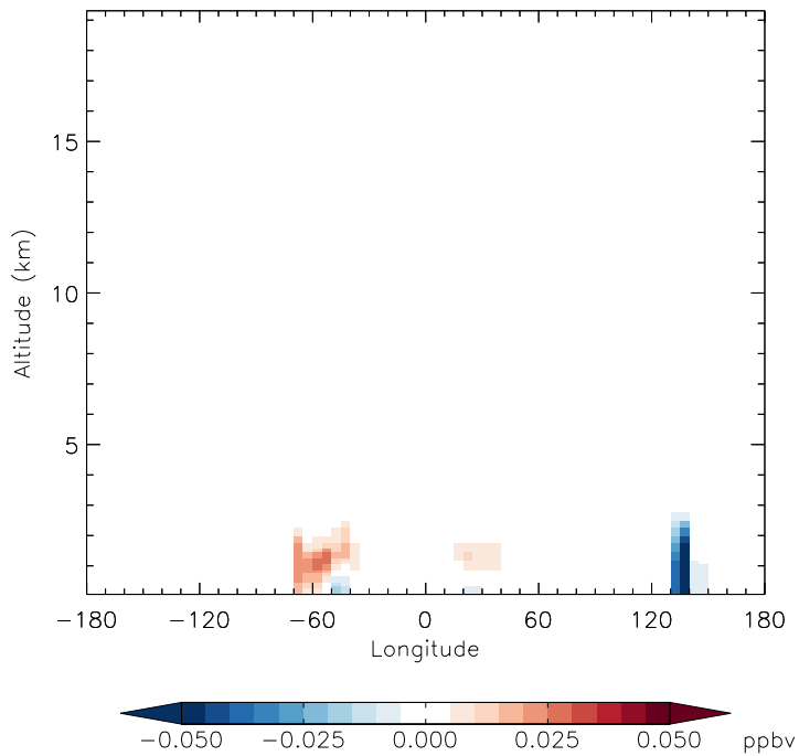
v11-01g-Run0 - v11-01d-Run1 MVK - Diff along 15S for Jan
