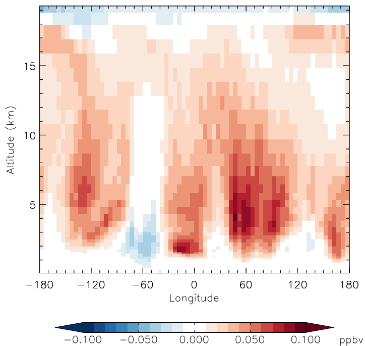
v11-01g-Run0 - v11-01f-geosp-Run0 CH4 - Diff along 15S for Jan
