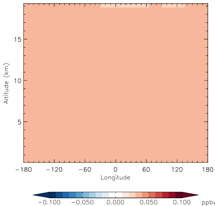
v11-01g-Run0 - v11-01f-geosfp-Run0 CFC113 - Diff along 15S for Jan
