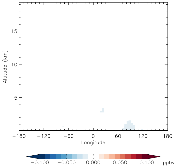
v11-01g-Run0 - v11-01d-Run1 H2O2 - Diff along 42N for Jan
