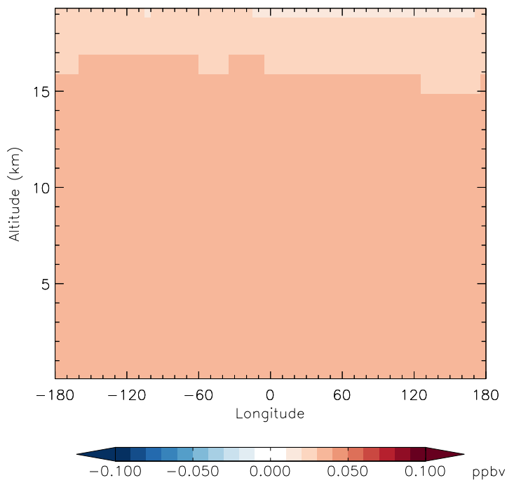
v11-01g-Run0 - v11-01f-geosfp-Run0 CFC113 - Diff along 42N for Jan
