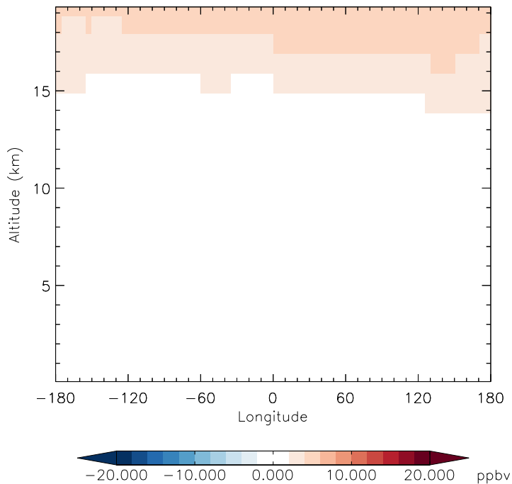
v11-01g-Run0 - v11-01f-geosfp-Run0 O3 - Diff along 42N for Jan
