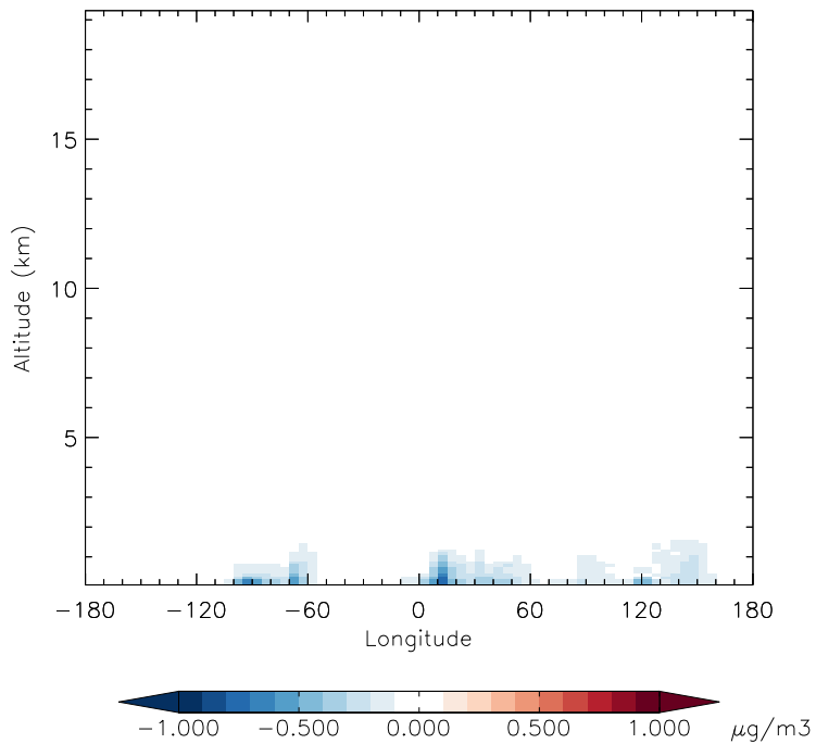
v11-01g-Run0 - v11-01d-Run1 NIT - Diff along 42N for Jan
