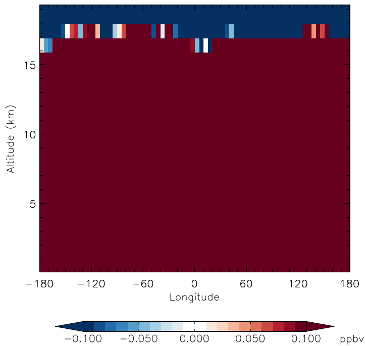
v11-01g-Run0 - v11-01d-Run1 CH4 - Diff along 42N for Jan
