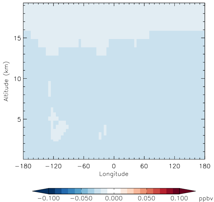
v11-01g-Run0 - v11-01d-Run1 HCFC123 - Diff along 15S for Jan
