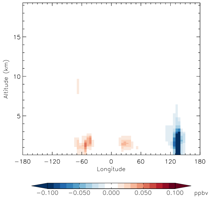
v11-01g-Run0 - v11-01d-Run1 HAC - Diff along 15S for Jan
