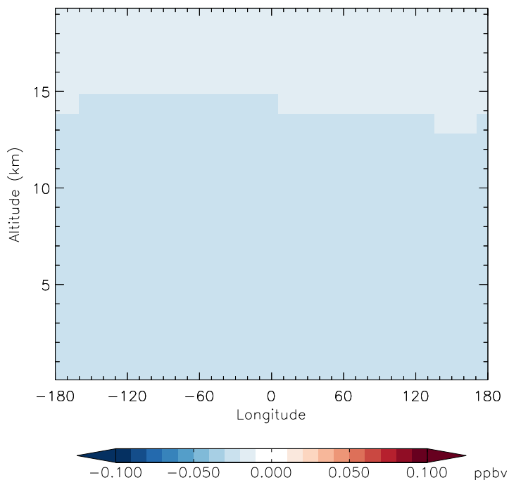
v11-01g-Run0 - v11-01f-geosfp-Run0 CFC115 - Diff along 42N for Jan
