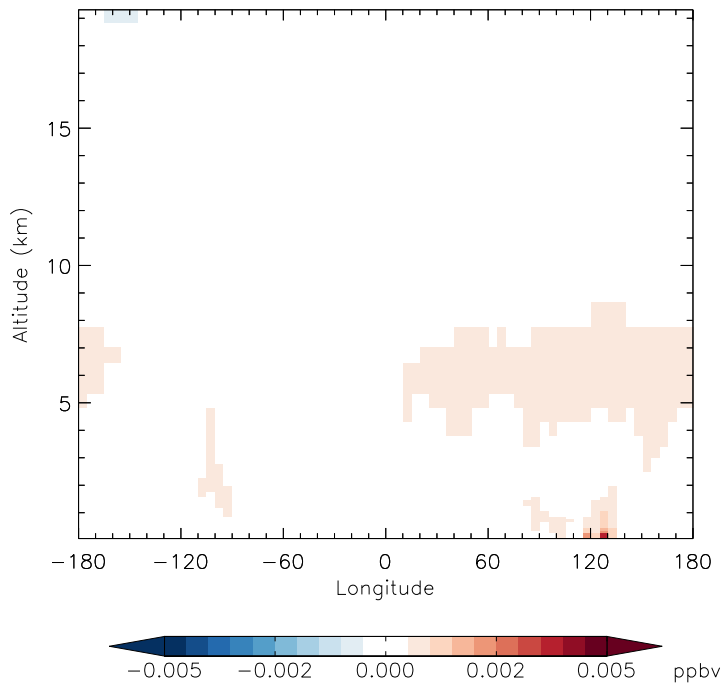
v11-01g-Run0 - v11-01d-Run1 HNO 4 - Diff along 42N for Jan
