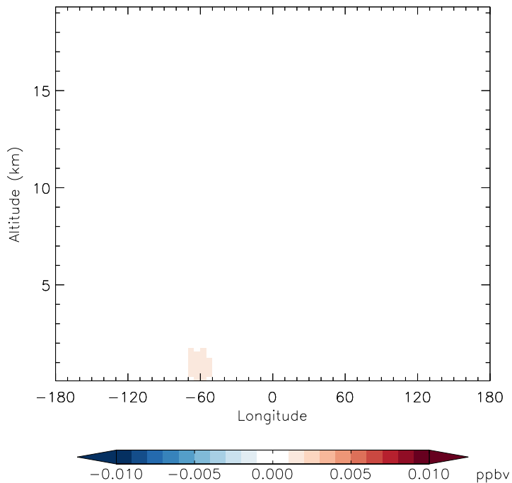
v11-01g-Run0 - v11-01f-geosfp-Run0 R4N2 - Diff along 15S for Jan
