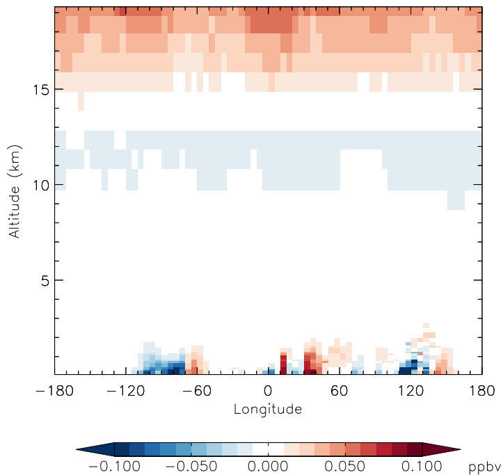
v11-01g-Run0 - v11-01d-Run1 HNO 3 - Diff along 42N for Jan
