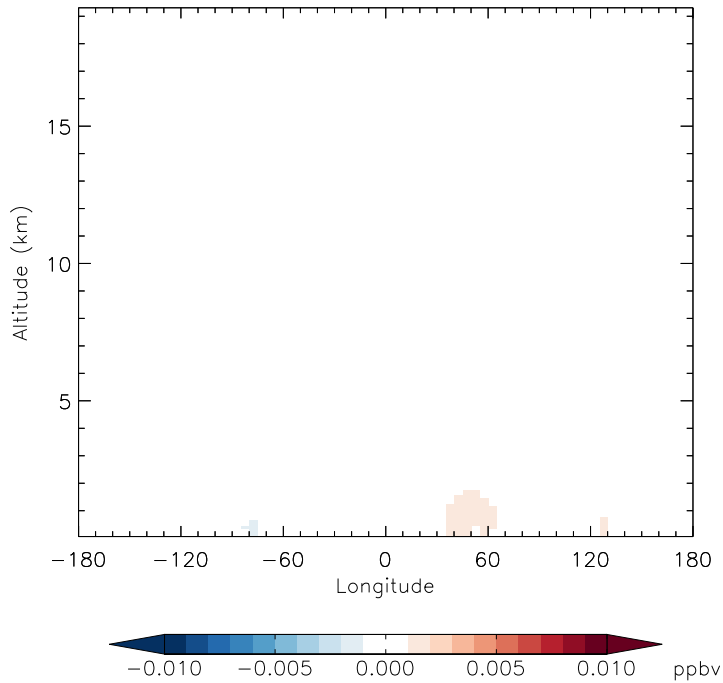
v11-01g-Run0 - v11-01d-Run1 R4N2 - Diff along 42N for Jan
