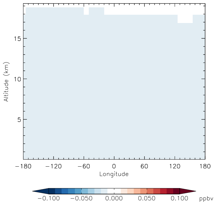
v11-01g-Run0 - v11-01f-geosfp-Run0 CFC114 - Diff along 42N for Jan
