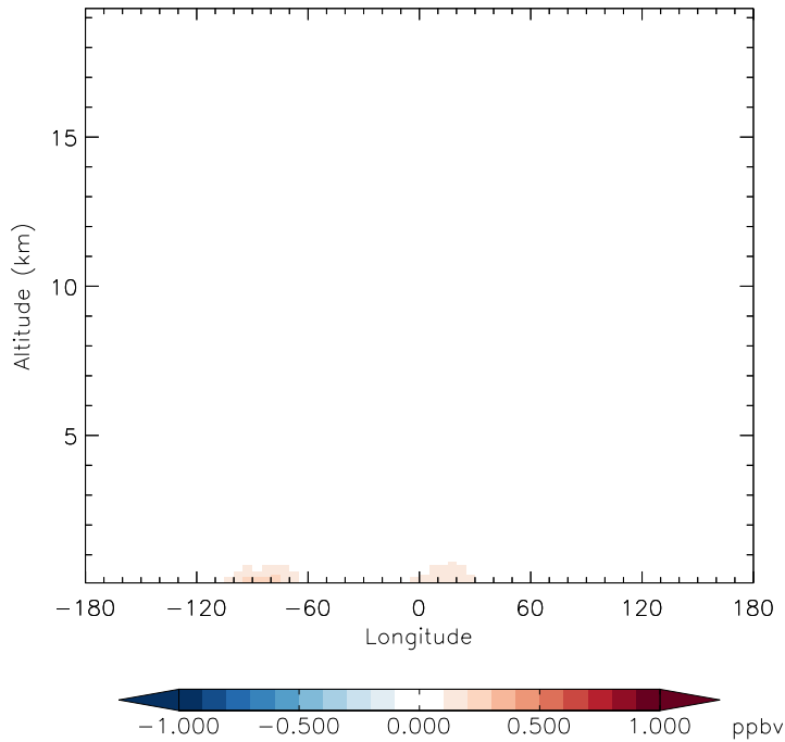
v11-01g-Run0 - v11-01d-Run1 NO2 - Diff along 42N for Jan
