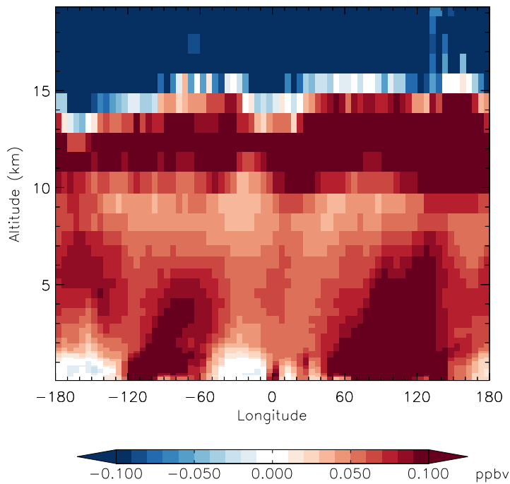
v11-01g-Run0 - v11-01d-Run1 N2O - Diff along 42N for Jan
