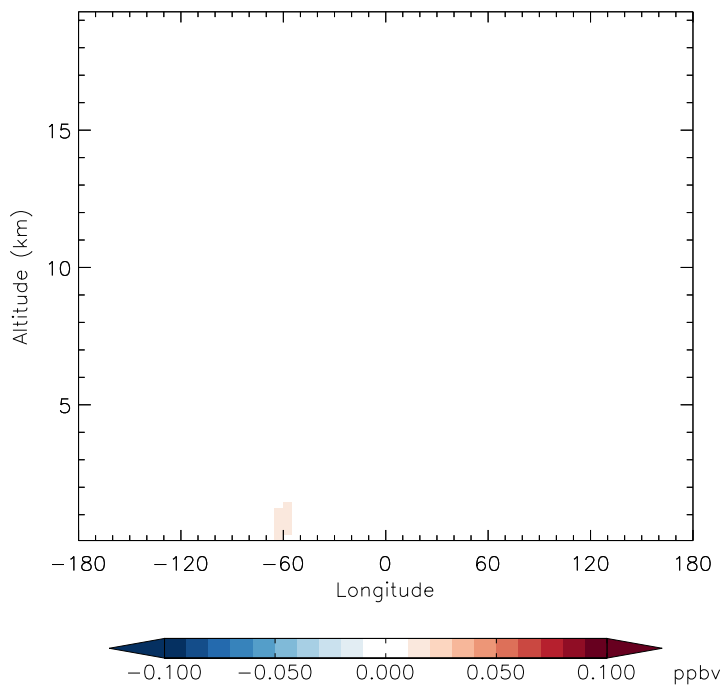
v11-01g-Run0 - v11-01f-geosfp-Run0 H2O2 - Diff along 15S for Jan
