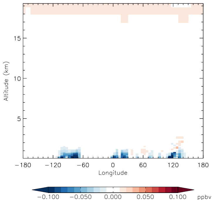
v11-01g-Run0 - v11-01f-geosfp-Run0 HNO 3 - Diff along 42N for Jan
