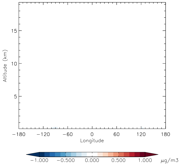
v11-01g-Run0 - v11-01f-geosfp-Run0 NH4 - Diff along 42N for Jan
