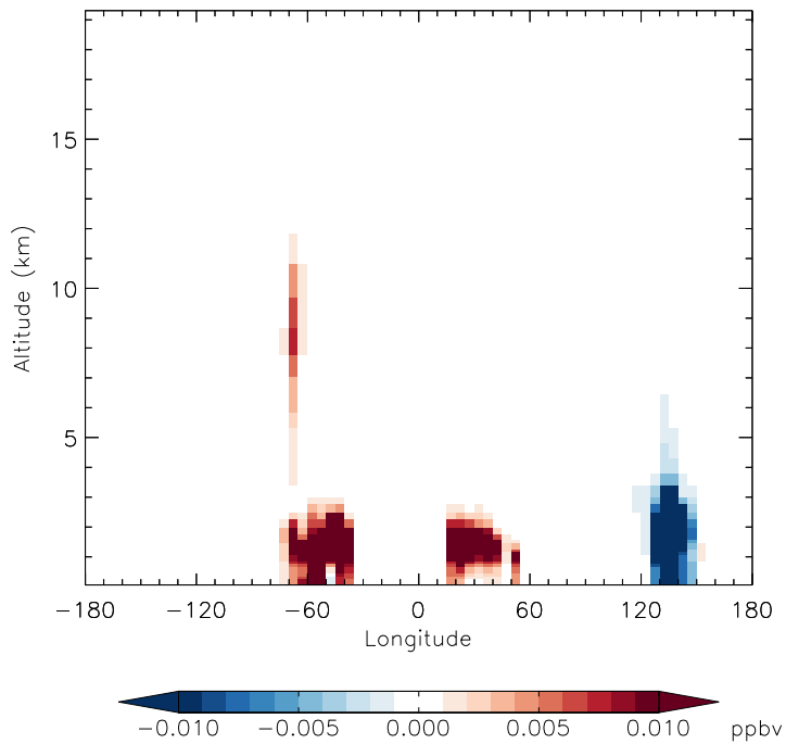
v11-01g-Run0 - v11-01d-Run1 IEPOX - Diff along 15S for Jan
