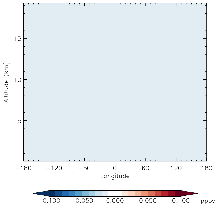
v11-01g-Run0 - v11-01d-Run1 CFC114 - Diff along 15S for Jan
