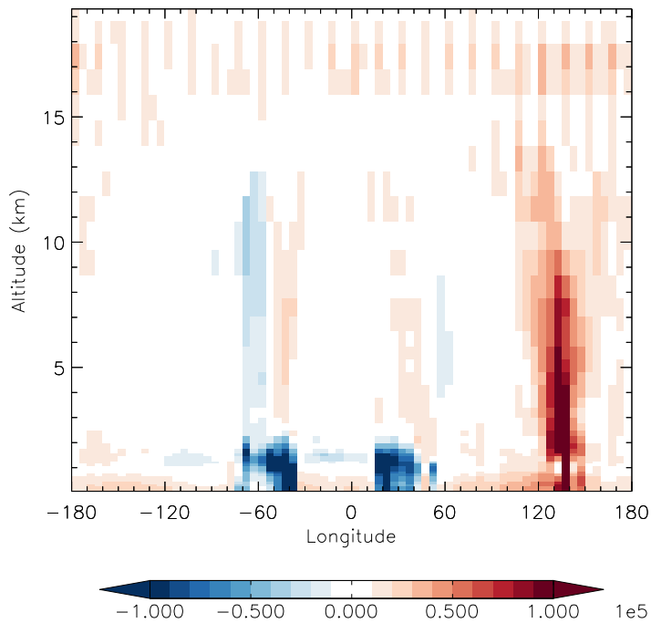
v11-01g-Run0 - v11-01d-Run1 OH - Diff along 15S for Jan
