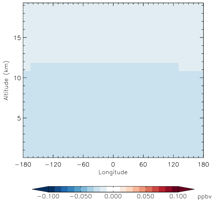
v11-01g-Run0 - v11-01d-Run1 HCFC123 - Diff along 42N for Jan
