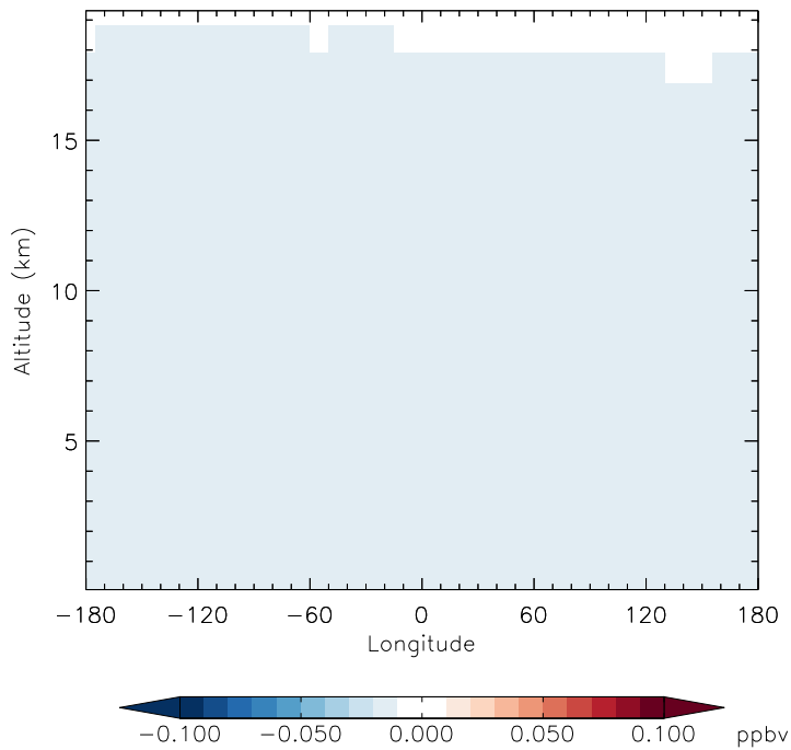
v11-01g-Run0 - v11-01d-Run1 CFC114 - Diff along 42N for Jan
