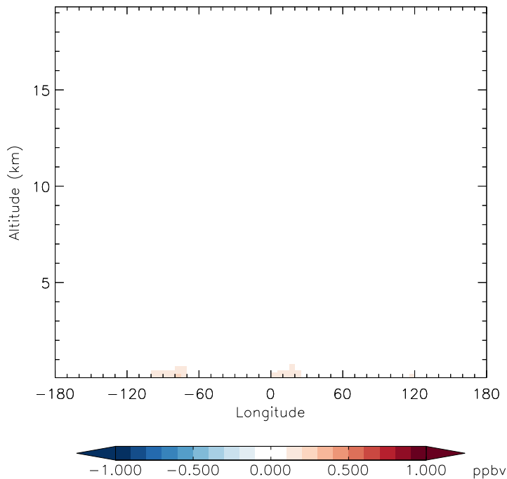
v11-01g-Run0 - v11-01f-geosfp-Run0 NO2 - Diff along 42N for Jan
