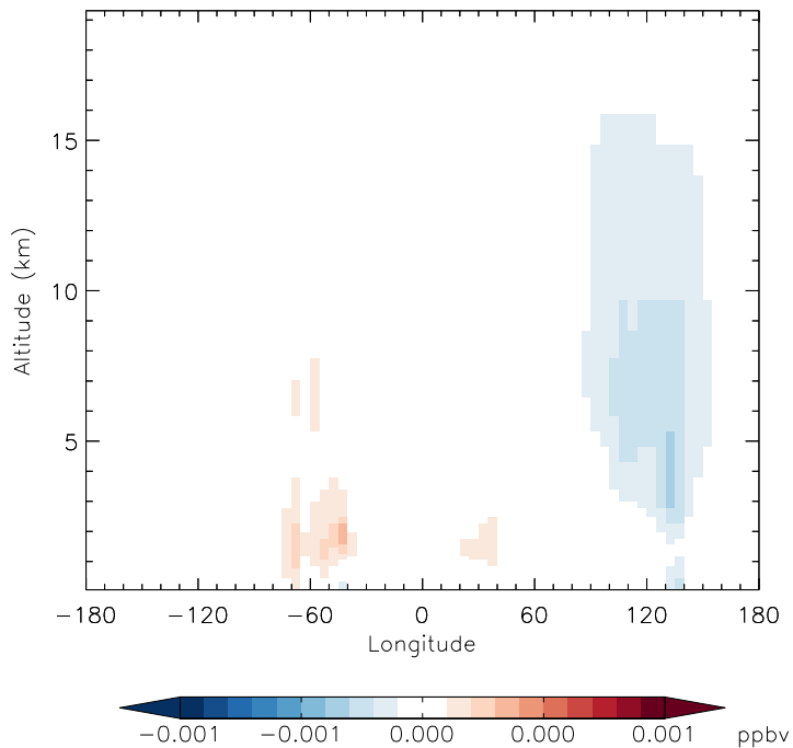
v11-01g-Run0 - v11-01d-Run1 PPN - Diff along 15S for Jan
