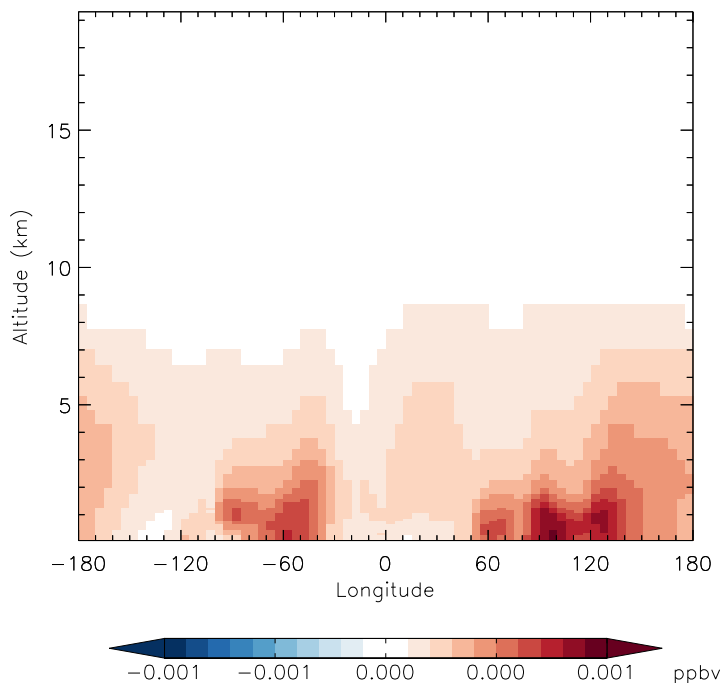
v11-01g-Run0 - v11-01f-geosfp-Run0 PPN - Diff along 42N for Jan
