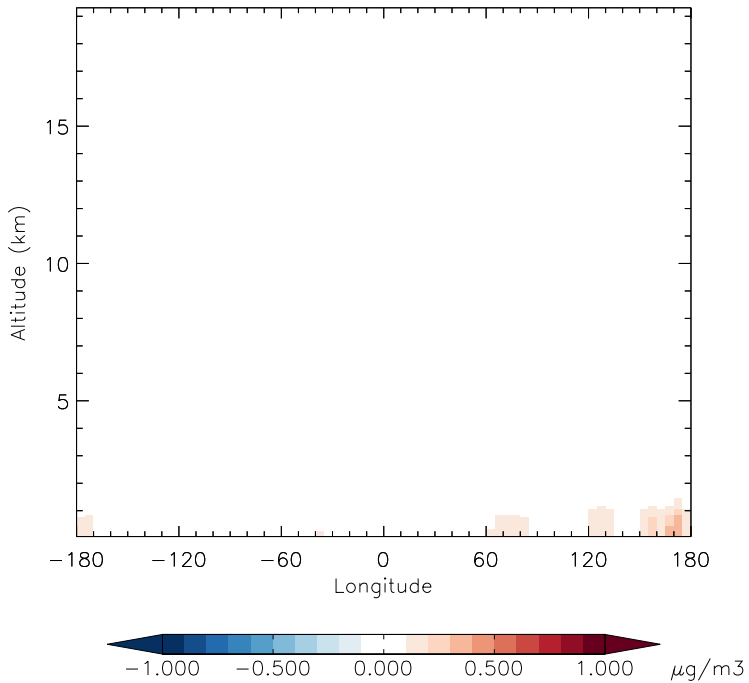
v11-01g-Run0 - v11-01d-Run1 S04 - Diff along 15S for Jan
