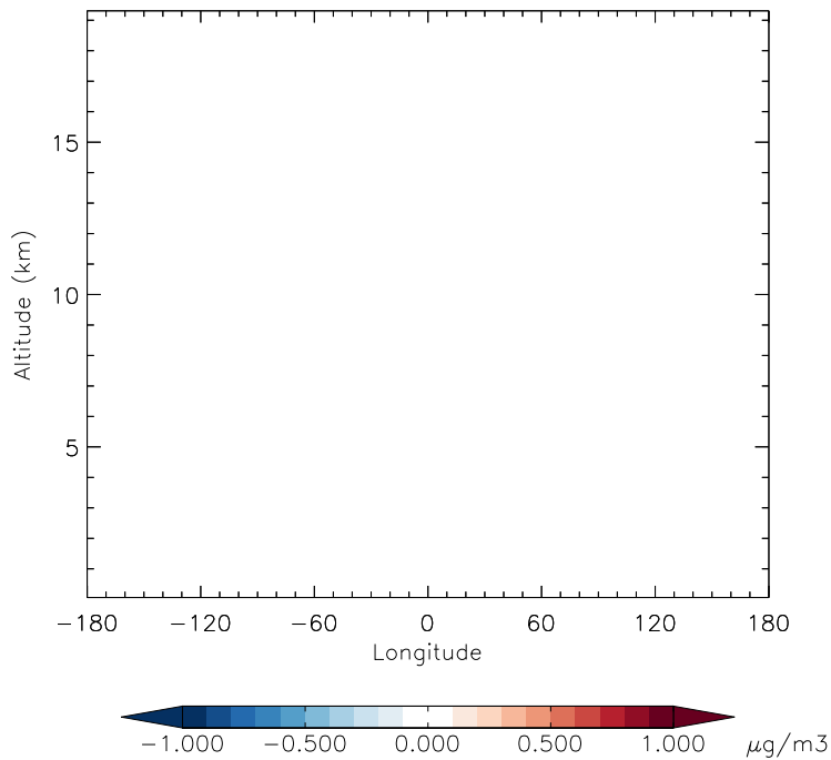
v11-01g-Run0 - v11-01d-Run1 OCPO - Diff along 42N for Jan
