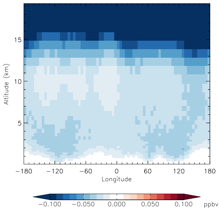
v11-01g-Run0 - v11-01f-geosp-Run0 CH4 - Diff along 42N for Jan
