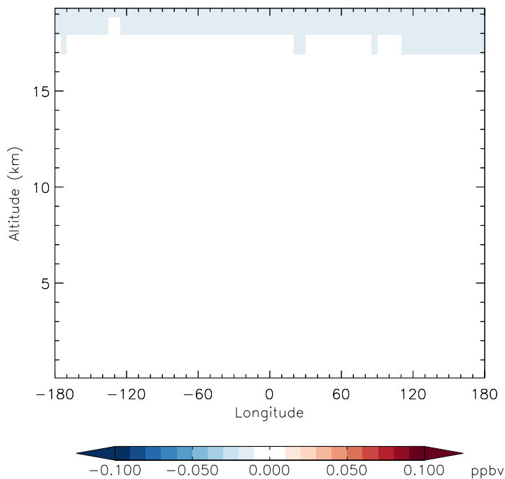
v11-01g-Run0 - v11-01f-geosfp-Run0 N2O - Diff along 42N for Jan
