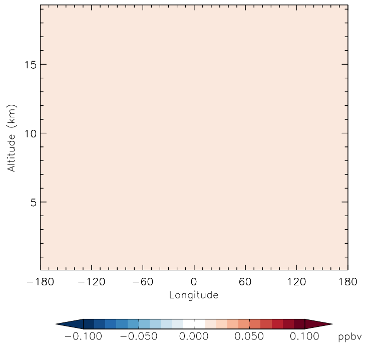
v11-01g-Run0 - v11-01f-geosfp-Run0 HCFC141b - Diff along 42N for Jan
