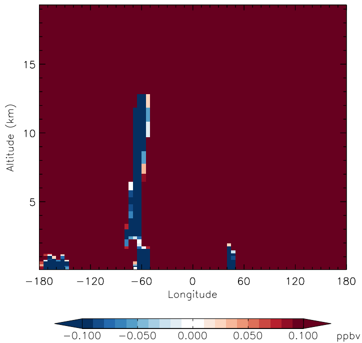
v11-01g-Run0 - v11-01d-Run1 CH4 - Diff along 15S for Jan
