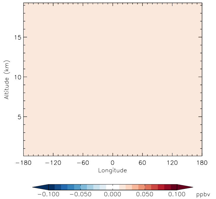
v11-01g-Run0 - v11-01d-Run1 HCFC141b - Diff along 42N for Jan
