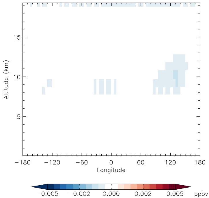
v11-01g-Run0 - v11-01d-Run1 HNO 4 - Diff along 15S for Jan
