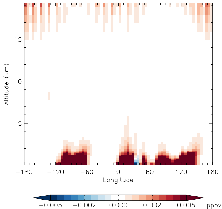
v11-01g-Run0 - v11-01d-Run1 N2O5 - Diff along 42N for Jan
