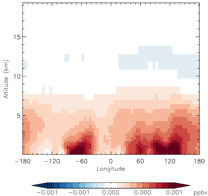
v11-01g-Run0 - v11-01d-Run1 PPN - Diff along 42N for Jan
