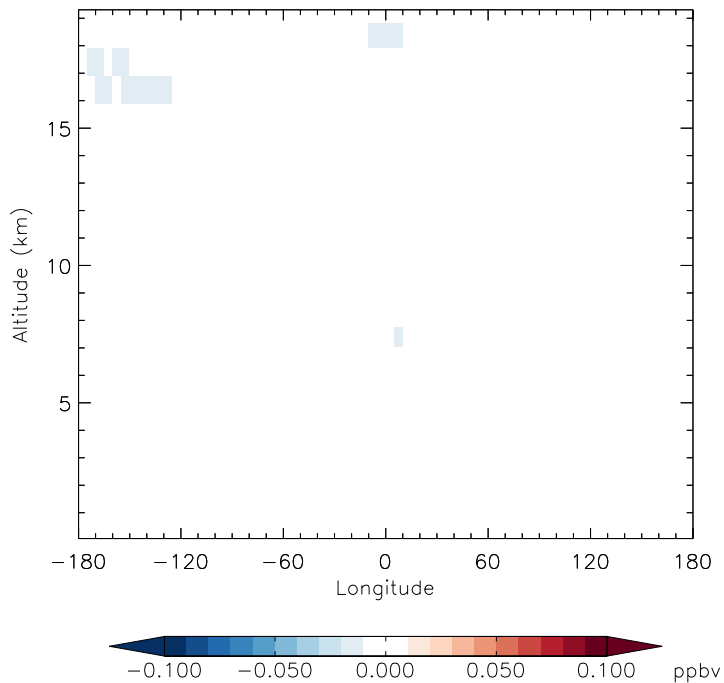
v11-01g-Run0 - v11-01d-Run1 HNO 3 - Diff along 15S for Jan
