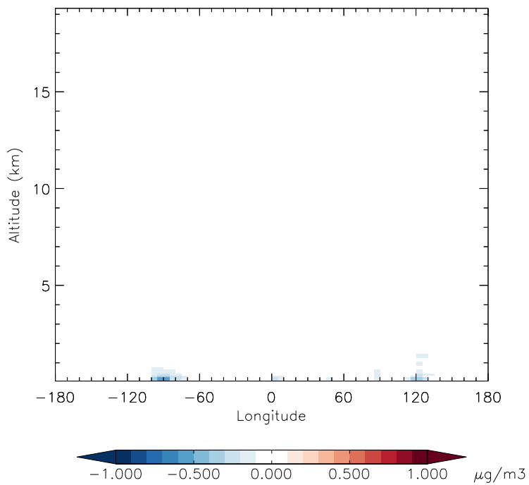
v11-01g-Run0 - v11-01f-geosfp-Run0 NIT - Diff along 42N for Jan
