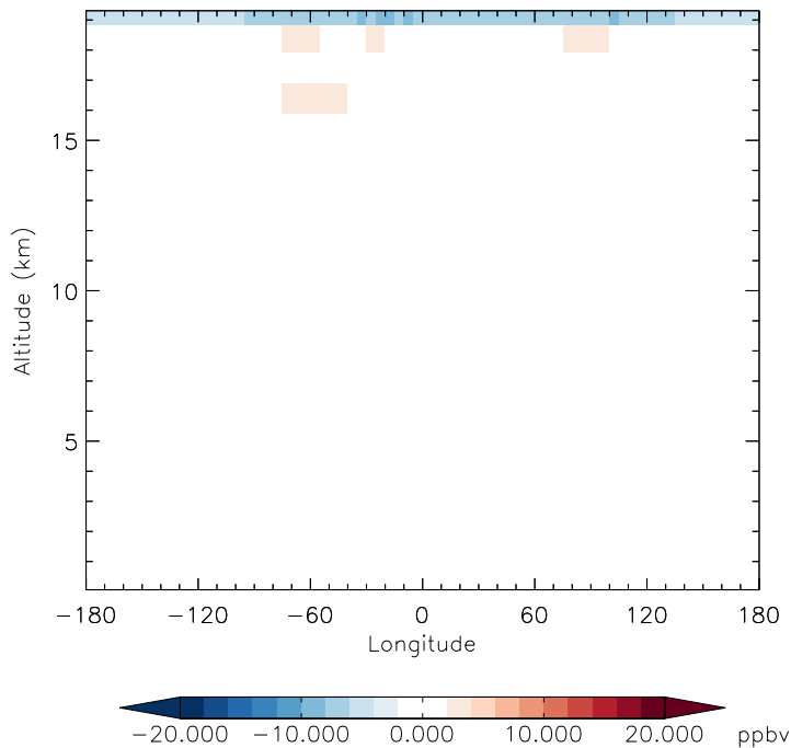
v11-01g-Run0 - v11-01d-Run1 O3 - Diff along 15S for Jan
