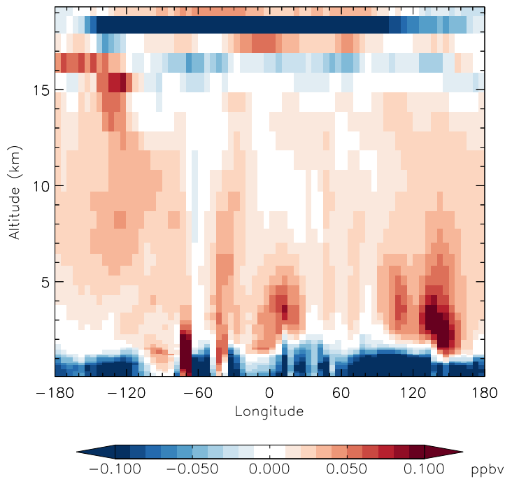
v11-01g-Run0 - v11-01d-Run1 N2O - Diff along 15S for Jan
