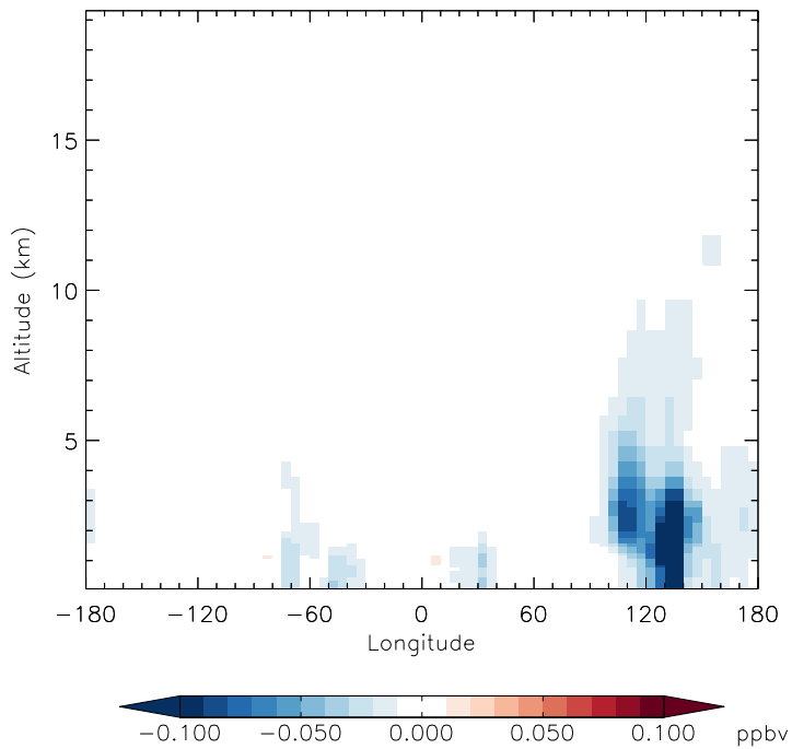
v11-01g-Run0 - v11-01d-Run1 H2O2 - Diff along 15S for Jan
