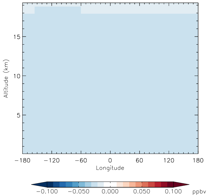
v11-01g-Run0 - v11-01d-Run1 CFC115 - Diff along 15S for Jan
