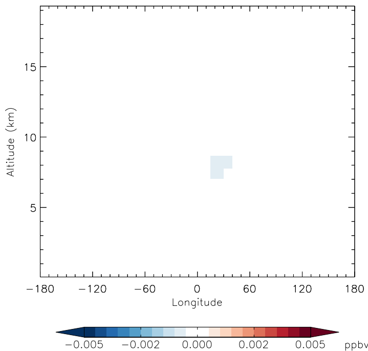
v11-01g-Run0 - v11-01f-geosfp-Run0 HNO 4 - Diff along 15S for Jan
