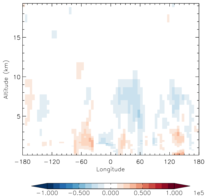
v11-01g-Run0 - v11-01f-geosp-Run0 OH - Diff along 15S for Jan
