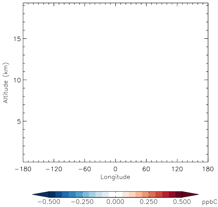
v11-01g-Run0 - v11-01f-geosfp-Run0 C3H8 - Diff along 15S for Jan
