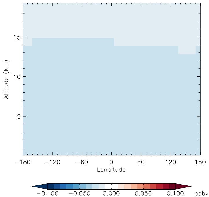
v11-01g-Run0 - v11-01d-Run1 CFC115 - Diff along 42N for Jan
