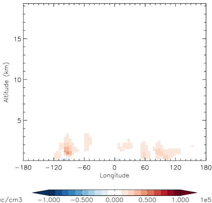
v11-01g-Run0 - v11-01f-geosp-Run0 OH - Diff along 42N for Jan
