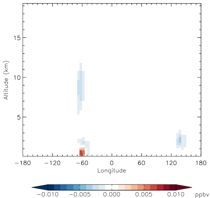
v11-01g-Run0 - v11-01f-geosfp-Run0 IEPOX - Diff along 15S for Jan
