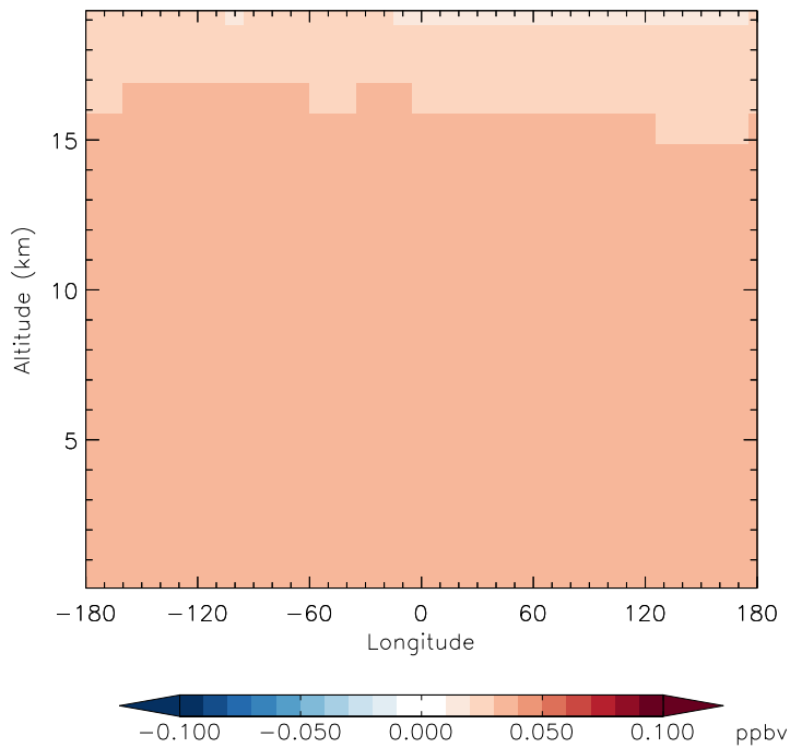
v11-01g-Run0 - v11-01d-Run1 CFC113 - Diff along 42N for Jan
