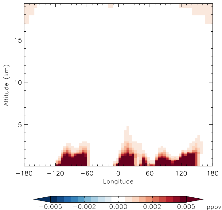
v11-01g-Run0 - v11-01f-geosfp-Run0 N2O5 - Diff along 42N for Jan
