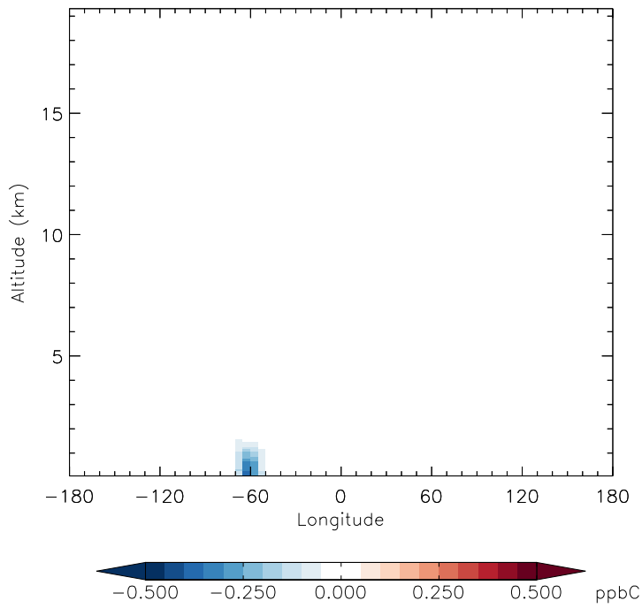
v11-01g-Run0 - v11-01f-geosfp-Run0 ISOP - Diff along 15S for Jan
