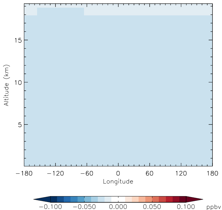
v11-01g-Run0 - v11-01f-geosfp-Run0 CFC115 - Diff along 15S for Jan
