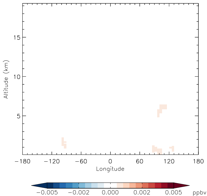
v11-01g-Run0 - v11-01f-geosfp-Run0 HNO 4 - Diff along 42N for Jan
