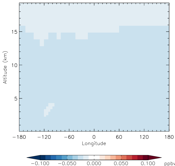
v11-01g-Run0 - v11-01f-geosfp-Run0 HCFC123 - Diff along 15S for Jan
