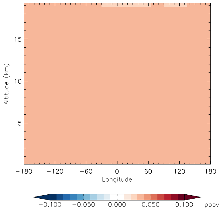
v11-01g-Run0 - v11-01d-Run1 CFC113 - Diff along 15S for Jan
