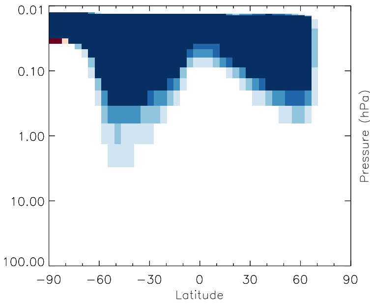
v11-01g-Run0 - v11-01f-geosfp-Run0 N2O5 - Strat zonal mean abs diff for Jul
