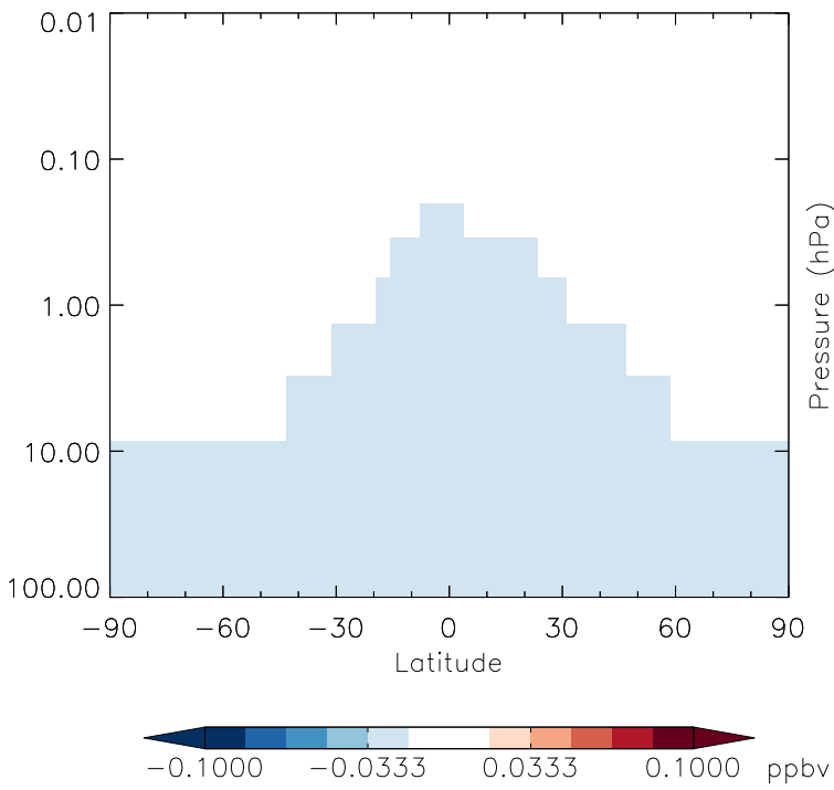
v11-01g-Run0 - v11-01f-geosfp-Run0 CFC115 - Strat zonal mean abs diff for Jul
