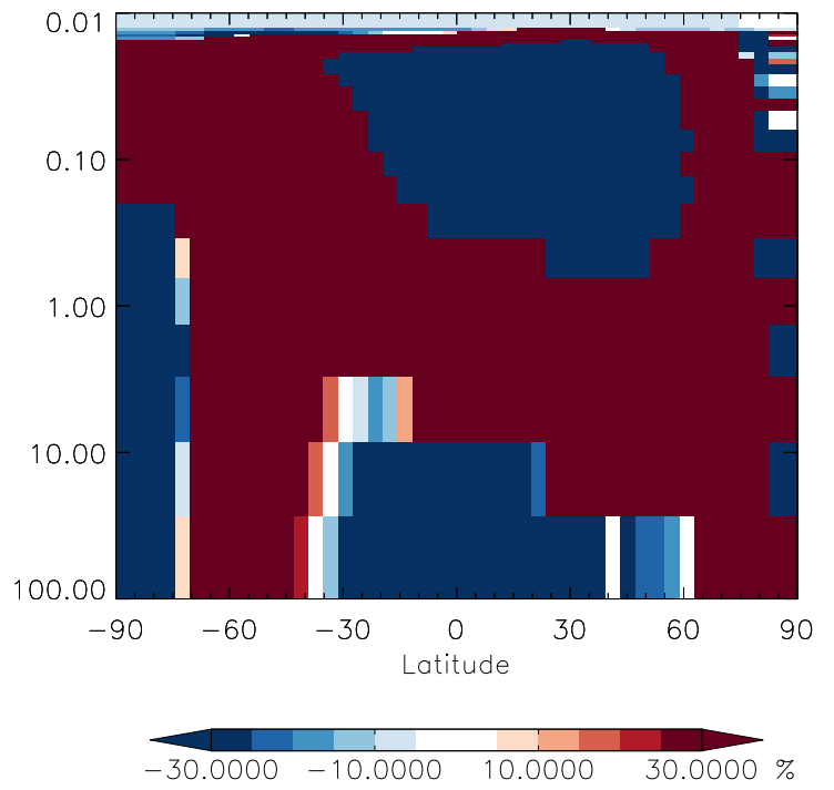
v11-01g-Run0 / v11-01f-geosfp-Run0 ISOPND - Strat zonal mean % diff for Jul
