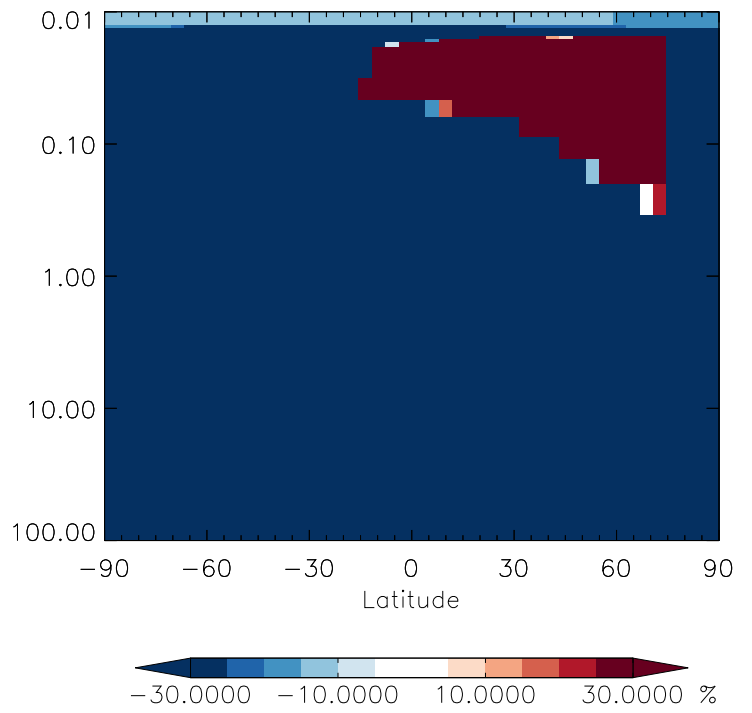
v11-01g-Run0 / v11-01f-geosfp-Run0 MACRN - Strat zonal mean % diff for Jul
