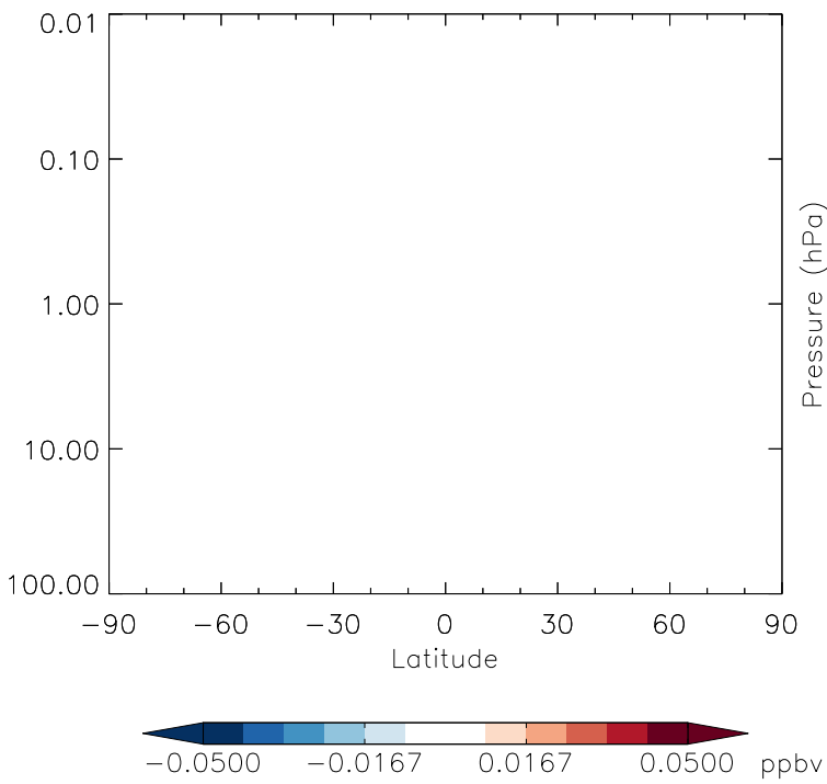
v11-01g-Run0 - v11-01d-Run1 RCHO - Strat zonal mean abs diff for Jul
