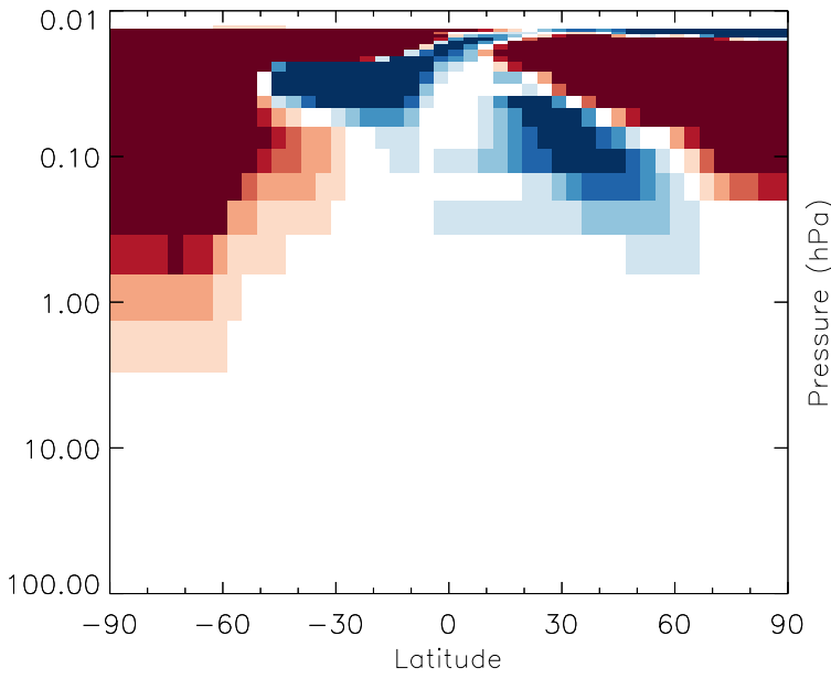
v11-01g-Run0 - v11-01f-geosfp-Run0 O3 - Strat zonal mean abs diff for Jul
