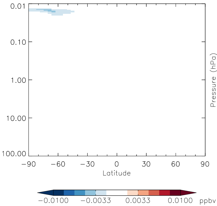
v11-01g-Run0 - v11-01d-Run1 BrNO3 - Strat zonal mean abs diff for Jul
