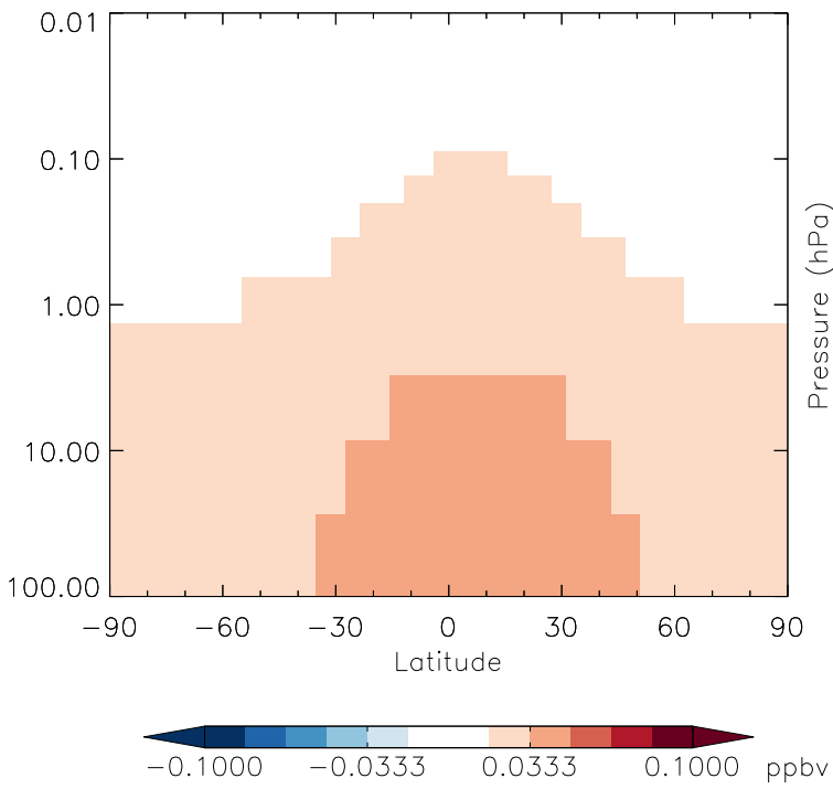
v11-01g-Run0 - v11-01f-geosfp-Run0 CFC113 - Strat zonal mean abs diff for Jul
