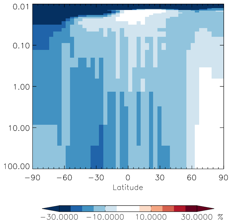
v11-01g-Run0 / v11-01d-Run1 BrNO2 - Strat zonal mean % diff for Jul
