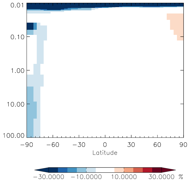
v11-01g-Run0 / v11-01f-geosfp-Run0 ClNO 3 - Strat zonal mean % diff for Jul
