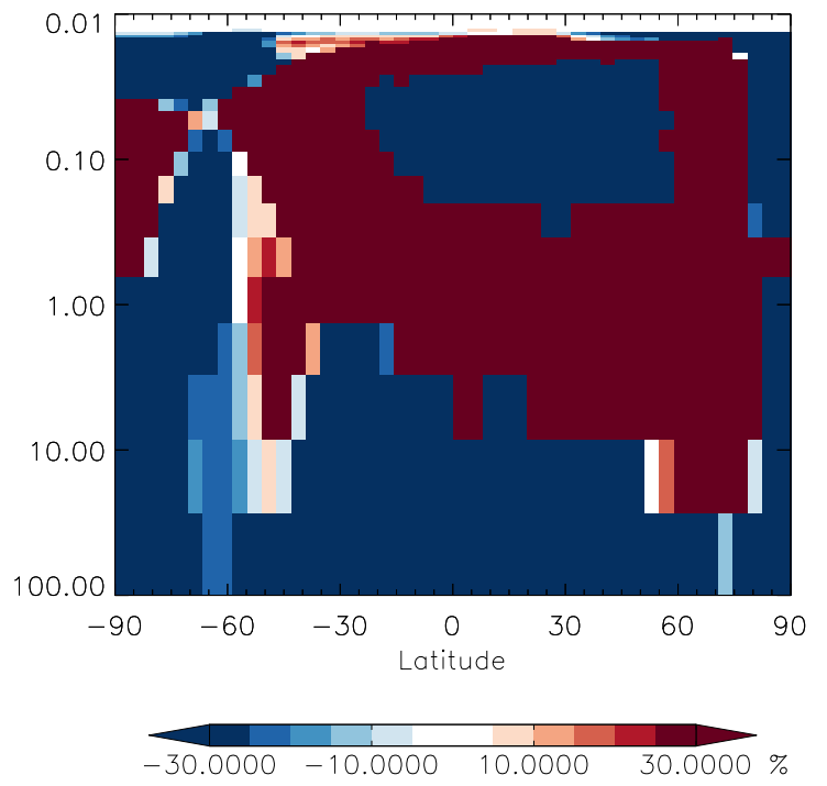
v11-01g-Run0 / v11-01d-Run1 MOBA - Strat zonal mean % diff for Jul
