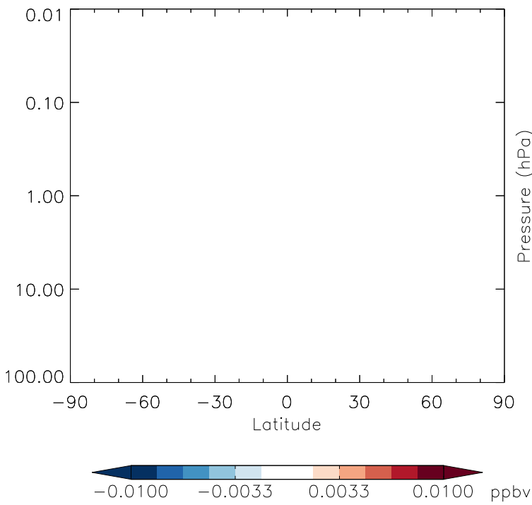
v11-01g-Run0 - v11-01d-Run1 R4N2 - Strat zonal mean abs diff for Jul
