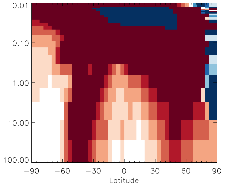
v11-01g-Run0 / v11-01d-Run1 PRPE - Strat zonal mean % diff for Jul
