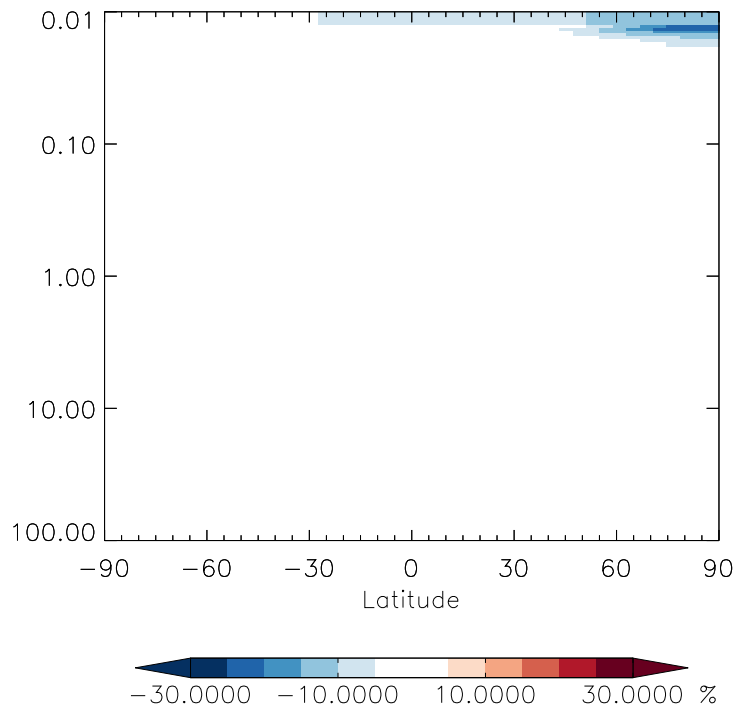
v11-01g-Run0 / v11-01f-geosfp-Run0 CH3Cl - Strat zonal mean % diff for Jul
