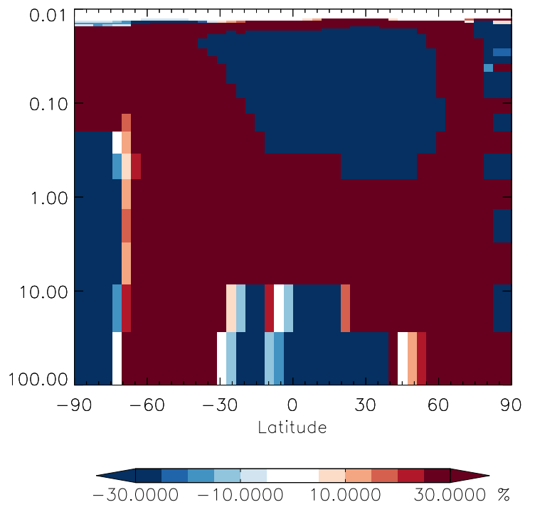
v11-01g-Run0 / v11-01d-Run1 ISOPND - Strat zonal mean % diff for Jul
