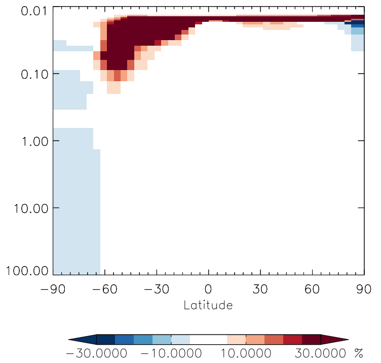
v11-01g-Run0 / v11-01d-Run1 R4N2 - Strat zonal mean % diff for Jul
