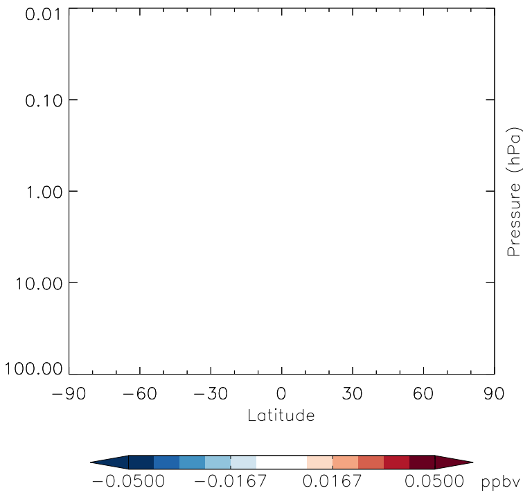
v11-01g-Run0 - v11-01f-geosfp-Run0 RCHO - Strat zonal mean abs diff for Jul
