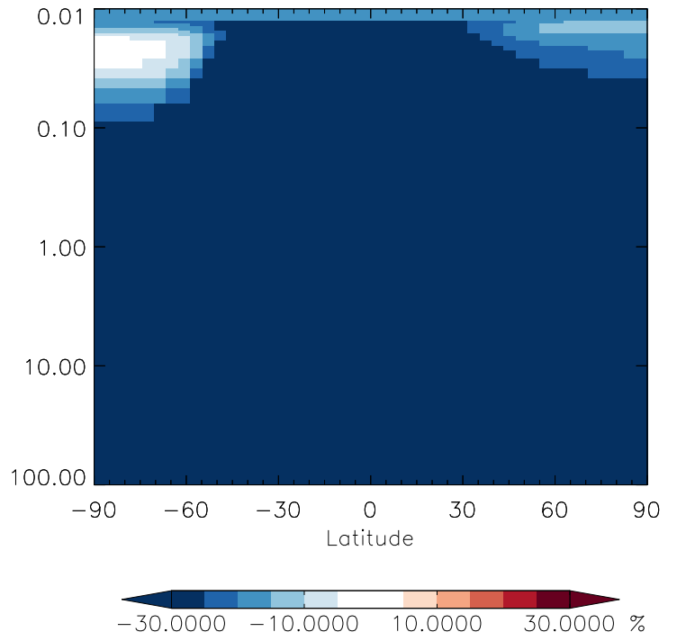
v11-01g-Run0 / v11-01d-Run1 CFC115 - Strat zonal mean % diff for Jul
