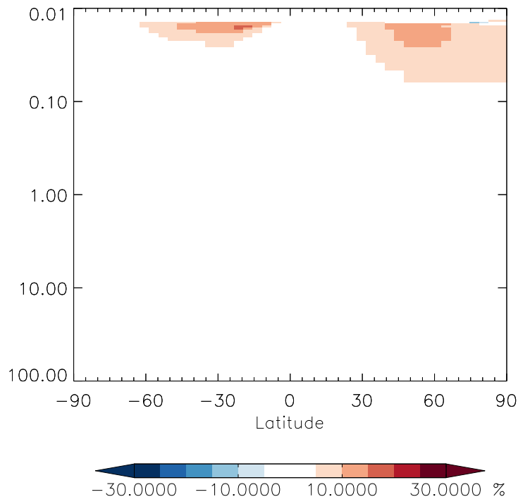
v11-01g-Run0 / v11-01f-geosfp-Run0 CH3Br - Strat zonal mean % diff for Jul
