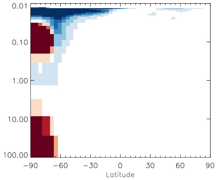
v11-01g-Run0 / v11-01f-geosfp-Run0 HNO 2 - Strat zonal mean % diff for Jul
