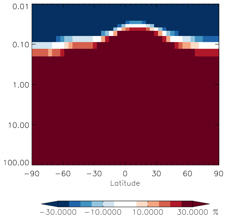
v11-01g-Run0 / v11-01d-Run1 CFC113 - Strat zonal mean % diff for Jul
