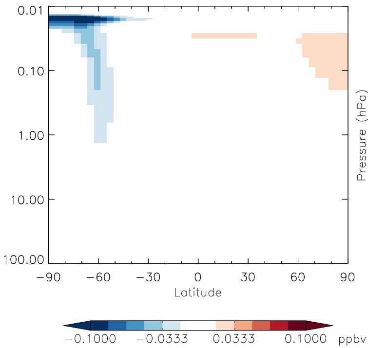
v11-01g-Run0 - v11-01d-Run1 ClNO 3 - Strat zonal mean abs diff for Jul
