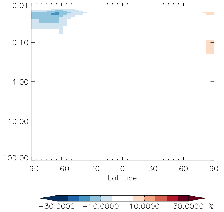
v11-01g-Run0 / v11-01d-Run1 CH2O - Strat zonal mean % diff for Jul
