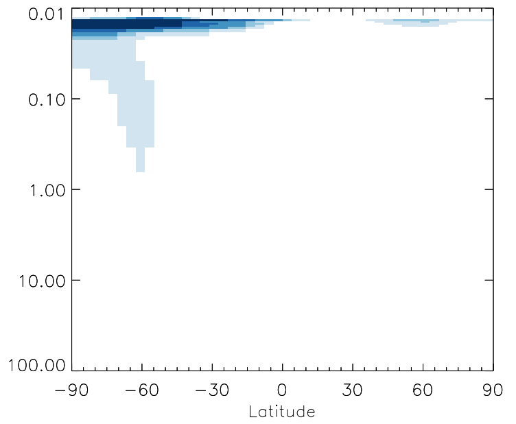
v11-01g-Run0 / v11-01f-geosfp-Run0 HNO 4 - Strat zonal mean % diff for Jul
