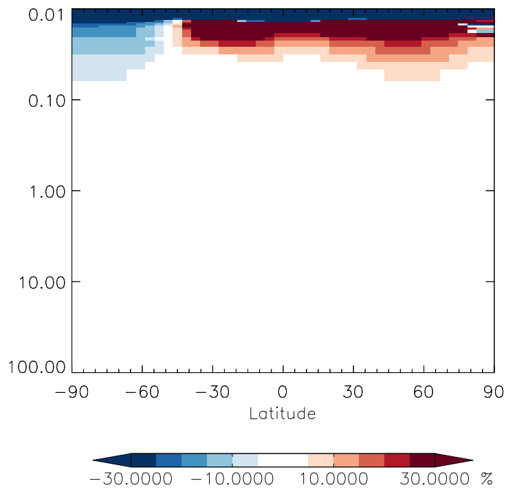
v11-01g-Run0 / v11-01d-Run1 CH 2 Br 2 - Strat zonal mean % diff for Jul
