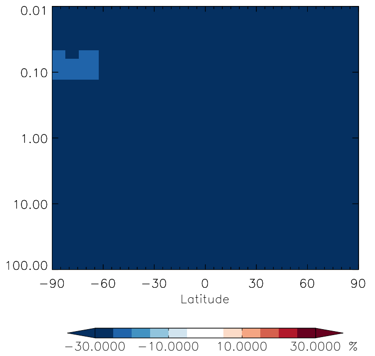
v11-01g-Run0 / v11-01d-Run1 CFC114 - Strat zonal mean % diff for Jul
