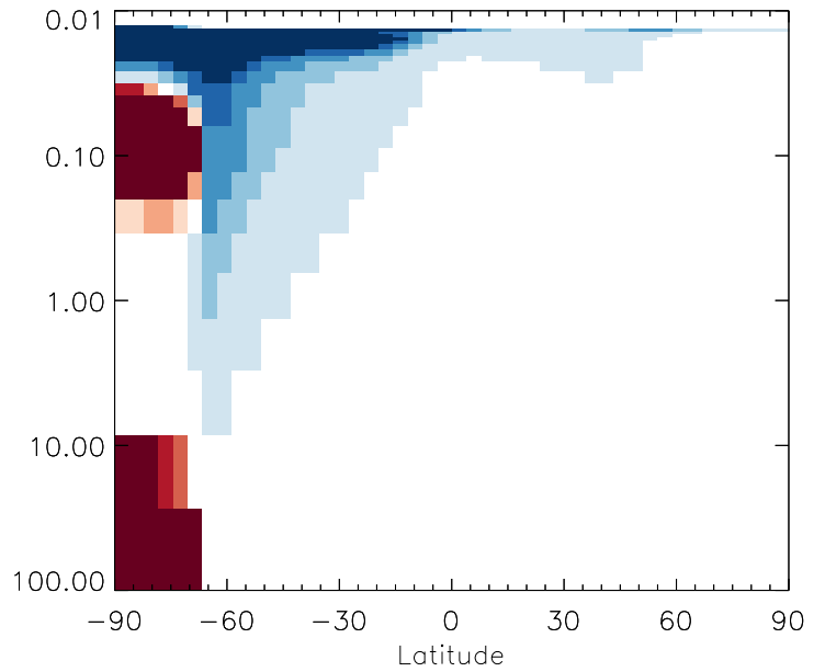
v11-01g-Run0 / v11-01d-Run1 HNO 2 - Strat zonal mean % diff for Jul
