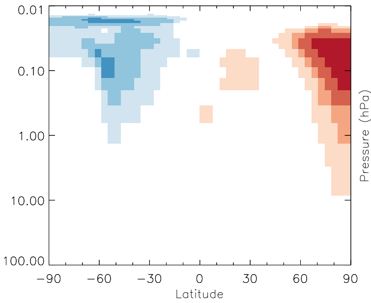
v11-01g-Run0 - v11-01f-geosfp-Run0 HNO 4 - Strat zonal mean abs diff for Jul
