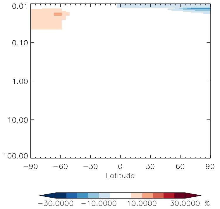
v11-01g-Run0 / v11-01d-Run1 CH3Cl - Strat zonal mean % diff for Jul
