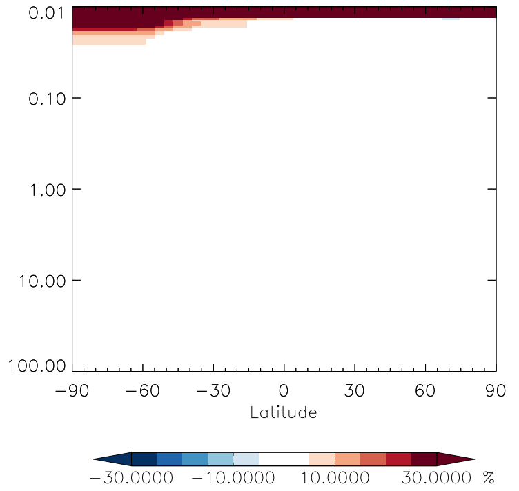
v11-01g-Run0 / v11-01d-Run1 N2O - Strat zonal mean % diff for Jul
