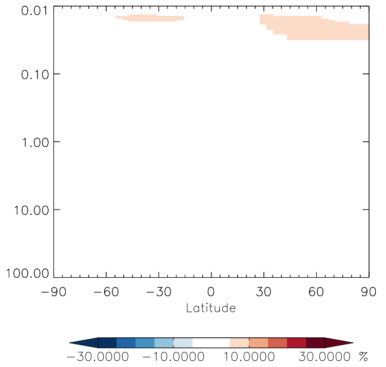
v11-01g-Run0 / v11-01f-geosfp-Run0 OCS - Strat zonal mean % diff for Jul
