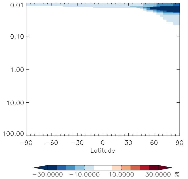
v11-01g-Run0 / v11-01f-geosfp-Run0 C2H6 - Strat zonal mean % diff for Jul
