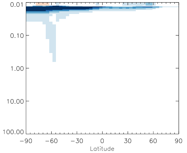
v11-01g-Run0 / v11-01d-Run1 HNO 4 - Strat zonal mean % diff for Jul
