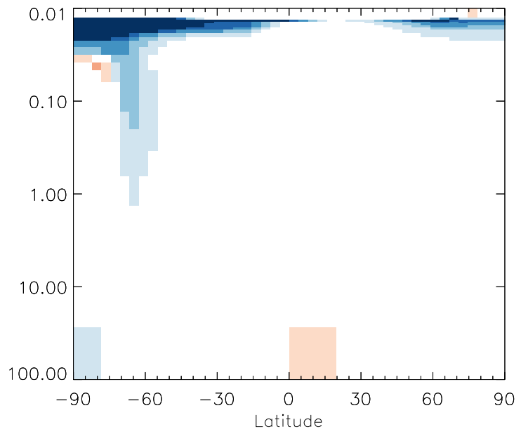
v11-01g-Run0 / v11-01f-geosfp-Run0 N2O5 - Strat zonal mean % diff for Jul
