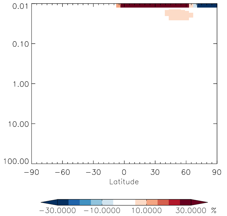
v11-01g-Run0 / v11-01f-geosfp-Run0 CFC11 - Strat zonal mean % diff for Jul
