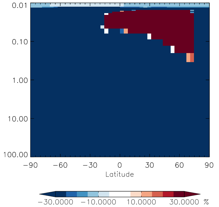
v11-01g-Run0 / v11-01d-Run1 MACRN - Strat zonal mean % diff for Jul
