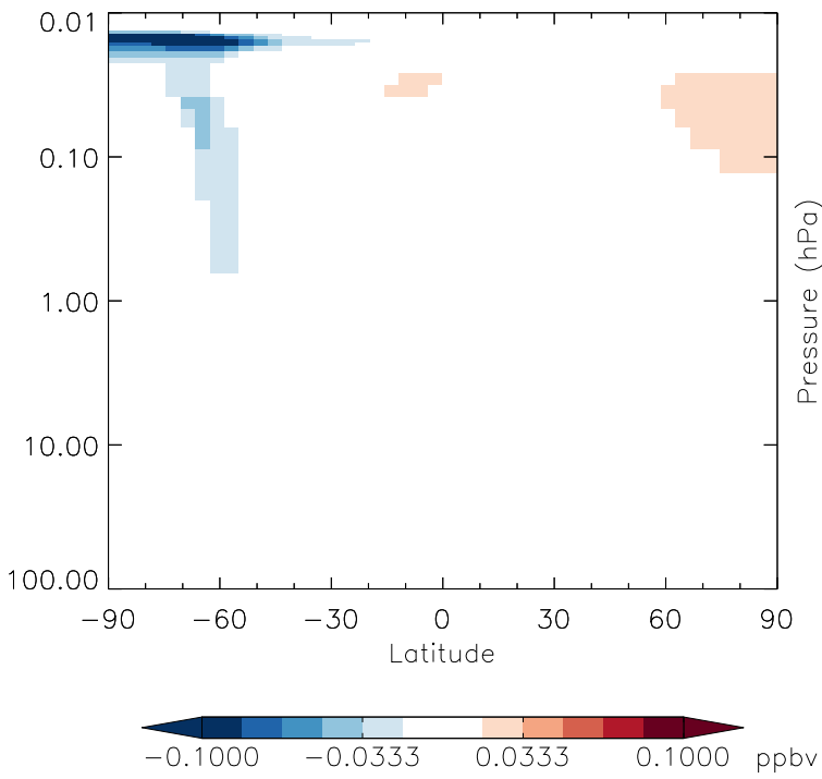
v11-01g-Run0 - v11-01f-geosfp-Run0 ClNO 3 - Strat zonal mean abs diff for Jul
