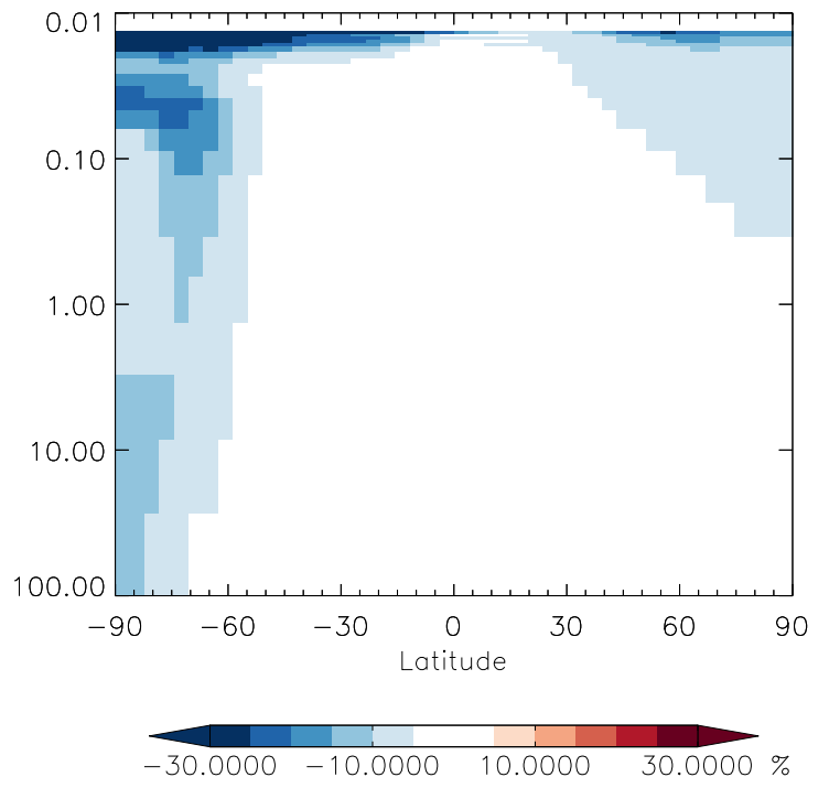
v11-01g-Run0 / v11-01f-geosfp-Run0 BrNO3 - Strat zonal mean % diff for Jul
