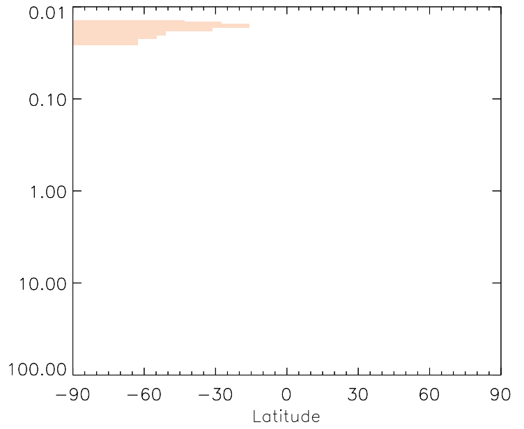
v11-01g-Run0 / v11-01f-geosfp-Run0 O3 - Strat zonal mean % diff for Jul
