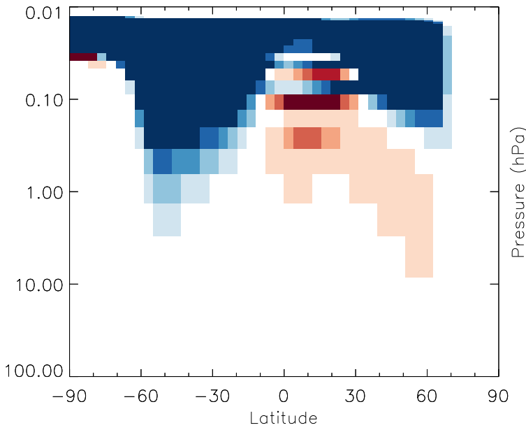
v11-01g-Run0 - v11-01d-Run1 N2O5 - Strat zonal mean abs diff for Jul
