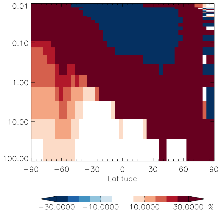
v11-01g-Run0 / v11-01f-geosfp-Run0 ISOP - Strat zonal mean % diff for Jul
