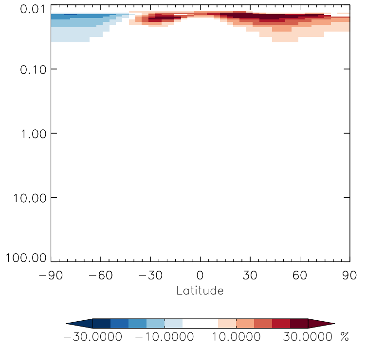
v11-01g-Run0 / v11-01d-Run1 CH3Br - Strat zonal mean % diff for Jul
