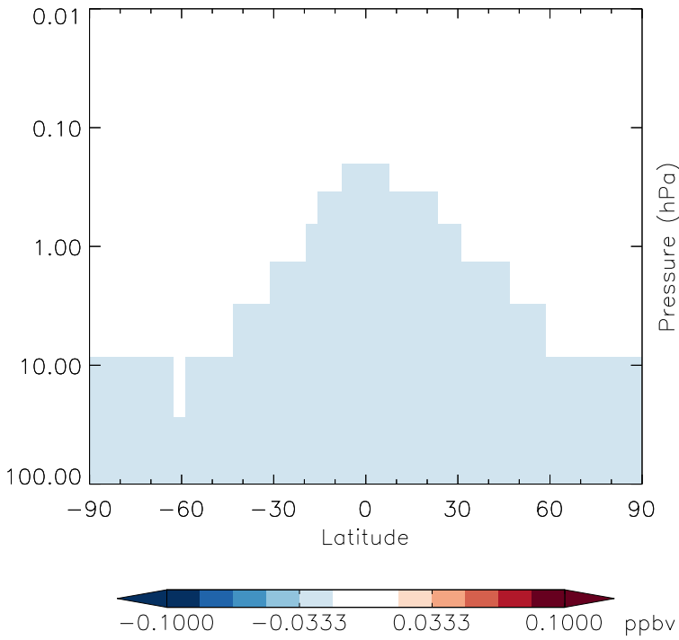
v11-01g-Run0 - v11-01d-Run1 CFC115 - Strat zonal mean abs diff for Jul
