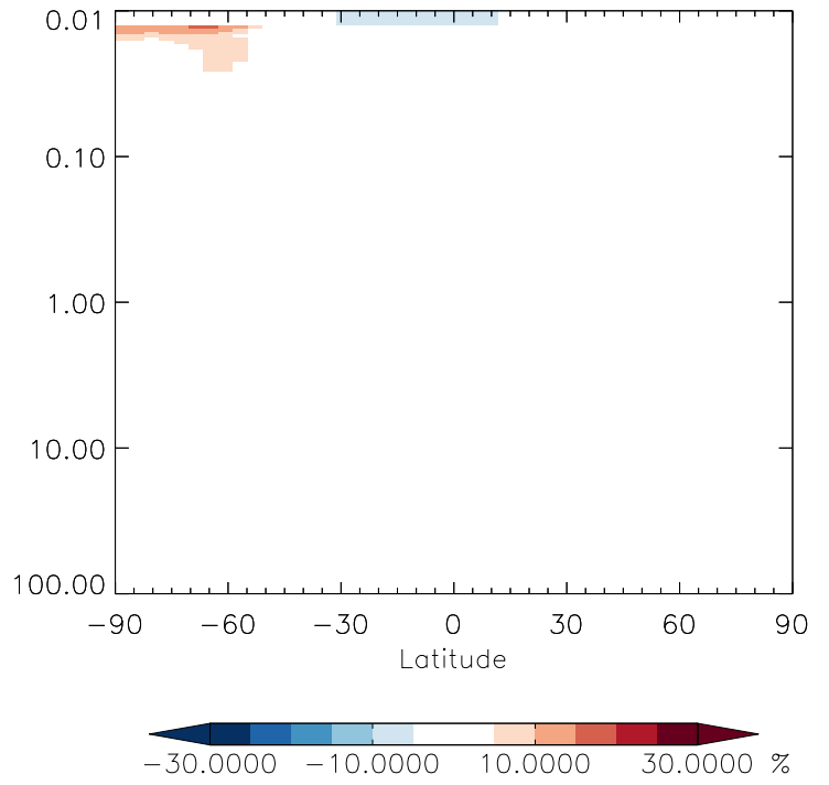
v11-01g-Run0 / v11-01d-Run1 CFC12 - Strat zonal mean % diff for Jul
