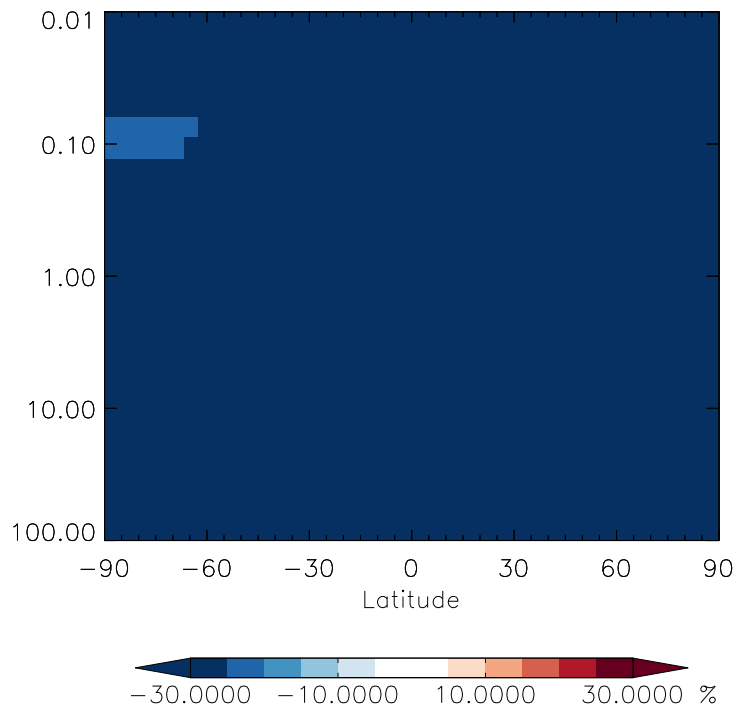
v11-01g-Run0 / v11-01f-geosfp-Run0 CFC114 - Strat zonal mean % diff for Jul
