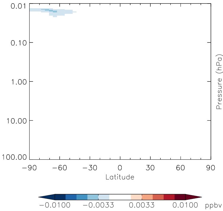
v11-01g-Run0 - v11-01f-geosfp-Run0 BrNO3 - Strat zonal mean abs diff for Jul
