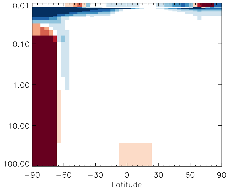
v11-01g-Run0 / v11-01d-Run1 N2O5 - Strat zonal mean % diff for Jul
