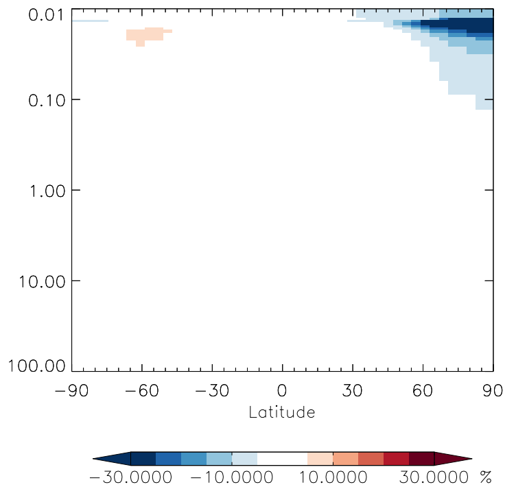
v11-01g-Run0 / v11-01d-Run1 C2H6 - Strat zonal mean % diff for Jul
