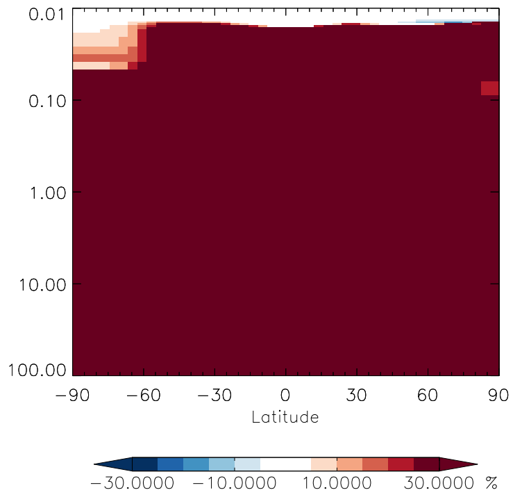
v11-01g-Run0 / v11-01f-geosfp-Run0 MVKN - Strat zonal mean % diff for Jul
