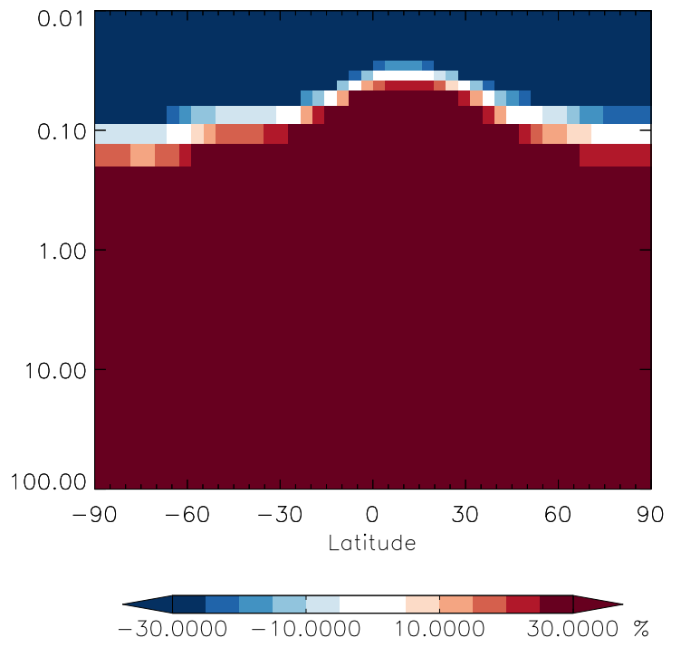
v11-01g-Run0 / v11-01f-geosfp-Run0 CFC113 - Strat zonal mean % diff for Jul
