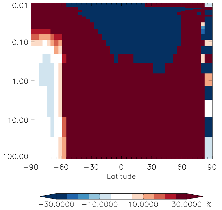
v11-01g-Run0 / v11-01d-Run1 ISOP - Strat zonal mean % diff for Jul
