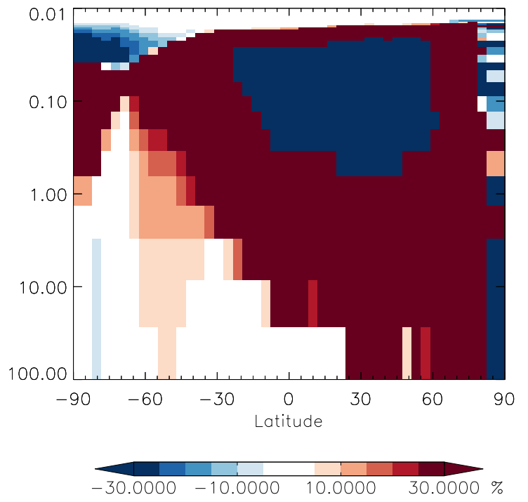
v11-01g-Run0 / v11-01f-geosp-Run0 MOBA - Strat zonal mean % diff for Jul
