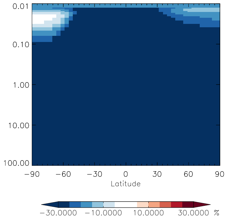
v11-01g-Run0 / v11-01f-geosfp-Run0 CFC115 - Strat zonal mean % diff for Jul
