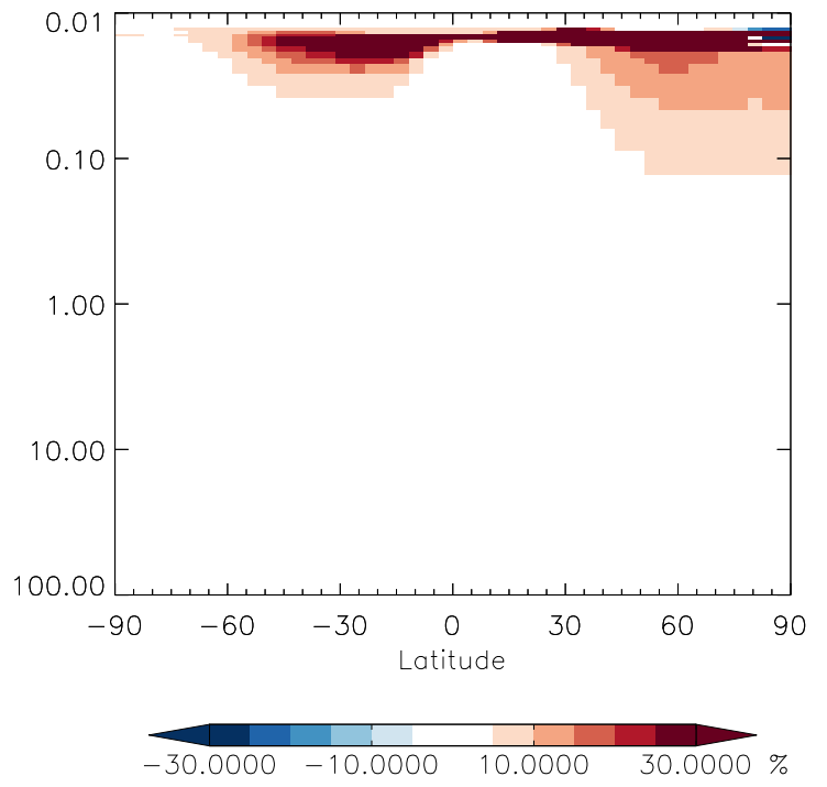
v11-01g-Run0 / v11-01f-geosfp-Run0 CH 2 Br 2 - Strat zonal mean % diff for Jul
