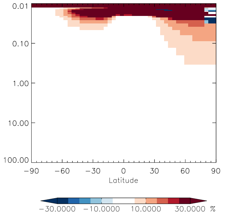
v11-01g-Run0 / v11-01f-geosfp-Run0 CHBr3 - Strat zonal mean % diff for Jul
