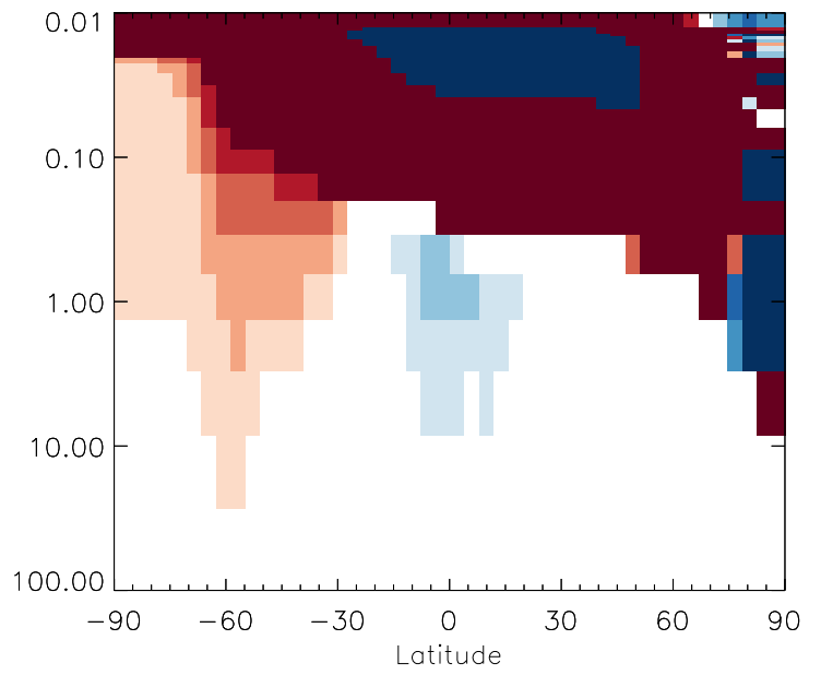
v11-01g-Run0 / v11-01f-geosfp-Run0 PRPE - Strat zonal mean % diff for Jul
