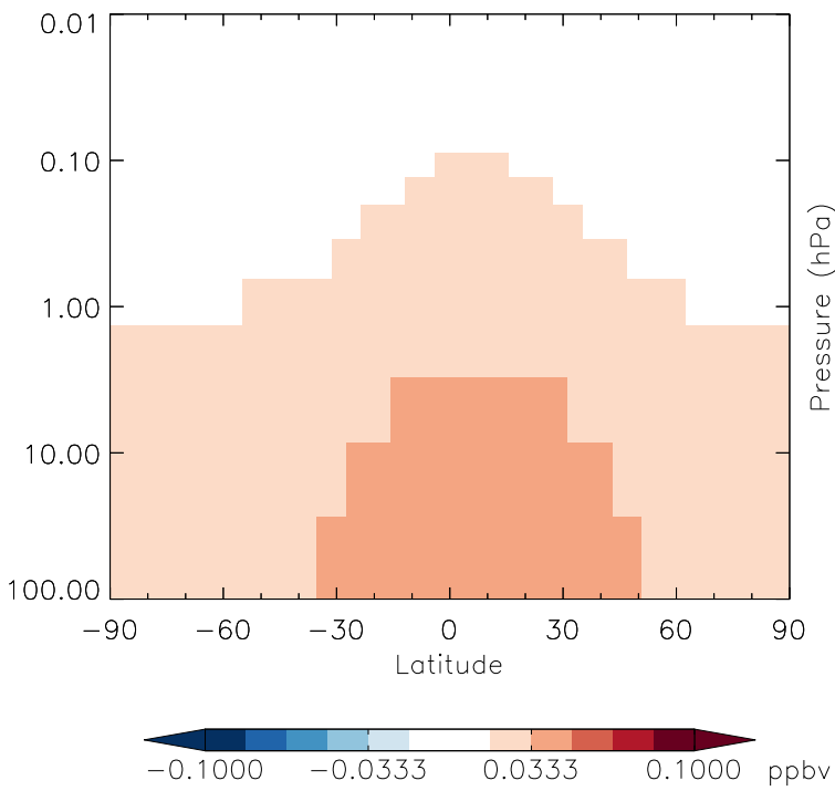
v11-01g-Run0 - v11-01d-Run1 CFC113 - Strat zonal mean abs diff for Jul
