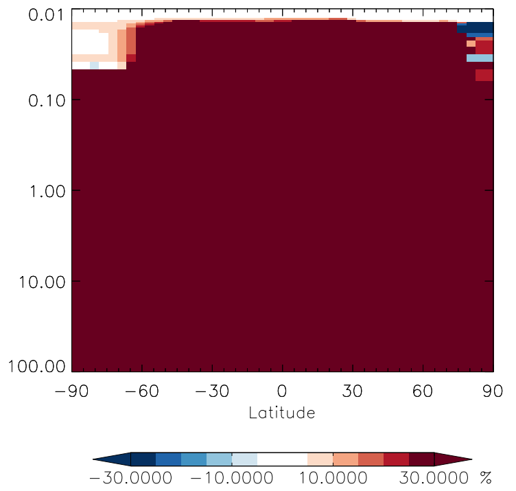
v11-01g-Run0 / v11-01d-Run1 MVKN - Strat zonal mean % diff for Jul
