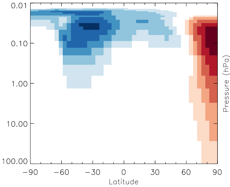
v11-01g-Run0 - v11-01d-Run1 HNO 4 - Strat zonal mean abs diff for Jul
