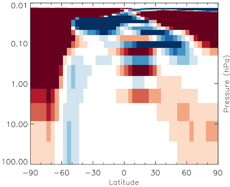
v11-01g-Run0 - v11-01d-Run1 O3 - Strat zonal mean abs diff for Jul
