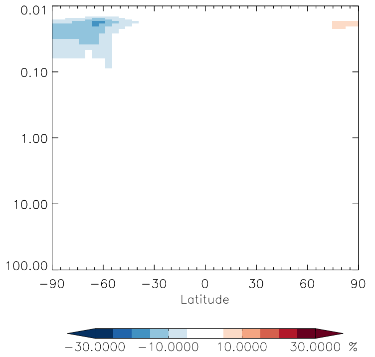
v11-01g-Run0 / v11-01f-geosfp-Run0 CH2O - Strat zonal mean % diff for Jul
