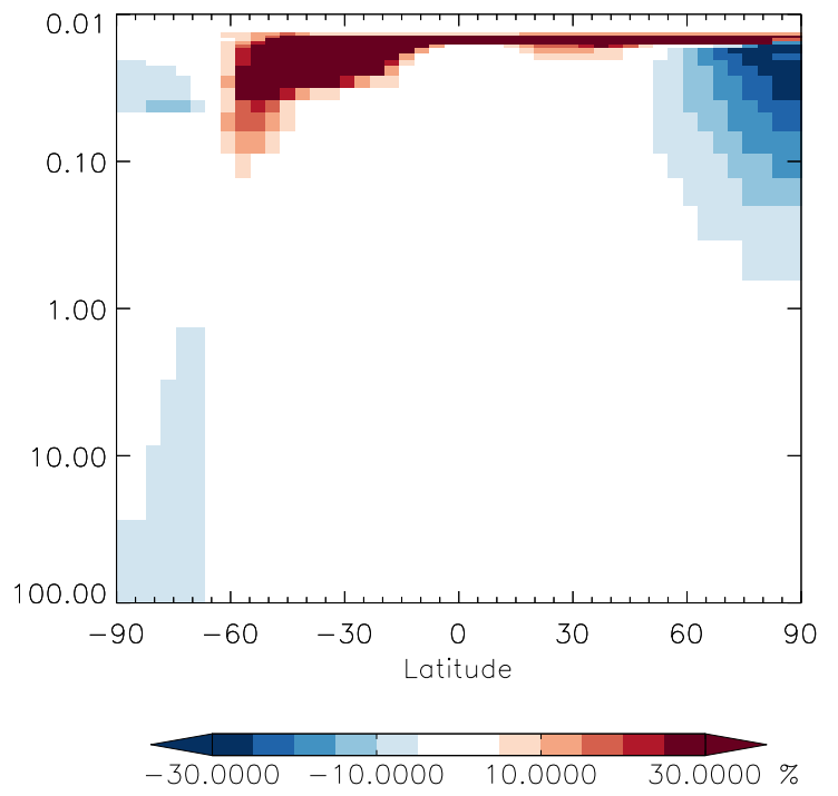
v11-01g-Run0 / v11-01d-Run1 RCHO - Strat zonal mean % diff for Jul
