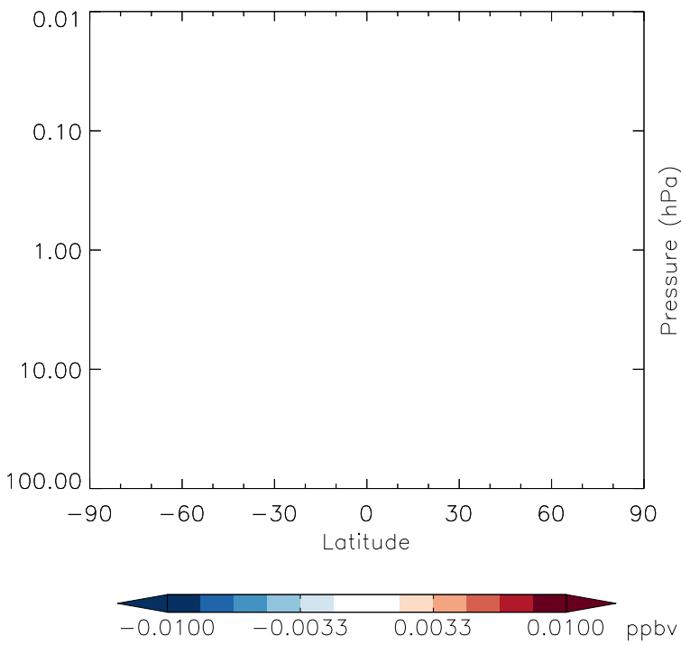
v11-01g-Run0 - v11-01d-Run1 MOBA - Strat zonal mean abs diff for Jul
