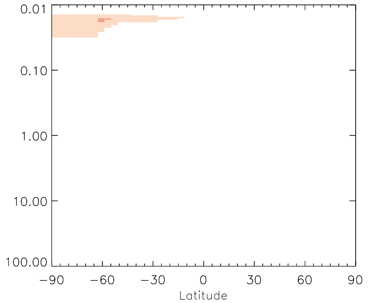
v11-01g-Run0 / v11-01d-Run1 O3 - Strat zonal mean % diff for Jul
