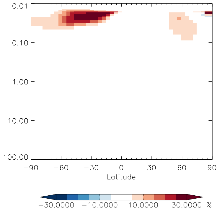
v11-01g-Run0 / v11-01f-geosfp-Run0 R4N2 - Strat zonal mean % diff for Jul
