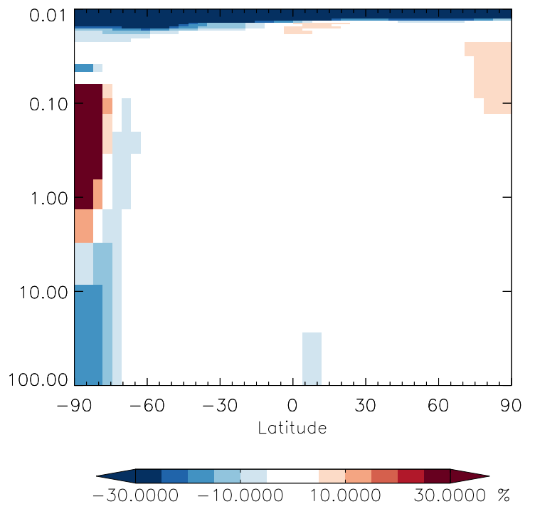
v11-01g-Run0 / v11-01d-Run1 ClNO 3 - Strat zonal mean % diff for Jul
