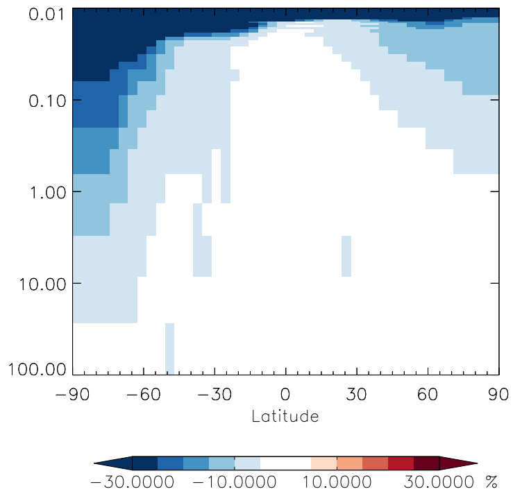
v11-01g-Run0 / v11-01f-geosfp-Run0 BrNO2 - Strat zonal mean % diff for Jul
