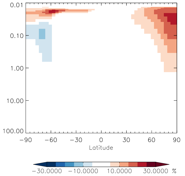
v11-01g-Run0 / v11-01f-geosfp-Run0 H2O2 - Strat zonal mean % diff for Jul
