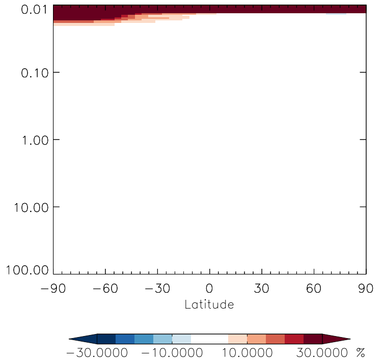
v11-01g-Run0 / v11-01f-geosfp-Run0 N2O - Strat zonal mean % diff for Jul
