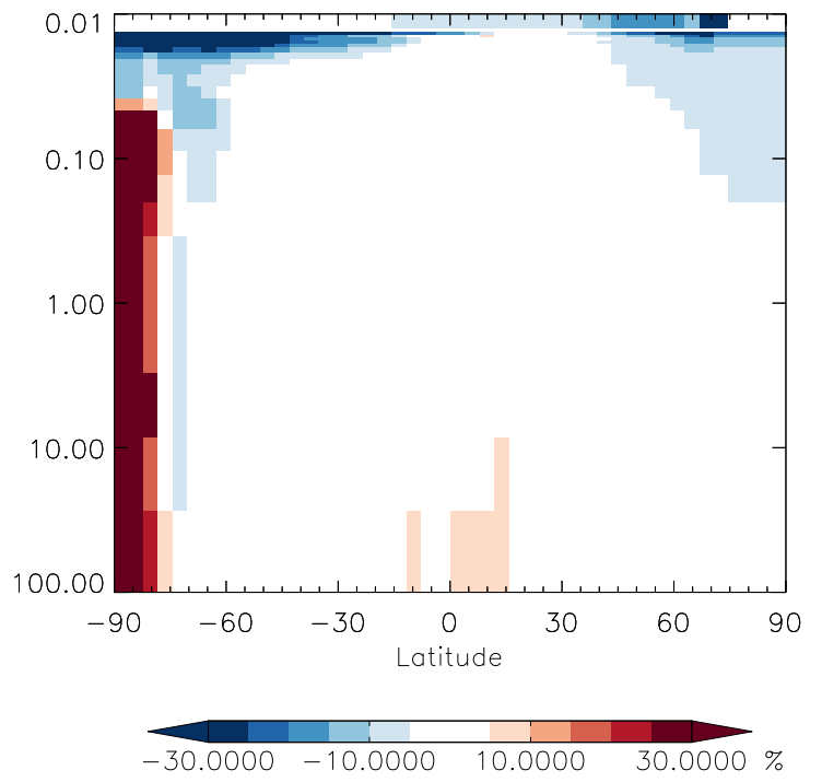
v11-01g-Run0 / v11-01d-Run1 BrNO3 - Strat zonal mean % diff for Jul
