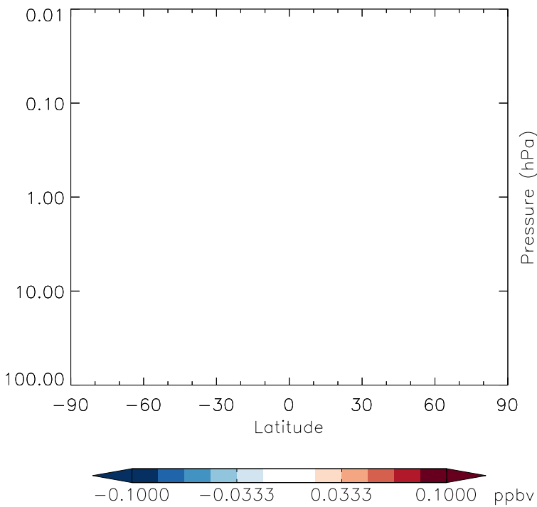
v11-01g-Run0 - v11-01d-Run1 CFC11 - Strat zonal mean abs diff for Jul
