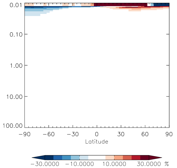
v11-01g-Run0 / v11-01d-Run1 CFC11 - Strat zonal mean % diff for Jul
