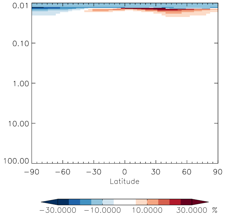
v11-01g-Run0 / v11-01d-Run1 OCS - Strat zonal mean % diff for Jul
