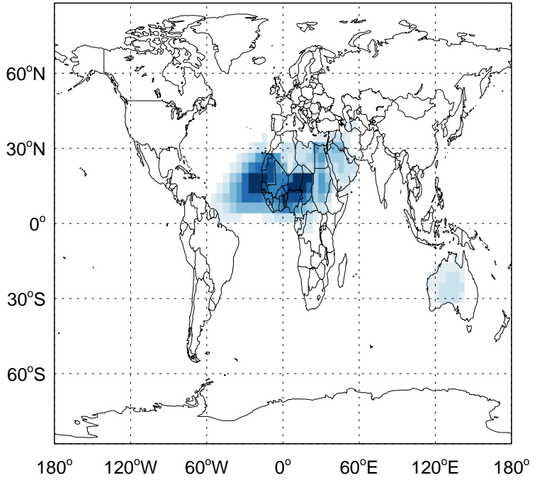
v11-02a - v11-01-public-Run0 SALC: Column AOD diff for Jan
