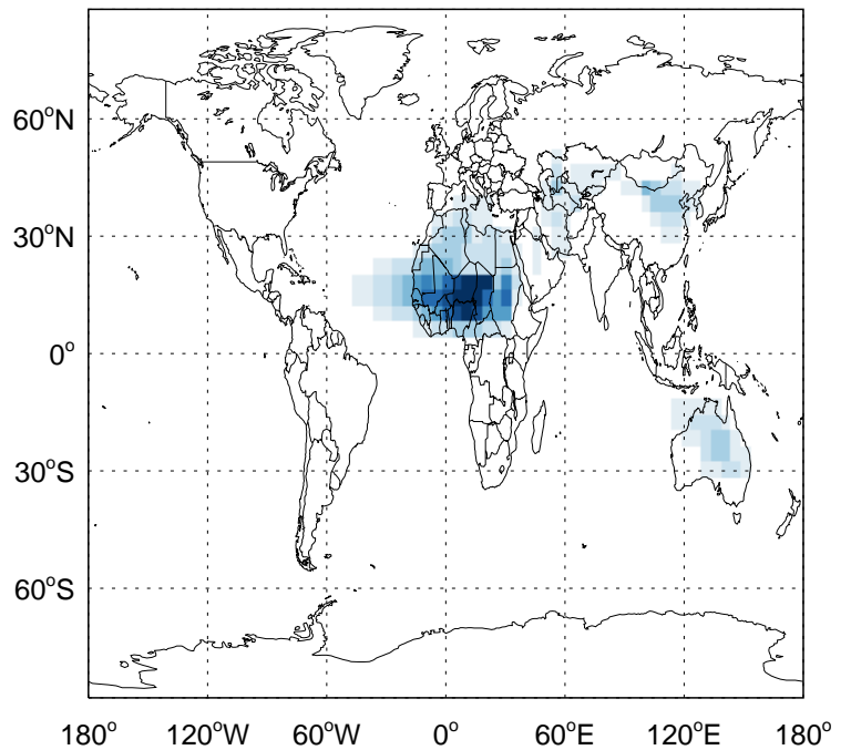
v11-02a - v11-01k-Run0 SALC: Column AOD diff for Oct
