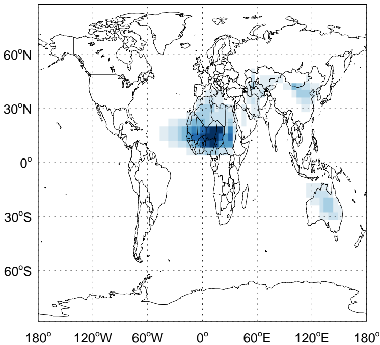
v11-02a - v11-01-public-Run0 SALC: Column AOD diff for Oct
