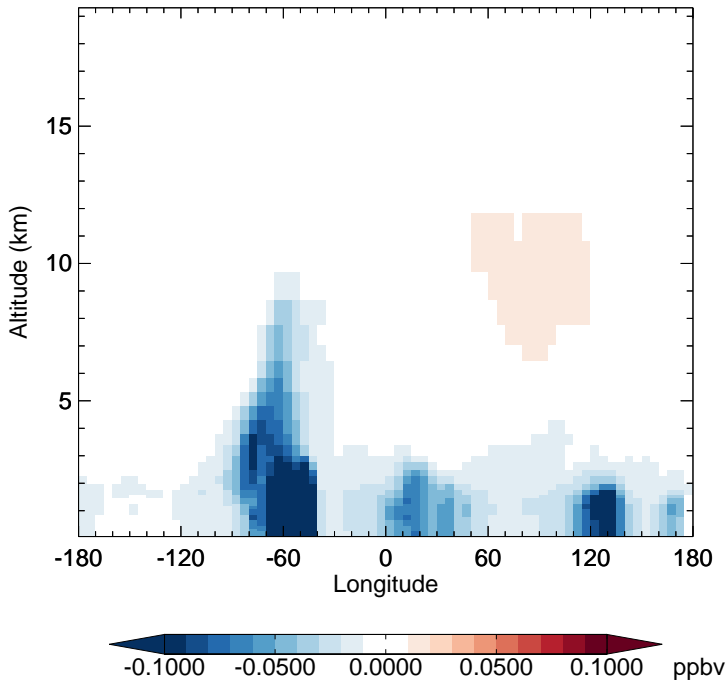
v11-02a - v11-01k-Run0 H2O2 - Diff along 15S for Jul
