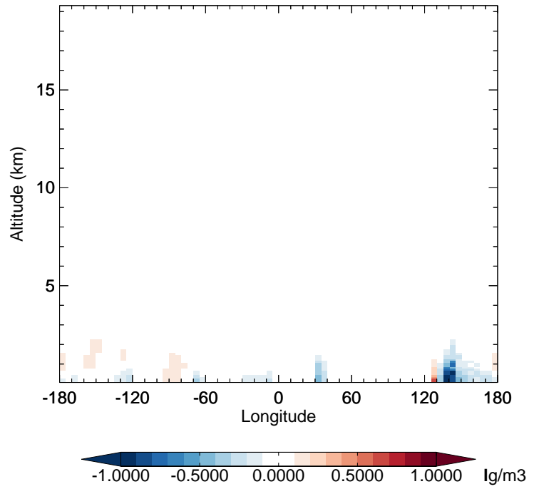
v11-02a - v11-01-public-Run0 SO4 - Diff along 42N for Jul
