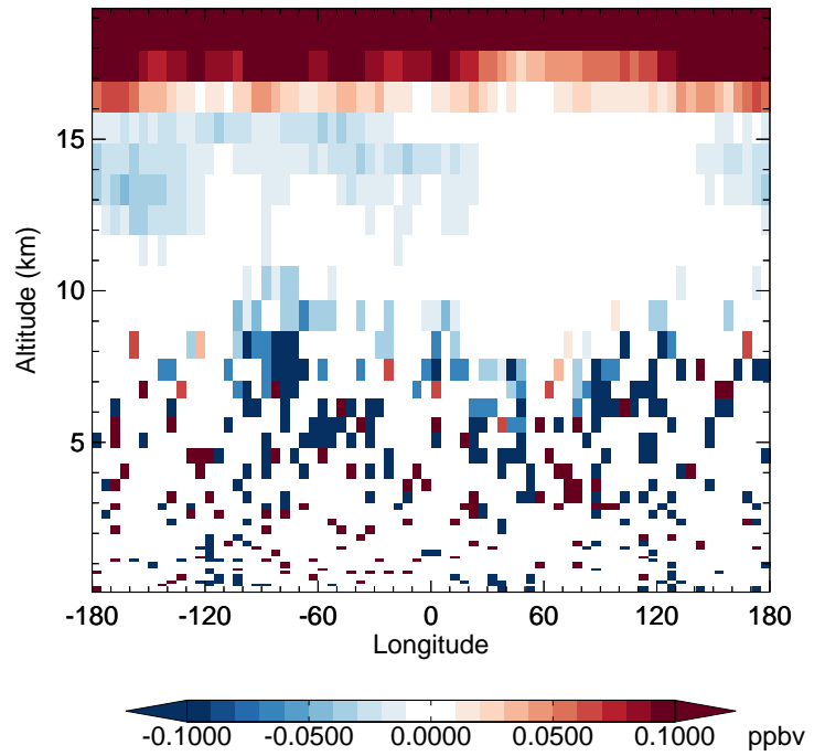
v11-02a - v11-01k-Run0 H 2 O - Diff along 42N for Jul
