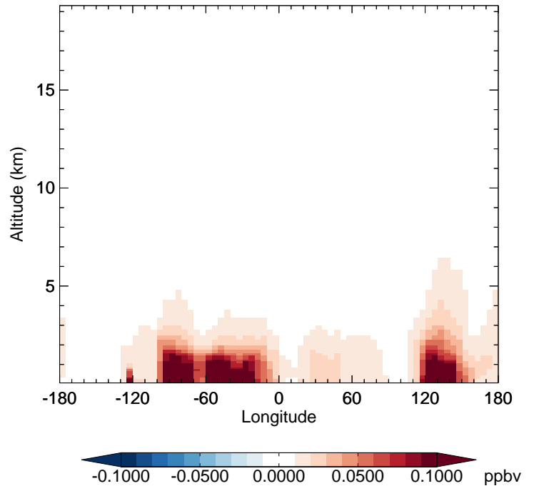
v11-02a - v11-01-public-Run0 BENZ - Diff along 42N for Jul
