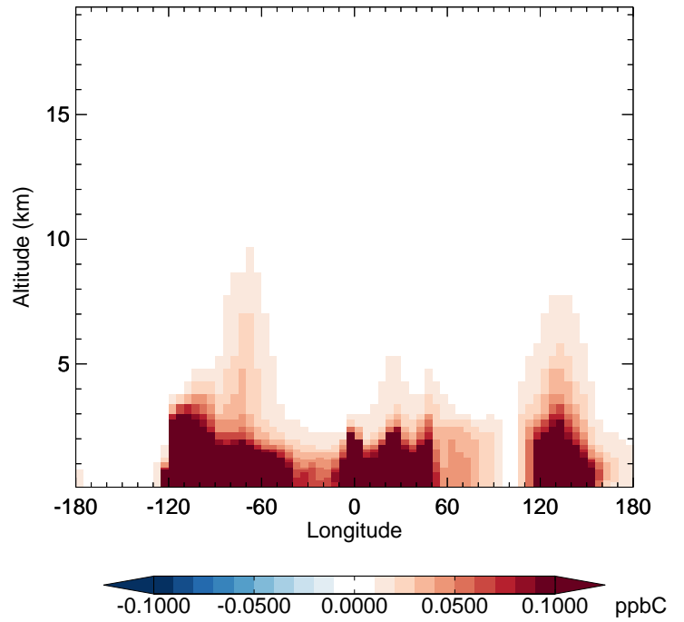
v11-02a - v11-01k-Run0 MEK - Diff along 42N for Jul
