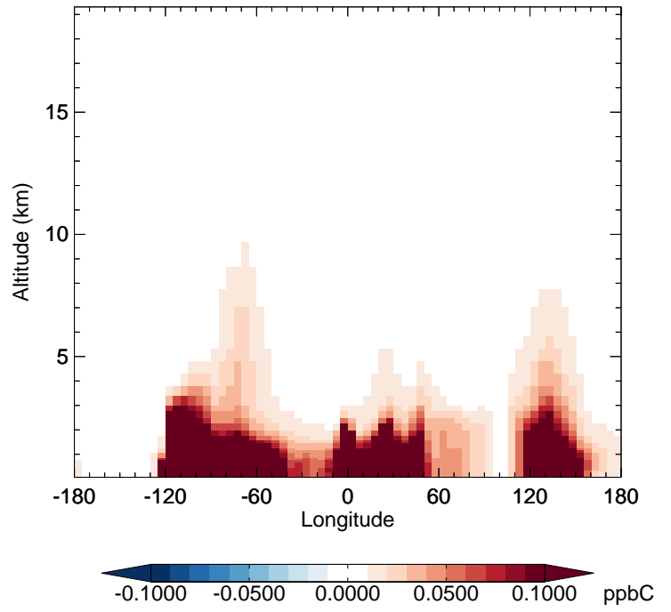
v11-02a - v11-01-public-Run0 MEK - Diff along 42N for Jul
