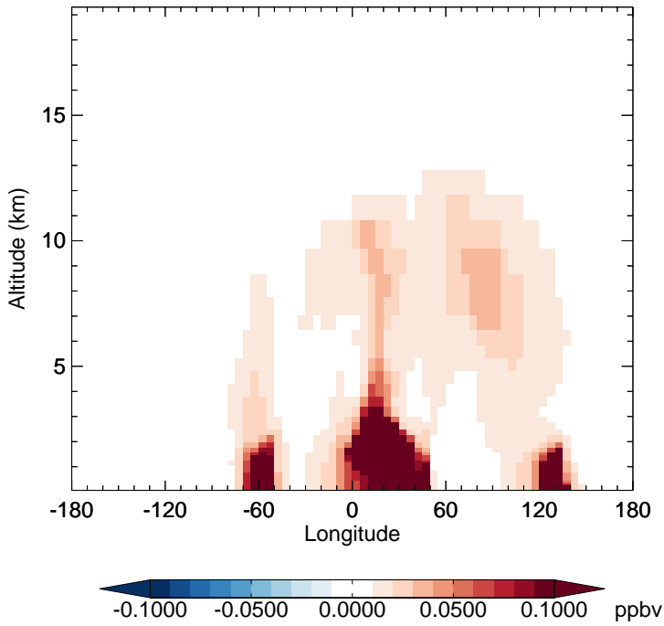
v11-02a - v11-01k-Run0 BENZ - Diff along 15S for Jul
