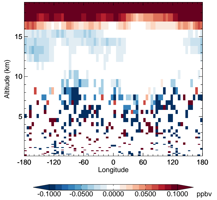
v11-02a - v11-01-public-Run0 H 2 O - Diff along 42N for Jul
