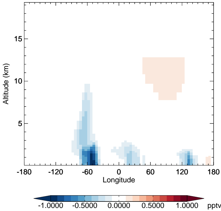
v11-02a - v11-01k-Run0 HO2 - Diff along 15S for Jul
