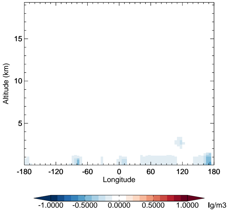
v11-02a - v11-01-public-Run0 SO4 - Diff along 15S for Jul
