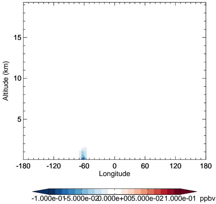
v11-02a - v11-01-public-Run0 MTPA - Diff along 15S for Jul
