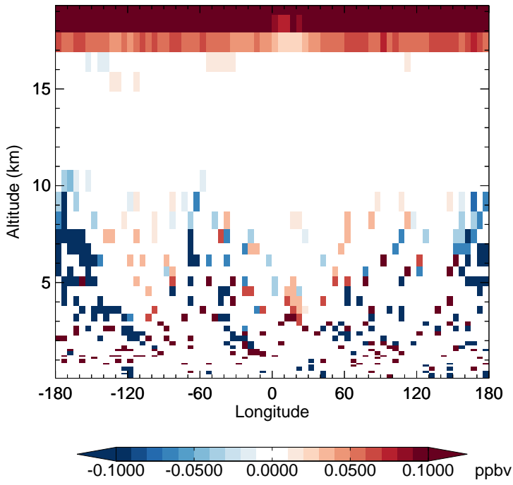
v11-02a - v11-01-public-Run0 H 2 O - Diff along 15S for Jul
