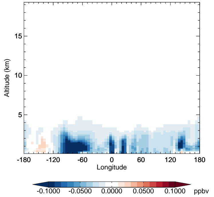
v11-02a - v11-01-public-Run0 H2O2 - Diff along 42N for Jul
