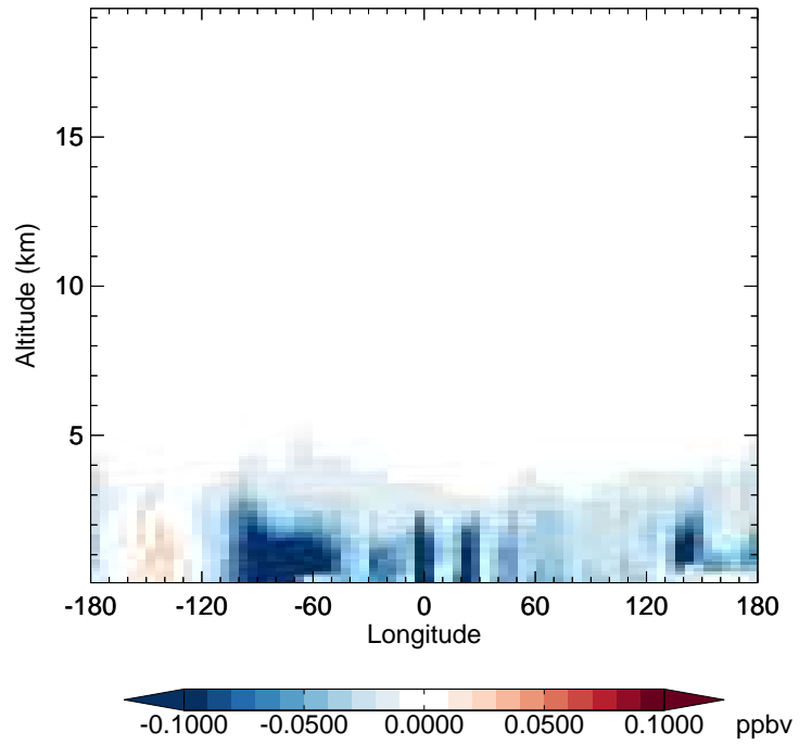
v11-02a - v11-01k-Run0 H2O2 - Diff along 42N for Jul
