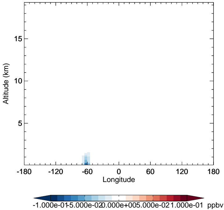
v11-02a - v11-01k-Run0 MTPA - Diff along 15S for Jul
