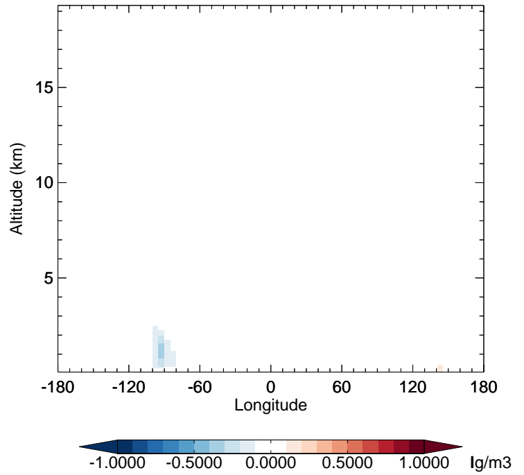
v11-02a - v11-01k-Run0 NH3 - Diff along 42N for Jul
