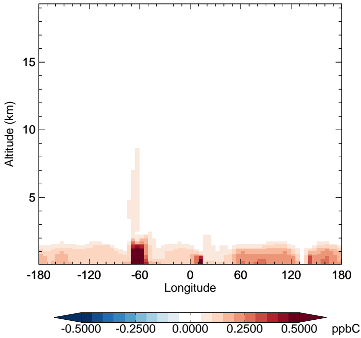
v11-02a - v11-01-public-Run0 ALD2 - Diff along 15S for Jul
