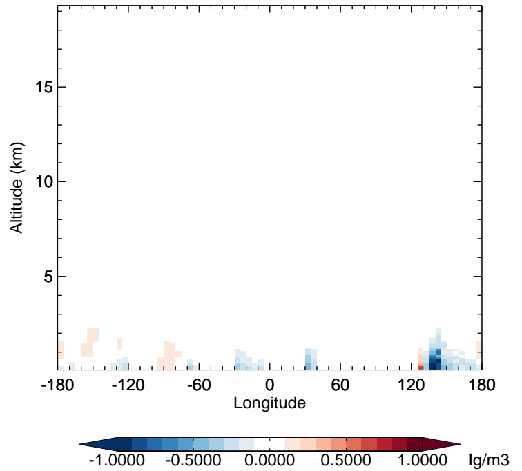
v11-02a - v11-01k-Run0 SO4 - Diff along 42N for Jul
