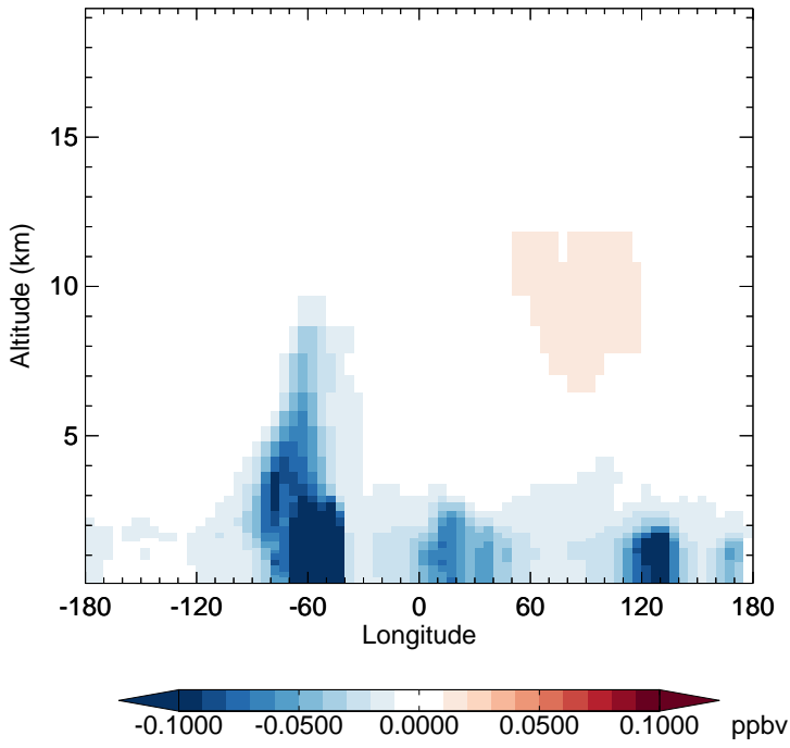
v11-02a - v11-01-public-Run0 H2O2 - Diff along 15S for Jul
