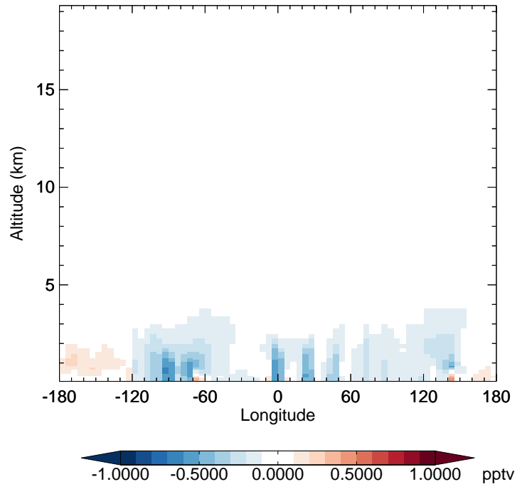
v11-02a - v11-01-public-Run0 HO2 - Diff along 42N for Jul
