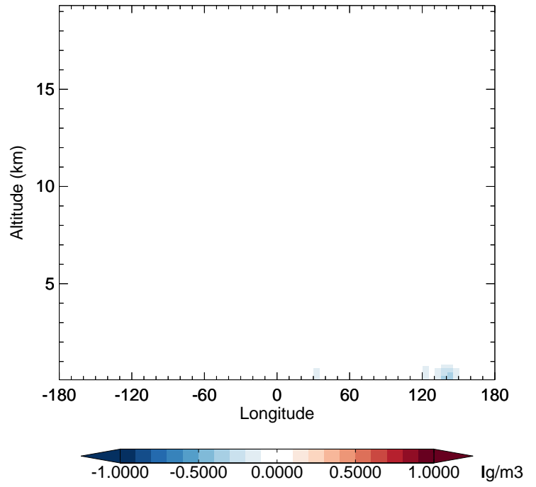
v11-02a - v11-01-public-Run0 NH4 - Diff along 42N for Jul
