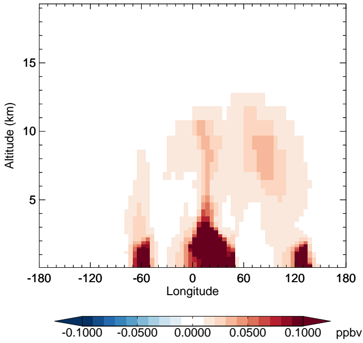
v11-02a - v11-01-public-Run0 BENZ - Diff along 15S for Jul
