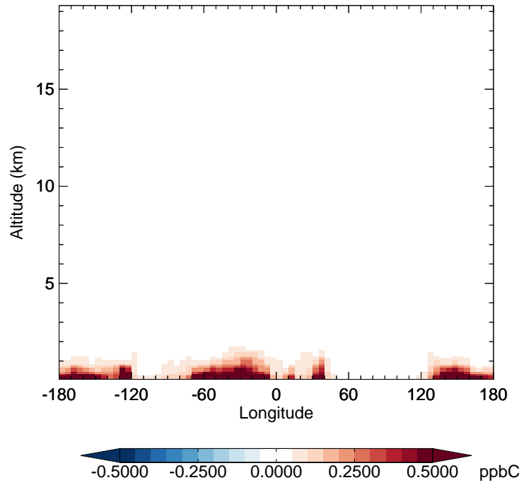
v11-02a - v11-01-public-Run0 ALD2 - Diff along 42N for Jul
