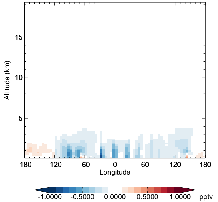
v11-02a - v11-01k-Run0 HO2 - Diff along 42N for Jul
