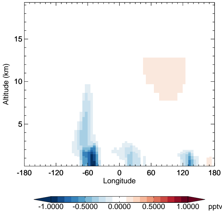
v11-02a - v11-01-public-Run0 HO2 - Diff along 15S for Jul
