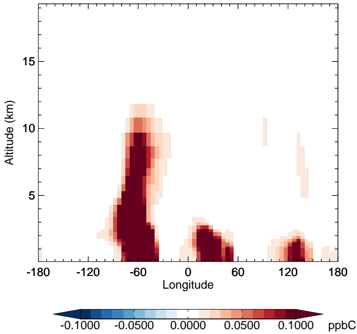
v11-02a - v11-01k-Run0 MEK - Diff along 15S for Jul
