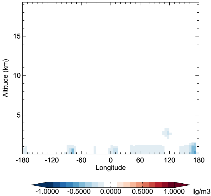
v11-02a - v11-01k-Run0 SO4 - Diff along 15S for Jul
