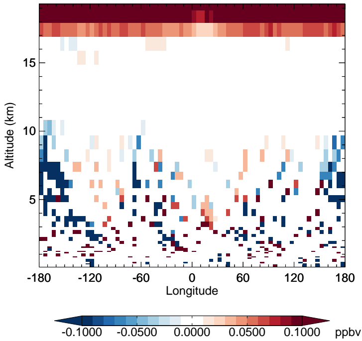
v11-02a - v11-01k-Run0 H 2 O - Diff along 15S for Jul
