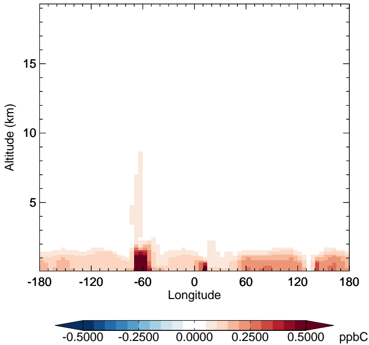
v11-02a - v11-01k-Run0 ALD2 - Diff along 15S for Jul
