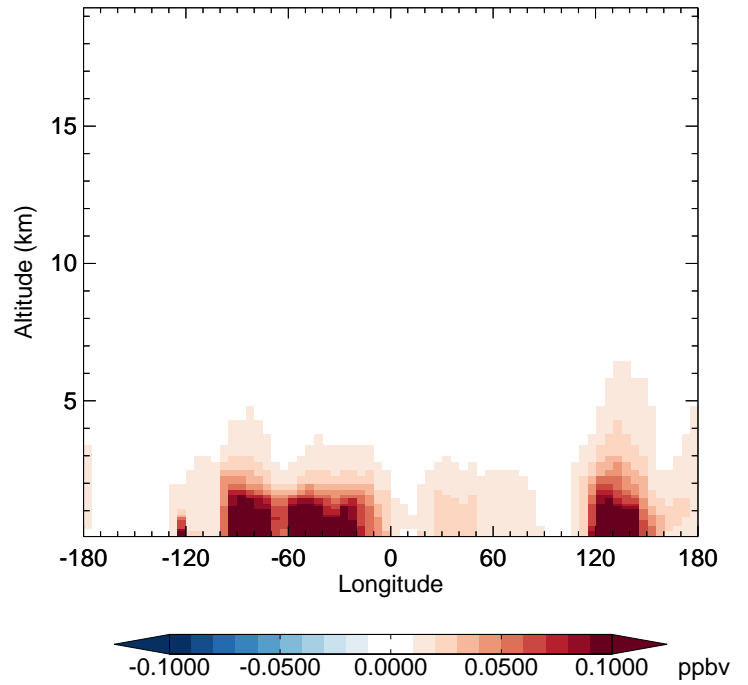
v11-02a - v11-01k-Run0 BENZ - Diff along 42N for Jul
