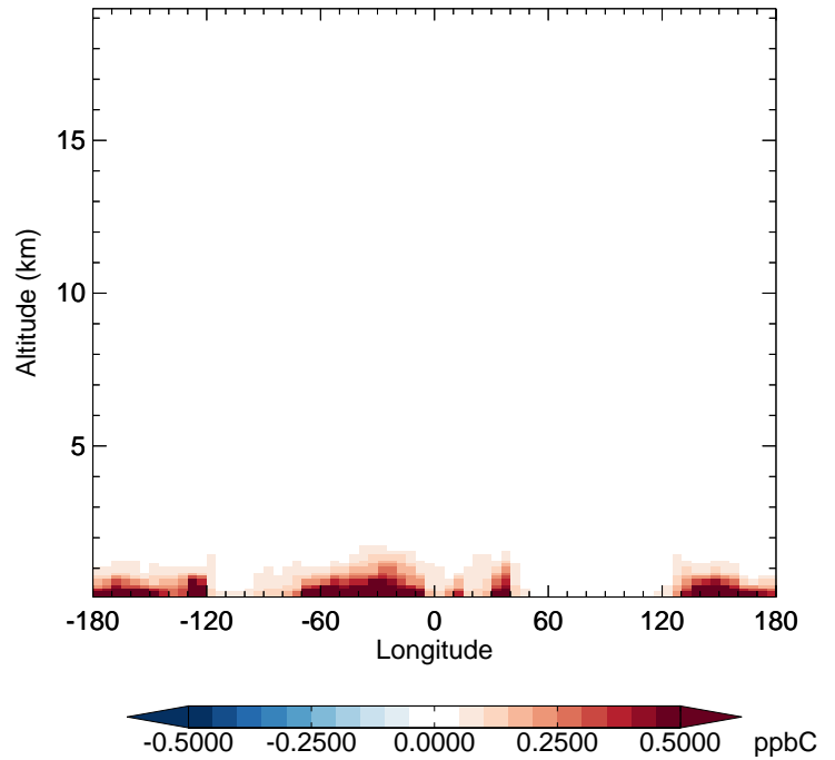
v11-02a - v11-01k-Run0 ALD2 - Diff along 42N for Jul
