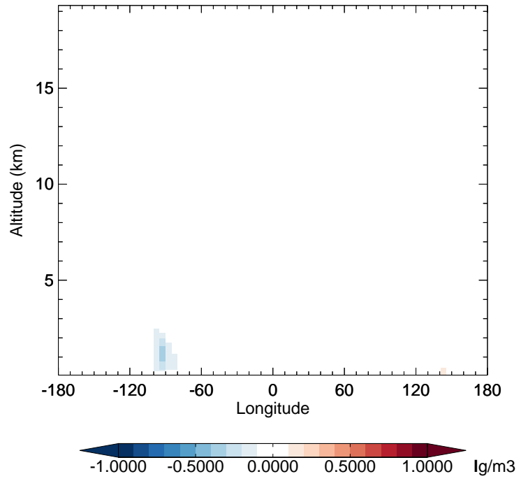
v11-02a - v11-01-public-Run0 NH3 - Diff along 42N for Jul
