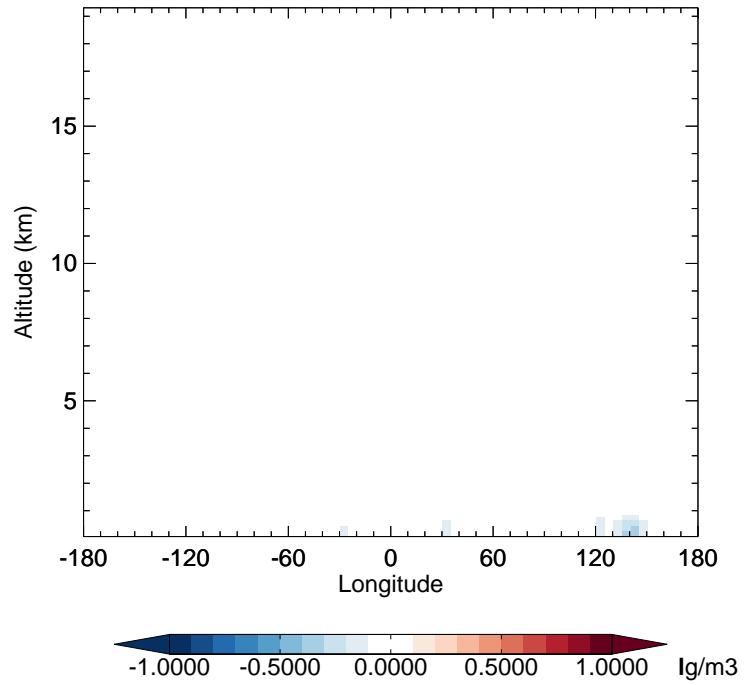
v11-02a - v11-01k-Run0 NH4 - Diff along 42N for Jul
