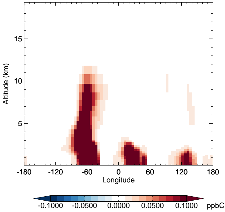
v11-02a - v11-01-public-Run0 MEK - Diff along 15S for Jul
