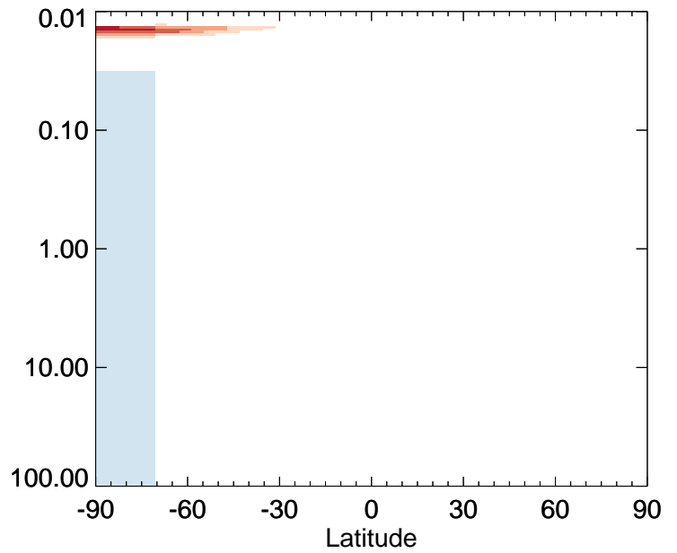
N2O5 - Strat zonal mean % diff for Jan
