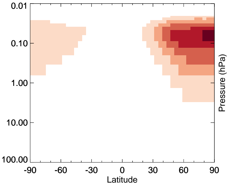
HNO 3 - Strat zonal mean abs diff for Jan
