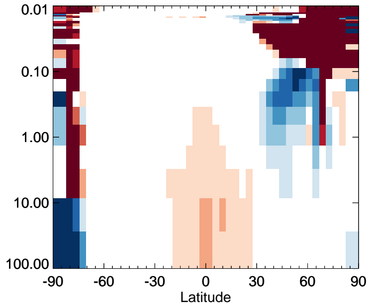
ISOP - Strat zonal mean % diff for Jan
