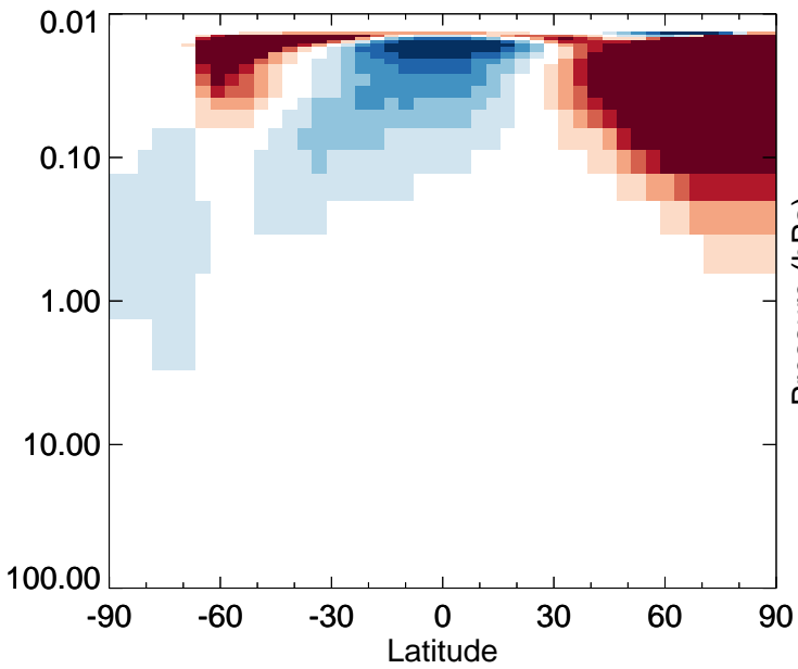
N2O5 - Strat zonal mean abs diff for Jan
