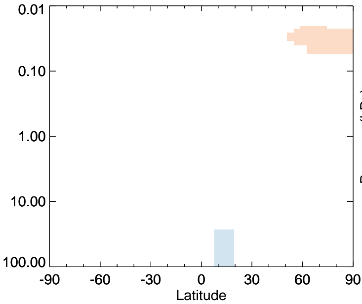
OH - Strat zonal mean abs diff for Jul
