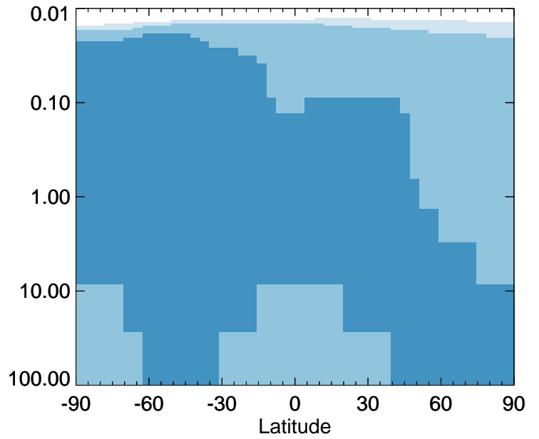
v11-02a / v11-01-public-Run0 CO - Strat zonal mean % diff for Jul
