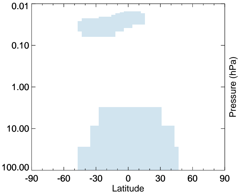
v11-02a - v11-01-public-Run0 CO - Strat zonal mean abs diff for Jul
