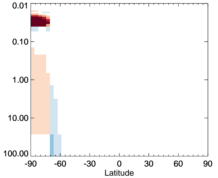
OH - Strat zonal mean % diff for Jul
