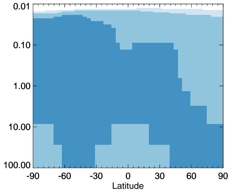
v11-02a / v11-01k-Run0 CO - Strat zonal mean % diff for Jul
