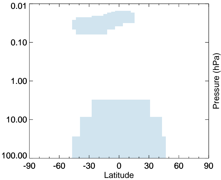
v11-02a - v11-01k-Run0 CO - Strat zonal mean abs diff for Jul
