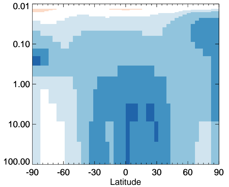
Cl2O2 - Strat zonal mean % diff for Oct
