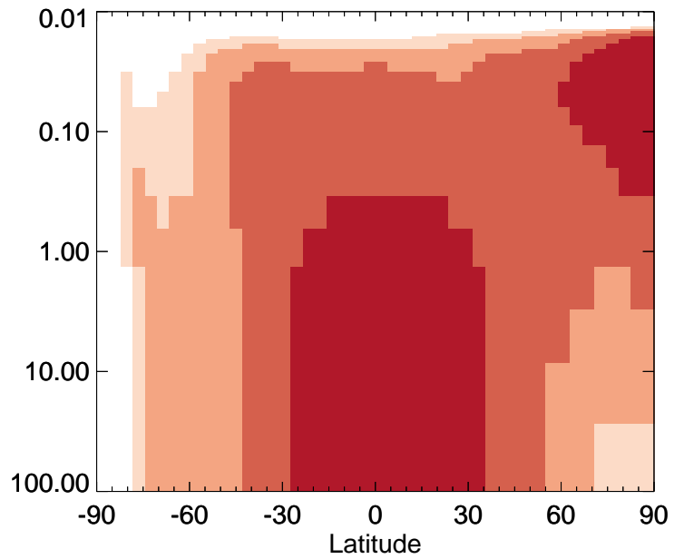
NO3 - Strat zonal mean % diff for Oct
