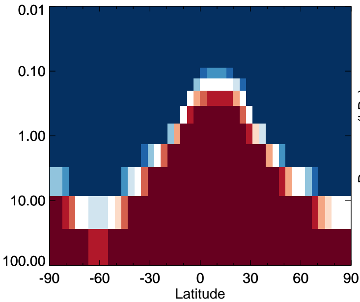
CH4 - Strat zonal mean abs diff for Oct
