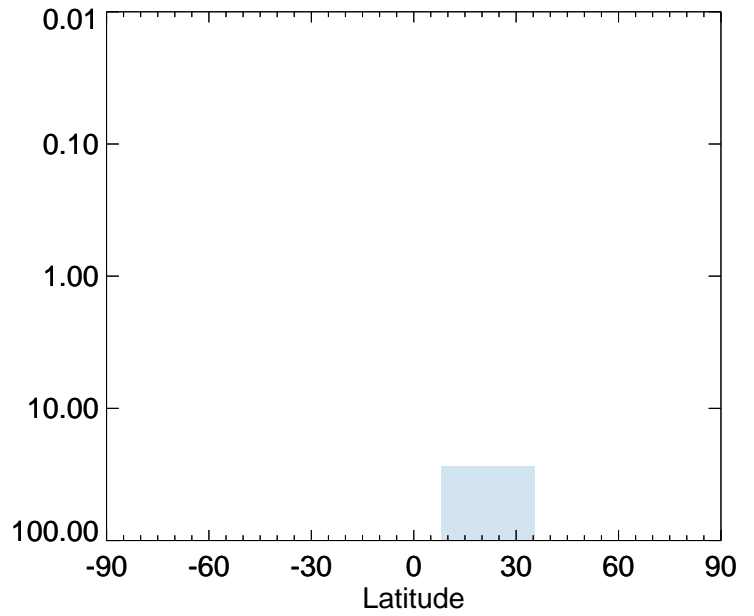
ISOG2 - Strat zonal mean % diff for Oct
