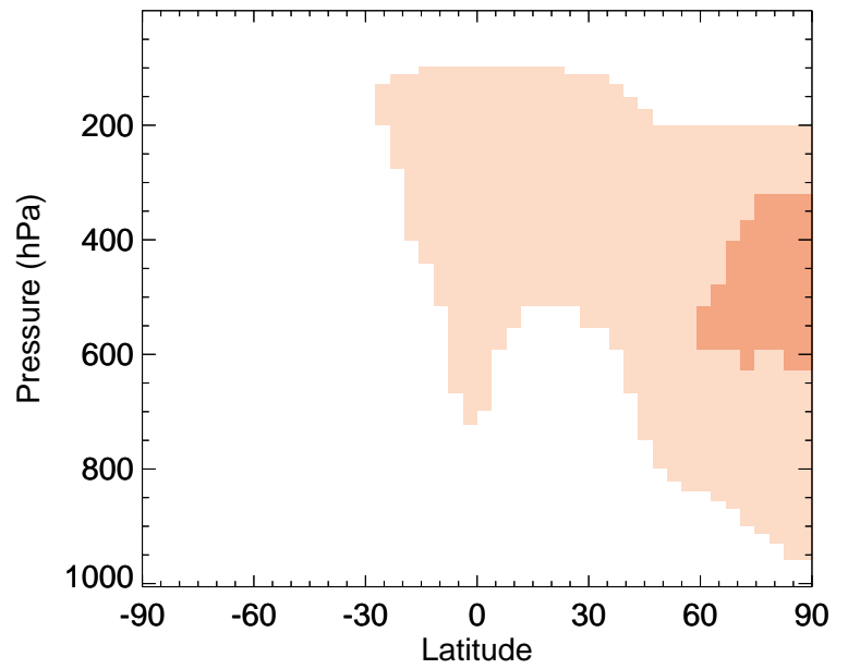
v11-02a / v11-01-public-Run0 MSA - Zonal mean % diff for Jul
