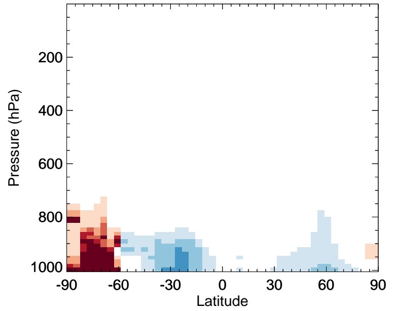
v11-02a / v11-01-public-Run0 HNO 3 - Zonal mean % diff for Jul
