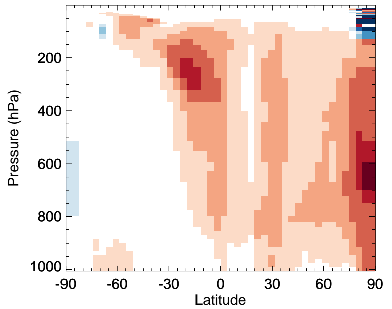
v11-02a / v11-01-public-Run0 ISOPNB - Zonal mean % diff for Jul
