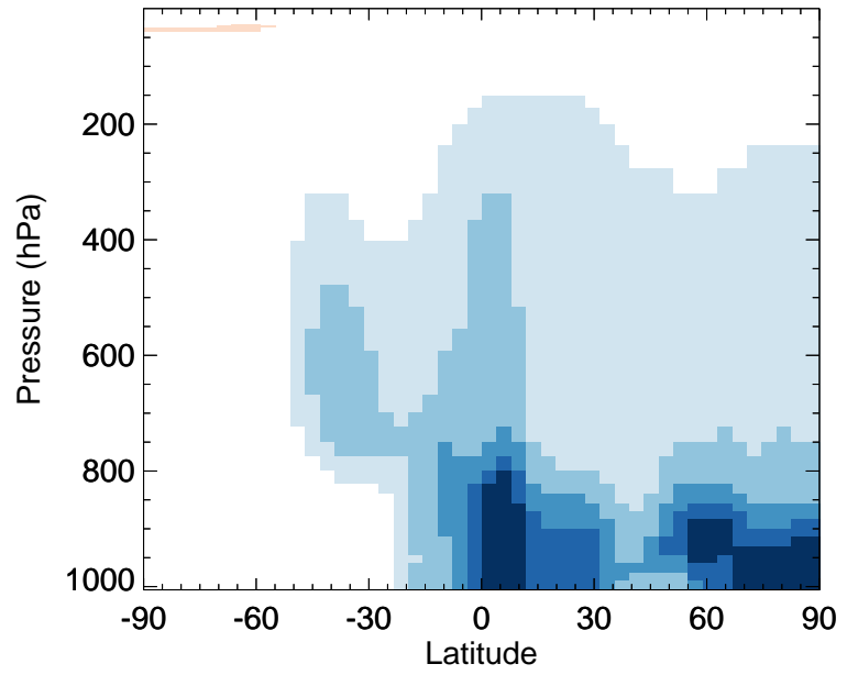
v11-02a / v11-01-public-Run0 BrCl - Zonal mean % diff for Jul
