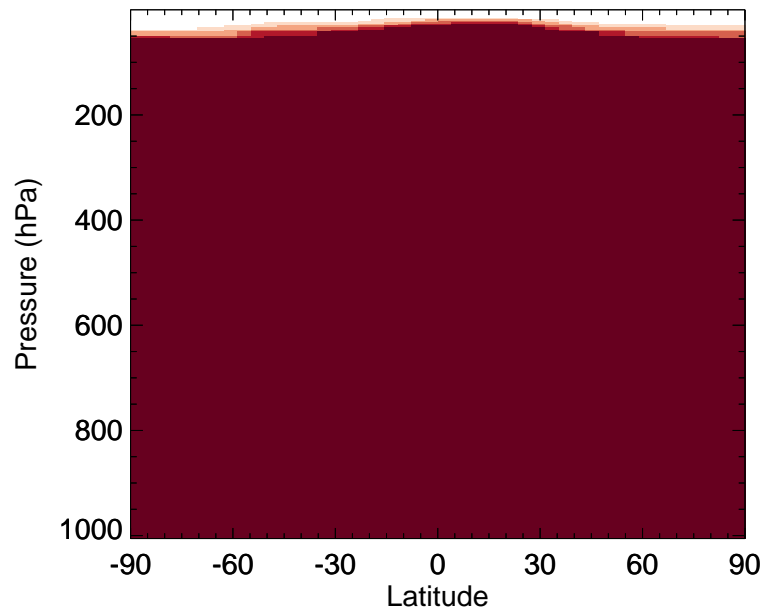
v11-02a / v11-01k-Run0 ASOAN - Zonal mean % diff for Jul
