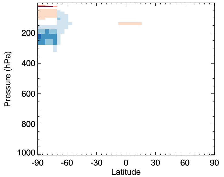
v11-02a / v11-01-public-Run0 HO2 - Zonal mean % diff for Jul
