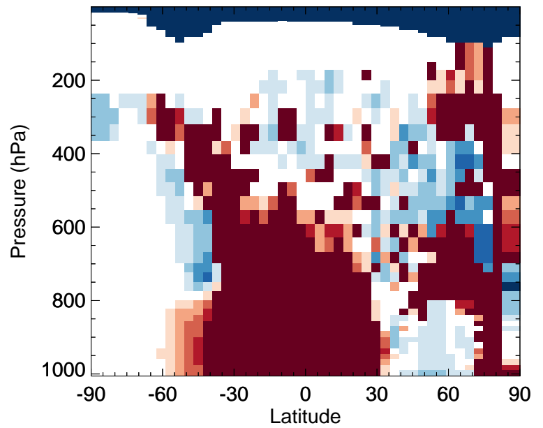
v11-02a / v11-01k-Run0 NIT - Zonal mean % diff for Jul
