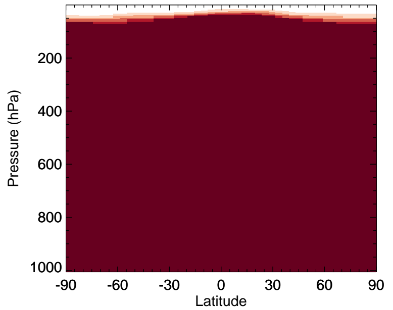
v11-02a / v11-01-public-Run0 ASOG1 - Zonal mean % diff for Jul
