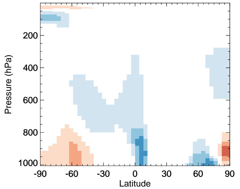
v11-02a / v11-01-public-Run0 BrNO 2 - Zonal mean % diff for Jul
