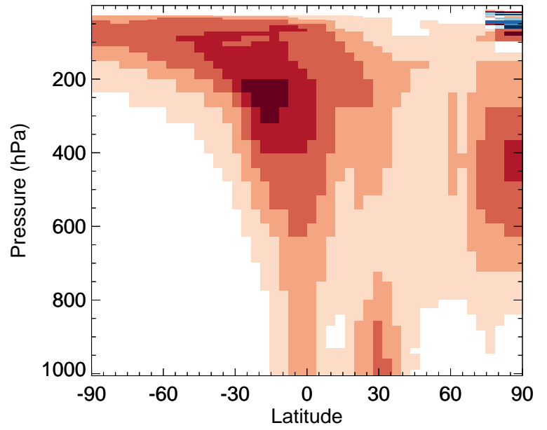
v11-02a / v11-01-public-Run0 GLYC - Zonal mean % diff for Jul
