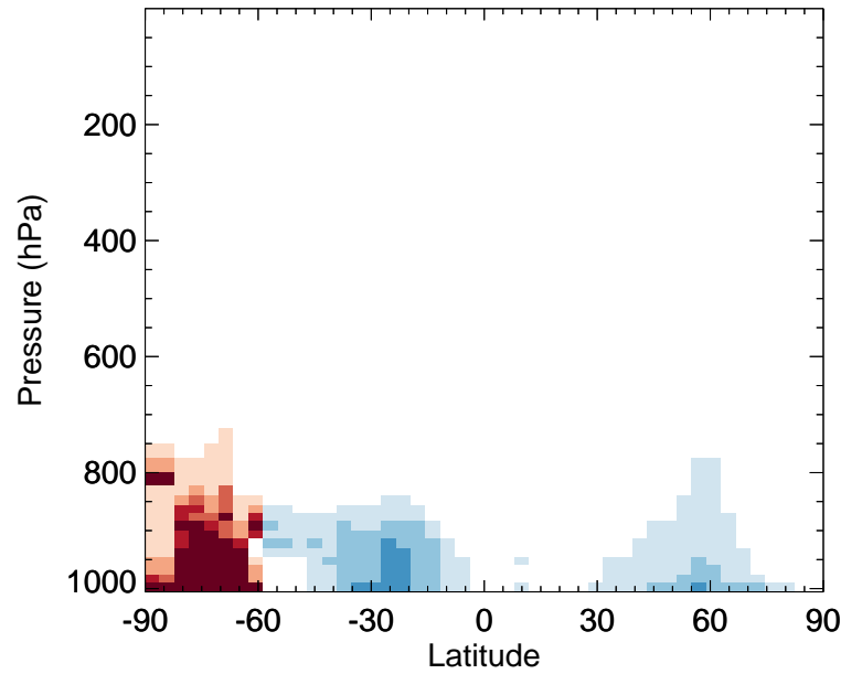
v11-02a / v11-01k-Run0 HNO 3 - Zonal mean % diff for Jul
