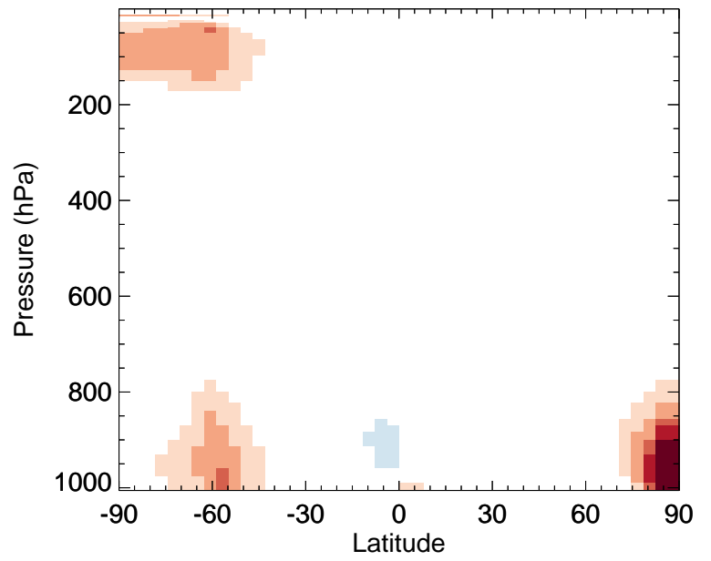
v11-02a / v11-01-public-Run0 MPN - Zonal mean % diff for Jul
