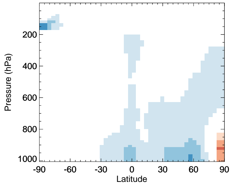
v11-02a / v11-01k-Run0 CINO3 - Zonal mean % diff for Jul
