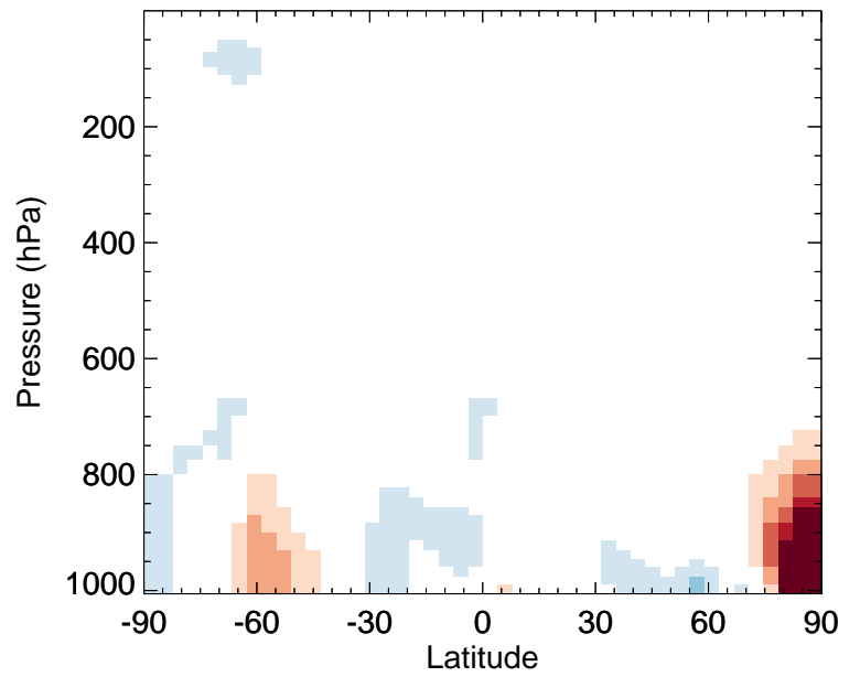
v11-02a / v11-01-public-Run0 HNO 4 - Zonal mean % diff for Jul
