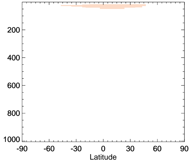
v11-02a / v11-01k-Run0 ACET - Zonal mean % diff for Jul
