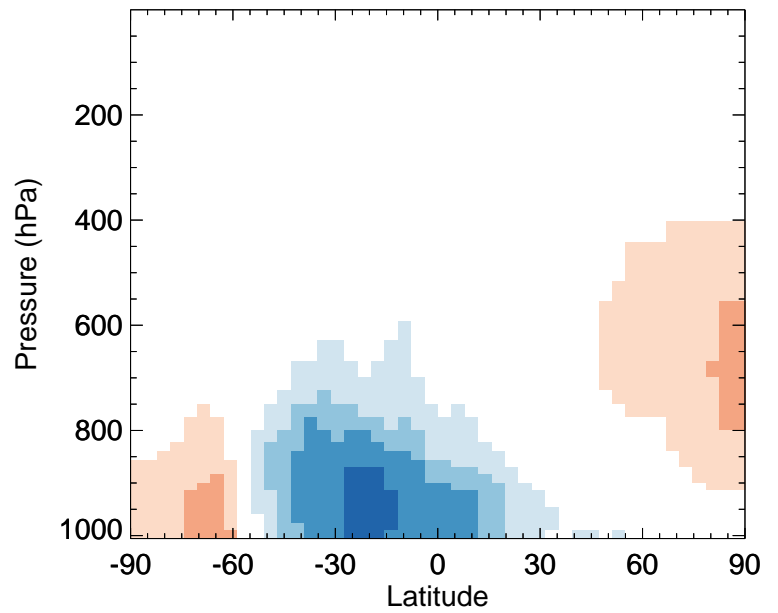
v11-02a / v11-01k-Run0 SO4 - Zonal mean % diff for Jul
