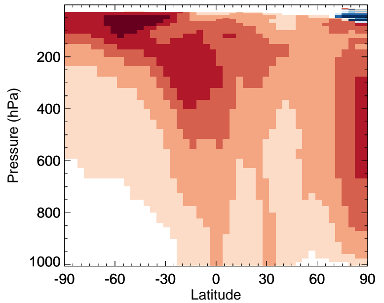
v11-02a / v11-01k-Run0 MVKN - Zonal mean % diff for Jul
