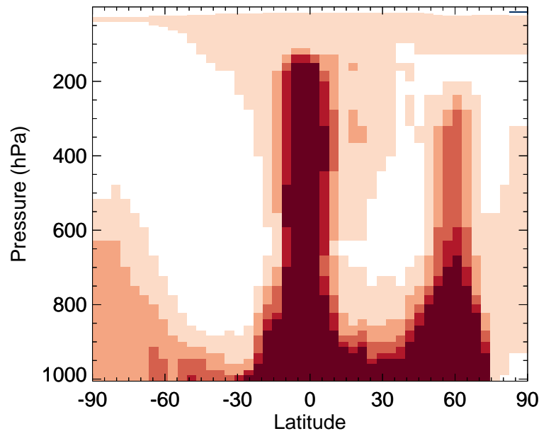
v11-02a / v11-01-public-Run0 RCHO - Zonal mean % diff for Jul
