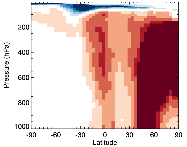
v11-02a / v11-01k-Run0 DMS - Zonal mean % diff for Jul
