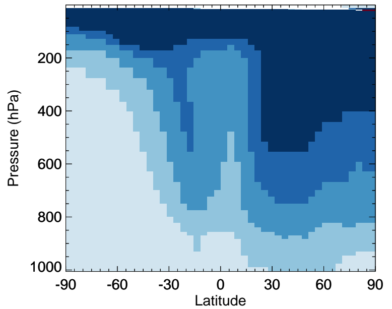
v11-02a / v11-01k-Run0 CHBr3 - Zonal mean % diff for Jul
