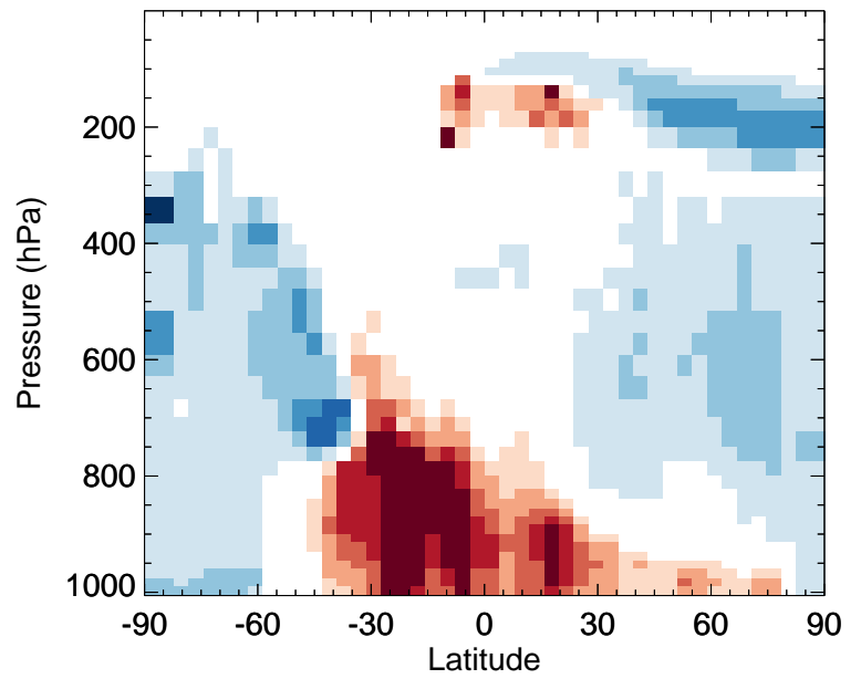
v11-02a / v11-01-public-Run0 NH3 - Zonal mean % diff for Jul
