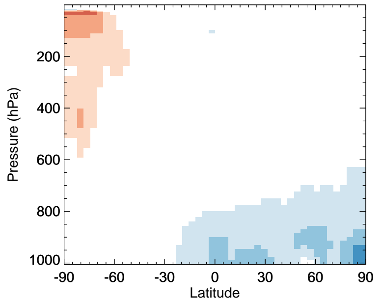
v11-02a / v11-01k-Run0 ClO - Zonal mean % diff for Jul
