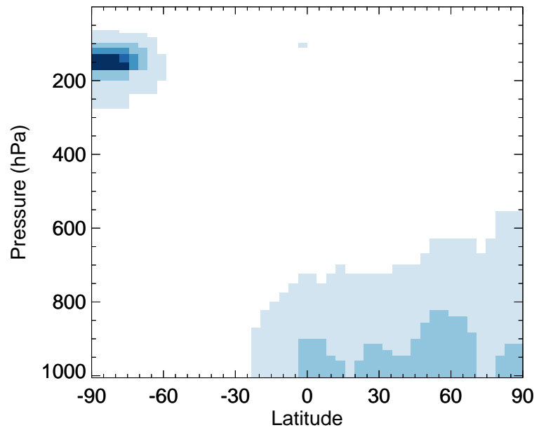
v11-02a / v11-01k-Run0 HOCl - Zonal mean % diff for Jul
