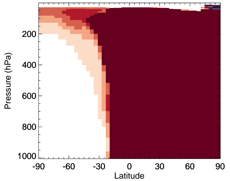
v11-02a / v11-01-public-Run0 XYLE - Zonal mean % diff for Jul
