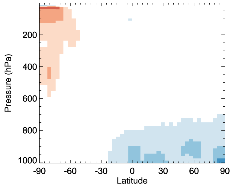
v11-02a / v11-01-public-Run0 ClO - Zonal mean % diff for Jul
