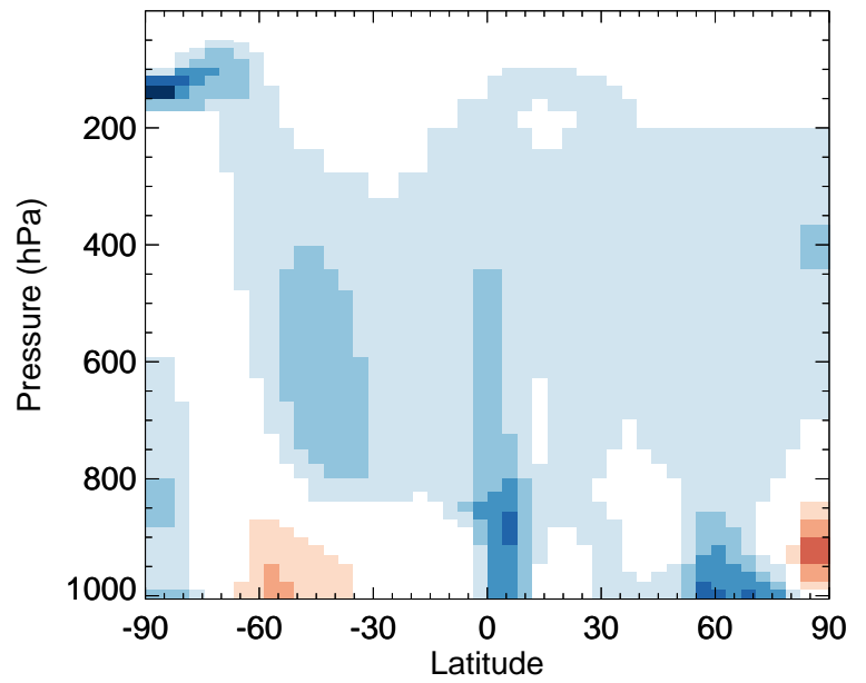
v11-02a / v11-01-public-Run0 BrNO3 - Zonal mean % diff for Jul
