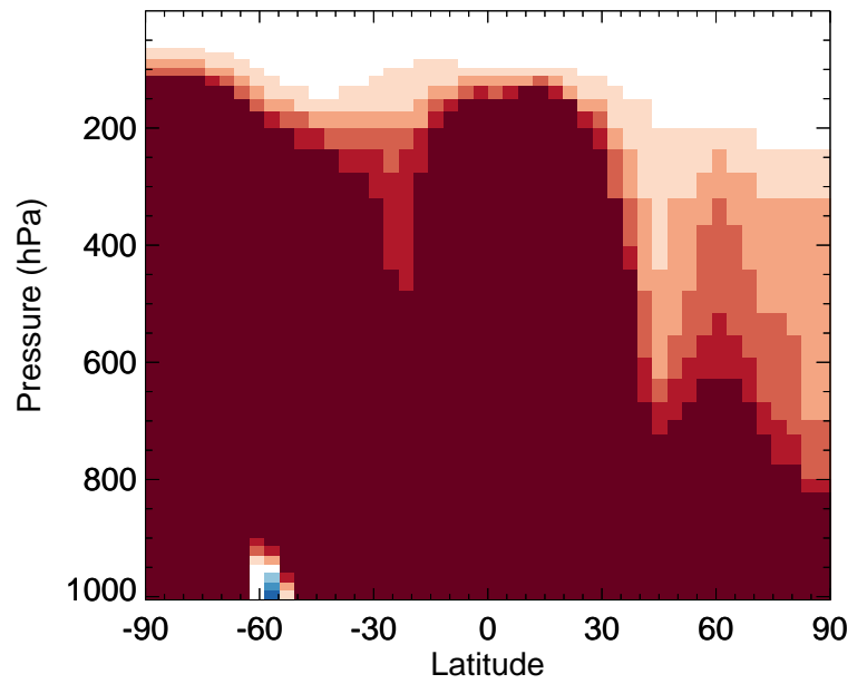
v11-02a / v11-01-public-Run0 ALD2 - Zonal mean % diff for Jul
