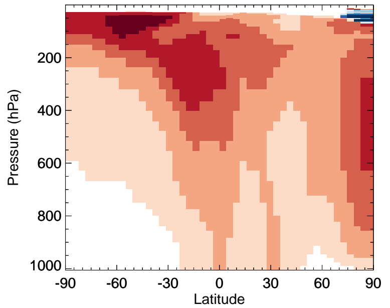
v11-02a / v11-01-public-Run0 MVKN - Zonal mean % diff for Jul
