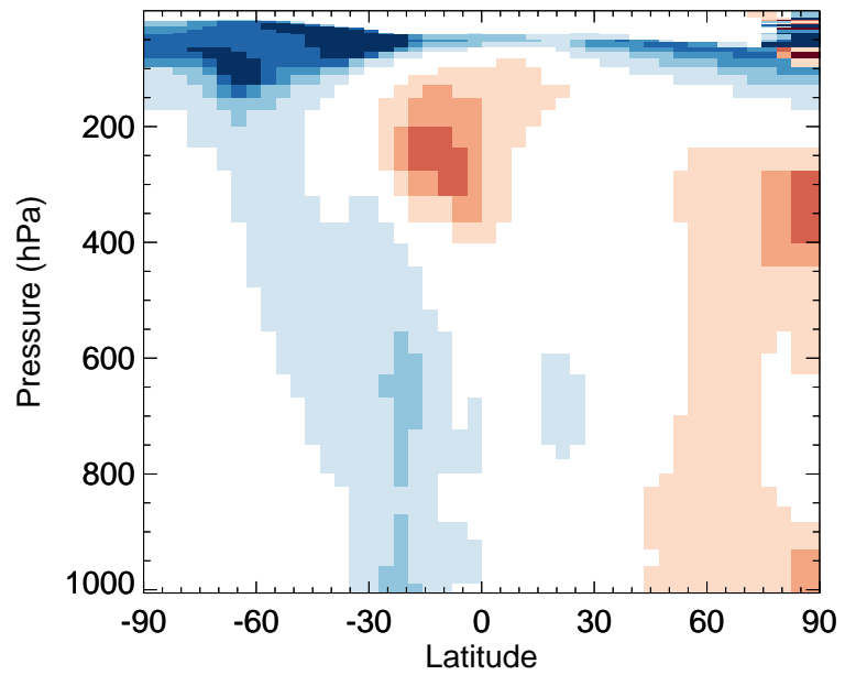
v11-02a / v11-01k-Run0 PMN - Zonal mean % diff for Jul
