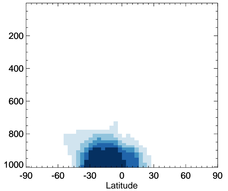
v11-02a / v11-01-public-Run0 NH4 - Zonal mean % diff for Jul
