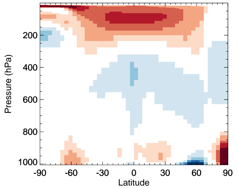
v11-02a / v11-01-public-Run0 NO3 - Zonal mean % diff for Jul
