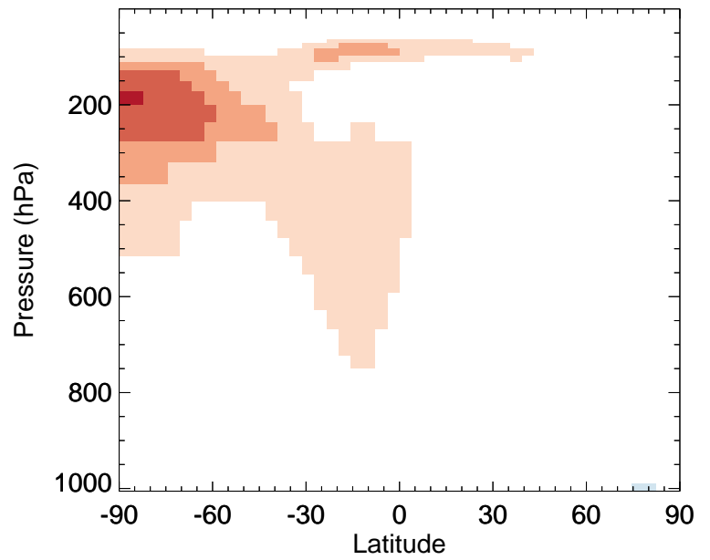
v11-02a / v11-01-public-Run0 ISOG1 - Zonal mean % diff for Jul
