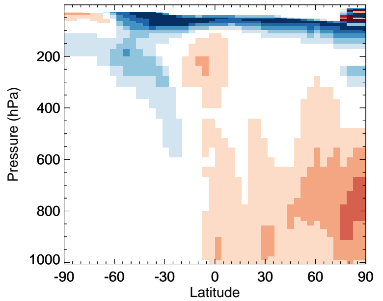
v11-02a / v11-01-public-Run0 MACRN - Zonal mean % diff for Jul
