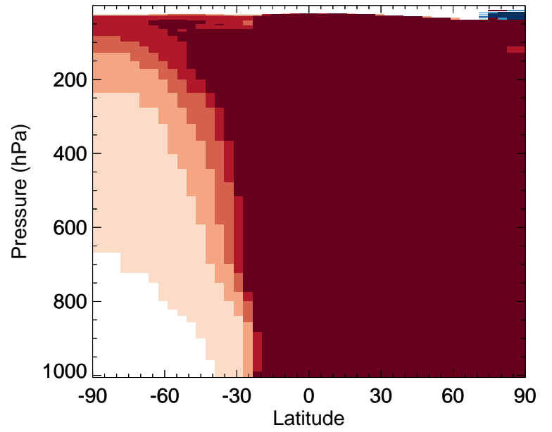
v11-02a / v11-01-public-Run0 TOLU - Zonal mean % diff for Jul
