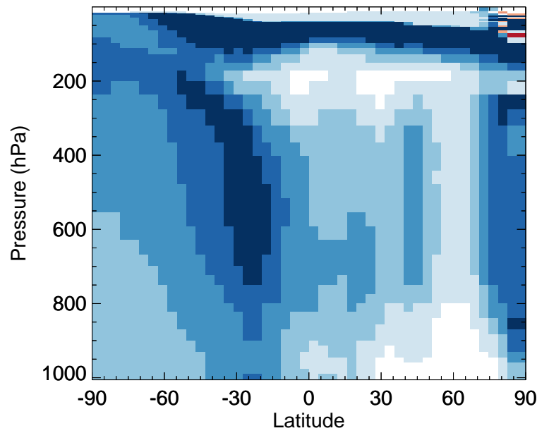
v11-02a / v11-01-public-Run0 MACR - Zonal mean % diff for Jul
