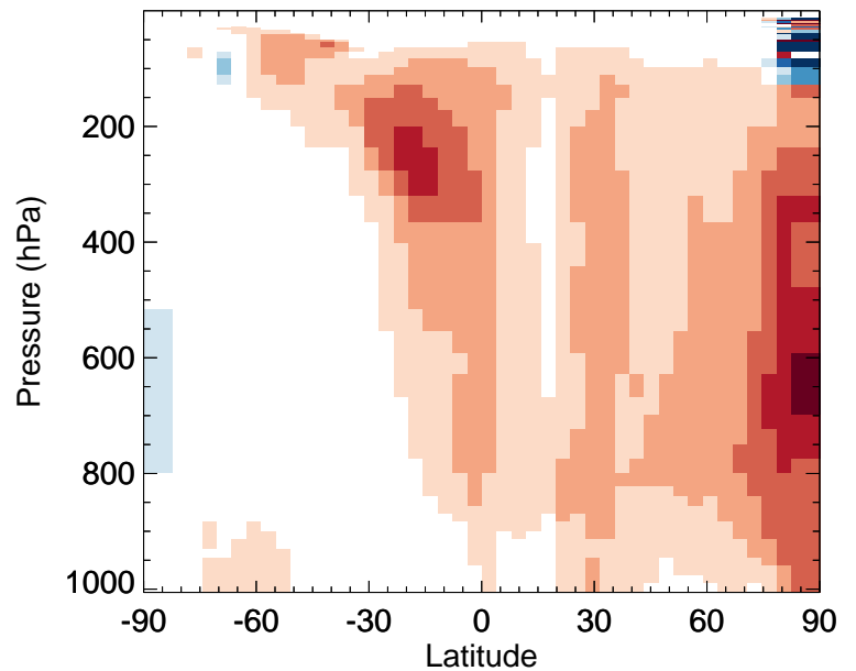
v11-02a / v11-01k-Run0 ISOPNB - Zonal mean % diff for Jul
