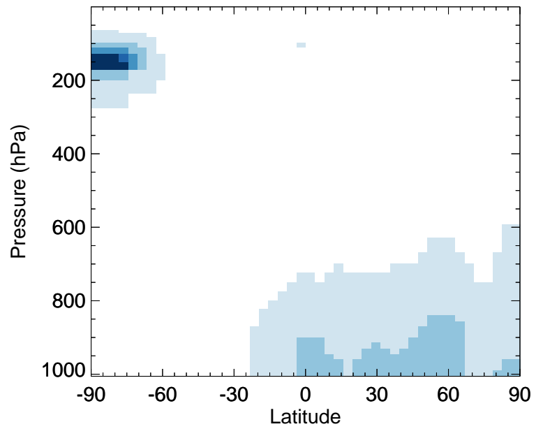
v11-02a / v11-01-public-Run0 HOCl - Zonal mean % diff for Jul
