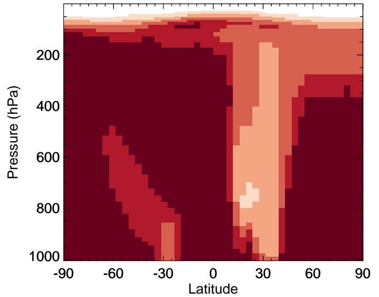
v11-02a / v11-01k-Run0 PPN - Zonal mean % diff for Jul
