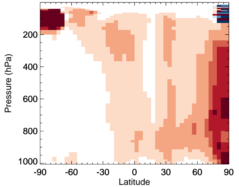
v11-02a / v11-01k-Run0 ISOPND - Zonal mean % diff for Jul
