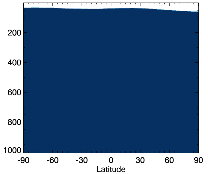
v11-02a / v11-01k-Run0 NITs - Zonal mean % diff for Jul
