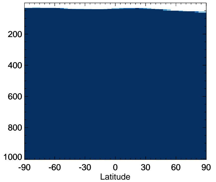
v11-02a / v11-01-public-Run0 NITs - Zonal mean % diff for Jul
