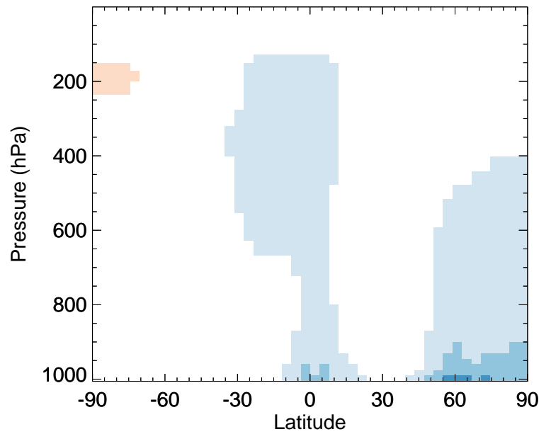
v11-02a / v11-01k-Run0 ISOG2 - Zonal mean % diff for Jul
