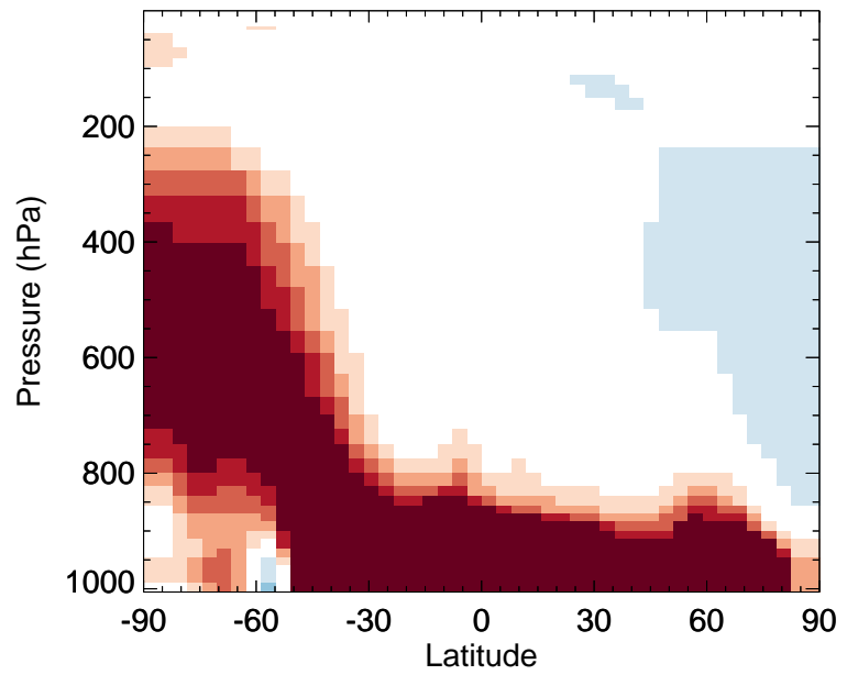
v11-02a / v11-01-public-Run0 HBr - Zonal mean % diff for Jul
