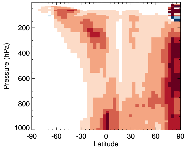
v11-02a / v11-01k-Run0 MOBA - Zonal mean % diff for Jul
