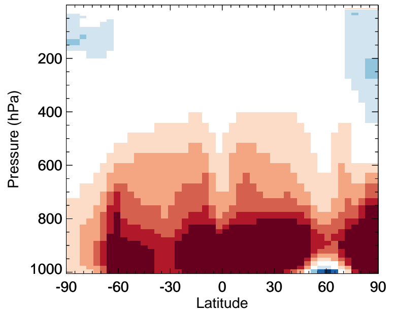
v11-02a / v11-01-public-Run0 N2O5 - Zonal mean % diff for Jul
