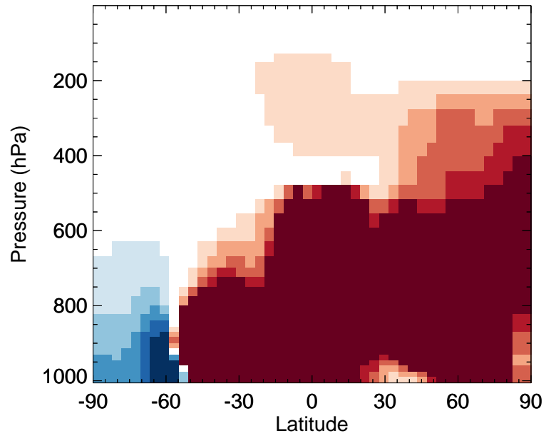
v11-02a / v11-01k-Run0 SO 2 - Zonal mean % diff for Jul
