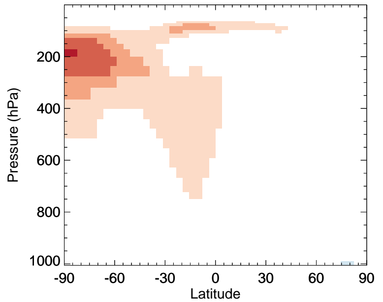
v11-02a / v11-01k-Run0 ISOG1 - Zonal mean % diff for Jul
