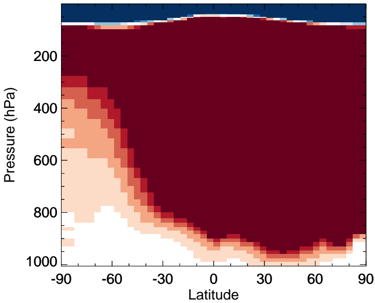
v11-02a - v11-01k-Run0 CH4 - Zonal mean abs diff for Jul
