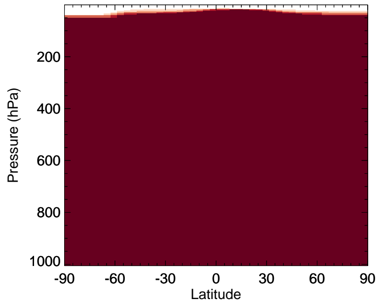
v11-02a / v11-01-public-Run0 ASOG2 - Zonal mean % diff for Jul
