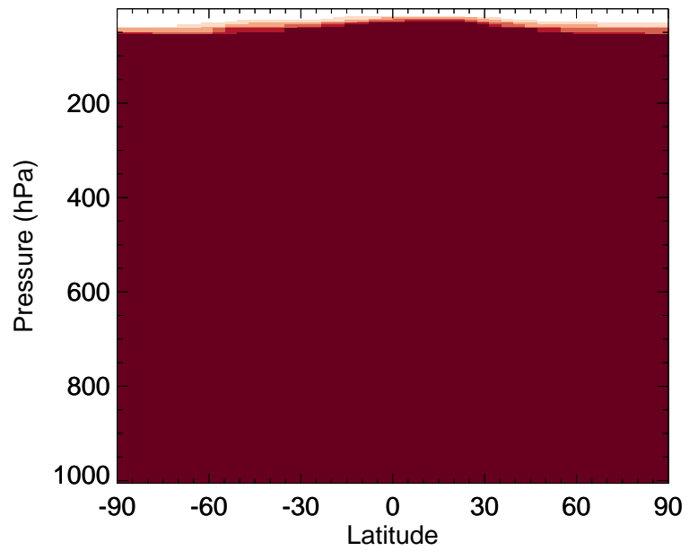
v11-02a / v11-01-public-Run0 ASOAN - Zonal mean % diff for Jul
