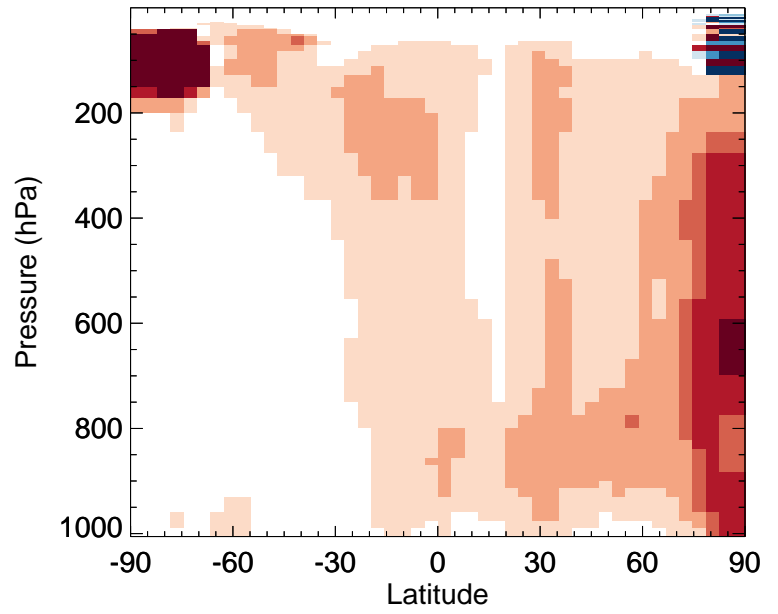
v11-02a / v11-01-public-Run0 ISOPND - Zonal mean % diff for Jul
