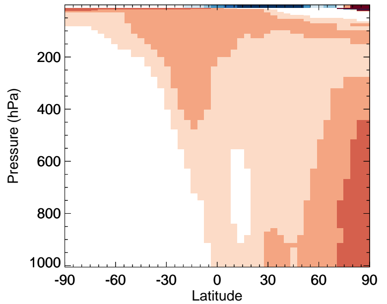
v11-02a / v11-01k-Run0 ALK4 - Zonal mean % diff for Jul
