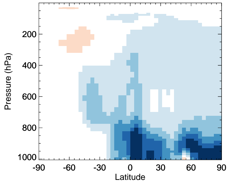
v11-02a / v11-01k-Run0 OCIO - Zonal mean % diff for Jul
