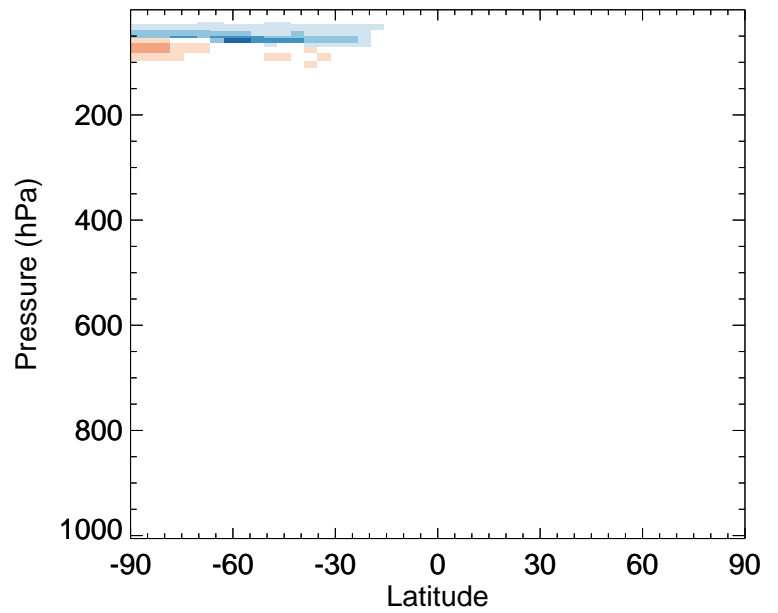
v11-02a / v11-01k-Run0 ClNO 2 - Zonal mean % diff for Jul
