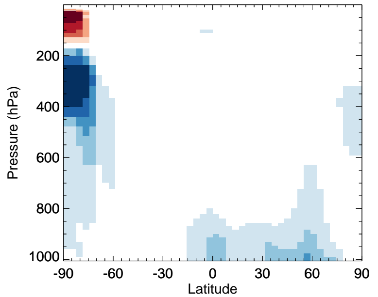
v11-02a / v11-01k-Run0 CIOO - Zonal mean % diff for Jul
