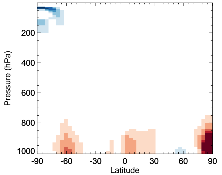
v11-02a / v11-01k-Run0 NO2 - Zonal mean % diff for Jul
