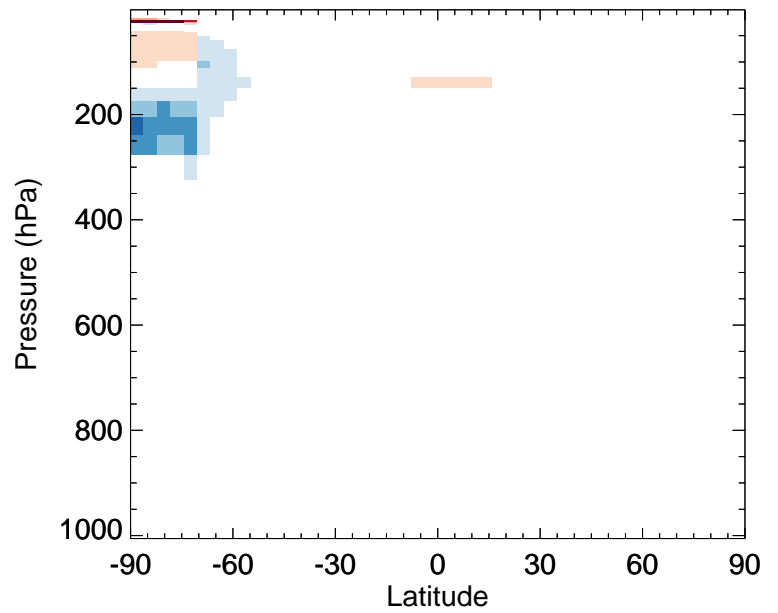
v11-02a / v11-01k-Run0 HO2 - Zonal mean % diff for Jul
