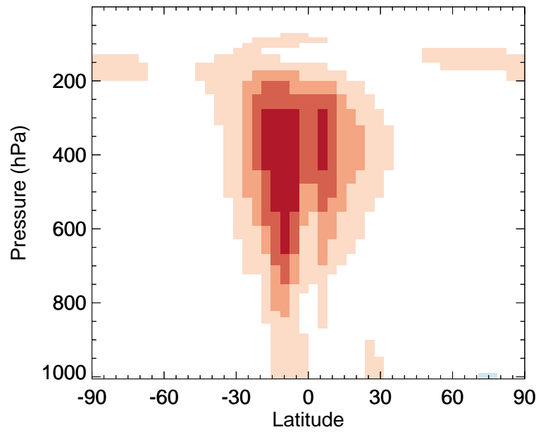
v11-02a / v11-01-public-Run0 ISOA1 - Zonal mean % diff for Jul
