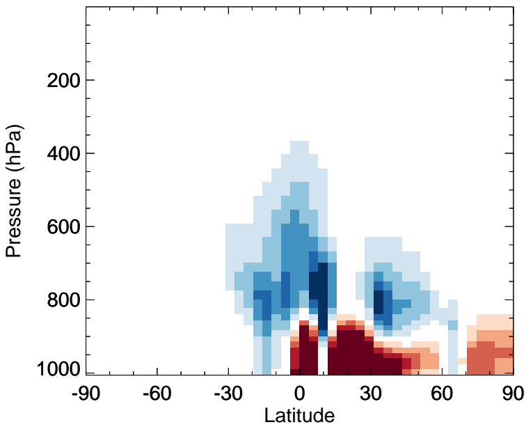
v11-02a - v11-01k-Run0 MAP - Zonal mean abs diff for Jul
