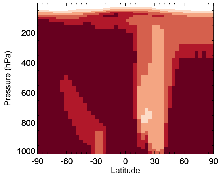
v11-02a / v11-01-public-Run0 PPN - Zonal mean % diff for Jul
