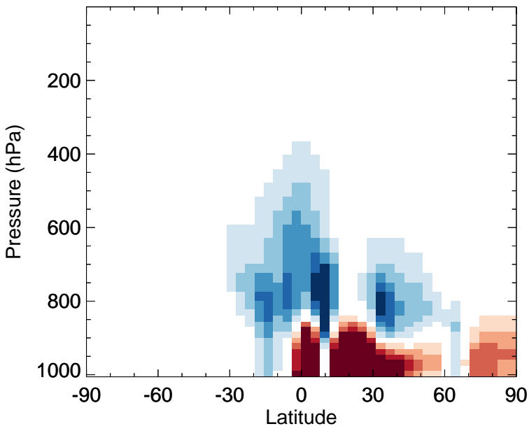
v11-02a - v11-01-public-Run0 MAP - Zonal mean abs diff for Jul
