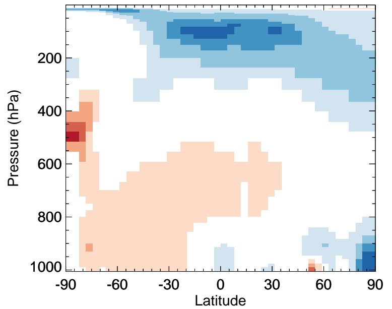
v11-02a / v11-01k-Run0 Cl2O2 - Zonal mean % diff for Jul
