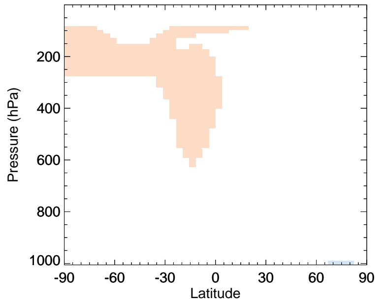
v11-02a / v11-01-public-Run0 ISO3 - Zonal mean % diff for Jul
