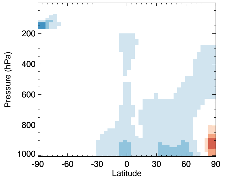
v11-02a / v11-01-public-Run0 CINO3 - Zonal mean % diff for Jul
