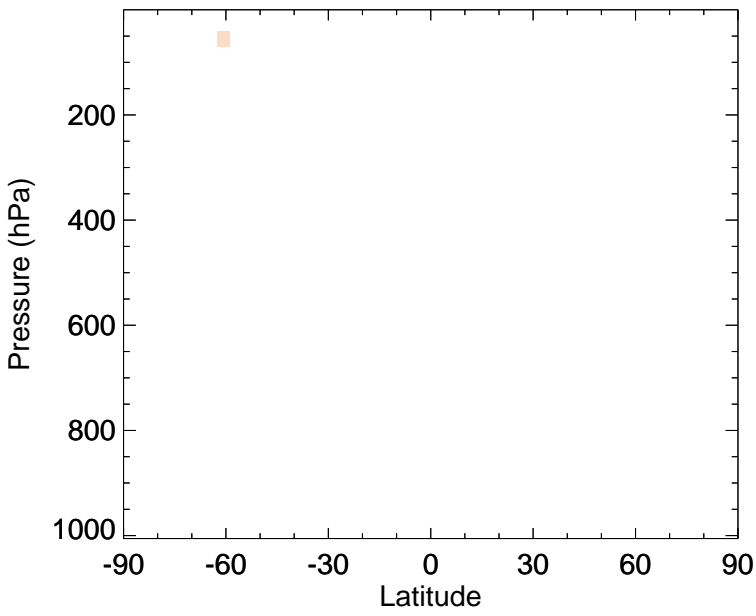
v11-02a - v11-01-public-Run0 MPN - Zonal mean abs diff for Jul
