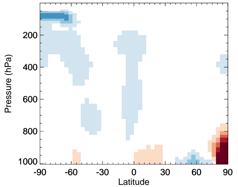
v11-02a / v11-01k-Run0 HNO 2 - Zonal mean % diff for Jul
