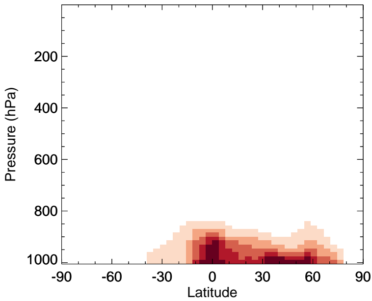
v11-02a - v11-01-public-Run0 ALD2 - Zonal mean abs diff for Jul
