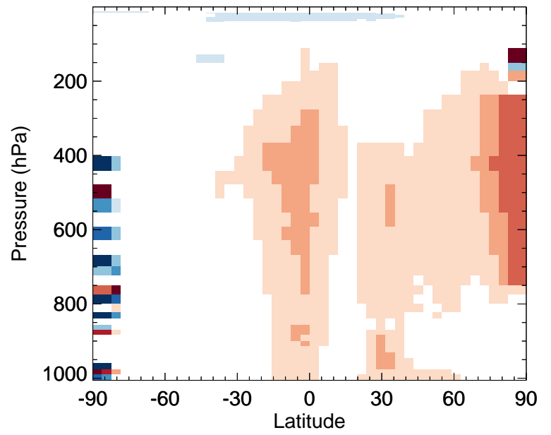
v11-02a / v11-01-public-Run0 MTPO - Zonal mean % diff for Jul
