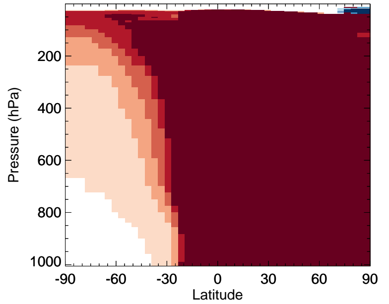
v11-02a / v11-01k-Run0 TOLU - Zonal mean % diff for Jul
