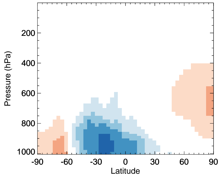
v11-02a / v11-01-public-Run0 SO4 - Zonal mean % diff for Jul
