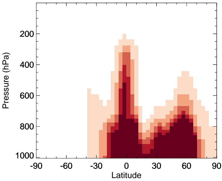
v11-02a - v11-01-public-Run0 MEK - Zonal mean abs diff for Jul
