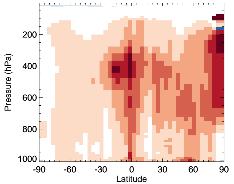
v11-02a / v11-01k-Run0 LIMO - Zonal mean % diff for Jul
