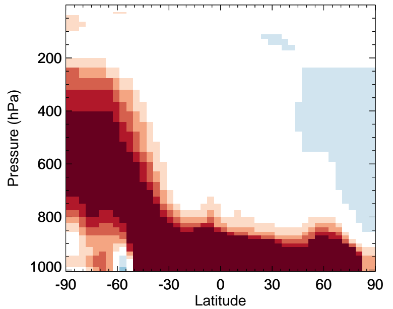
v11-02a / v11-01k-Run0 HBr - Zonal mean % diff for Jul
