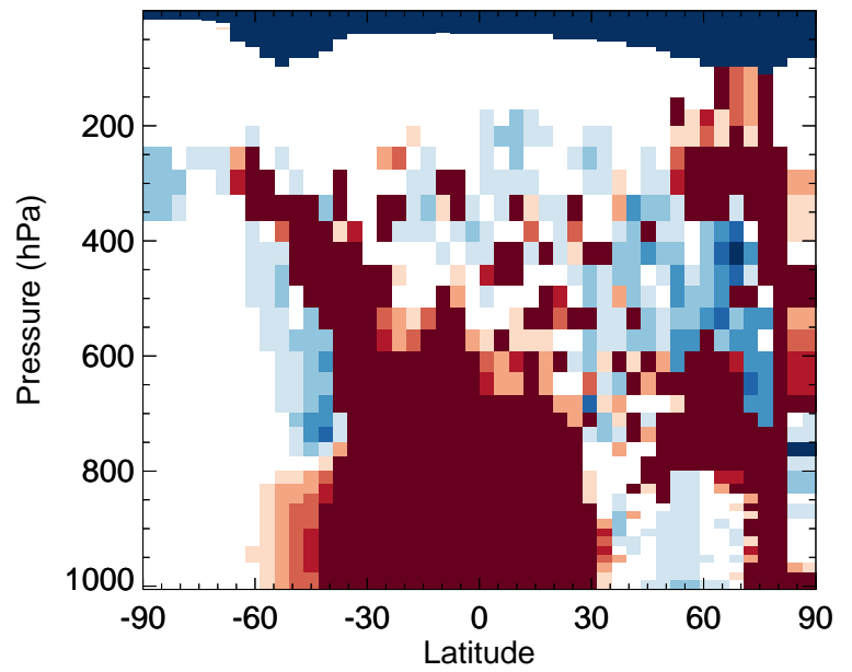
v11-02a / v11-01-public-Run0 NIT - Zonal mean % diff for Jul
