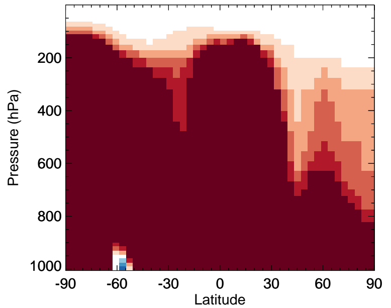
v11-02a / v11-01k-Run0 ALD2 - Zonal mean % diff for Jul
