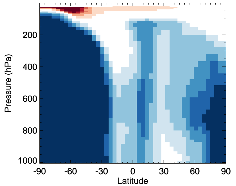
v11-02a / v11-01k-Run0 HAC - Zonal mean % diff for Jul
