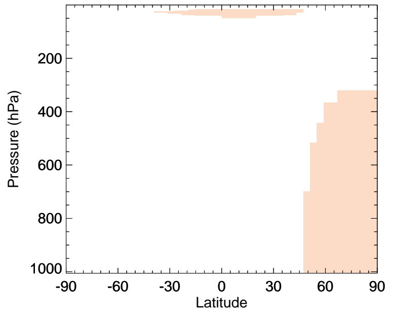
v11-02a / v11-01k-Run0 R4N2 - Zonal mean % diff for Jul
