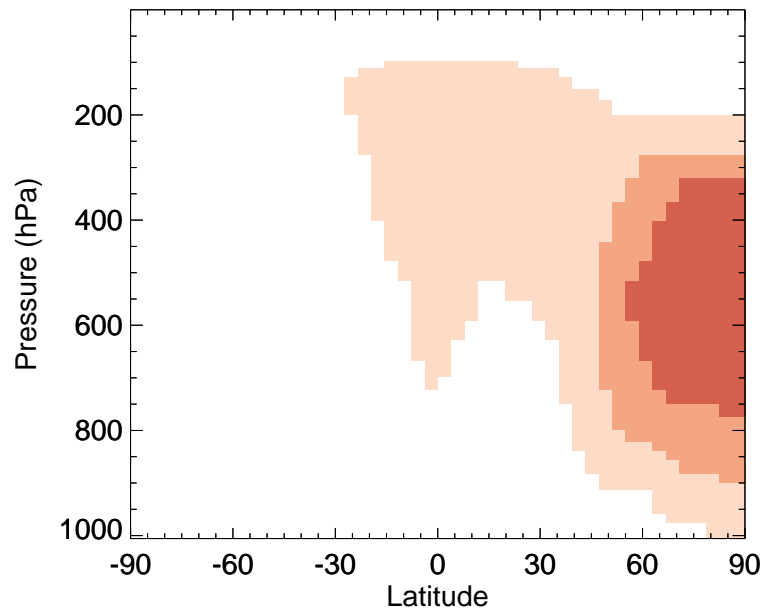
v11-02a / v11-01k-Run0 MSA - Zonal mean % diff for Jul
