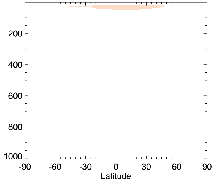
v11-02a / v11-01-public-Run0 ACET - Zonal mean % diff for Jul
