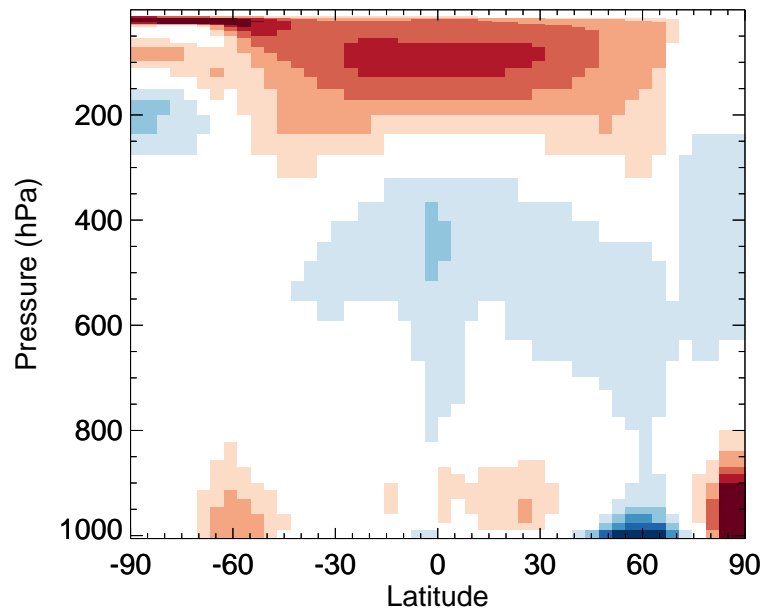
v11-02a / v11-01k-Run0 NO3 - Zonal mean % diff for Jul
