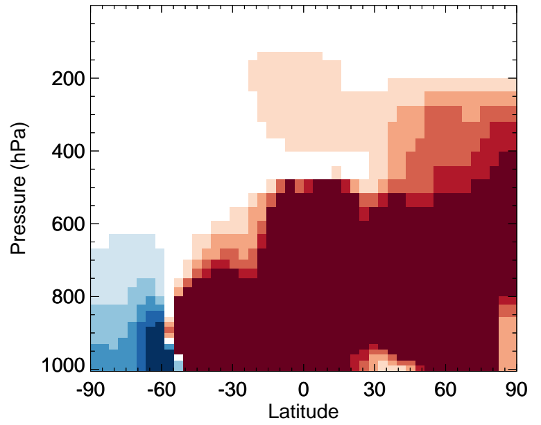
v11-02a / v11-01-public-Run0 SO 2 - Zonal mean % diff for Jul
