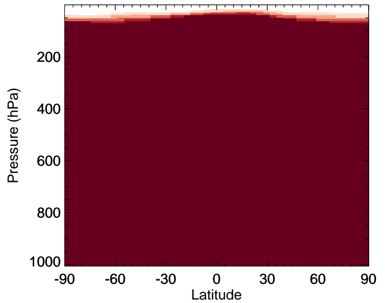
v11-02a / v11-01k-Run0 ASOG1 - Zonal mean % diff for Jul
