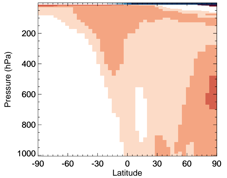
v11-02a / v11-01-public-Run0 ALK4 - Zonal mean % diff for Jul
