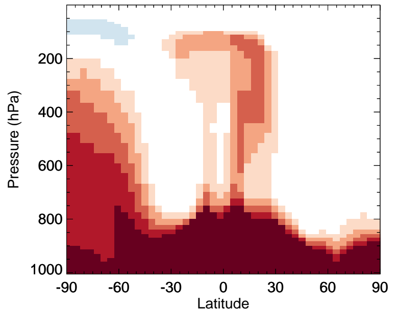
v11-02a / v11-01k-Run0 MAP - Zonal mean % diff for Jul
