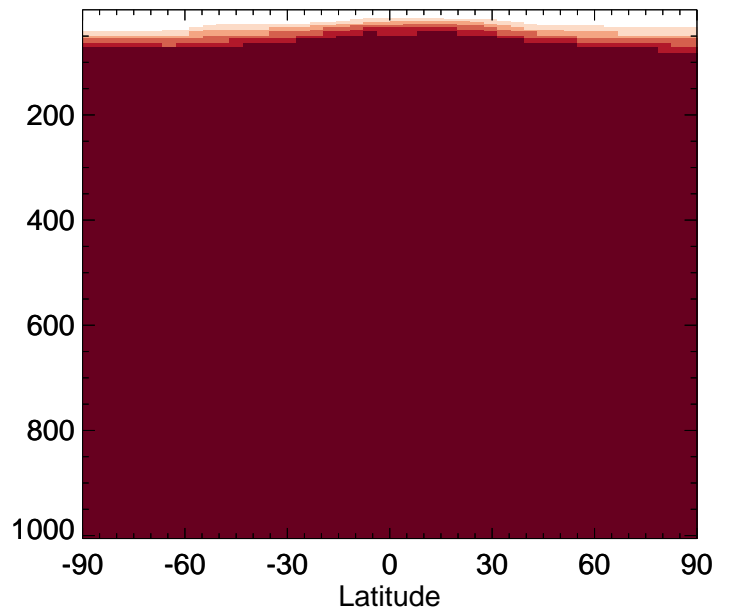
v11-02a / v11-01-public-Run0 ASOG3 - Zonal mean % diff for Jul
