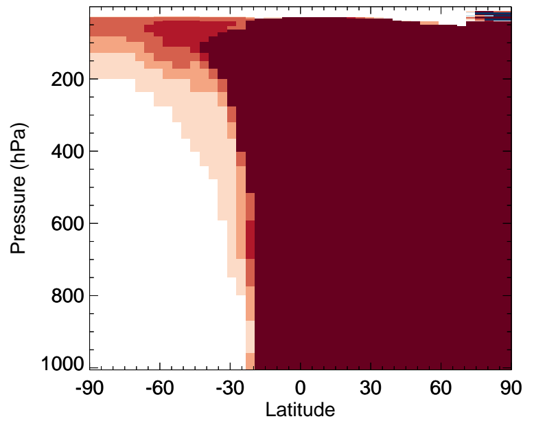
v11-02a / v11-01k-Run0 XYLE - Zonal mean % diff for Jul
