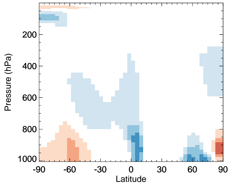
v11-02a / v11-01k-Run0 BrNO 2 - Zonal mean % diff for Jul
