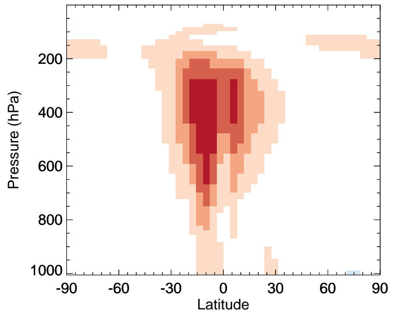
v11-02a / v11-01k-Run0 ISOA1 - Zonal mean % diff for Jul
