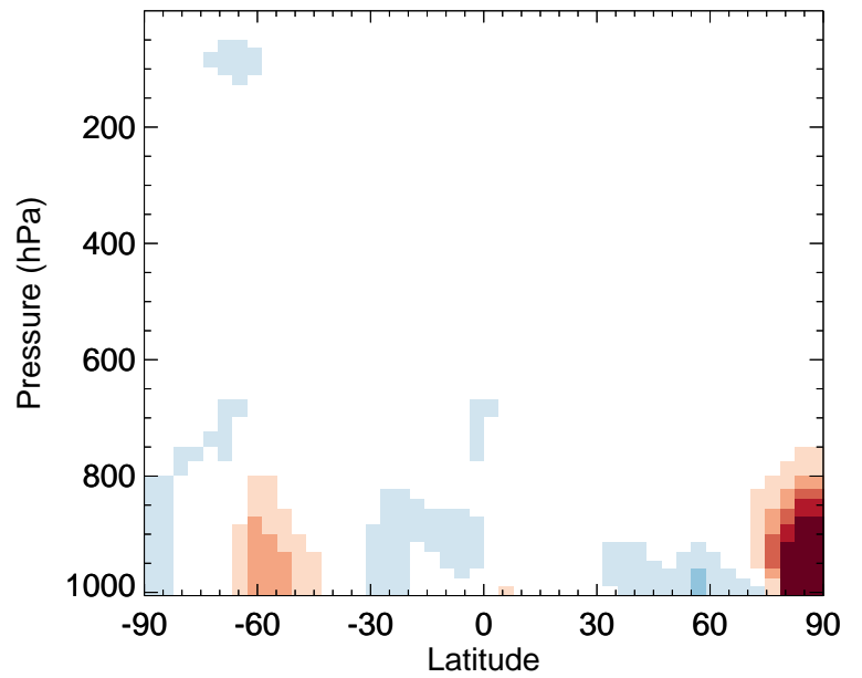
v11-02a / v11-01k-Run0 HNO 4 - Zonal mean % diff for Jul
