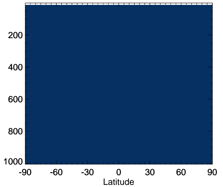
v11-02a / v11-01k-Run0 SO4s - Zonal mean % diff for Jul
