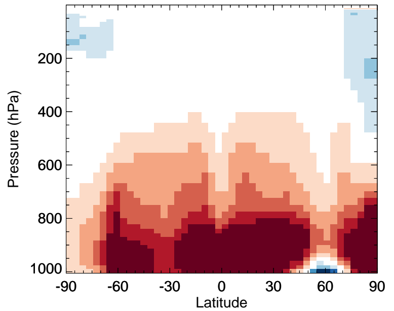
v11-02a / v11-01k-Run0 N2O5 - Zonal mean % diff for Jul
