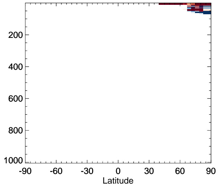
v11-02a / v11-01-public-Run0 BCPO - Zonal mean % diff for Jul
