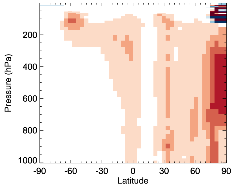
v11-02a / v11-01-public-Run0 ISOP - Zonal mean % diff for Jul
