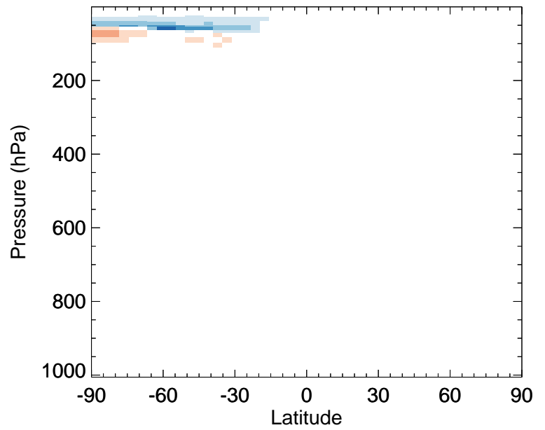
v11-02a / v11-01-public-Run0 ClNO 2 - Zonal mean % diff for Jul
