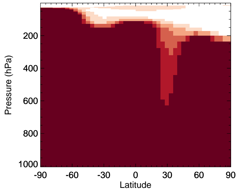
v11-02a / v11-01-public-Run0 MEK - Zonal mean % diff for Jul
