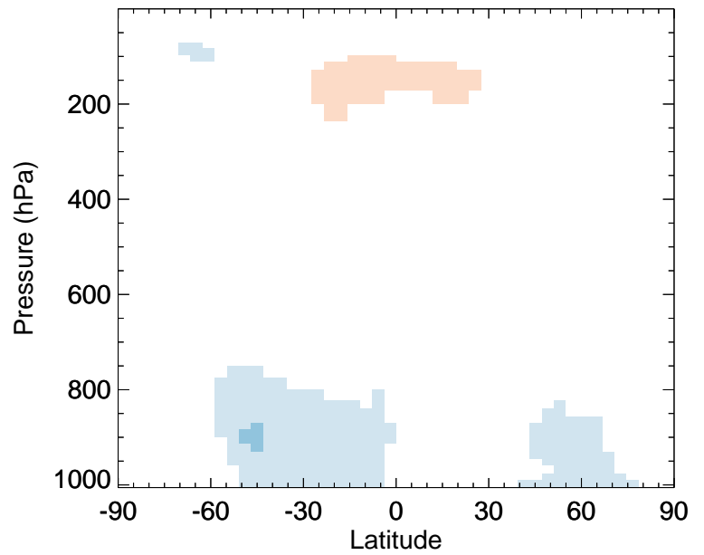
v11-02a / v11-01k-Run0 H2O2 - Zonal mean % diff for Jul
