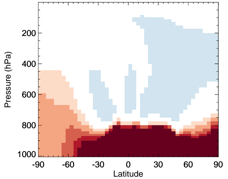
v11-02a / v11-01-public-Run0 PAN - Zonal mean % diff for Jul
