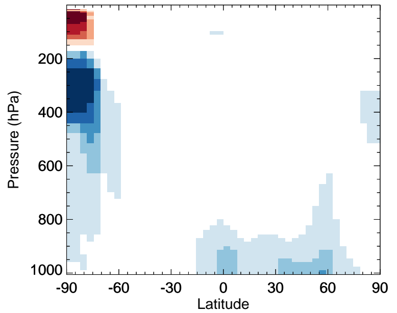
v11-02a / v11-01-public-Run0 CIOO - Zonal mean % diff for Jul
