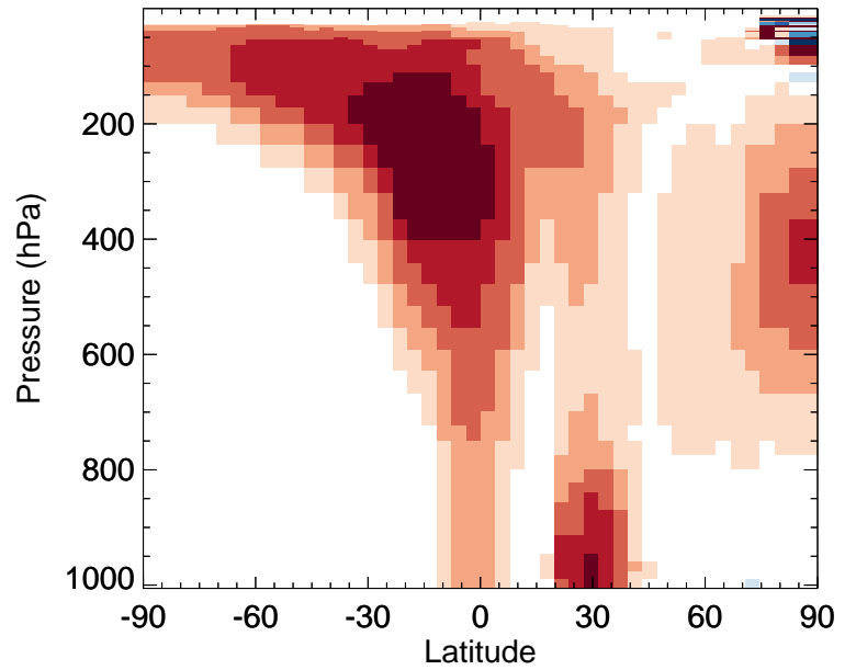
v11-02a / v11-01k-Run0 IEPOX - Zonal mean % diff for Jul
