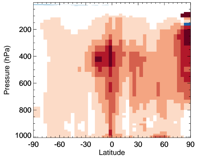
v11-02a / v11-01-public-Run0 LIMO - Zonal mean % diff for Jul
