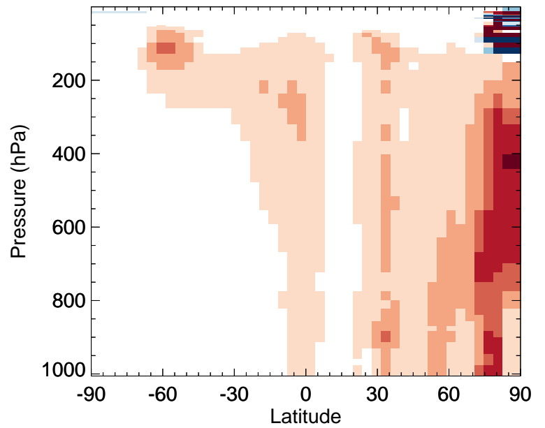
v11-02a / v11-01k-Run0 ISOP - Zonal mean % diff for Jul
