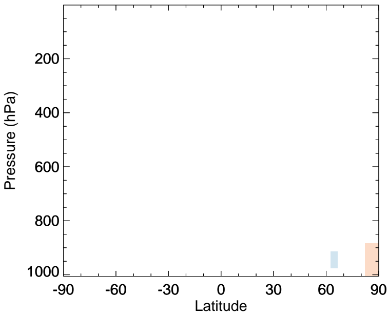
v11-02a - v11-01-public-Run0 HO2 - Zonal mean abs diff for Jul
