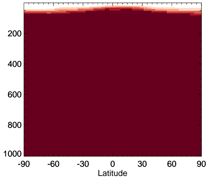
v11-02a / v11-01k-Run0 ASOG3 - Zonal mean % diff for Jul
