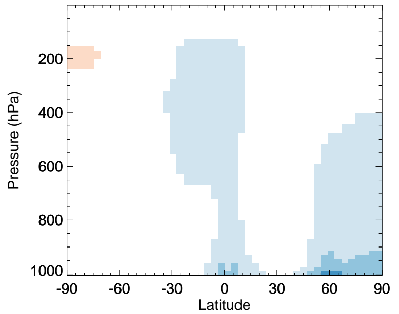
v11-02a / v11-01-public-Run0 ISOG2 - Zonal mean % diff for Jul
