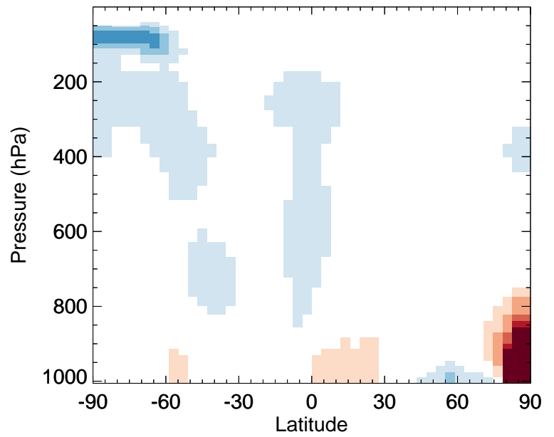
v11-02a / v11-01-public-Run0 HNO 2 - Zonal mean % diff for Jul
