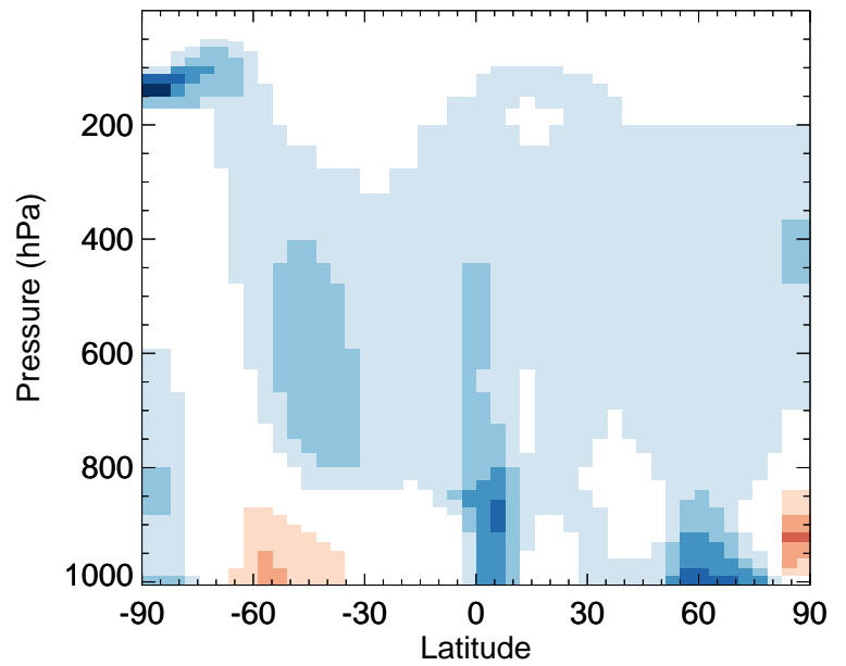
v11-02a / v11-01k-Run0 BrNO3 - Zonal mean % diff for Jul
