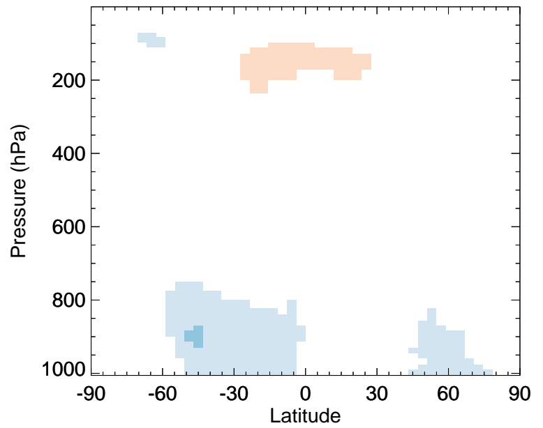
v11-02a / v11-01-public-Run0 H2O2 - Zonal mean % diff for Jul
