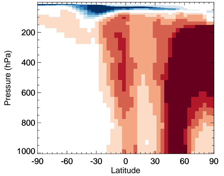
v11-02a / v11-01-public-Run0 DMS - Zonal mean % diff for Jul
