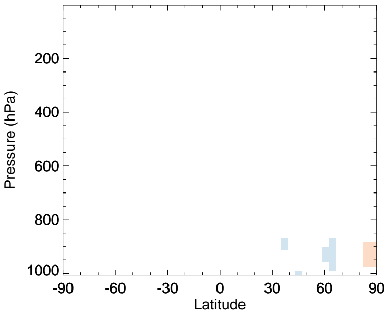
v11-02a - v11-01k-Run0 HO2 - Zonal mean abs diff for Jul
