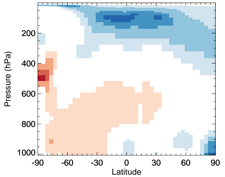
v11-02a / v11-01-public-Run0 Cl2O2 - Zonal mean % diff for Jul
