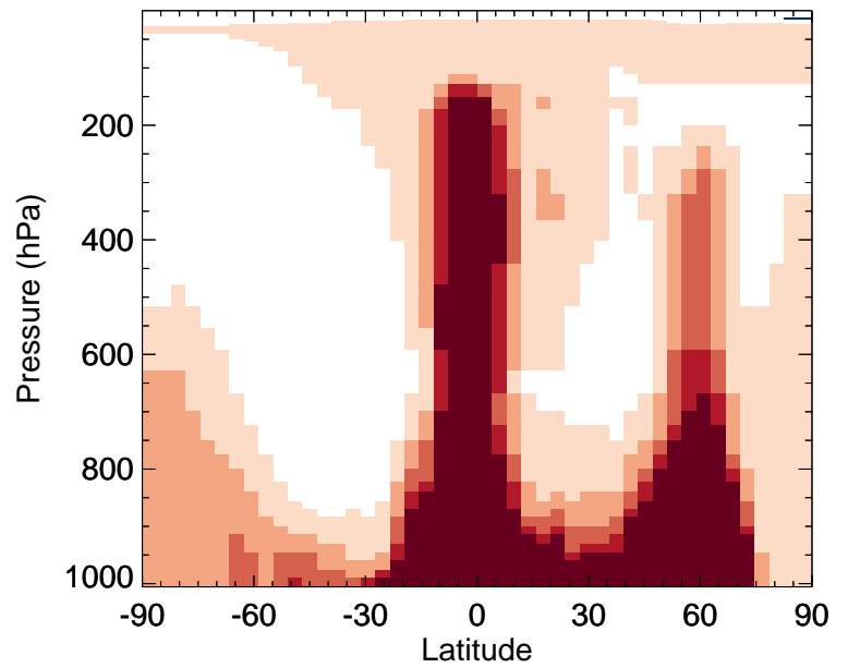
v11-02a / v11-01k-Run0 RCHO - Zonal mean % diff for Jul
