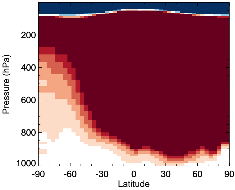
v11-02a - v11-01-public-Run0 CH4 - Zonal mean abs diff for Jul
