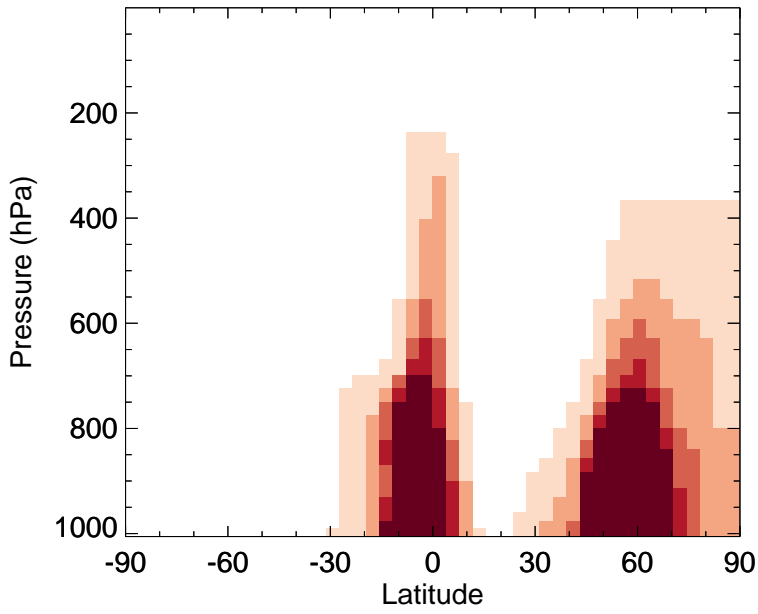
v11-02a - v11-01-public-Run0 BENZ - Zonal mean abs diff for Jul
