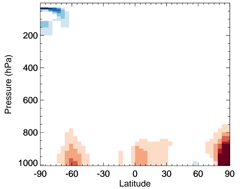
v11-02a / v11-01-public-Run0 NO2 - Zonal mean % diff for Jul
