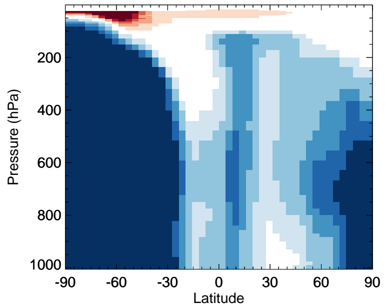
v11-02a / v11-01-public-Run0 HAC - Zonal mean % diff for Jul
