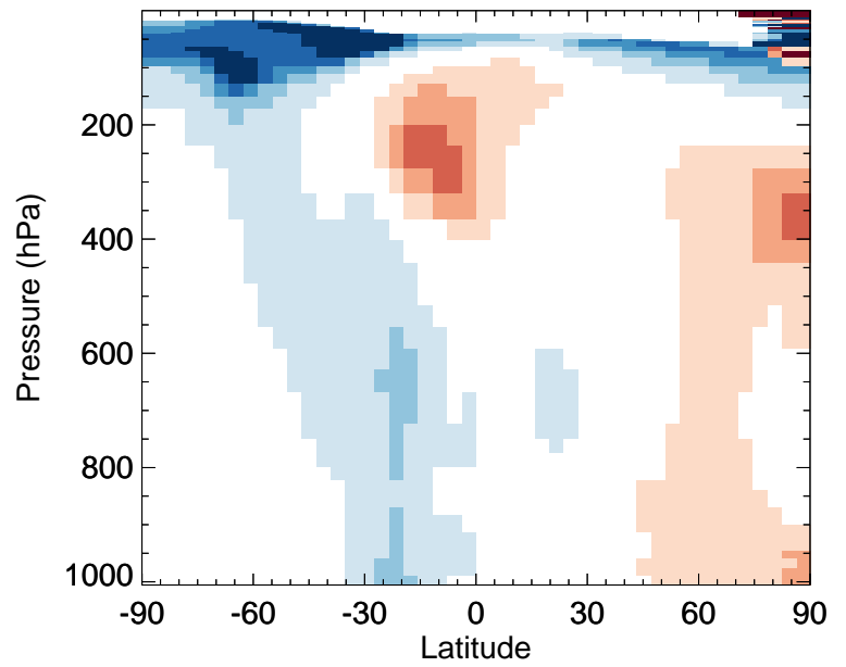
v11-02a / v11-01-public-Run0 PMN - Zonal mean % diff for Jul
