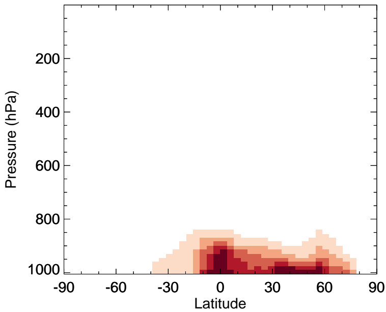
v11-02a - v11-01k-Run0 ALD2 - Zonal mean abs diff for Jul
