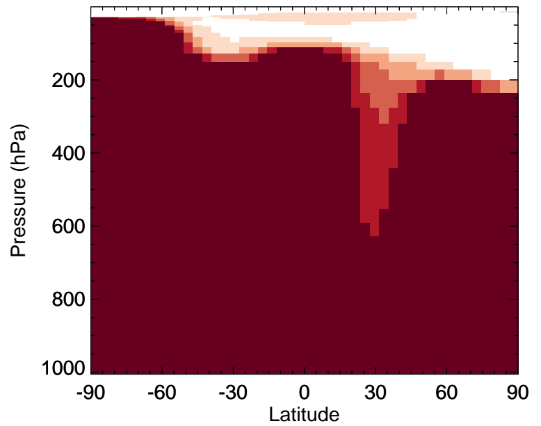
v11-02a / v11-01k-Run0 MEK - Zonal mean % diff for Jul
