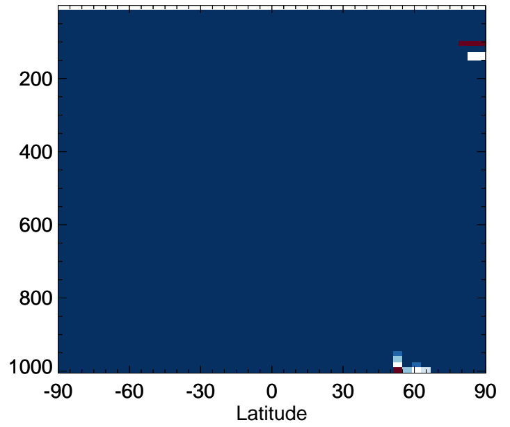
v11-02a / v11-01-public-Run0 MTPA - Zonal mean % diff for Jul
