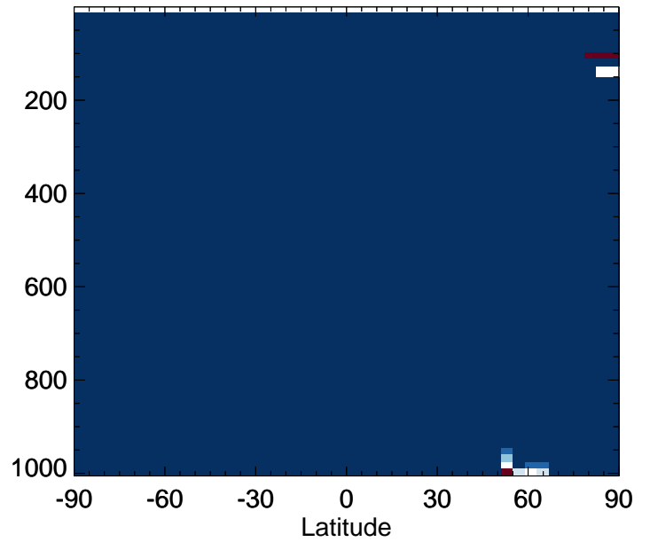
v11-02a / v11-01k-Run0 MTPA - Zonal mean % diff for Jul
