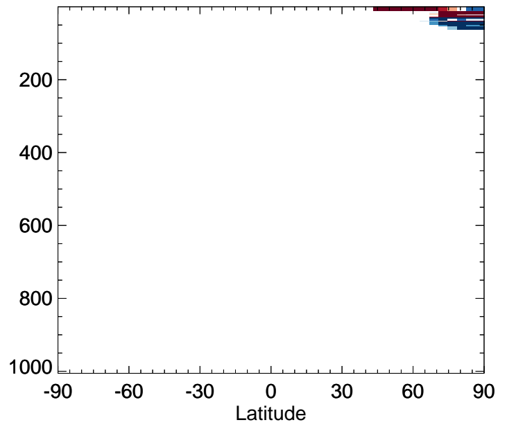
v11-02a / v11-01-public-Run0 OCPO - Zonal mean % diff for Jul
