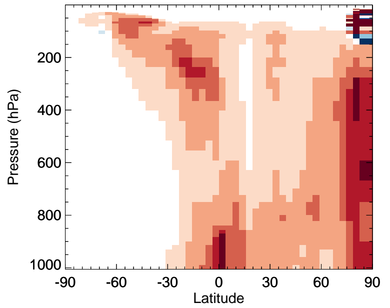
v11-02a / v11-01-public-Run0 MOBA - Zonal mean % diff for Jul
