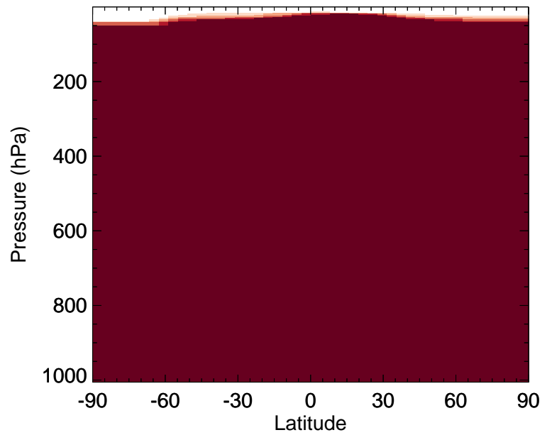
v11-02a / v11-01k-Run0 ASOG2 - Zonal mean % diff for Jul
