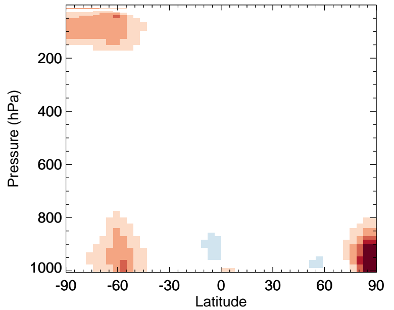
v11-02a / v11-01k-Run0 MPN - Zonal mean % diff for Jul
