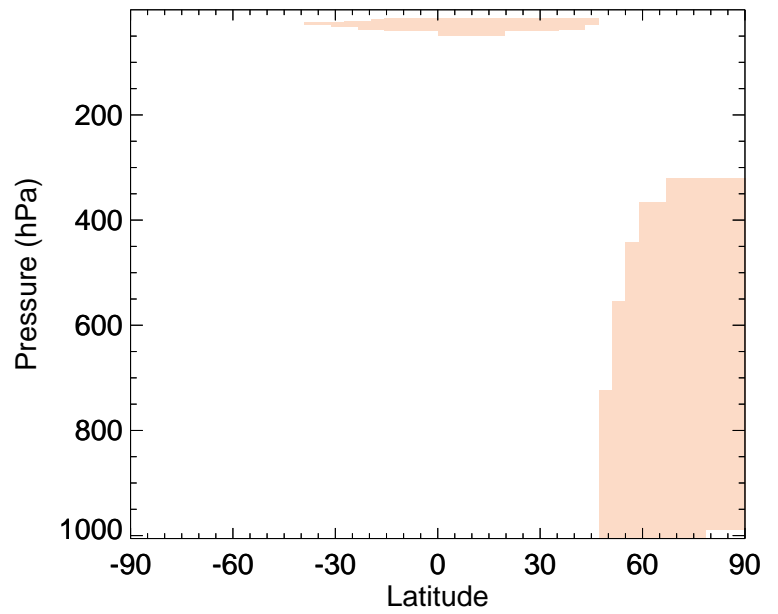
v11-02a / v11-01-public-Run0 R4N2 - Zonal mean % diff for Jul
