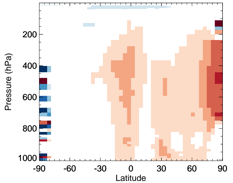
v11-02a / v11-01k-Run0 MTPO - Zonal mean % diff for Jul
