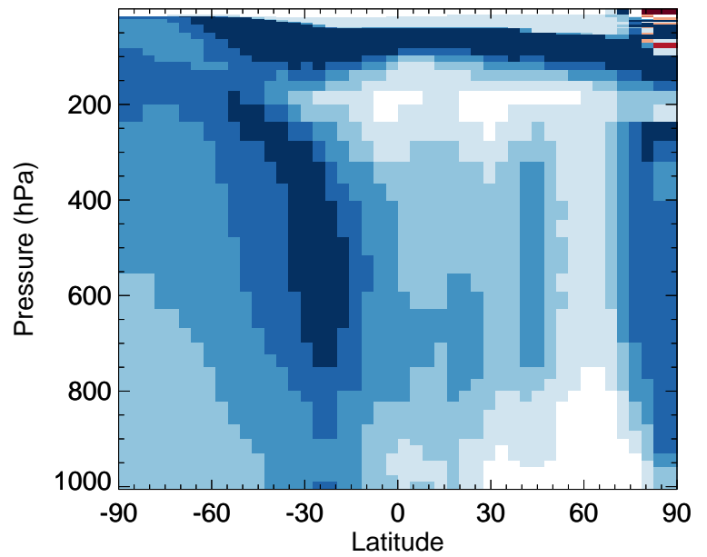
v11-02a / v11-01k-Run0 MACR - Zonal mean % diff for Jul
