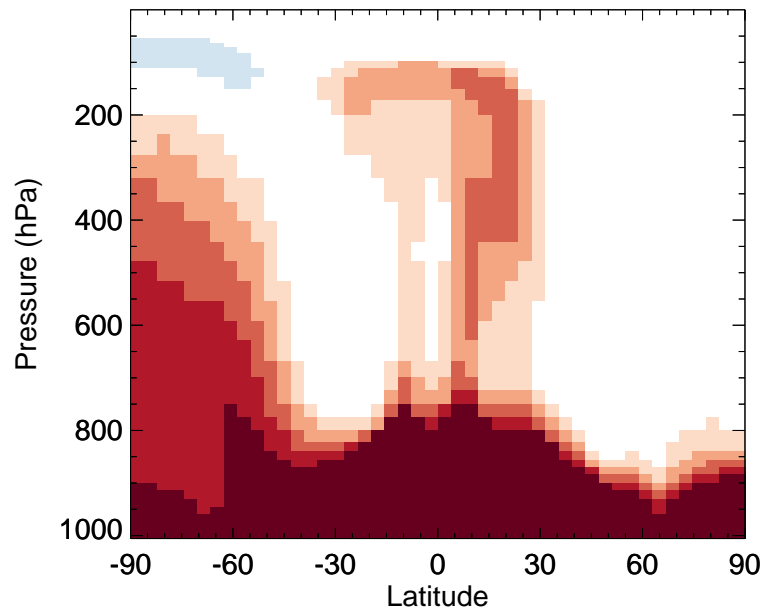
v11-02a / v11-01-public-Run0 MAP - Zonal mean % diff for Jul
