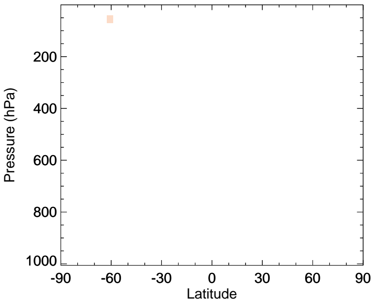
v11-02a - v11-01k-Run0 MPN - Zonal mean abs diff for Jul
