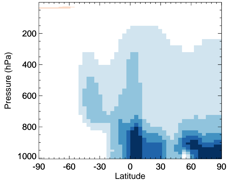
v11-02a / v11-01k-Run0 BrCl - Zonal mean % diff for Jul
