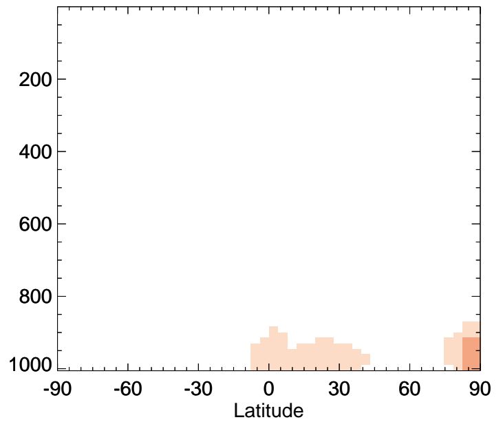
v11-02a / v11-01k-Run0 CH 2 O - Zonal mean % diff for Jul
