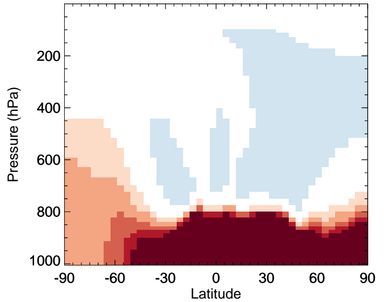
v11-02a / v11-01k-Run0 PAN - Zonal mean % diff for Jul
