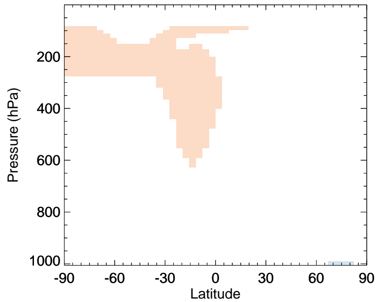
v11-02a / v11-01k-Run0 ISO3 - Zonal mean % diff for Jul
