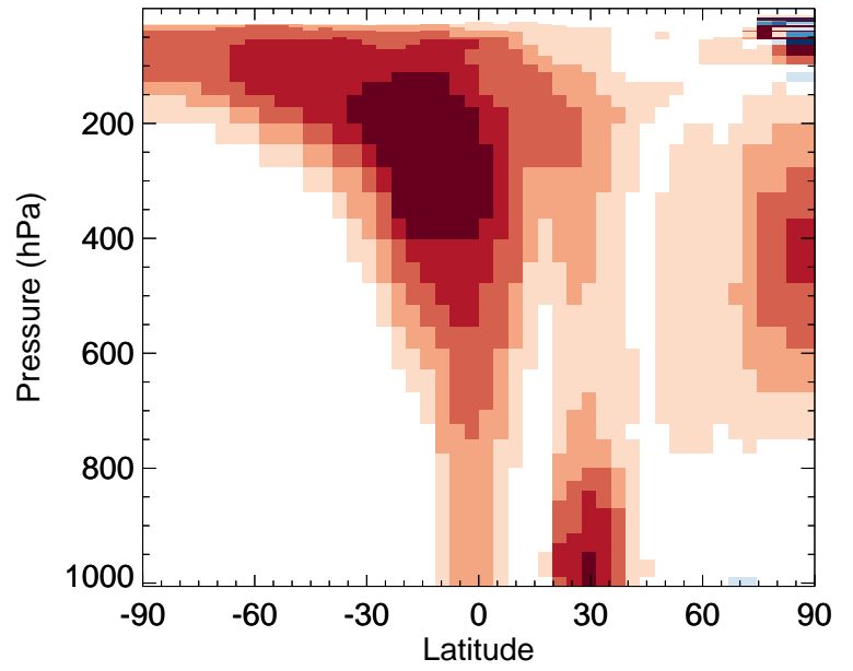
v11-02a / v11-01-public-Run0 IEPOX - Zonal mean % diff for Jul
