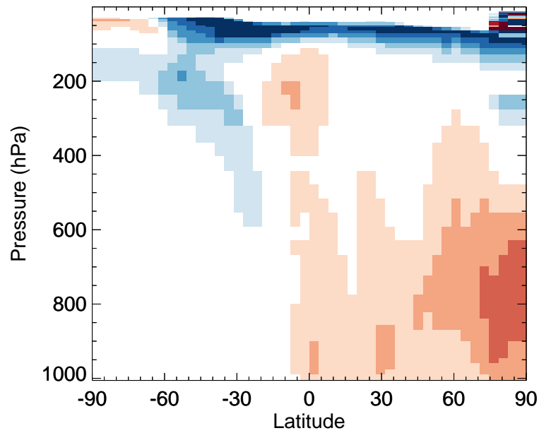
v11-02a / v11-01k-Run0 MACRN - Zonal mean % diff for Jul
