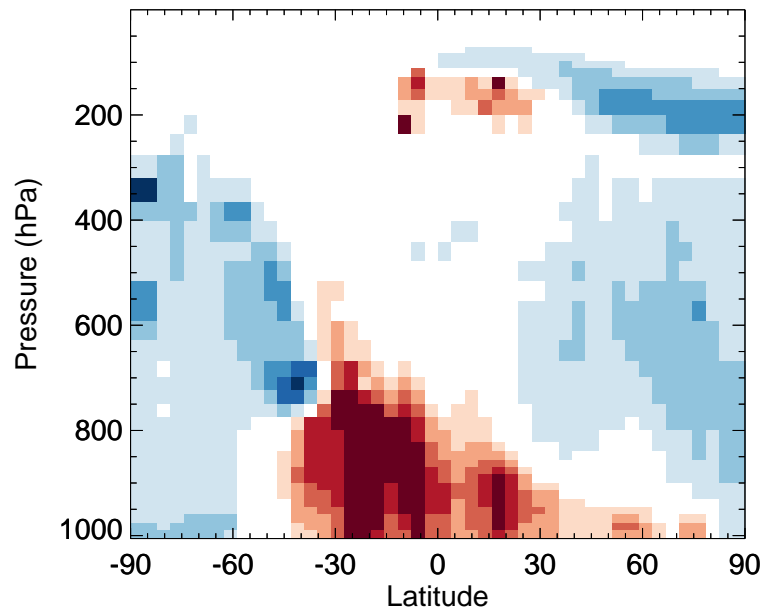
v11-02a / v11-01k-Run0 NH3 - Zonal mean % diff for Jul
