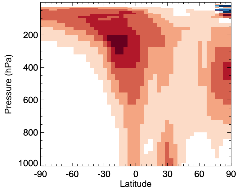
v11-02a / v11-01k-Run0 GLYC - Zonal mean % diff for Jul
