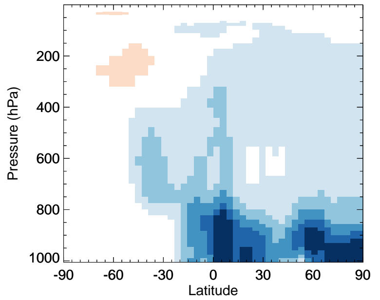
v11-02a / v11-01-public-Run0 OCIO - Zonal mean % diff for Jul
