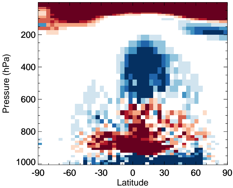
v11-02a - v11-01-public-Run0 H2O - Zonal mean abs diff for Jul
