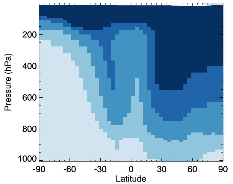
v11-02a / v11-01-public-Run0 CHBr3 - Zonal mean % diff for Jul
