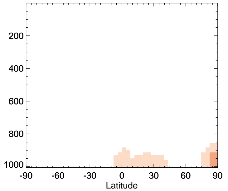
v11-02a / v11-01-public-Run0 CH 2 O - Zonal mean % diff for Jul
