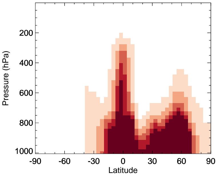
v11-02a - v11-01k-Run0 MEK - Zonal mean abs diff for Jul
