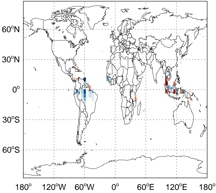
v11-02c - v11-01-public-Run0 ALD2 biogenic emissions for Apr
