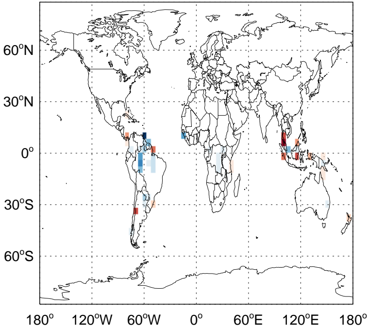
v11-02c - v11-01-public-Run0 ALD2 biogenic emissions for Jan
