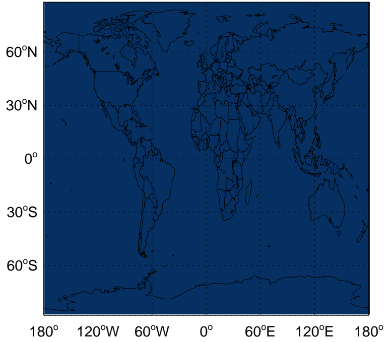
v11-02c - v11-02a CH 2 Br 2 biogenic emissions for Apr
