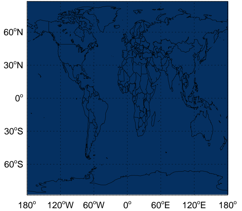
v11-02c - v11-02a CO from MONOT emissions for Apr
