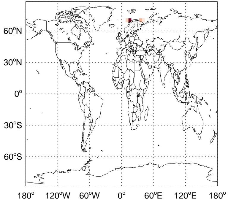
v11-02c - v11-02a CO ship emissions for Apr
