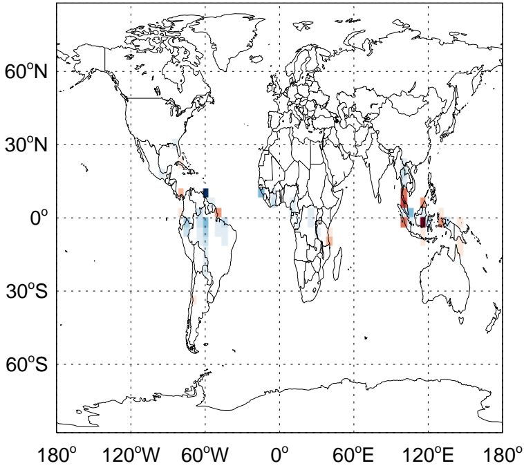
v11-02c - v11-01-public-Run0 CO from MONOT emissions for Apr
