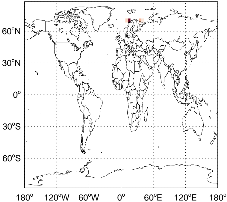
v11-02c - v11-01-public-Run0 CO ship emissions for Apr
