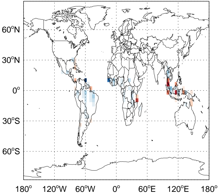
v11-02c - v11-01-public-Run0 PRPE biogenic emissions for Apr
