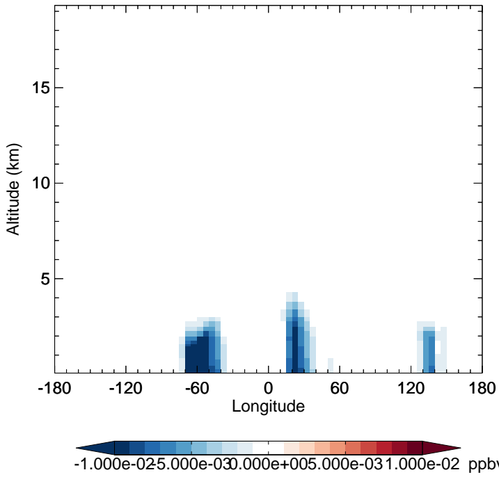
v11-02c - v11-02a NPMN - Diff along 15S for Oct
