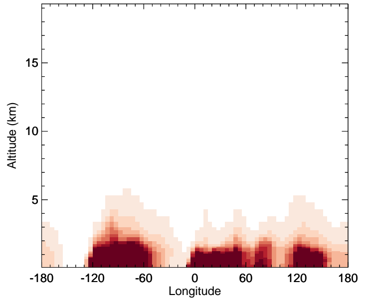
v11-02c - v11-01-public-Run0 EOH - Diff along 42N for Oct
