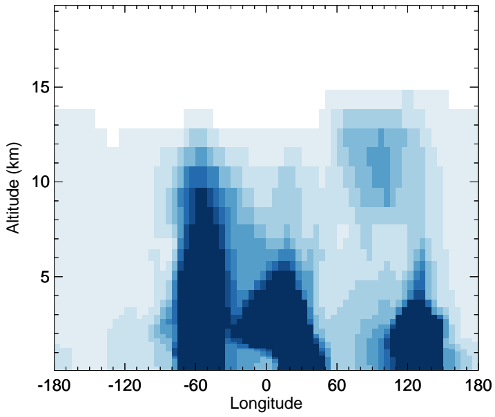
v11-02c - v11-02a R4N2 - Diff along 15S for Oct
