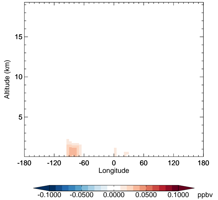
v11-02c - v11-01-public-Run0 IMAE - Diff along 42N for Oct
