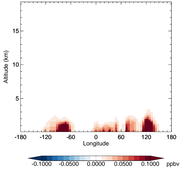
v11-02c - v11-02a SOAP - Diff along 42N for Oct
