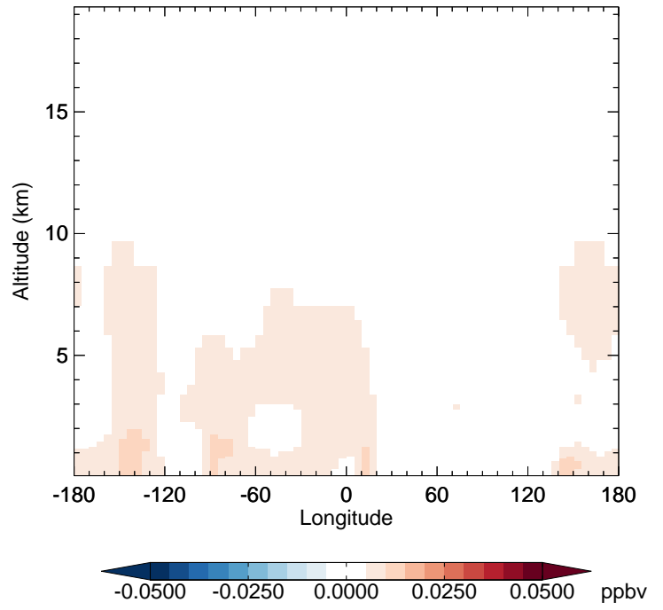
v11-02c - v11-02a MP - Diff along 42N for Oct
