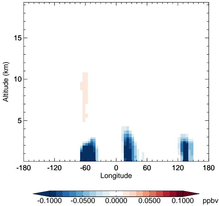
v11-02c - v11-01-public-Run0 GLYC - Diff along 15S for Oct
