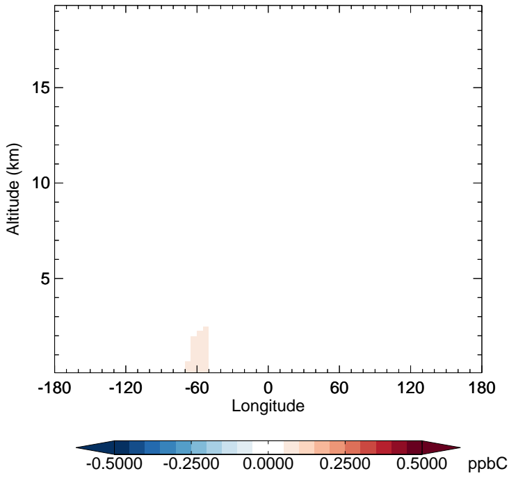
v11-02c - v11-02a C2H6 - Diff along 15S for Oct
