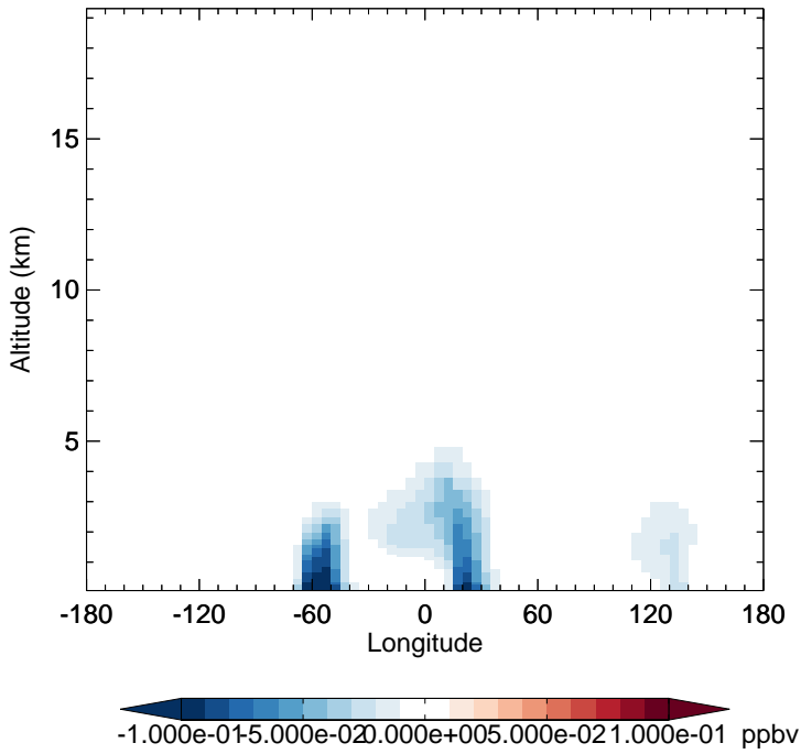
v11-02c - v11-01-public-Run0 TSOG3 - Diff along 15S for Oct
