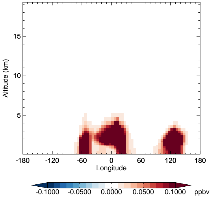
v11-02c - v11-01-public-Run0 INDIOL - Diff along 15S for Oct
