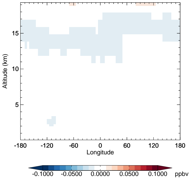
v11-02c - v11-01-public-Run0 CFC11 - Diff along 15S for Oct
