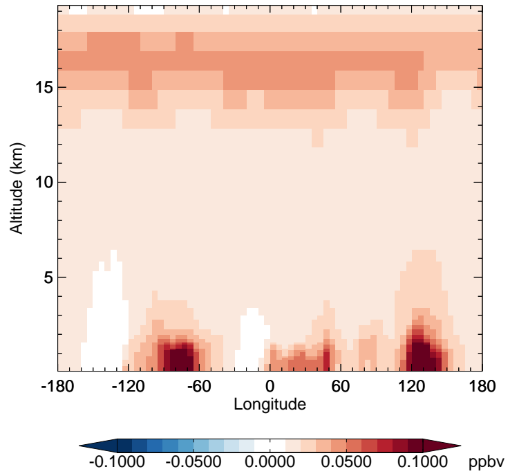
v11-02c - v11-02a PAN - Diff along 42N for Oct
