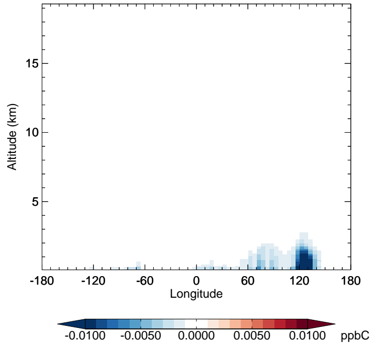
v11-02c - v11-02a PRPE - Diff along 42N for Oct
