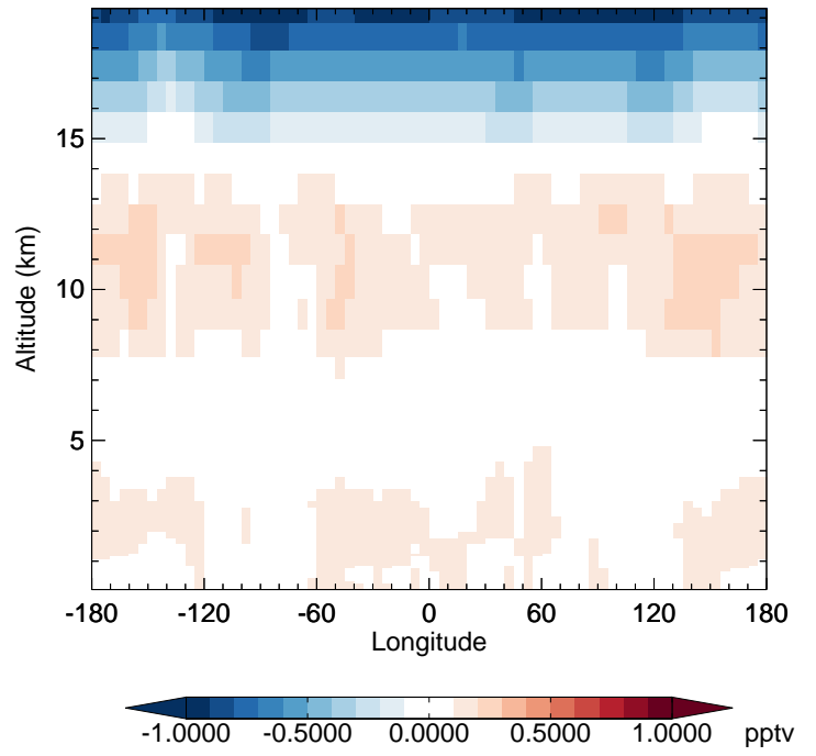
v11-02c - v11-02a HO2 - Diff along 42N for Oct
