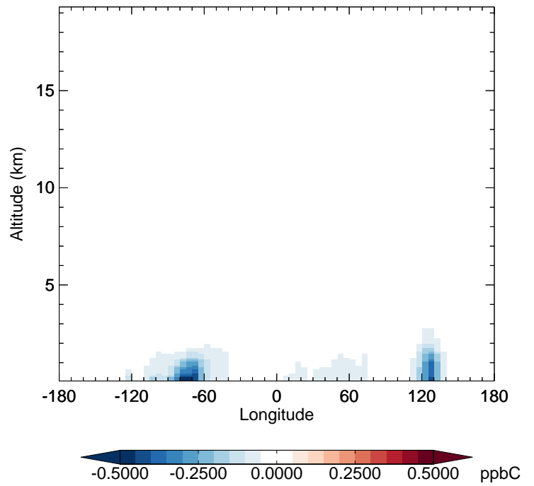
v11-02c - v11-01-public-Run0 ALK4 - Diff along 42N for Oct
