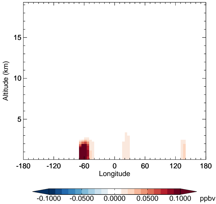
v11-02c - v11-02a RIPB - Diff along 15S for Oct
