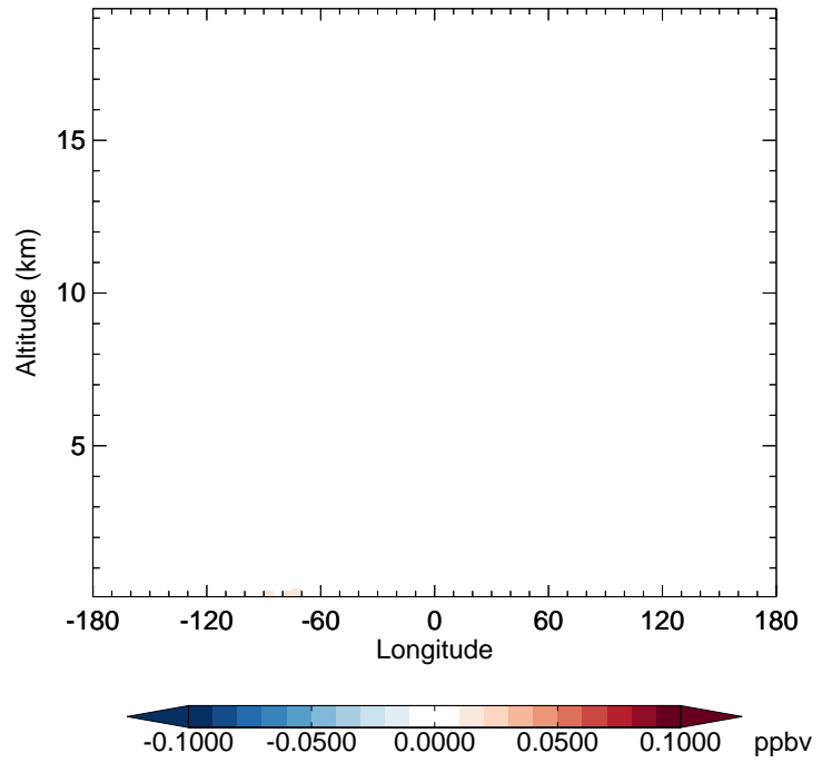
v11-02c - v11-02a MONITA - Diff along 42N for Oct
