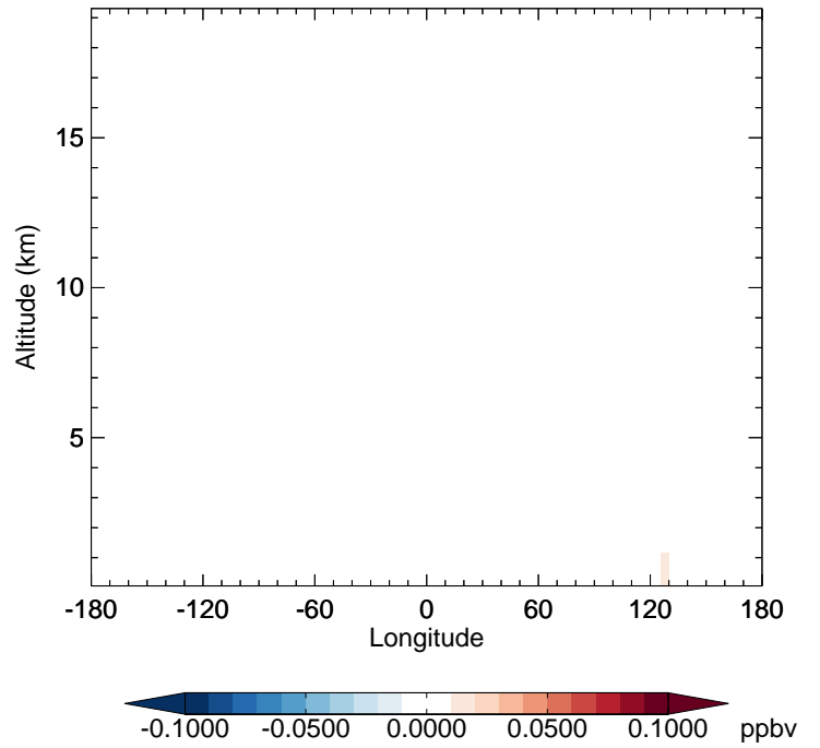
v11-02c - v11-01-public-Run0 ASOA2 - Diff along 42N for Oct
