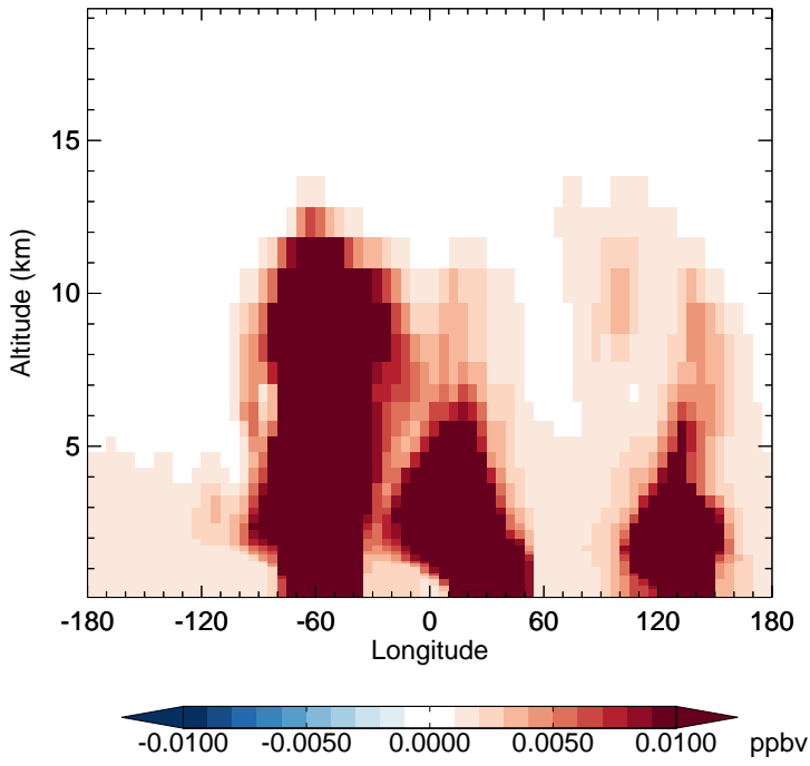
v11-02c - v11-02a MAP - Diff along 15S for Oct
