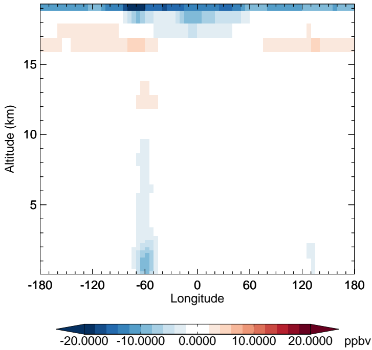
v11-02c - v11-01-public-Run0 O3 - Diff along 15S for Oct
