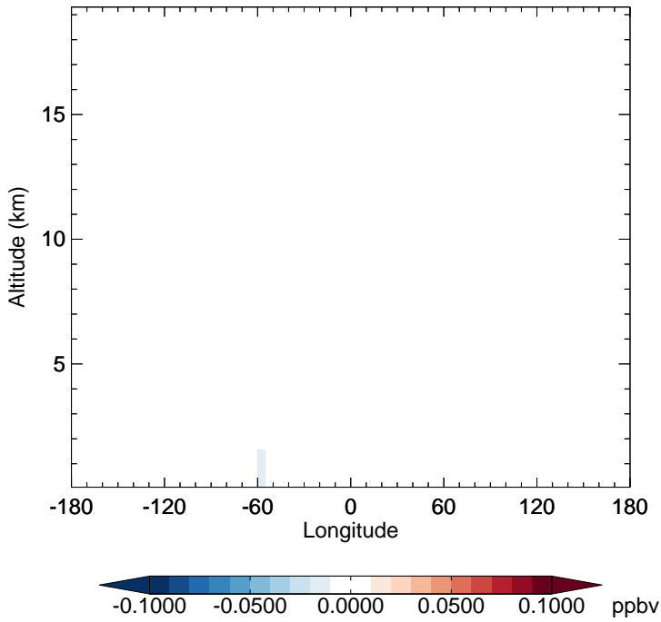
v11-02c - v11-01-public-Run0 ISOA3 - Diff along 15S for Oct
