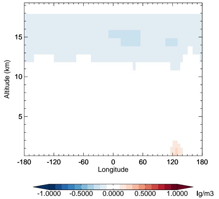
v11-02c - v11-02a SO4 - Diff along 42N for Oct
