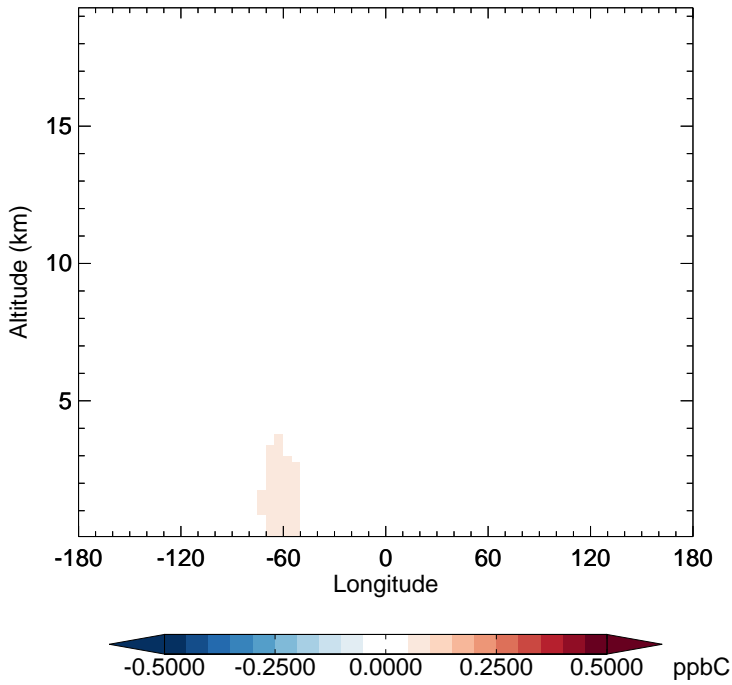
v11-02c - v11-01-public-Run0 C2H6 - Diff along 15S for Oct
