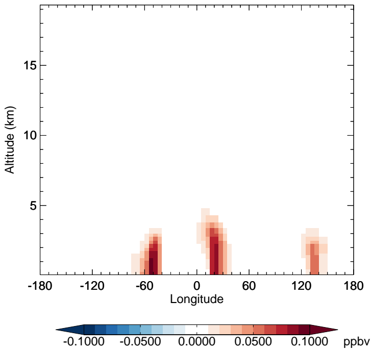
v11-02c - v11-02a IONITA - Diff along 15S for Oct
