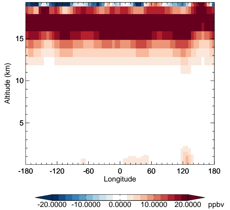
v11-02c - v11-01-public-Run0 O3 - Diff along 42N for Oct
