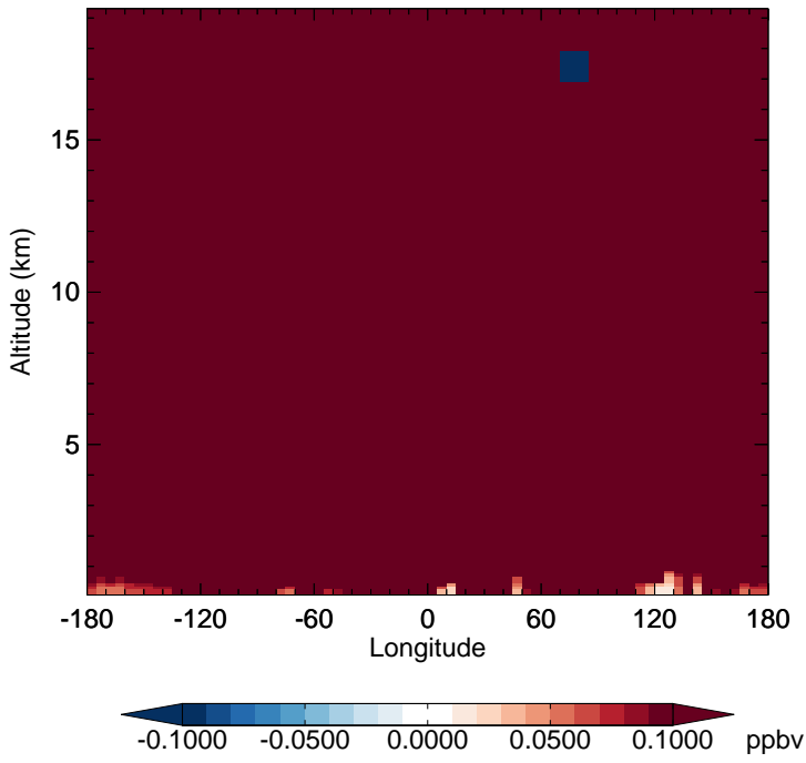
v11-02c - v11-02a N2O - Diff along 15S for Oct
