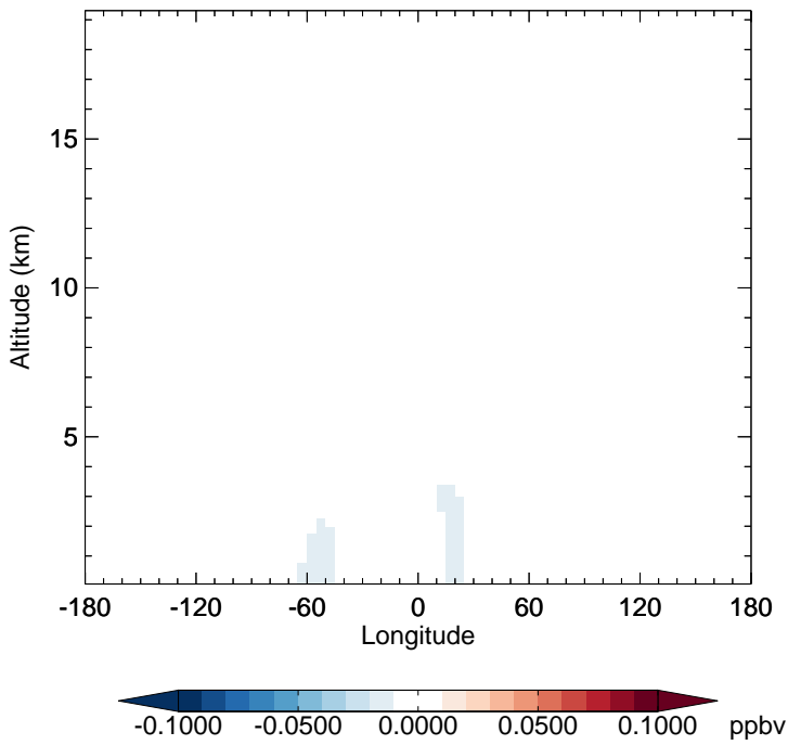
v11-02c - v11-01-public-Run0 TSOA1 - Diff along 15S for Oct
