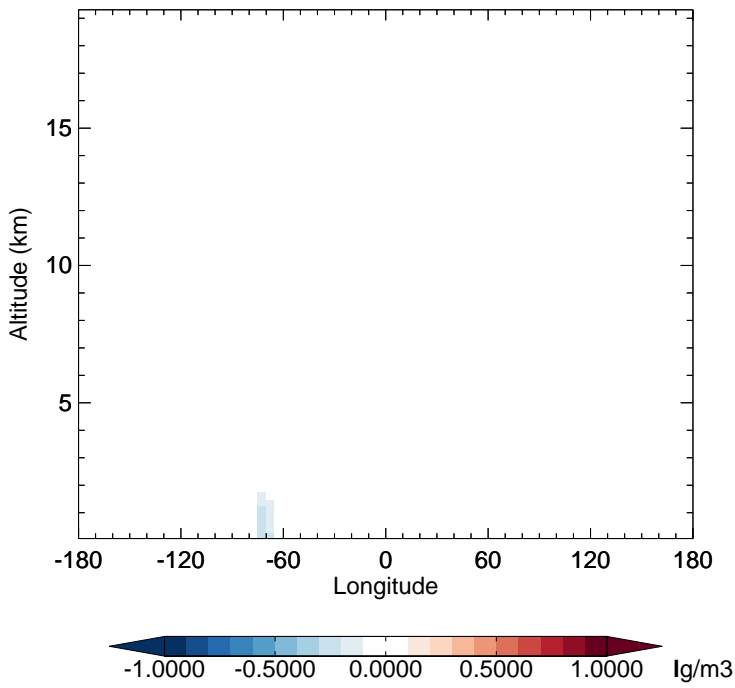
v11-02c - v11-02a SO4 - Diff along 15S for Oct
