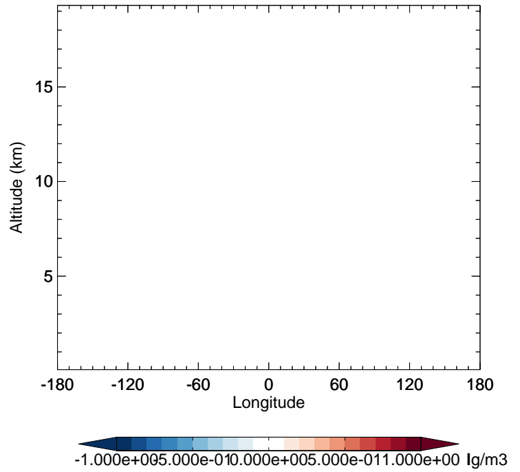
v11-02c - v11-01-public-Run0 BCPO - Diff along 42N for Oct
