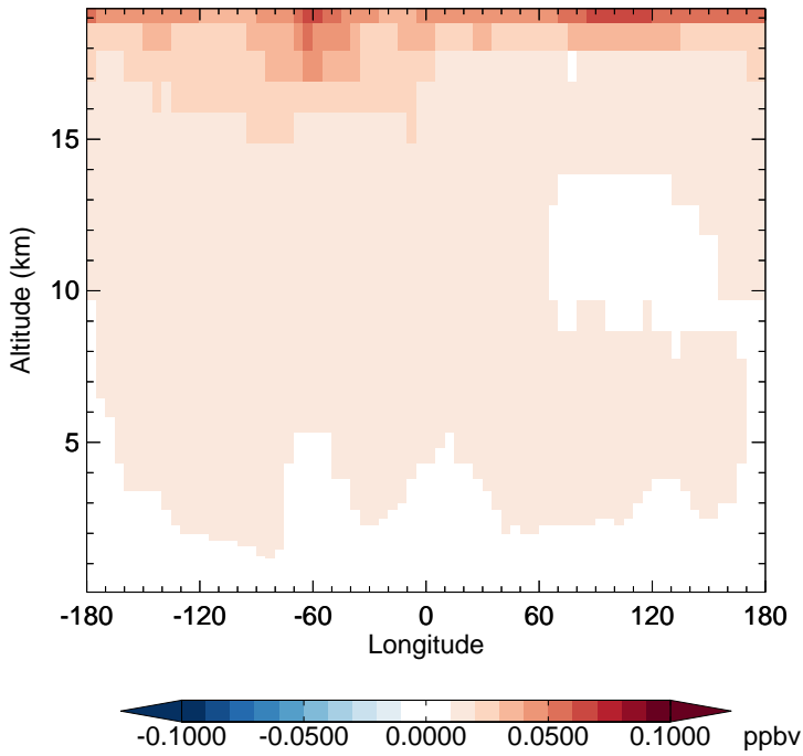
v11-02c - v11-01-public-Run0 OCS - Diff along 15S for Oct
