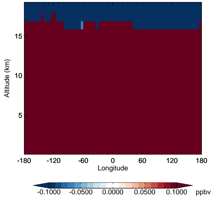
v11-02c - v11-02a CH4 - Diff along 42N for Oct
