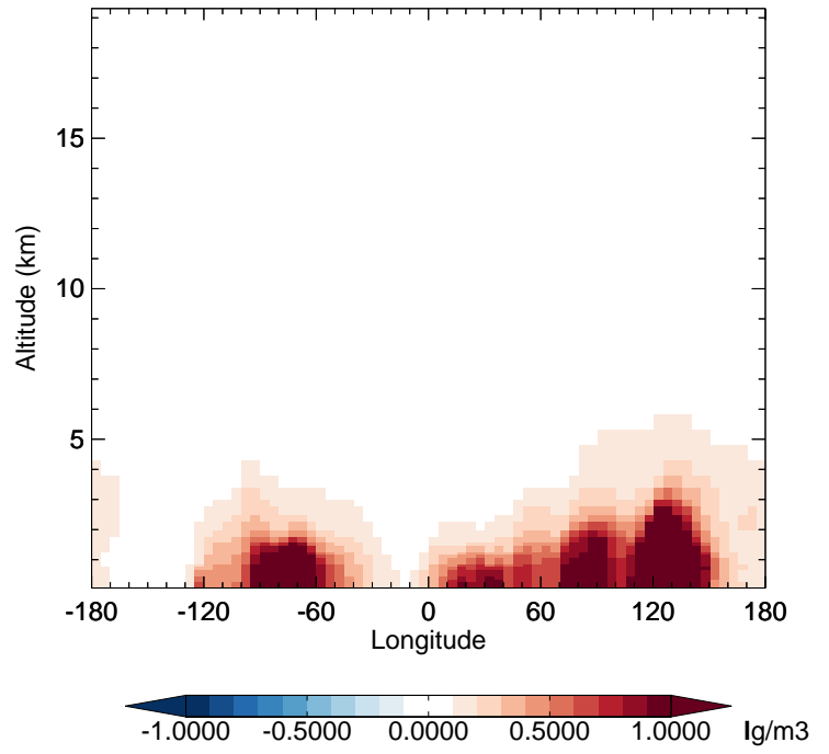
v11-02c - v11-02a SOAS - Diff along 42N for Oct
