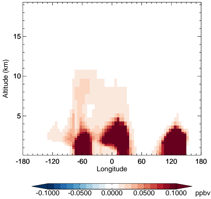
v11-02c - v11-02a SOAIE - Diff along 15S for Oct
