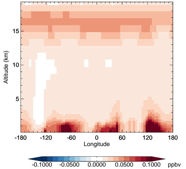
v11-02c - v11-01-public-Run0 PAN - Diff along 42N for Oct
