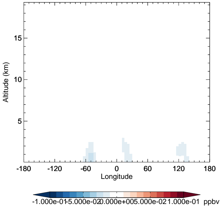
v11-02c - v11-01-public-Run0 ISOG2 - Diff along 15S for Oct
