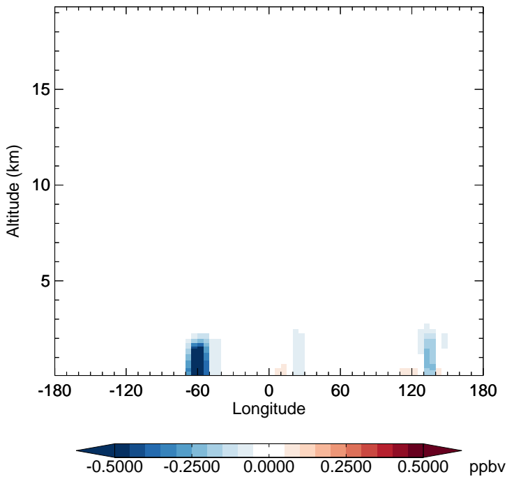
v11-02c - v11-01-public-Run0 CH 2 O - Diff along 15S for Oct
