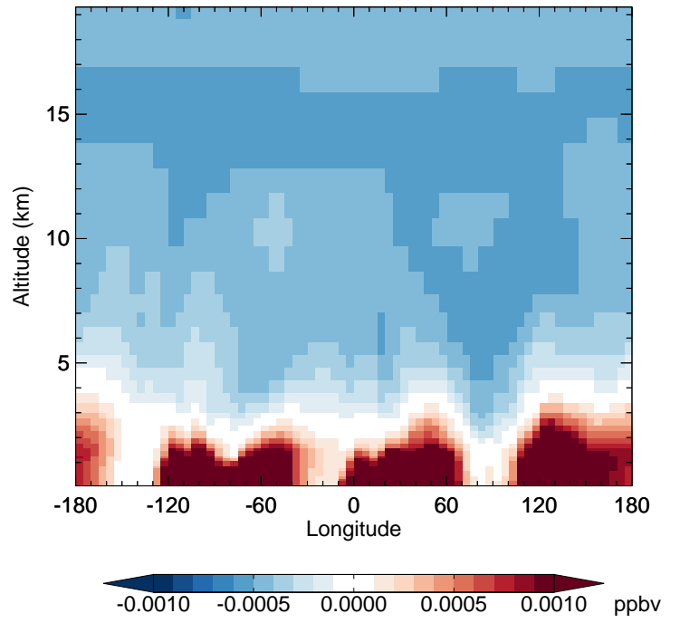
v11-02c - v11-02a PPN - Diff along 42N for Oct
