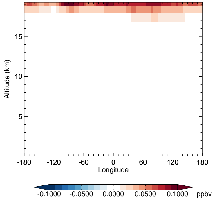
v11-02c - v11-02a CINO3 - Diff along 42N for Oct
