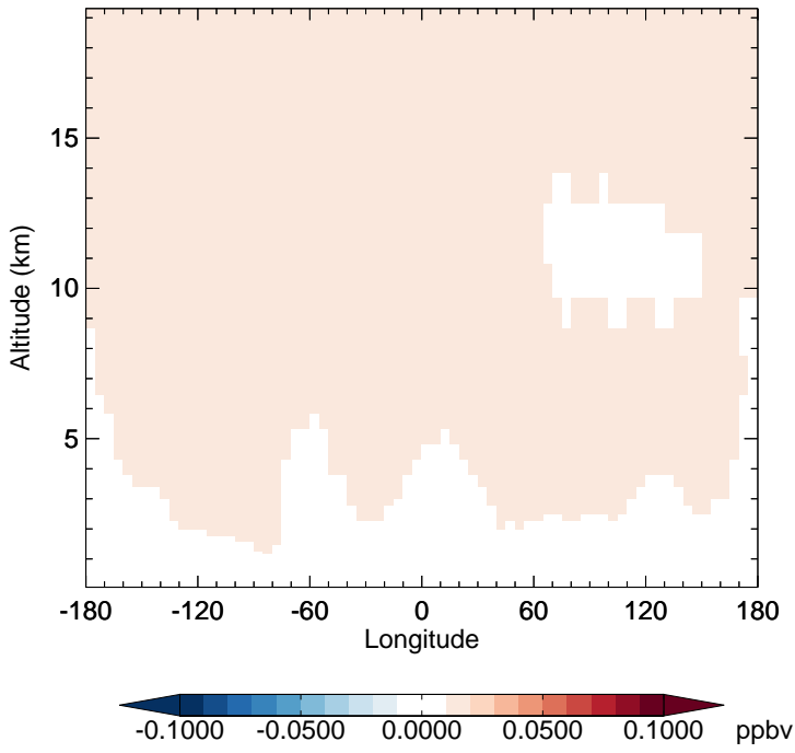
v11-02c - v11-02a HCFC141b - Diff along 15S for Oct
