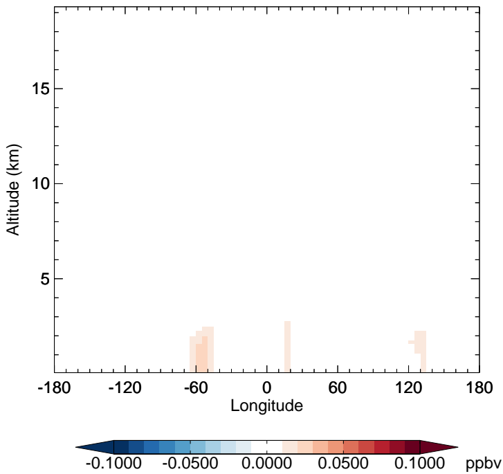
v11-02c - v11-01-public-Run0 LVOCOA - Diff along 15S for Oct
