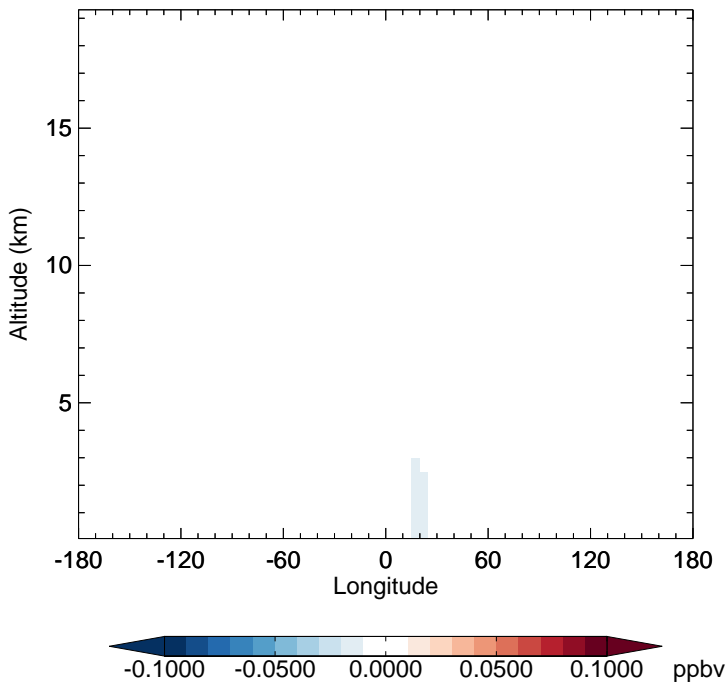
v11-02c - v11-02a TSOA1 - Diff along 15S for Oct
