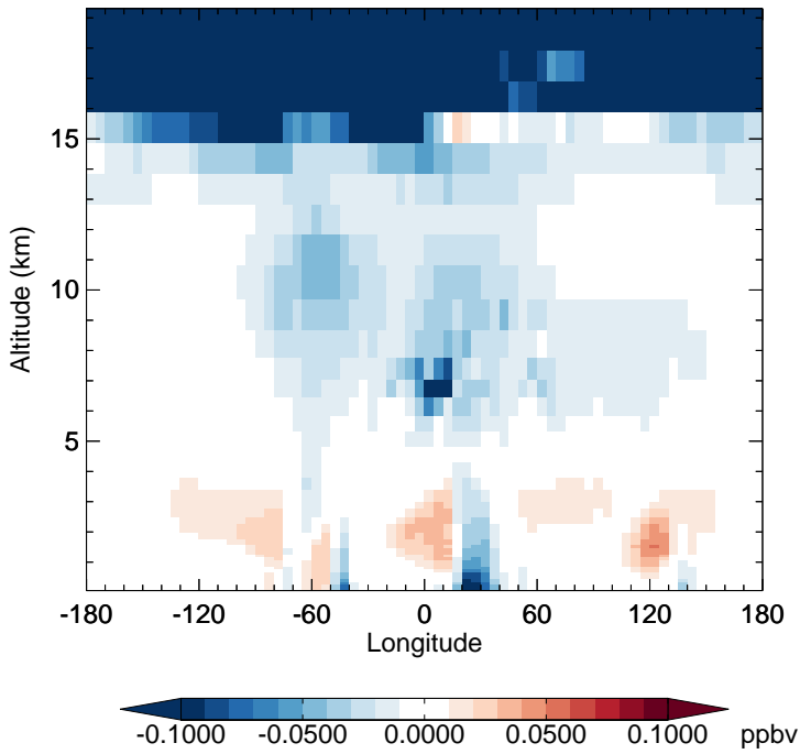
v11-02c - v11-01-public-Run0 HNO 3 - Diff along 15S for Oct
