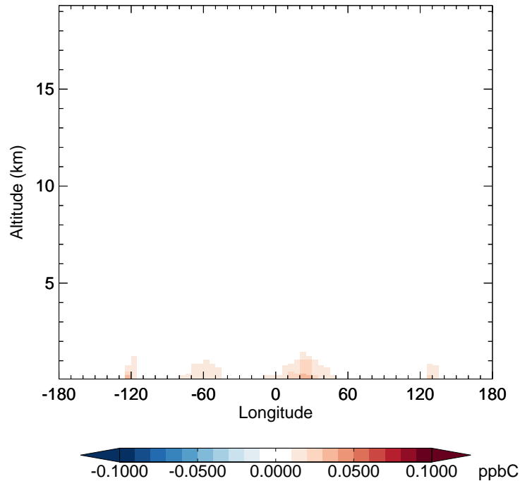
v11-02c - v11-02a MEK - Diff along 42N for Oct
