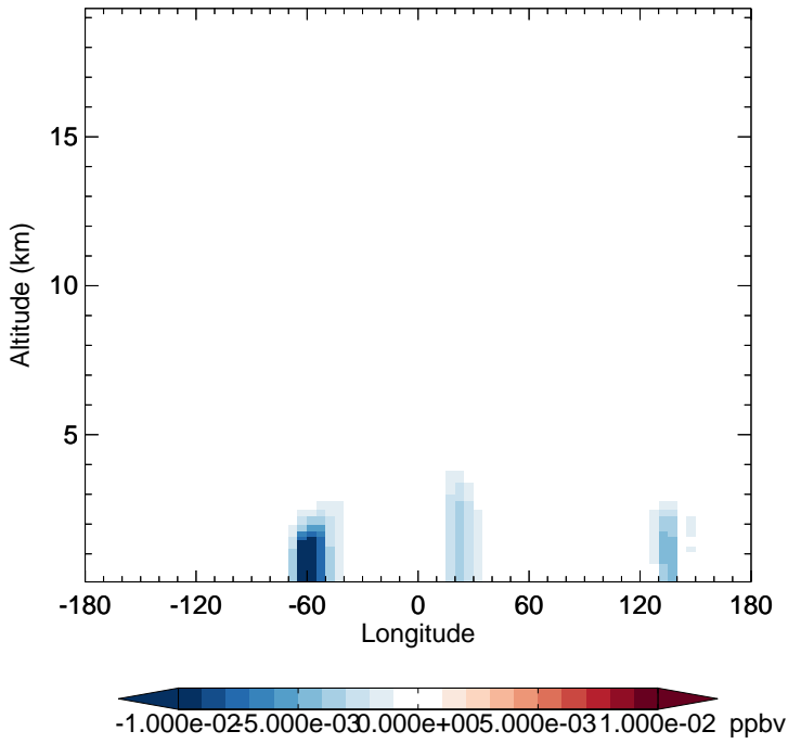
v11-02c - v11-02a MACRN - Diff along 15S for Oct
