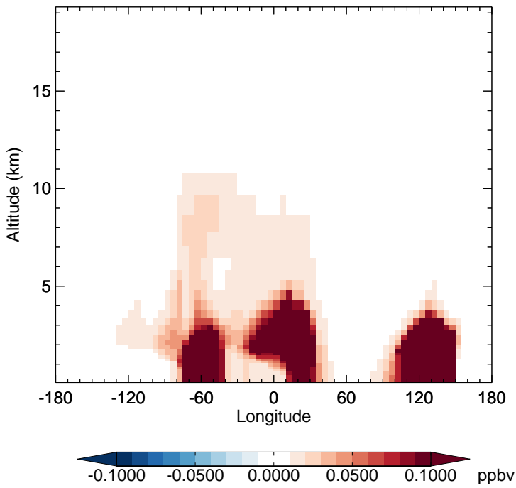
v11-02c - v11-01-public-Run0 SOAIE - Diff along 15S for Oct
