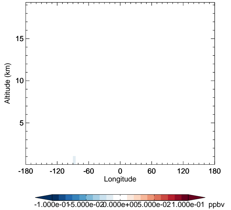
v11-02c - v11-01-public-Run0 GLYC - Diff along 42N for Oct
