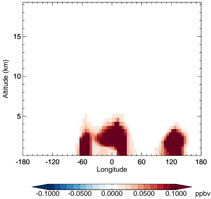
v11-02c - v11-02a INDIOL - Diff along 15S for Oct
