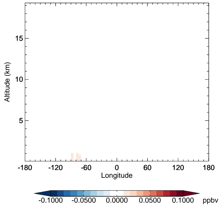
v11-02c - v11-01-public-Run0 IPMN - Diff along 42N for Oct
