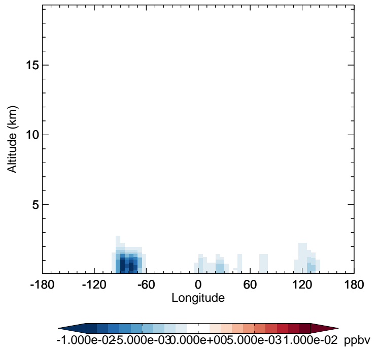
v11-02c - v11-01-public-Run0 MVKN - Diff along 42N for Oct
