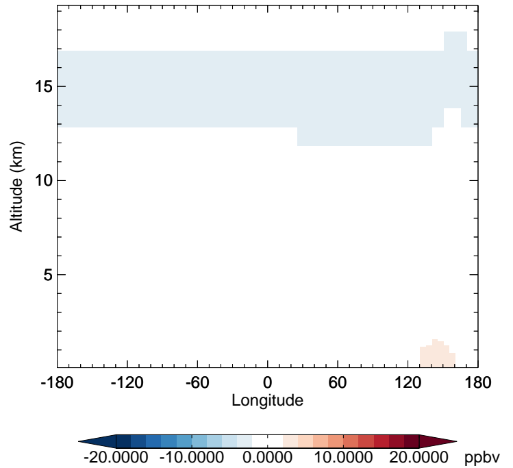
v11-02c - v11-01-public-Run0 CO - Diff along 42N for Oct
