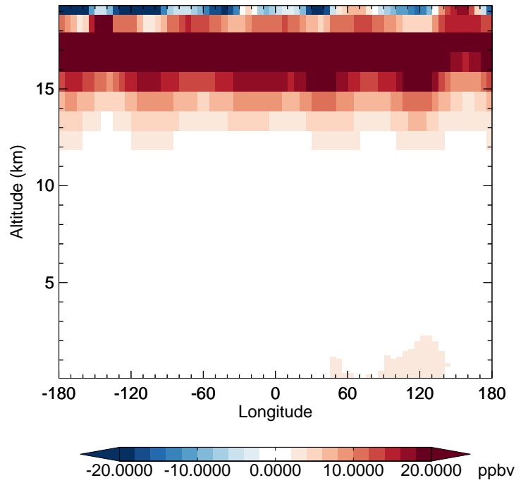
v11-02c - v11-02a O3 - Diff along 42N for Oct
