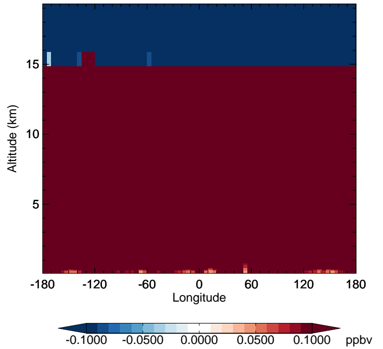
v11-02c - v11-01-public-Run0 N2O - Diff along 42N for Oct
