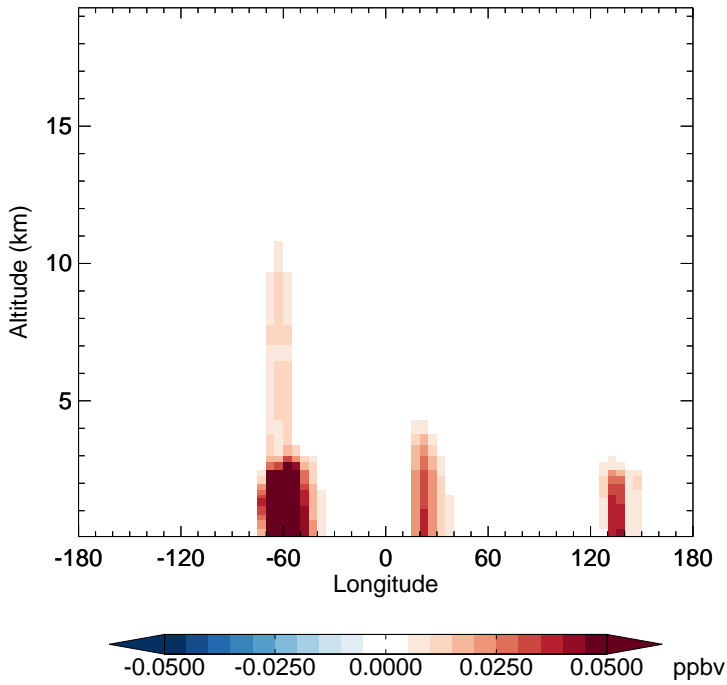
v11-02c - v11-01-public-Run0 MACR - Diff along 15S for Oct
