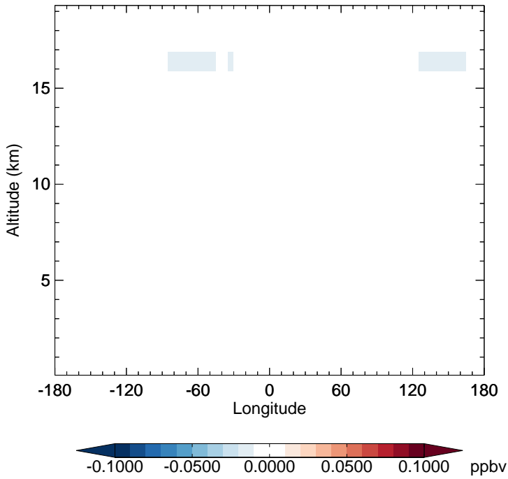
v11-02c - v11-01-public-Run0 HOCl - Diff along 15S for Oct
