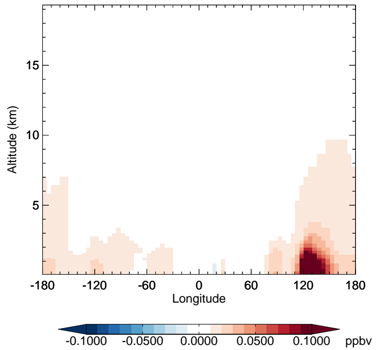
v11-02c - v11-01-public-Run0 BENZ - Diff along 42N for Oct
