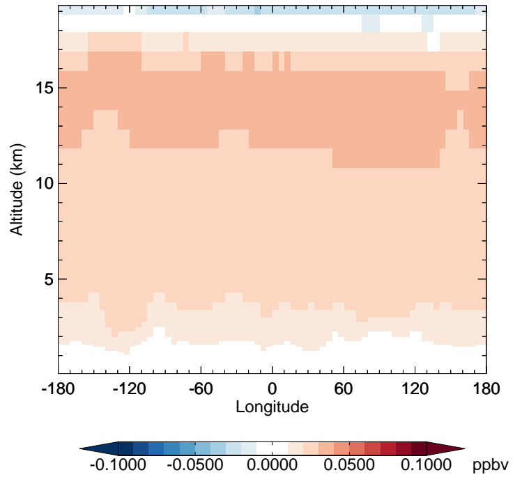
v11-02c - v11-01-public-Run0 CH3Cl - Diff along 42N for Oct
