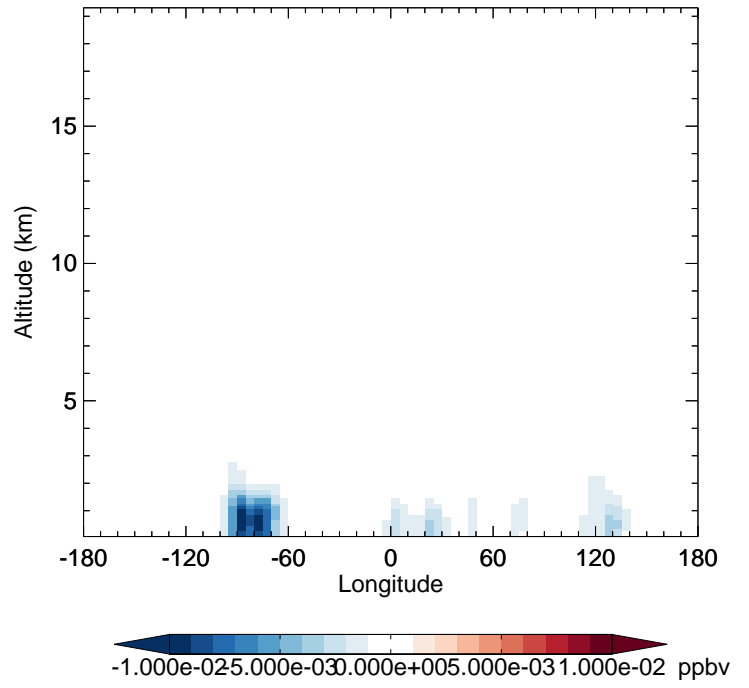
v11-02c - v11-02a MVKN - Diff along 42N for Oct
