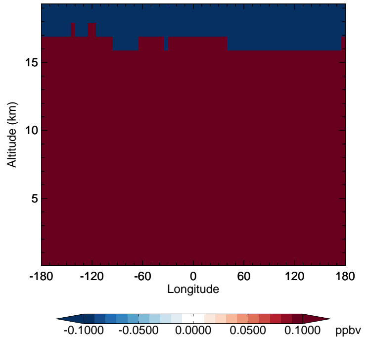
v11-02c - v11-01-public-Run0 CH4 - Diff along 42N for Oct
