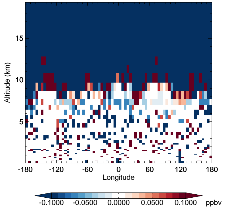
v11-02c - v11-01-public-Run0 H2O - Diff along 42N for Oct
