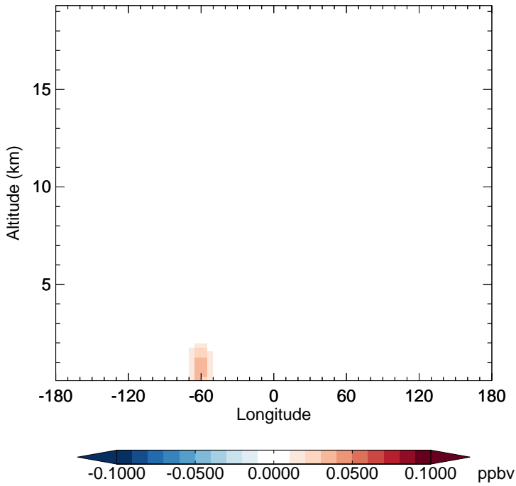
v11-02c - v11-01-public-Run0 RIPD - Diff along 15S for Oct
