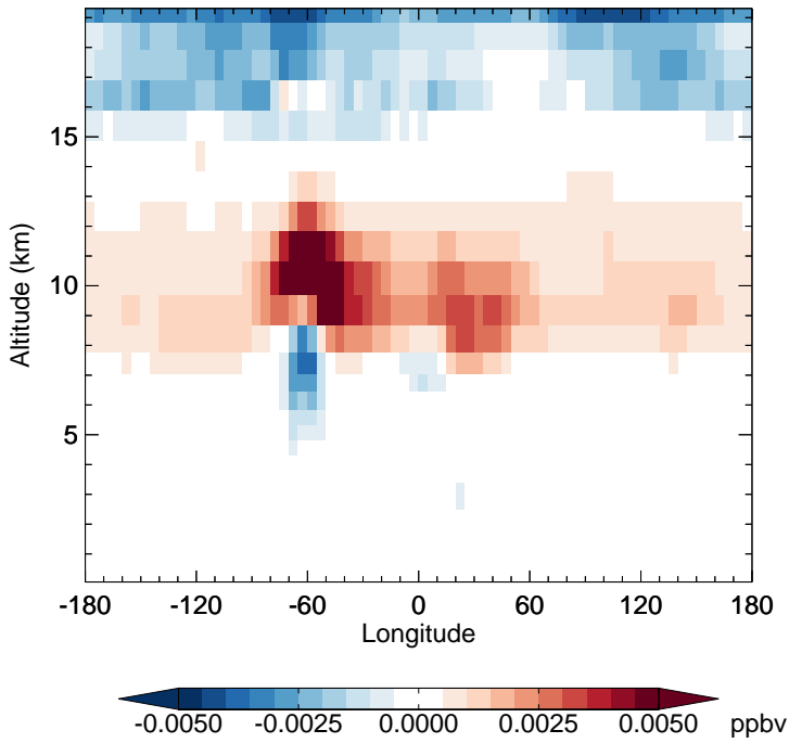
v11-02c - v11-01-public-Run0 HNO 4 - Diff along 15S for Oct
