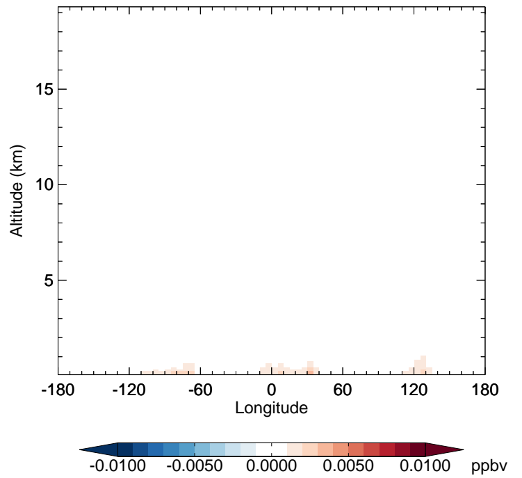
v11-02c - v11-01-public-Run0 NO 3 - Diff along 42N for Oct
