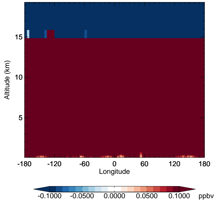
v11-02c - v11-02a N2O - Diff along 42N for Oct
