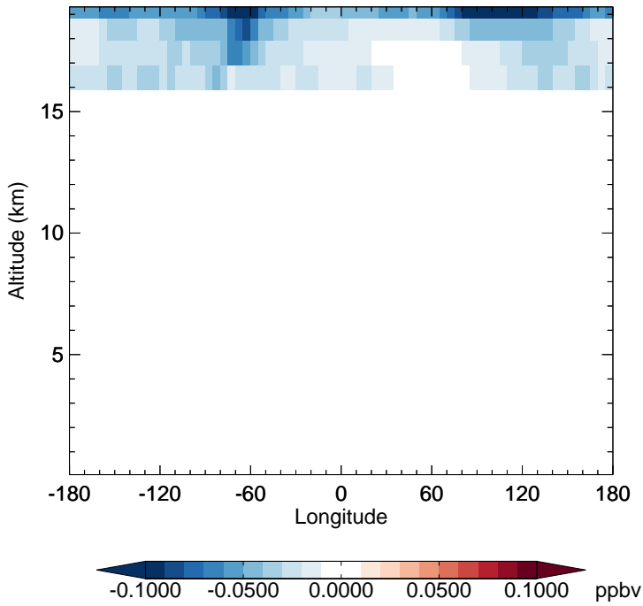
v11-02c - v11-01-public-Run0 CINO3 - Diff along 15S for Oct
