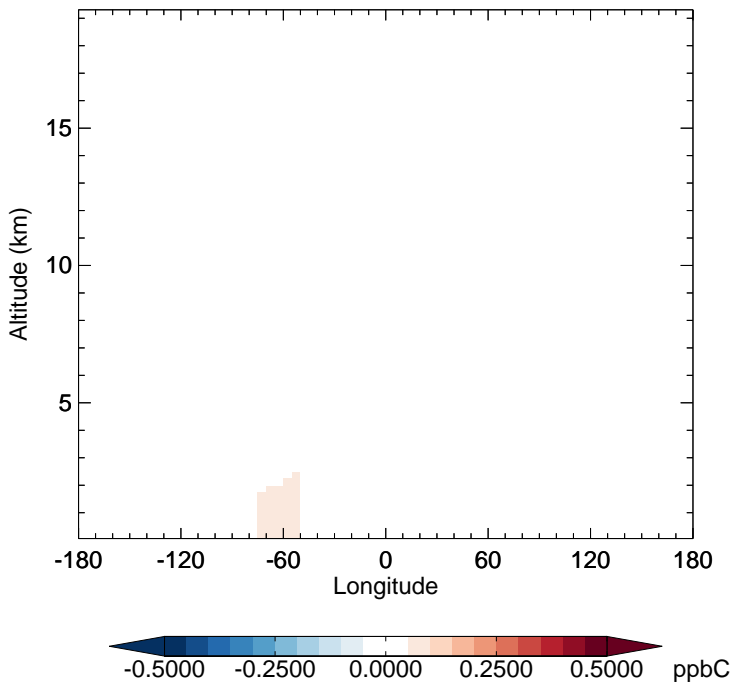
v11-02c - v11-01-public-Run0 ALK4 - Diff along 15S for Oct
