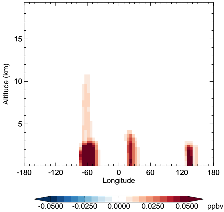
v11-02c - v11-02a MVK - Diff along 15S for Oct
