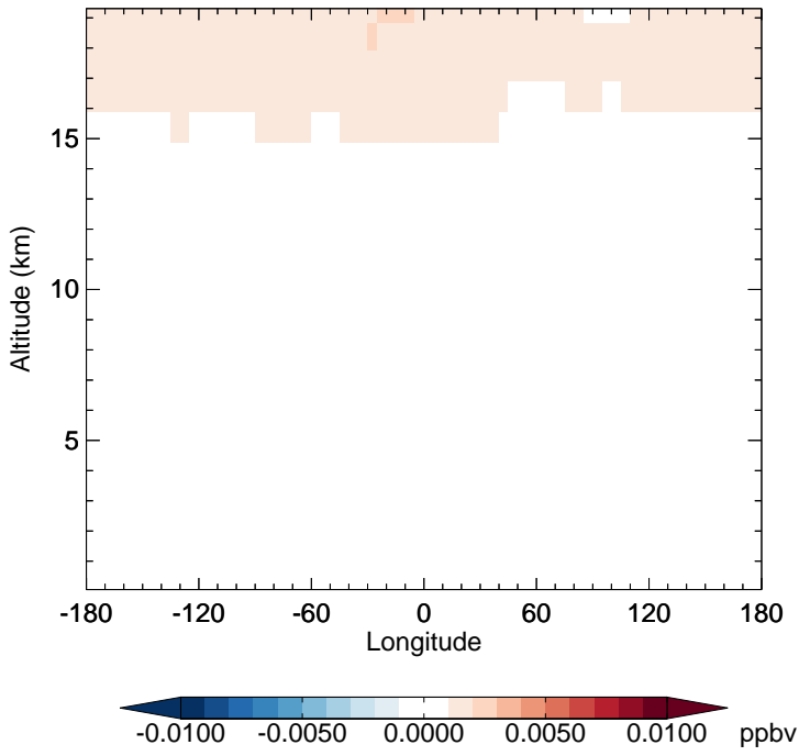
v11-02c - v11-02a BrNO3 - Diff along 15S for Oct
