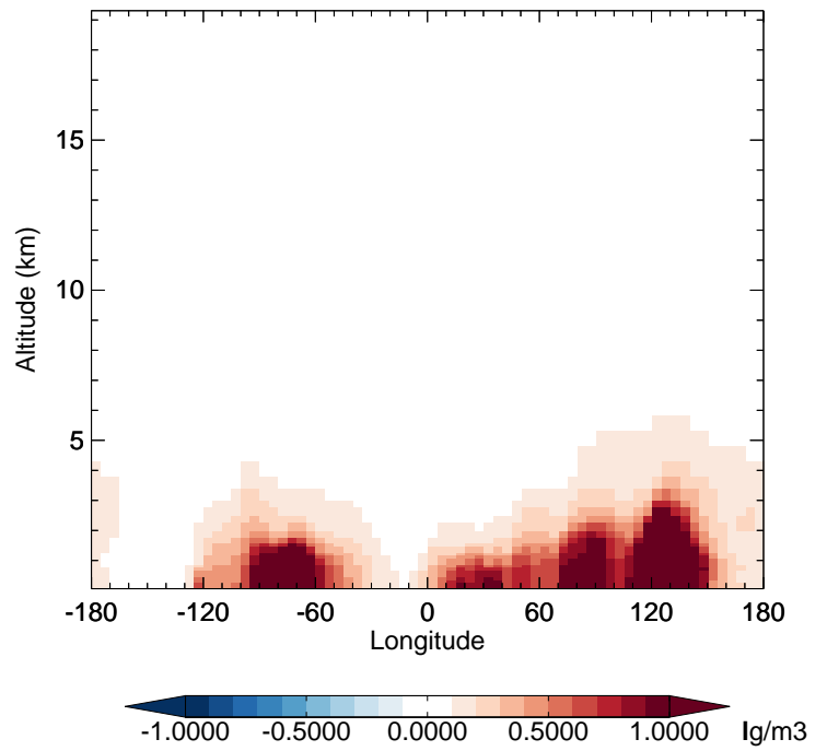
v11-02c - v11-01-public-Run0 SOAS - Diff along 42N for Oct
