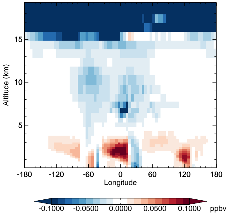
v11-02c - v11-02a HNO 3 - Diff along 15S for Oct
