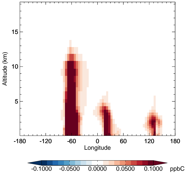
v11-02c - v11-02a MEK - Diff along 15S for Oct
