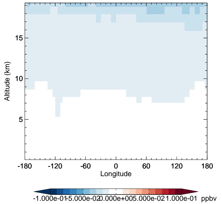
v11-02c - v11-02a CFC11 - Diff along 42N for Oct
