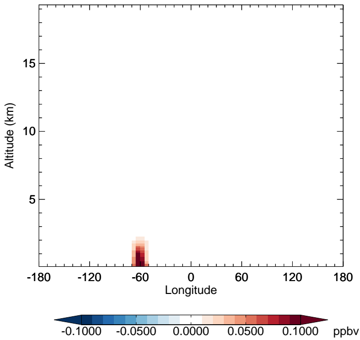
v11-02c - v11-01-public-Run0 MTPA - Diff along 15S for Oct
