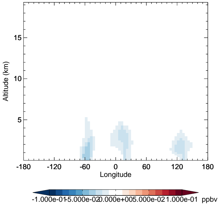
v11-02c - v11-02a PROPNN - Diff along 15S for Oct
