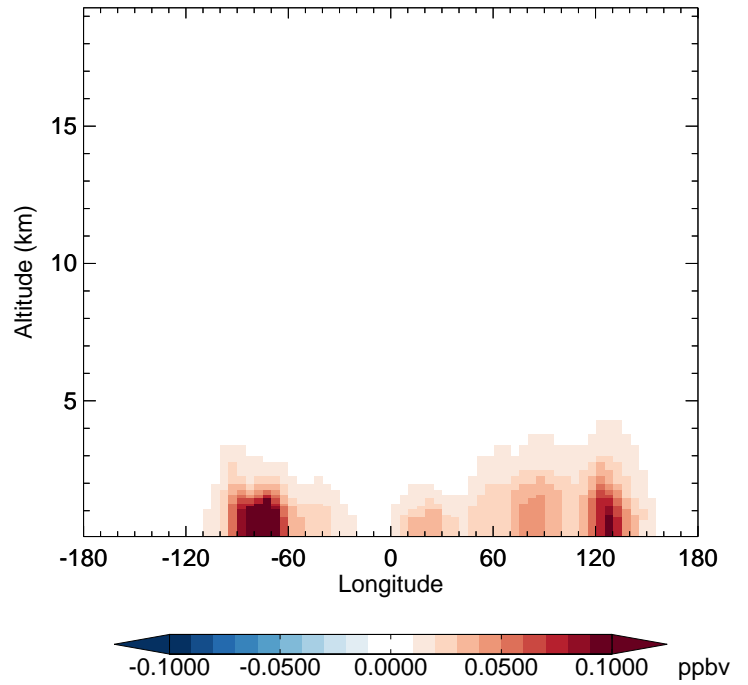
v11-02c - v11-01-public-Run0 INDIOL - Diff along 42N for Oct
