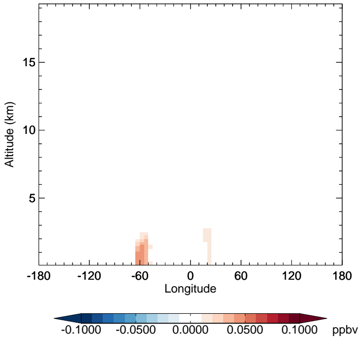
v11-02c - v11-02a TSOA2 - Diff along 15S for Oct
