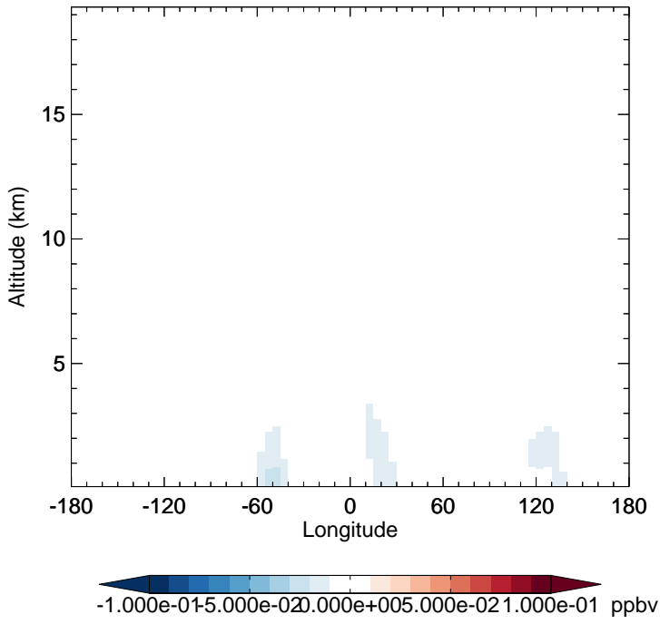
v11-02c - v11-02a ISOG2 - Diff along 15S for Oct
