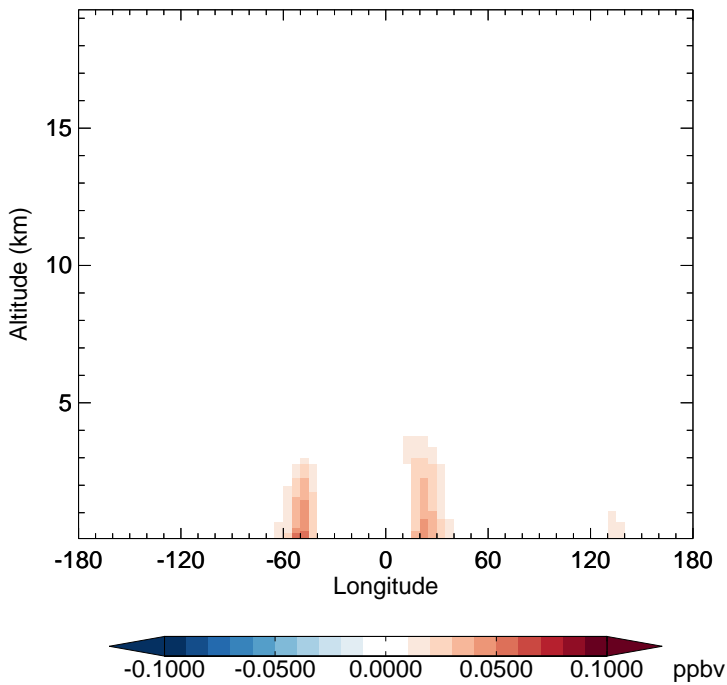
v11-02c - v11-01-public-Run0 MONITA - Diff along 15S for Oct
