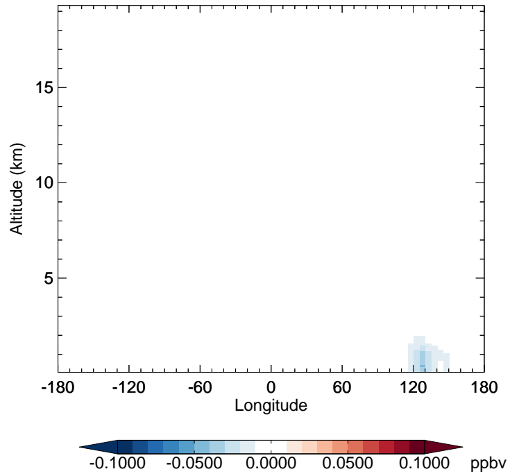
v11-02c - v11-02a XYLE - Diff along 42N for Oct
