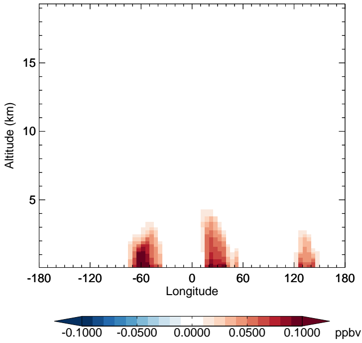
v11-02c - v11-02a SOAP - Diff along 15S for Oct
