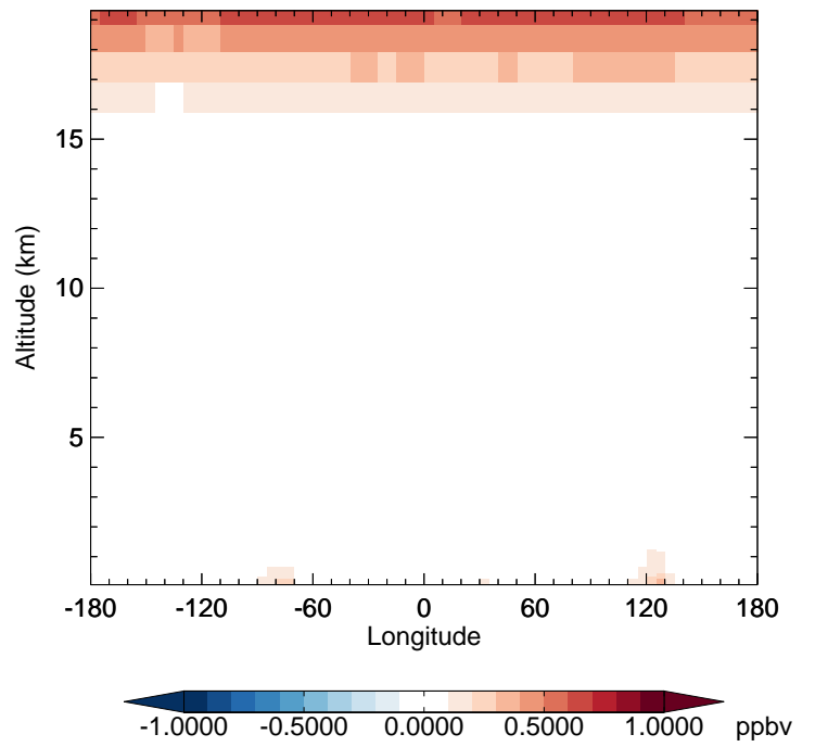
v11-02c - v11-02a NO 2 - Diff along 42N for Oct
