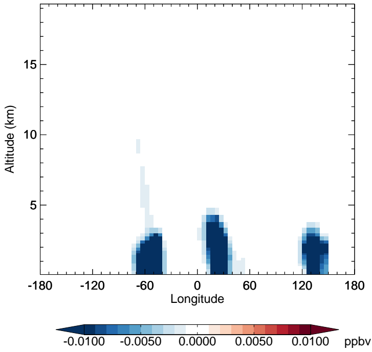
v11-02c - v11-02a MVKN - Diff along 15S for Oct
