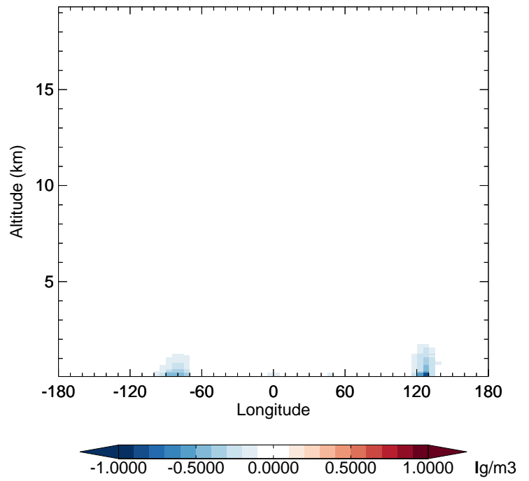
v11-02c - v11-02a NIT - Diff along 42N for Oct
