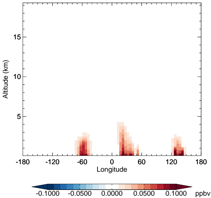
v11-02c - v11-01-public-Run0 TOLU - Diff along 15S for Oct
