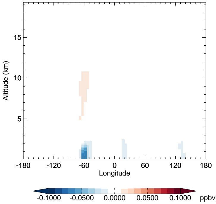
v11-02c - v11-02a ISO3 - Diff along 15S for Oct
