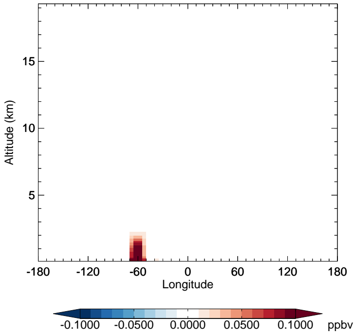
v11-02c - v11-02a MTPA - Diff along 15S for Oct
