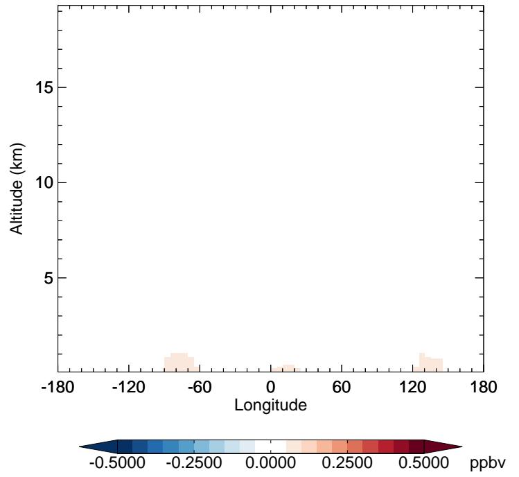
v11-02c - v11-02a CH 2 O - Diff along 42N for Oct
