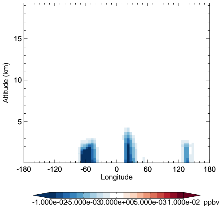
v11-02c - v11-01-public-Run0 NPMN - Diff along 15S for Oct
