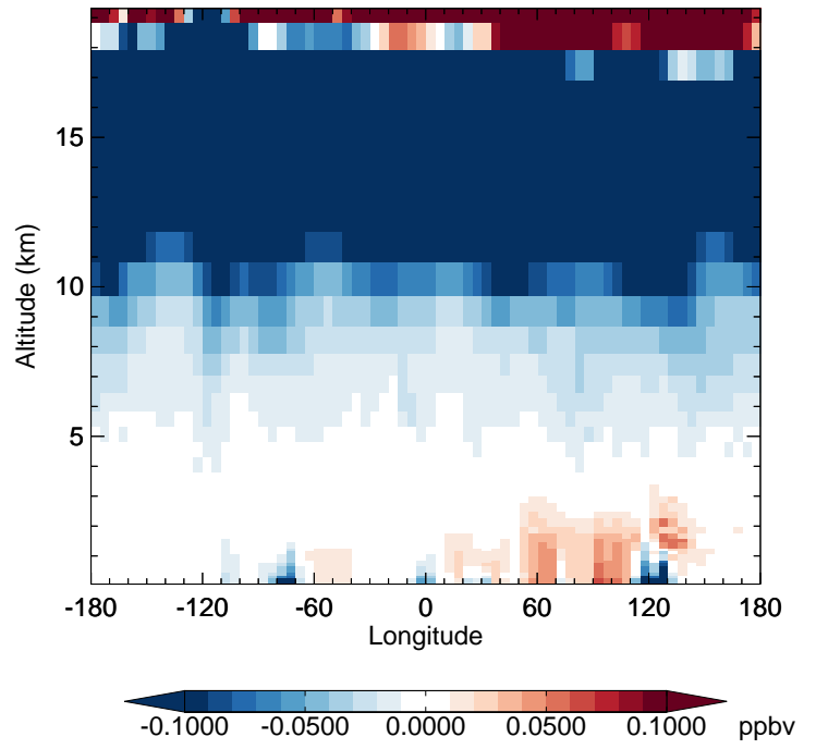
v11-02c - v11-02a HNO 3 - Diff along 42N for Oct
