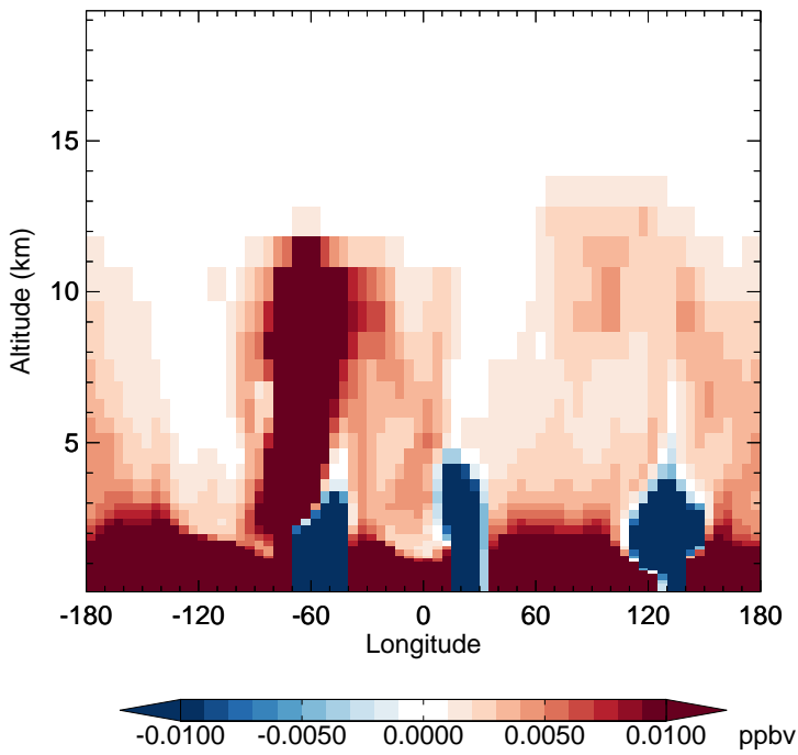
v11-02c - v11-01-public-Run0 MAP - Diff along 15S for Oct
