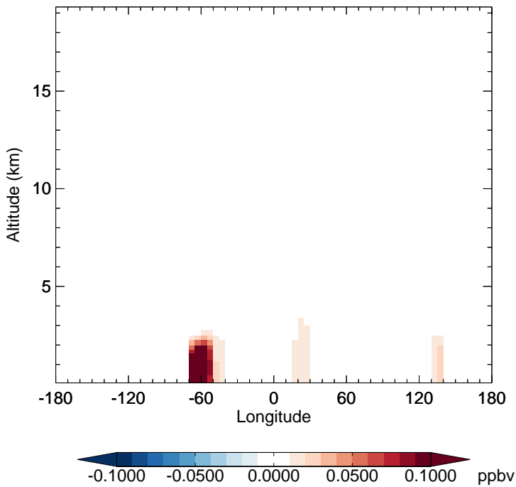
v11-02c - v11-01-public-Run0 RIPB - Diff along 15S for Oct
