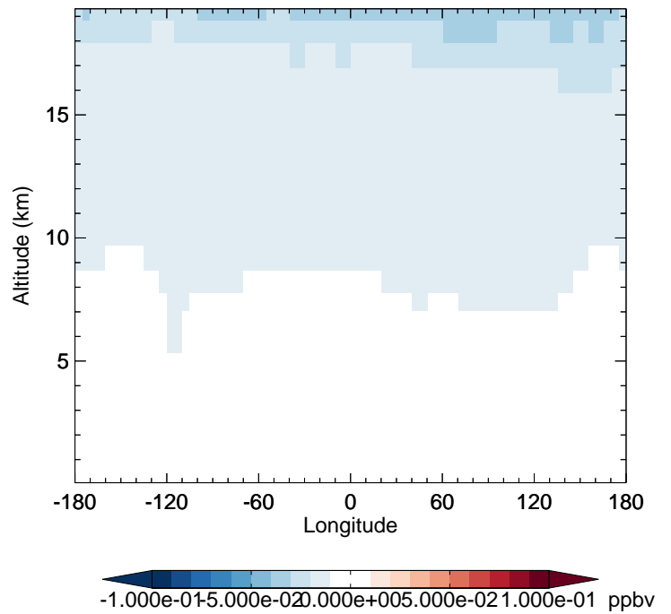
v11-02c - v11-01-public-Run0 CFC11 - Diff along 42N for Oct
