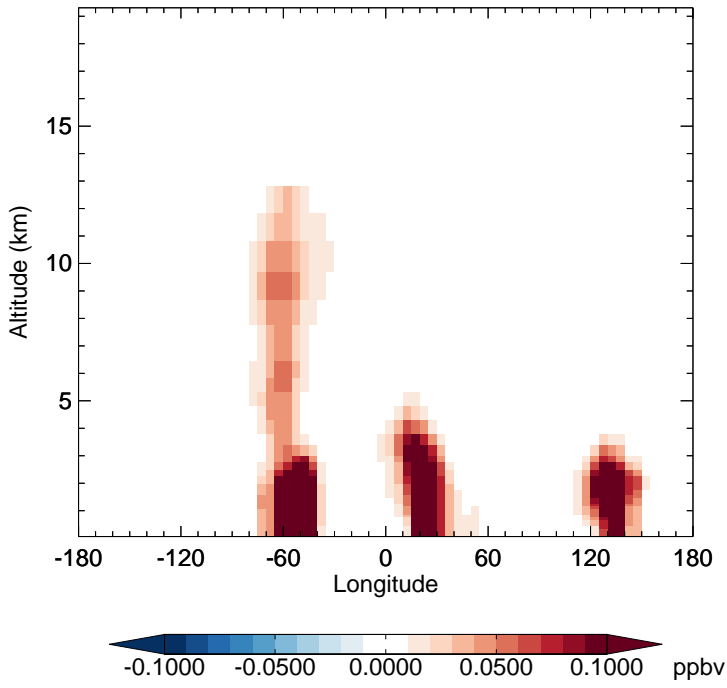
v11-02c - v11-02a IMAE - Diff along 15S for Oct
