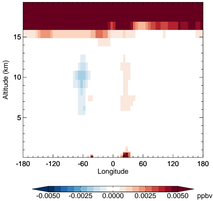
v11-02c - v11-01-public-Run0 N2O5 - Diff along 15S for Oct
