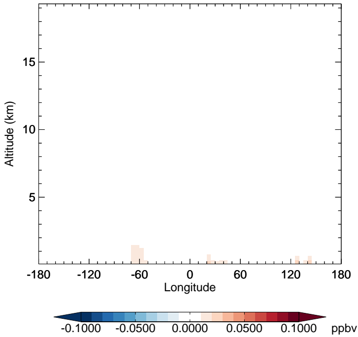
v11-02c - v11-01-public-Run0 XYLE - Diff along 15S for Oct
