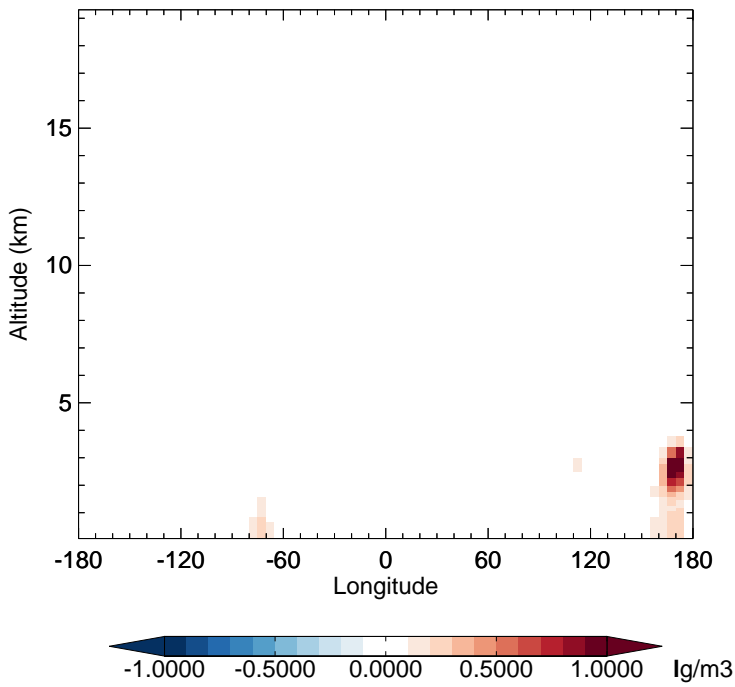
v11-02c - v11-01-public-Run0 SO 2 - Diff along 15S for Oct
