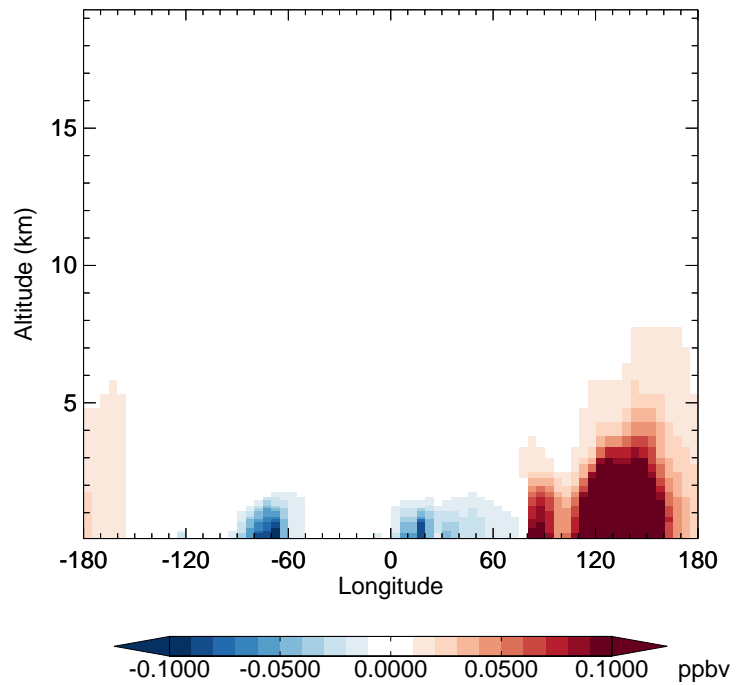
v11-02c - v11-01-public-Run0 TOLU - Diff along 42N for Oct
