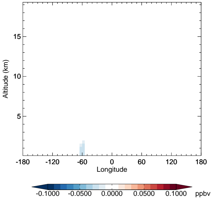
v11-02c - v11-02a ISOA1 - Diff along 15S for Oct
