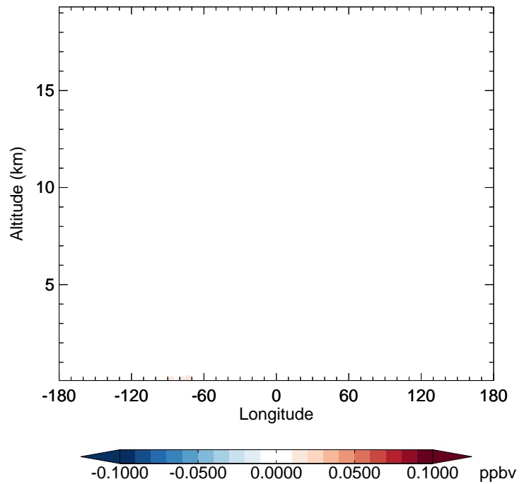
v11-02c - v11-01-public-Run0 MONITA - Diff along 42N for Oct
