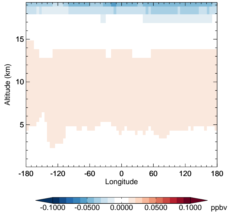
v11-02c - v11-02a OCS - Diff along 42N for Oct
