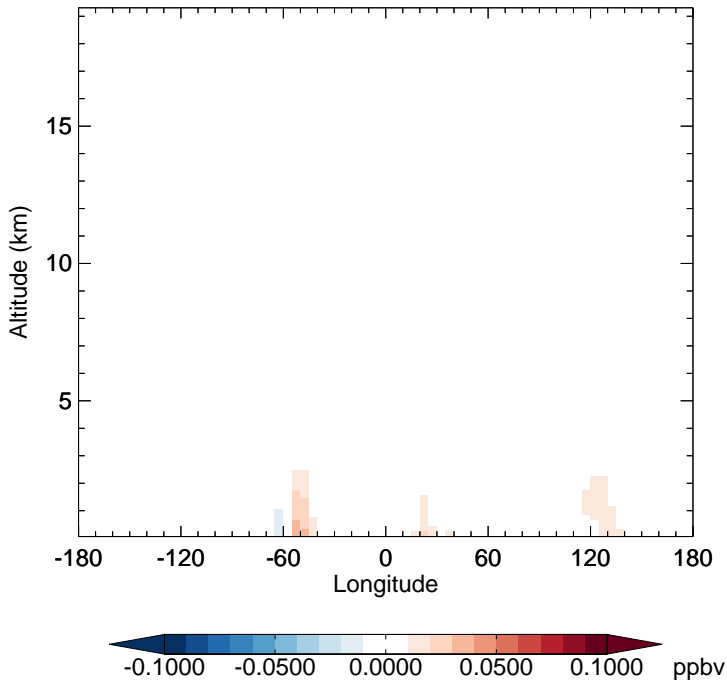
v11-02c - v11-02a TSOG3 - Diff along 15S for Oct
