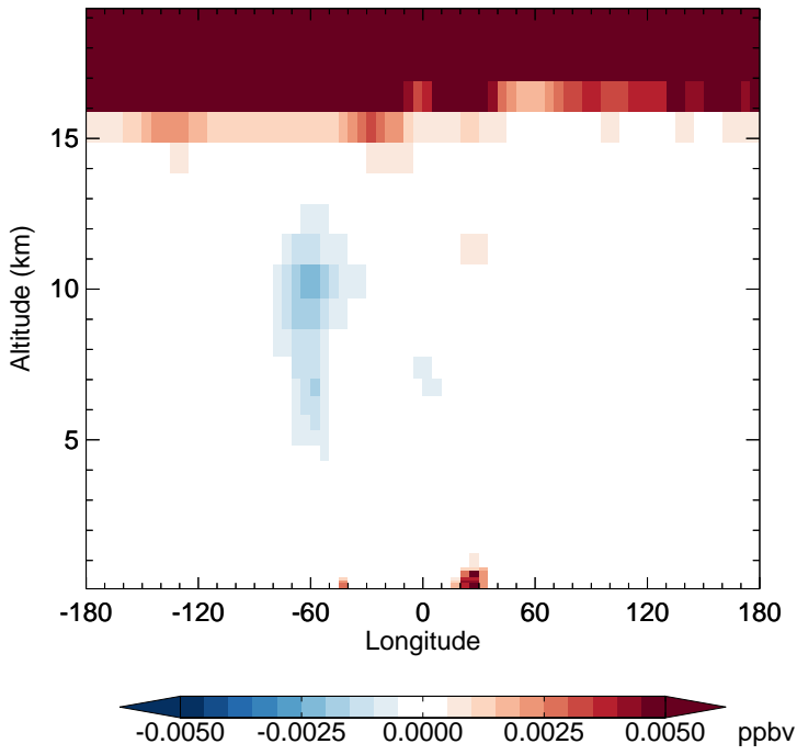
v11-02c - v11-02a N2O5 - Diff along 15S for Oct
