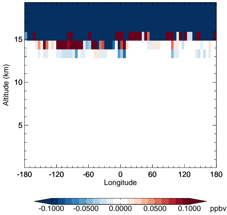
v11-02c - v11-02a H2O - Diff along 15S for Oct
