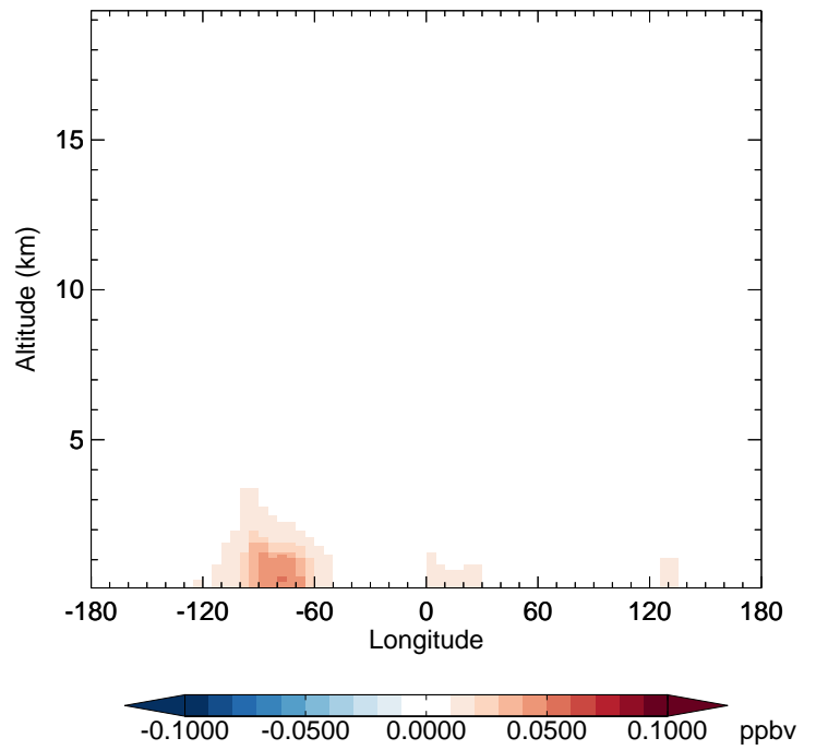
v11-02c - v11-01-public-Run0 IONITA - Diff along 42N for Oct
