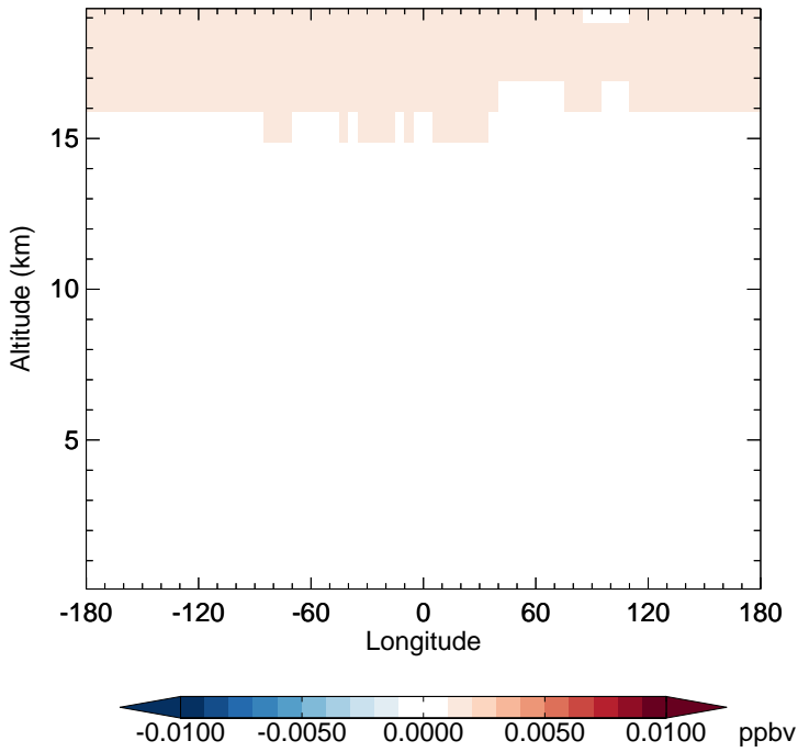
v11-02c - v11-01-public-Run0 BrNO3 - Diff along 15S for Oct
