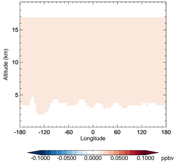
v11-02c - v11-02a HCFC141b - Diff along 42N for Oct
