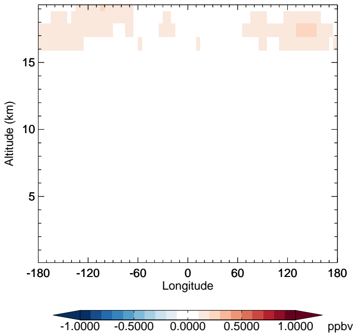
v11-02c - v11-01-public-Run0 NO 2 - Diff along 15S for Oct
