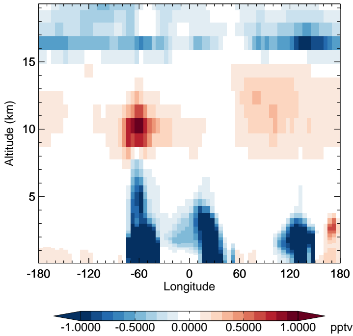
v11-02c - v11-01-public-Run0 HO2 - Diff along 15S for Oct
