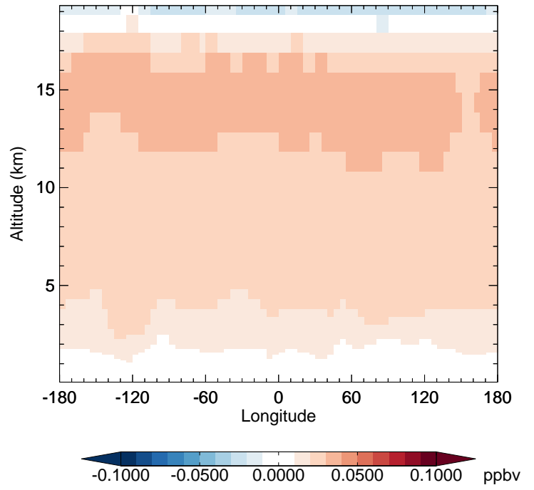
v11-02c - v11-02a CH3Cl - Diff along 42N for Oct
