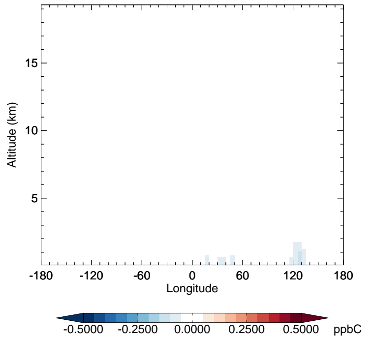
v11-02c - v11-01-public-Run0 C3H8 - Diff along 42N for Oct
