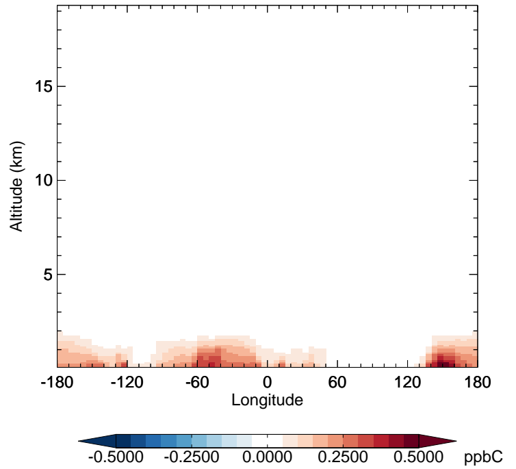
v11-02c - v11-01-public-Run0 ALD2 - Diff along 42N for Oct
