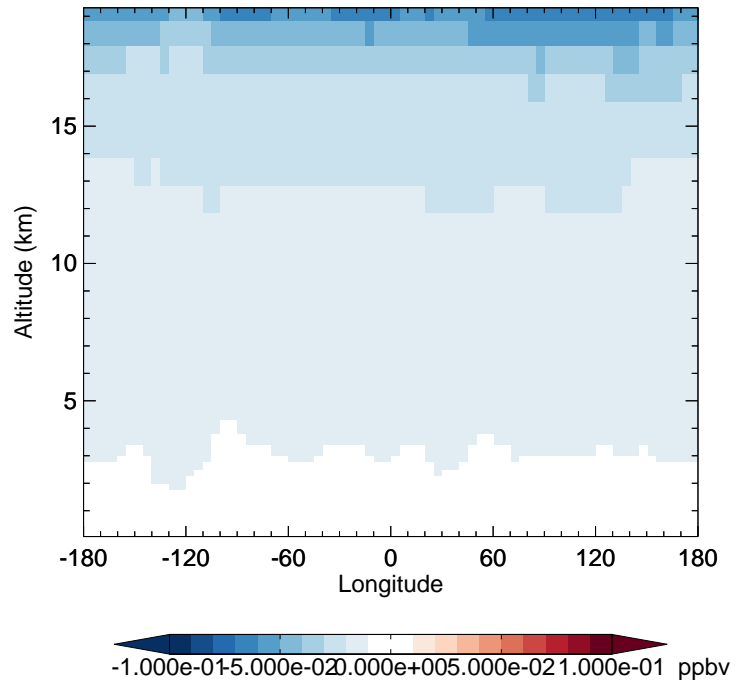
v11-02c - v11-01-public-Run0 CFC12 - Diff along 42N for Oct
