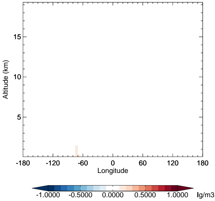
v11-02c - v11-02a SO 2 - Diff along 15S for Oct
