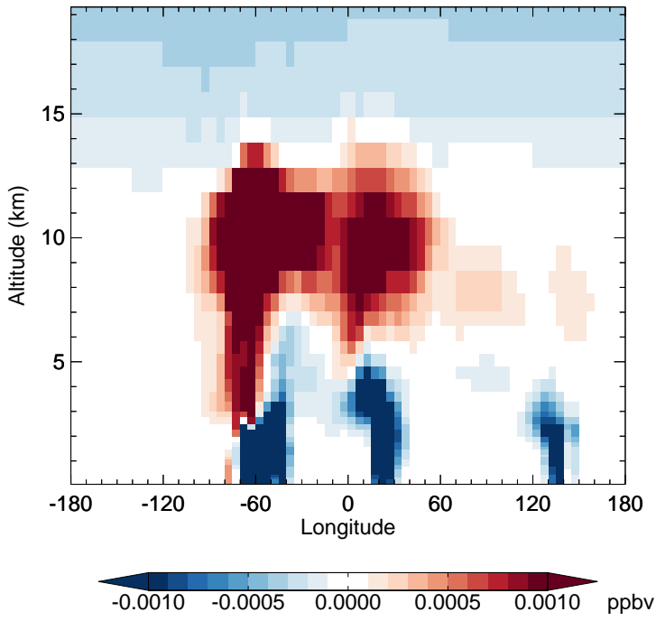
v11-02c - v11-02a PPN - Diff along 15S for Oct
