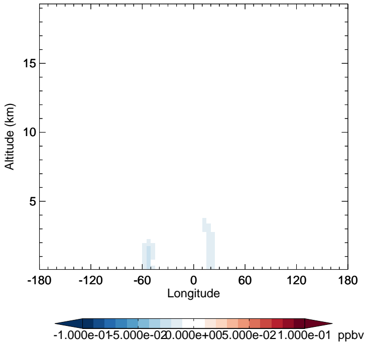
v11-02c - v11-01-public-Run0 ISOA2 - Diff along 15S for Oct
