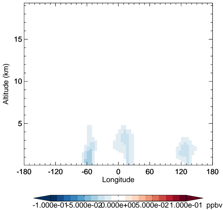
v11-02c - v11-01-public-Run0 PROPNN - Diff along 15S for Oct
