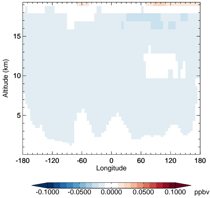
v11-02c - v11-02a CFC12 - Diff along 15S for Oct
