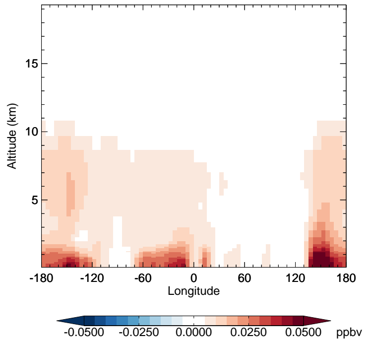
v11-02c - v11-01-public-Run0 MP - Diff along 42N for Oct
