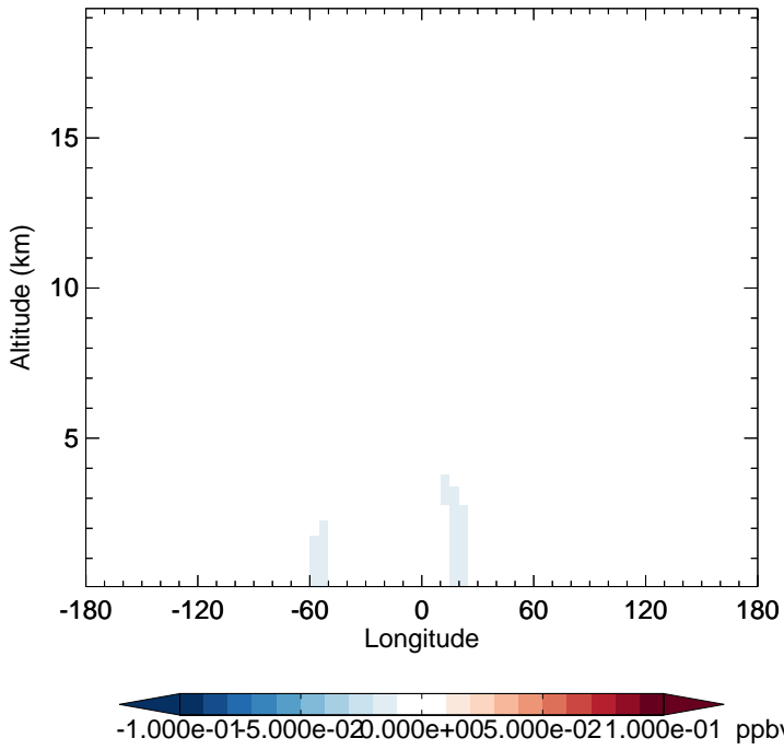
v11-02c - v11-02a ISOA2 - Diff along 15S for Oct
