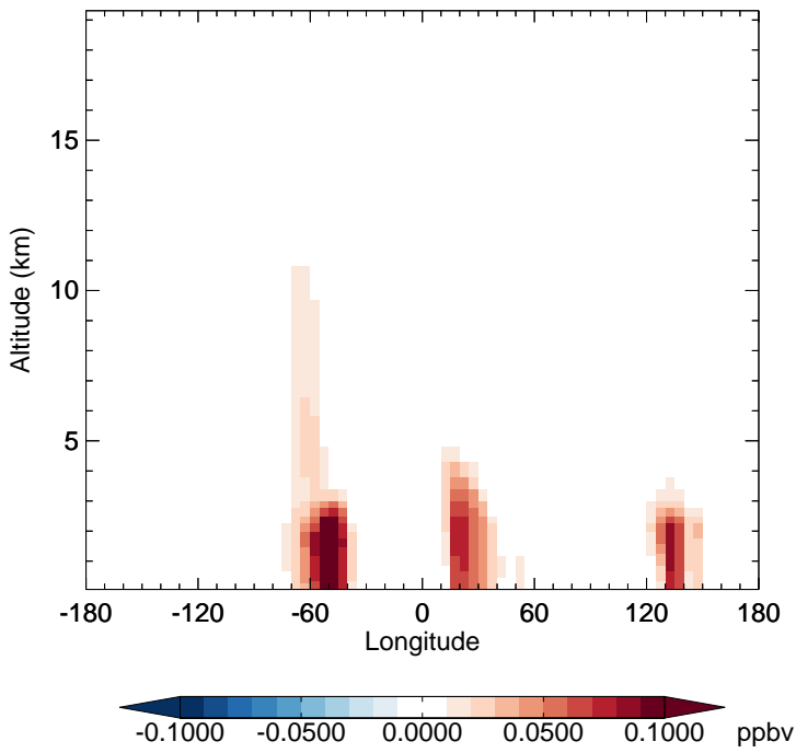
v11-02c - v11-02a HC187 - Diff along 15S for Oct
