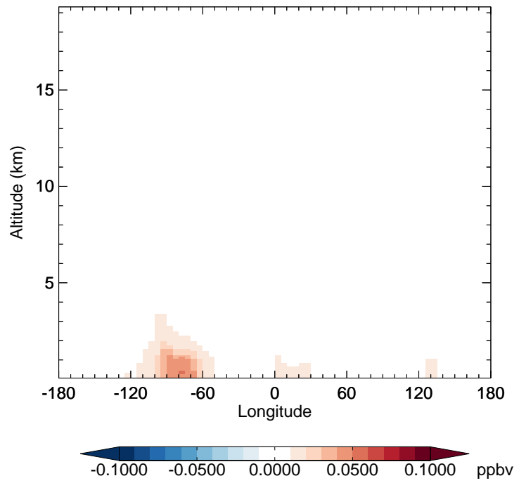
v11-02c - v11-02a IONITA - Diff along 42N for Oct
