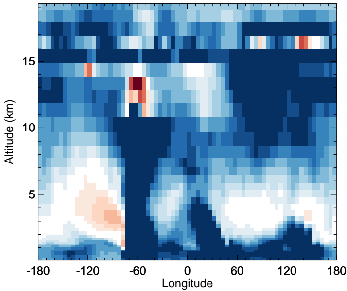
v11-02c - v11-01-public-Run0 OH - Diff along 15S for Oct
