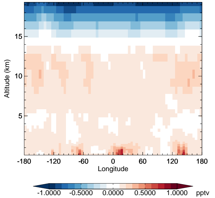
v11-02c - v11-01-public-Run0 HO2 - Diff along 42N for Oct
