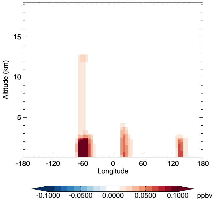
v11-02c - v11-02a IPMN - Diff along 15S for Oct
