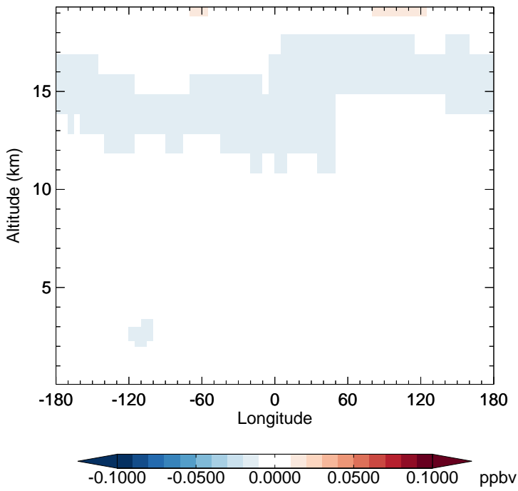
v11-02c - v11-02a CFC11 - Diff along 15S for Oct
