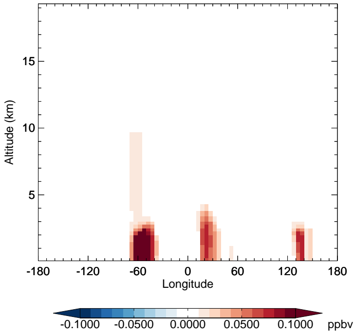
v11-02c - v11-01-public-Run0 IEPOXB - Diff along 15S for Oct
