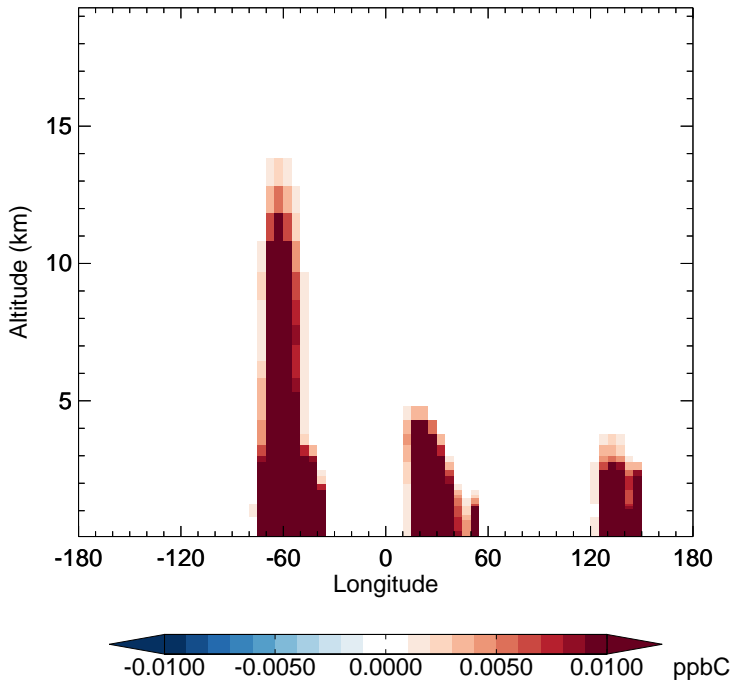
v11-02c - v11-01-public-Run0 PRPE - Diff along 15S for Oct
