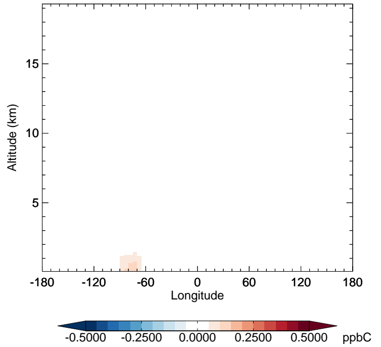
v11-02c - v11-02a ALD2 - Diff along 42N for Oct
