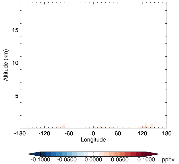
v11-02c - v11-02a GLYX - Diff along 42N for Oct
