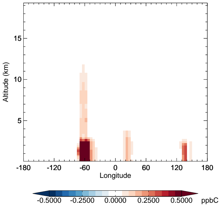
v11-02c - v11-02a ISOP - Diff along 15S for Oct
