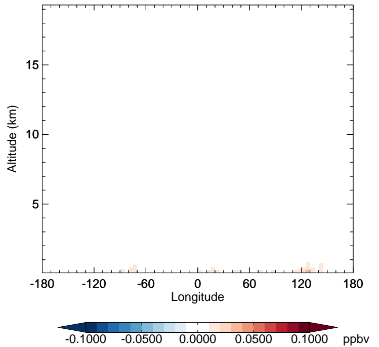
v11-02c - v11-01-public-Run0 GLYX - Diff along 42N for Oct
