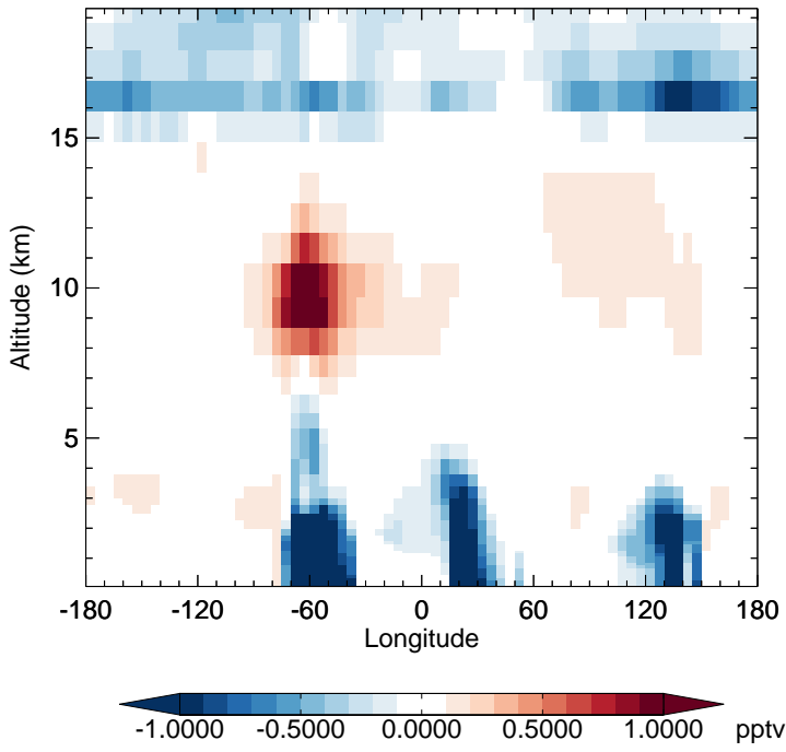
v11-02c - v11-02a HO2 - Diff along 15S for Oct
