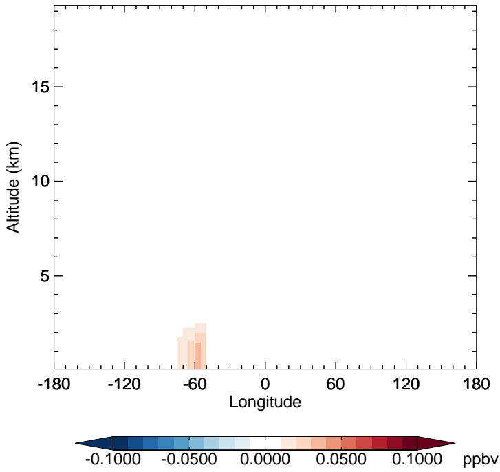
v11-02c - v11-02a TOLU - Diff along 15S for Oct
