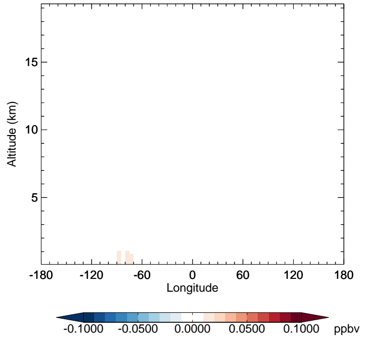
v11-02c - v11-02a IPMN - Diff along 42N for Oct
