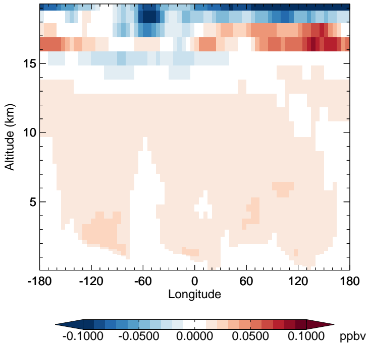
v11-02c - v11-01-public-Run0 HCl - Diff along 15S for Oct
