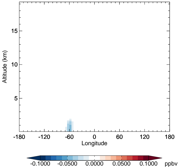
v11-02c - v11-01-public-Run0 ISOA1 - Diff along 15S for Oct
