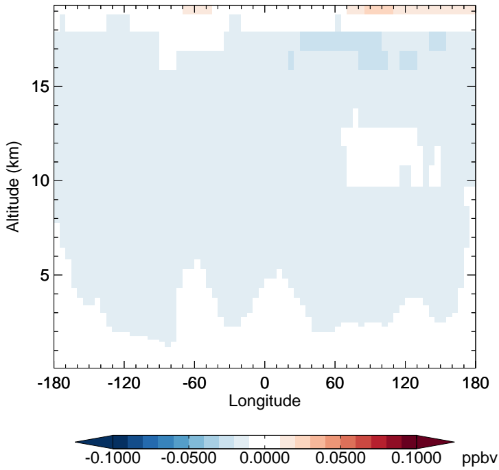
v11-02c - v11-01-public-Run0 CFC12 - Diff along 15S for Oct
