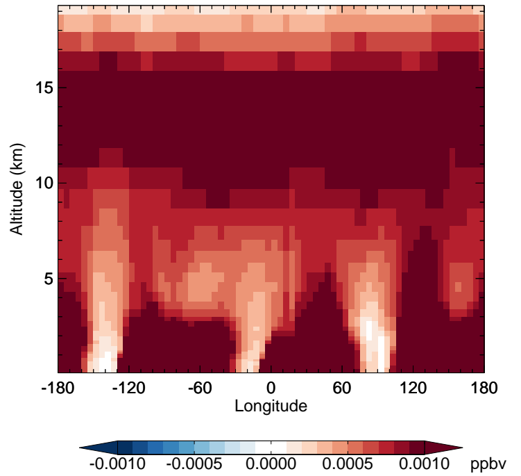
v11-02c - v11-01-public-Run0 PPN - Diff along 42N for Oct
