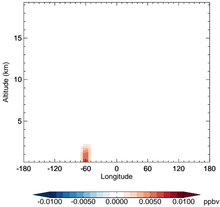
v11-02c - v11-01-public-Run0 MOBA - Diff along 15S for Oct
