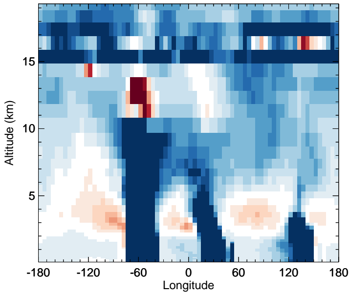
v11-02c - v11-02a OH - Diff along 15S for Oct
