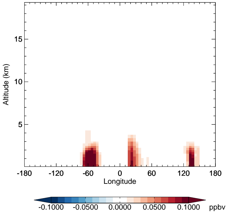
v11-02c - v11-02a MGLY - Diff along 15S for Oct
