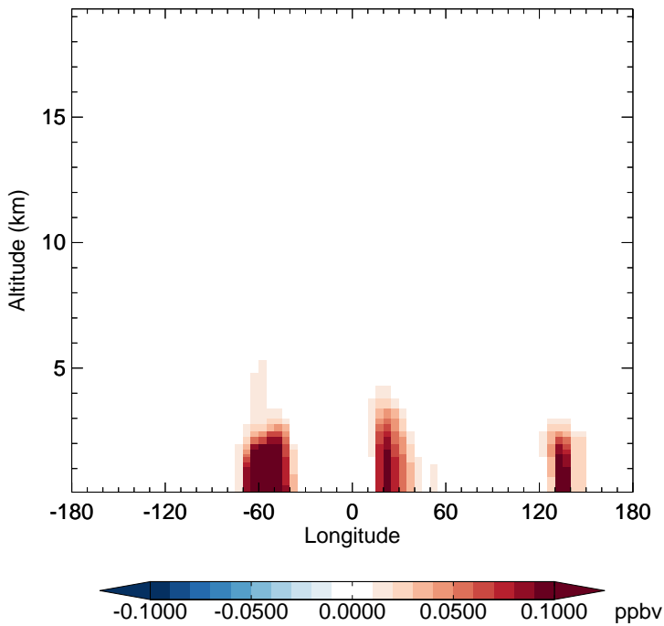
v11-02c - v11-01-public-Run0 MGLY - Diff along 15S for Oct
