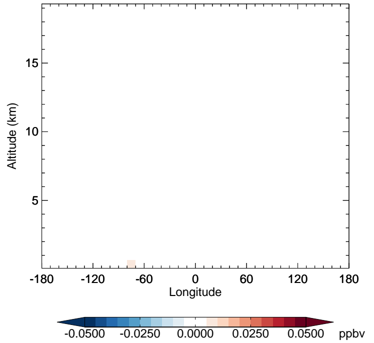
v11-02c - v11-02a MACR - Diff along 42N for Oct
