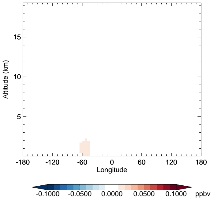
v11-02c - v11-01-public-Run0 IEPOXD - Diff along 15S for Oct
