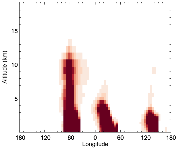
v11-02c - v11-01-public-Run0 EOH - Diff along 15S for Oct
