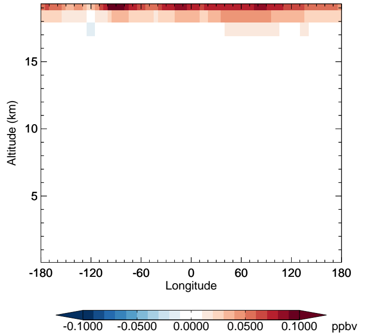
v11-02c - v11-01-public-Run0 CINO3 - Diff along 42N for Oct
