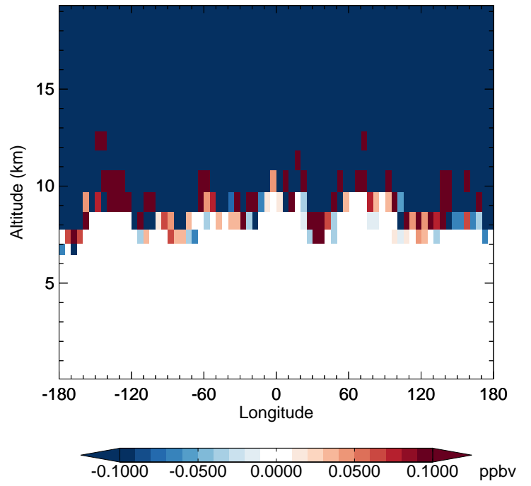
v11-02c - v11-02a H2O - Diff along 42N for Oct
