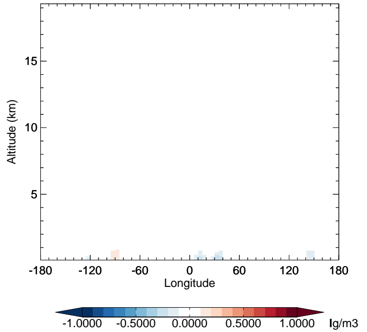
v11-02c - v11-01-public-Run0 NH4 - Diff along 42N for Oct
