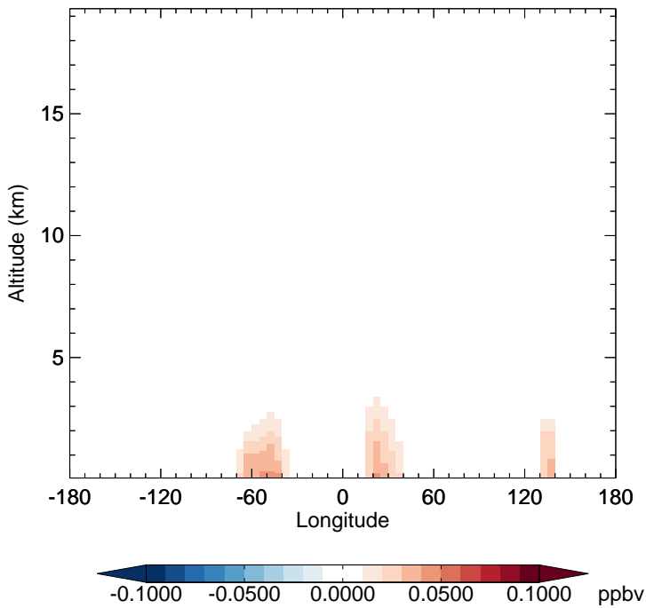
v11-02c - v11-01-public-Run0 GLYX - Diff along 15S for Oct
