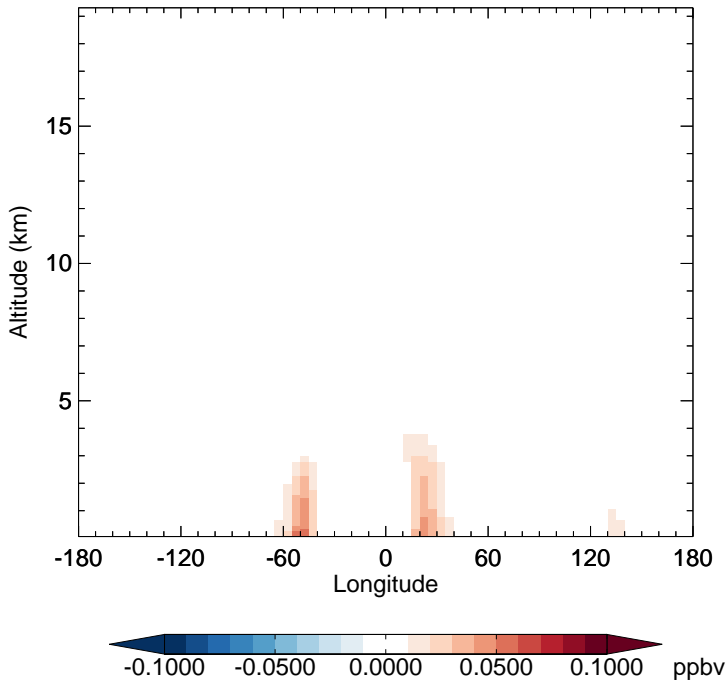
v11-02c - v11-02a MONITA - Diff along 15S for Oct
