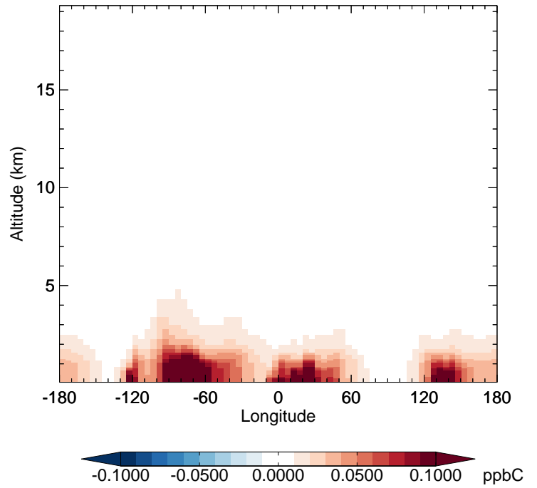
v11-02c - v11-01-public-Run0 MEK - Diff along 42N for Oct
