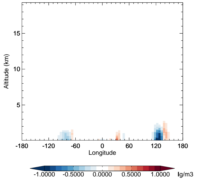
v11-02c - v11-01-public-Run0 NIT - Diff along 42N for Oct
