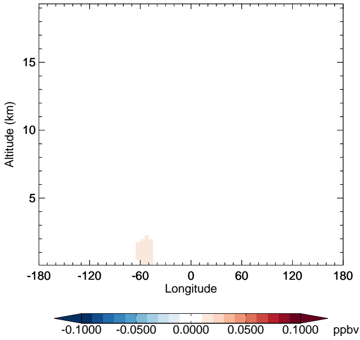
v11-02c - v11-02a IEPOXD - Diff along 15S for Oct
