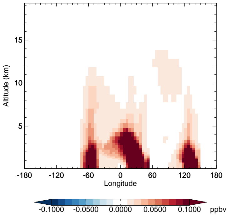
v11-02c - v11-01-public-Run0 BENZ - Diff along 15S for Oct
