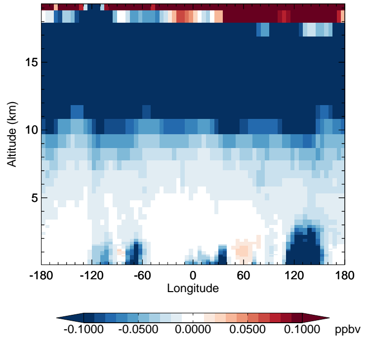
v11-02c - v11-01-public-Run0 HNO 3 - Diff along 42N for Oct
