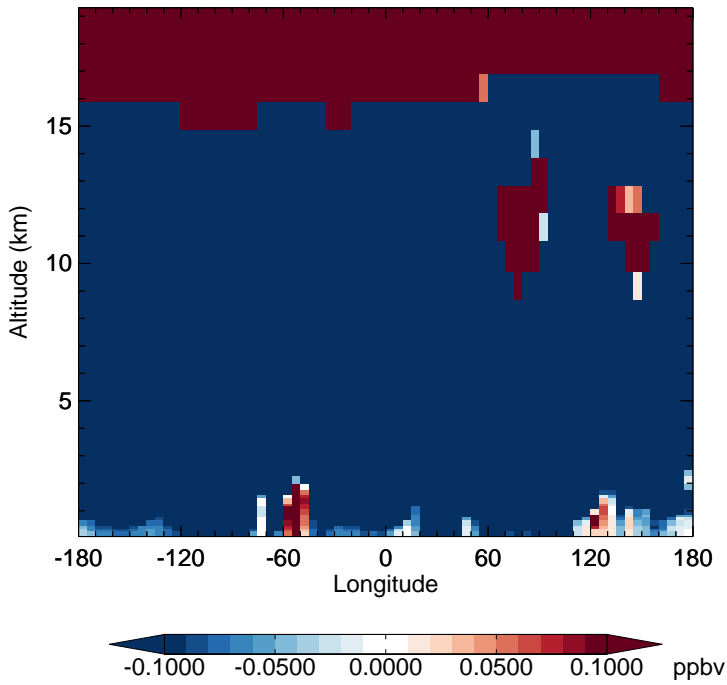
v11-02c - v11-01-public-Run0 CH4 - Diff along 15S for Oct
