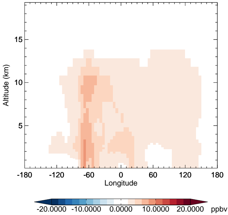
v11-02c - v11-02a CO - Diff along 15S for Oct
