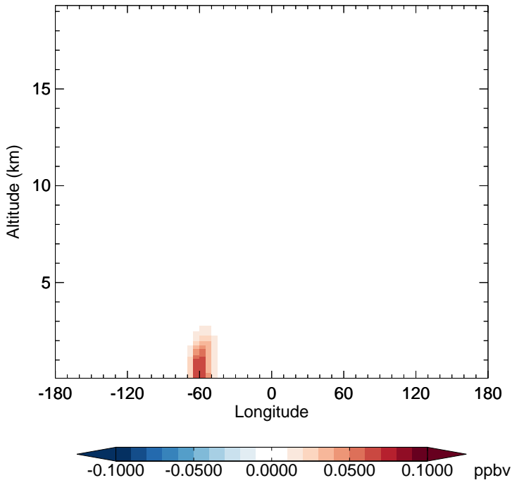
v11-02c - v11-02a TSOA0 - Diff along 15S for Oct
