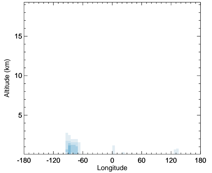
v11-02c - v11-02a HAC - Diff along 42N for Oct
