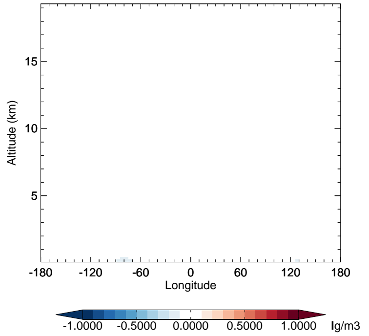
v11-02c - v11-02a NH4 - Diff along 42N for Oct
