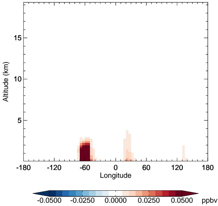
v11-02c - v11-02a RCHO - Diff along 15S for Oct
