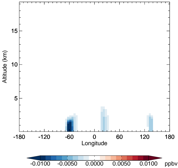
v11-02c - v11-01-public-Run0 MACRN - Diff along 15S for Oct
