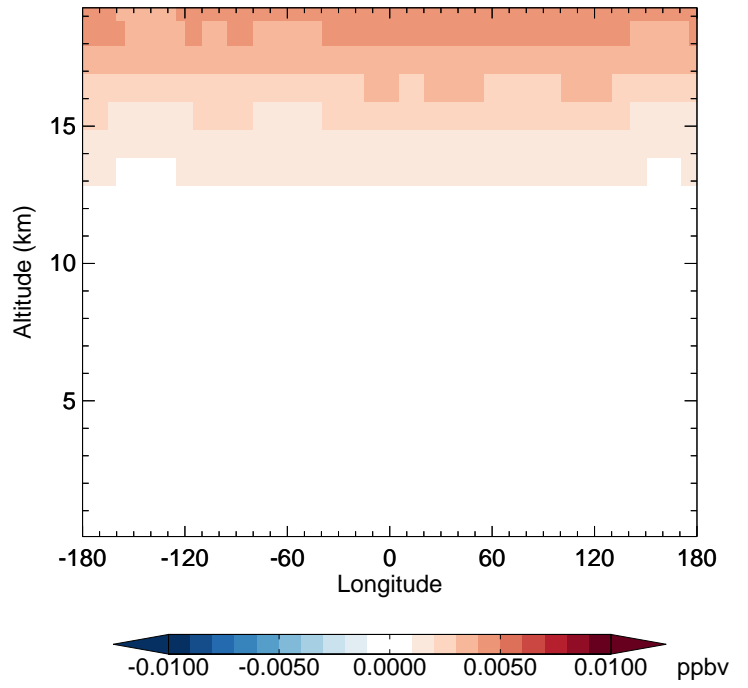
v11-02c - v11-02a BrNO3 - Diff along 42N for Oct
