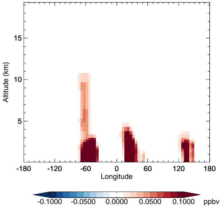
v11-02c - v11-01-public-Run0 IEPOXA - Diff along 15S for Oct
