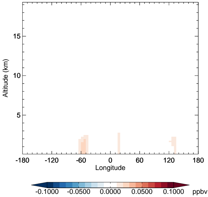
v11-02c - v11-02a LVOCOA - Diff along 15S for Oct
