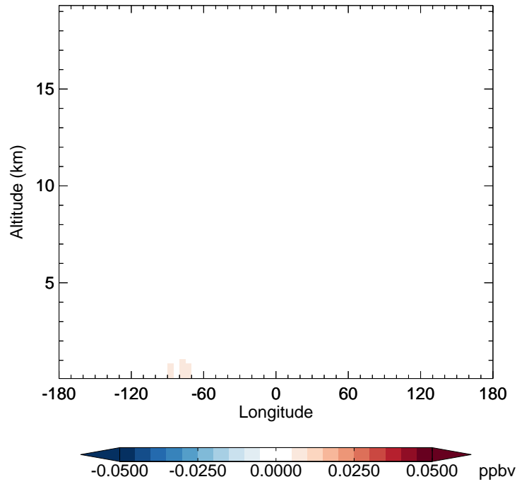
v11-02c - v11-02a MVK - Diff along 42N for Oct
