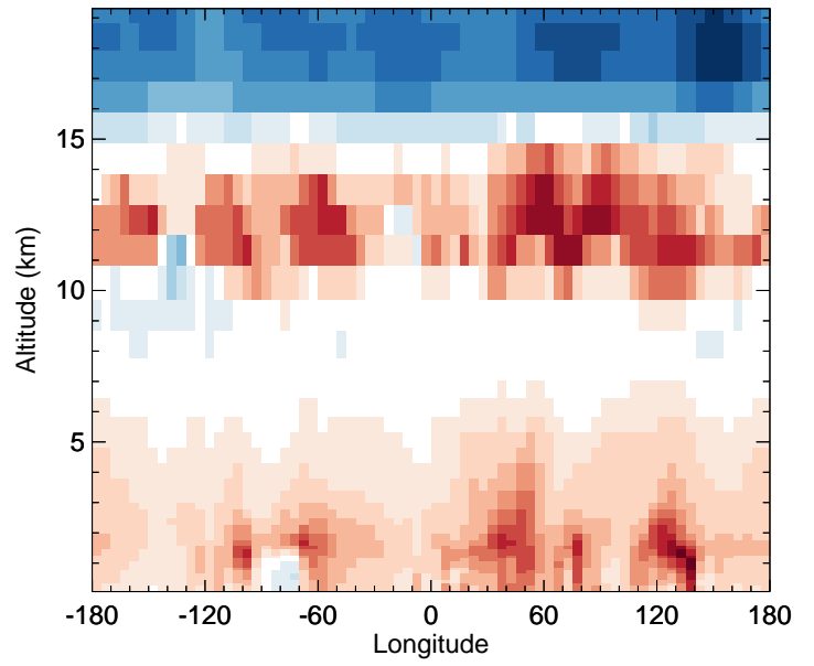
v11-02c - v11-02a OH - Diff along 42N for Oct
