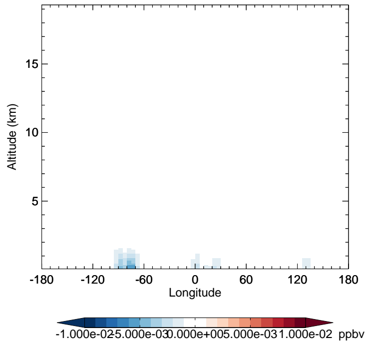
v11-02c - v11-01-public-Run0 NPMN - Diff along 42N for Oct
