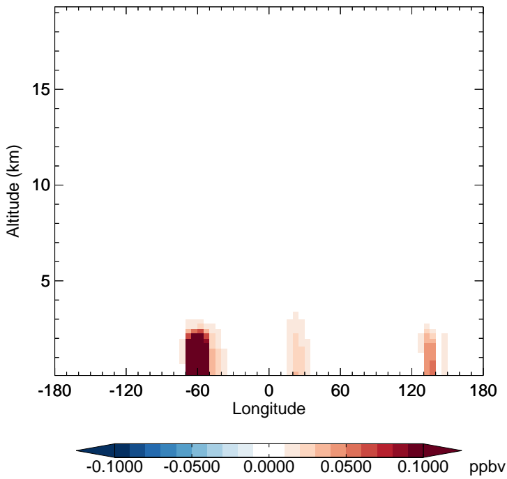
v11-02c - v11-01-public-Run0 HPALD - Diff along 15S for Oct
