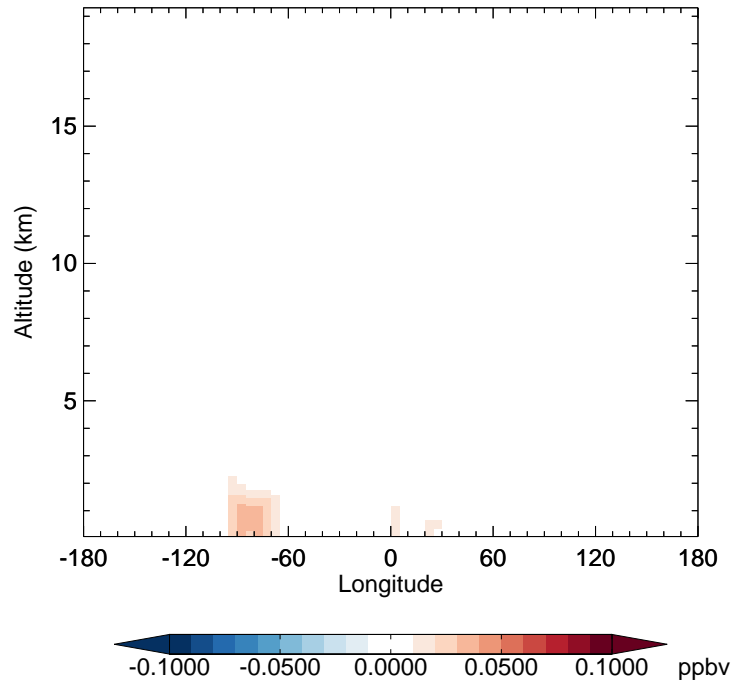
v11-02c - v11-02a IMAE - Diff along 42N for Oct
