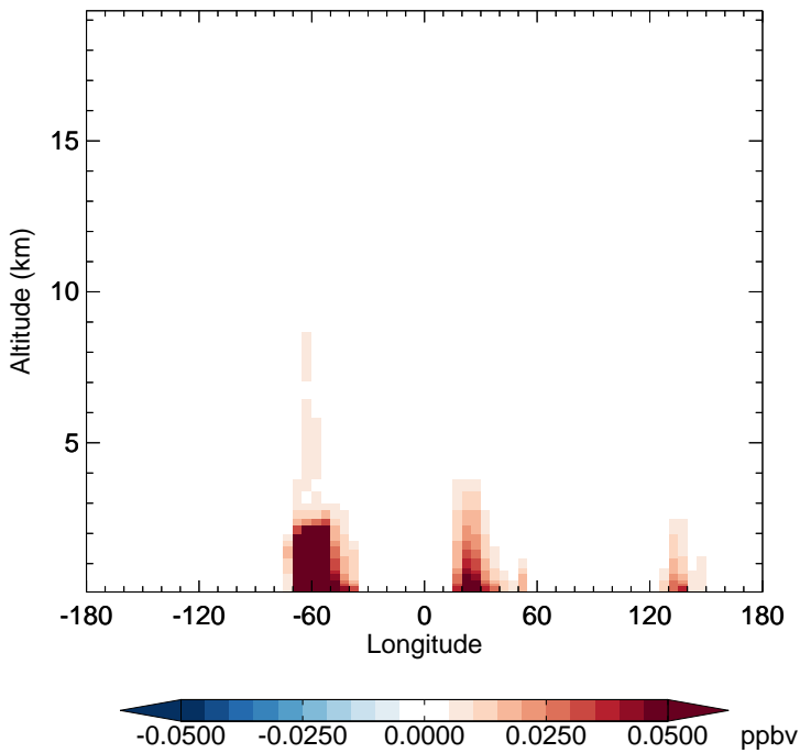
v11-02c - v11-01-public-Run0 RCHO - Diff along 15S for Oct
