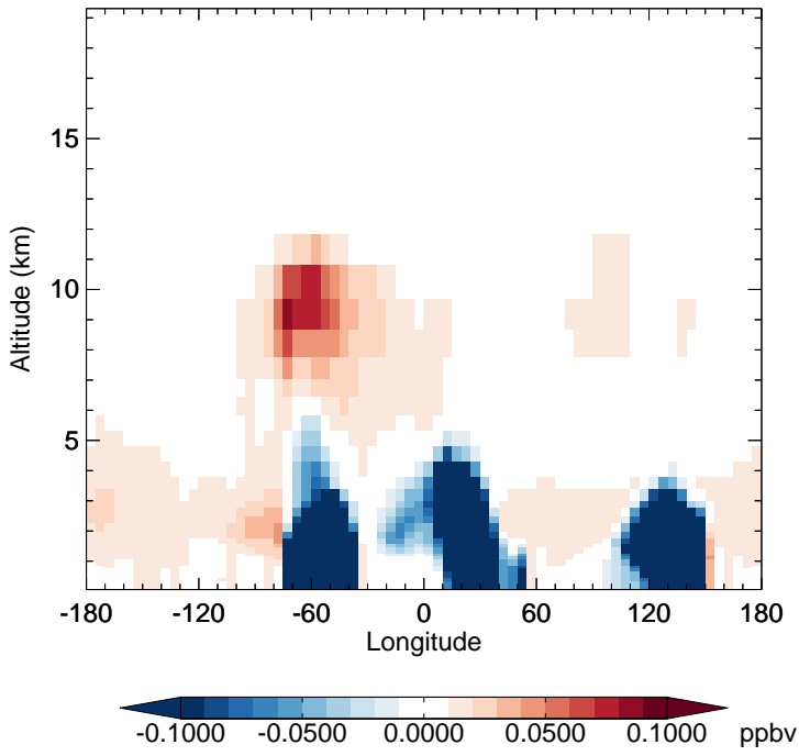
v11-02c - v11-02a H2O2 - Diff along 15S for Oct
