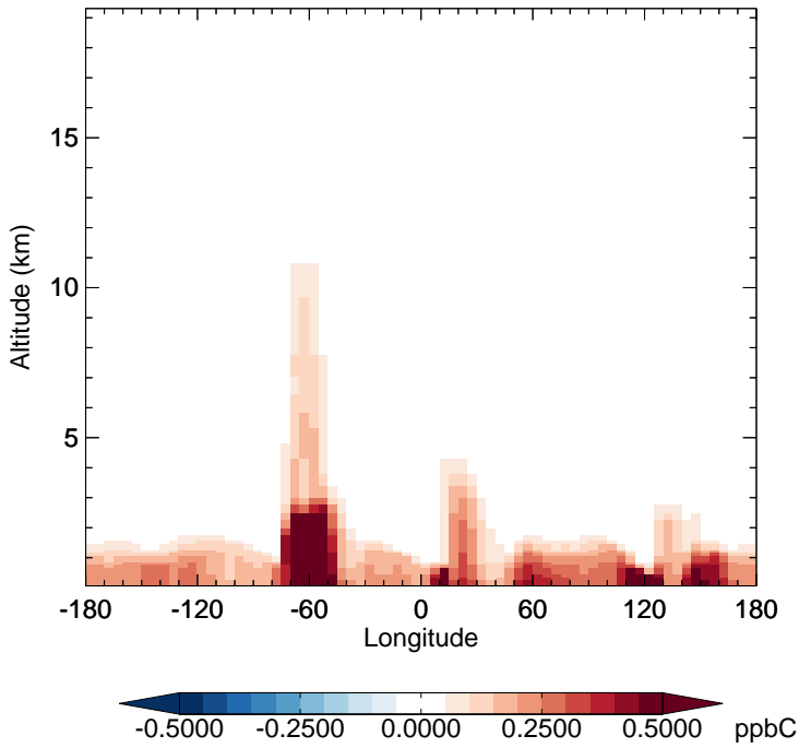
v11-02c - v11-01-public-Run0 ALD2 - Diff along 15S for Oct
