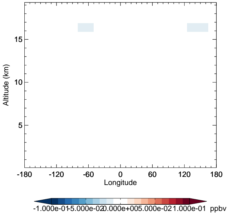
v11-02c - v11-02a ClO - Diff along 15S for Oct
