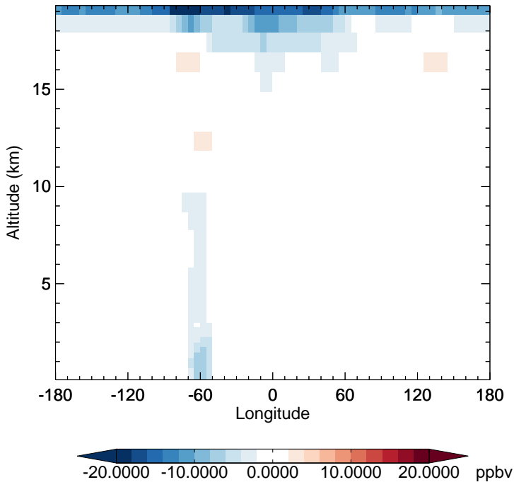
v11-02c - v11-02a O3 - Diff along 15S for Oct
