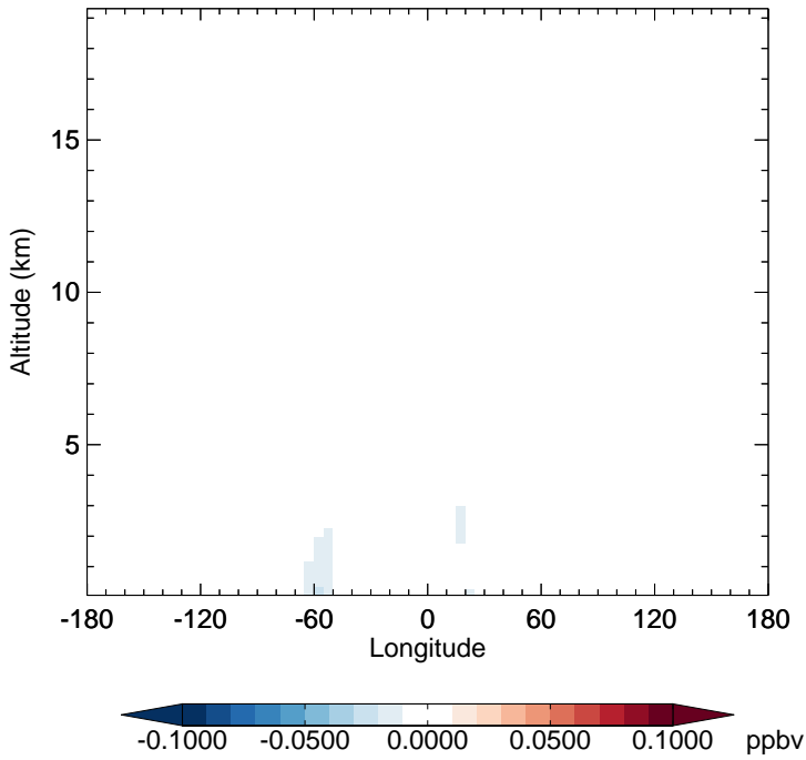
v11-02c - v11-01-public-Run0 TSOA3 - Diff along 15S for Oct
