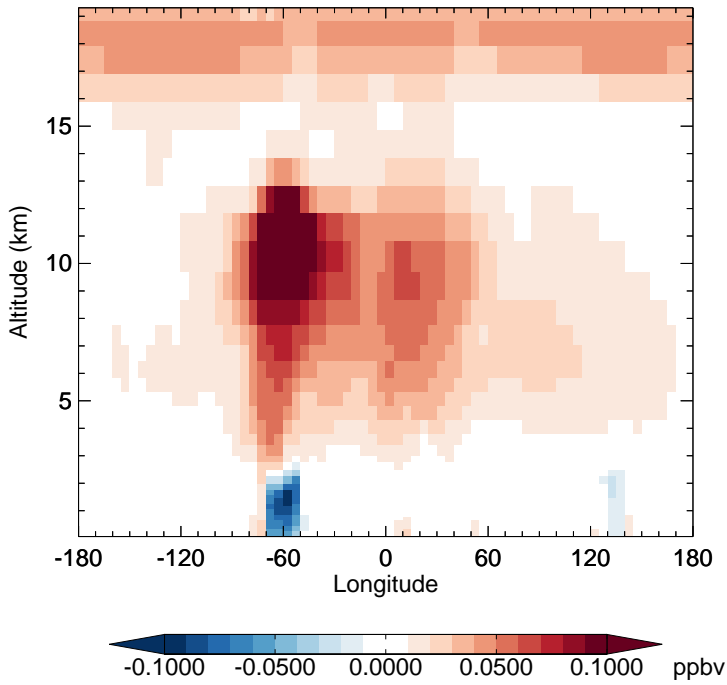
v11-02c - v11-01-public-Run0 PAN - Diff along 15S for Oct
