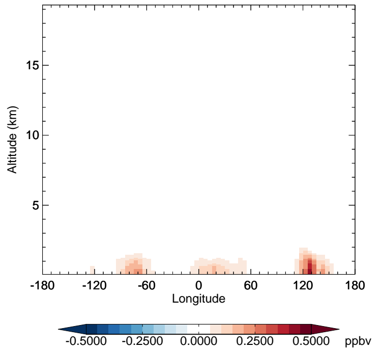
v11-02c - v11-01-public-Run0 CH 2 O - Diff along 42N for Oct
