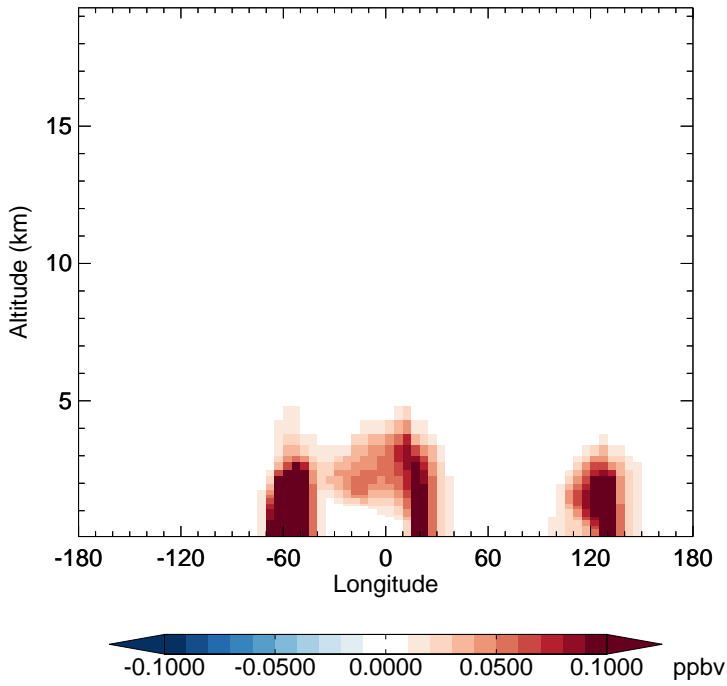
v11-02c - v11-02a SOAGX - Diff along 15S for Oct
