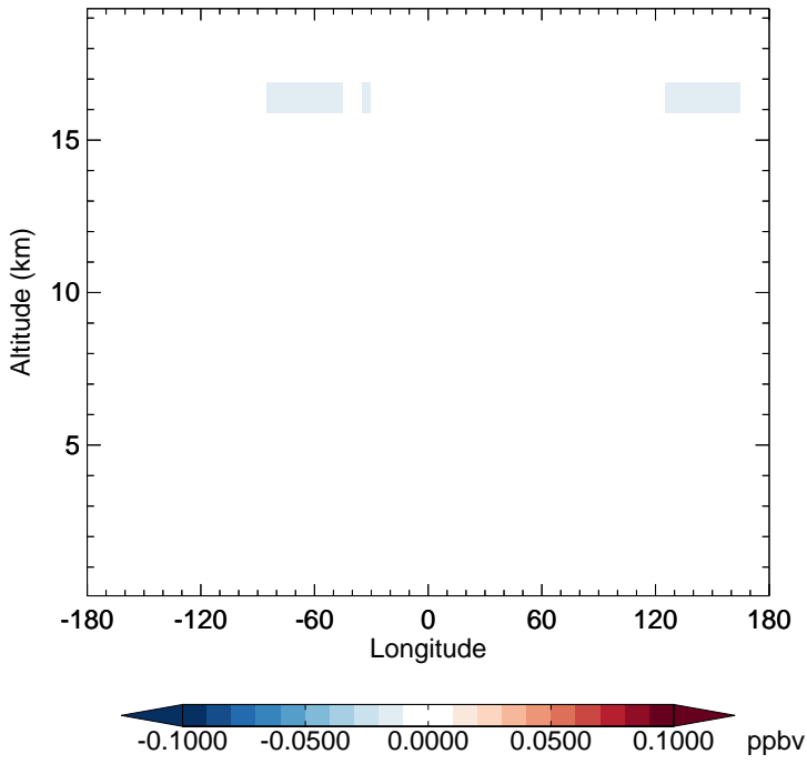
v11-02c - v11-02a HOCl - Diff along 15S for Oct
