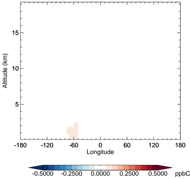
v11-02c - v11-02a ALK4 - Diff along 15S for Oct
