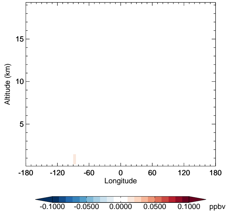
v11-02c - v11-02a IEPOXA - Diff along 42N for Oct
