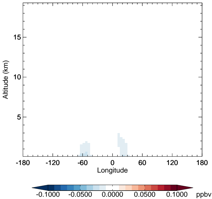
v11-02c - v11-01-public-Run0 TSOG2 - Diff along 15S for Oct
