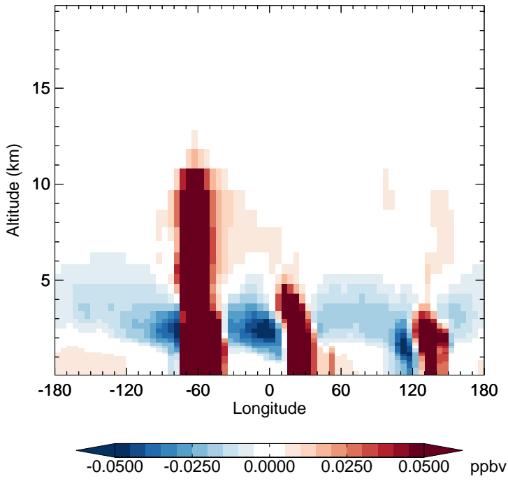
v11-02c - v11-02a MP - Diff along 15S for Oct
