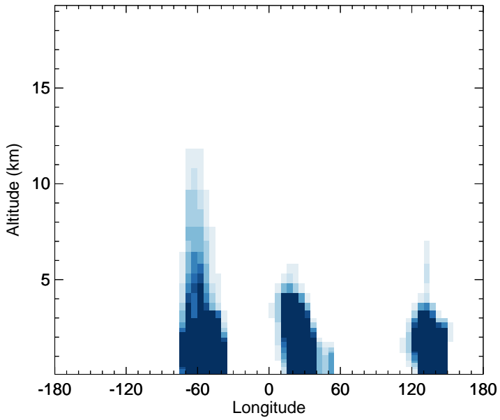
v11-02c - v11-02a HAC - Diff along 15S for Oct
