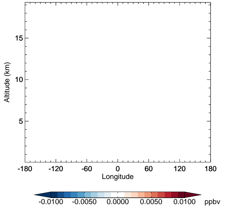
v11-02c - v11-02a HOBr - Diff along 42N for Oct
