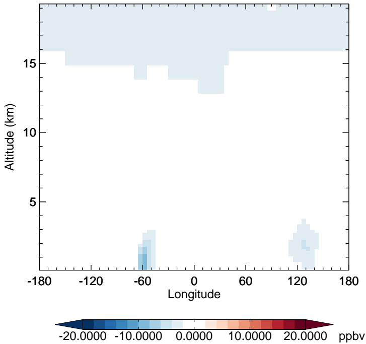
v11-02c - v11-01-public-Run0 CO - Diff along 15S for Oct
