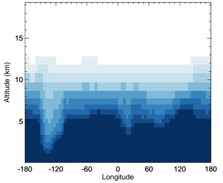
v11-02c - v11-02a R4N2 - Diff along 42N for Oct
