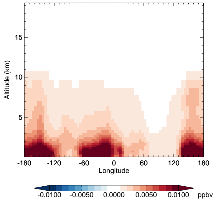
v11-02c - v11-01-public-Run0 MAP - Diff along 42N for Oct
