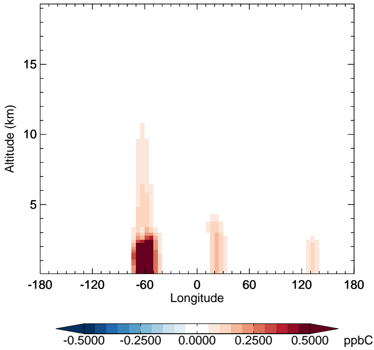
v11-02c - v11-02a ALD2 - Diff along 15S for Oct
