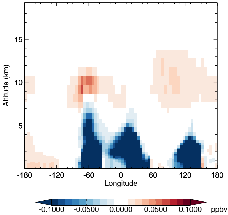
v11-02c - v11-01-public-Run0 H2O2 - Diff along 15S for Oct
