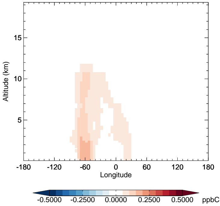
v11-02c - v11-02a ACET - Diff along 15S for Oct
