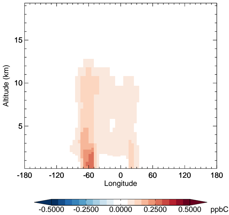
v11-02c - v11-01-public-Run0 ACET - Diff along 15S for Oct
