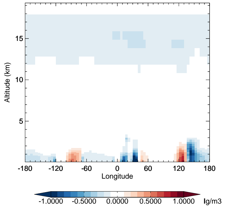
v11-02c - v11-01-public-Run0 SO4 - Diff along 42N for Oct
