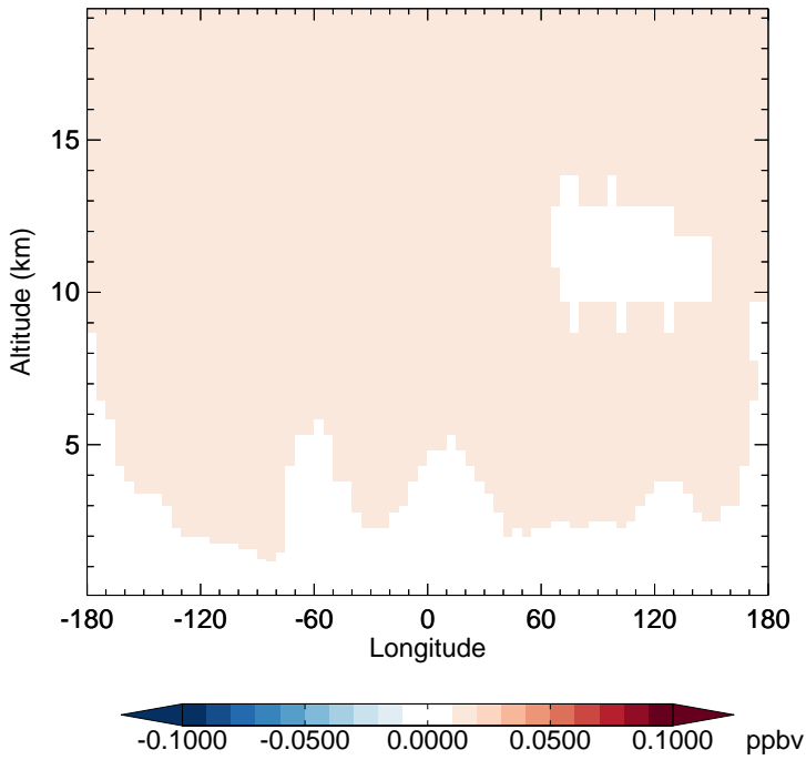
v11-02c - v11-01-public-Run0 HCFC141b - Diff along 15S for Oct
