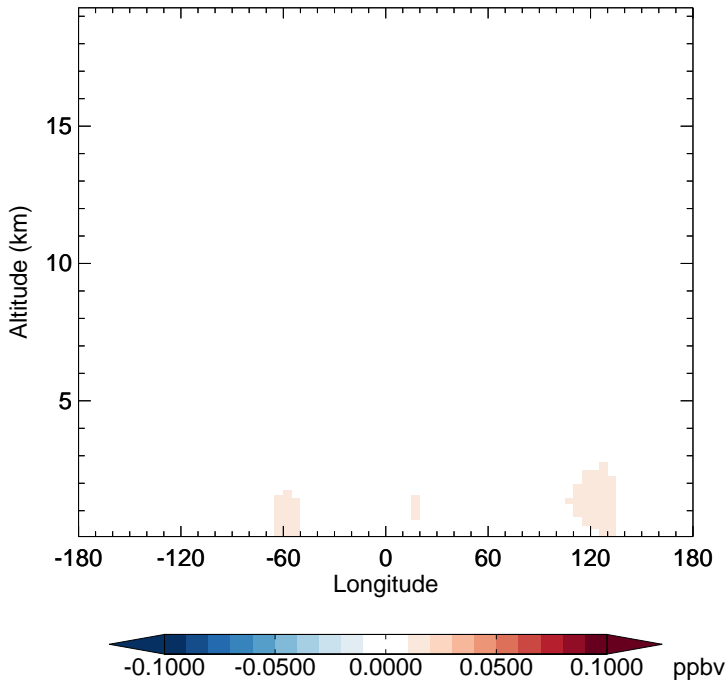
v11-02c - v11-01-public-Run0 SOAME - Diff along 15S for Oct
