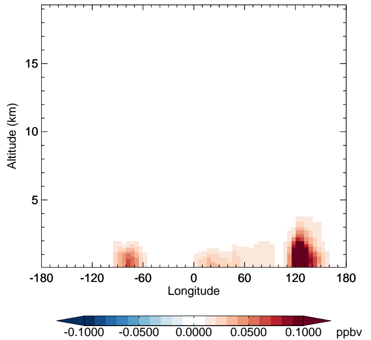
v11-02c - v11-01-public-Run0 SOAGX - Diff along 42N for Oct
