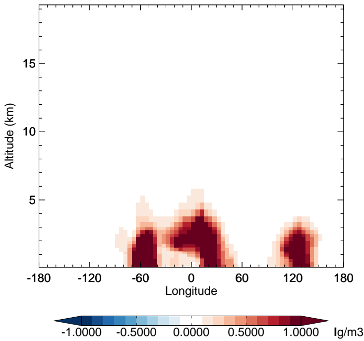
v11-02c - v11-01-public-Run0 SOAS - Diff along 15S for Oct
