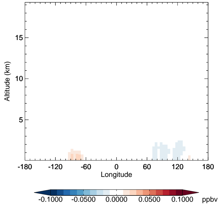
v11-02c - v11-02a MGLY - Diff along 42N for Oct
