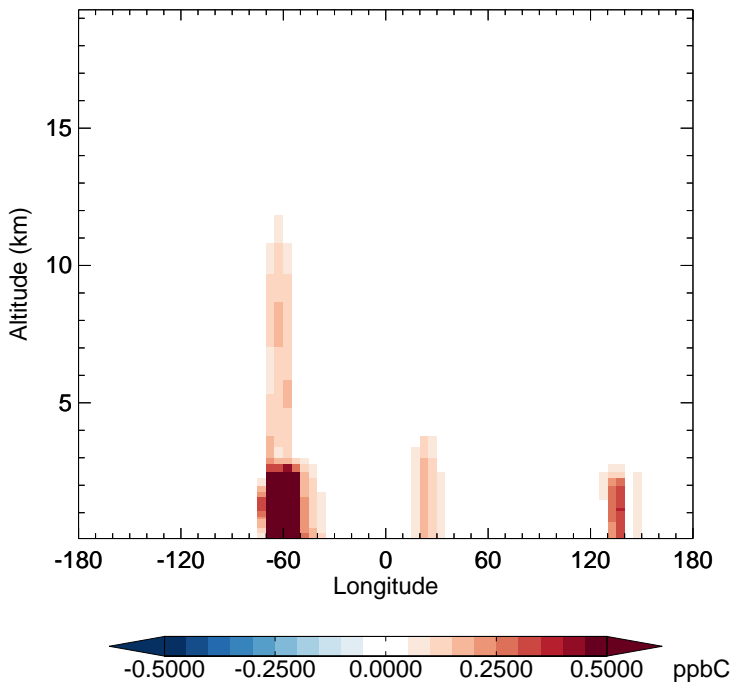
v11-02c - v11-01-public-Run0 ISOP - Diff along 15S for Oct
