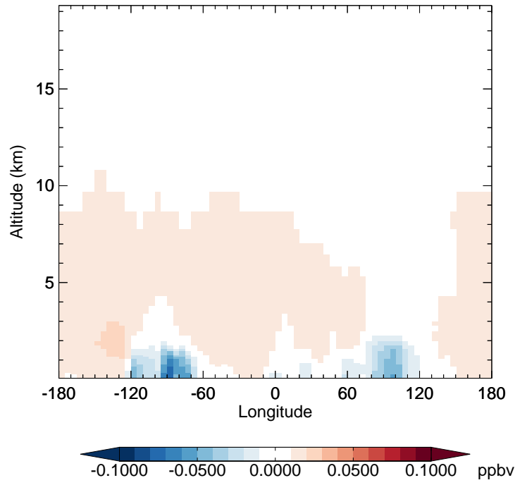
v11-02c - v11-02a H2O2 - Diff along 42N for Oct
