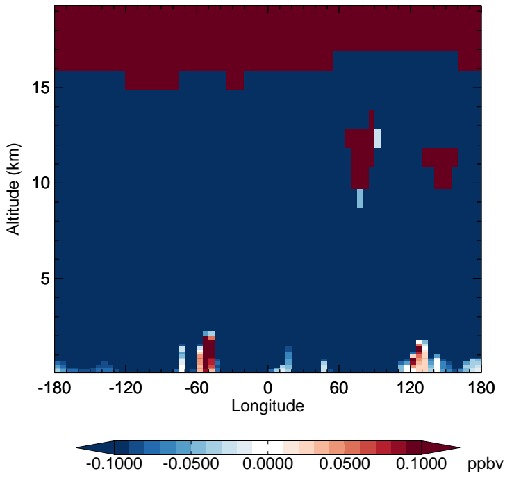
v11-02c - v11-02a CH4 - Diff along 15S for Oct
