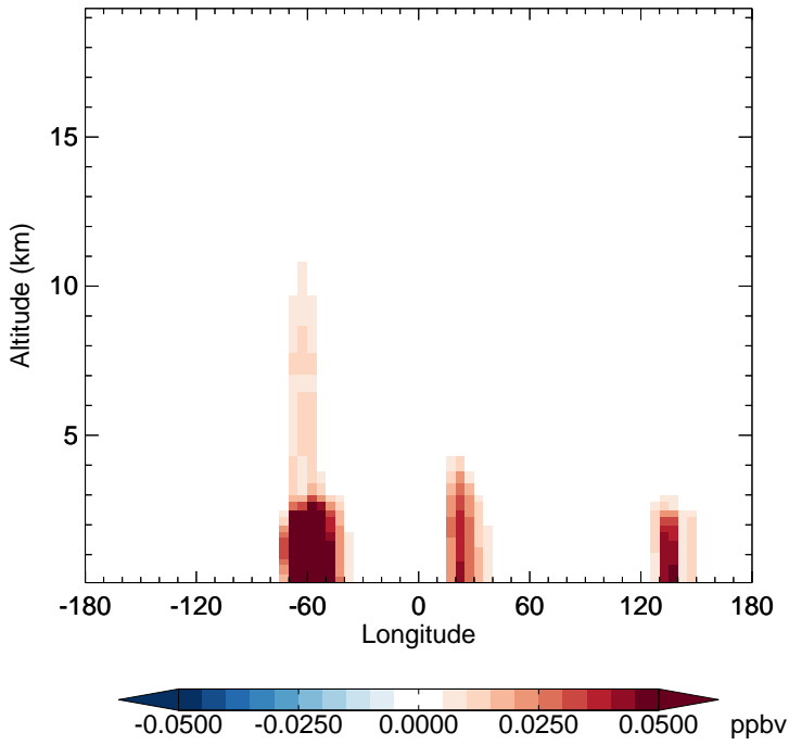
v11-02c - v11-02a MACR - Diff along 15S for Oct
