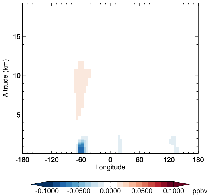
v11-02c - v11-01-public-Run0 ISO3 - Diff along 15S for Oct
