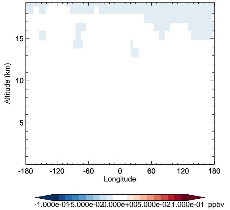
v11-02c - v11-01-public-Run0 CCI4 - Diff along 42N for Oct
