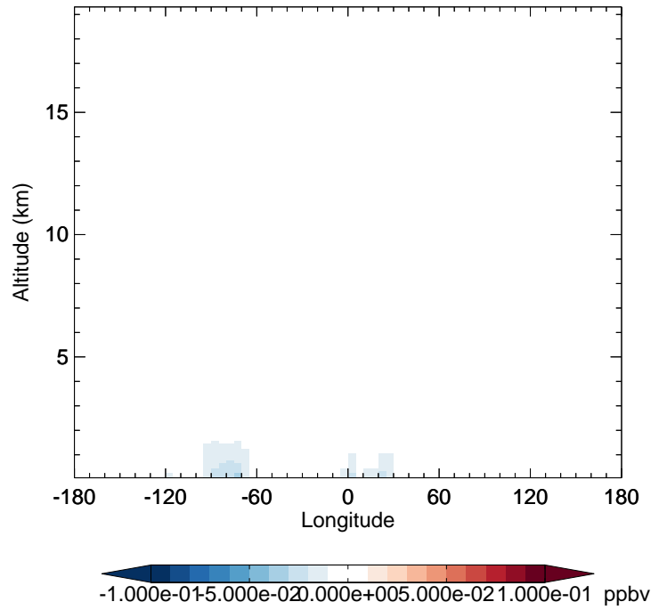
v11-02c - v11-01-public-Run0 TSOG3 - Diff along 42N for Oct
