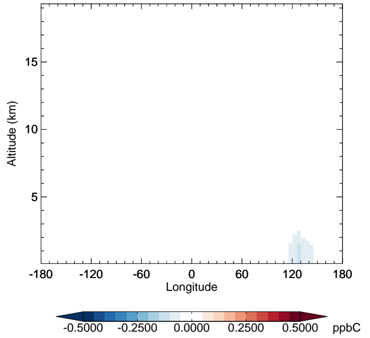
v11-02c - v11-02a ALK4 - Diff along 42N for Oct
