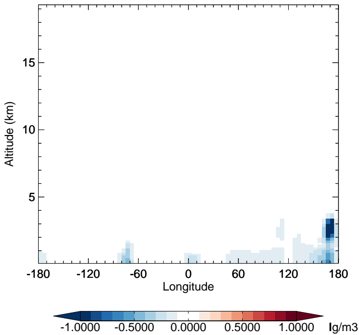
v11-02c - v11-01-public-Run0 SO4 - Diff along 15S for Oct
