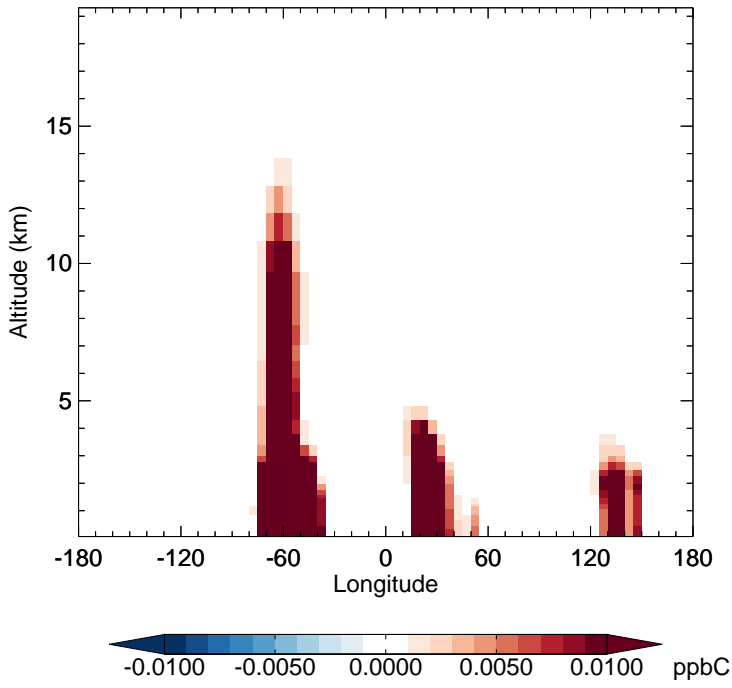
v11-02c - v11-02a PRPE - Diff along 15S for Oct
