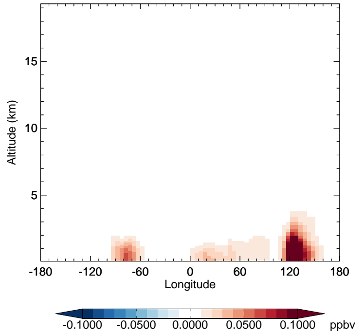
v11-02c - v11-02a SOAGX - Diff along 42N for Oct
