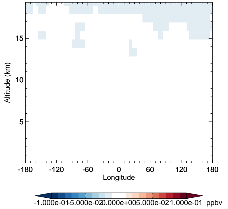
v11-02c - v11-02a CCI4 - Diff along 42N for Oct
