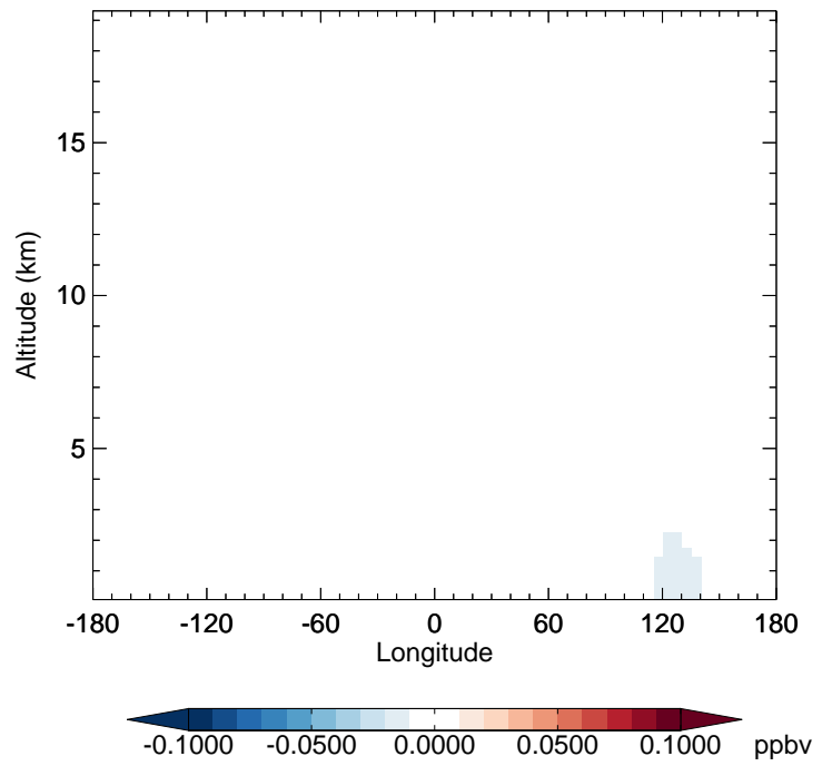
v11-02c - v11-02a BENZ - Diff along 42N for Oct
