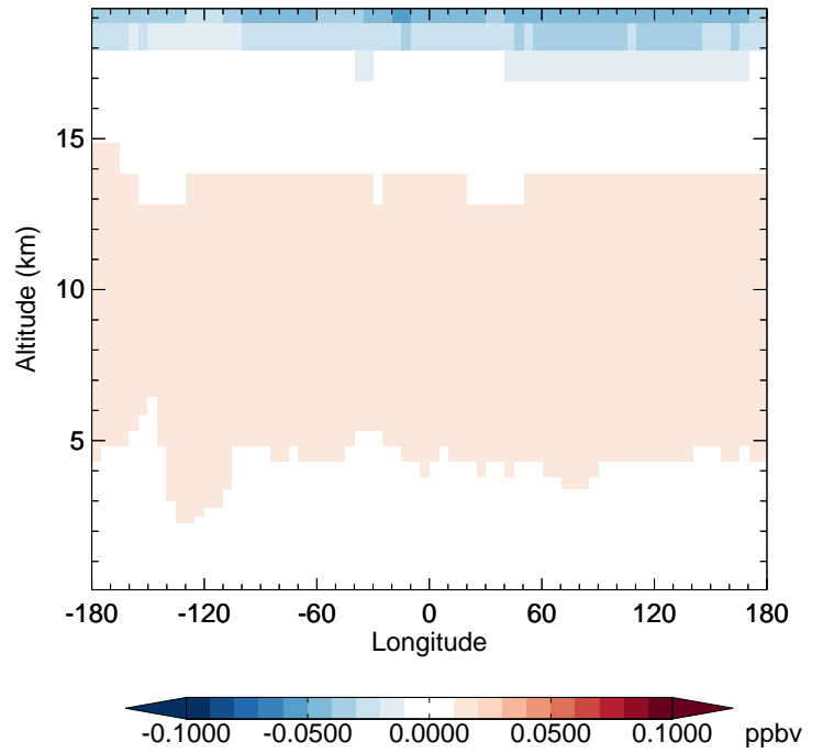
v11-02c - v11-01-public-Run0 OCS - Diff along 42N for Oct
