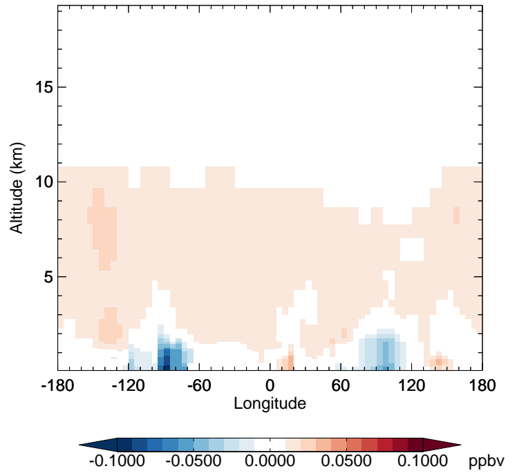
v11-02c - v11-01-public-Run0 H2O2 - Diff along 42N for Oct
