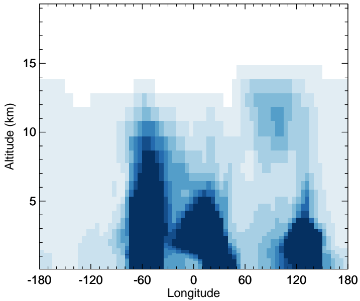
v11-02c - v11-01-public-Run0 R4N2 - Diff along 15S for Oct
