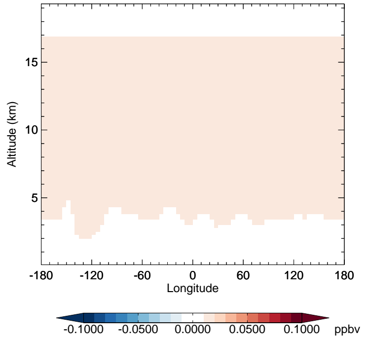
v11-02c - v11-01-public-Run0 HCFC141b - Diff along 42N for Oct
