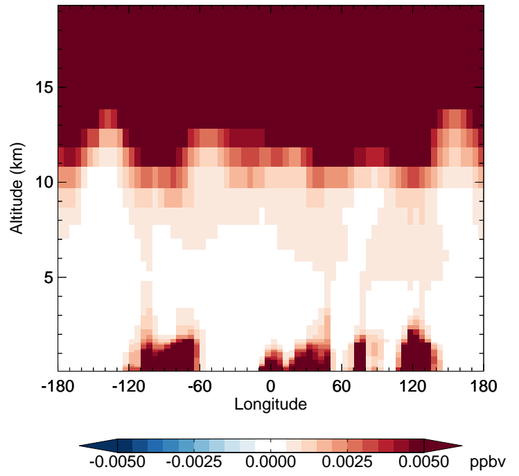
v11-02c - v11-02a N2O5 - Diff along 42N for Oct
