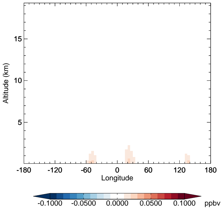
v11-02c - v11-01-public-Run0 ISN1 - Diff along 15S for Oct
