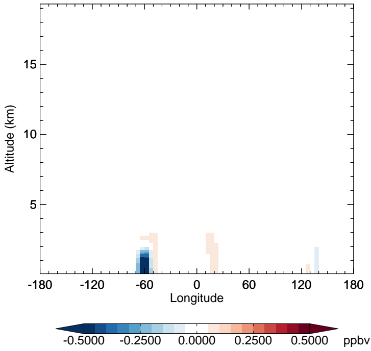
v11-02c - v11-02a CH 2 O - Diff along 15S for Oct
