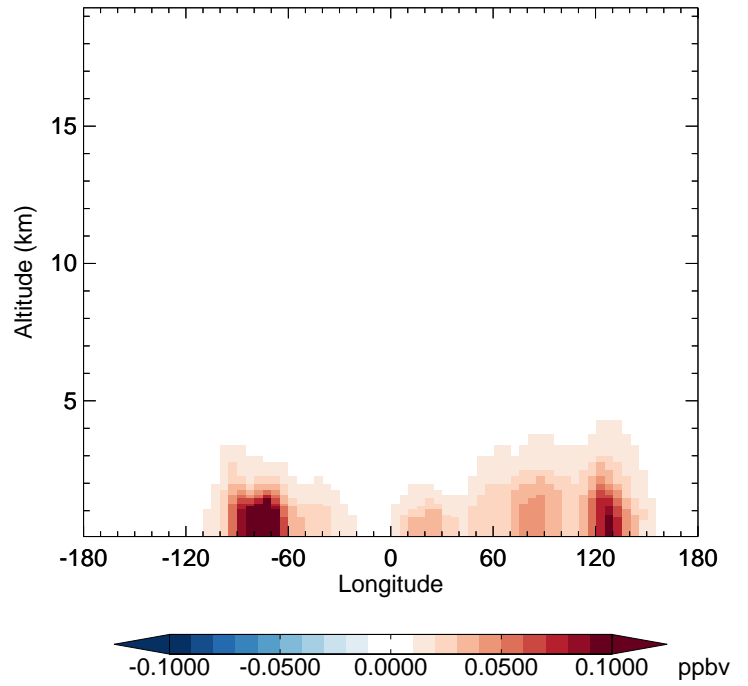
v11-02c - v11-02a INDIOL - Diff along 42N for Oct
