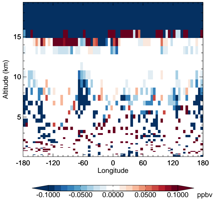
v11-02c - v11-01-public-Run0 H2O - Diff along 15S for Oct
