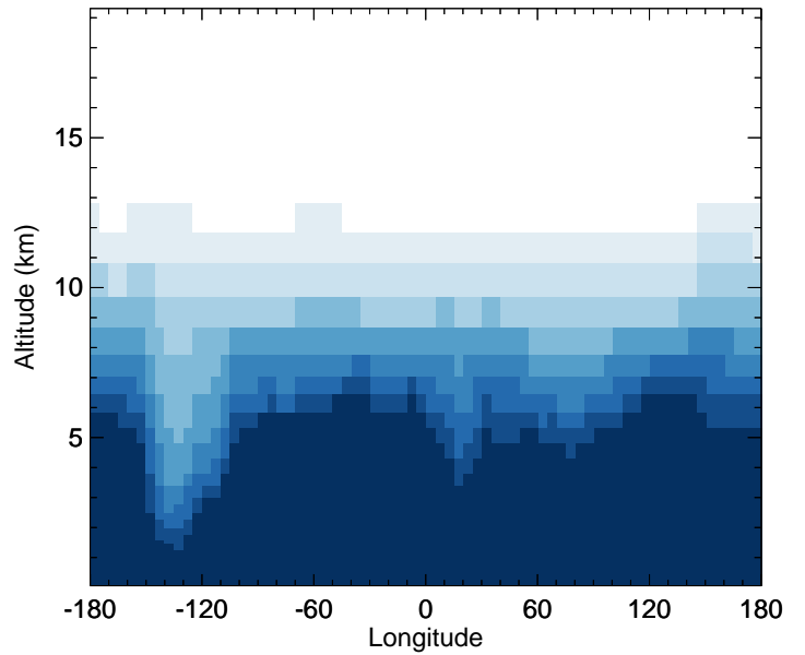
v11-02c - v11-01-public-Run0 R4N2 - Diff along 42N for Oct
