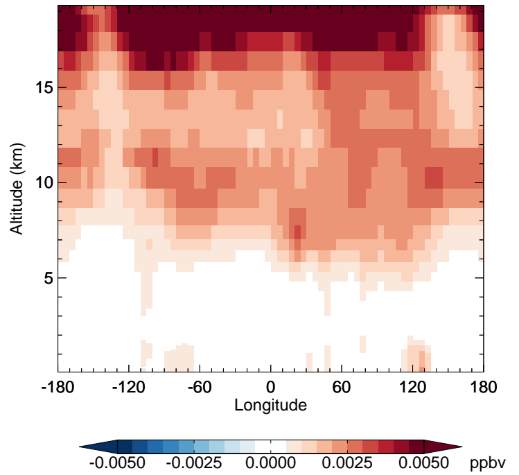
v11-02c - v11-01-public-Run0 HNO 4 - Diff along 42N for Oct
