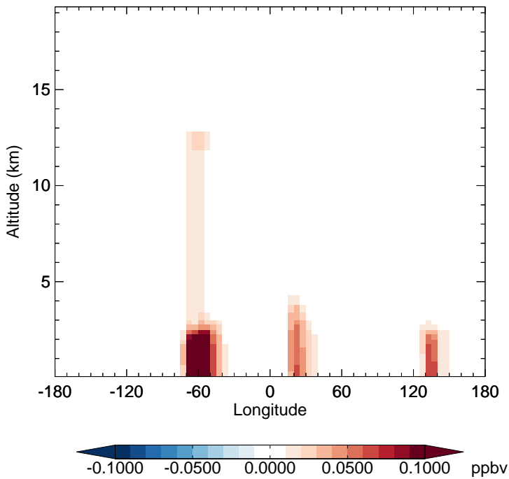
v11-02c - v11-01-public-Run0 IPMN - Diff along 15S for Oct
