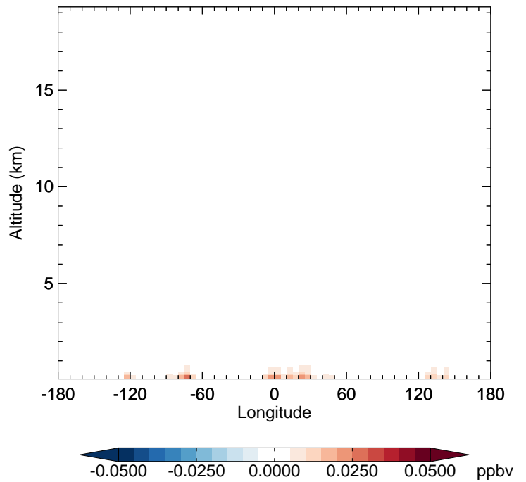
v11-02c - v11-01-public-Run0 RCHO - Diff along 42N for Oct
