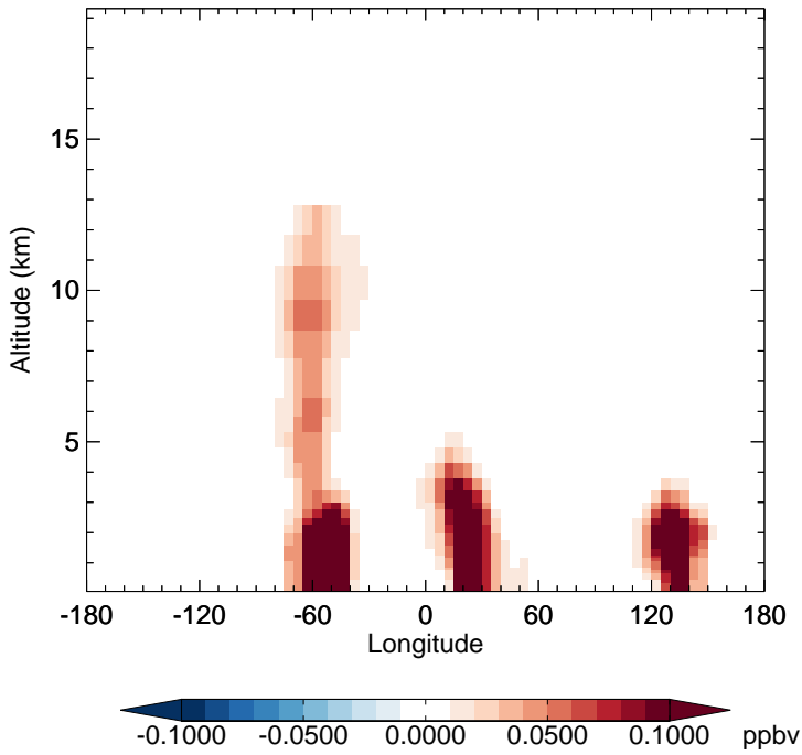
v11-02c - v11-01-public-Run0 IMAE - Diff along 15S for Oct
