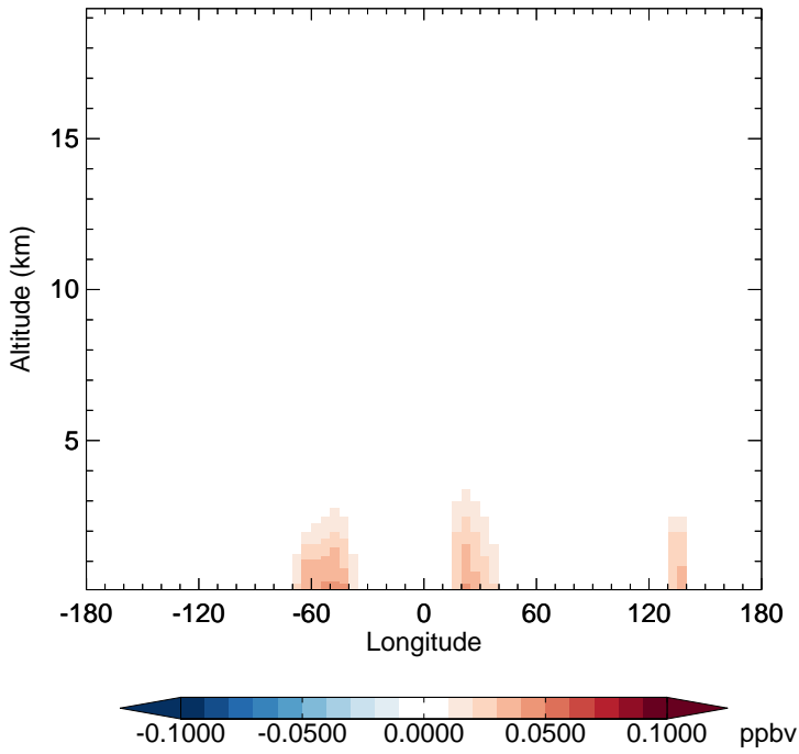
v11-02c - v11-02a GLYX - Diff along 15S for Oct
