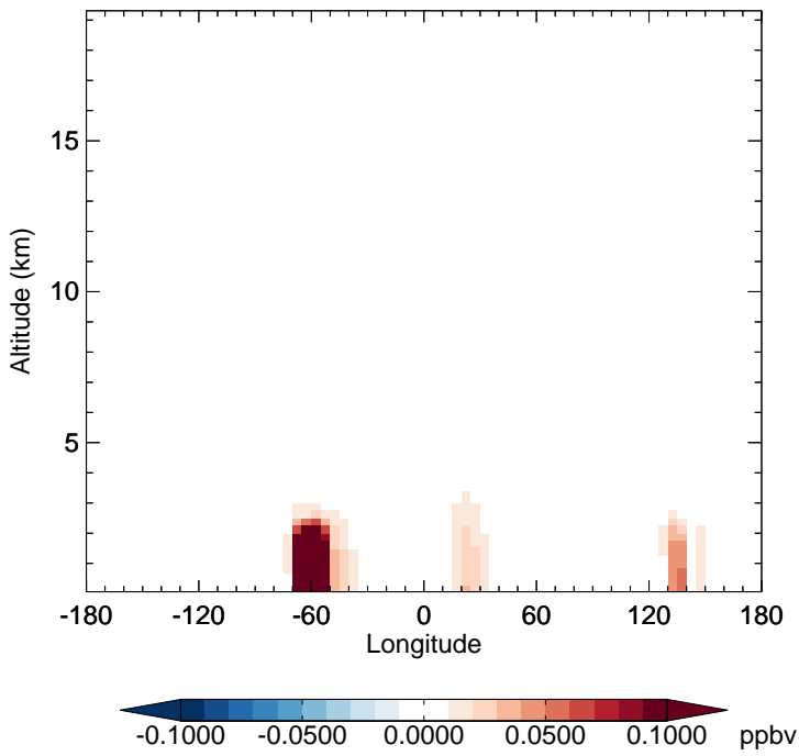
v11-02c - v11-02a HPALD - Diff along 15S for Oct
