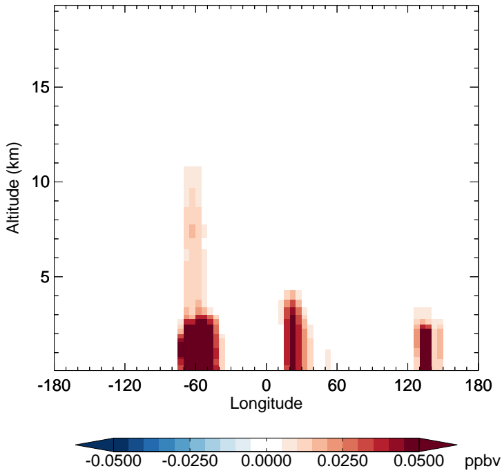
v11-02c - v11-01-public-Run0 MVK - Diff along 15S for Oct
