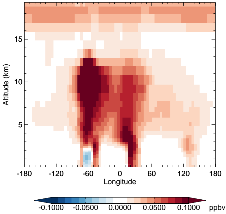
v11-02c - v11-02a PAN - Diff along 15S for Oct
