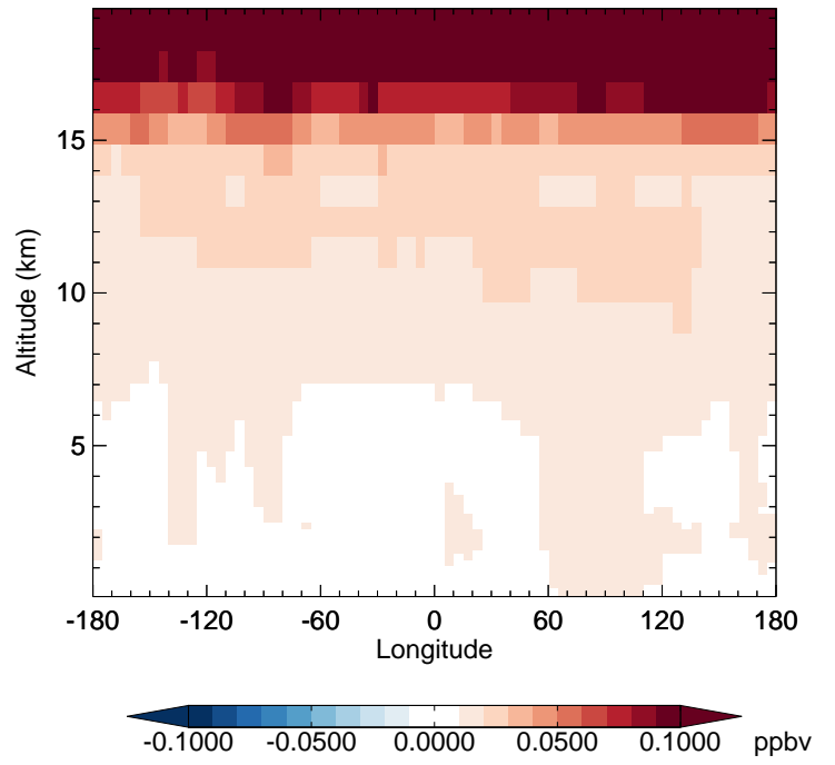
v11-02c - v11-02a HCl - Diff along 42N for Oct
