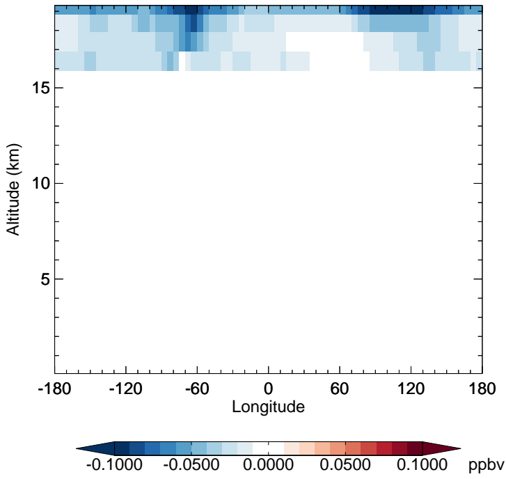
v11-02c - v11-02a CINO3 - Diff along 15S for Oct
