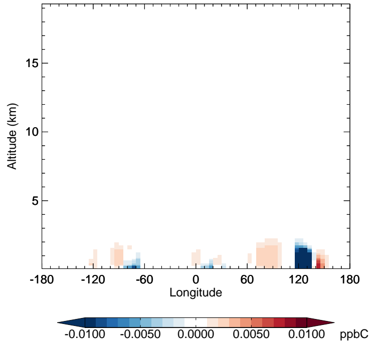
v11-02c - v11-01-public-Run0 PRPE - Diff along 42N for Oct
