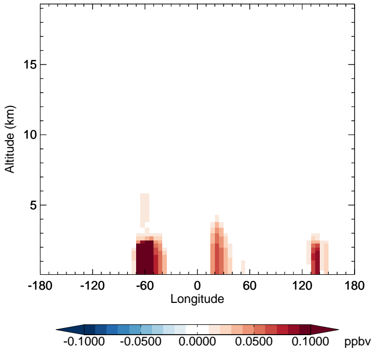
v11-02c - v11-02a RIPA - Diff along 15S for Oct
