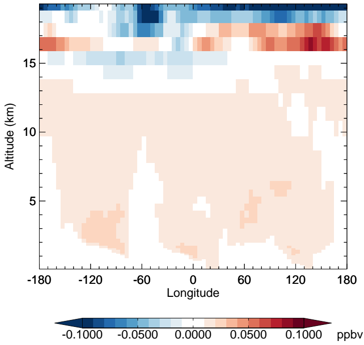
v11-02c - v11-02a HCl - Diff along 15S for Oct
