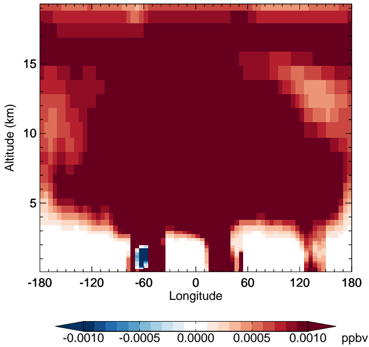
v11-02c - v11-01-public-Run0 PPN - Diff along 15S for Oct
