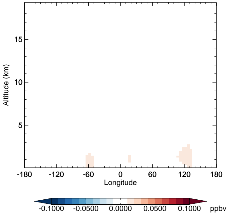
v11-02c - v11-02a SOAME - Diff along 15S for Oct
