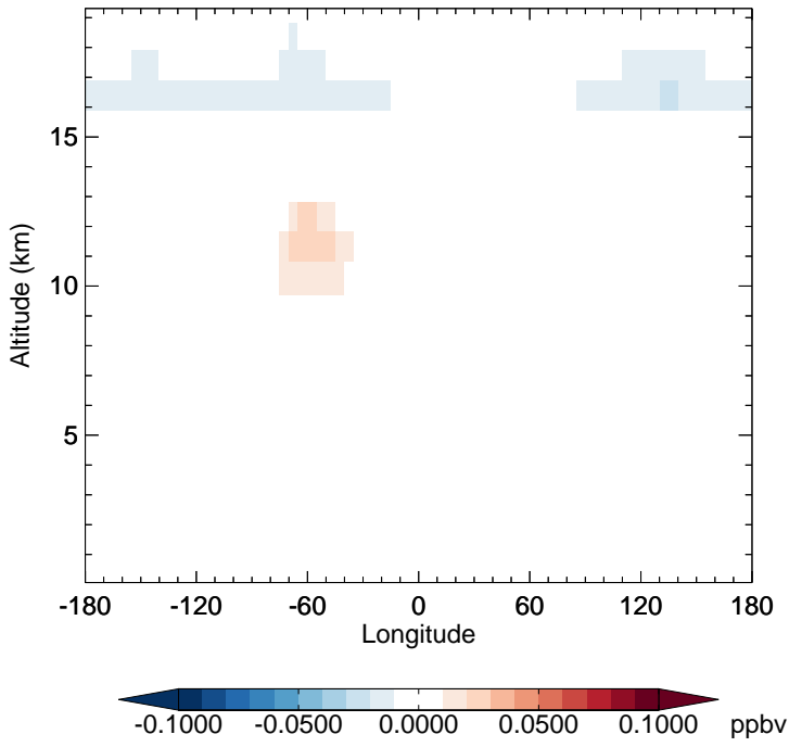
v11-02c - v11-02a MPN - Diff along 15S for Oct
