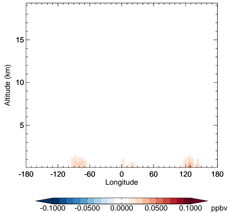
v11-02c - v11-01-public-Run0 MGLY - Diff along 42N for Oct
