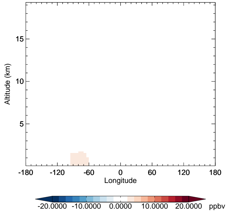
v11-02c - v11-02a CO - Diff along 42N for Oct
