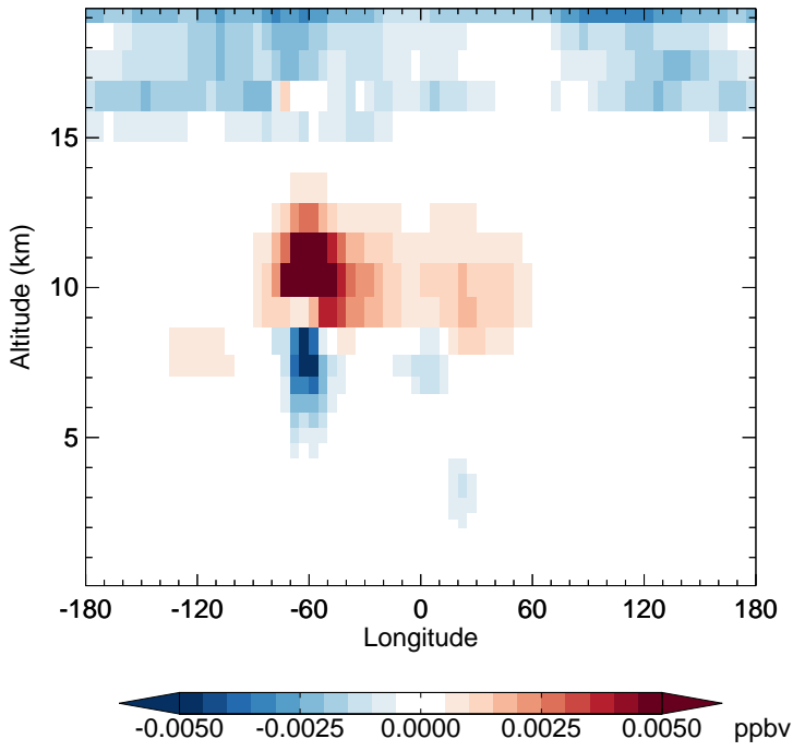
v11-02c - v11-02a HNO 4 - Diff along 15S for Oct
