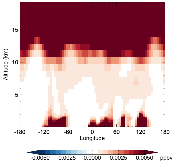
v11-02c - v11-01-public-Run0 N2O5 - Diff along 42N for Oct
