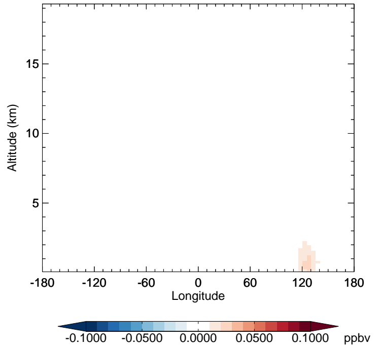
v11-02c - v11-01-public-Run0 ASOG3 - Diff along 42N for Oct
