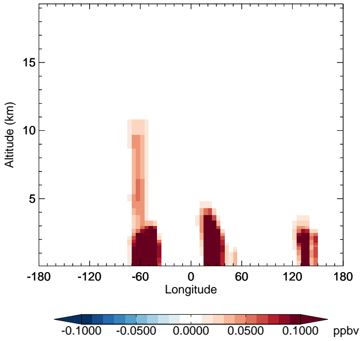
v11-02c - v11-02a IEPOXA - Diff along 15S for Oct
