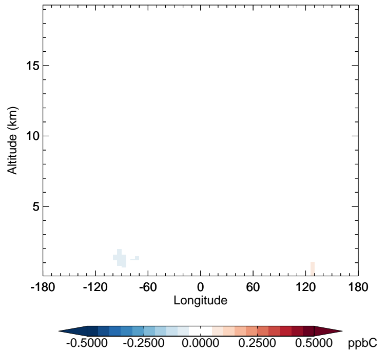
v11-02c - v11-01-public-Run0 ACET - Diff along 42N for Oct
