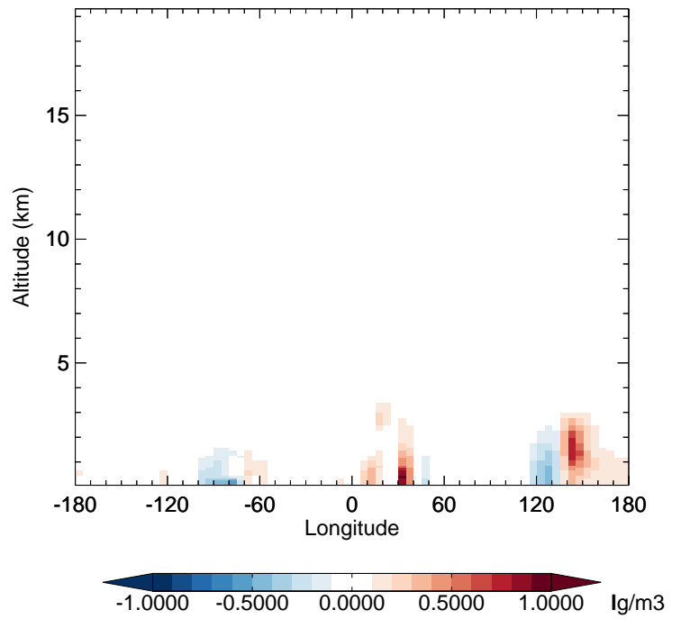
v11-02c - v11-01-public-Run0 SO 2 - Diff along 42N for Oct
