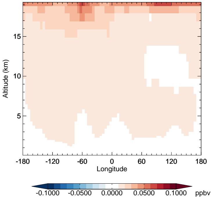
v11-02c - v11-02a OCS - Diff along 15S for Oct
