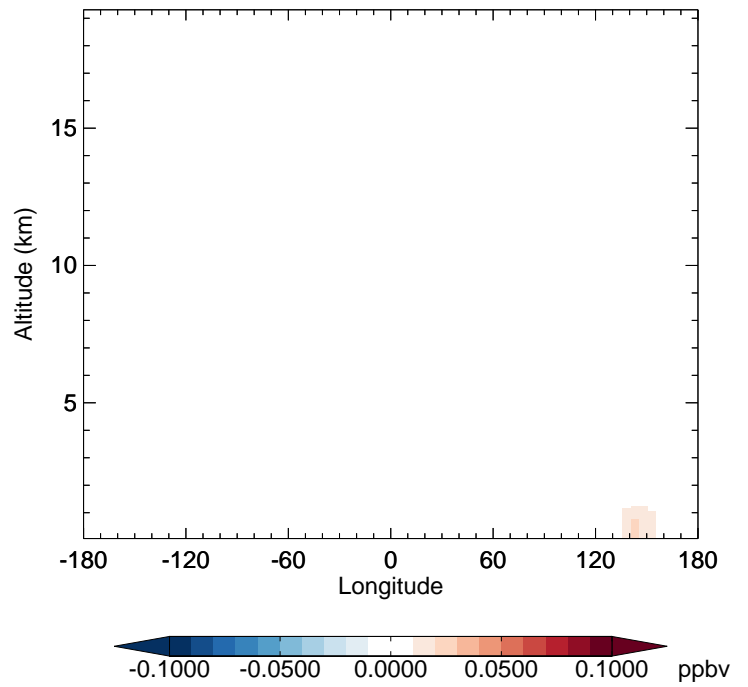
v11-02c - v11-01-public-Run0 ASOAN - Diff along 42N for Oct
