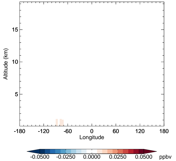
v11-02c - v11-01-public-Run0 MVK - Diff along 42N for Oct
