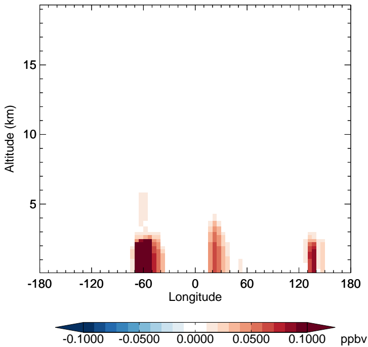
v11-02c - v11-01-public-Run0 RIPA - Diff along 15S for Oct
