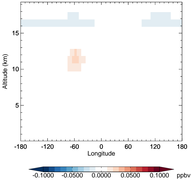
v11-02c - v11-01-public-Run0 MPN - Diff along 15S for Oct
