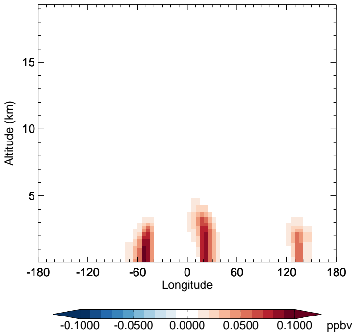
v11-02c - v11-01-public-Run0 IONITA - Diff along 15S for Oct
