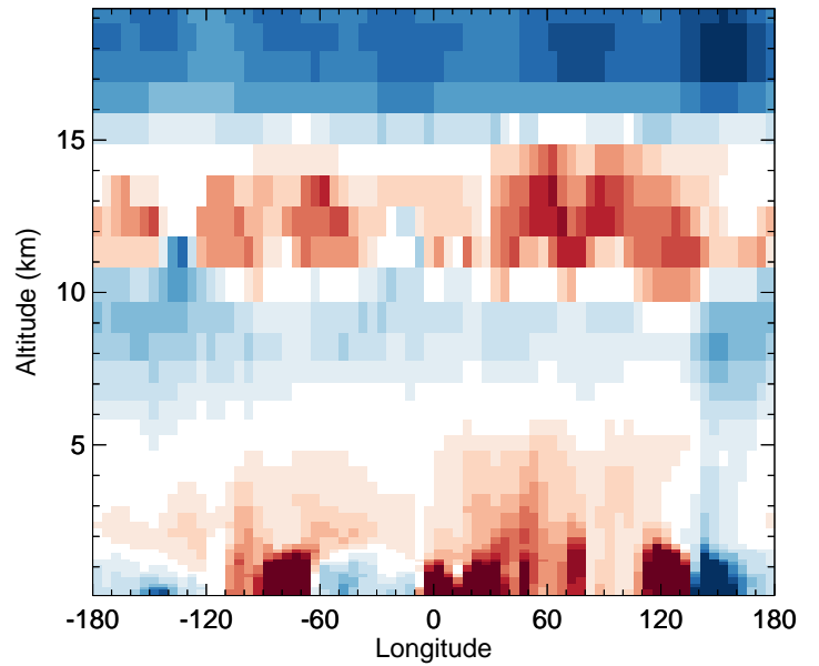
v11-02c - v11-01-public-Run0 OH - Diff along 42N for Oct
