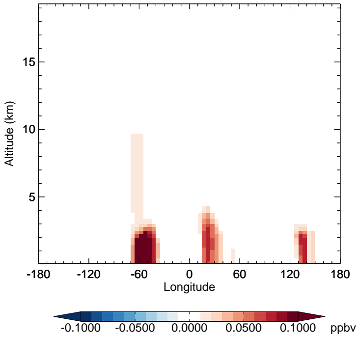
v11-02c - v11-02a IEPOXB - Diff along 15S for Oct
