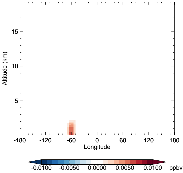
v11-02c - v11-02a MOBA - Diff along 15S for Oct
