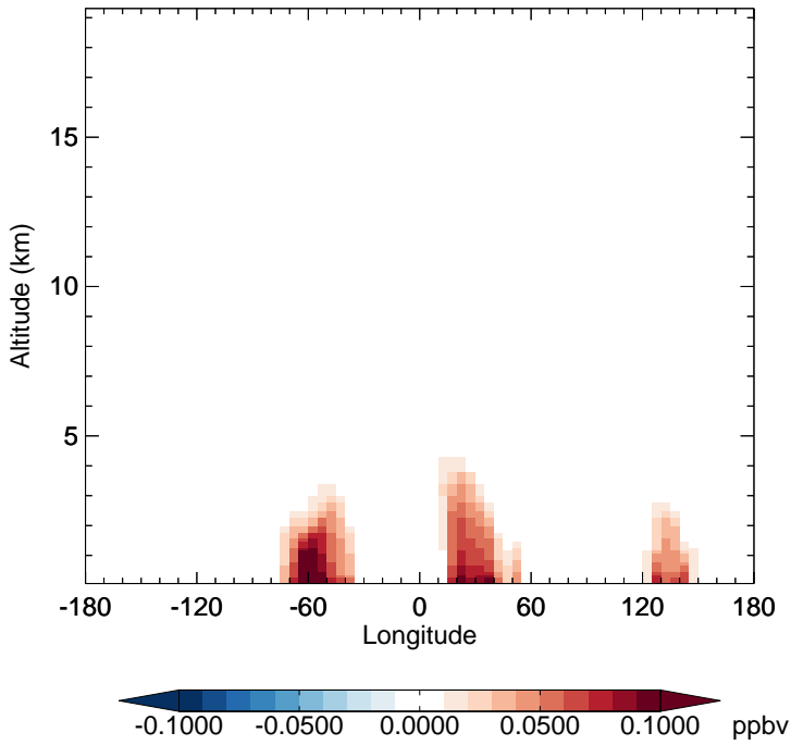
v11-02c - v11-01-public-Run0 SOAP - Diff along 15S for Oct
