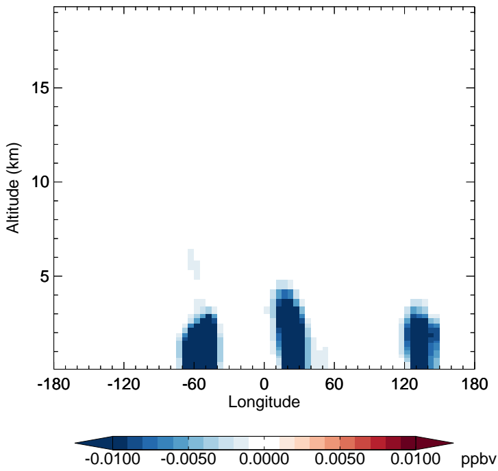
v11-02c - v11-01-public-Run0 MVKN - Diff along 15S for Oct
