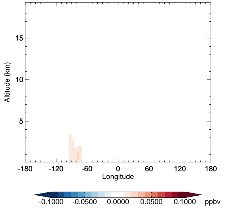
v11-02c - v11-02a SOAIE - Diff along 42N for Oct
