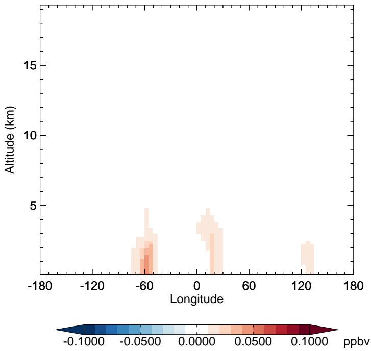
v11-02c - v11-02a BENZ - Diff along 15S for Oct
