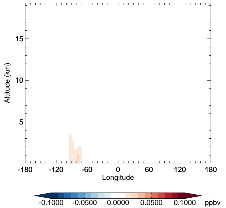
v11-02c - v11-01-public-Run0 SOAIE - Diff along 42N for Oct
