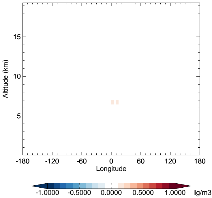
v11-02c - v11-02a NIT - Diff along 15S for Oct
