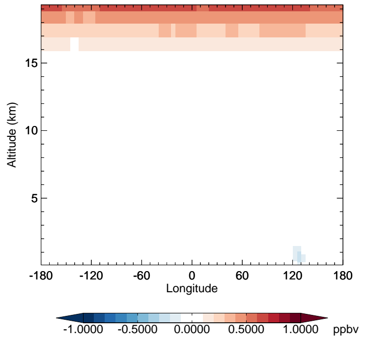
v11-02c - v11-01-public-Run0 NO 2 - Diff along 42N for Oct
