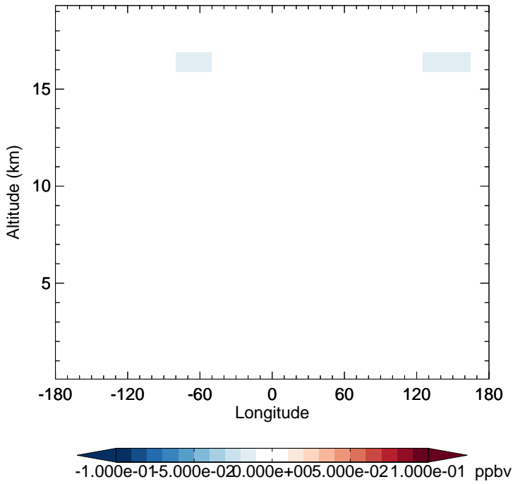
v11-02c - v11-01-public-Run0 ClO - Diff along 15S for Oct
