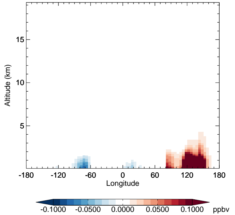
v11-02c - v11-01-public-Run0 XYLE - Diff along 42N for Oct
