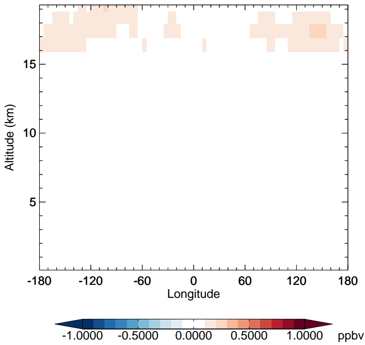
v11-02c - v11-02a NO 2 - Diff along 15S for Oct
