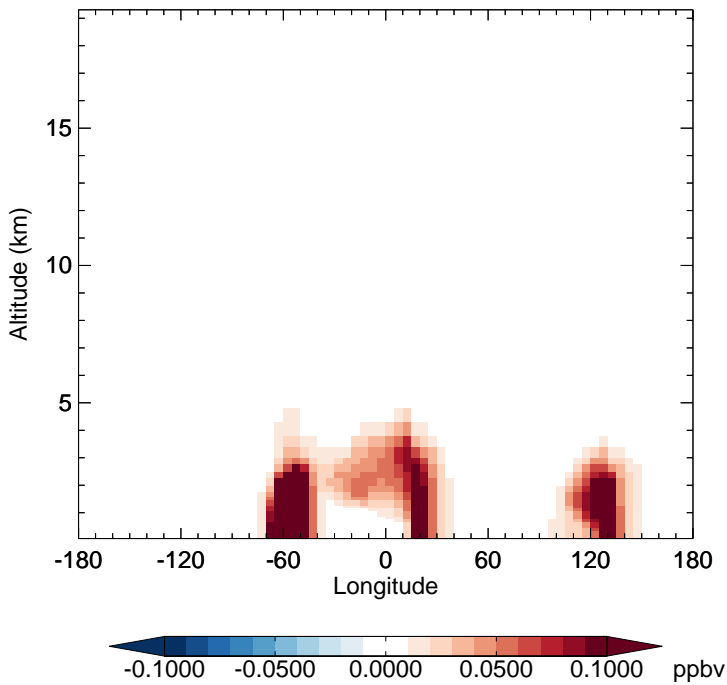
v11-02c - v11-01-public-Run0 SOAGX - Diff along 15S for Oct
