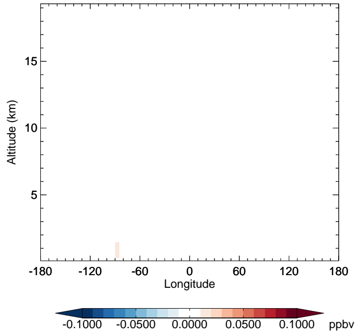
v11-02c - v11-01-public-Run0 IEPOXA - Diff along 42N for Oct
