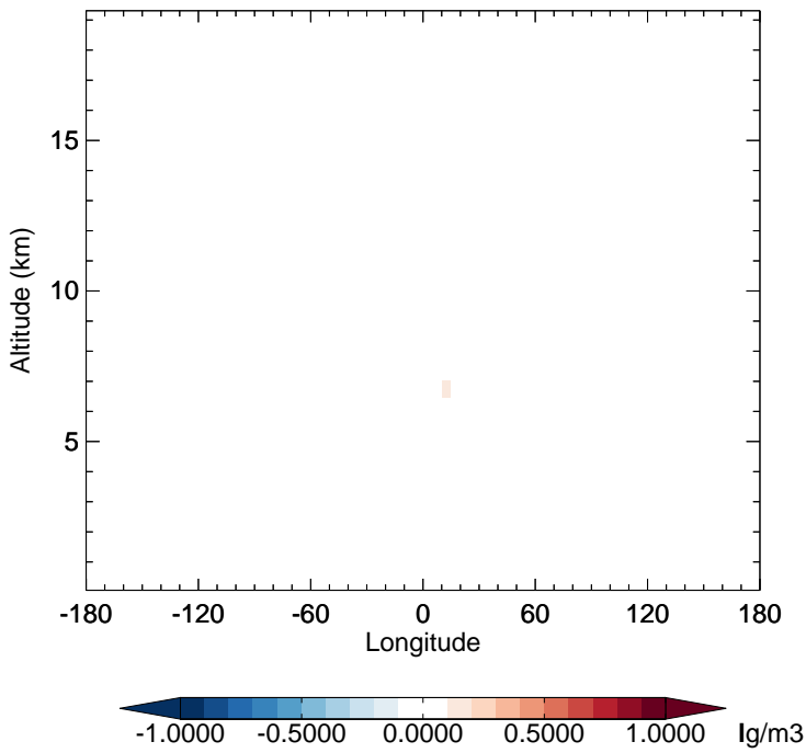
v11-02c - v11-01-public-Run0 NIT - Diff along 15S for Oct
