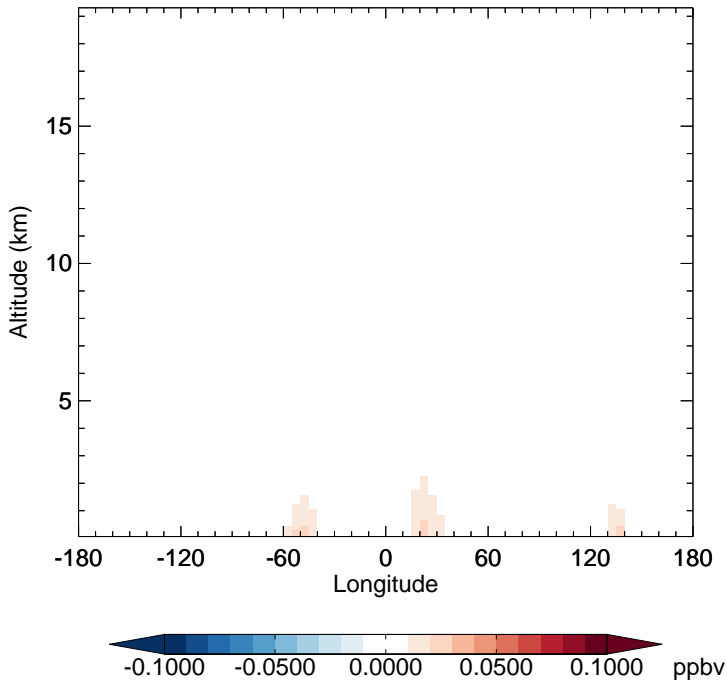
v11-02c - v11-02a ISN1 - Diff along 15S for Oct
