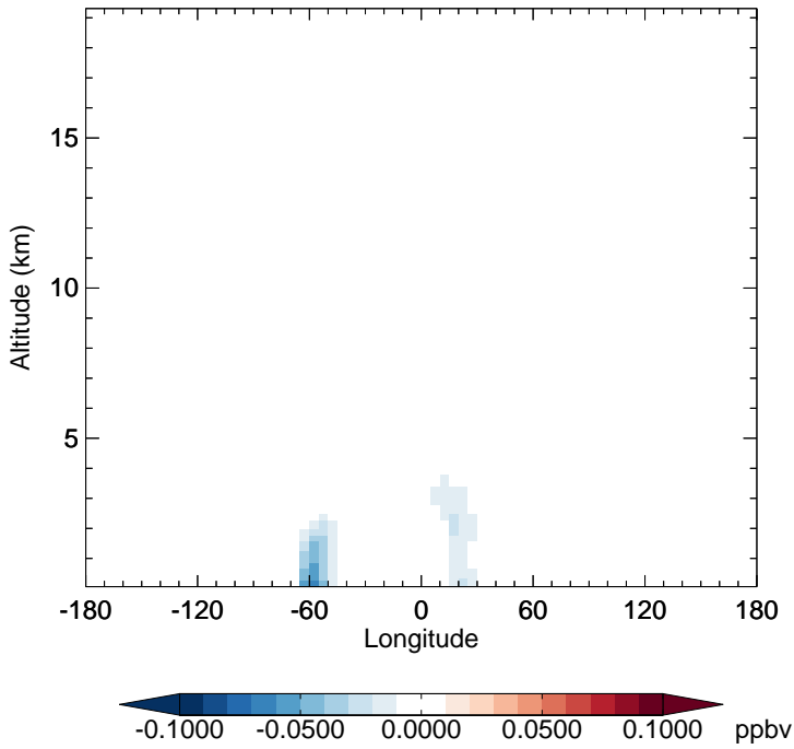
v11-02c - v11-01-public-Run0 TSOA2 - Diff along 15S for Oct
