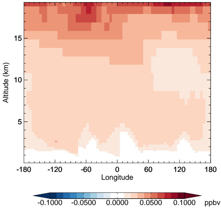
v11-02c - v11-01-public-Run0 CH3Cl - Diff along 15S for Oct
