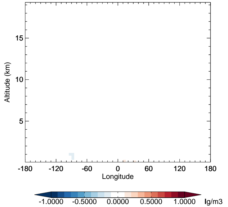
v11-02c - v11-01-public-Run0 NH3 - Diff along 42N for Oct
