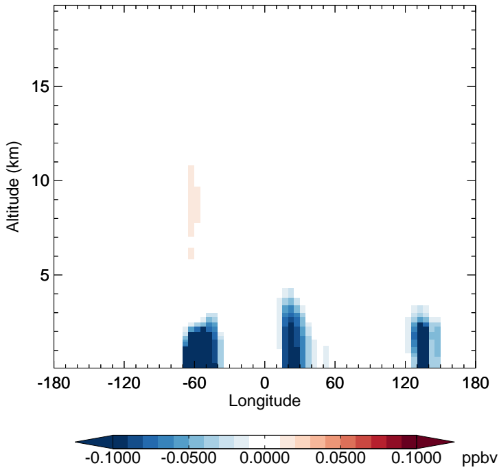
v11-02c - v11-02a GLYC - Diff along 15S for Oct
