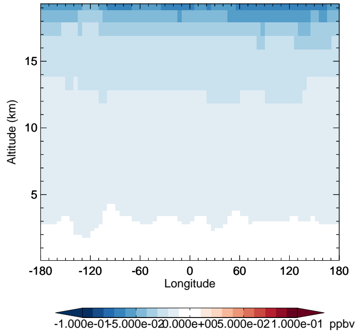
v11-02c - v11-02a CFC12 - Diff along 42N for Oct
