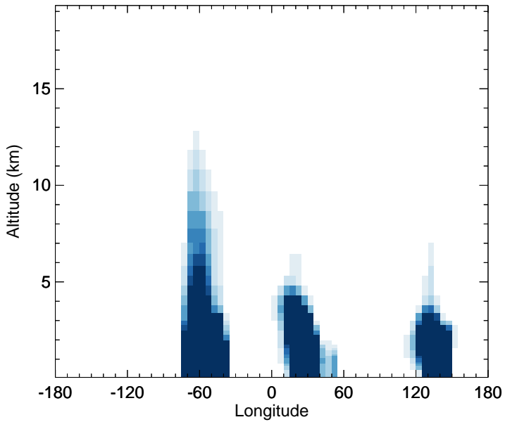
v11-02c - v11-01-public-Run0 HAC - Diff along 15S for Oct
