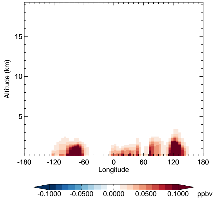
v11-02c - v11-01-public-Run0 SOAP - Diff along 42N for Oct
