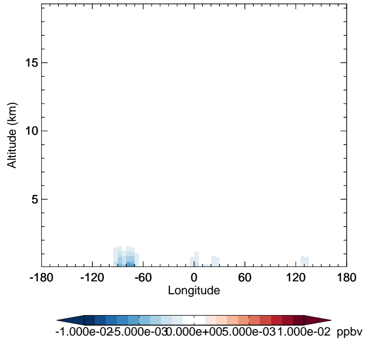
v11-02c - v11-02a NPMN - Diff along 42N for Oct
