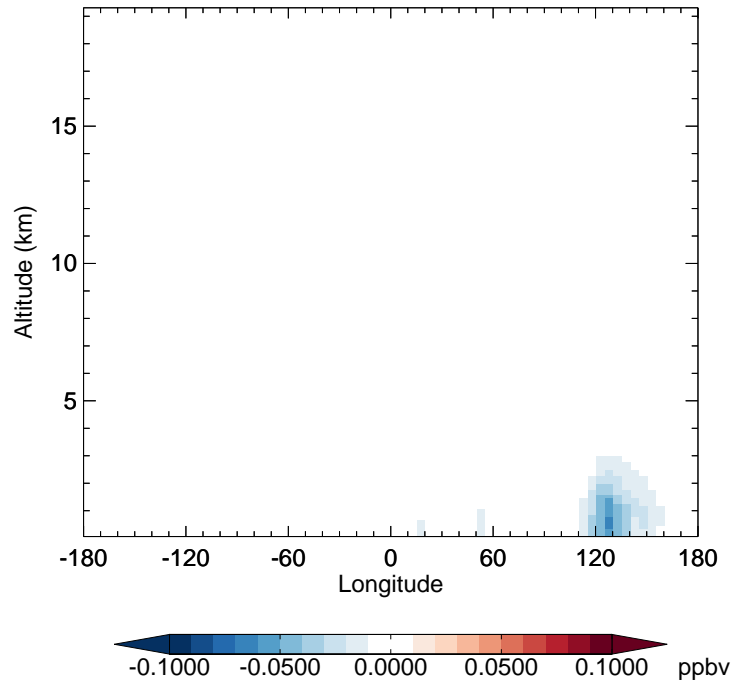
v11-02c - v11-02a TOLU - Diff along 42N for Oct
