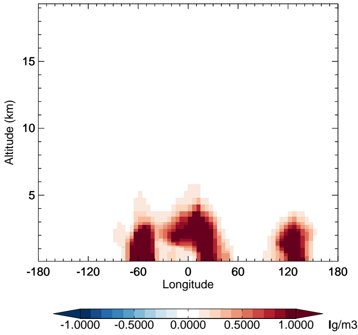
v11-02c - v11-02a SOAS - Diff along 15S for Oct
