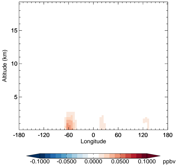
v11-02c - v11-02a TSOG2 - Diff along 15S for Oct
