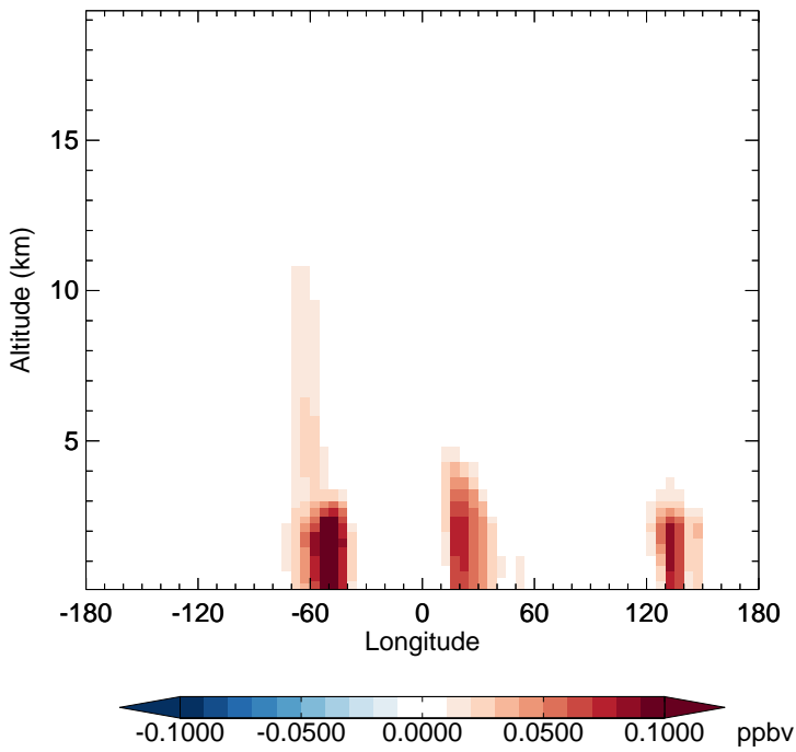
v11-02c - v11-01-public-Run0 HC187 - Diff along 15S for Oct
