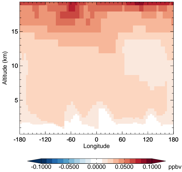
v11-02c - v11-02a CH3Cl - Diff along 15S for Oct
