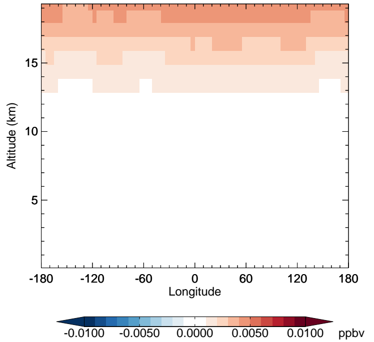
v11-02c - v11-01-public-Run0 BrNO3 - Diff along 42N for Oct
