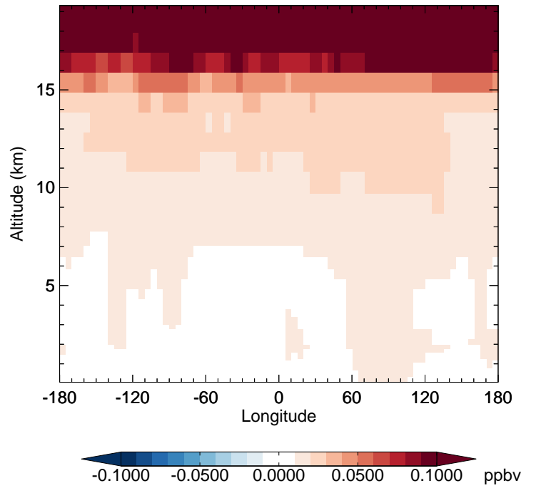
v11-02c - v11-01-public-Run0 HCl - Diff along 42N for Oct
