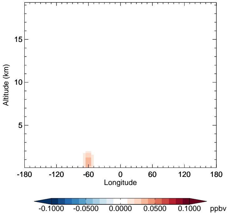
v11-02c - v11-02a RIPD - Diff along 15S for Oct
