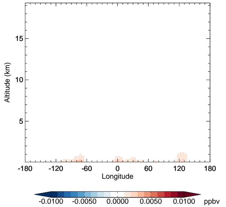
v11-02c - v11-02a NO 3 - Diff along 42N for Oct
