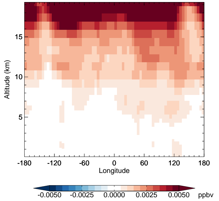
v11-02c - v11-02a HNO 4 - Diff along 42N for Oct
