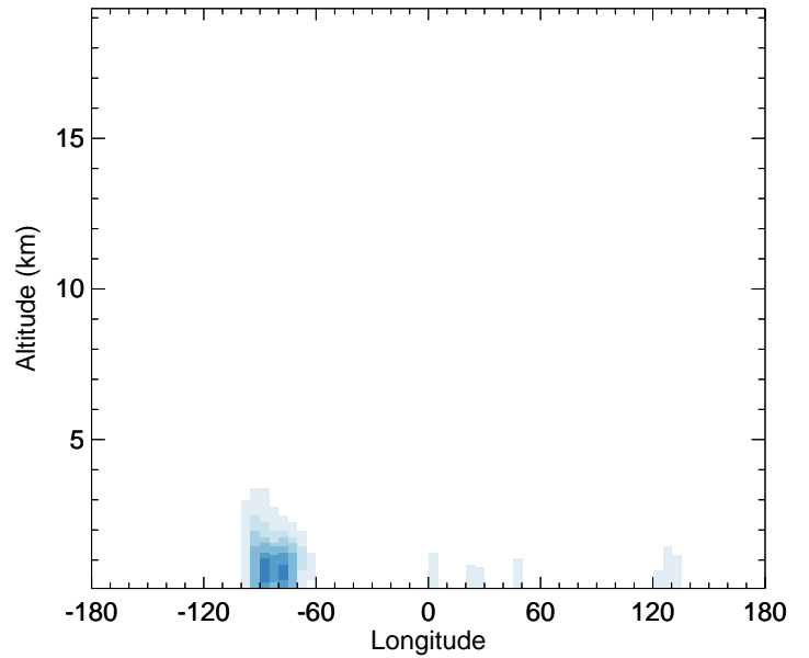
v11-02c - v11-01-public-Run0 HAC - Diff along 42N for Oct
