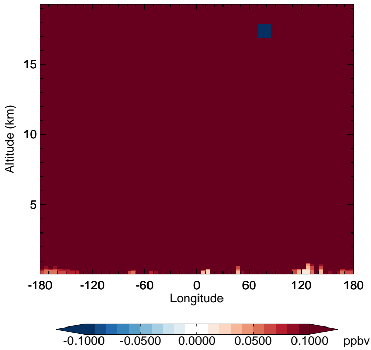
v11-02c - v11-01-public-Run0 N2O - Diff along 15S for Oct
