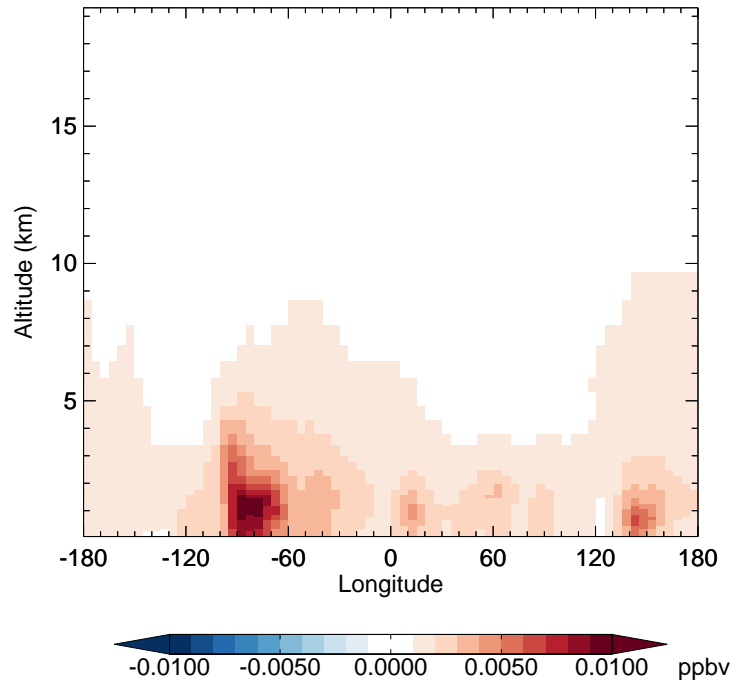
v11-02c - v11-02a MAP - Diff along 42N for Oct
