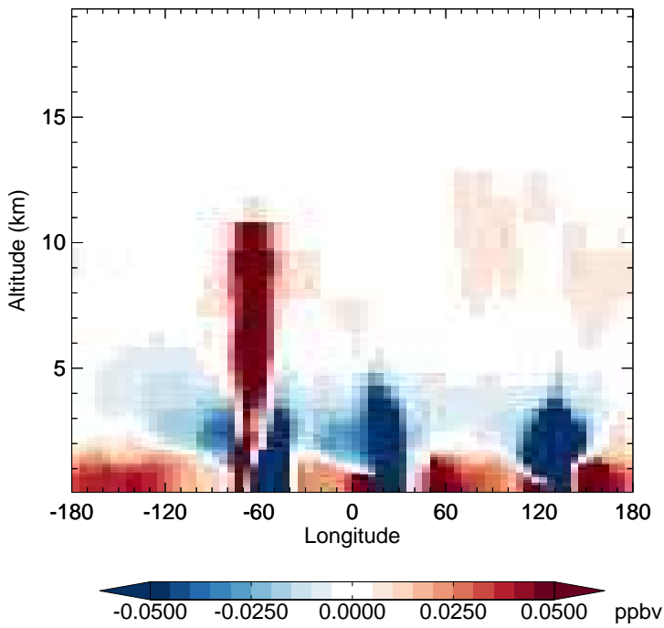
v11-02c - v11-01-public-Run0 MP - Diff along 15S for Oct
