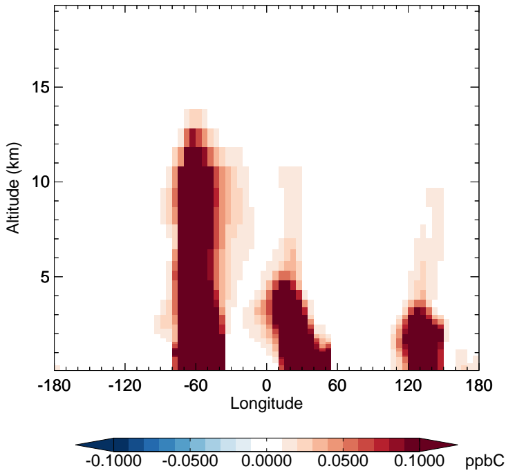
v11-02c - v11-01-public-Run0 MEK - Diff along 15S for Oct
