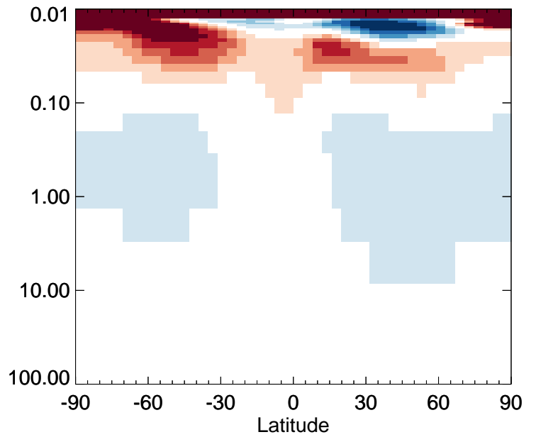
CFC114 - Strat zonal mean % diff for Apr
