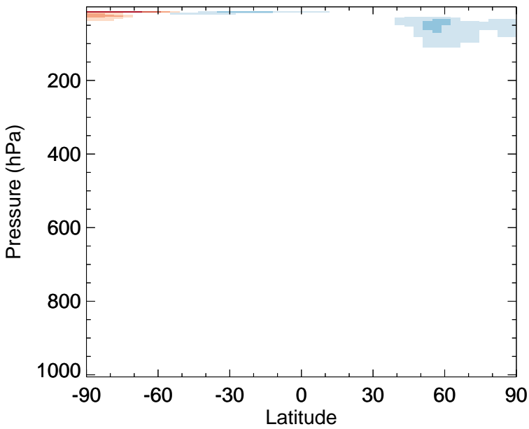
v11-02c - v11-01-public-Run0 ClO - Zonal mean abs diff for Jan
