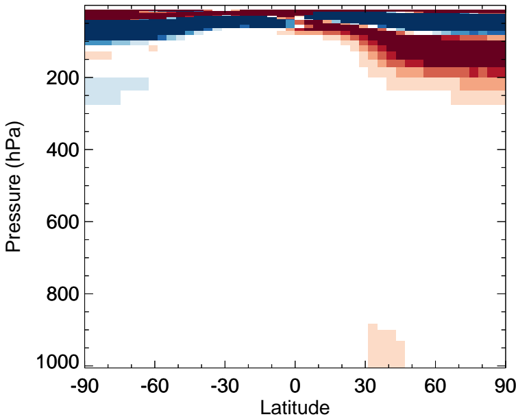
v11-02c - v11-01-public-Run0 O3 - Zonal mean abs diff for Jan
