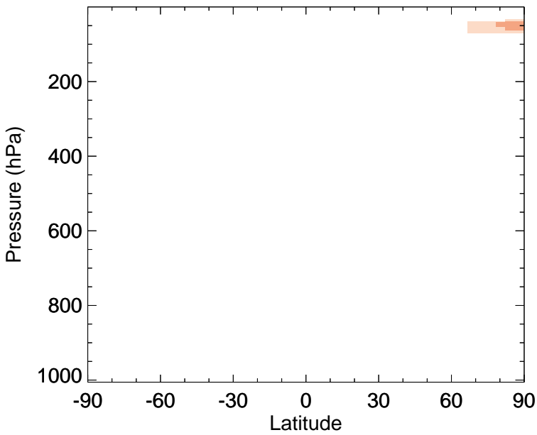
v11-02c - v11-01-public-Run0 Cl2 - Zonal mean abs diff for Jan
