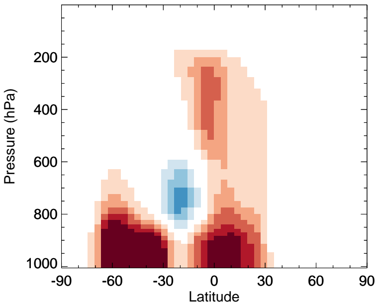
v11-02c - v11-01-public-Run0 MP - Zonal mean abs diff for Jan
