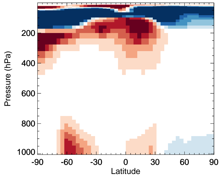
v11-02c / v11-01-public-Run0 MP - Zonal mean % diff for Jan
