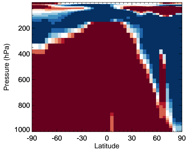
v11-02c / v11-01-public-Run0 Cl2 - Zonal mean % diff for Jan
