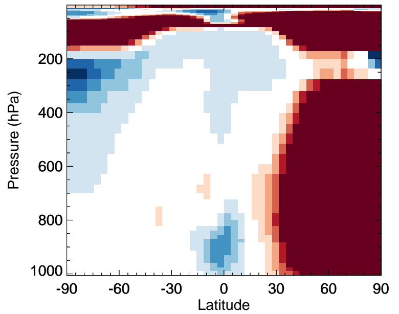
v11-02c / v11-02a NO - Zonal mean % diff for Jan
