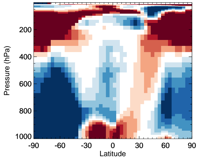
v11-02c / v11-01-public-Run0 Br2 - Zonal mean % diff for Jan
