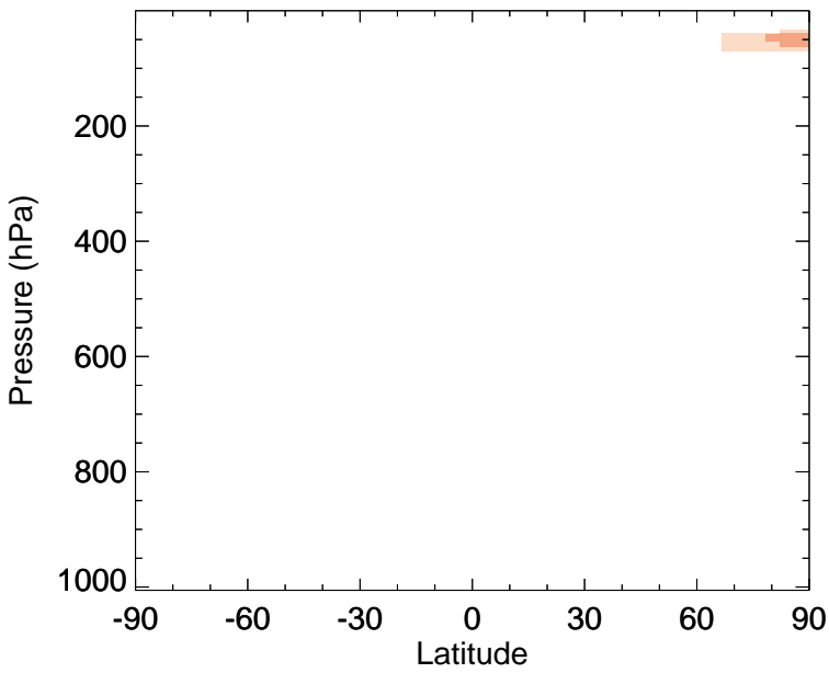
v11-02c - v11-02a Cl2 - Zonal mean abs diff for Jan
