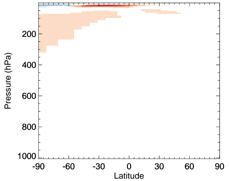
v11-02c / v11-02a CO - Zonal mean % diff for Jan
