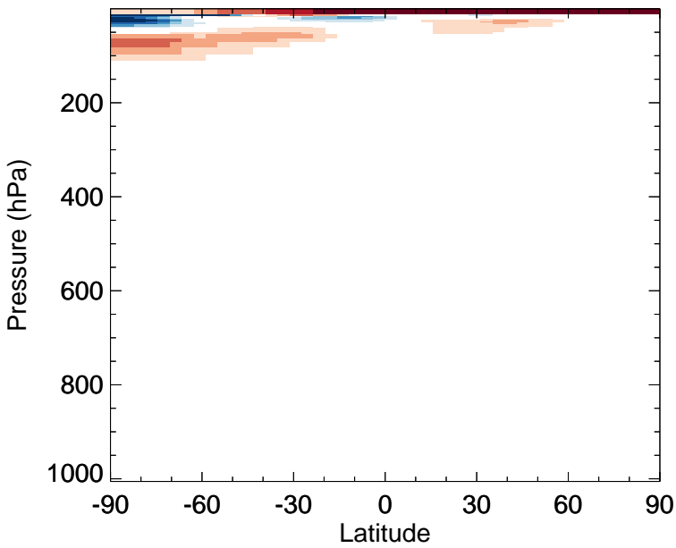
v11-02c - v11-01-public-Run0 NO - Zonal mean abs diff for Jan
