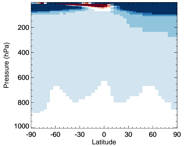
v11-02c / v11-01-public-Run0 CCI4 - Zonal mean % diff for Jan
