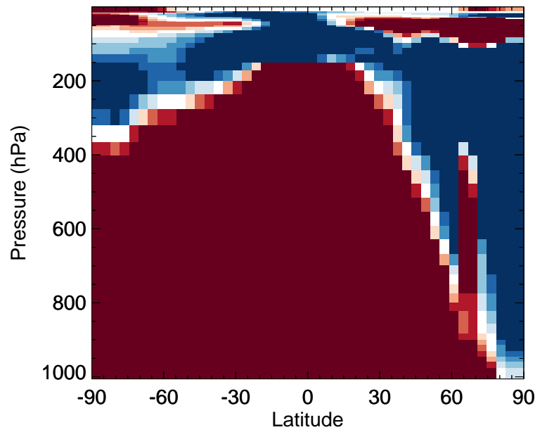
v11-02c / v11-02a Cl2 - Zonal mean % diff for Jan
