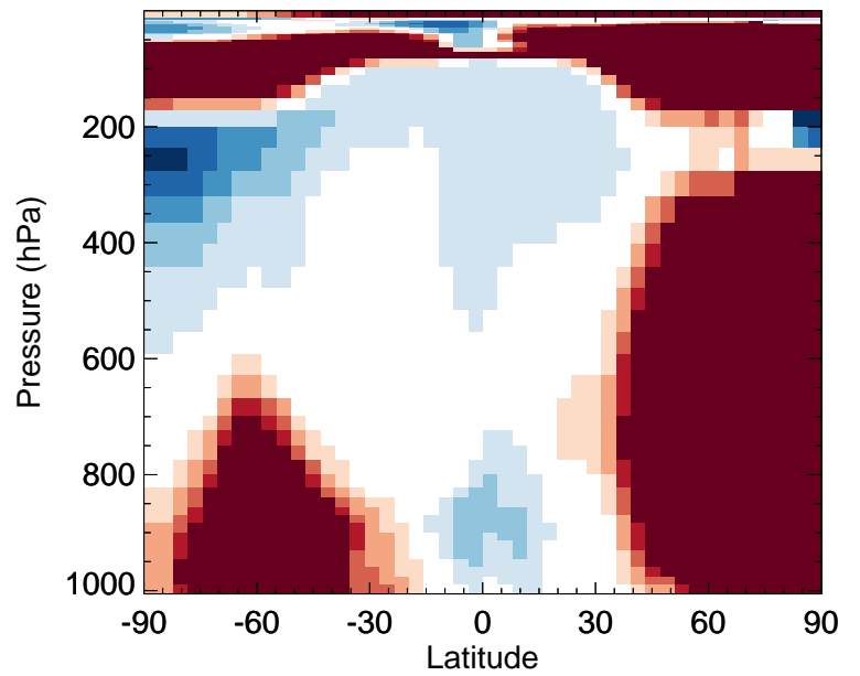
v11-02c / v11-01-public-Run0 NO - Zonal mean % diff for Jan
