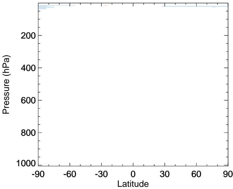
v11-02c - v11-01-public-Run0 CO - Zonal mean abs diff for Jan
