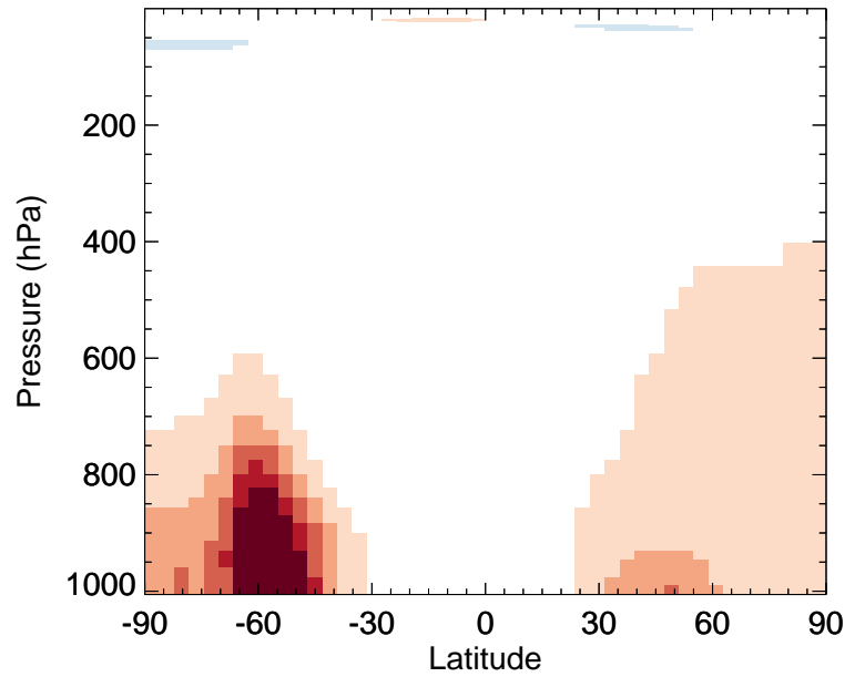
v11-02c / v11-01-public-Run0 O3 - Zonal mean % diff for Jan
