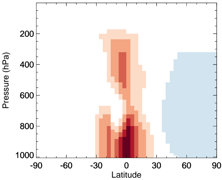
v11-02c - v11-02a MP - Zonal mean abs diff for Jan
