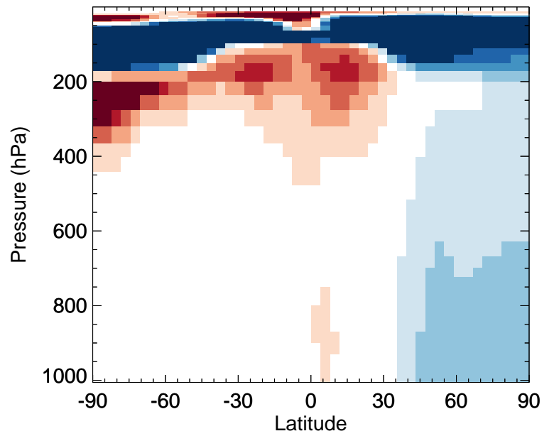
v11-02c / v11-02a MP - Zonal mean % diff for Jan
