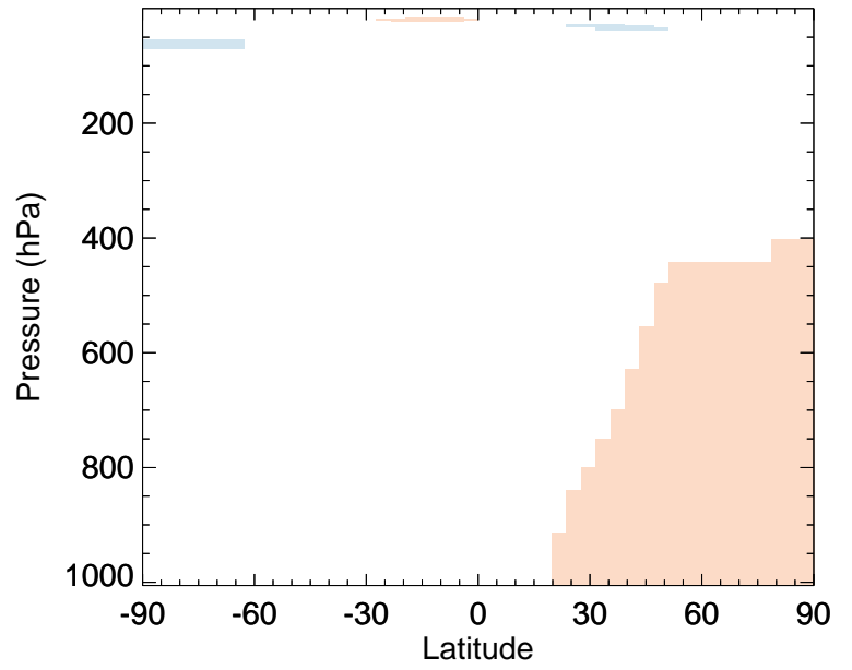
v11-02c / v11-02a O3 - Zonal mean % diff for Jan
