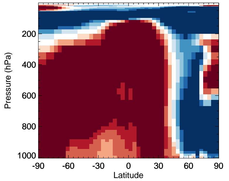
v11-02c / v11-02a ClO - Zonal mean % diff for Jan
