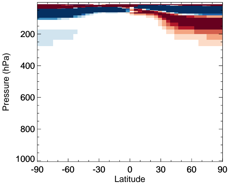
v11-02c - v11-02a O3 - Zonal mean abs diff for Jan
