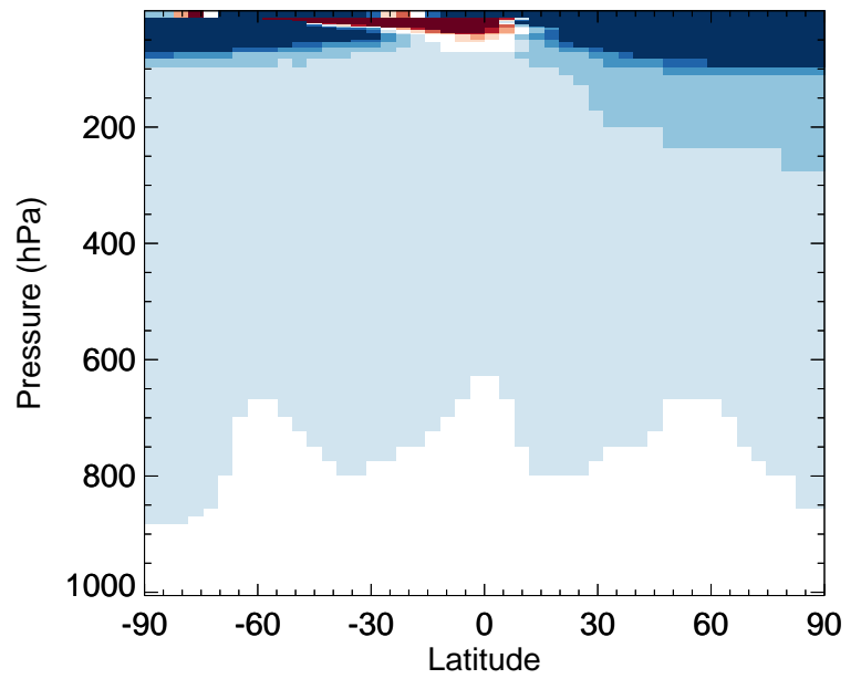
v11-02c / v11-02a CCI4 - Zonal mean % diff for Jan
