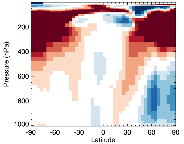
v11-02c / v11-02a Br2 - Zonal mean % diff for Jan
