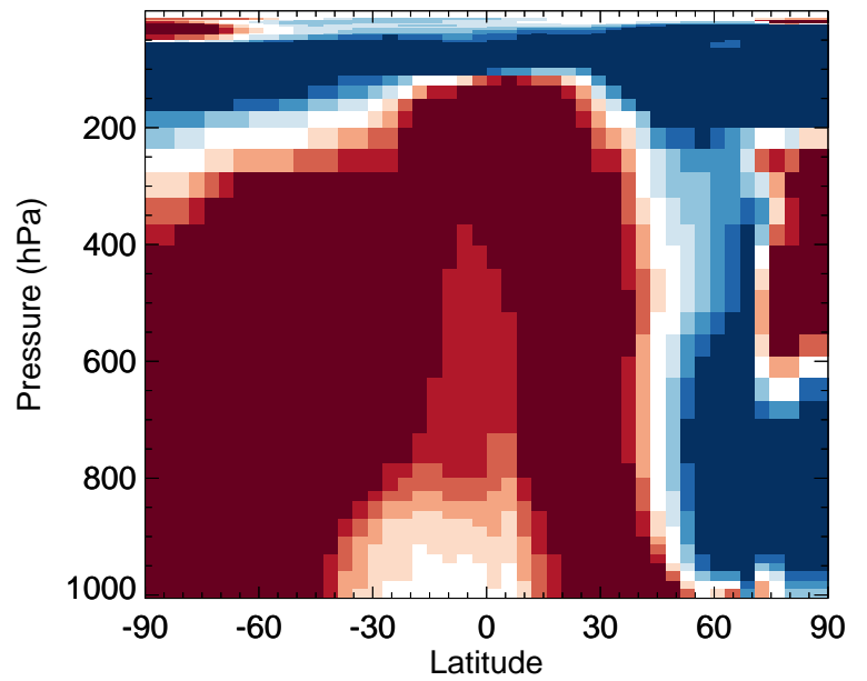
v11-02c / v11-01-public-Run0 ClO - Zonal mean % diff for Jan
