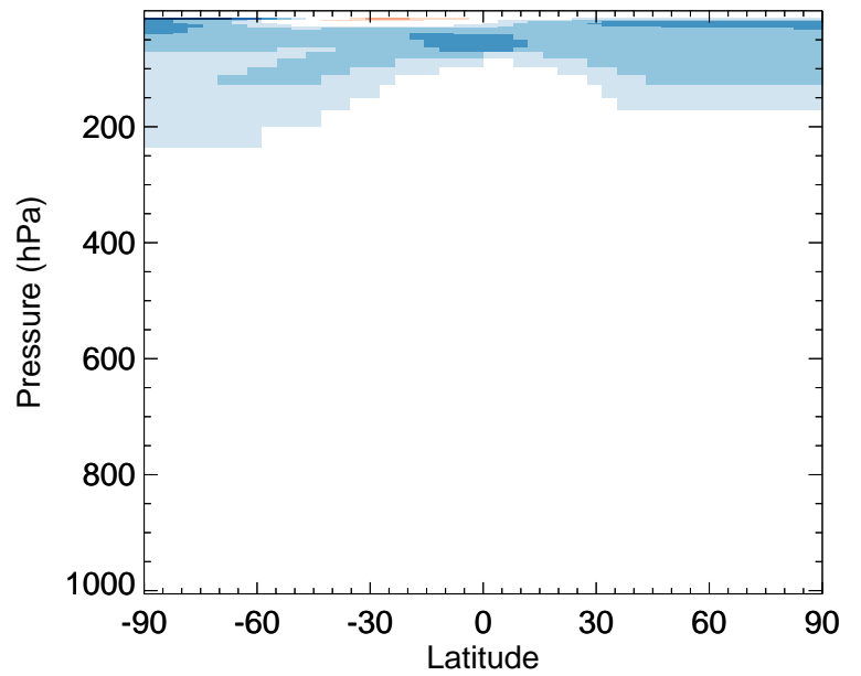
v11-02c / v11-01-public-Run0 CO - Zonal mean % diff for Jan
