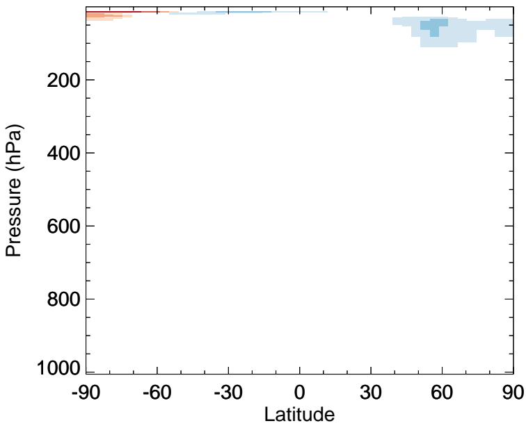
v11-02c - v11-02a ClO - Zonal mean abs diff for Jan
