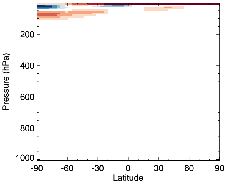
v11-02c - v11-02a NO - Zonal mean abs diff for Jan
