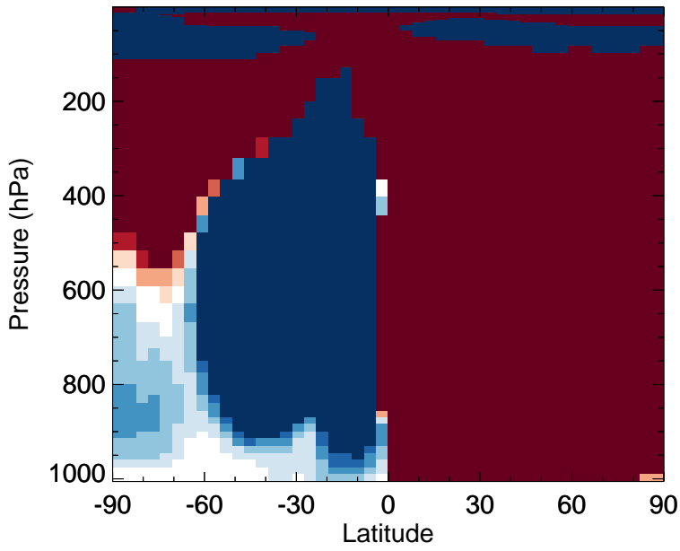
v11-02c - v11-02a CH4 - Zonal mean abs diff for Jul
