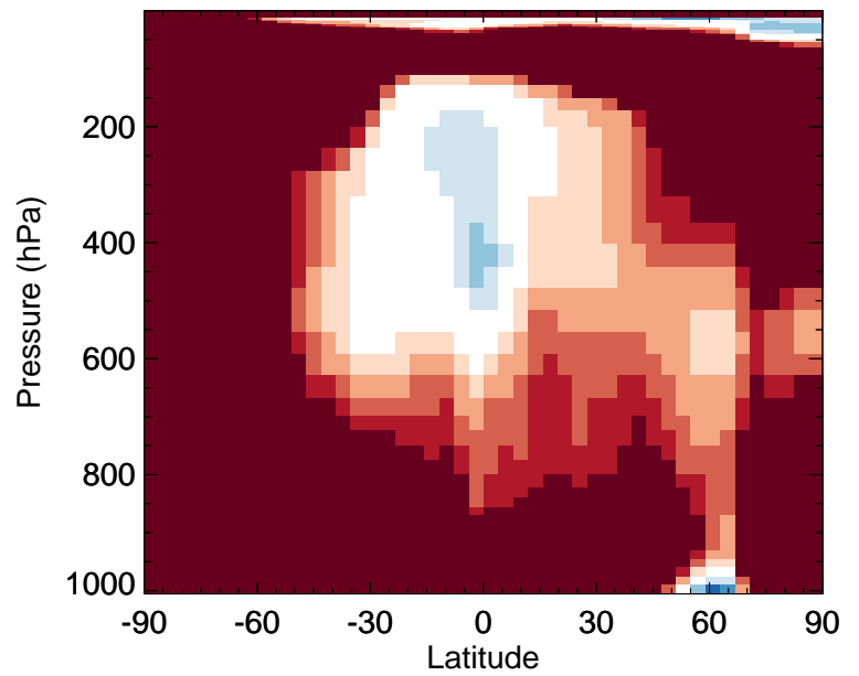
v11-02c / v11-01-public-Run0 N2O5 - Zonal mean % diff for Jul
