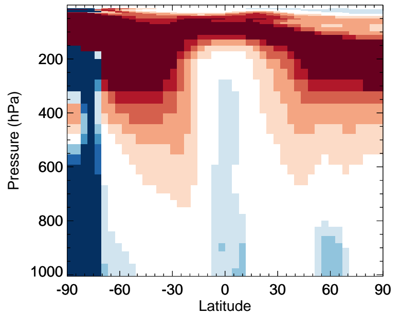
v11-02c / v11-02a Br - Zonal mean % diff for Jul
