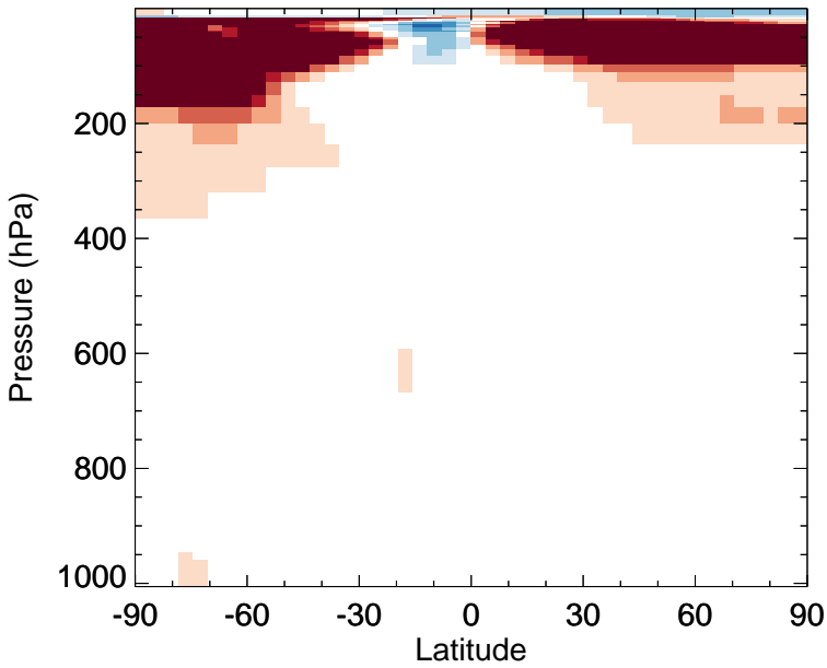
v11-02c - v11-01-public-Run0 HCl - Zonal mean abs diff for Jul
