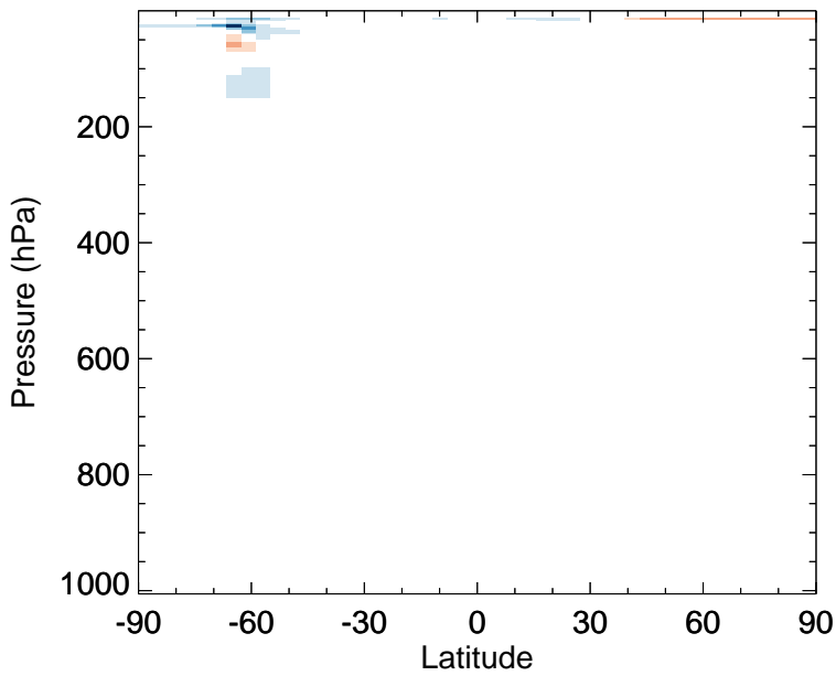
v11-02c - v11-01-public-Run0 ClO - Zonal mean abs diff for Jul
