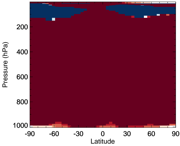
v11-02c - v11-02a N2O - Zonal mean abs diff for Jul
