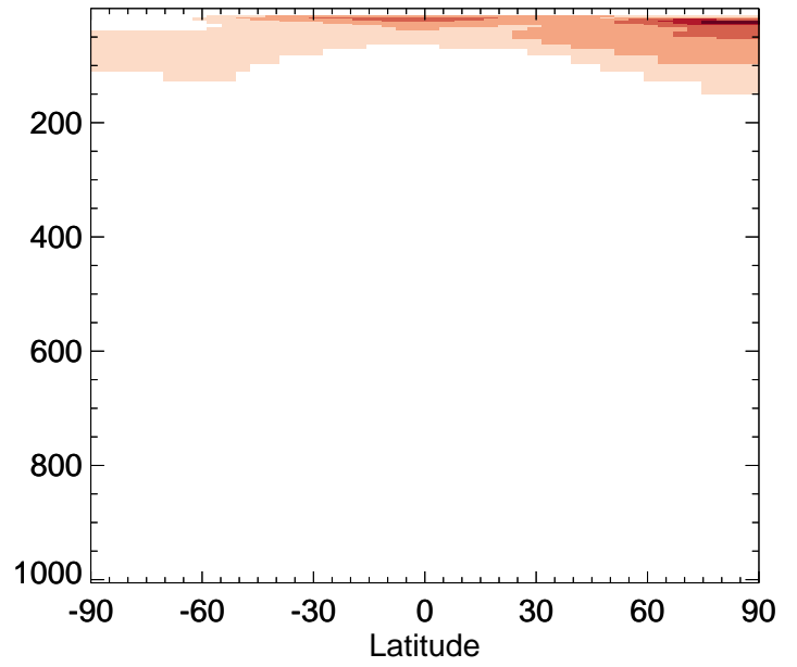
v11-02c / v11-02a C2H6 - Zonal mean % diff for Jul
