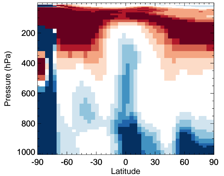
v11-02c / v11-01-public-Run0 Br - Zonal mean % diff for Jul
