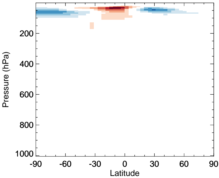
v11-02c - v11-01-public-Run0 OCS - Zonal mean abs diff for Jul
