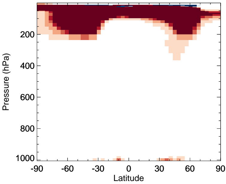
v11-02c - v11-02a N2O5 - Zonal mean abs diff for Jul
