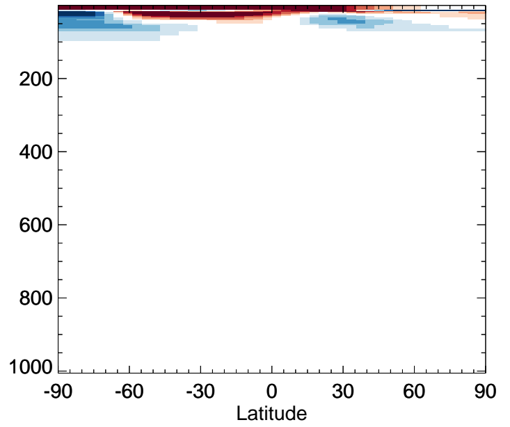
v11-02c / v11-02a N2O - Zonal mean % diff for Jul
