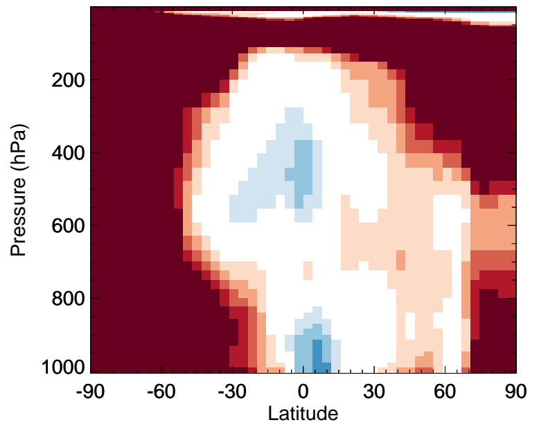
v11-02c / v11-02a N2O5 - Zonal mean % diff for Jul
