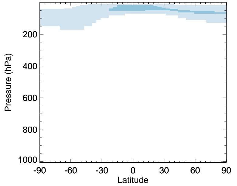
v11-02c / v11-02a NH4 - Zonal mean % diff for Jul
