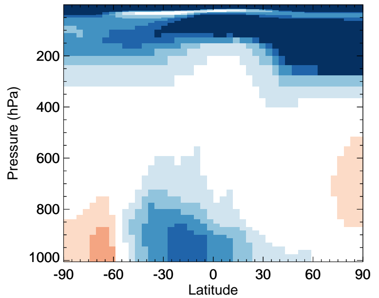
v11-02c / v11-01-public-Run0 SO4 - Zonal mean % diff for Jul
