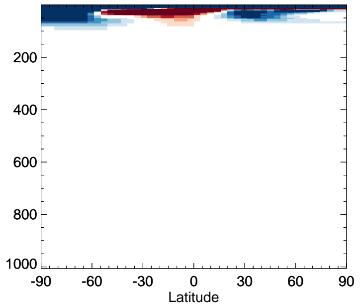
v11-02c / v11-02a OCS - Zonal mean % diff for Jul
