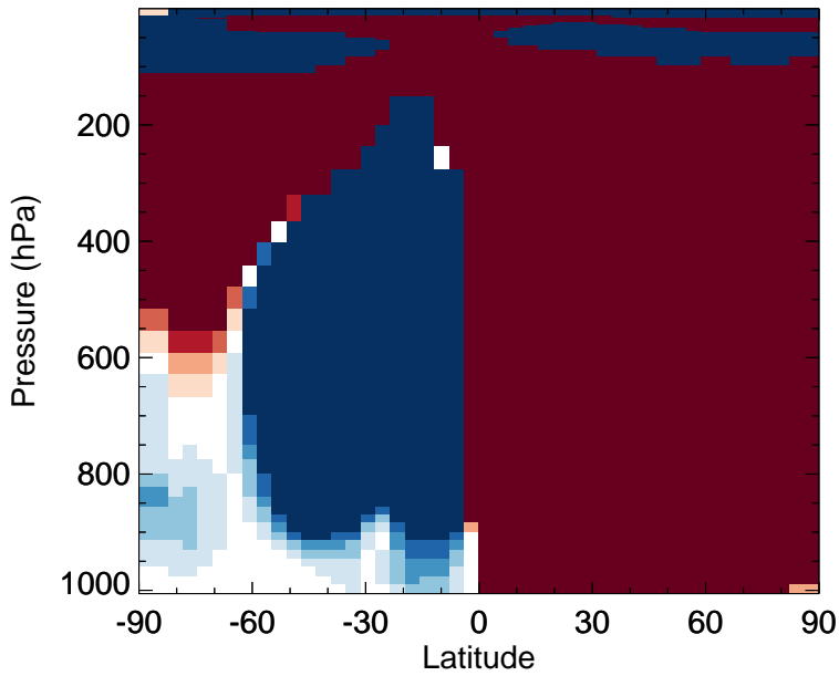
v11-02c - v11-01-public-Run0 CH4 - Zonal mean abs diff for Jul
