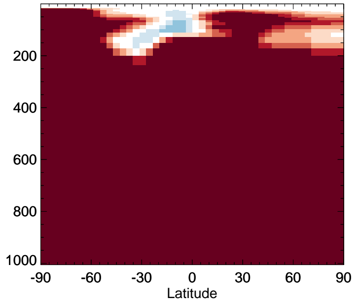
v11-02c / v11-02a HCl - Zonal mean % diff for Jul
