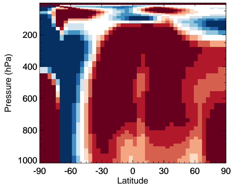
v11-02c / v11-02a CIOO - Zonal mean % diff for Jul
