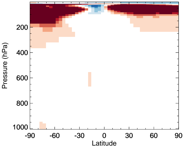
v11-02c - v11-02a HCl - Zonal mean abs diff for Jul
