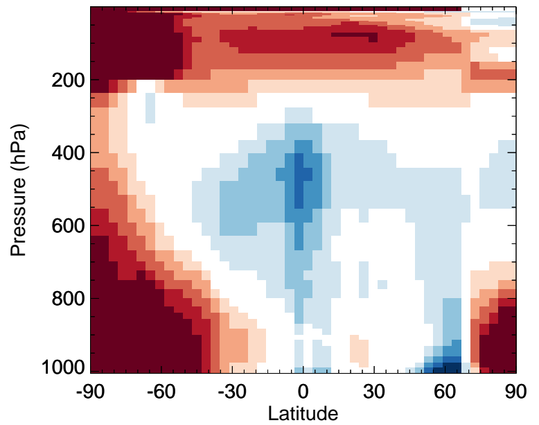
v11-02c / v11-01-public-Run0 NO3 - Zonal mean % diff for Jul
