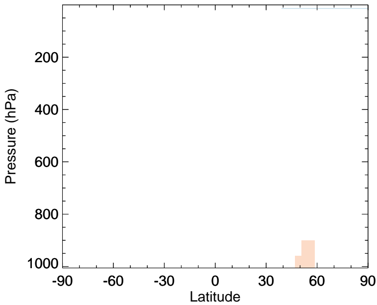
v11-02c - v11-01-public-Run0 CO - Zonal mean abs diff for Jul
