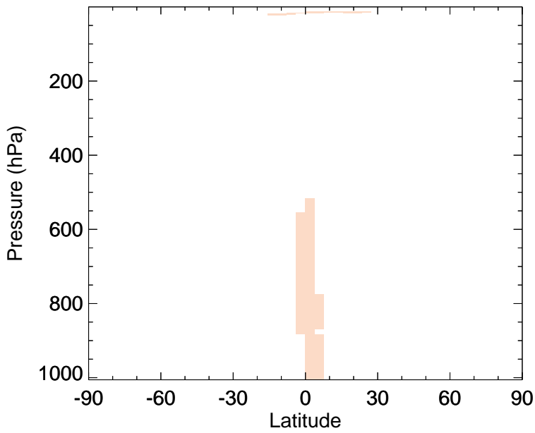
v11-02c - v11-02a CO - Zonal mean abs diff for Jul
