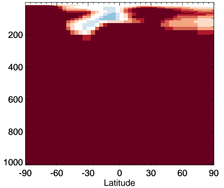
v11-02c / v11-01-public-Run0 HCl - Zonal mean % diff for Jul
