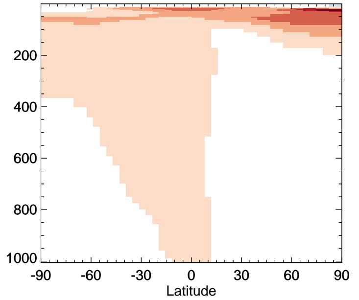
v11-02c / v11-01-public-Run0 C2H6 - Zonal mean % diff for Jul
