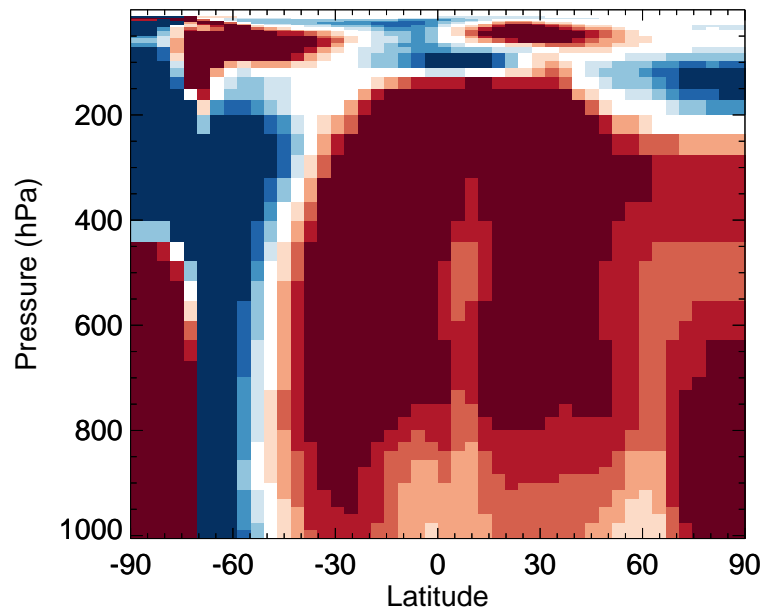
v11-02c / v11-02a Cl - Zonal mean % diff for Jul
