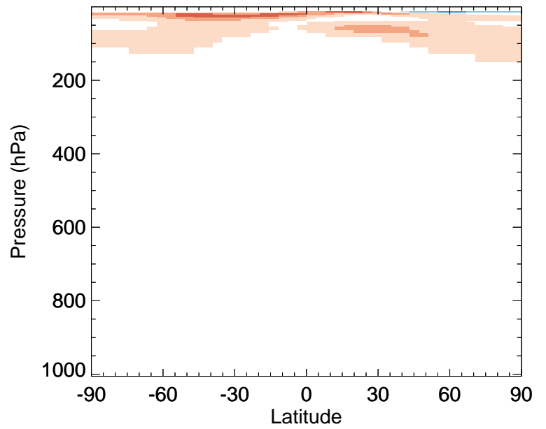
v11-02c / v11-02a CO - Zonal mean % diff for Jul
