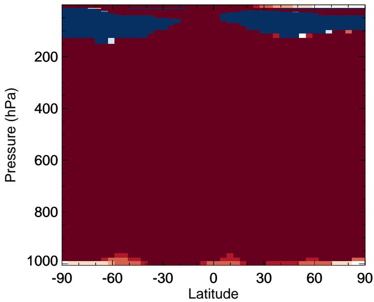
v11-02c - v11-01-public-Run0 N2O - Zonal mean abs diff for Jul
