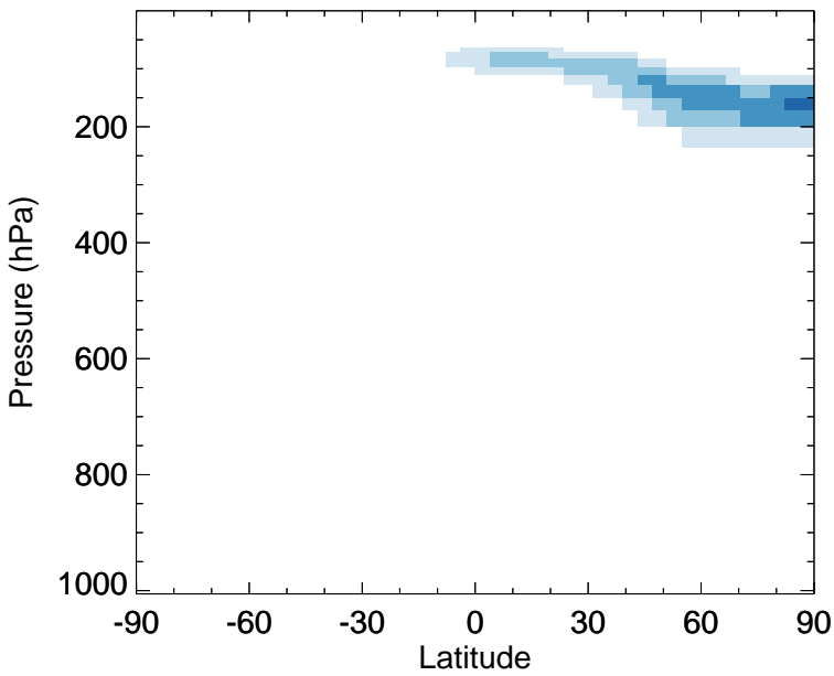
v11-02c - v11-01-public-Run0 SO4 - Zonal mean abs diff for Jul
