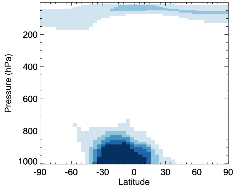
v11-02c / v11-01-public-Run0 NH4 - Zonal mean % diff for Jul
