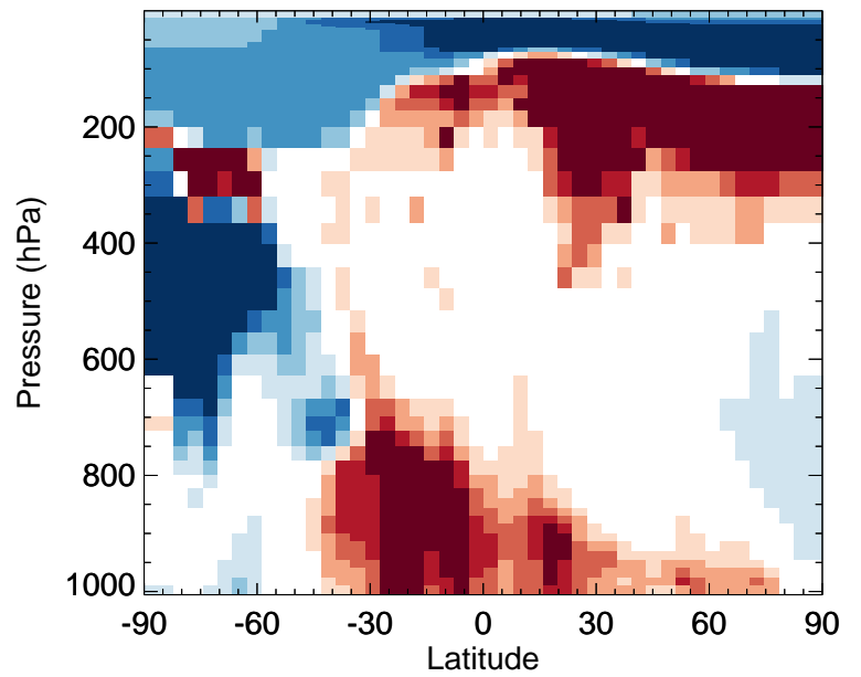
v11-02c / v11-01-public-Run0 NH3 - Zonal mean % diff for Jul
