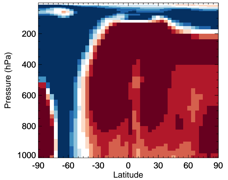
v11-02c / v11-02a ClO - Zonal mean % diff for Jul
