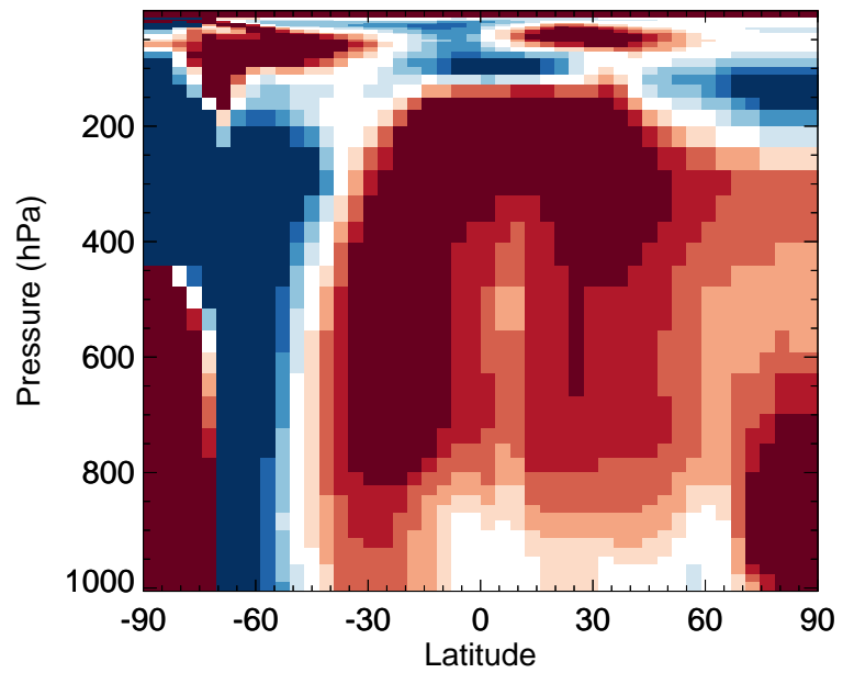
v11-02c / v11-01-public-Run0 CIOO - Zonal mean % diff for Jul
