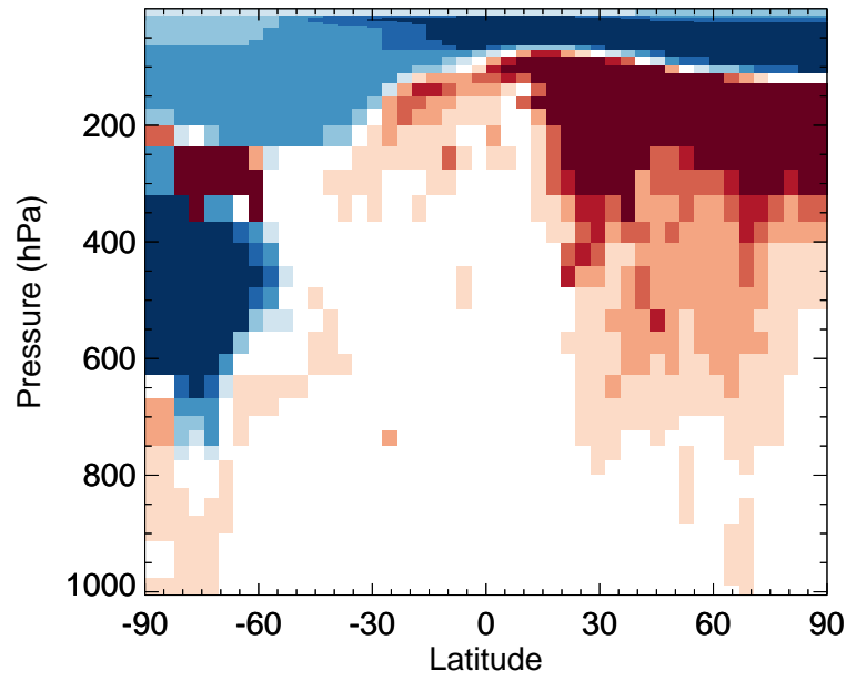
v11-02c / v11-02a NH3 - Zonal mean % diff for Jul
