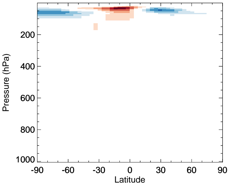
v11-02c - v11-02a OCS - Zonal mean abs diff for Jul
