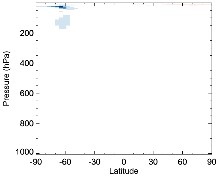
v11-02c - v11-02a ClO - Zonal mean abs diff for Jul
