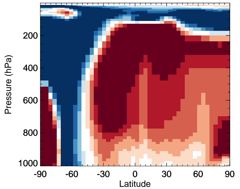
v11-02c / v11-01-public-Run0 ClO - Zonal mean % diff for Jul
