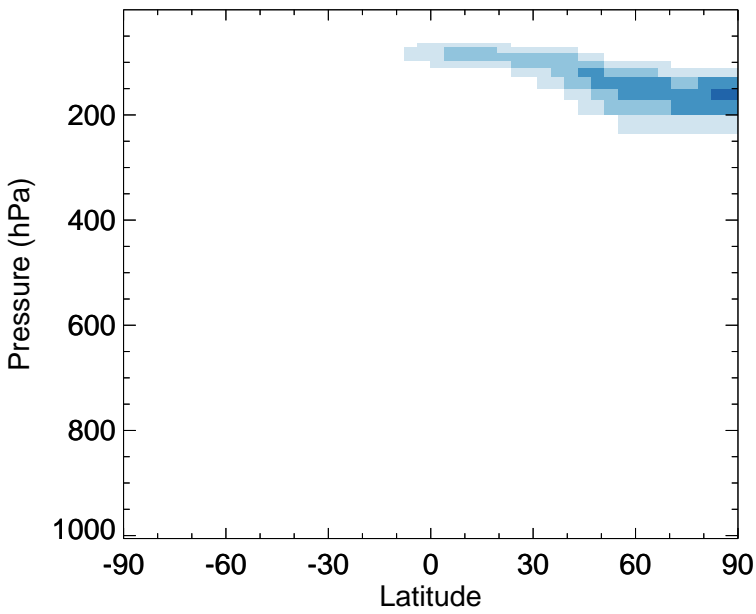
v11-02c - v11-02a SO4 - Zonal mean abs diff for Jul
