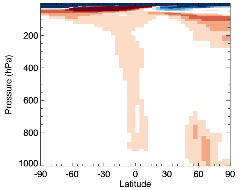
v11-02c / v11-02a SO 2 - Zonal mean % diff for Jul
