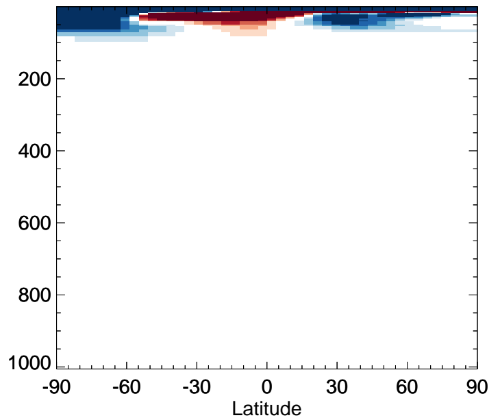
v11-02c / v11-01-public-Run0 OCS - Zonal mean % diff for Jul
