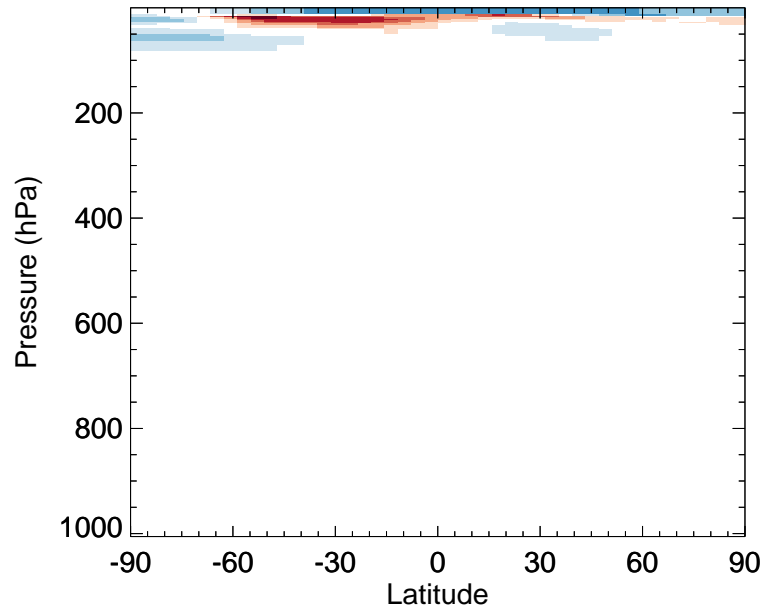
v11-02c / v11-02a CH4 - Zonal mean % diff for Jul
