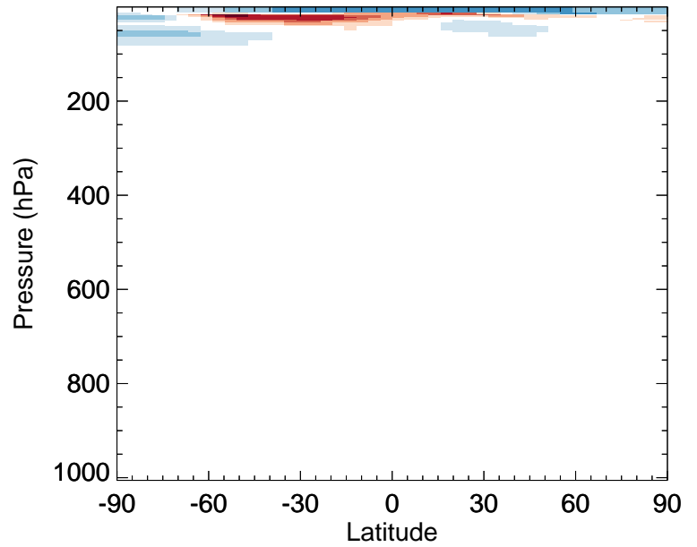
v11-02c / v11-01-public-Run0 CH4 - Zonal mean % diff for Jul
