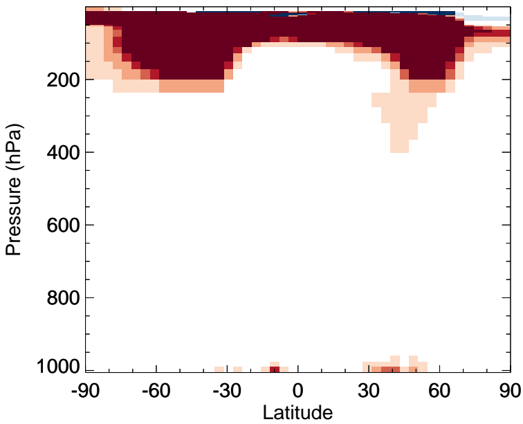
v11-02c - v11-01-public-Run0 N2O5 - Zonal mean abs diff for Jul
