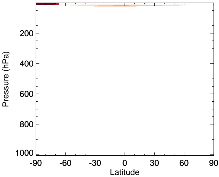
v11-02c - v11-01-public-Run0 NO3 - Zonal mean abs diff for Jul
