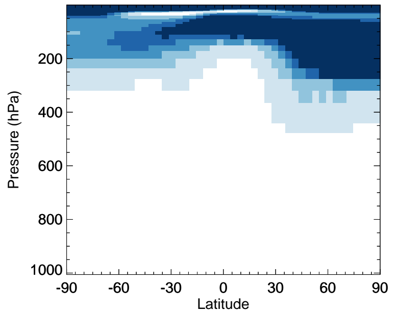
v11-02c / v11-02a SO4 - Zonal mean % diff for Jul
