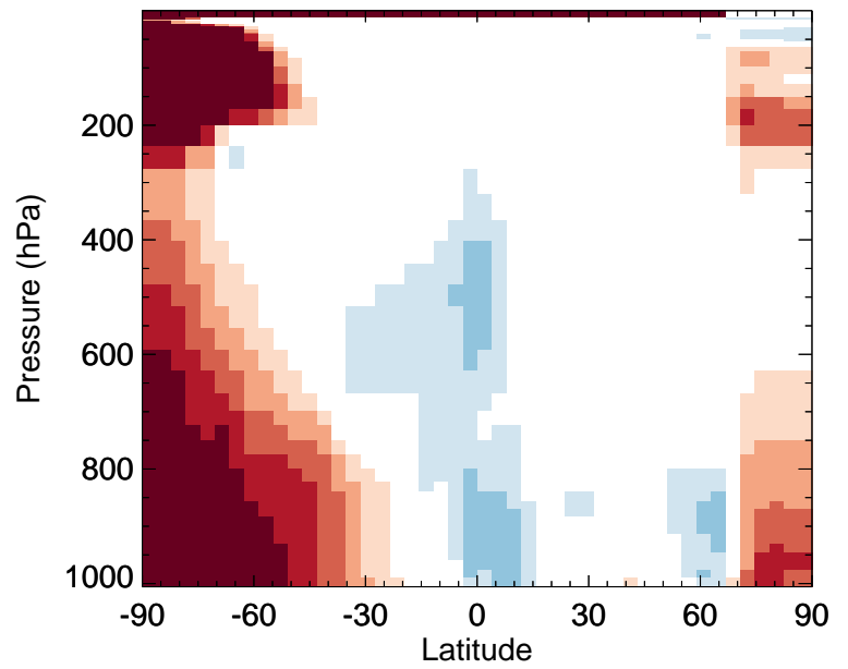
v11-02c / v11-02a NO3 - Zonal mean % diff for Jul
