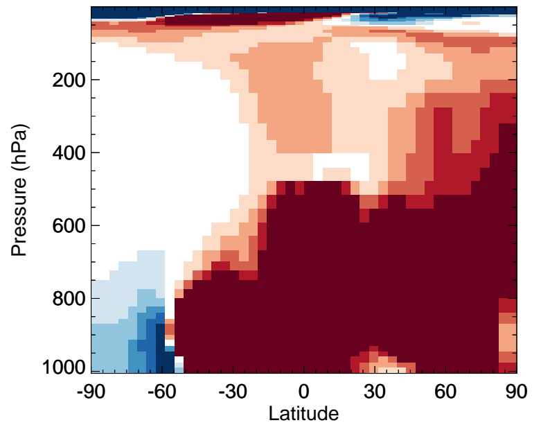
v11-02c / v11-01-public-Run0 SO 2 - Zonal mean % diff for Jul
