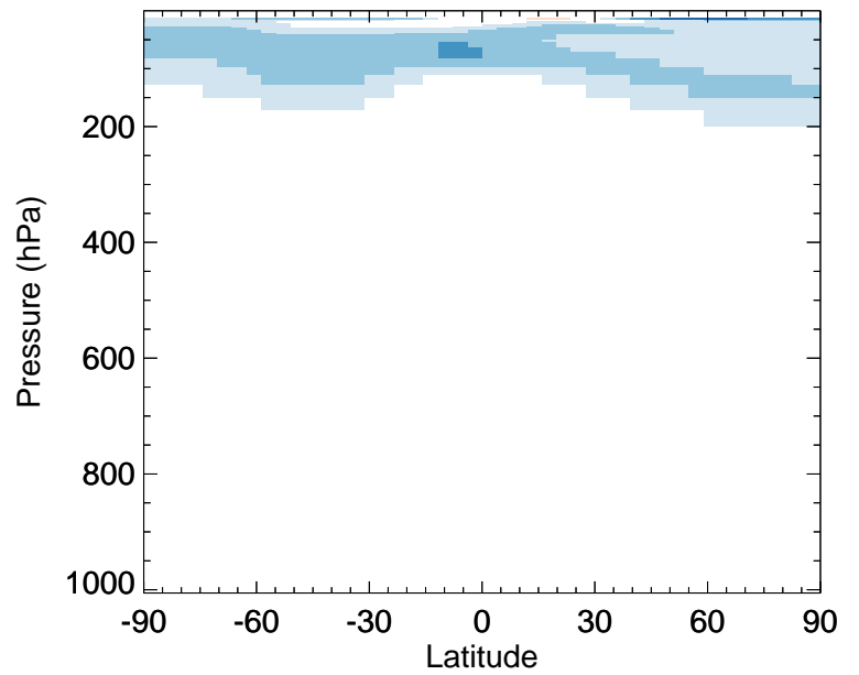
v11-02c / v11-01-public-Run0 CO - Zonal mean % diff for Jul
