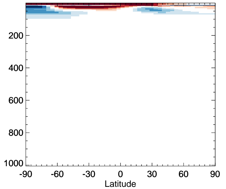
v11-02c / v11-01-public-Run0 N2O - Zonal mean % diff for Jul
