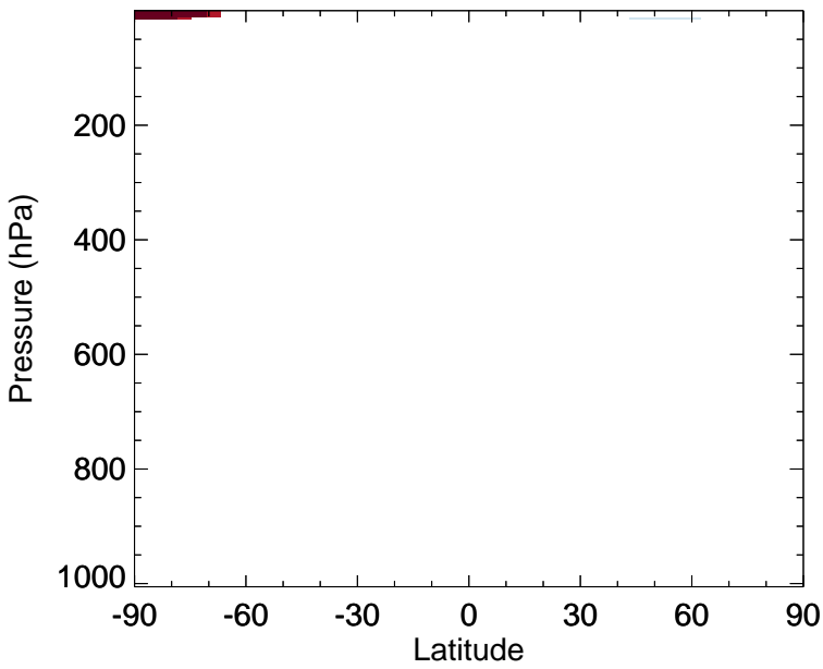
v11-02c - v11-02a NO3 - Zonal mean abs diff for Jul
