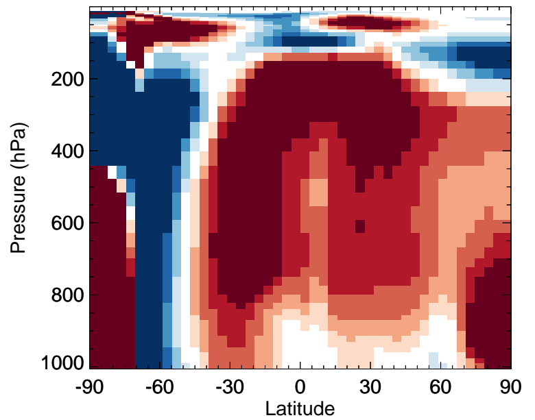
v11-02c / v11-01-public-Run0 Cl - Zonal mean % diff for Jul
